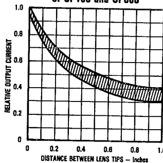
Coupling Characteristics of OP130 and OP800
