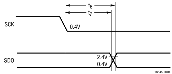
t_6 (Delay Time, \text{SCK} \square to SDO Valid) t_7 (Time from Previous Data Remains Valid After \text{SCK} \square )
