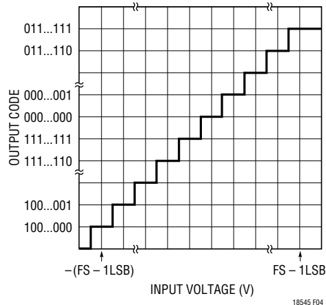
Figure 4. Bipolar Transfer Characteristics
