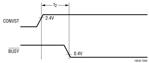
t_2 (CONVST to \overline{\text{BUSY}} Delay)
