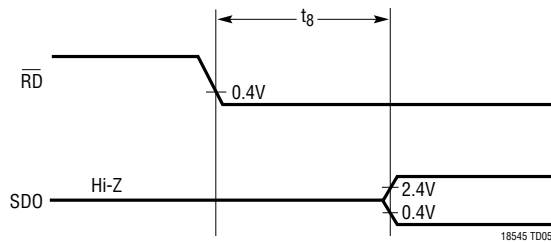
t_8 (SDO Valid After \overline{\text{RD}} \square )
