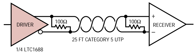
Figure 12. 100Mbps Differential Data Connection
