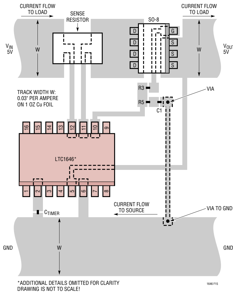
Figure 15. Recommended Layout for Power MOSFET, Sense Resistor, and Gate Components
