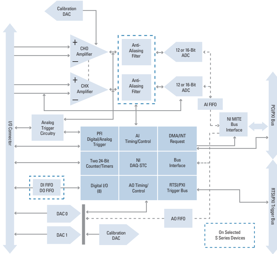
Figure 1. S Series Hardware Block Diagram
