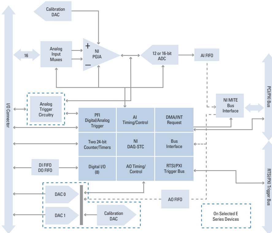
Figure 2. E Series Hardware Block Diagram
