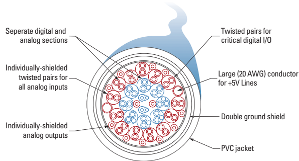
Figure 1. SH68-68-EP Cable
