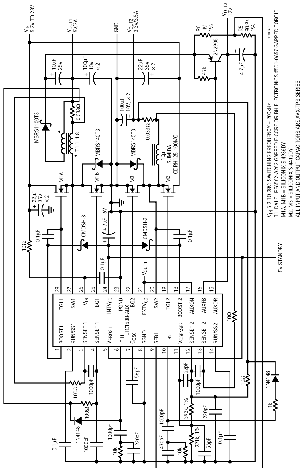
LTC1538-AUX 5V/3A, 3.3V/3.5A, 12V/0.2A Regulator
