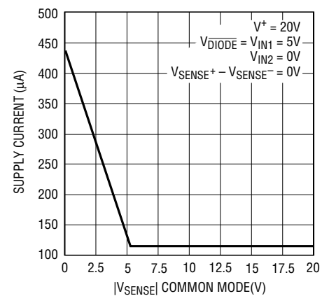
DC Supply Current vs V_{\text{SENSE}}
