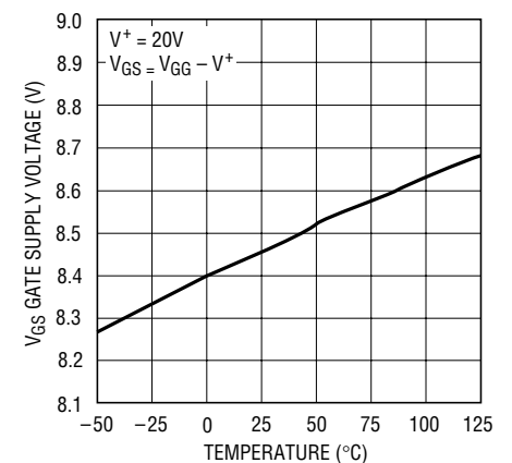
V_{\text{GS}} Gate Supply Voltage vs Temperature
