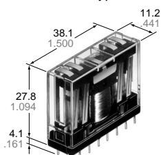
4C Vertical type (PC board)
