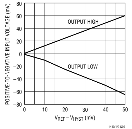
LTC1440/LTC1442 Hysteresis Control
