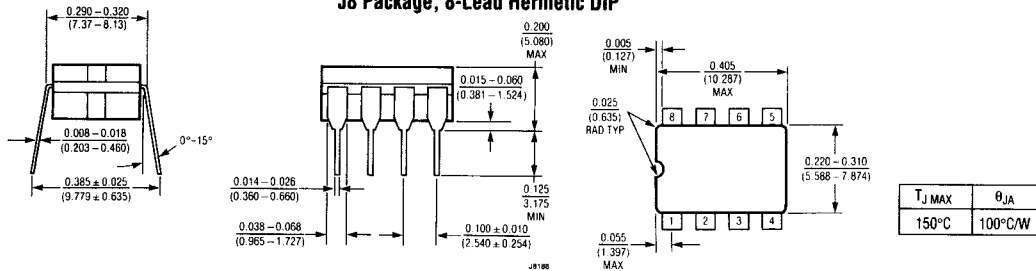
N8 Package, 8-Lead Plastic DIP
