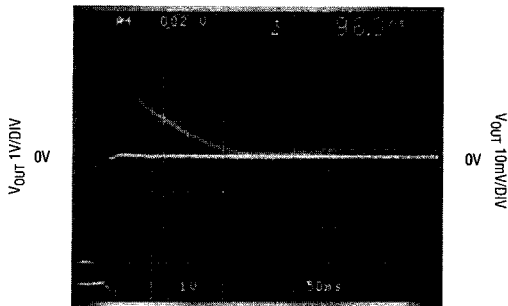
SETTLING TIME TO 10mV, A_V = 2 SUPPLY BYPASS CAPACITORS = 0.1\mu\text{F} + 4.7\mu\text{F} TANTALUM LT1193 - TA06
