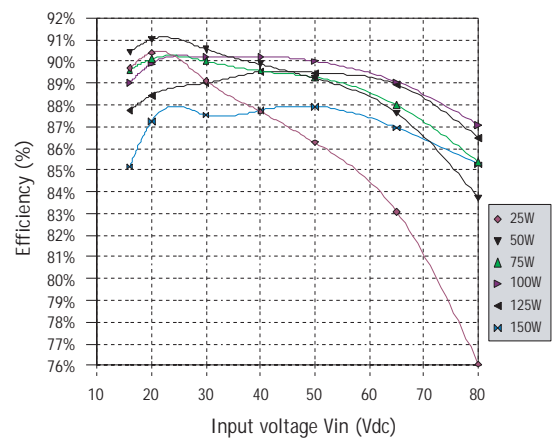
Typical efficiency MGDS-150-0-F at 25°C
