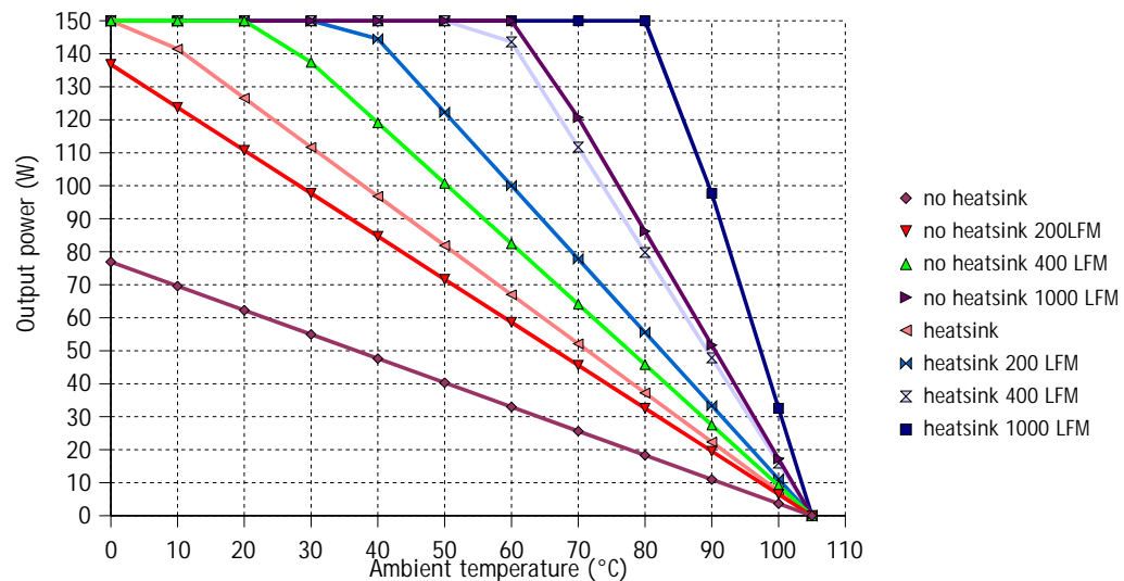
MGDS-150-O-x Series Thermal Curves
