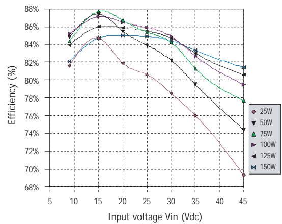
Typical efficiency MGDS-150-H-J at 25°C
