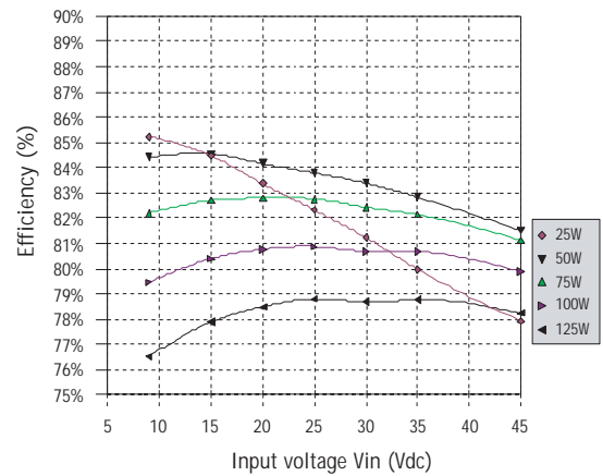
Typical efficiency MGDS-150-H-C at 25°C
