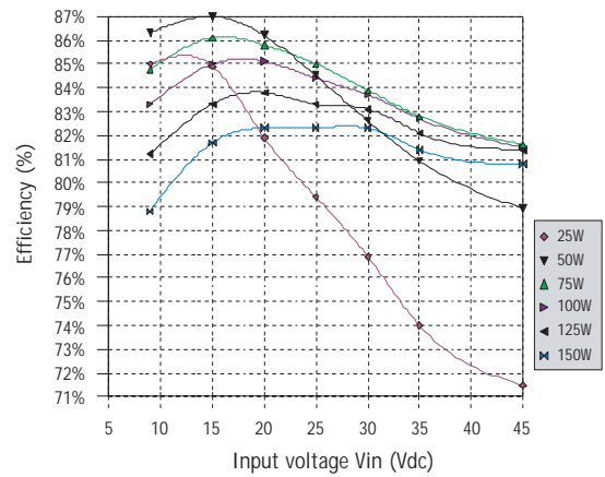
Typical efficiency MGDS-150-H-F at 25°C
