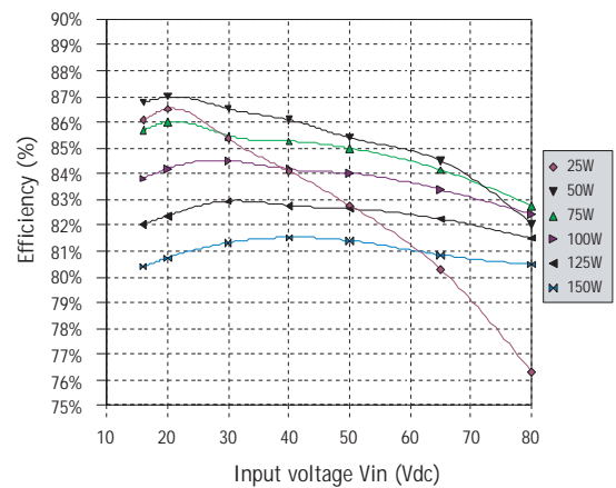
Typical efficiency MGDS-150-0-C at 25°C
