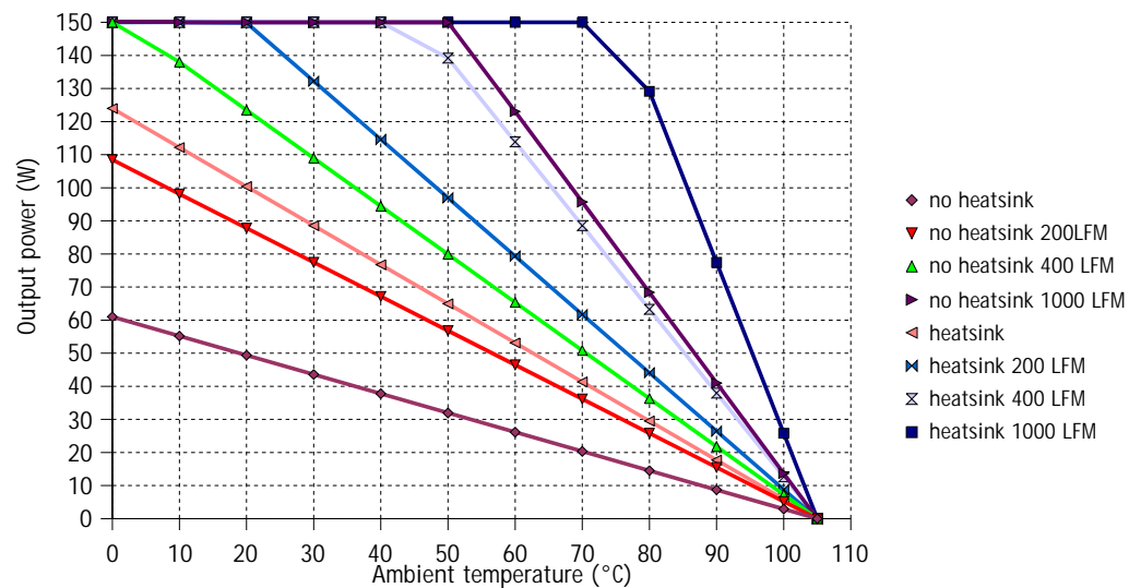
MGDS-150-H-x Series Thermal Curves
