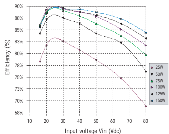
Typical efficiency MGDS-150-0-J at 25°C
