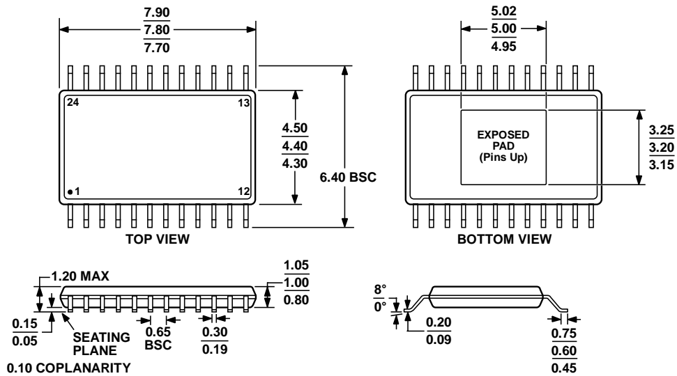
Figure 69. 24-Lead Thin Shrink Small Outline Package, Exposed Pad [TSSOP_EP] (RE-24) Dimensions shown in millimeters
