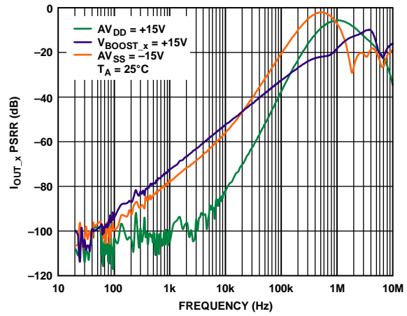
Figure 52. I_{OUT,x} PSRR vs. Frequency
