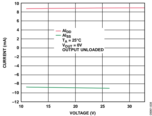
Figure 65. Supply Current (A DD /A SS ) vs. Supply Voltage (A VDD /A VSS )
