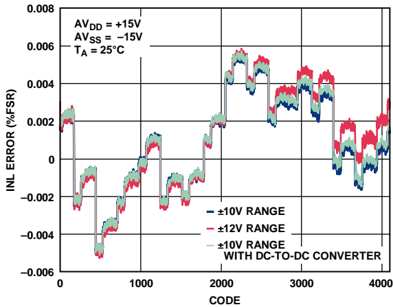
Figure 8. Integral Nonlinearity Error vs. DAC Code
