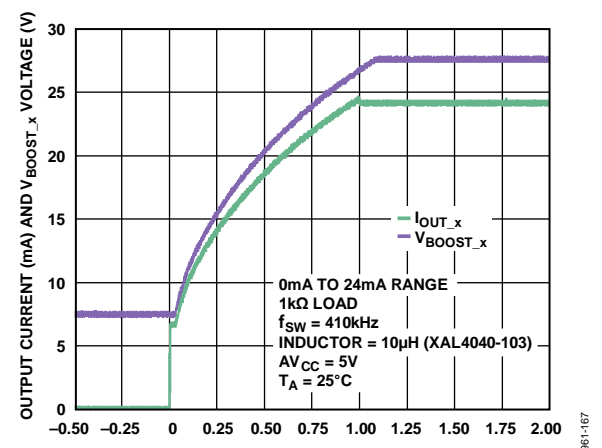
Figure 47. Output Current and V_{BOOST\_x} Settling Time with DC-to-DC Converter (See Figure 77)
