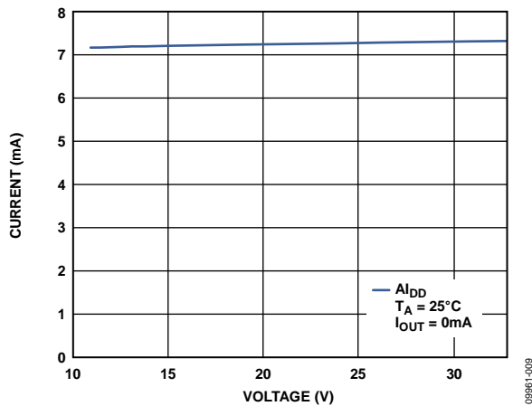
Figure 66. Supply Current (A DD ) vs. Supply Voltage (A VDD )
