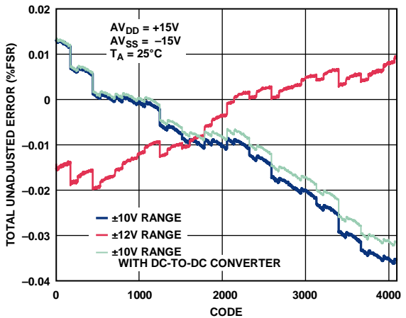
Figure 10. Total Unadjusted Error vs. DAC Code
