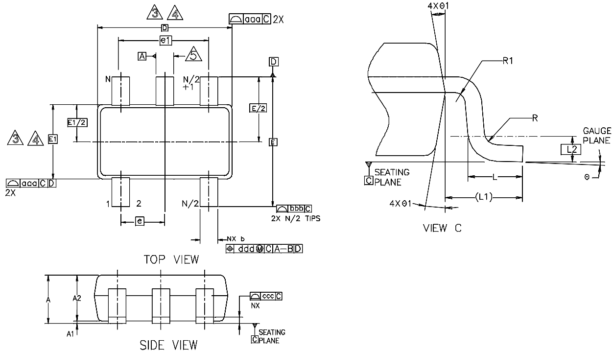
Figure 13. TSOT23-5 Package
