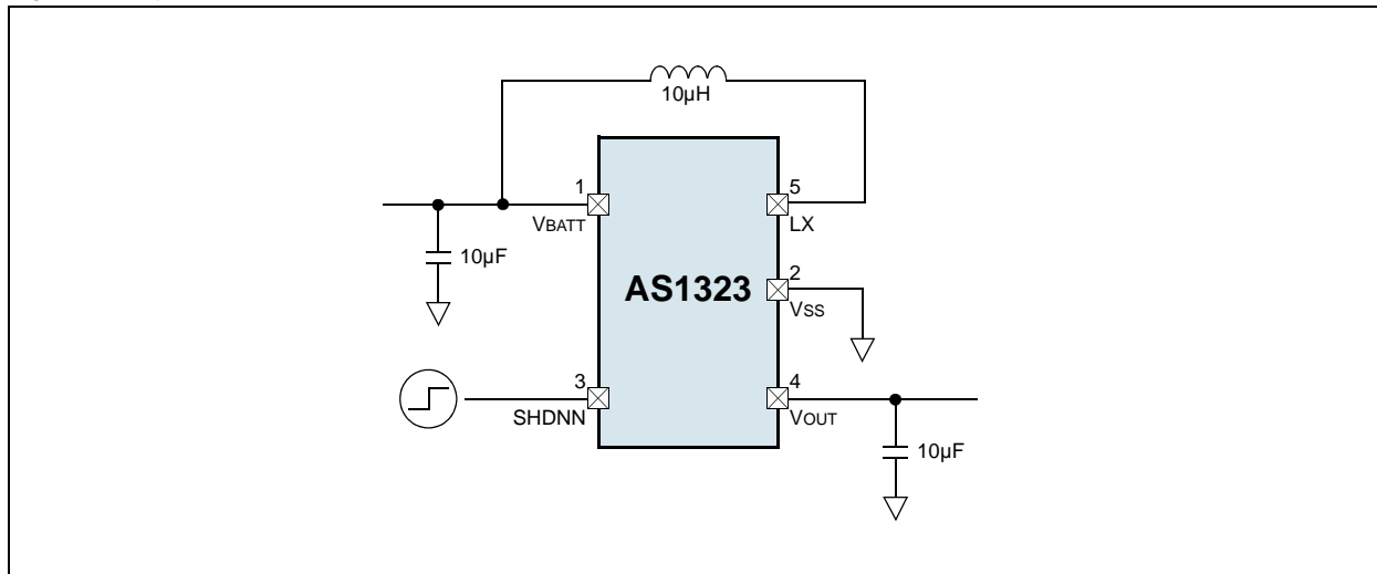
Figure 12. Typical Application
