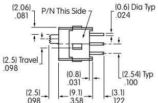
Actuator shown in LEFT position
