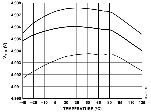
Figure 5. ADR365 Output Voltage vs. Temperature
