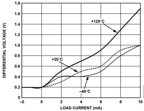
Figure 14. ADR365 Minimum Input Voltage vs. Load Current
