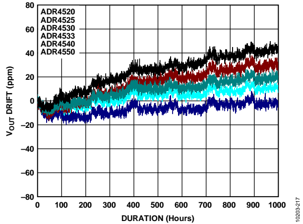
Figure 32. ADR4525 Typical Long-Term Output Voltage Drift (1000 Hours)
