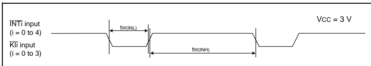
Figure 5.15 Input Timing Diagram for External Interrupt \overline{INT}_i and Key Input Interrupt \overline{K}_i when Vcc = 3 V
