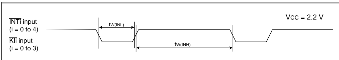
Figure 5.19 Input Timing Diagram for External Interrupt \overline{INT}_i and Key Input Interrupt \overline{K}_i when Vcc = 2.2 V
