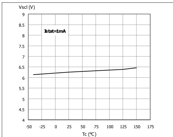
Figure 17. Status clamp voltage
