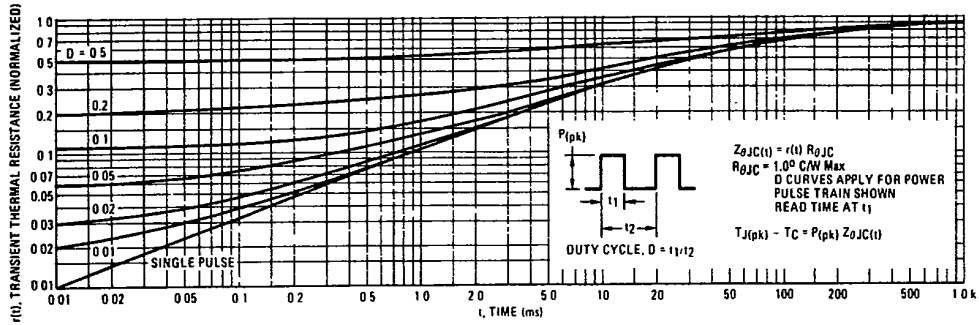
FIGURE 15 - THERMAL RESPONSE
