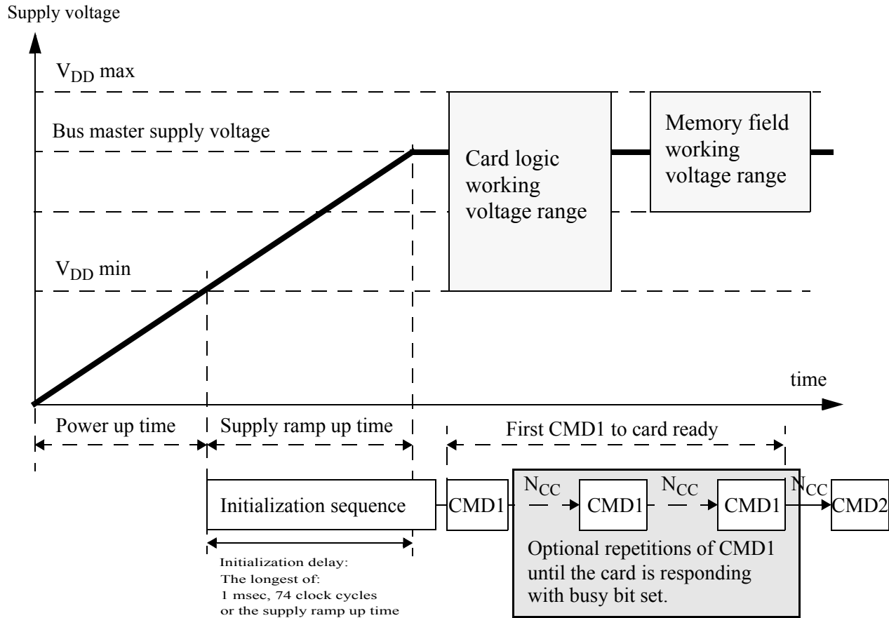
Figure 5-3 : Power-up Diagram
