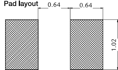
Pad layout
