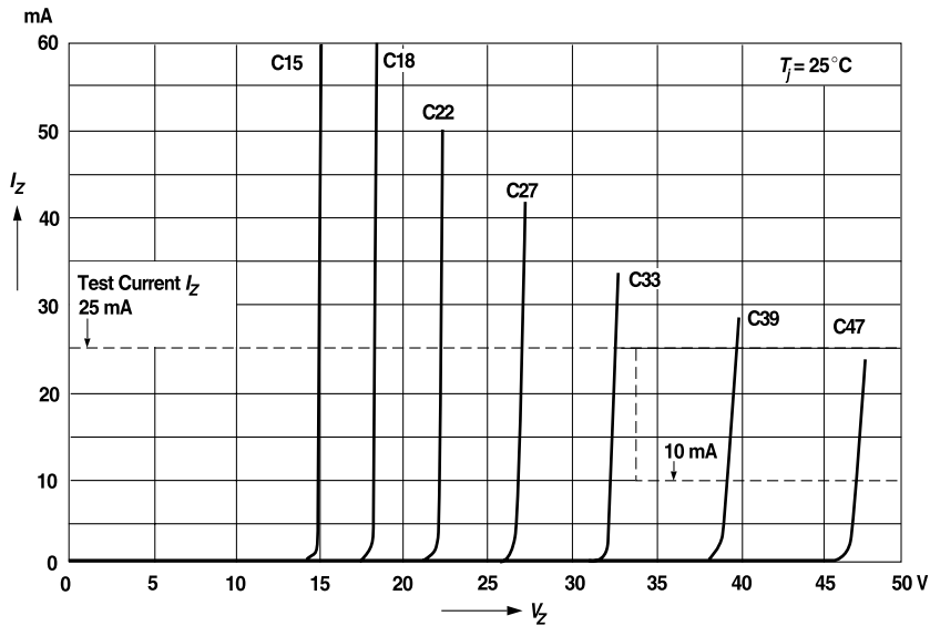
Figure 7. Breakdown Characteristics
