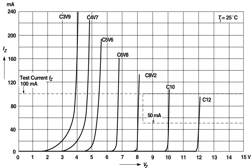
Figure 6. Breakdown Characteristics
