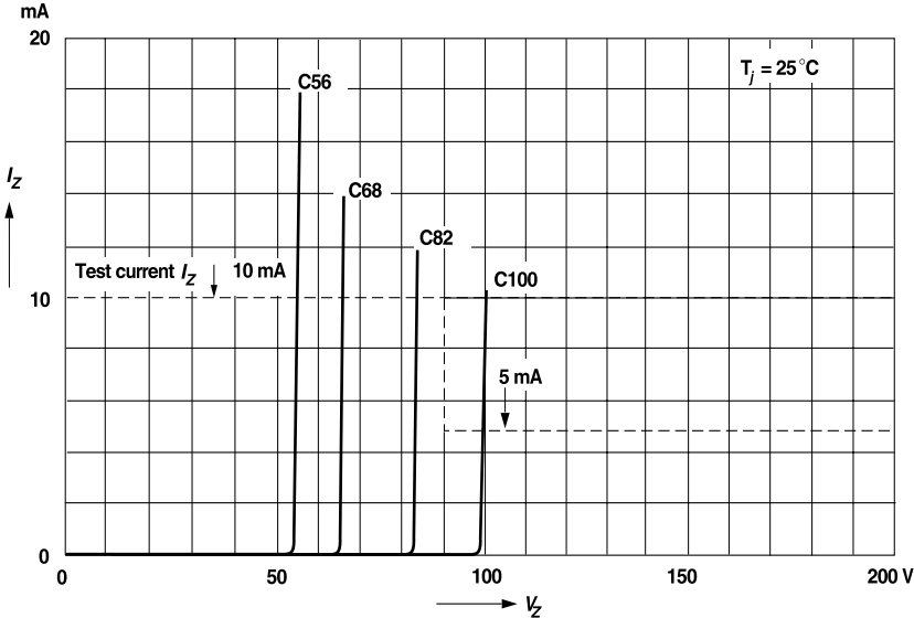
Figure 8. Breakdown Characteristics
