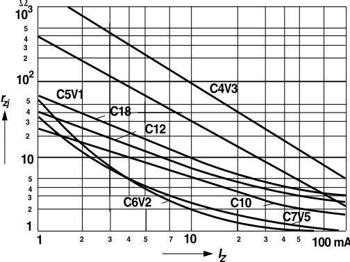
Figure 5. Dynamic Resistance vs. Zener Current
