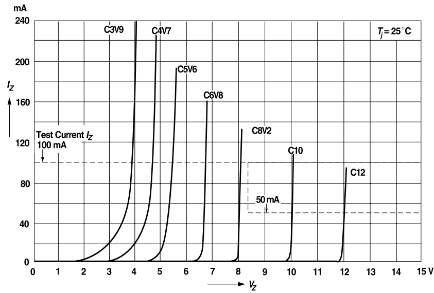
Figure 6. Breakdown Characteristics
