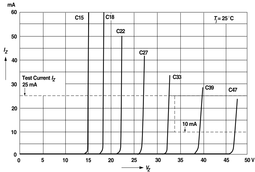
Figure 7. Breakdown Characteristics
