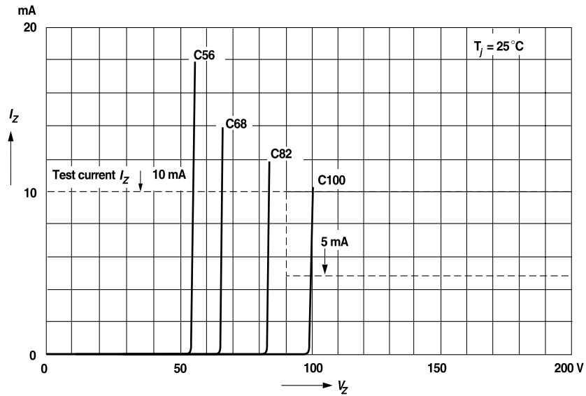
Figure 8. Breakdown Characteristics
