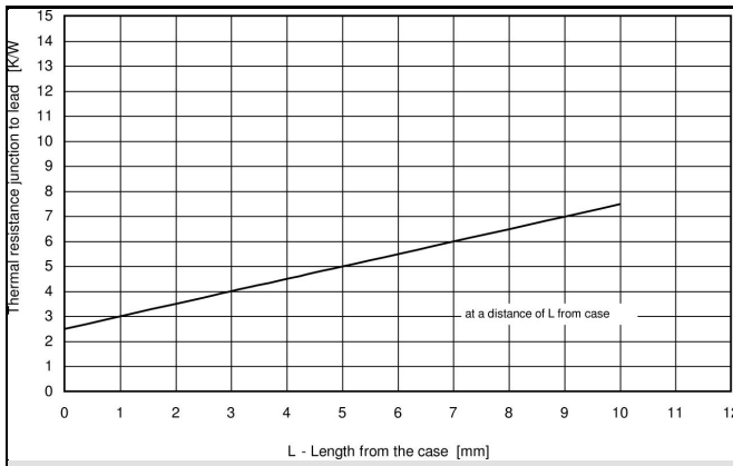
Fig. 3, Thermal resistance versus distance from case
