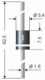
Axial lead diode
