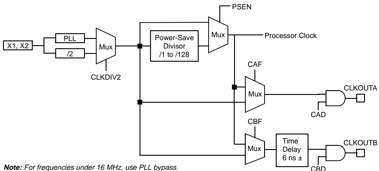
Figure 9. Clock Organization
