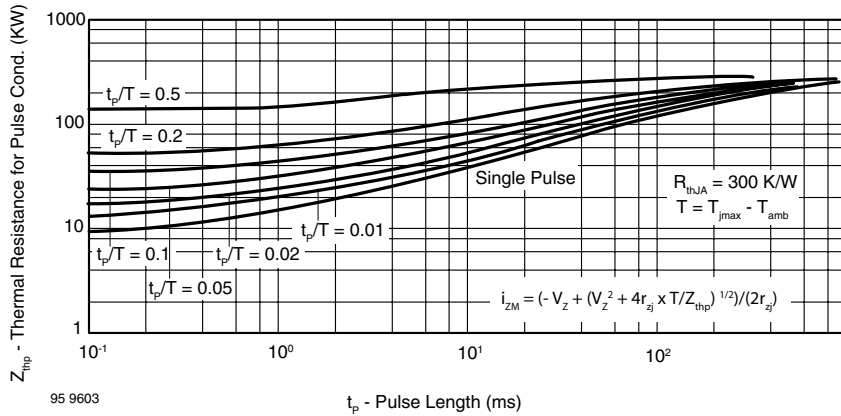
Figure 11. Thermal Response
