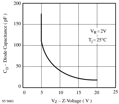
Diode Capacitance vs. Z-Voltage
