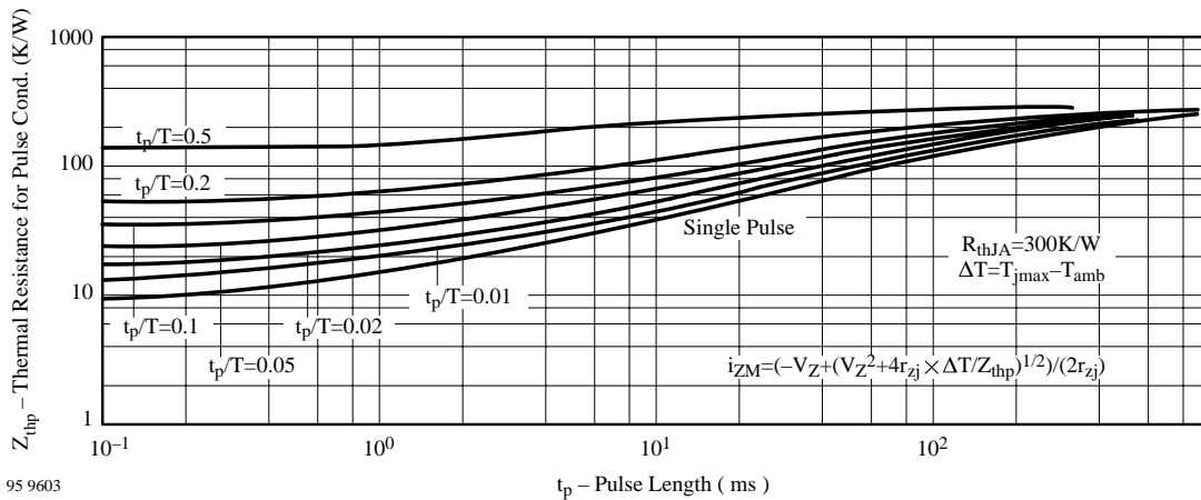
Thermal Response
