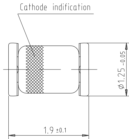
Glass case Micro MELF
