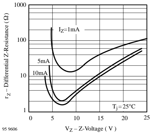
Differential Z-Resistance vs. Z-Voltage
