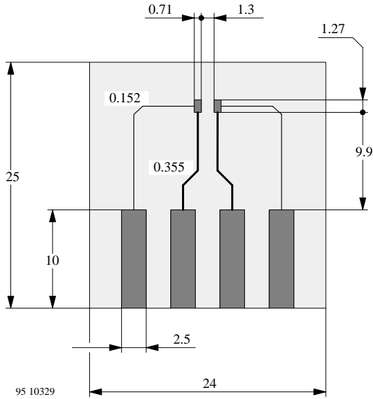
Board for R_{thJA} definition (in mm) Reflow Soldering
