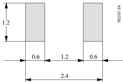
Recommended foot pads (in mm)
