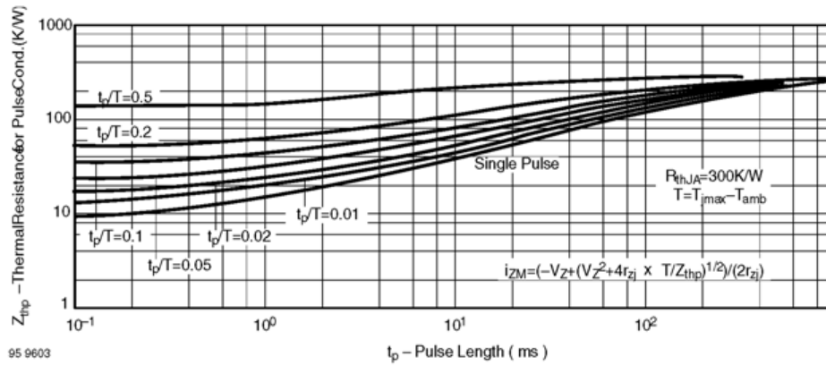
Fig. 13 Thermal Response
