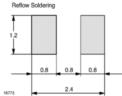
Fig. 11 Recommended foot pads (in mm)
