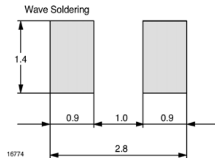
Fig. 12 Recommended foot pads (in mm)
