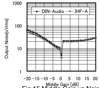
Fig.15 Middle Gain vs Noise
