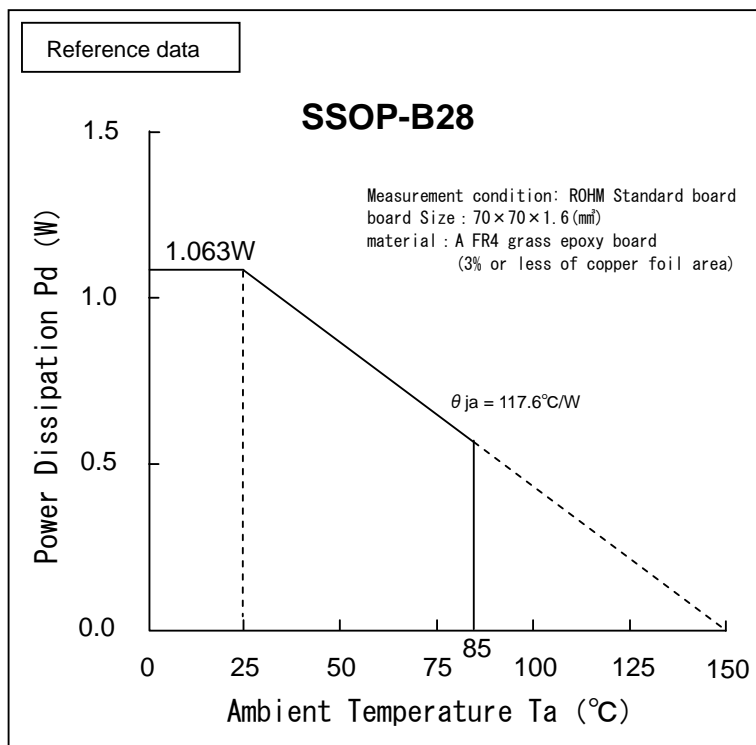
Fig.34 Temperature Derating Curve
