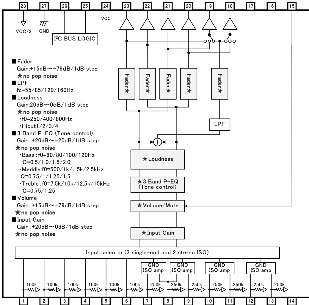
Fig.23 BD37532FV
