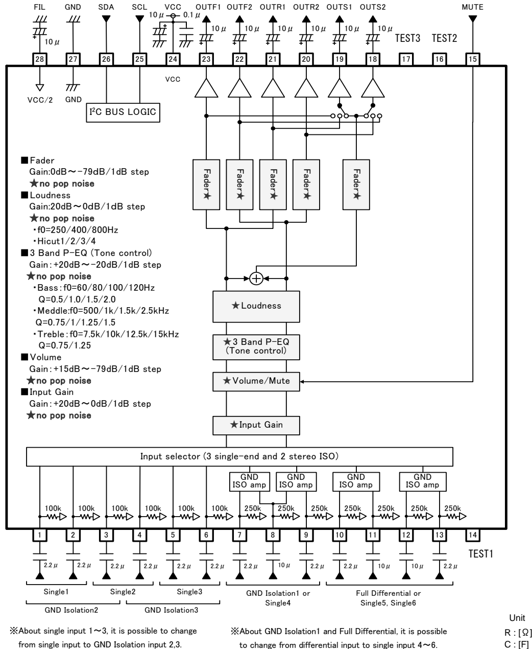
Fig. 28 BD37531FV
