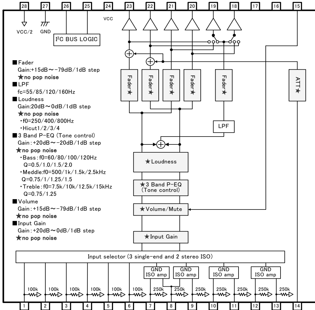
Fig.24 BD37533FV
