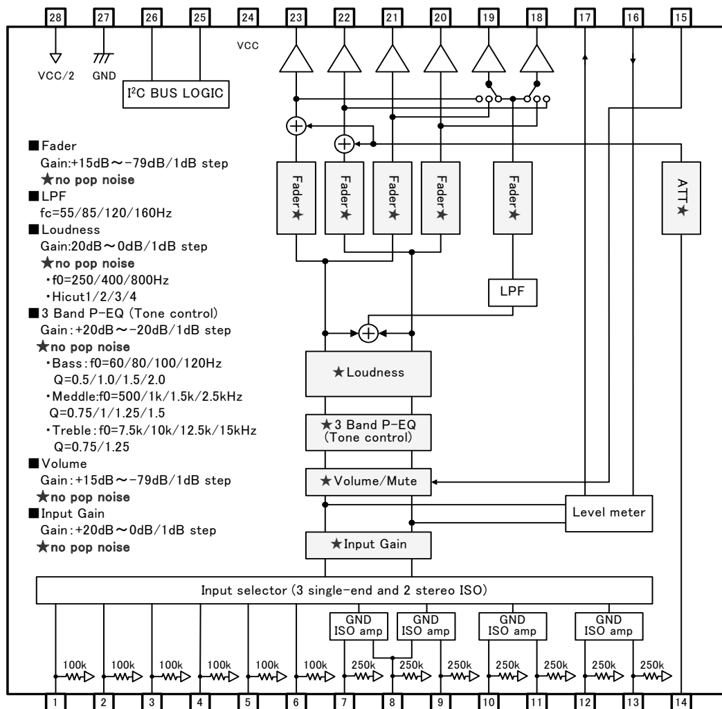
Fig.25 BD37534FV
