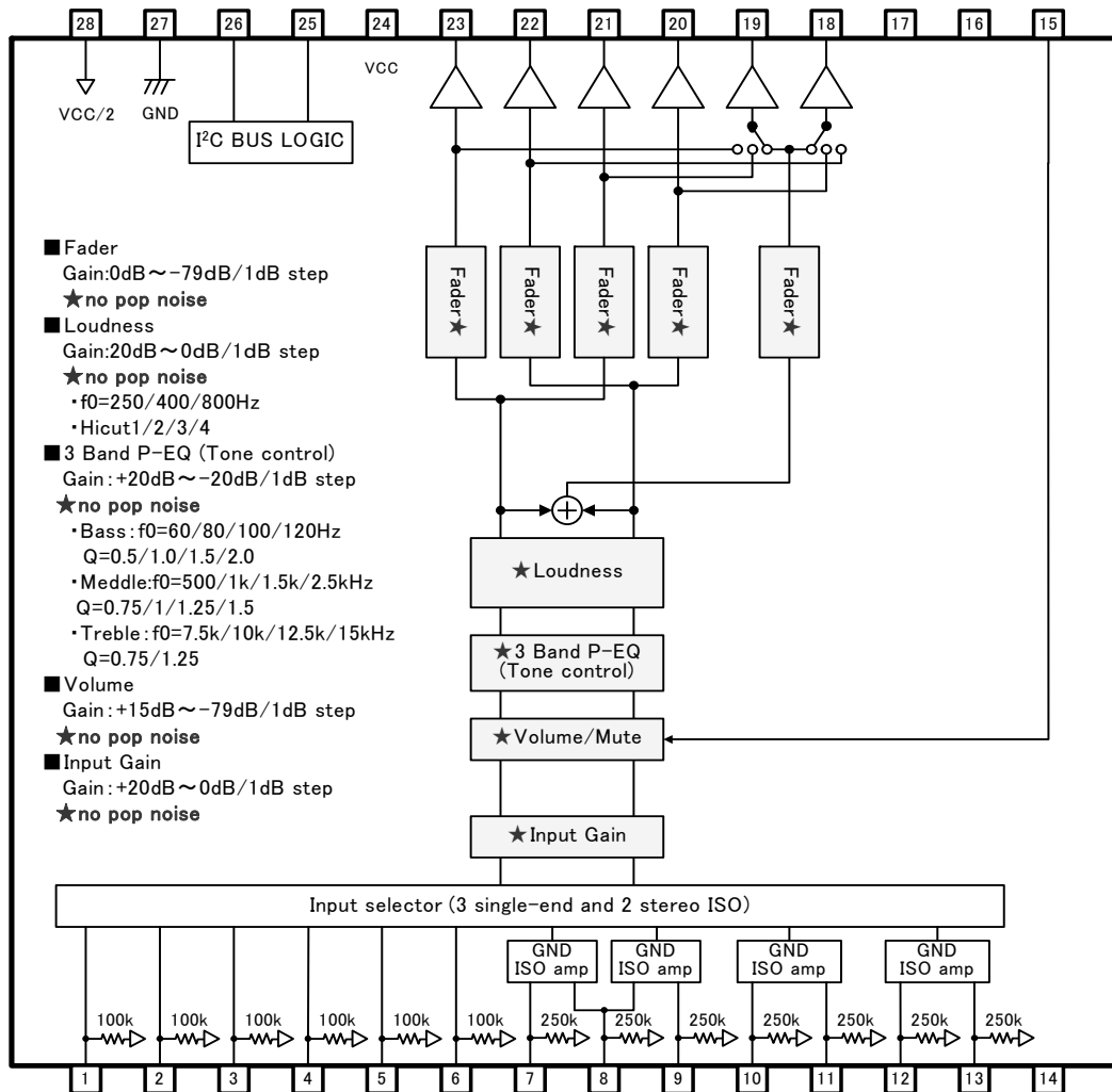
Fig.22 BD37531FV
