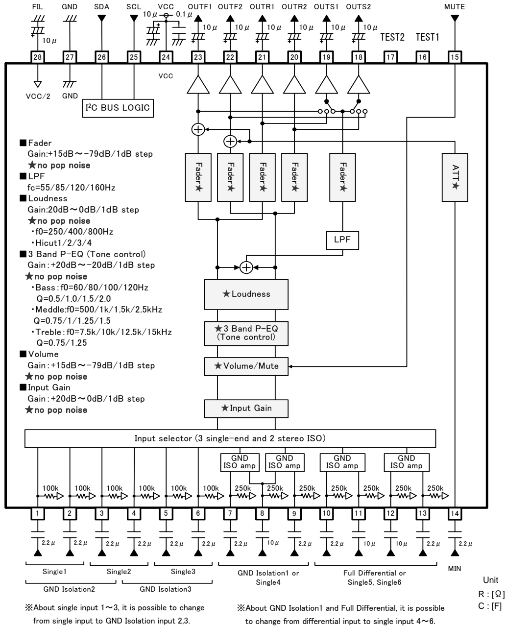
Fig. 30 BD37533FV
