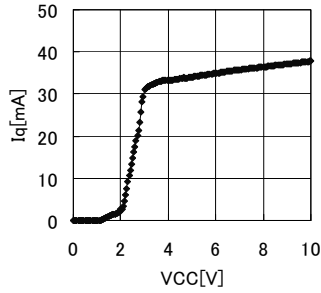
Fig.1 Iq vs Vcc
