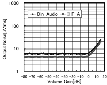
Fig.13 Volume Gain vs Noise
