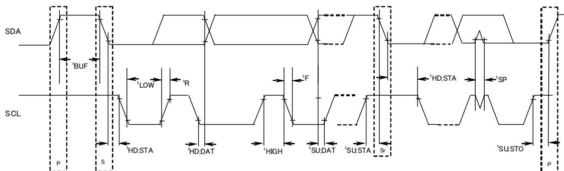
Fig.26 Definition of timing on the I 2 C-bus
