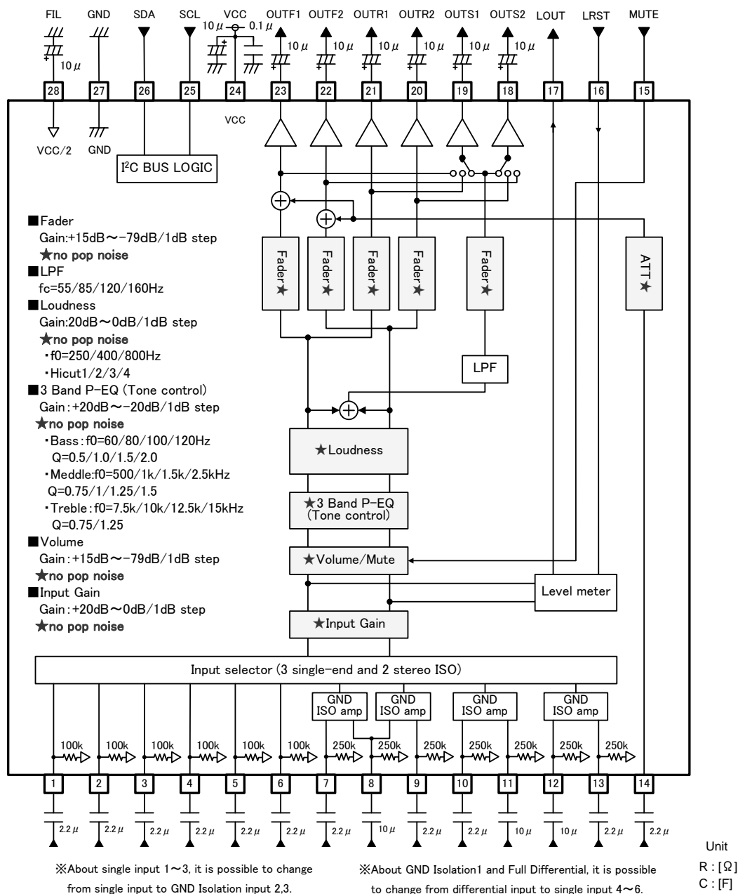
Fig. 31 BD37534FV
