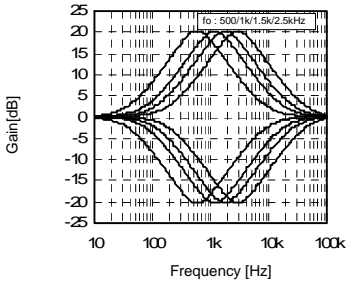
Fig.8 Middle fo vs Freq
