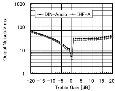
Fig.16 Treble Gain vs Noise
