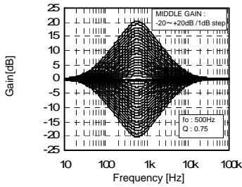
Fig.7 Middle Gain vs Freq
