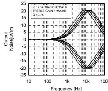
Fig.11 Treble fo vs Freq
