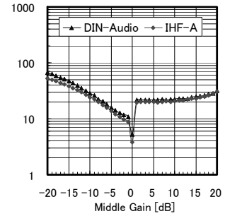
Fig.15 Middle Gain vs Noise
