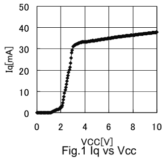
Fig.1 Iq vs Vcc
