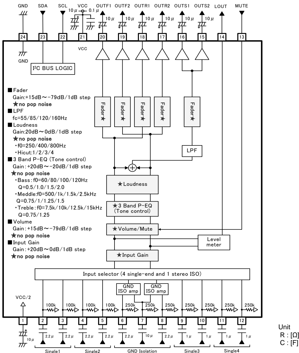
Fig. 25 Application Circuit Diagram
