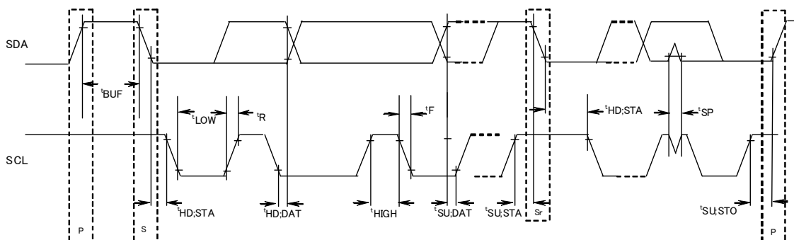
Fig.23 Definition of timing on the I 2 C-bus
