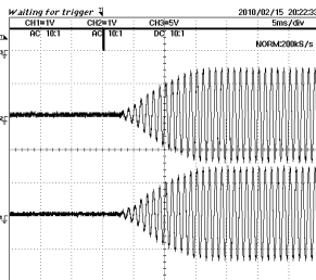
Fig.19 Advanced Switch 1
