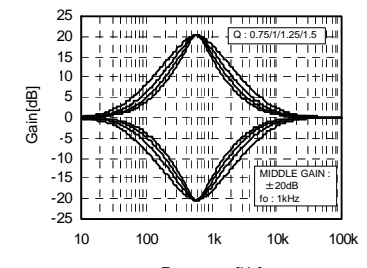
Fig.9 Middle Q vs Freq
