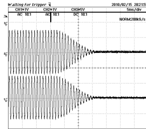
Fig.20 Advanced Switch 2
