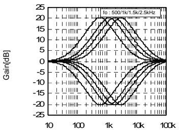
Fig.8 Middle fo vs Freq
