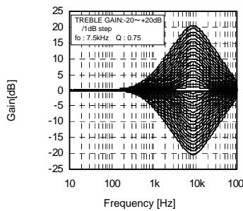
Fig.10 Treble Gain vs Freq
