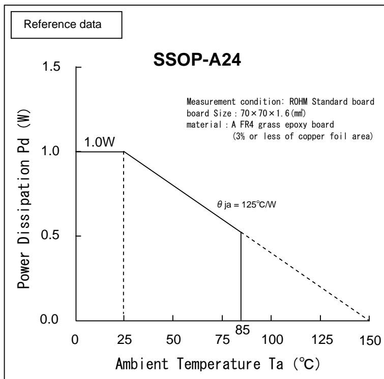
Fig.26 Temperature Derating Curve
