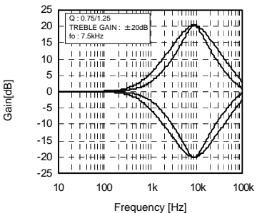
Fig.12 Treble Q vs Freq
