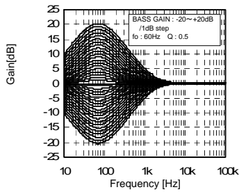
Fig.4 Bass Gain vs Freq
