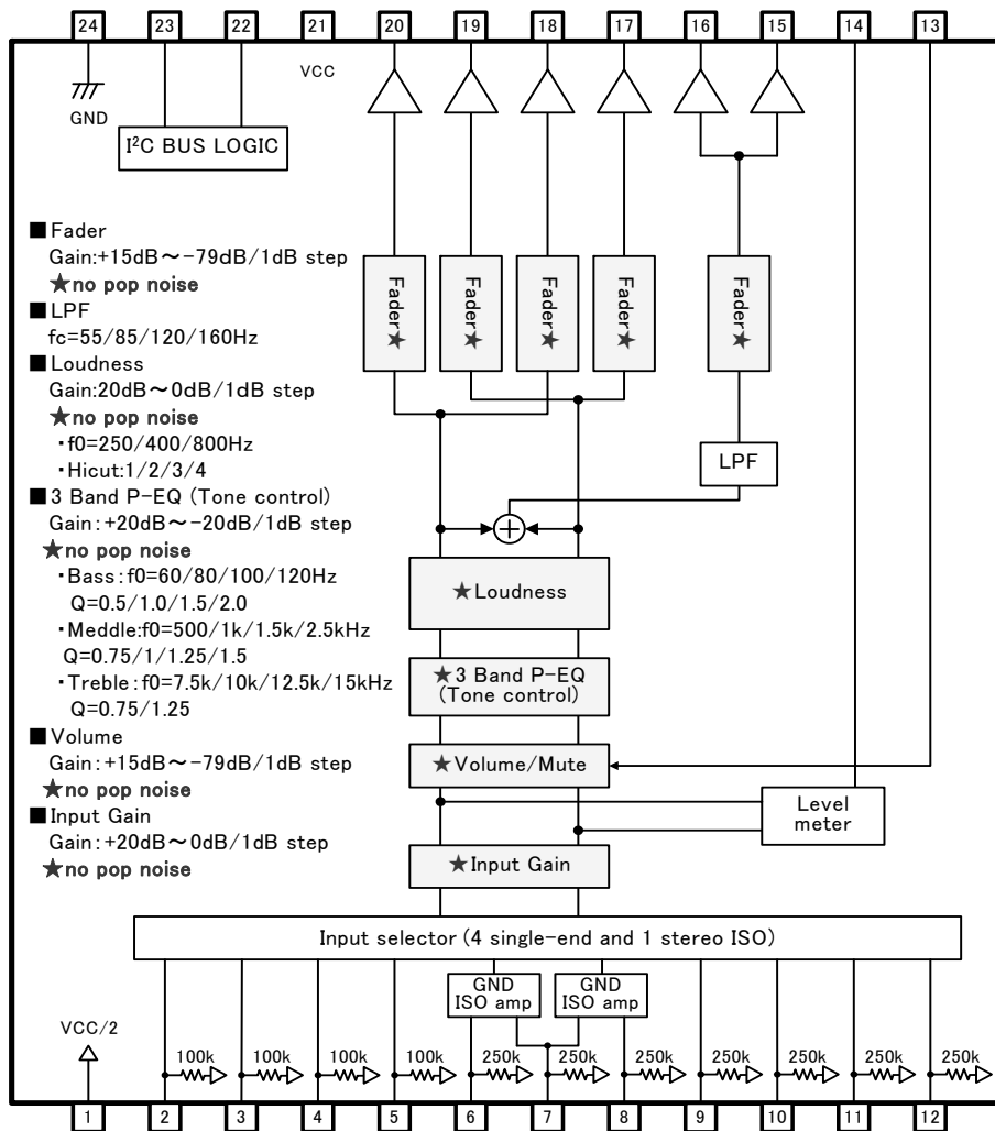
Fig.22 BD37524FS
