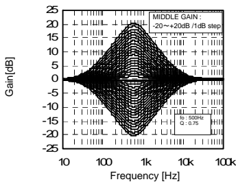
Fig.7 Middle Gain vs Freq
