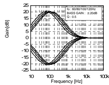
Fig.5 Bass fo vs Freq
