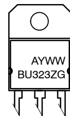
SOT-93 CASE 340D STYLE 1
