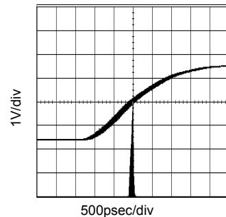
Fig.8 36MHz Period-Jitter (VDD=3.3V,CL=15pF,Ta=25°C)
