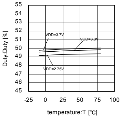
Fig.74 36MHz Duty temperature characteristics
