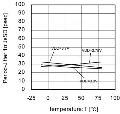
Fig.72 49.5MHz Period-Jitter 1 \sigma temperature characteristics
