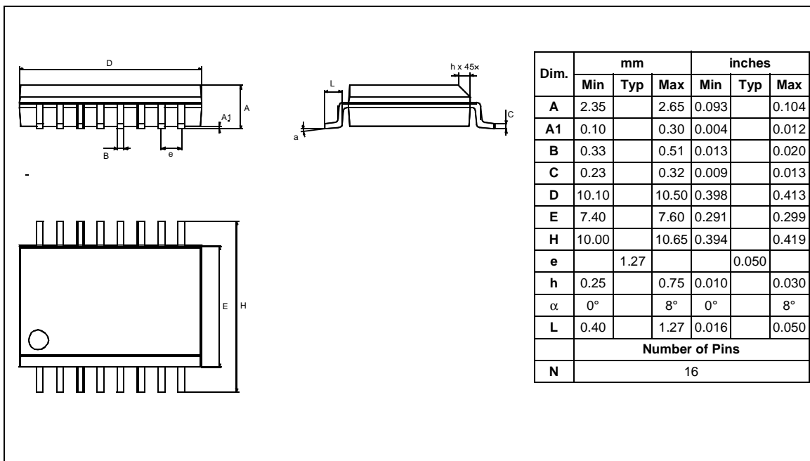
Figure 69. 16-Pin Plastic Small Outline Package, 300-mil Width
