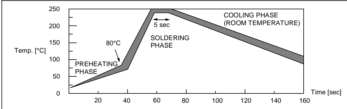
Figure 73. Recommended Reflow Soldering Oven Profile (MID JEDEC)
