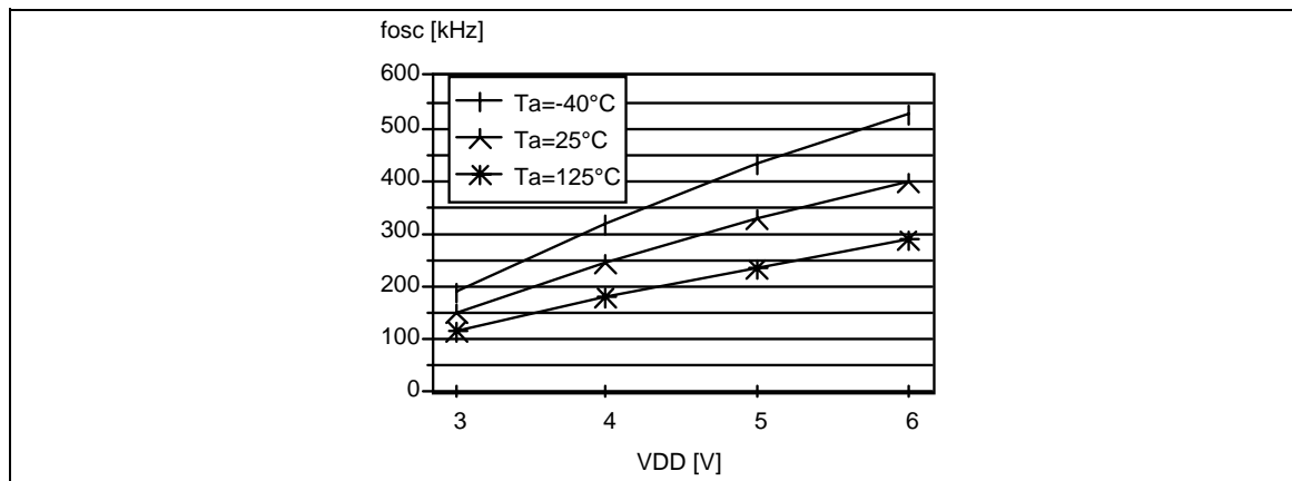
Figure 48. Typical LFAO Frequencies
