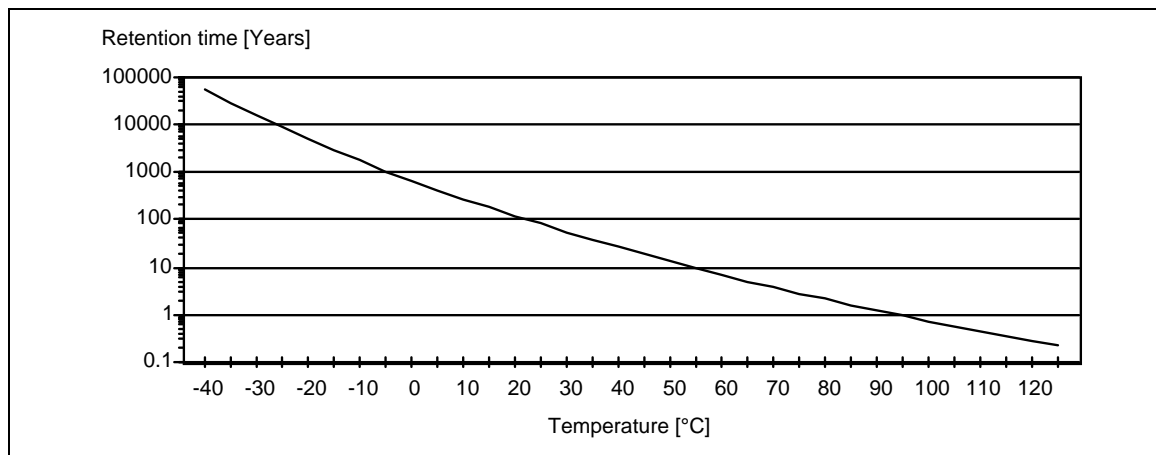
Figure 49. EPROM Retention Time vs. Temperature
