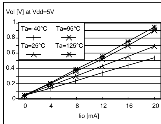
Figure 58. Typical V_{OL} at V_{DD} = 5V (high-sink)
