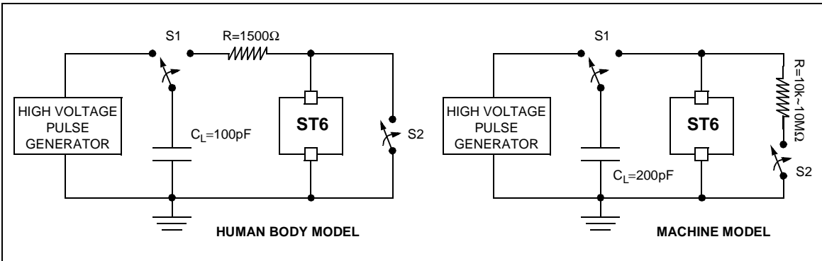
Figure 51. Typical Equivalent ESD Circuits
