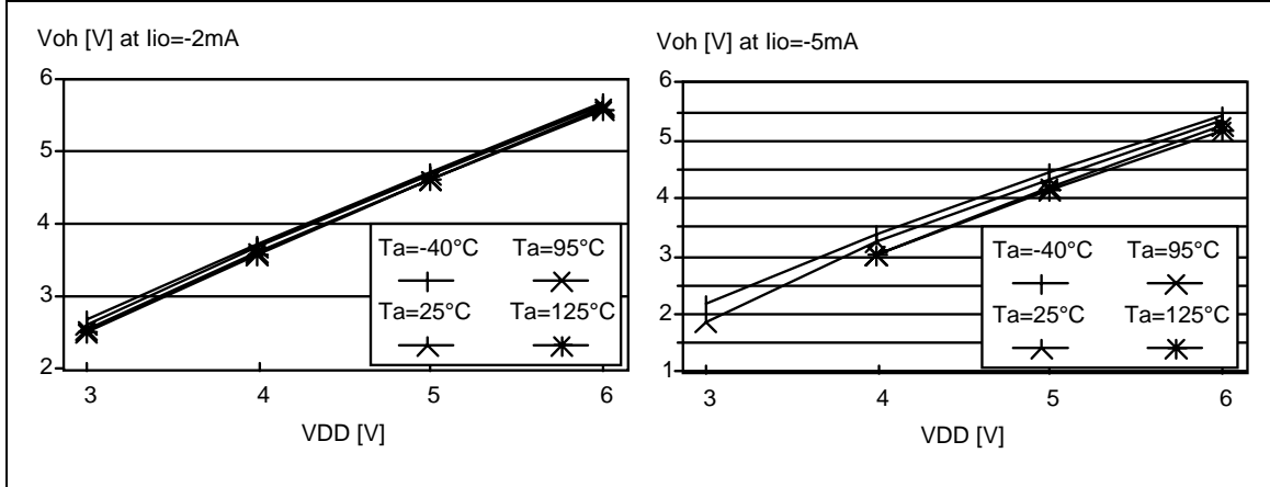
Figure 62. Typical V_{OH} vs V_{DD}
