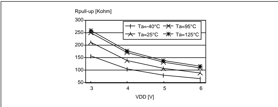
Figure 65. Typical R_{\text{pull-up}} vs. V_{\text{DD}} with V_{\text{IN}}=V_{\text{SS}}
