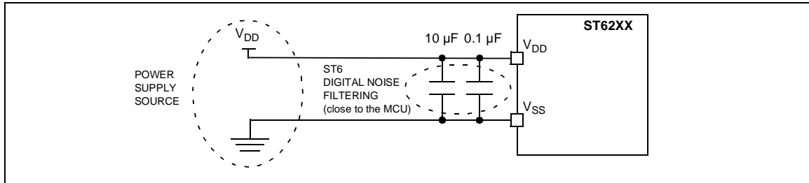
Figure 50. EMC Recommended Star Network Power Supply Connection 2)
