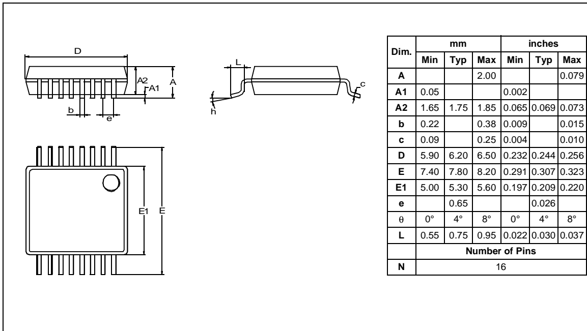
Figure 71. 16-Pin Plastic Shrink Small Outline Package
