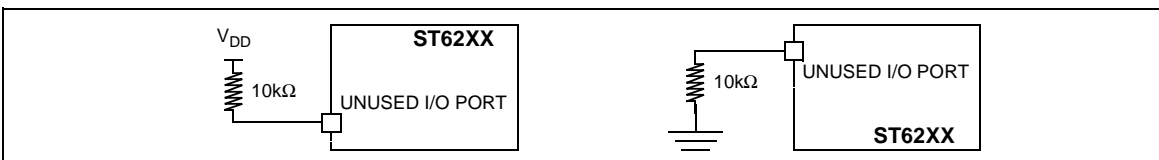
Figure 56. Two typical Applications with unused I/O Pin
