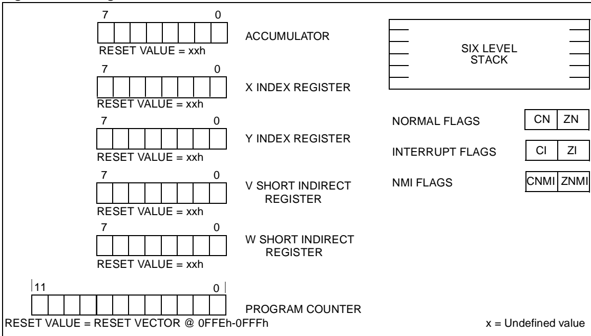
Figure 7. CPU Registers
