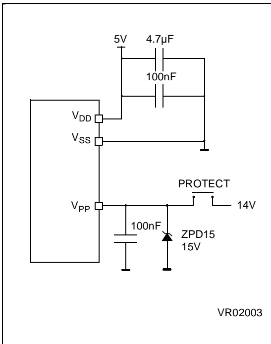
Figure 75. Programming Circuit
