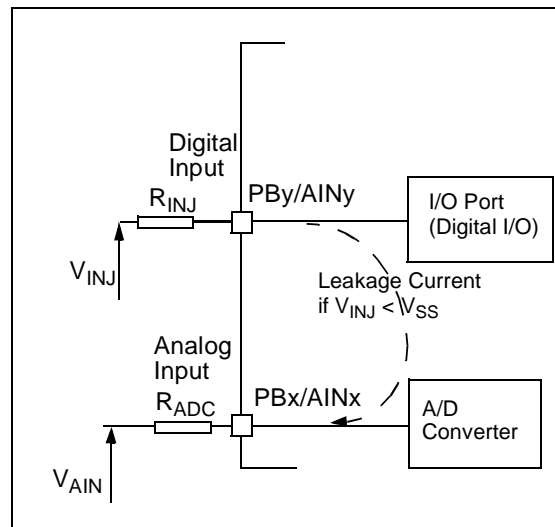
Figure 29. Leakage from Digital Inputs
