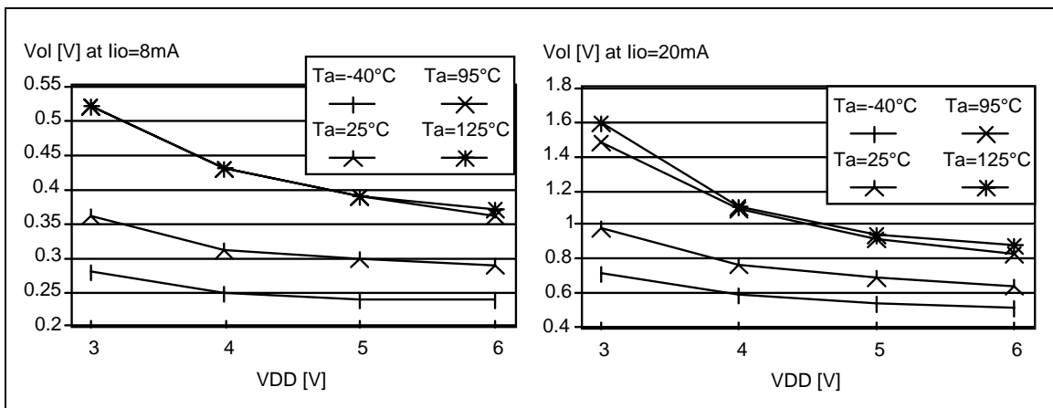
Figure 61. Typical V_{OL} vs V_{DD} (high-sink I/Os)
