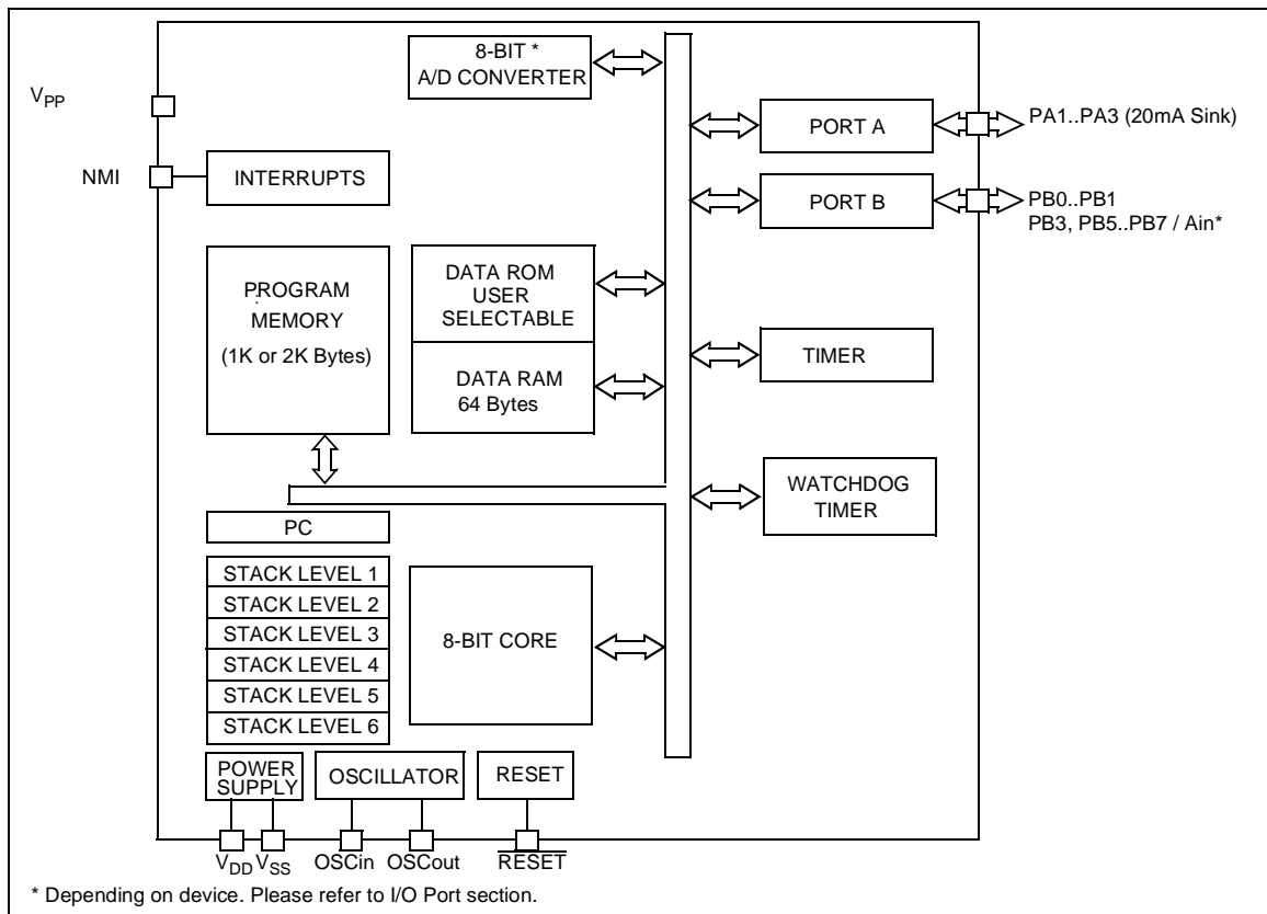
Figure 1. Block Diagram
