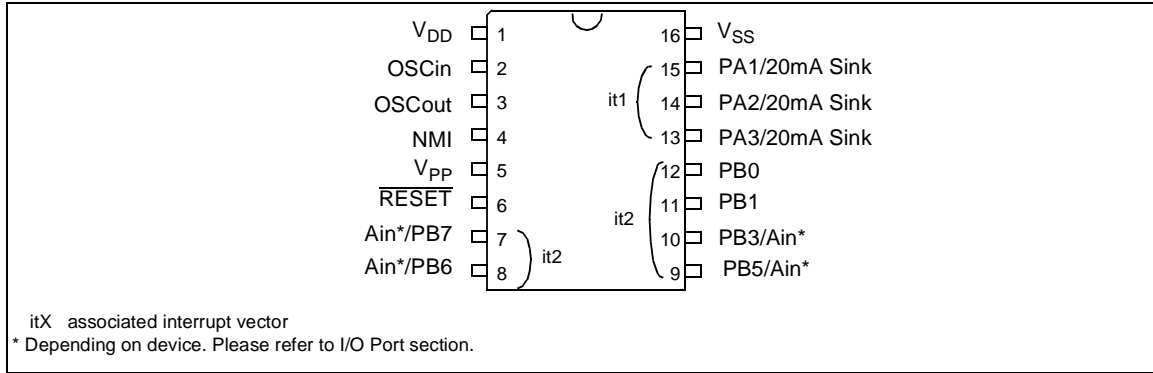
Figure 2. 16-Pin Package Pinout
