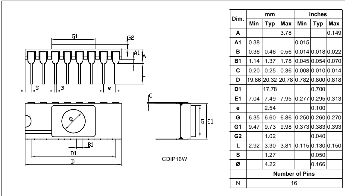
Figure 70. 16-Pin Ceramic Side-Brazed Dual In-Line Package
