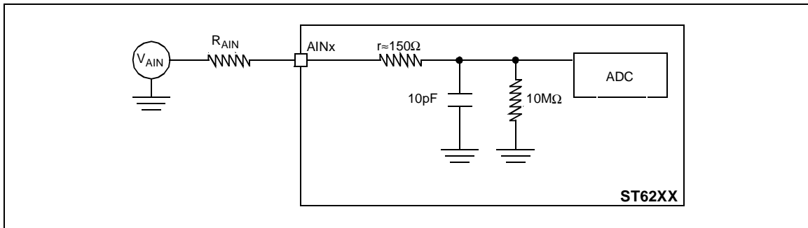
Figure 66. Typical Application with ADC
