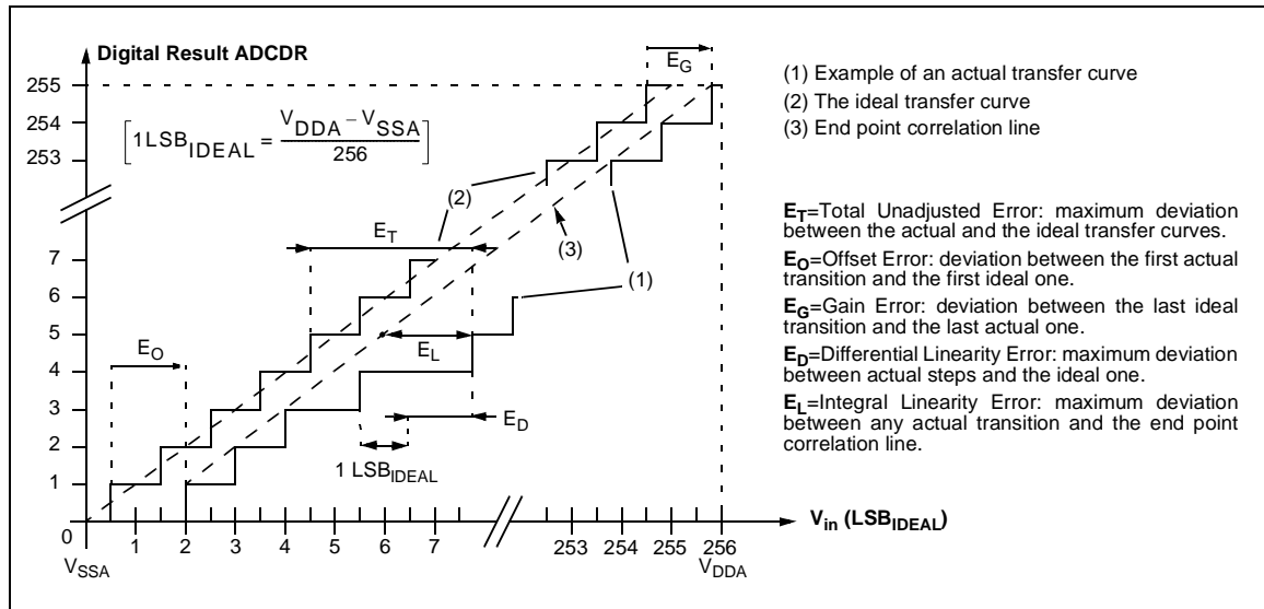
Figure 67. ADC Accuracy Characteristics
