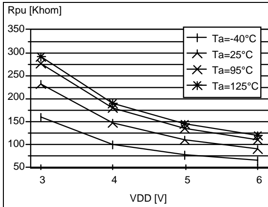
Figure 55. Typical R_{PU} vs. V_{DD} with V_{IN} = V_{SS}
