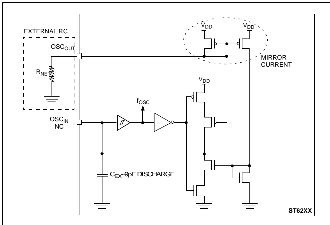
Figure 45. Typical Application with RC Oscillator
