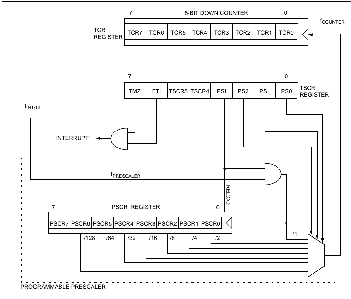
Figure 27. Timer Block Diagram
