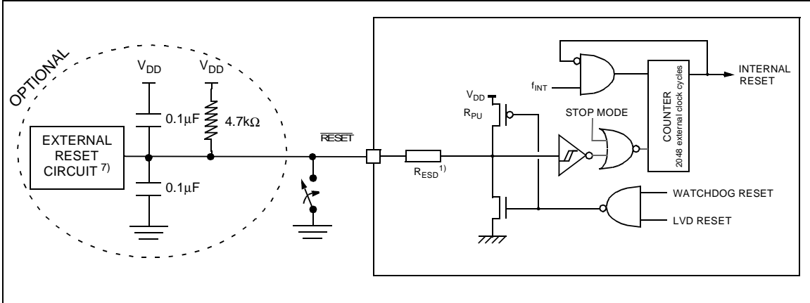
Figure 64. Typical Application with \overline{\text{RESET}} pin 8)
