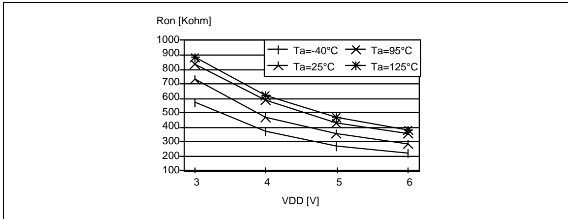
Figure 63. Typical R_{ON} vs V_{DD} with V_{IN}=V_{SS}
