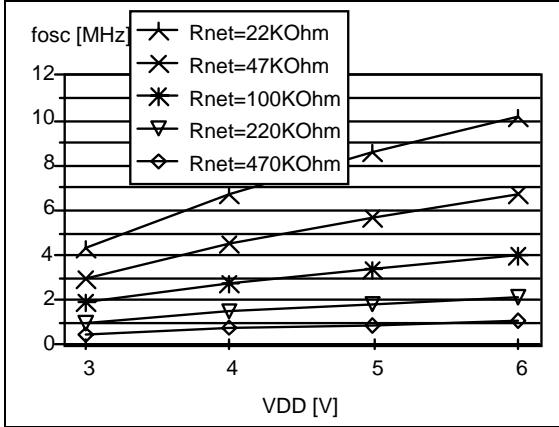
Figure 46. Typical RC Oscillator frequency vs. V DD
