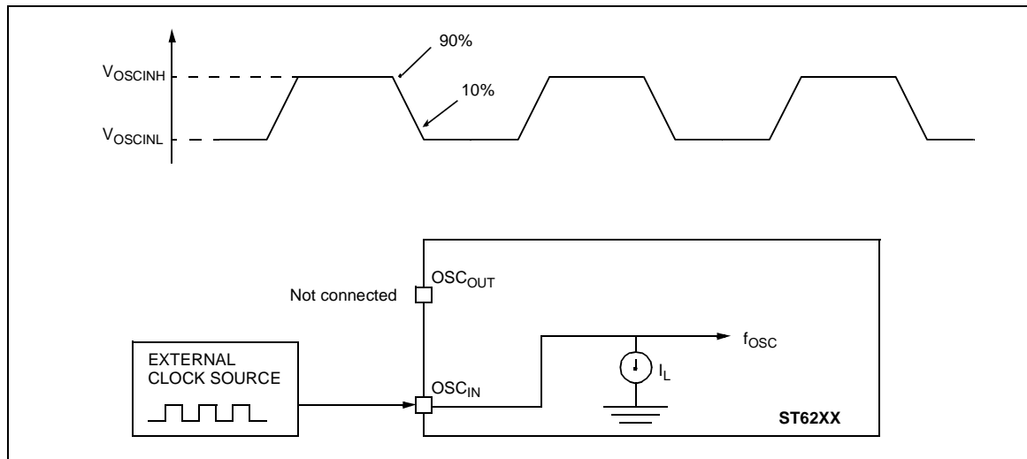
Figure 43. Typical Application with an External Clock Source
