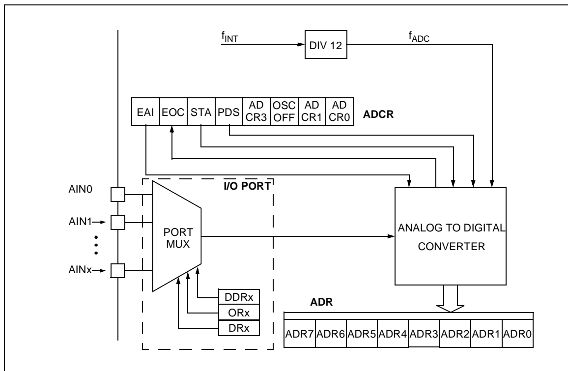
Figure 28. ADC Block Diagram
