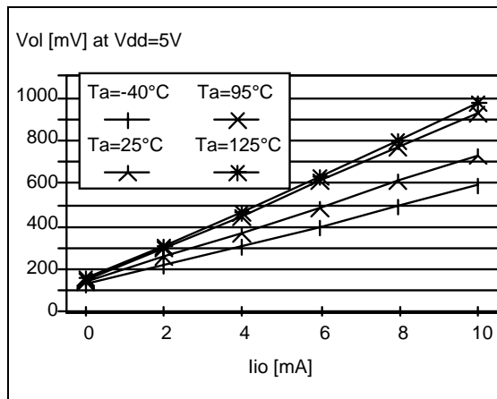
Figure 57. Typical V_{OL} at V_{DD} = 5V (standard)
