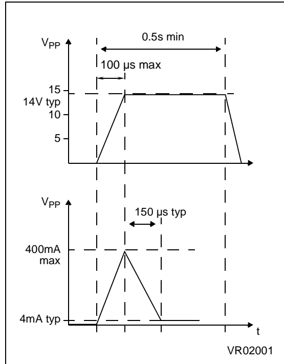
Figure 76. Programming wave form
