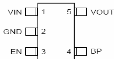
SC-70(Top View)
