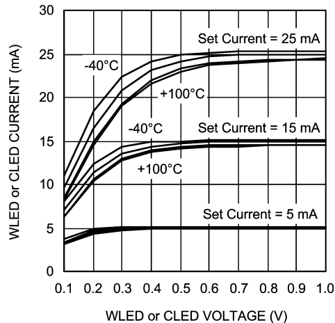
WLED or CLED Output Current vs Voltage Temperatures –40°C, 25°C, 85°C, 100°C
