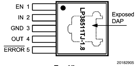
Top View TO-263 THIN 5 Pin Package
