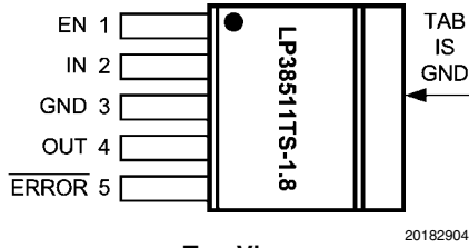
Top View TO-263 5 Pin Package
