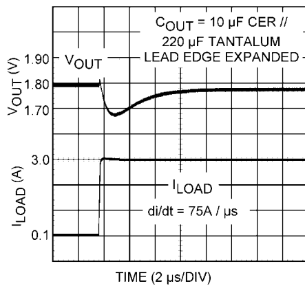
FIGURE 10. 10 µF Ceramic Paralleled By 220 µF Tantalum
