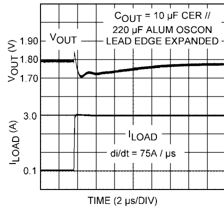
FIGURE 11. 10 µF Ceramic Paralleled By 220 µF OSCON
