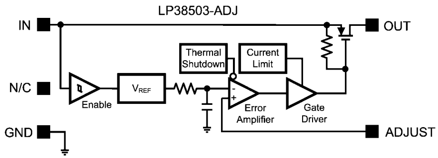
LP38503-ADJ Block Diagram
