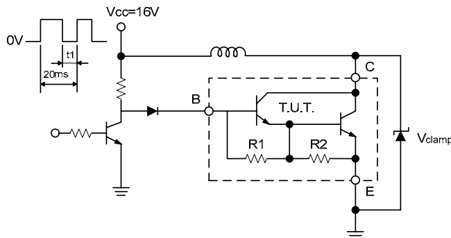
Fig. 1 Sustaining Voltage Test Circuit
