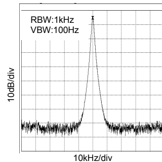
Fig.3 40.5MHz spectrum (CL=15pF, Ta=25 °C)
