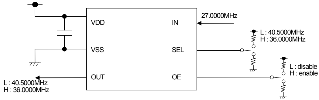
Fig.55 Application circuit example(BU7344HFV)
