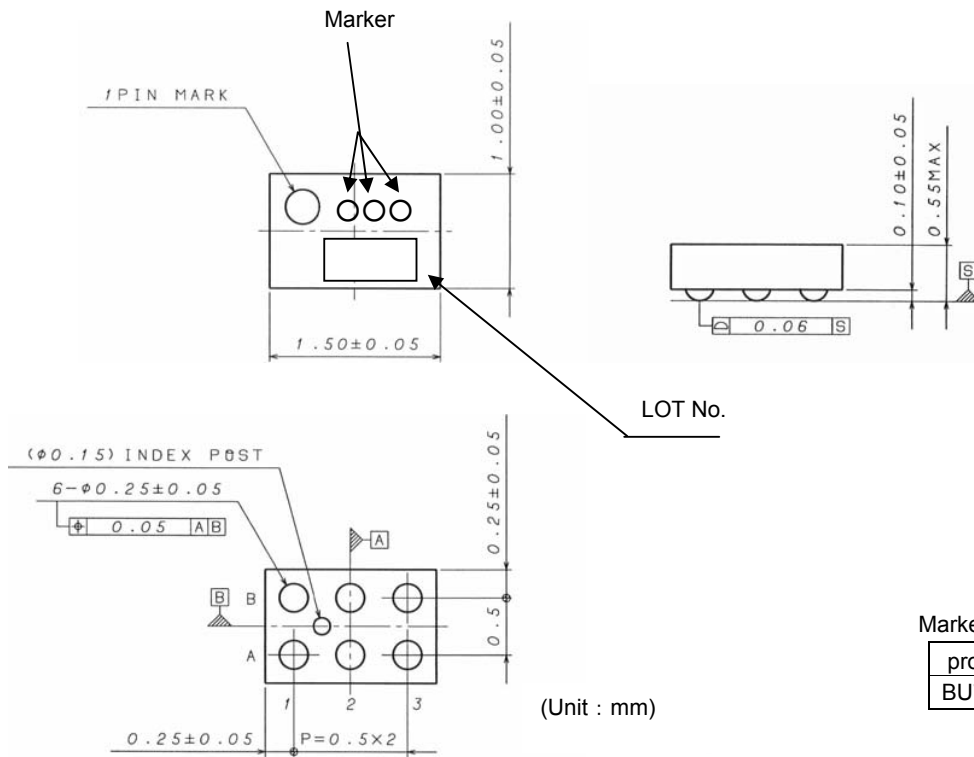
Fig.57 VCSP50L1 Appearance of Marker
