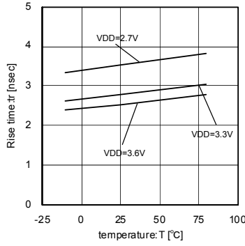
Fig.30 38MHz Temperature - Rise-time
