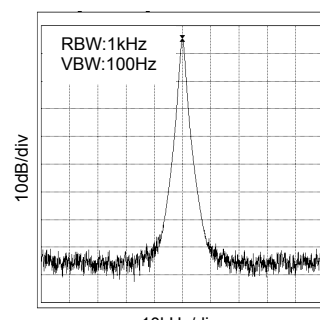
Fig.6 36MHz spectrum (CL=15pF, Ta=25 °C)
