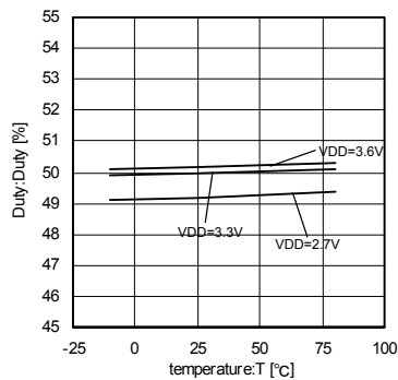
Fig.24 36MHz Temperature-Duty
