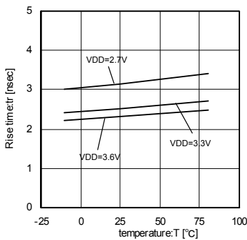
Fig.20 40.5MHz Temperature-Rise-time
