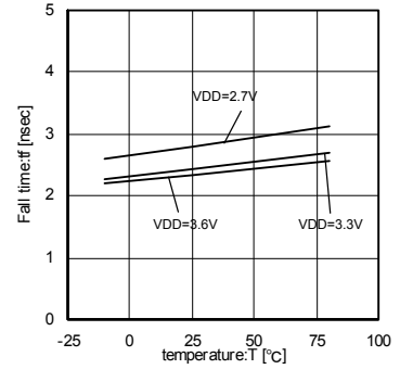
Fig.36 36MHz Temperature - Fall-time
