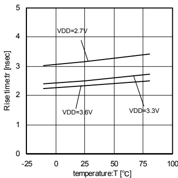
Fig.25 36MHz Temperature-Rise-time
