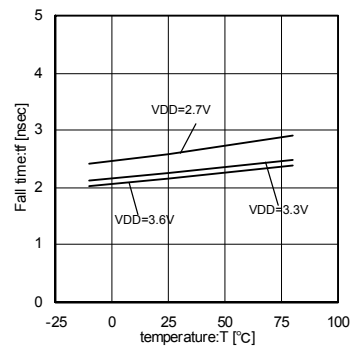
Fig.26 36MHz Temperature-Fall-time
