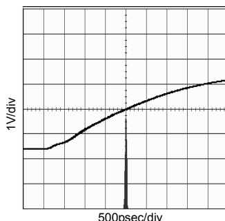
Fig.5 36MHz Period-Jitter (CL=15pF, Ta=25 °C)
