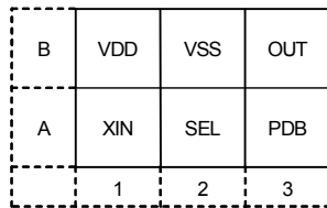
Bottom view Fig.53 Pin assignment
