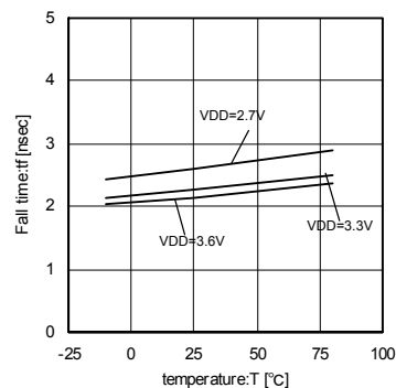
Fig.21 40.5MHz Temperature-Fall-time
