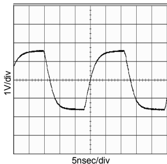
Fig.7 38MHz output waveform (CL=15pF, Ta=25 °C)
