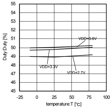
Fig.44 36MHz Temperature - Duty
