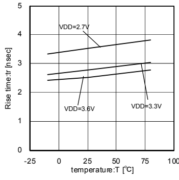
Fig.35 36MHz Temperature - Rise-time
