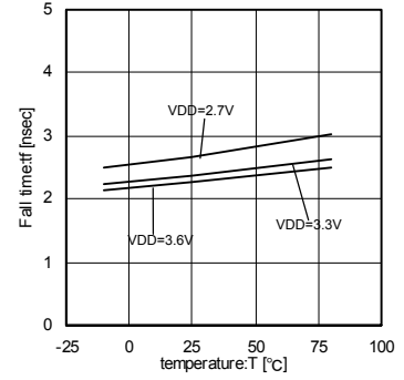
Fig.41 38MHz Temperature - Fall-time
