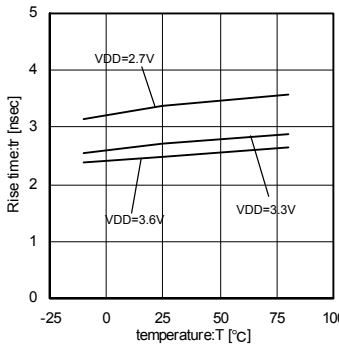
Fig.45 36MHz Temperature - Rise-time
