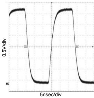
Fig.16 36MHz output waveform (CL=15pF,Ta=25 °C)
