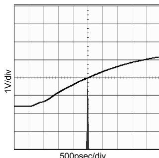
Fig.2 40.5MHz Period-Jitter (CL=15pF, Ta=25 °C)
