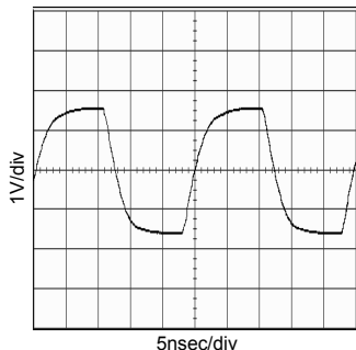
Fig.1 40.5MHz output waveform (CL=15pF, Ta=25 °C)
