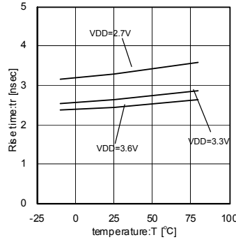
Fig.40 38MHz Temperature - Rise-time
