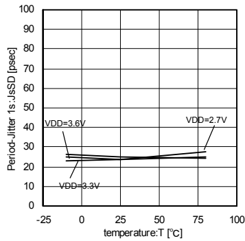
Fig.42 38MHz Temperature - Period-Jitter 1σ
