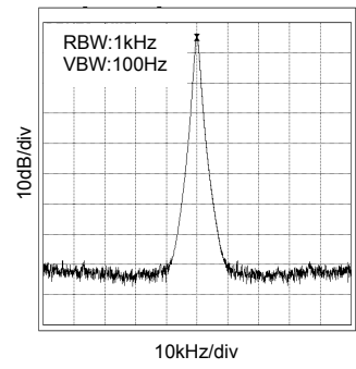
Fig.18 36MHz spectrum (CL=15pF,Ta=25 °C)
