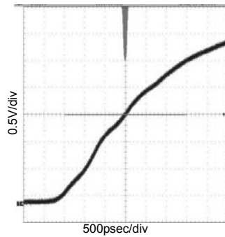
Fig.17 36MHz Period-Jitter (CL=15pF,Ta=25 °C)
