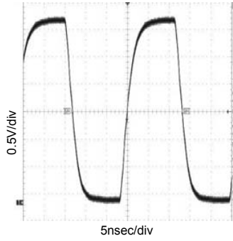
Fig.13 38MHz output waveform (CL=15pF,Ta=25 °C)
