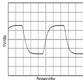
Fig.4 36MHz output waveform (CL=15pF, Ta=25 °C)
