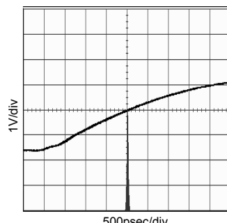
Fig.11 36MHz Period-Jitter (CL=15pF, Ta=25 °C)
