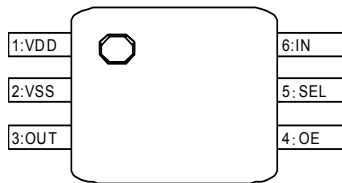
Fig.51 Pin assignment
