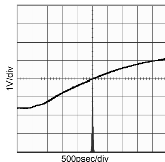
Fig.8 38MHz Period-Jitter (CL=15pF, Ta=25 °C)
