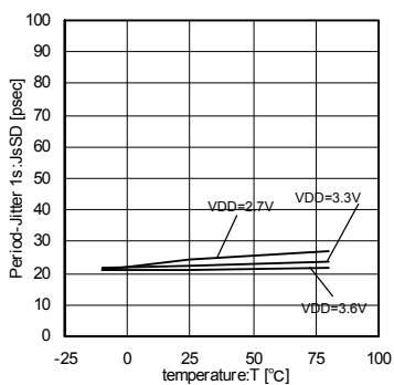
Fig.27 36MHz Temperature-Period-Jitter 1σ
