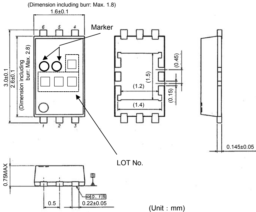
Fig.56 HVSO6 Appearance of Marker
