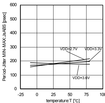
Fig.48 36MHz Temperature - Period-Jitter MIN-MAX
