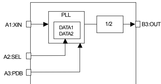
Fig.54 Block diagram
