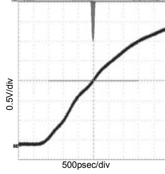
Fig.14 38MHz Period-Jitter (CL=15pF,Ta=25 °C)
