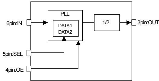
Fig.52 Block diagram
