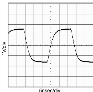
Fig.10 36MHz output waveform (CL=15pF, Ta=25 °C)
