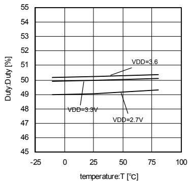
Fig.19 40.5MHz Temperature-Duty
