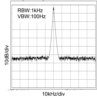
Fig.15 38MHz spectrum (CL=15pF,Ta=25 °C)
