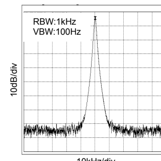
Fig.12 36MHz spectrum (CL=15pF, Ta=25 °C)
