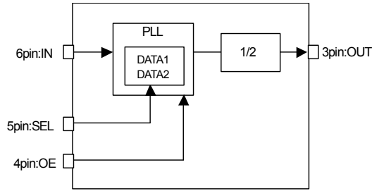
Fig.50 Block diagram
