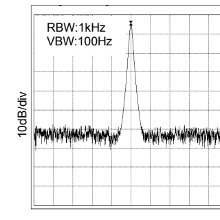
Fig.9 38MHz spectrum (CL=15pF, Ta=25 °C)
