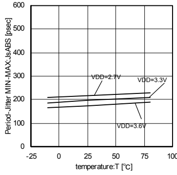
Fig.33 38MHz Temperature - Period-Jitter MIN-MAX
