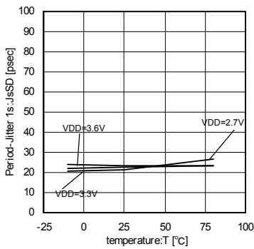
Fig.47 36MHz Temperature - Period-Jitter 1σ
