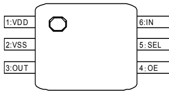
Fig.49 Pin assignment
