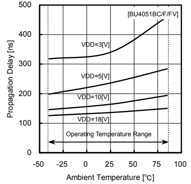
Fig.13 propagation delay time tPL (CONT—OUT)
