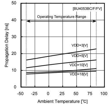
Fig.32 propagation delay time tPHL (IN—OUT)
