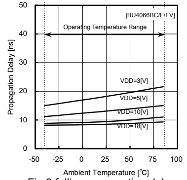
Fig.3 falling propagation delay (IN—OUT)
