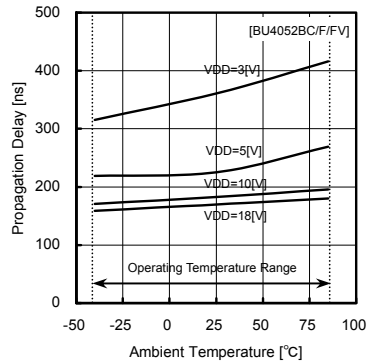
Fig.27 propagation delay time tPHZ (INH—OUT)
