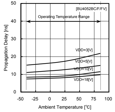
Fig.21 propagation delay time tPHL (IN—OUT)
