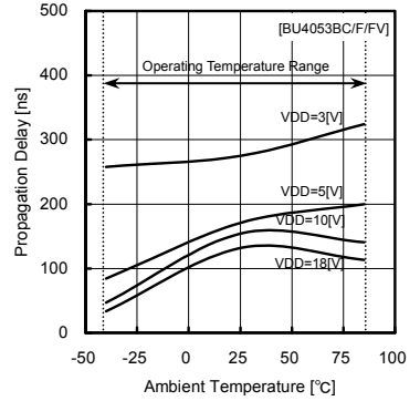
Fig.35 propagation delay time tPLZ (CONT—OUT)
