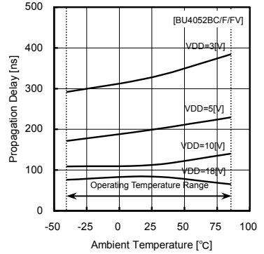
Fig.24 propagation delay time tPLZ (CONT—OUT)
