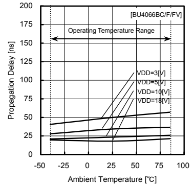
Fig.6 rising propagation delay (CONT—OUT, tPLZ)
