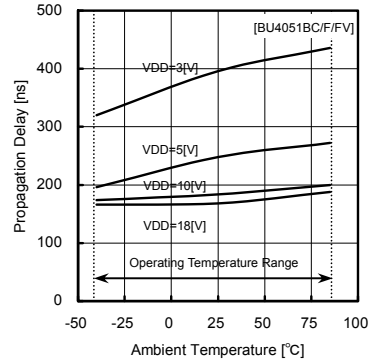
Fig.16 propagation delay time tPHZ (INH—OUT)
