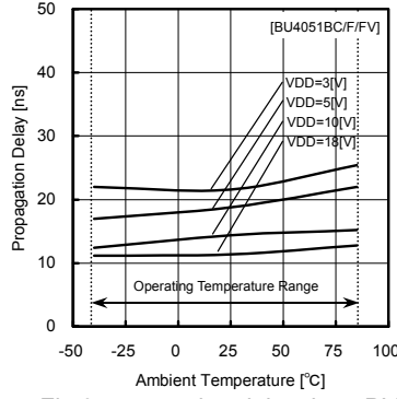
Fig.9 propagation delay time tPL (IN—OUT)
