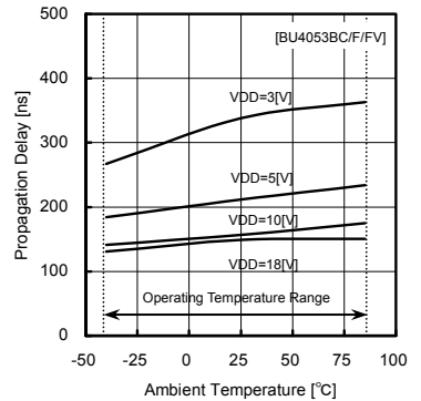
Fig.38 propagation delay time tPHZ (INH—OUT)
