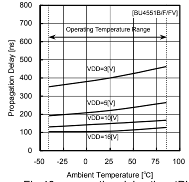
Fig.46 propagation delay time tPLZ (CONT – OUT)
