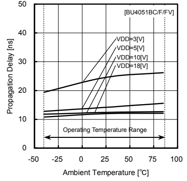
Fig.10 propagation delay time tPH (IN—OUT)
