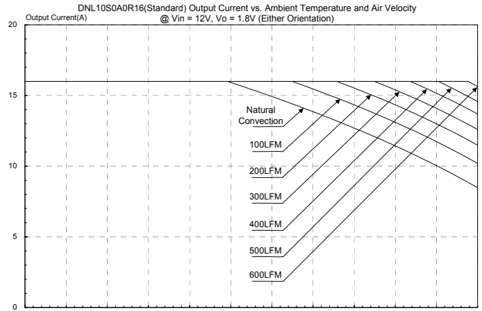
Figure 34: Output current vs. ambient temperature and air velocity @ Vin=12V, Vout=1.8V(Either Orientation)
