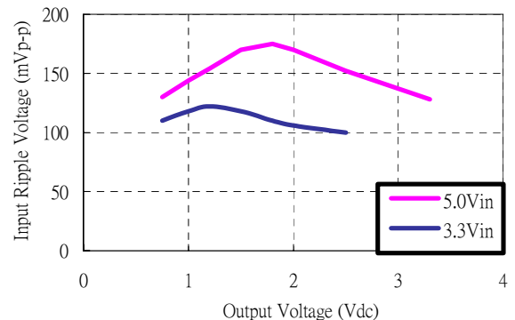
Figure 33: Input voltage ripple for various output models, IO = 16 A (CIN = 4x100 µF tantalum // 2x47 µF ceramic)
