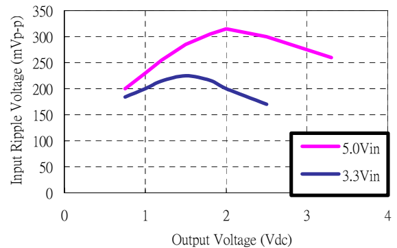
Figure 32: Input voltage ripple for various output models, IO = 16 A (CIN = 2x100 µF tantalum // 47 µF ceramic)
