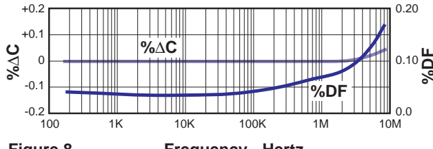
Figure 8. Frequency - Hertz Capacitance & DF vs Frequency - C0G
