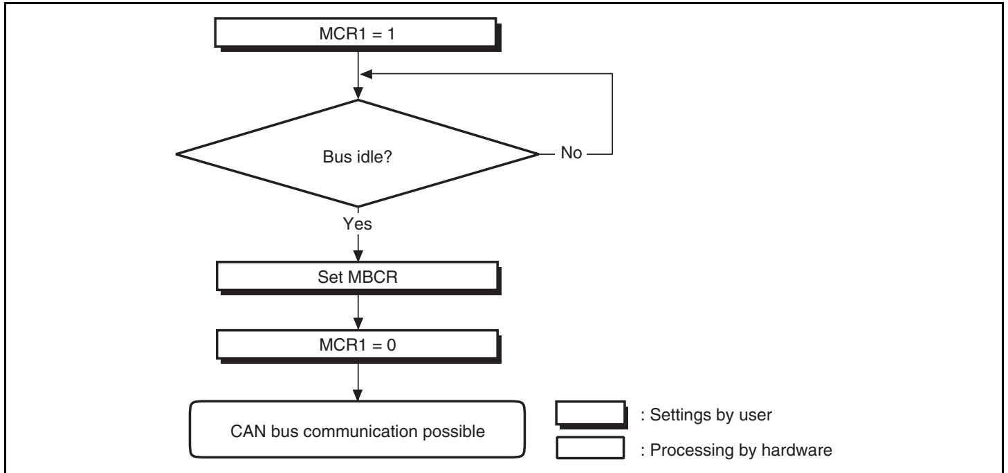
Figure 14.14 HCAN Halt Mode Flowchart
