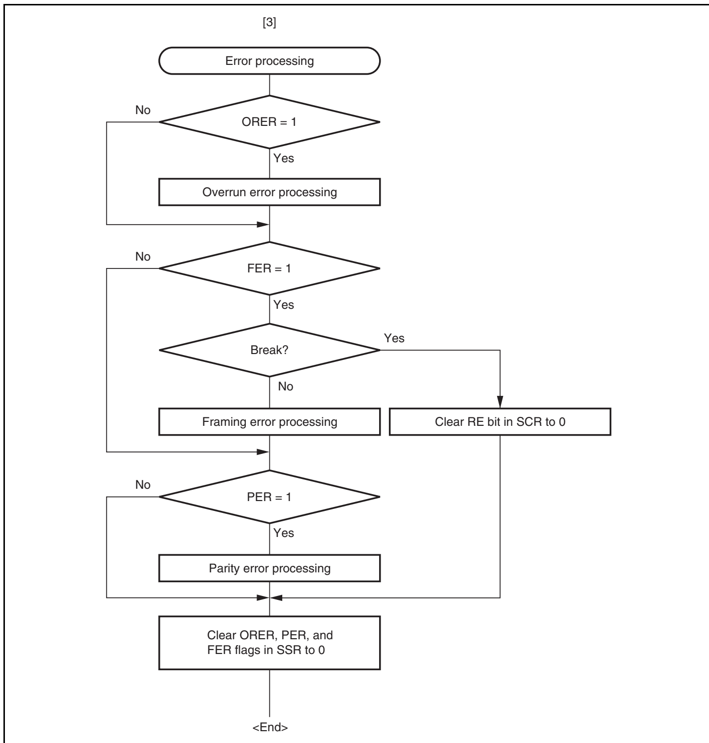
Figure 13.9 Sample Serial Reception Data Flowchart (2)
