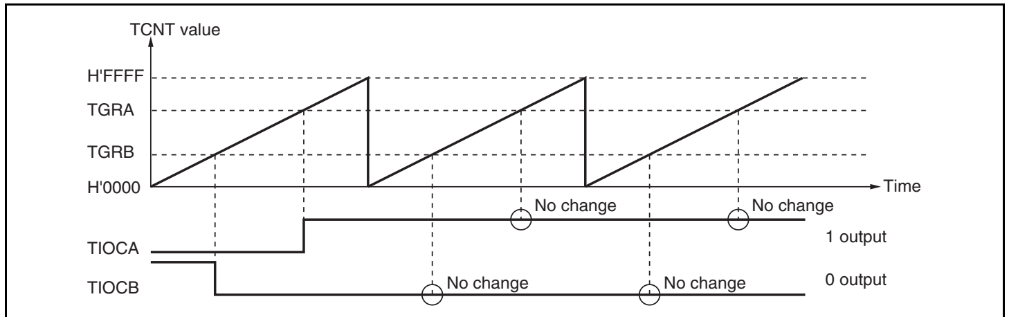
Figure 10.6 Example of 0 Output/1 Output Operation
