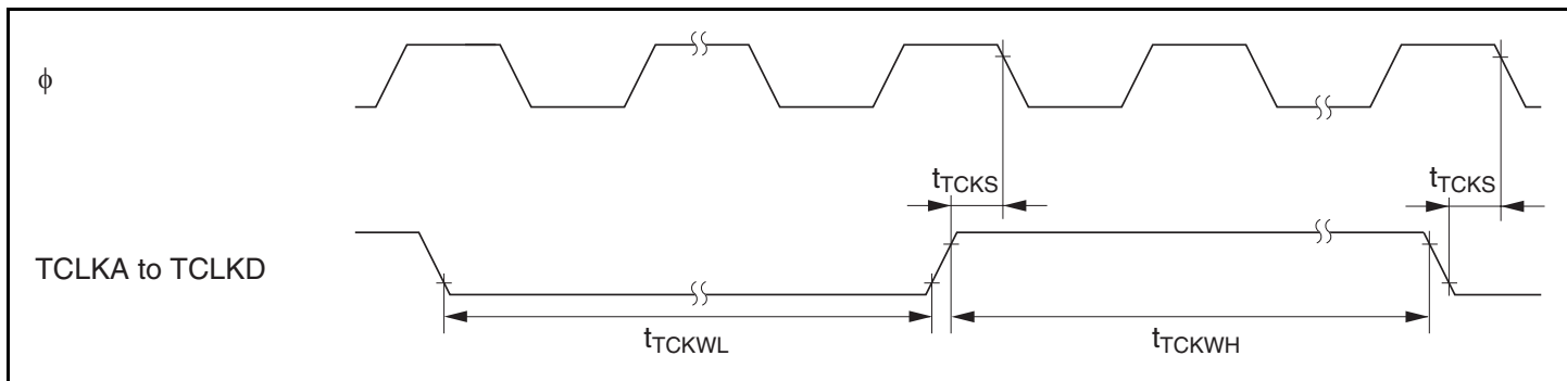
Figure 23.14 TPU Clock Input Timing
