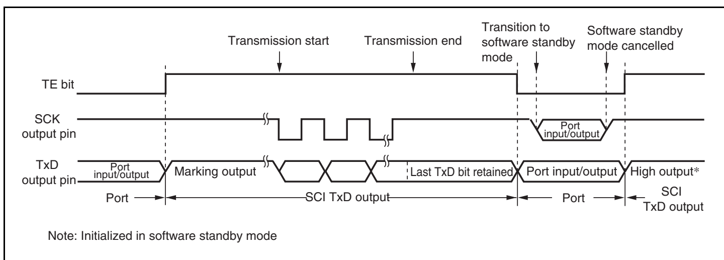
Figure 13.36 Pin States during Transmission in Clocked Synchronous Mode (Internal Clock)
