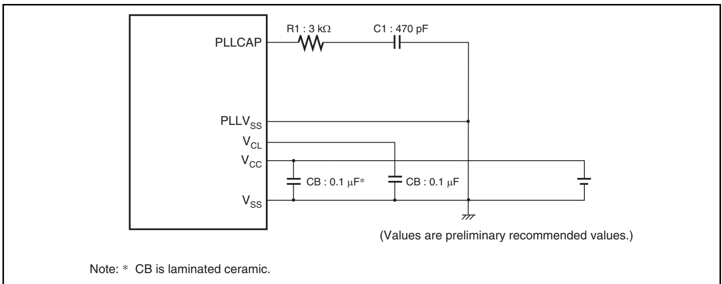
Figure 20.10 External Circuitry Recommended for PLL Circuit
