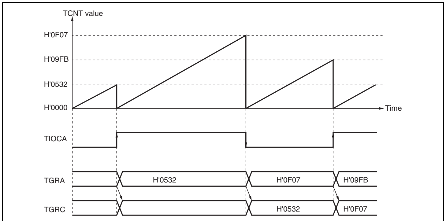
Figure 10.16 Example of Buffer Operation (2)
