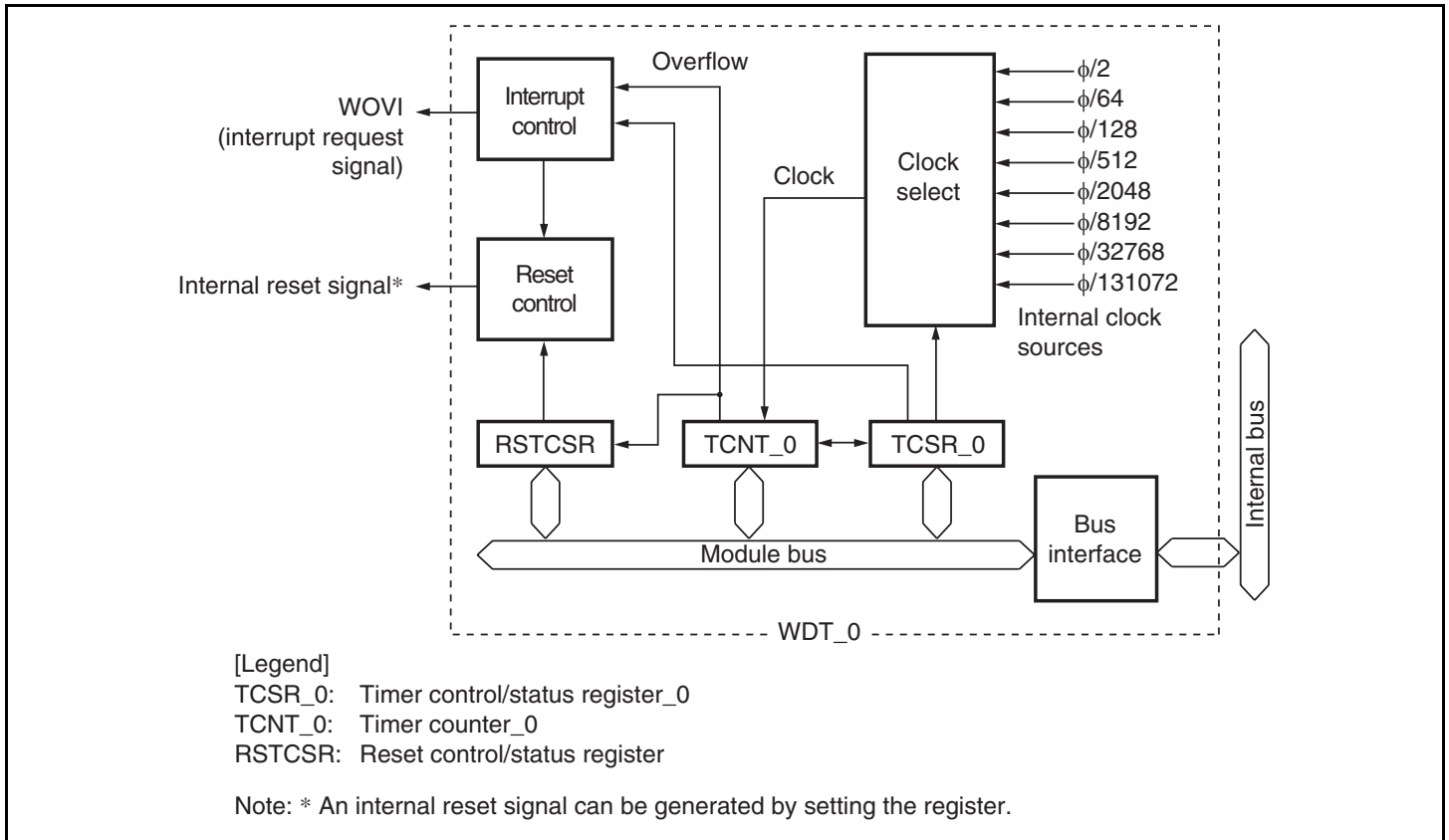
Figure 12.1 Block Diagram of WDT_0
