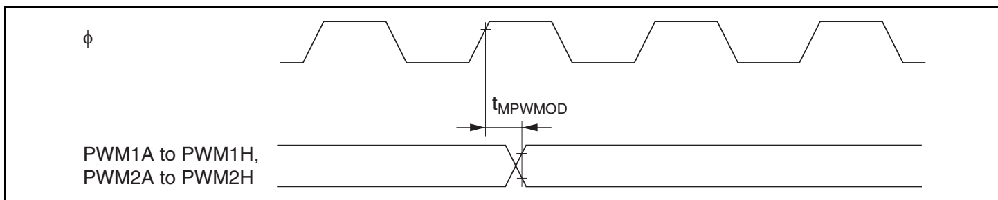
Figure 23.15 Motor Control PWM Output Timing
