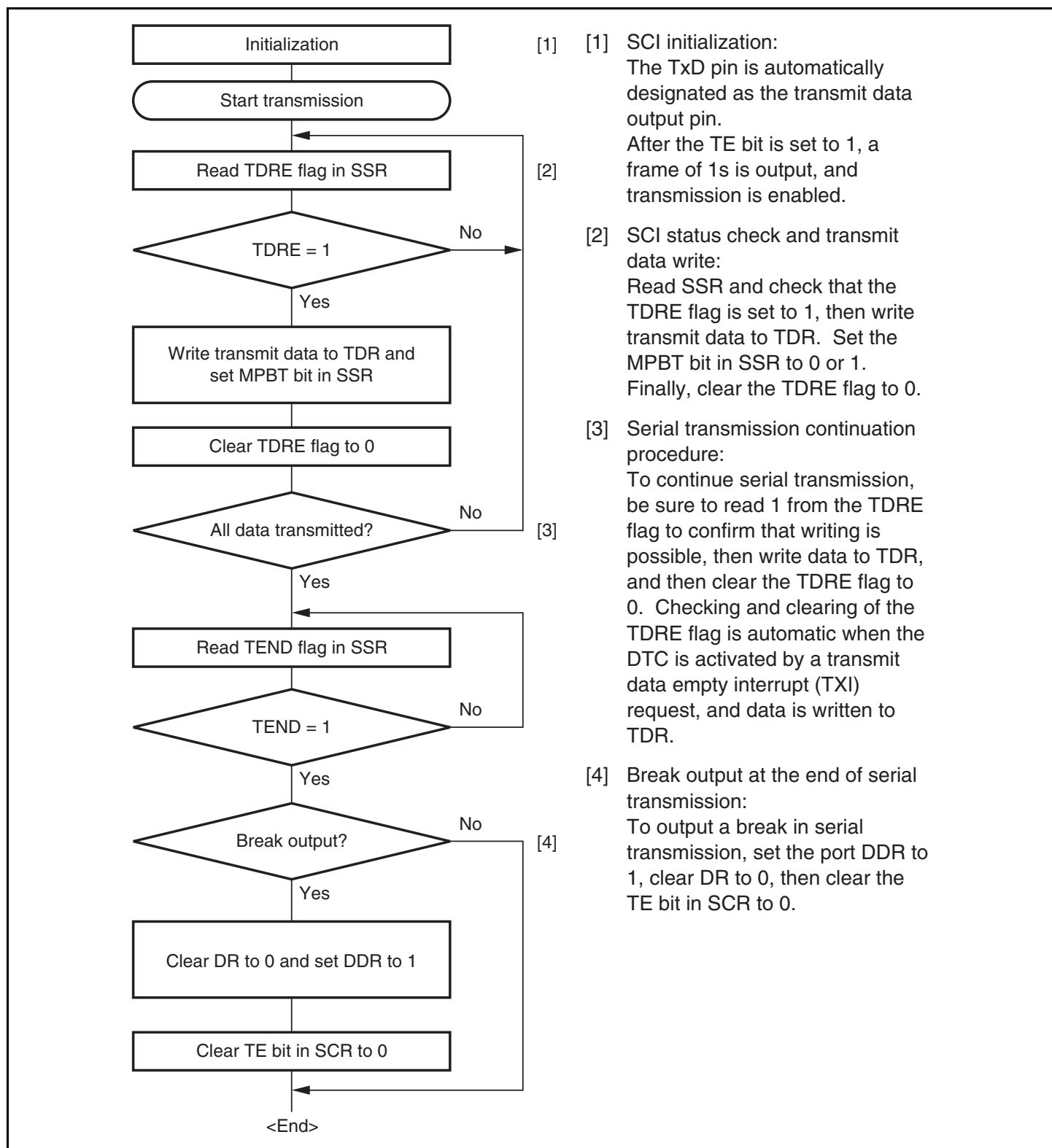
Figure 13.11 Sample Multiprocessor Serial Transmission Flowchart
