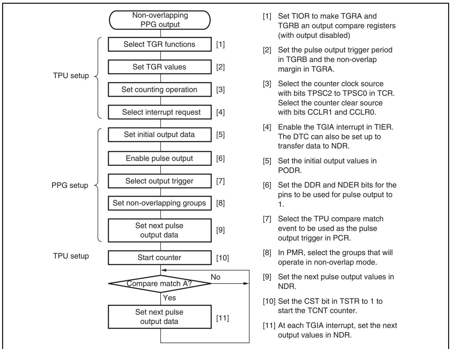
Figure 11.8 Setup Procedure for Non-Overlapping Pulse Output (Example)
