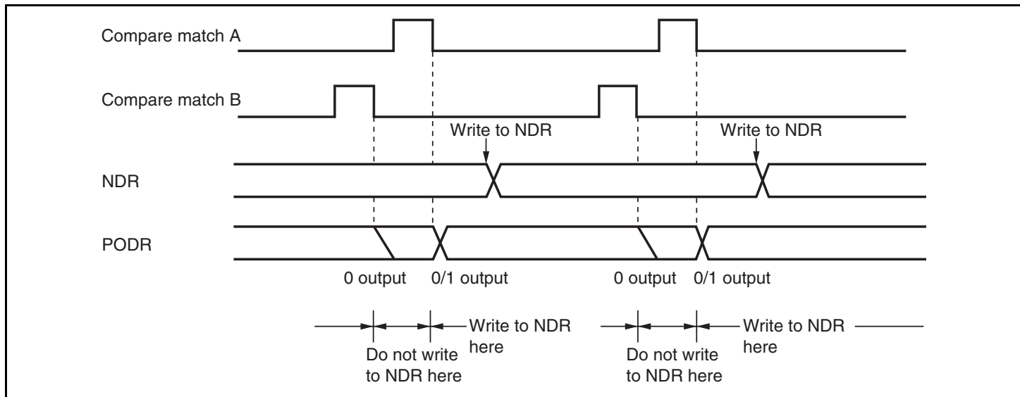
Figure 11.7 Non-Overlapping Operation and NDR Write Timing
