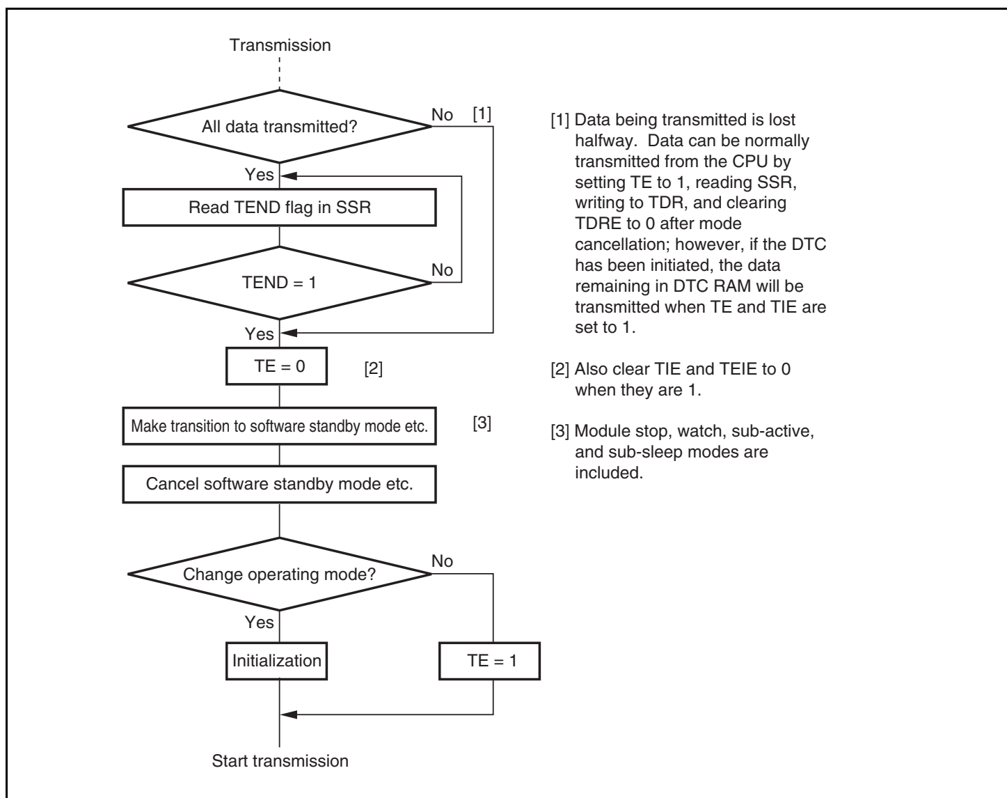
Figure 13.34 Sample Flowchart for Mode Transition during Transmission
