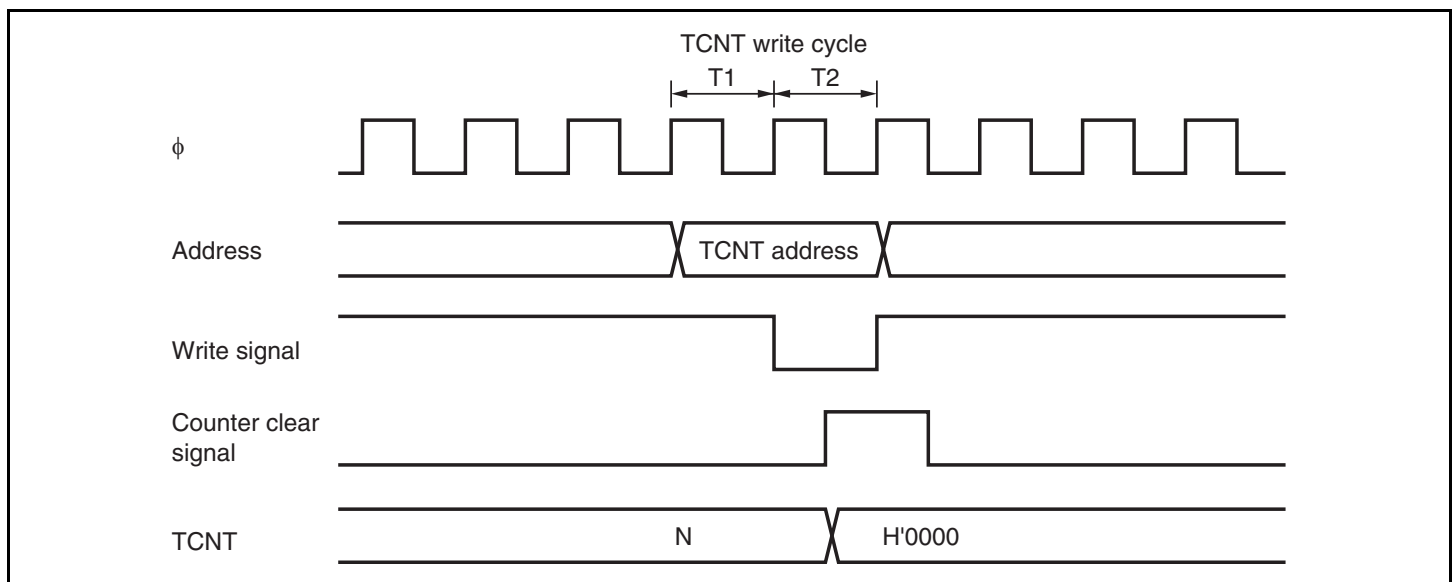
Figure 10.45 Conflict between TCNT Write and Clear Operations
