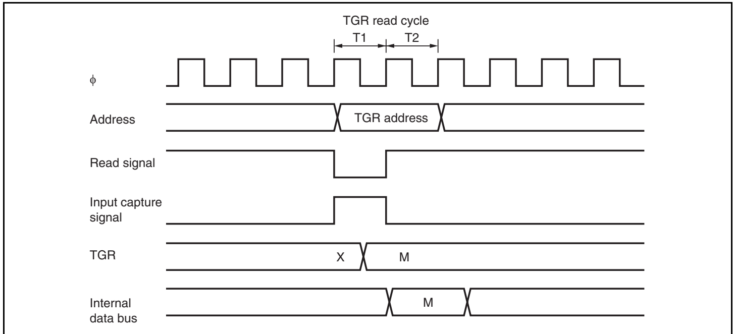
Figure 10.49 Conflict between TGR Read and Input Capture
