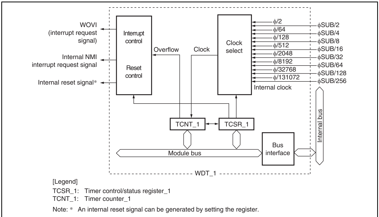
Figure 12.2 Block Diagram of WDT_1
