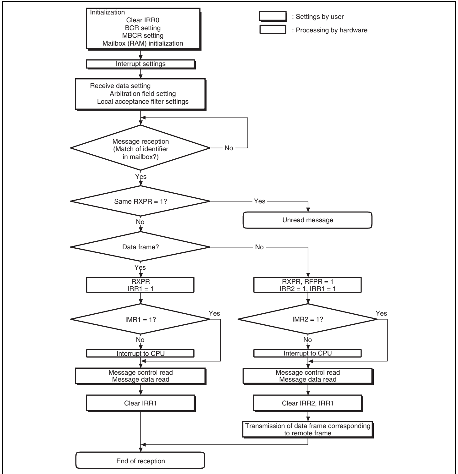
Figure 14.11 Reception Flowchart
