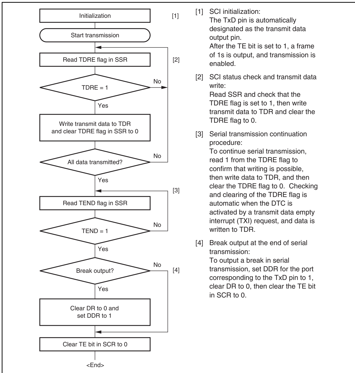
Figure 13.7 Sample Serial Transmission Flowchart
