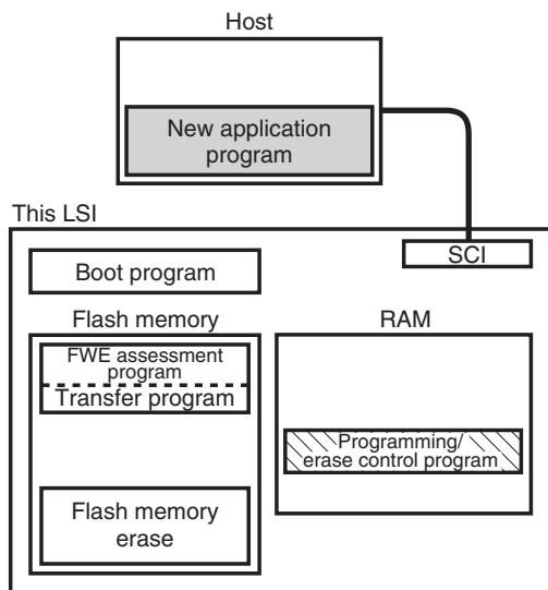
Figure 19.4 User Program Mode (Example)
