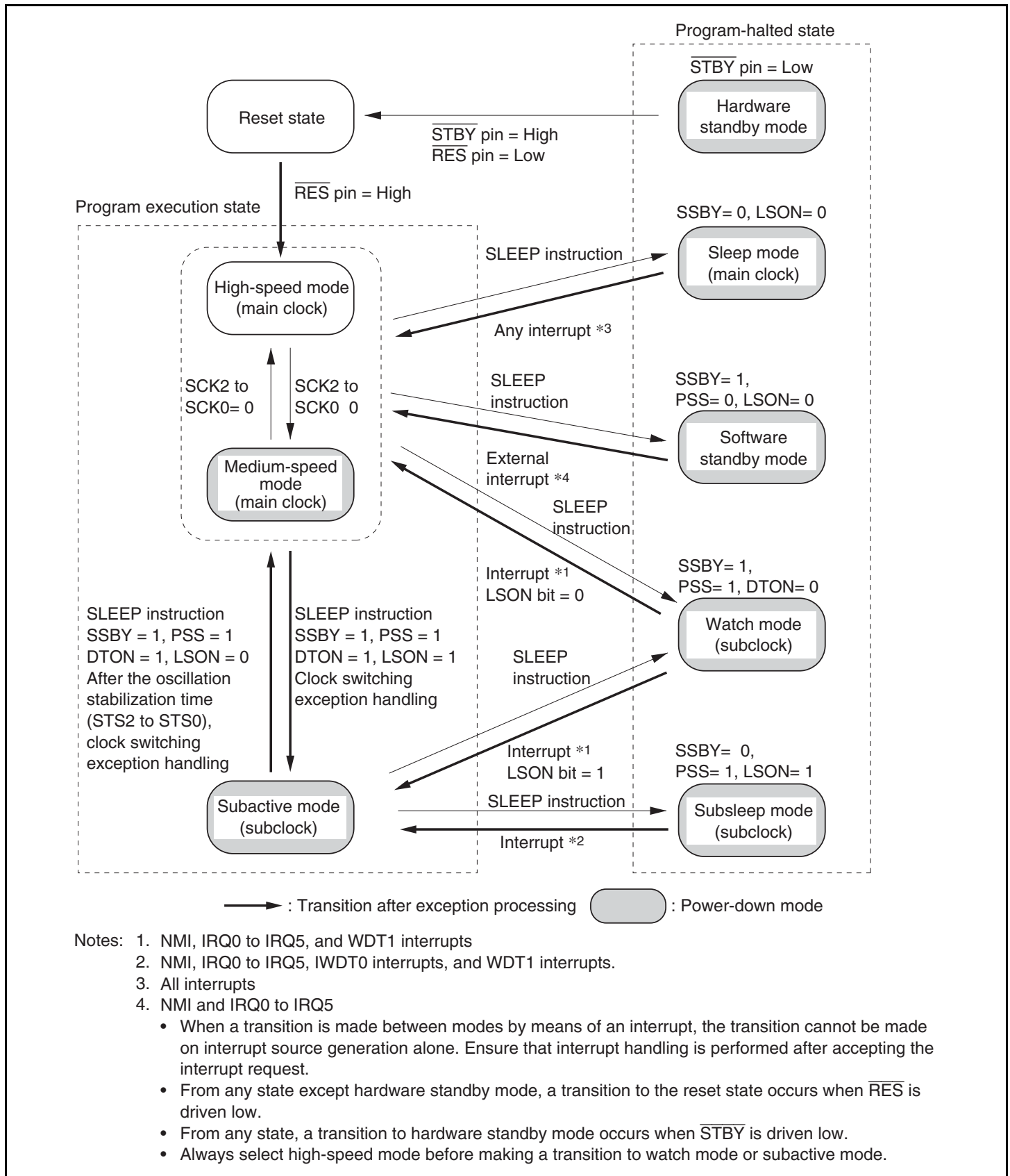
Figure 21.1 Mode Transition Diagram
