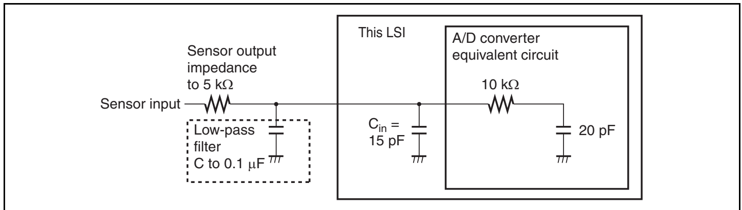
Figure 15.6 Example of Analog Input Circuit
