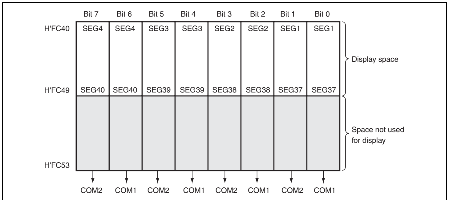
Figure 17.5 LCD RAM Map (1/2 Duty)
