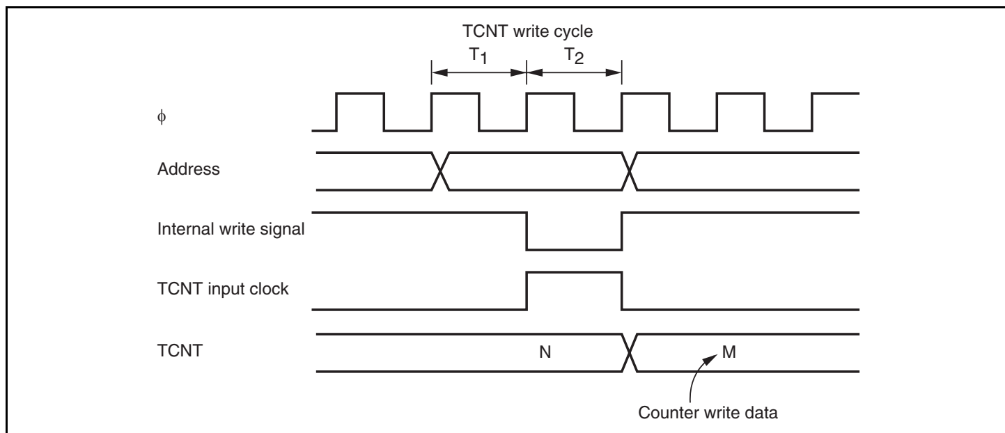
Figure 12.5 Contention between TCNT Write and Increment
