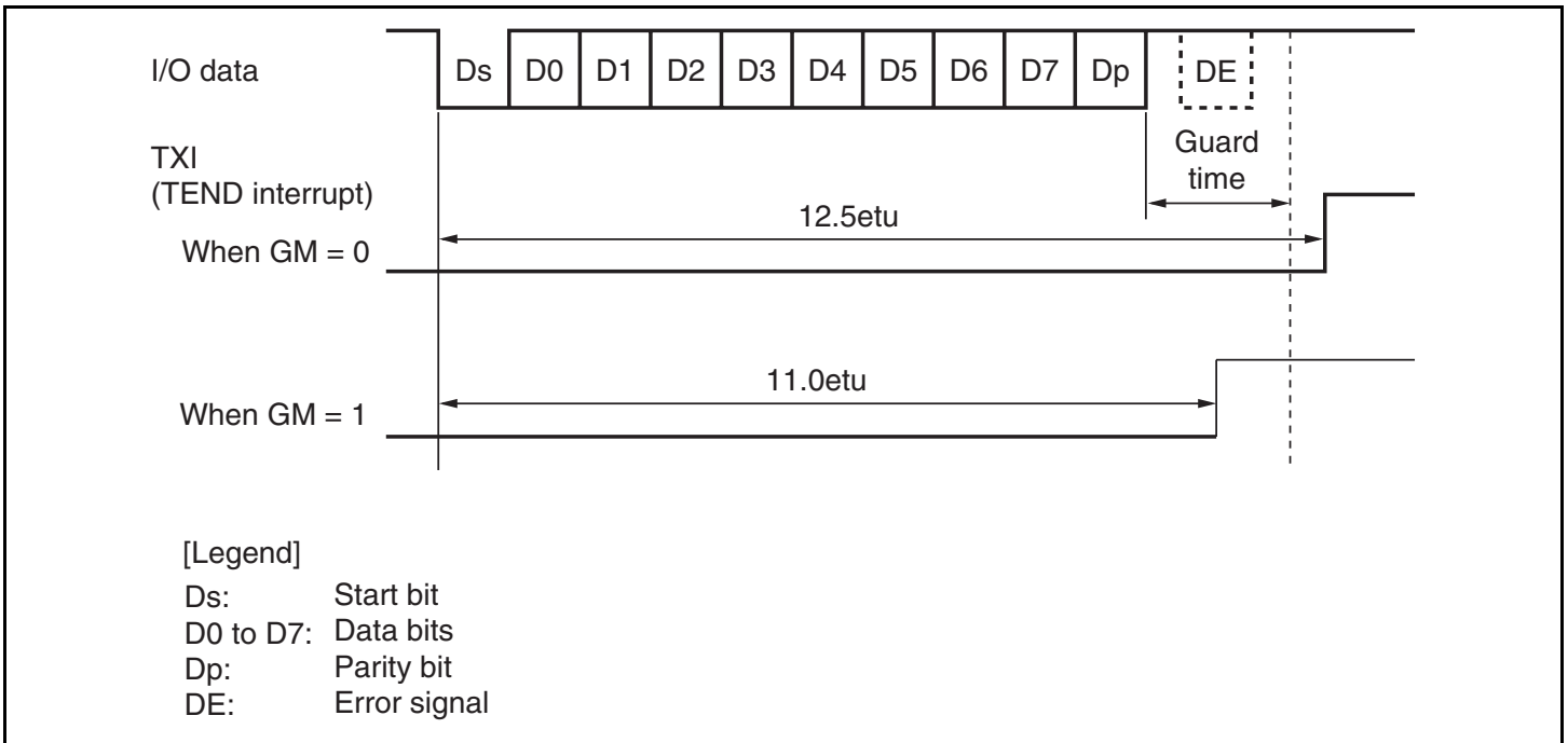
Figure 13.27 TEND Flag Generation Timing in Transmission Operation
