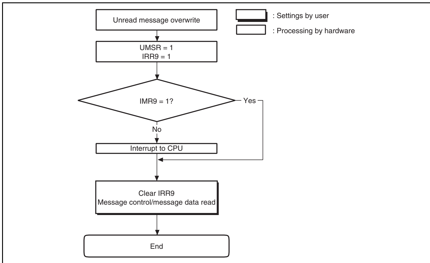
Figure 14.12 Unread Message Overwrite Flowchart
