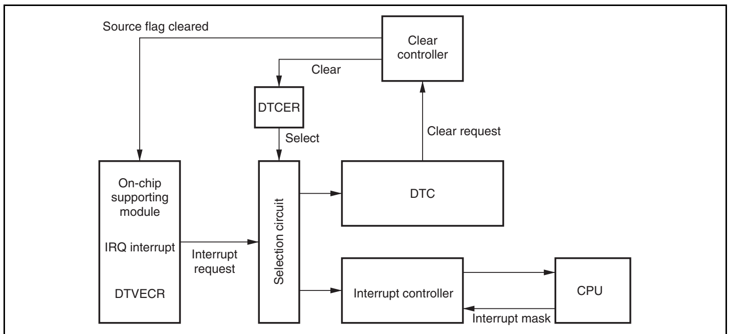
Figure 8.2 Block Diagram of DTC Activation Source Control
