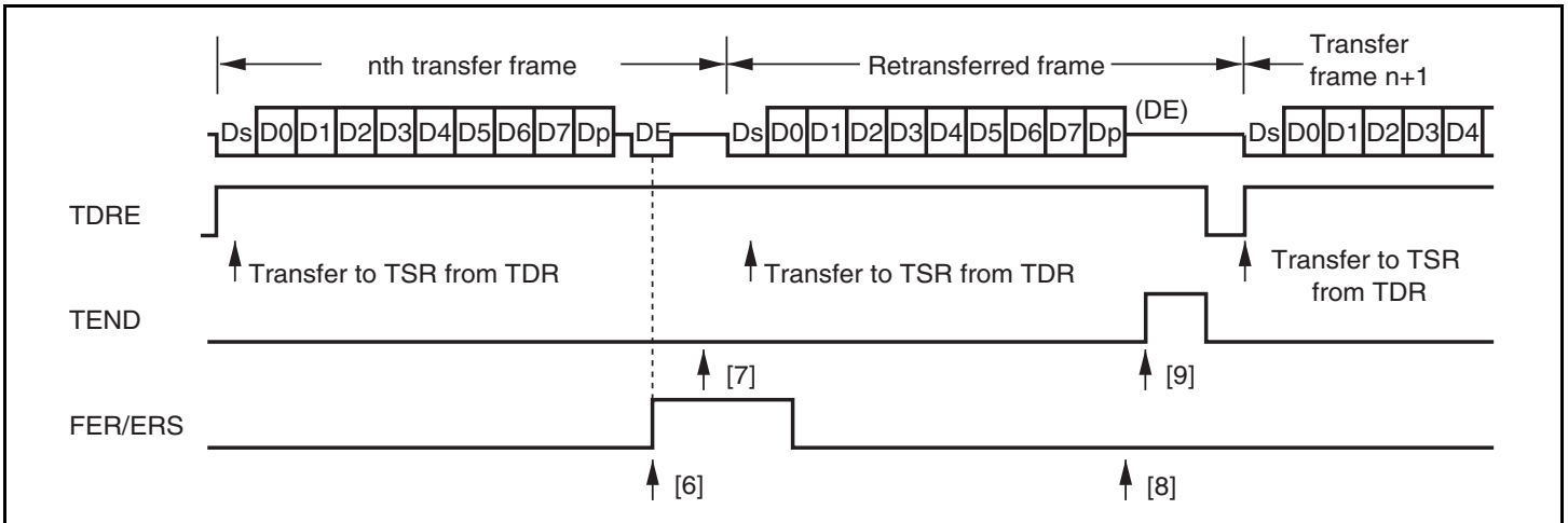
Figure 13.26 Retransfer Operation in SCI Transmit Mode
