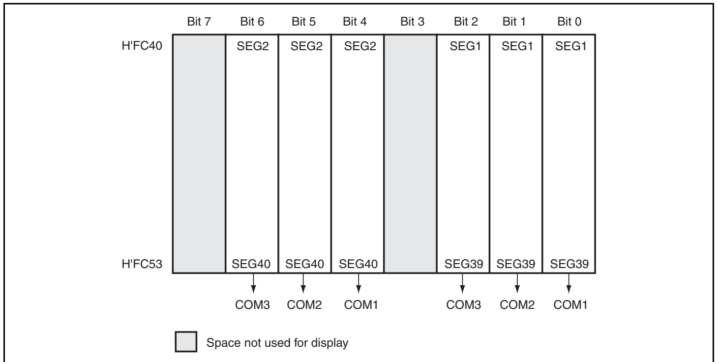
Figure 17.4 LCD RAM Map (1/3 Duty)
