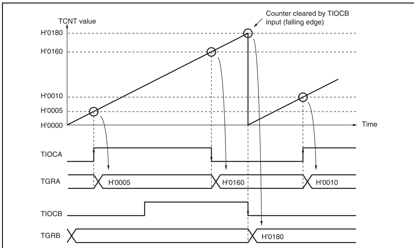
Figure 10.9 Example of Input Capture Operation
