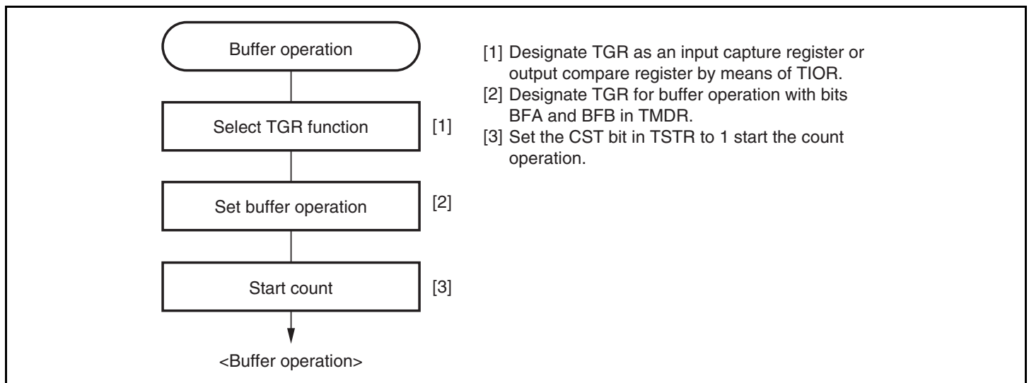
Figure 10.14 Example of Buffer Operation Setting Procedure
