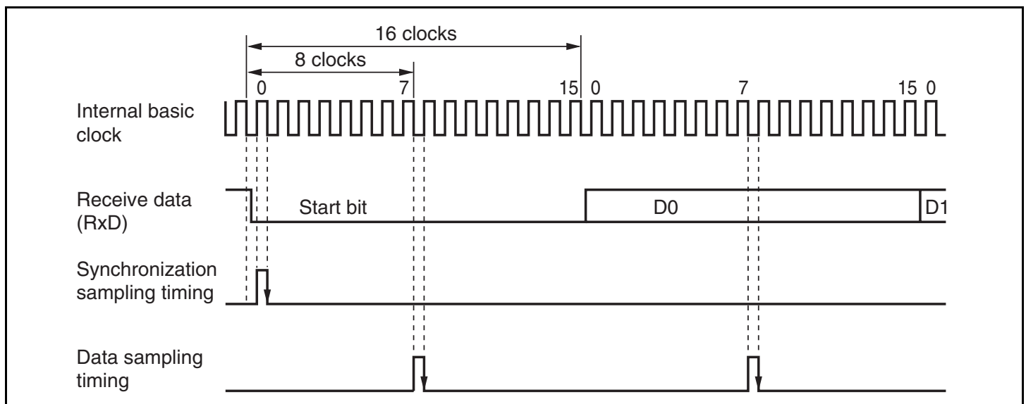
Figure 13.3 Receive Data Sampling Timing in Asynchronous Mode
