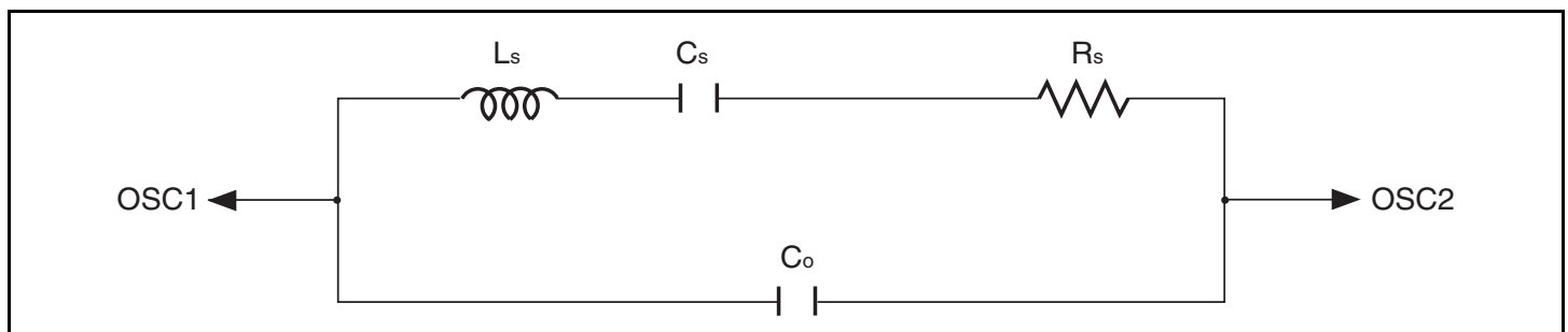
Figure 20.7 Equivalent Circuit for 32.768-kHz Crystal Resonator
