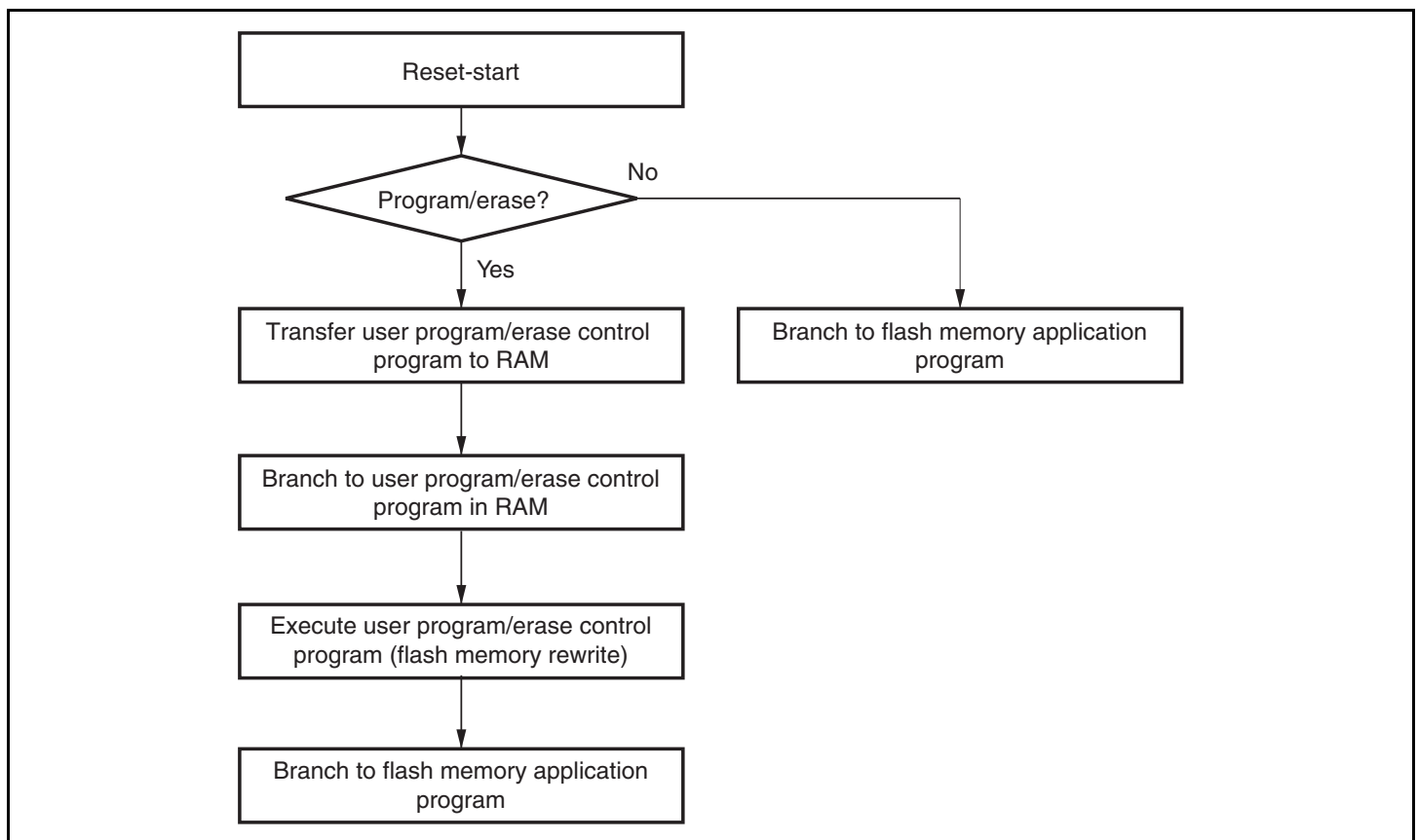
Figure 19.6 Programming/Erasing Flowchart Example in User Program Mode
