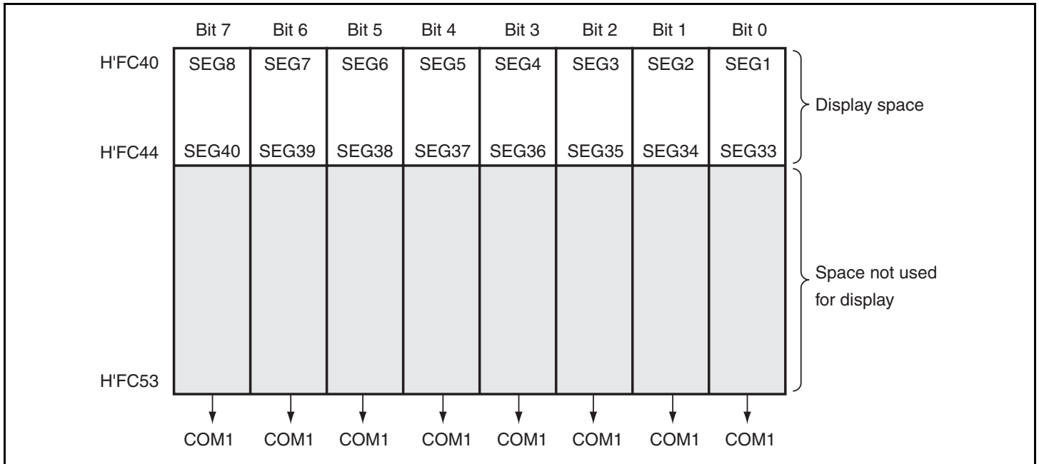
Figure 17.6 LCD RAM Map (Static Mode)
