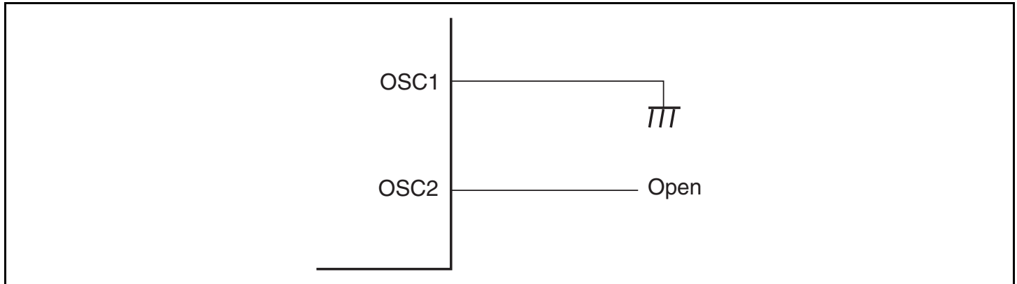
Figure 20.8 Pin Handling when Subclock is not Used
