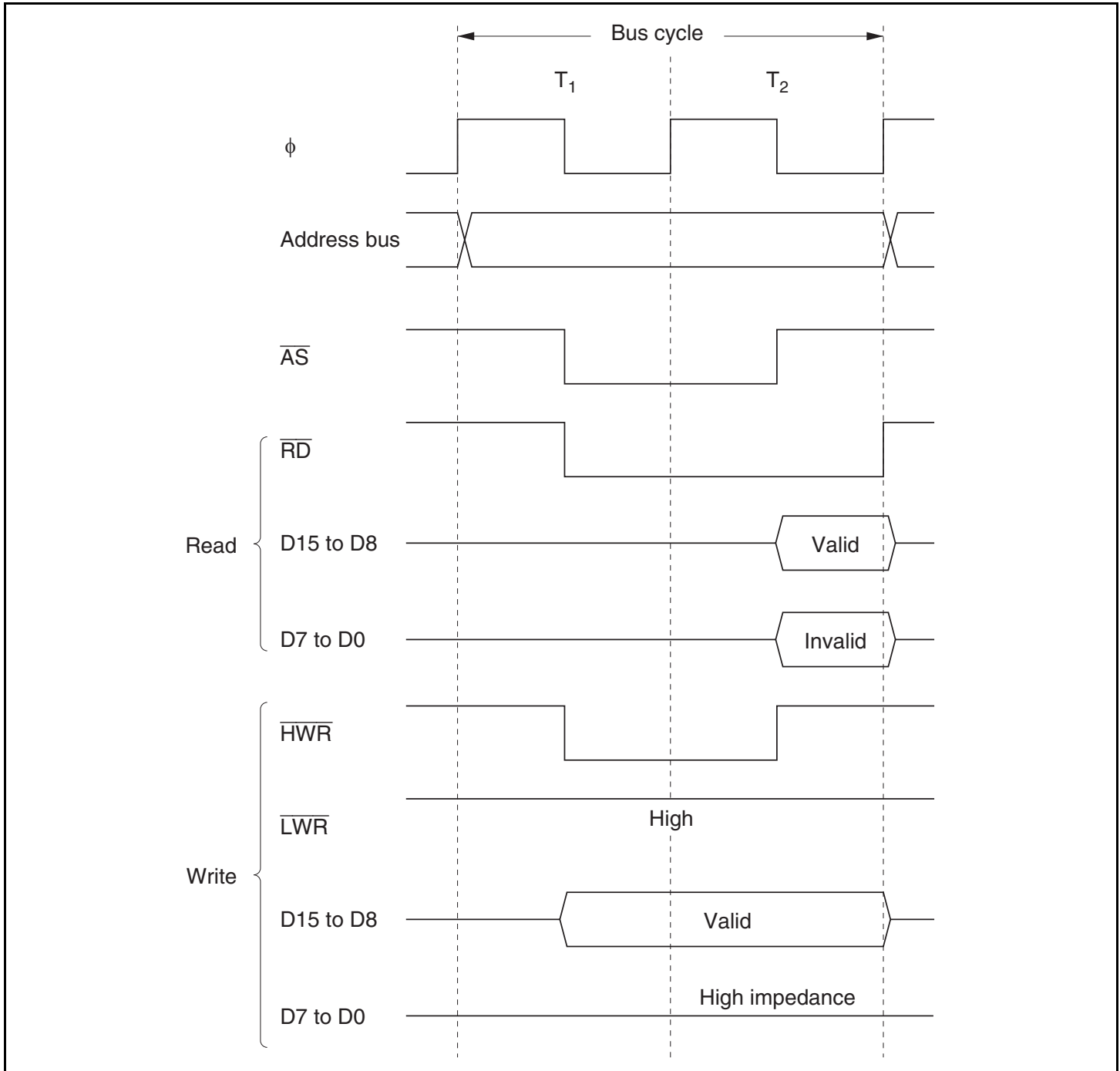
Figure 7.5 Bus Timing for 8-Bit, 2-State Access Space
