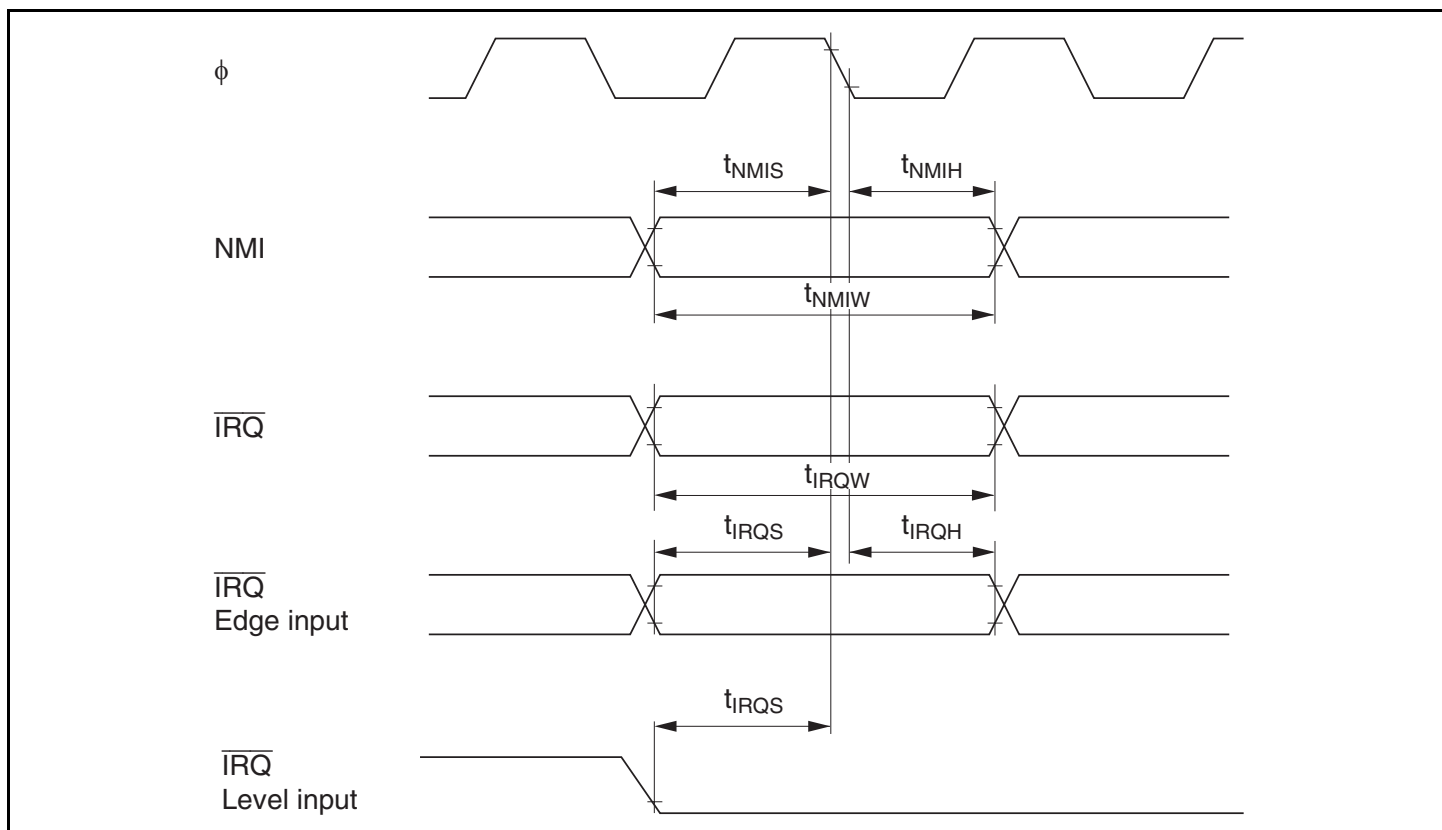
Figure 23.5 Interrupt Input Timing
