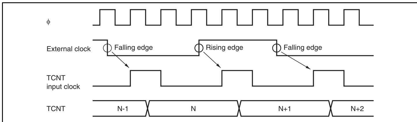
Figure 10.31 Count Timing in External Clock Operation
