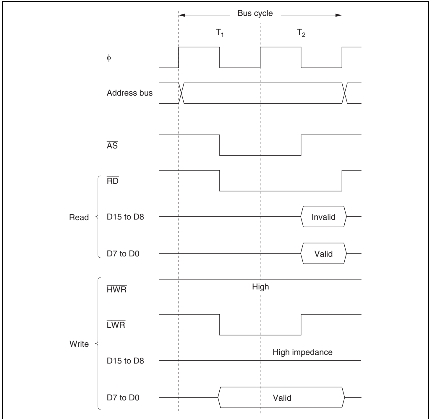
Figure 7.8 Bus Timing for 16-Bit, 2-State Access Space (Odd Address Byte Access)
