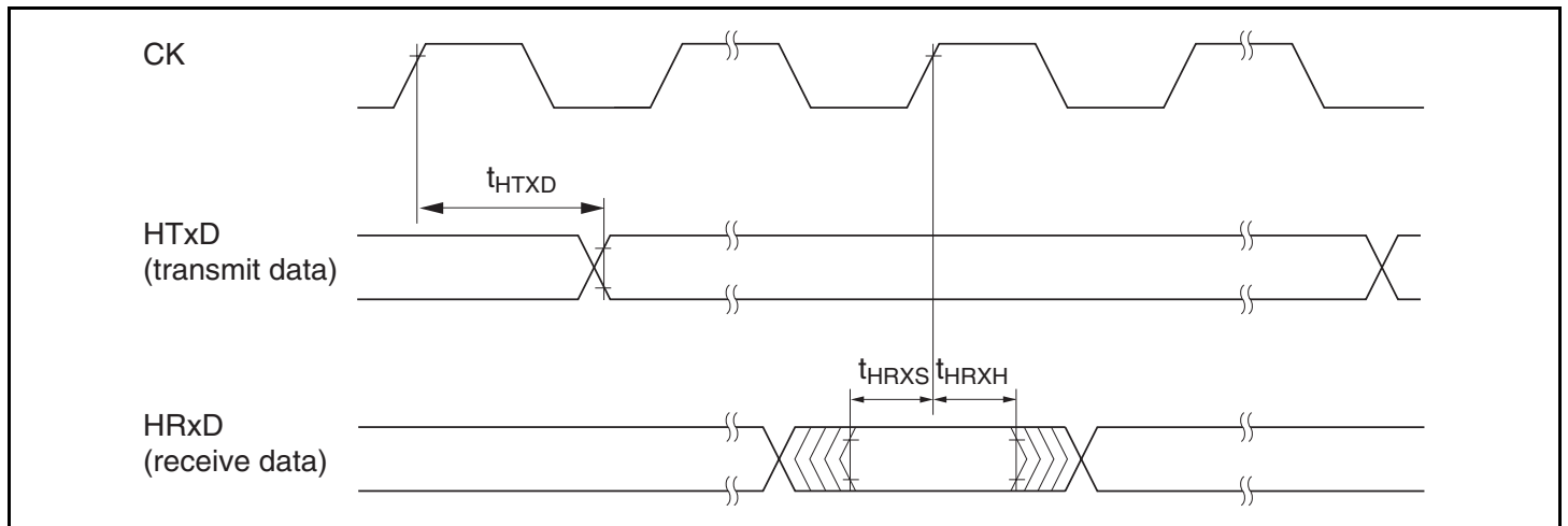
Figure 23.19 HCAN Input/Output Timing
