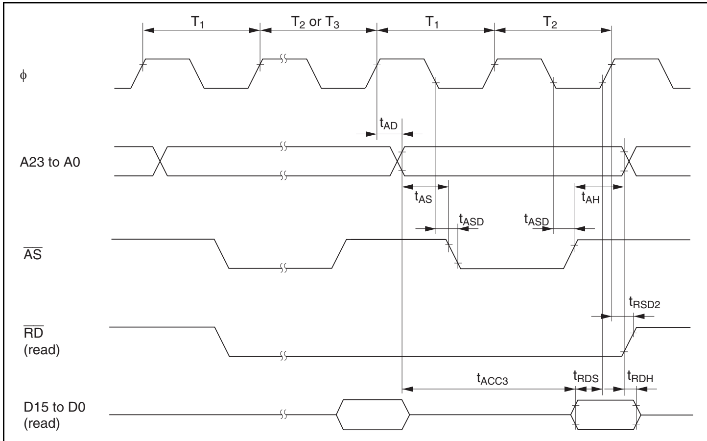
Figure 23.9 Burst ROM Access Timing (Two-State Access)
