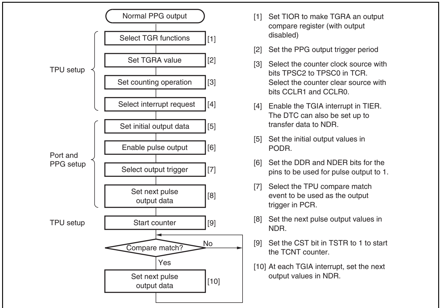
Figure 11.4 Setup Procedure for Normal Pulse Output (Example)
