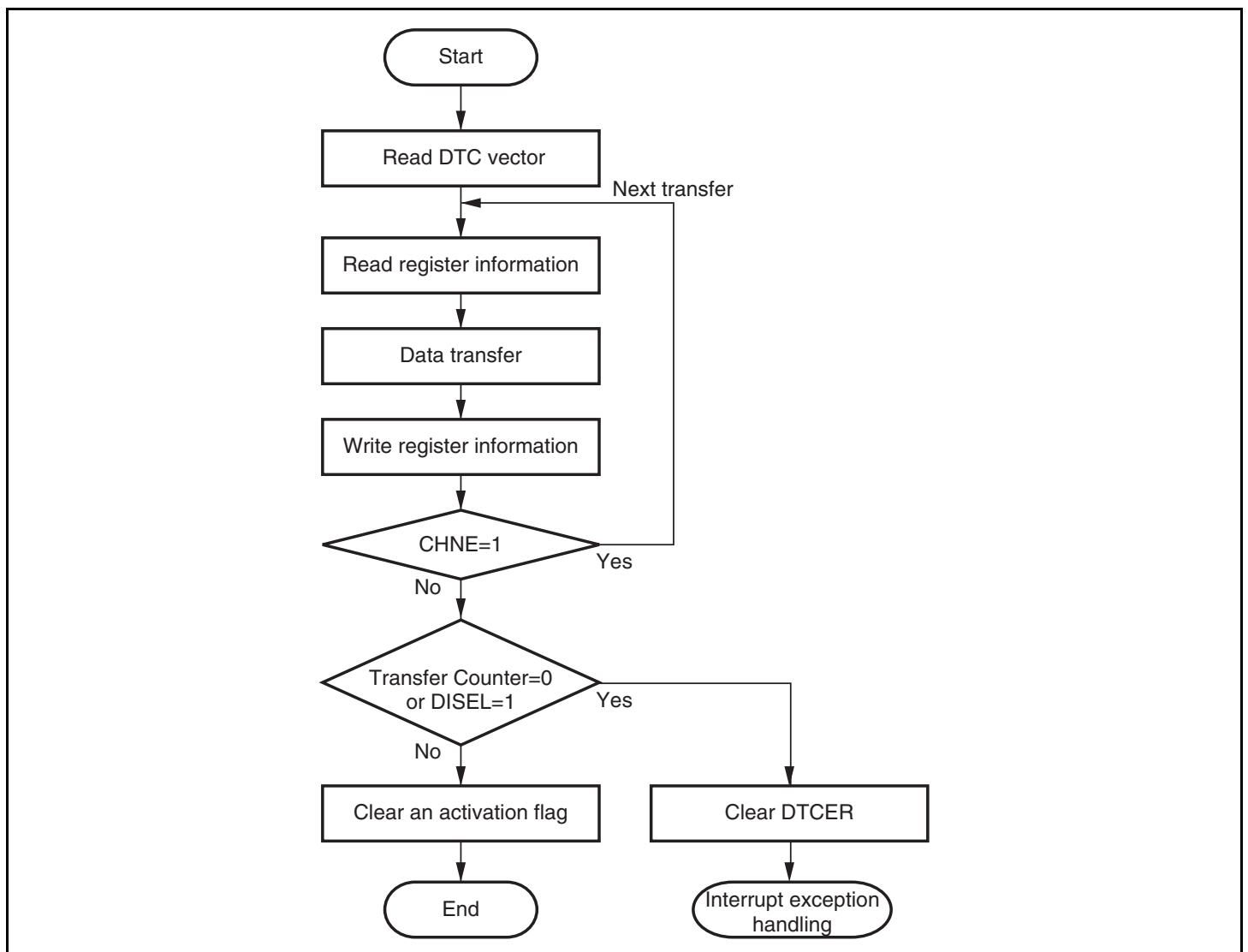
Figure 8.4 Flowchart of DTC Operation
