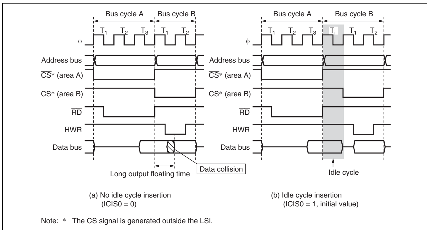
Figure 7.17 Example of Idle Cycle Operation (Write after Read)
