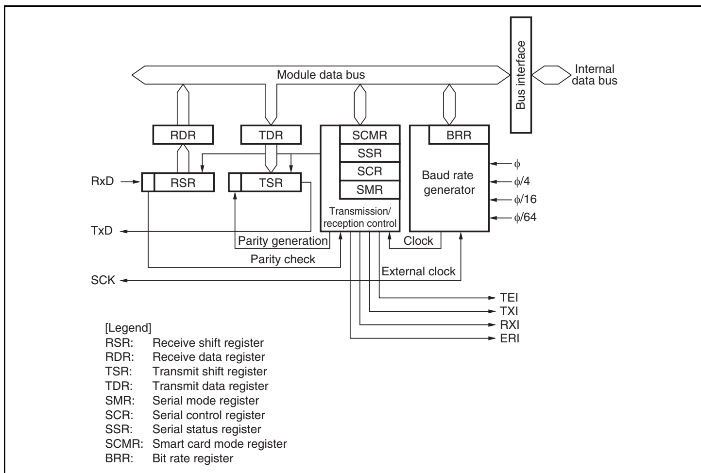
Figure 13.1 Block Diagram of SCI
