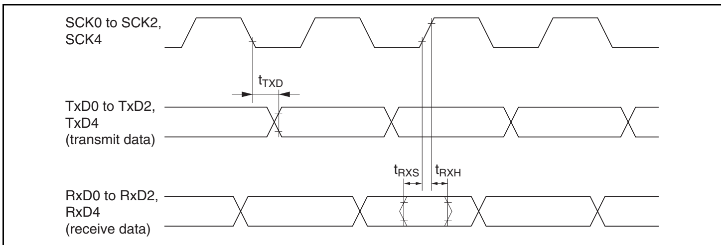
Figure 23.17 SCI Input/Output Timing (Clock Synchronous Mode)
