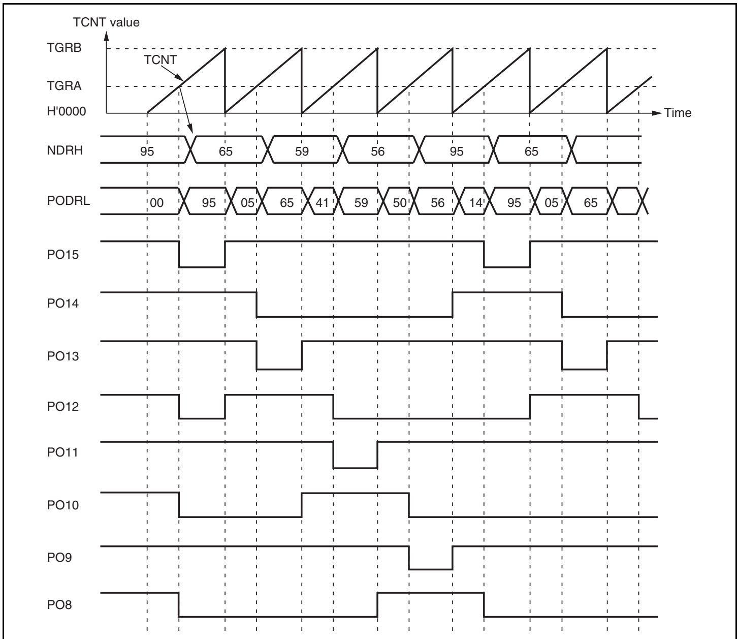
Figure 11.10 Inverted Pulse Output (Example)
