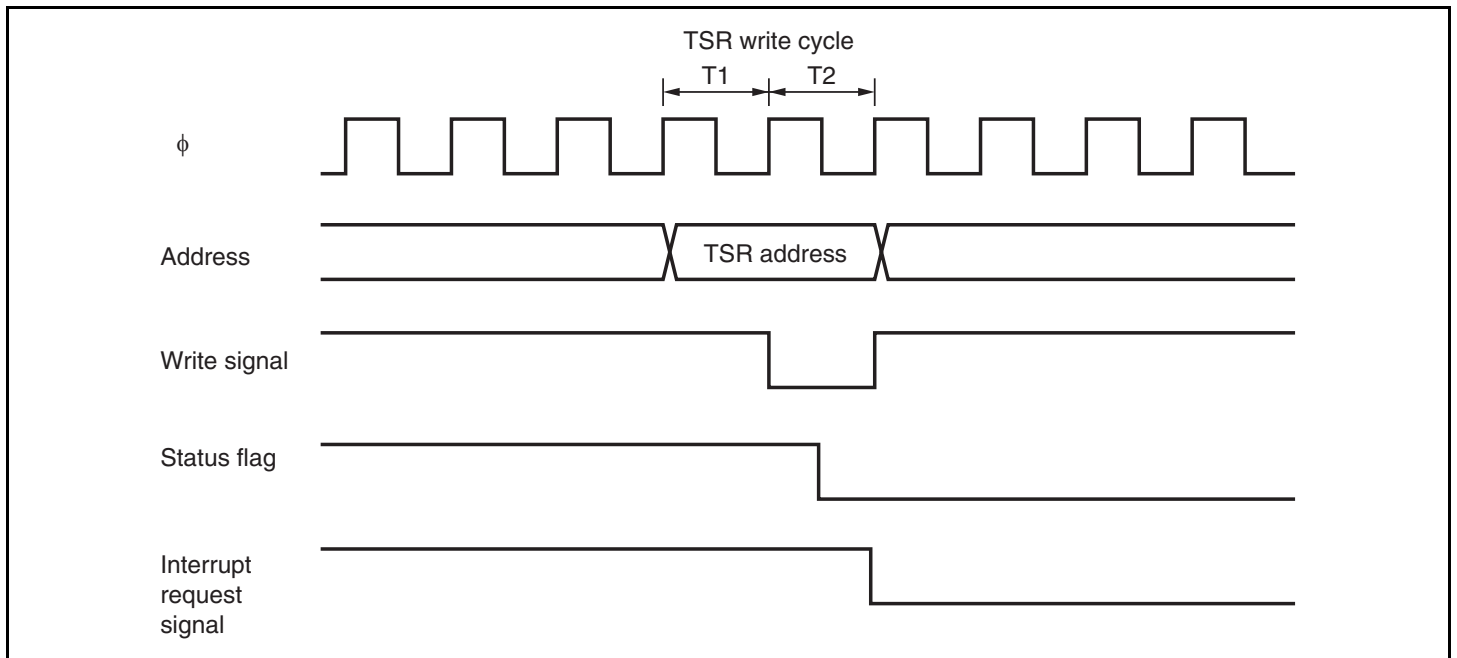
Figure 10.42 Timing for Status Flag Clearing by CPU
