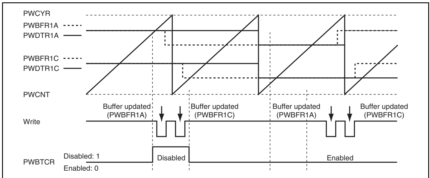
Figure 16.8 Disabling Buffer Transfer
