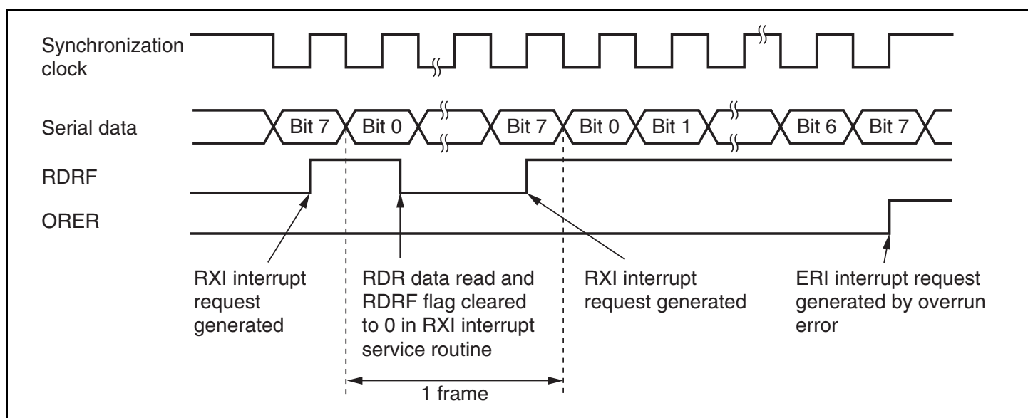
Figure 13.18 Example of SCI Operation in Reception
