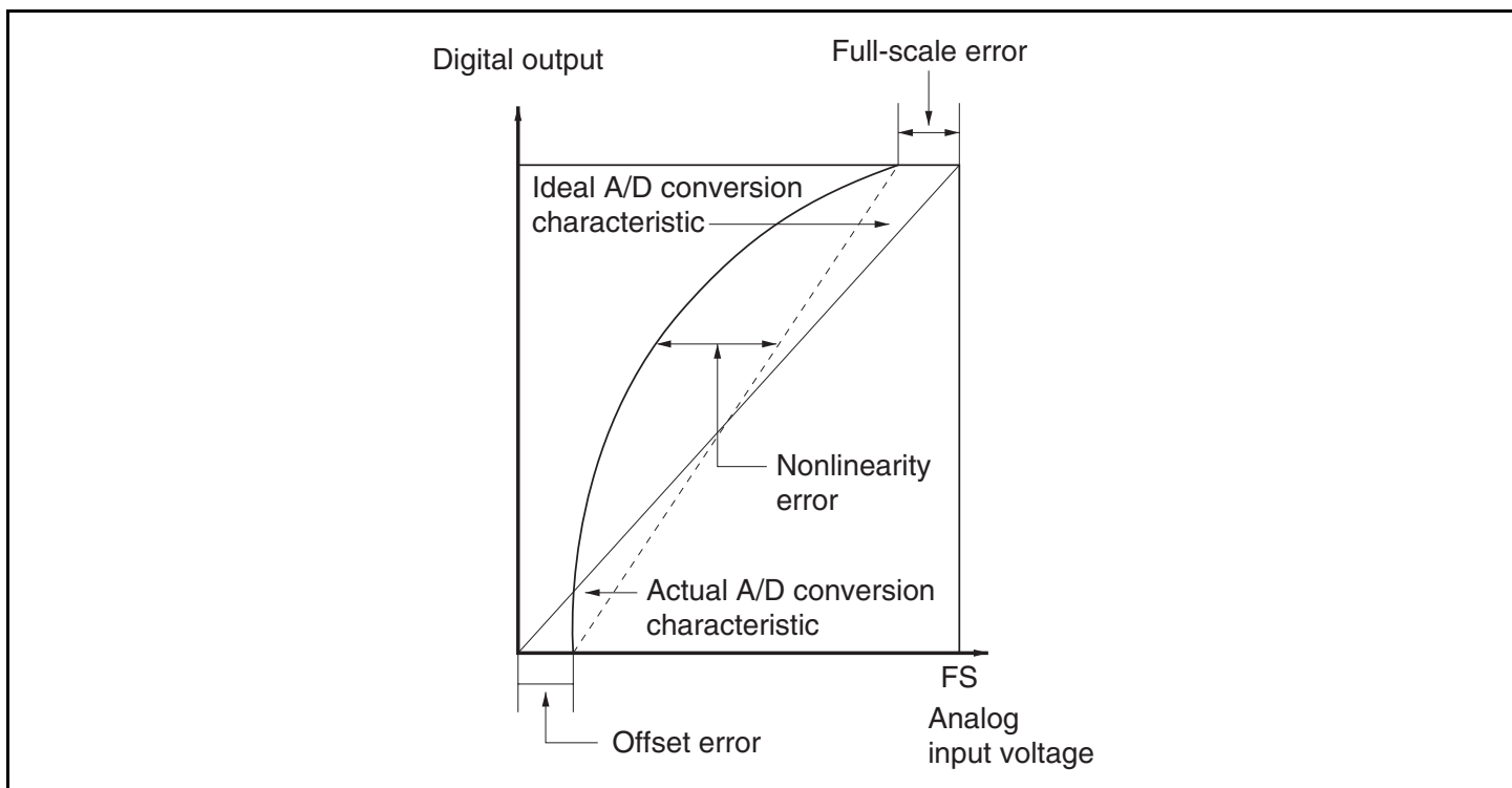
Figure 15.5 A/D Conversion Accuracy Definitions
