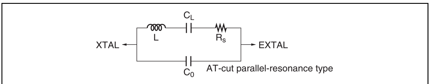
Figure 20.3 Crystal Resonator Equivalent Circuit
