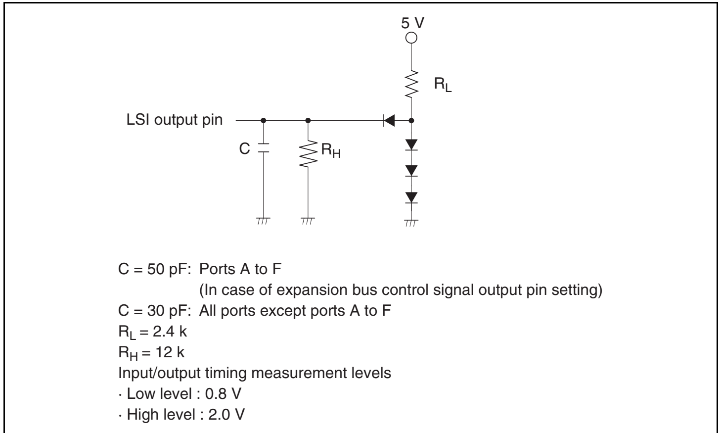
Figure 23.1 Output Load Circuit
