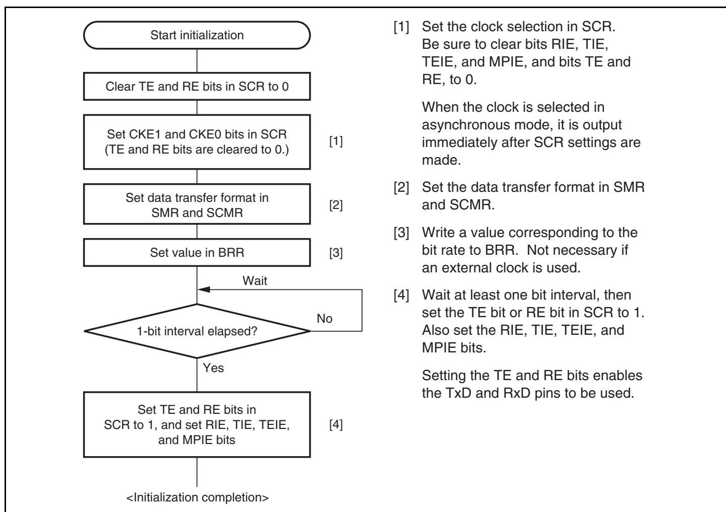
Figure 13.5 Sample SCI Initialization Flowchart
