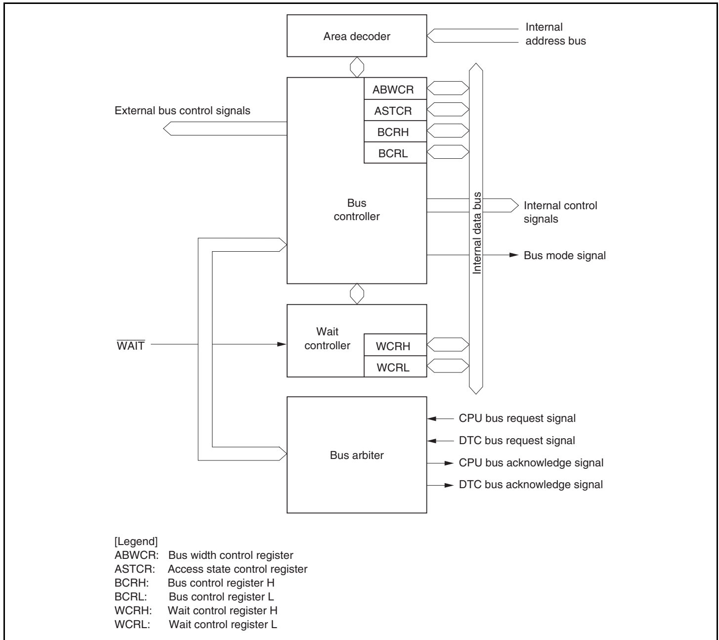
Figure 7.1 Block Diagram of Bus Controller
