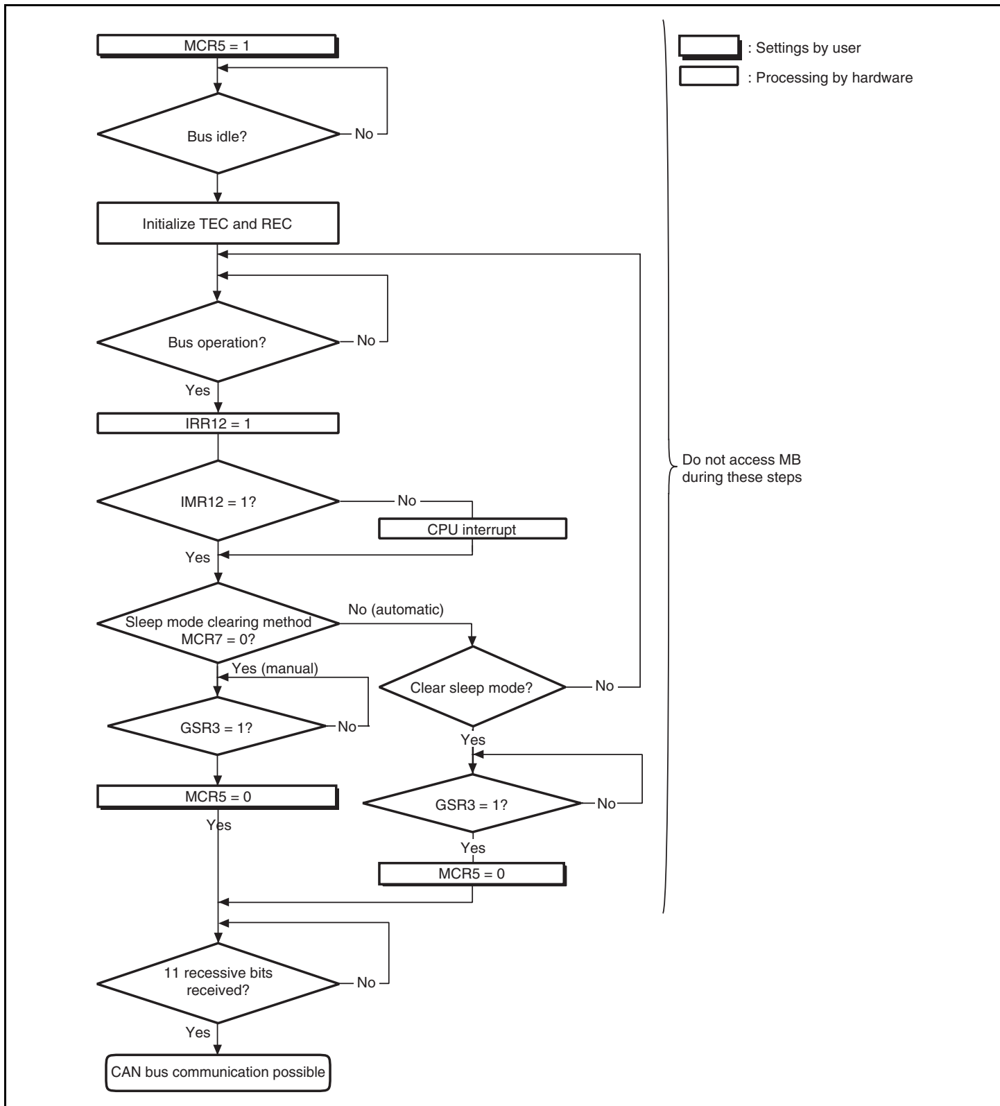
Figure 14.13 HCAN Sleep Mode Flowchart
