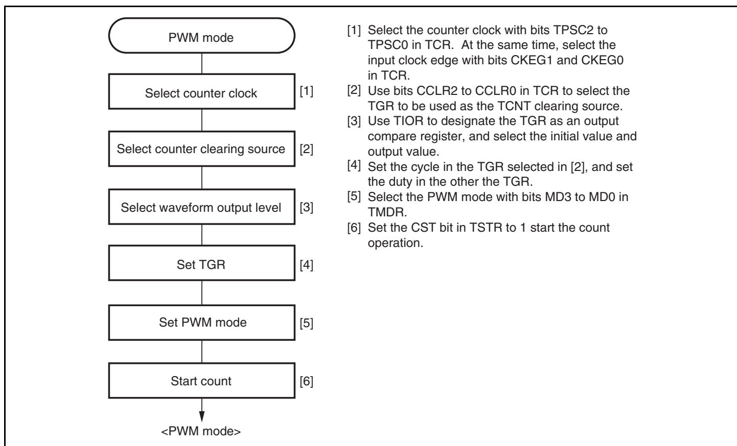
Figure 10.20 Example of PWM Mode Setting Procedure
