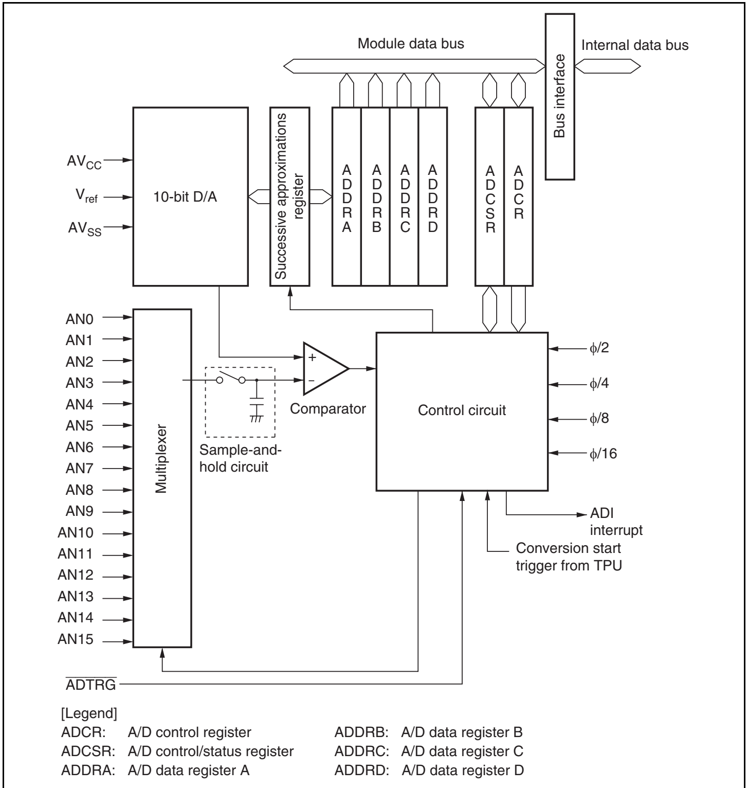
Figure 15.1 Block Diagram of A/D Converter
