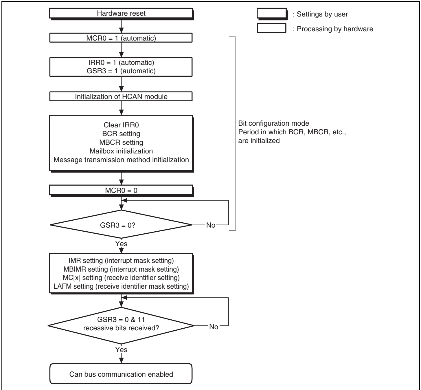
Figure 14.6 Hardware Reset Flowchart
