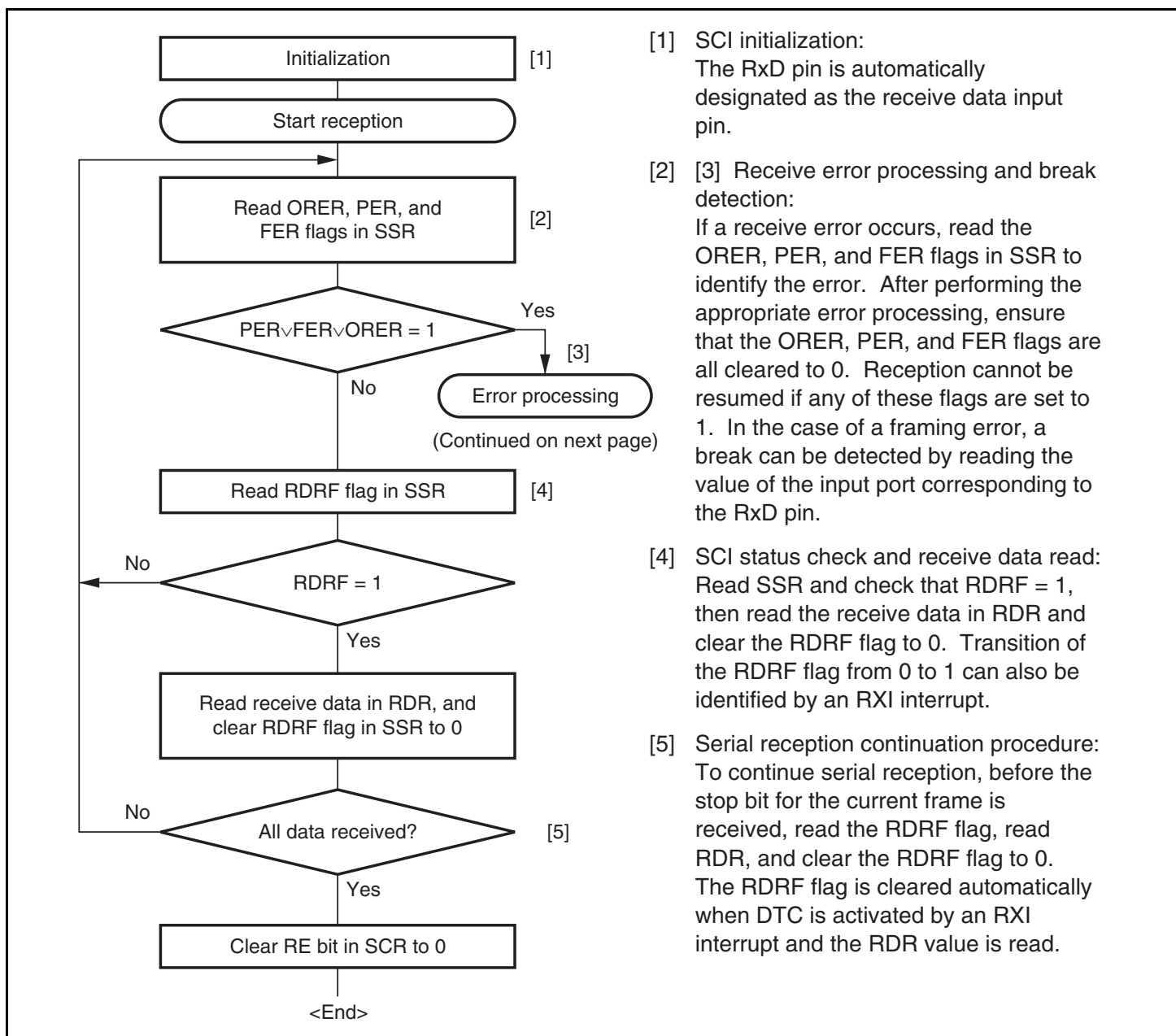
Figure 13.9 Sample Serial Reception Data Flowchart (1)
