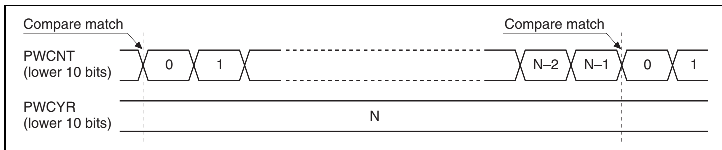
Figure 16.2 Cycle Register Compare Match
