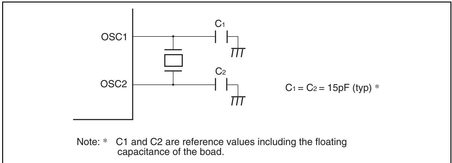
Figure 20.6 Connection Example of 32.768-kHz Crystal Resonator
