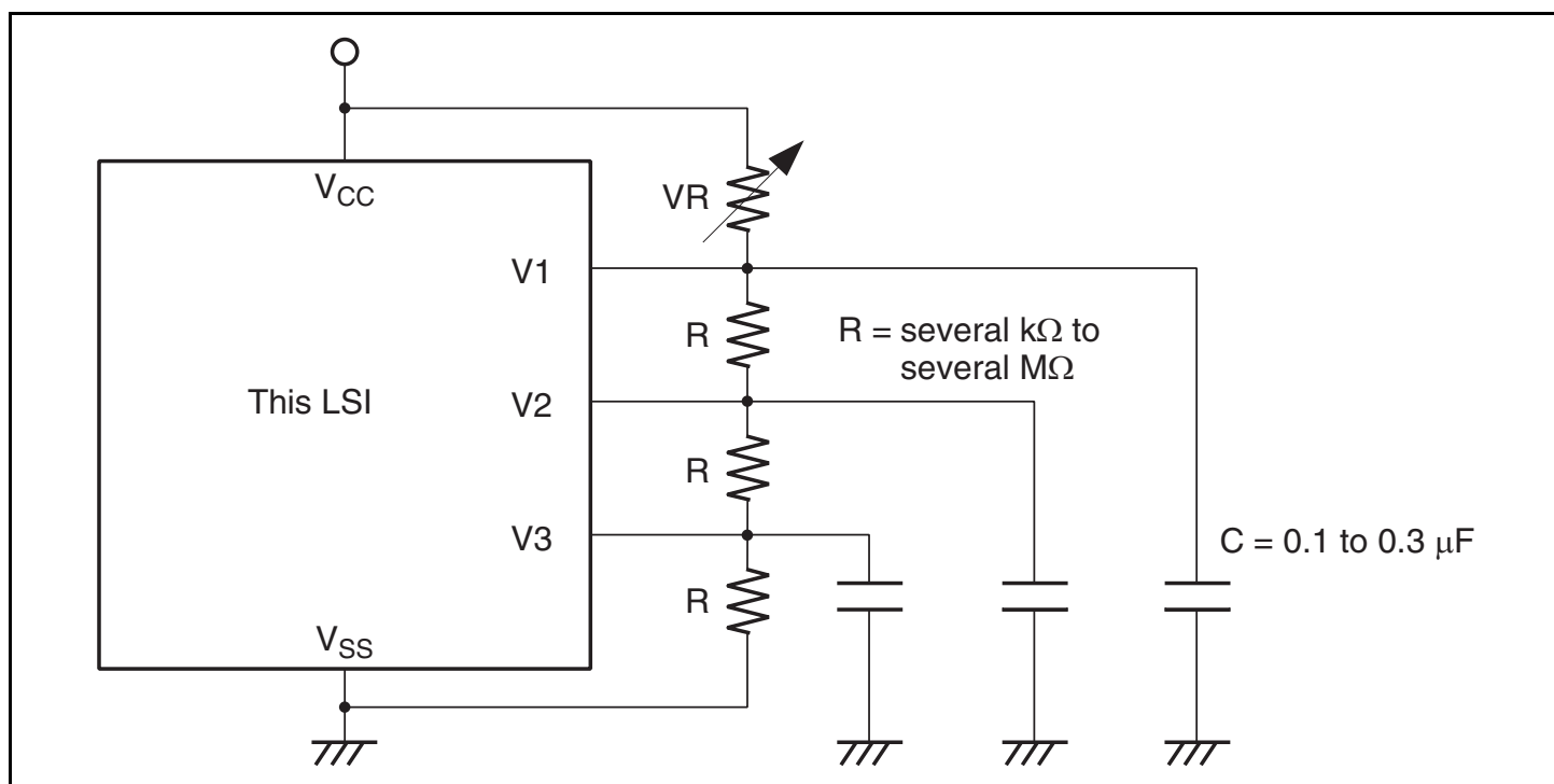
Figure 17.9 Connection of External Split-Resistance
