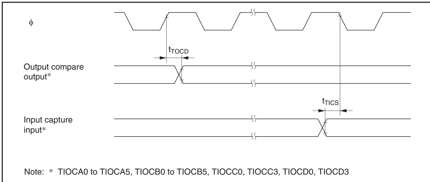
Figure 23.13 TPU Input/Output Timing
