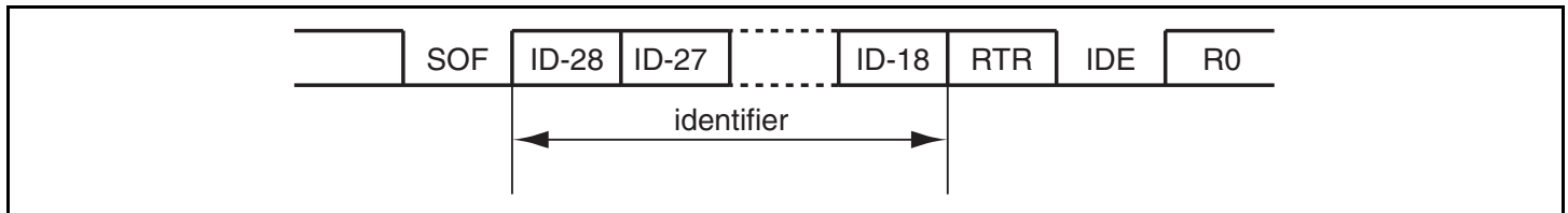
Figure 14.3 Standard Format
