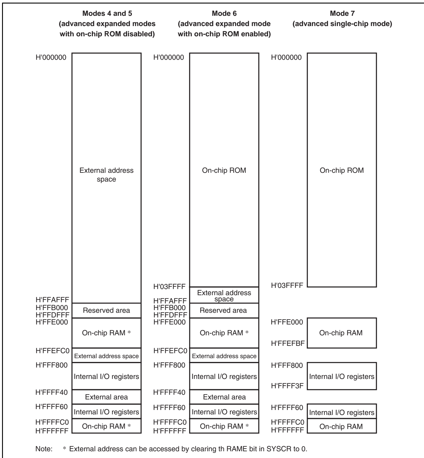
Figure 3.1 Address Map
