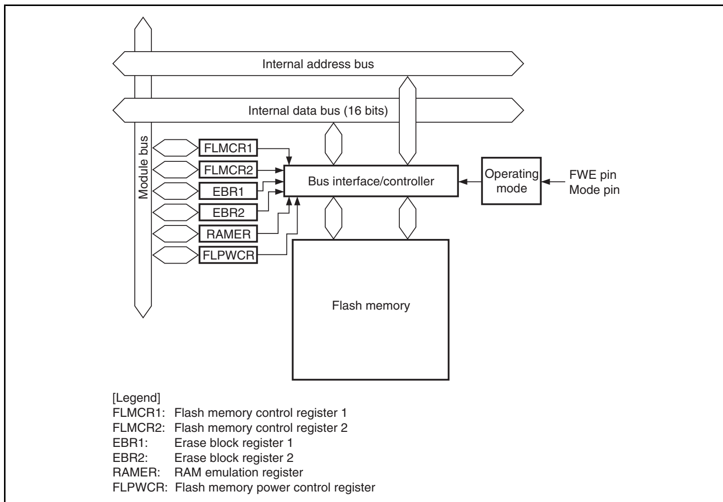
Figure 19.1 Block Diagram of Flash Memory
