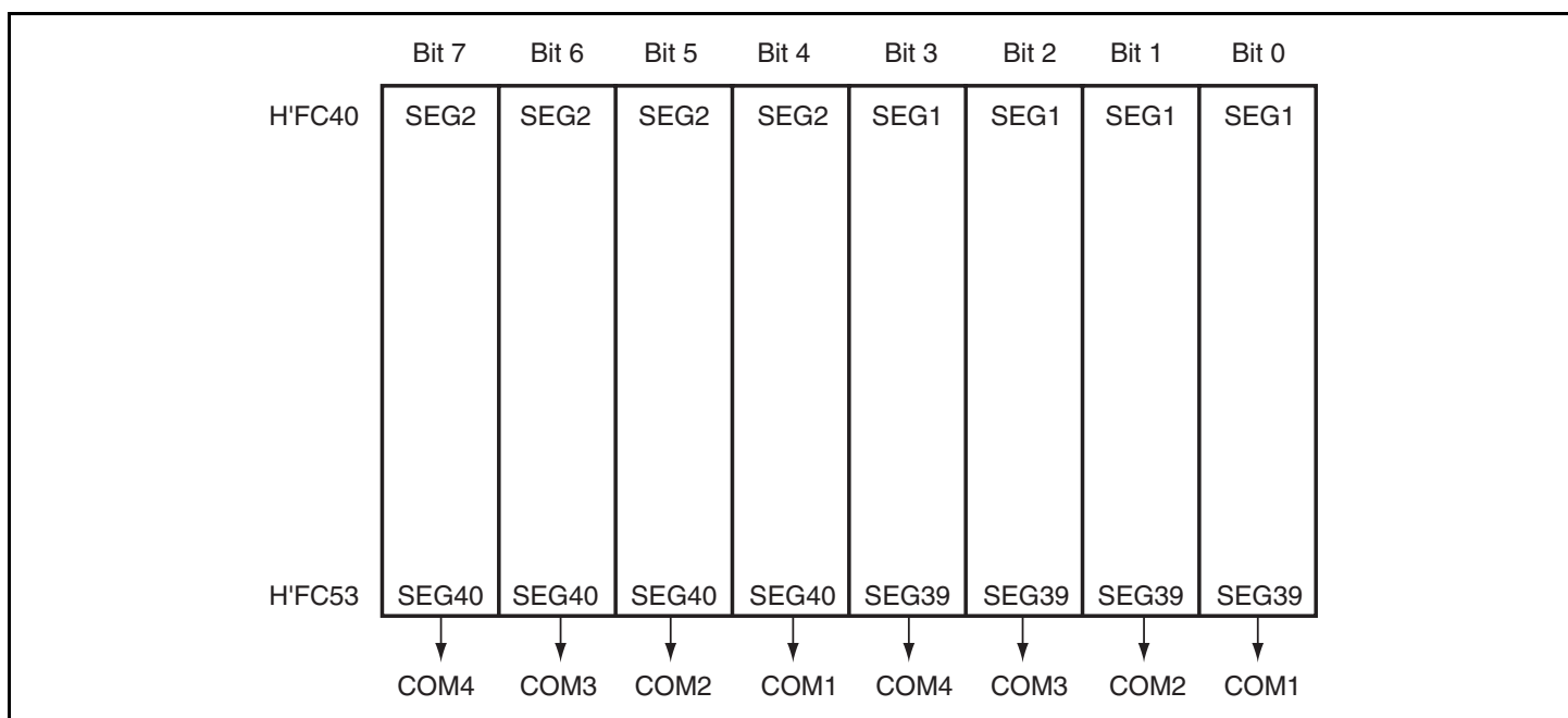
Figure 17.3 LCD RAM Map (1/4 Duty)
