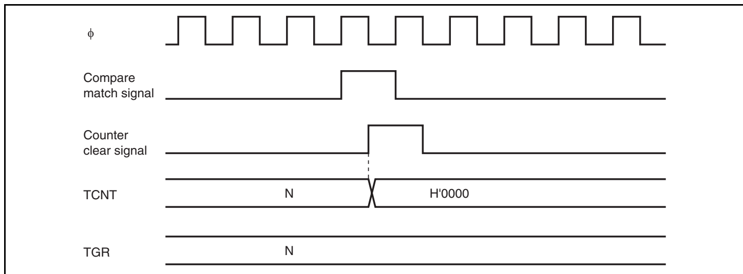
Figure 10.34 Counter Clear Timing (Compare Match)
