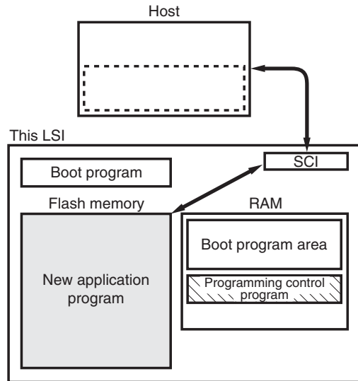
Figure 19.3 Boot Mode
