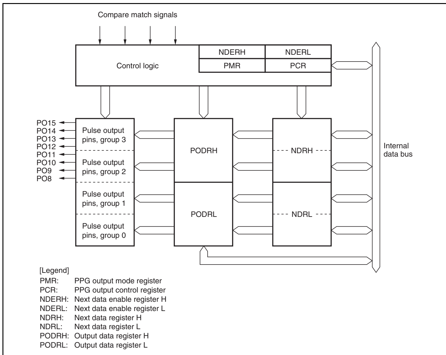
Figure 11.1 Block Diagram of PPG
