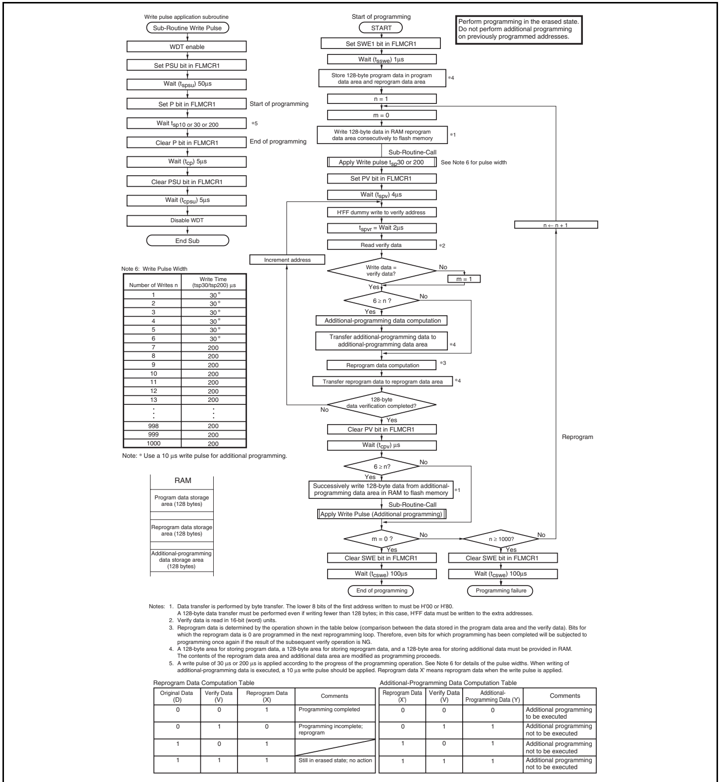
Figure 19.9 Program/Program-Verify Flowchart
