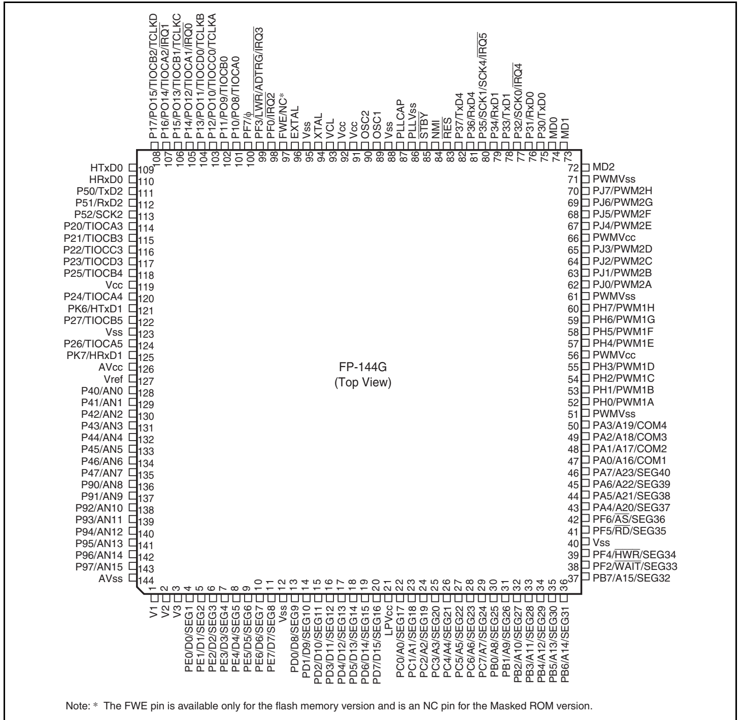
Figure 1.2 Pin Assignments (FP-144G)
