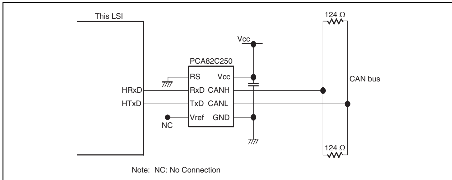
Figure 14.16 High-Speed Interface Using PCA82C250
