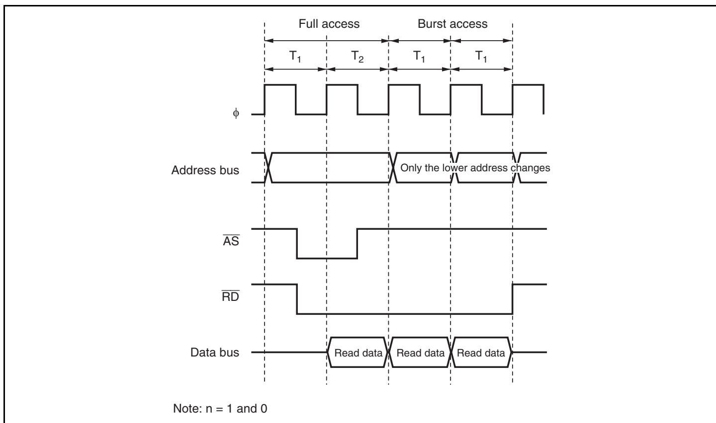
Figure 7.15 Example of Burst ROM Access Timing (AST0 = 0 and BRSTS1 = 0)
