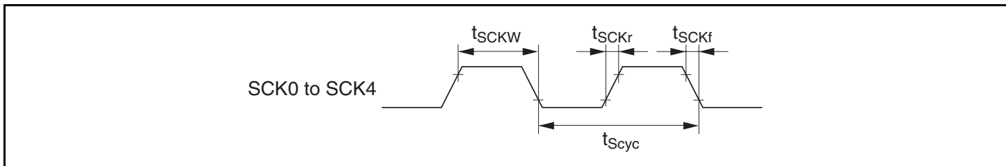
Figure 23.16 SCK Clock Input Timing
