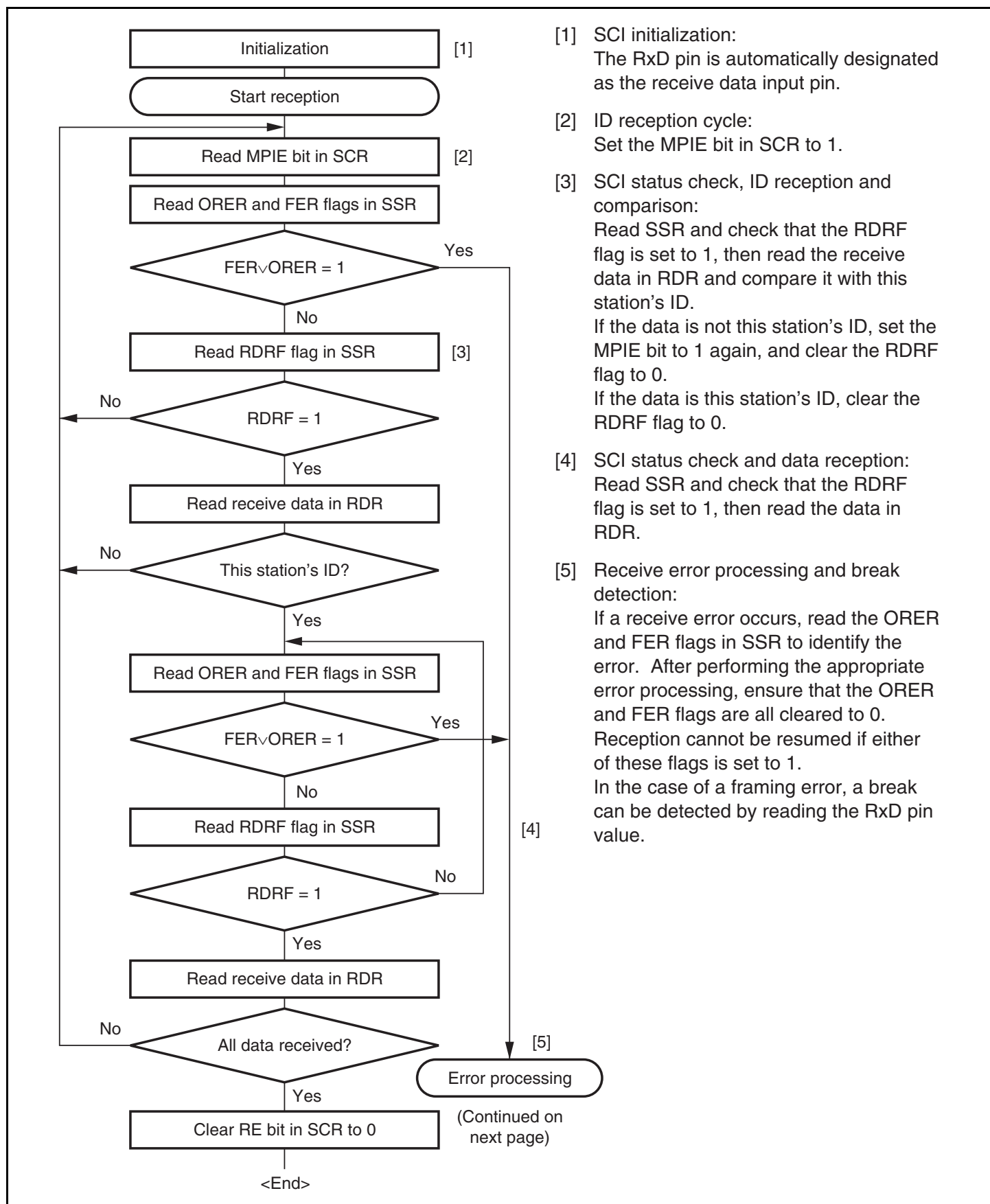
Figure 13.13 Sample Multiprocessor Serial Reception Flowchart (1)
