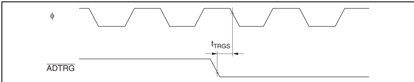
Figure 23.18 A/D Converter External Trigger Input Timing
