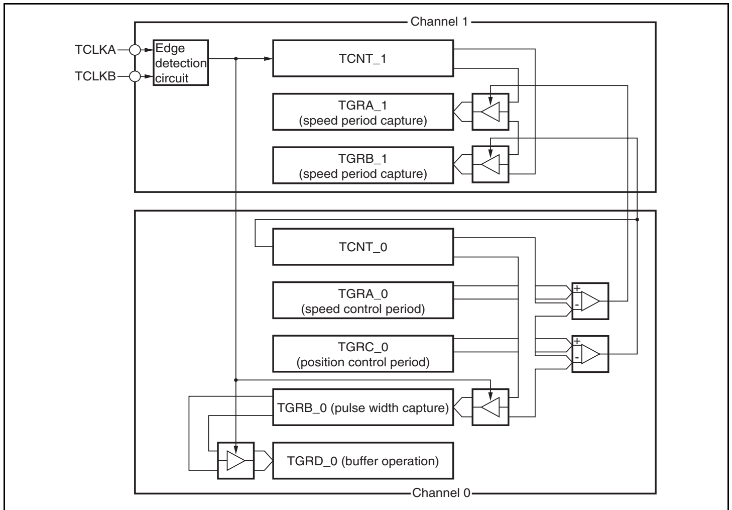
Figure 10.29 Phase Counting Mode Application Example
