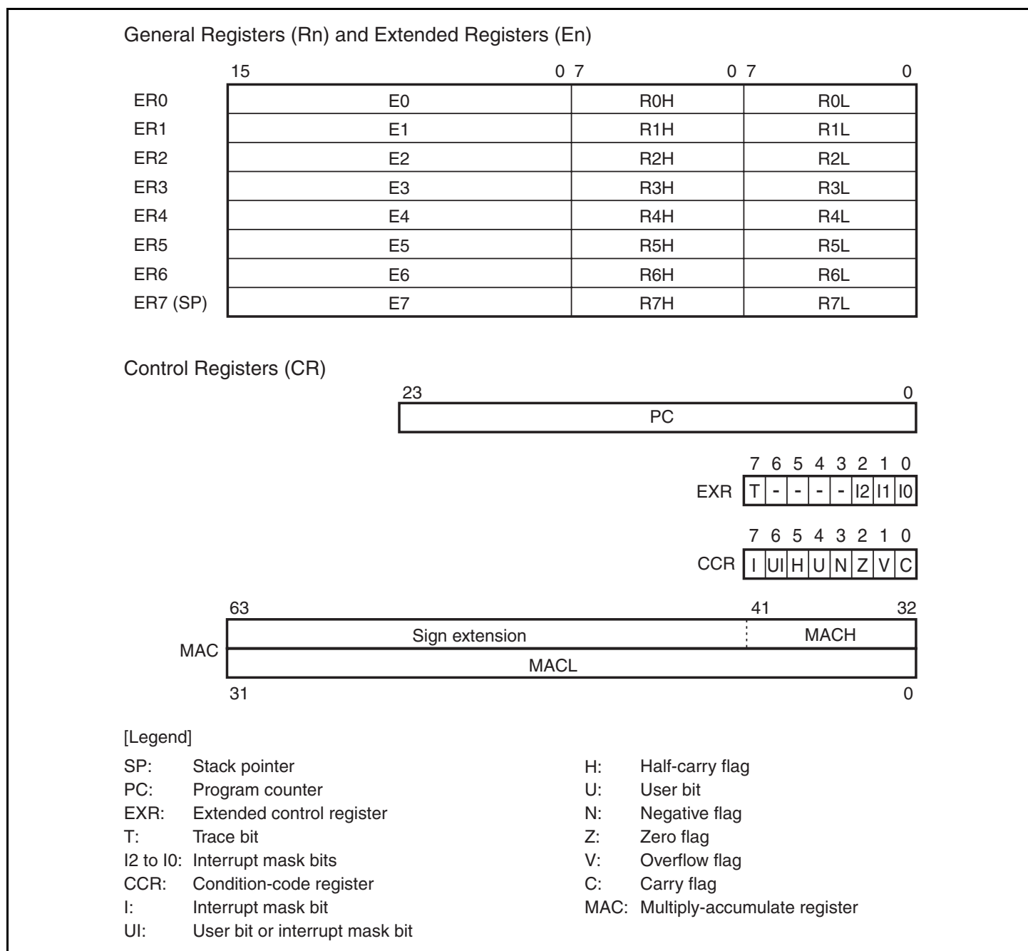
Figure 2.6 CPU Registers
