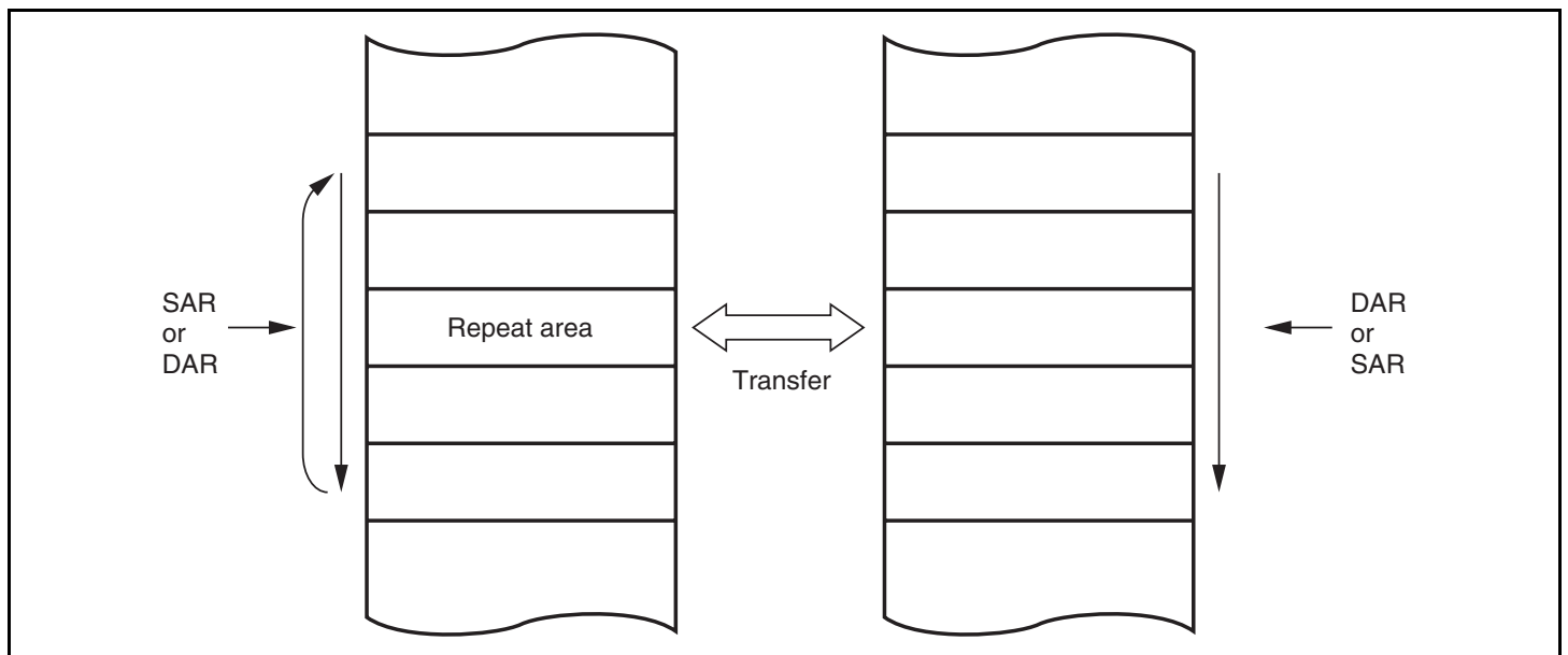
Figure 8.6 Memory Mapping in Repeat Mode
