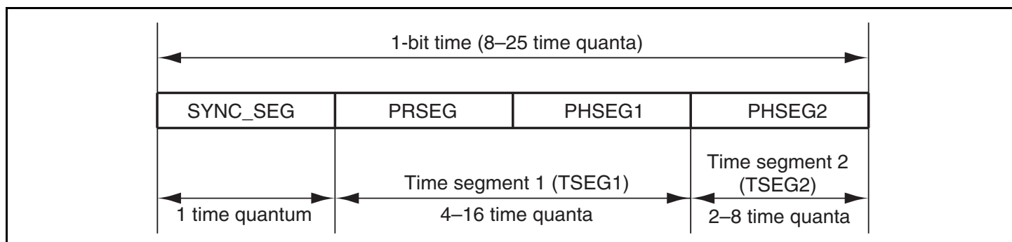
Figure 14.8 Detailed Description of One-Bit Time
