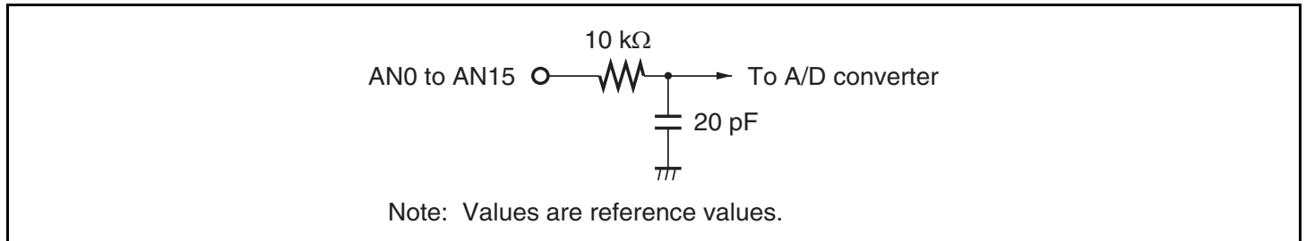
Figure 15.8 Analog Input Pin Equivalent Circuit
