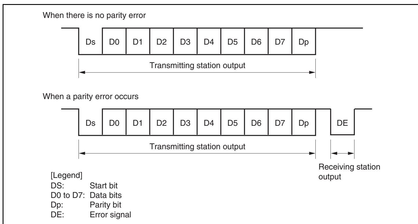
Figure 13.22 Normal Smart Card Interface Data Format
