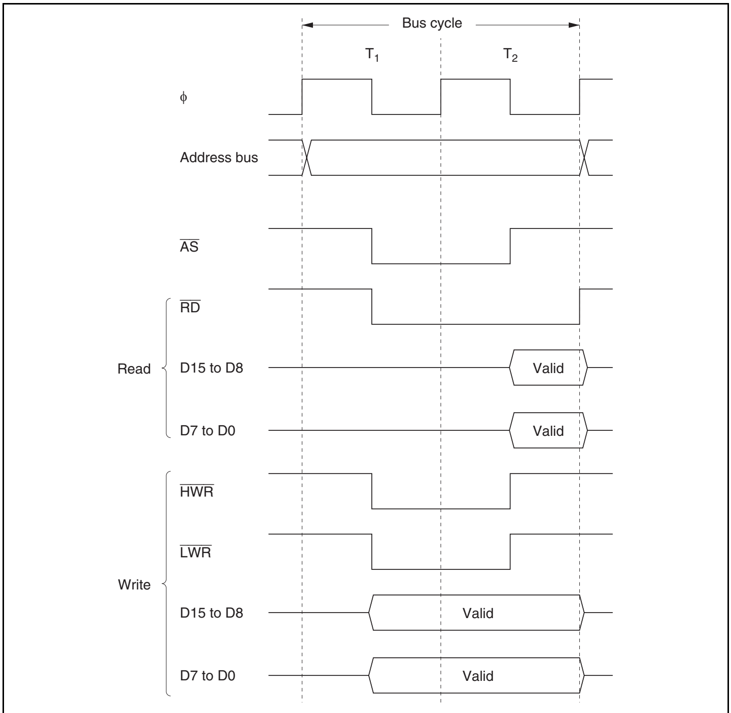
Figure 7.9 Bus Timing for 16-Bit, 2-State Access Space (Word Access)
