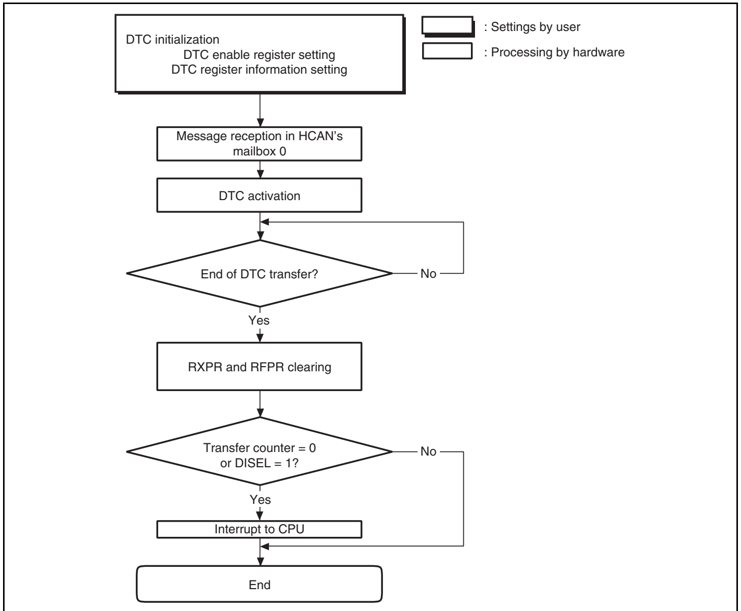
Figure 14.15 DTC Transfer Flowchart
