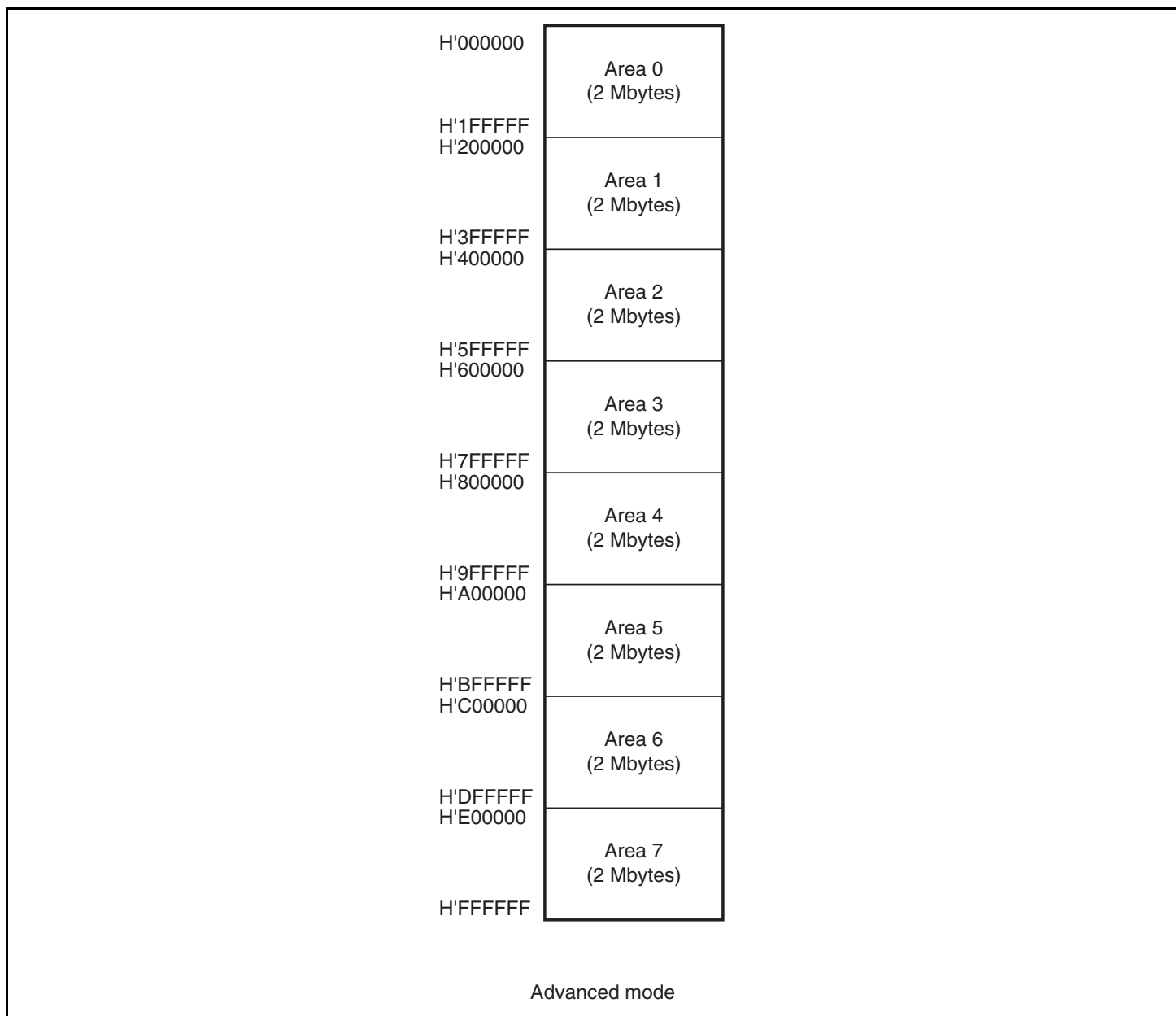
Figure 7.2 Area Divisions
