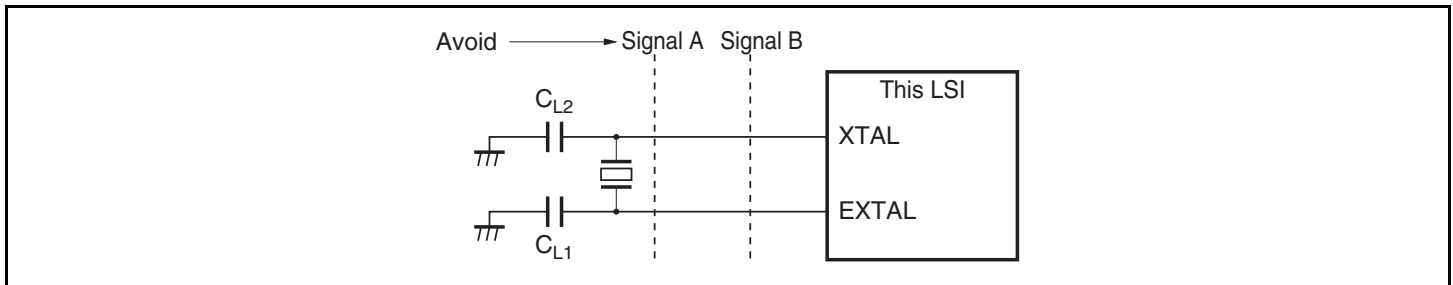
Figure 20.9 Note on Board Design of Oscillator Circuit
