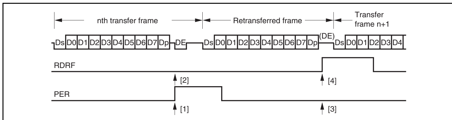
Figure 13.29 Retransfer Operation in SCI Receive Mode
