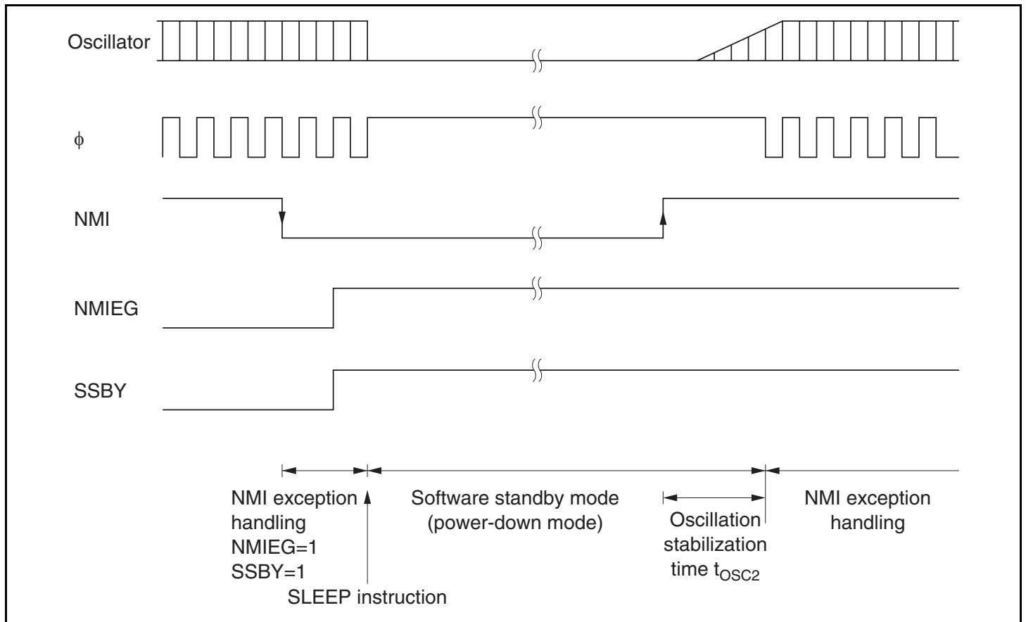
Figure 21.3 Software Standby Mode Application Example
