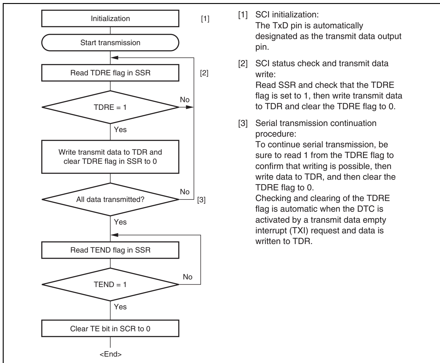
Figure 13.17 Sample Serial Transmission Flowchart
