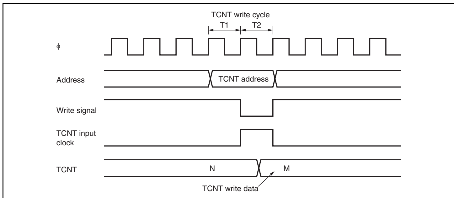
Figure 10.46 Conflict between TCNT Write and Increment Operations
