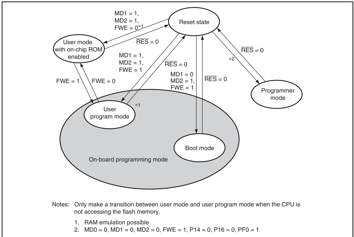
Figure 19.2 Flash Memory State Transitions
