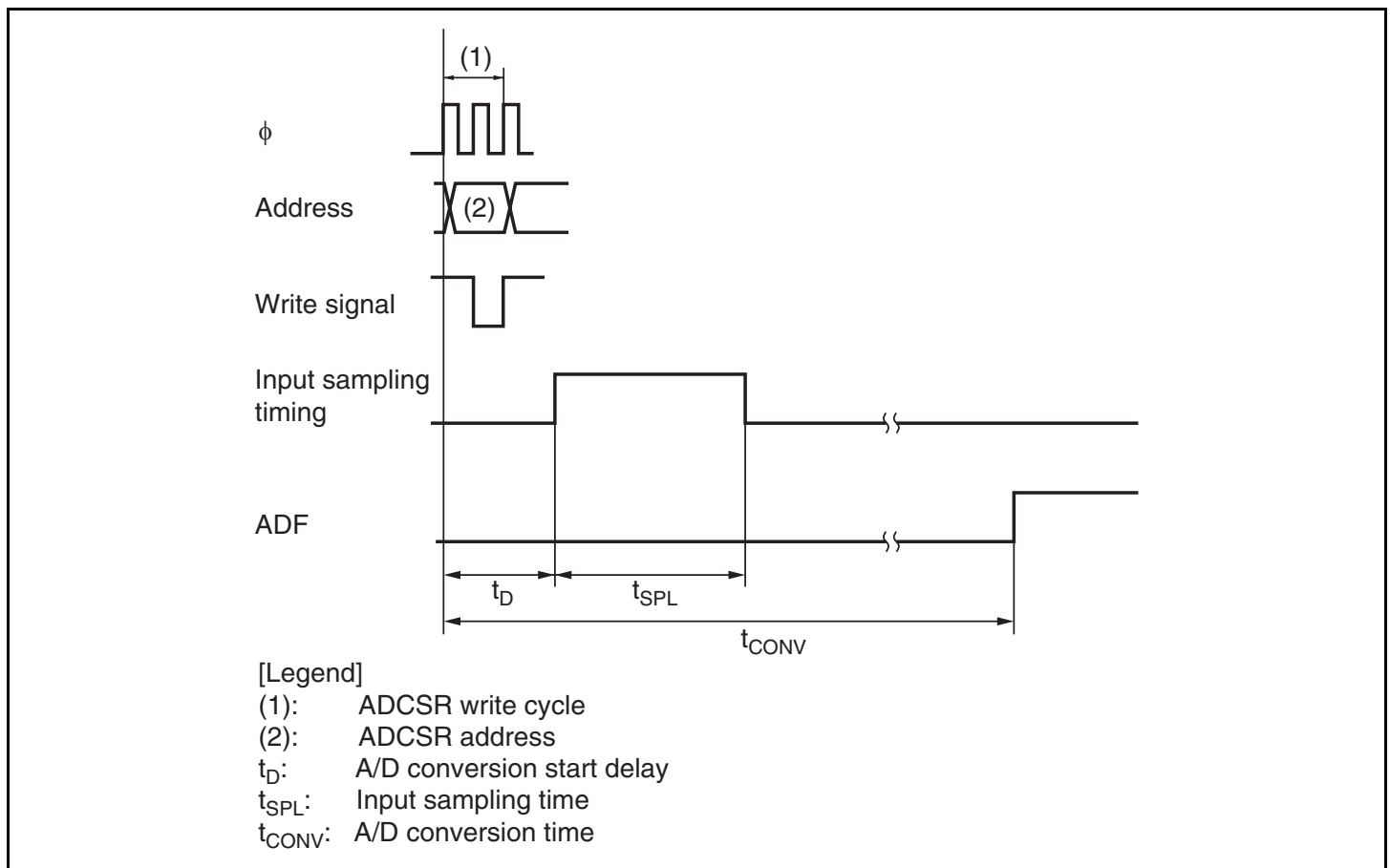
Figure 15.2 A/D Conversion Timing
