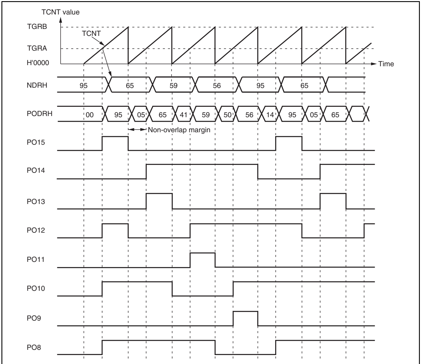
Figure 11.9 Non-Overlapping Pulse Output Example (Four-Phase Complementary)
