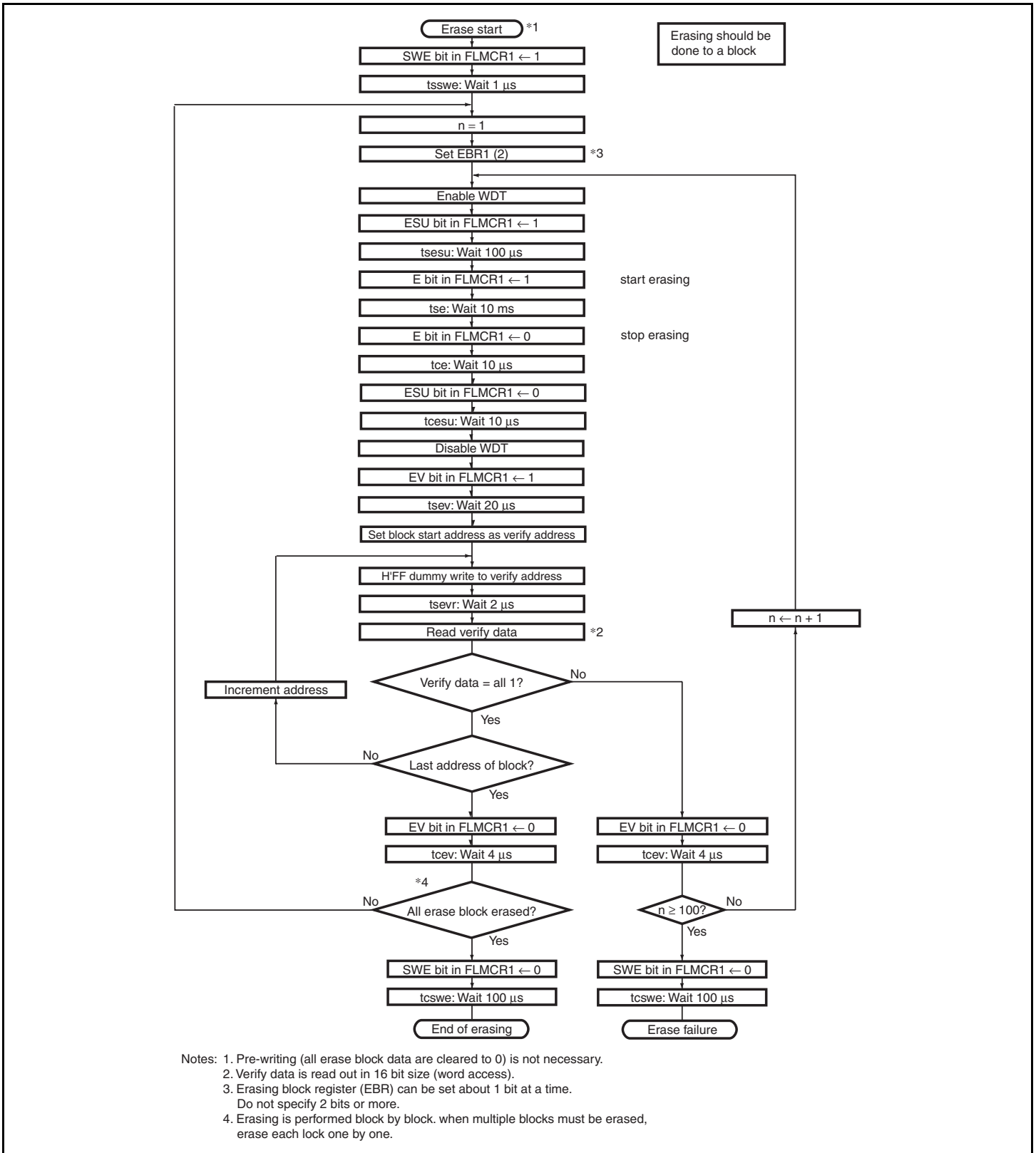
Figure 19.10 Erase/Erase-Verify Flowchart
