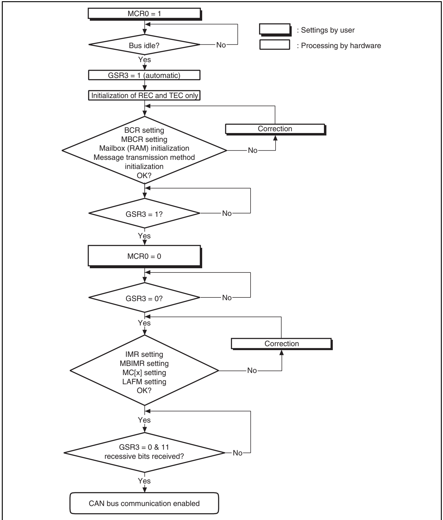
Figure 14.7 Software Reset Flowchart
