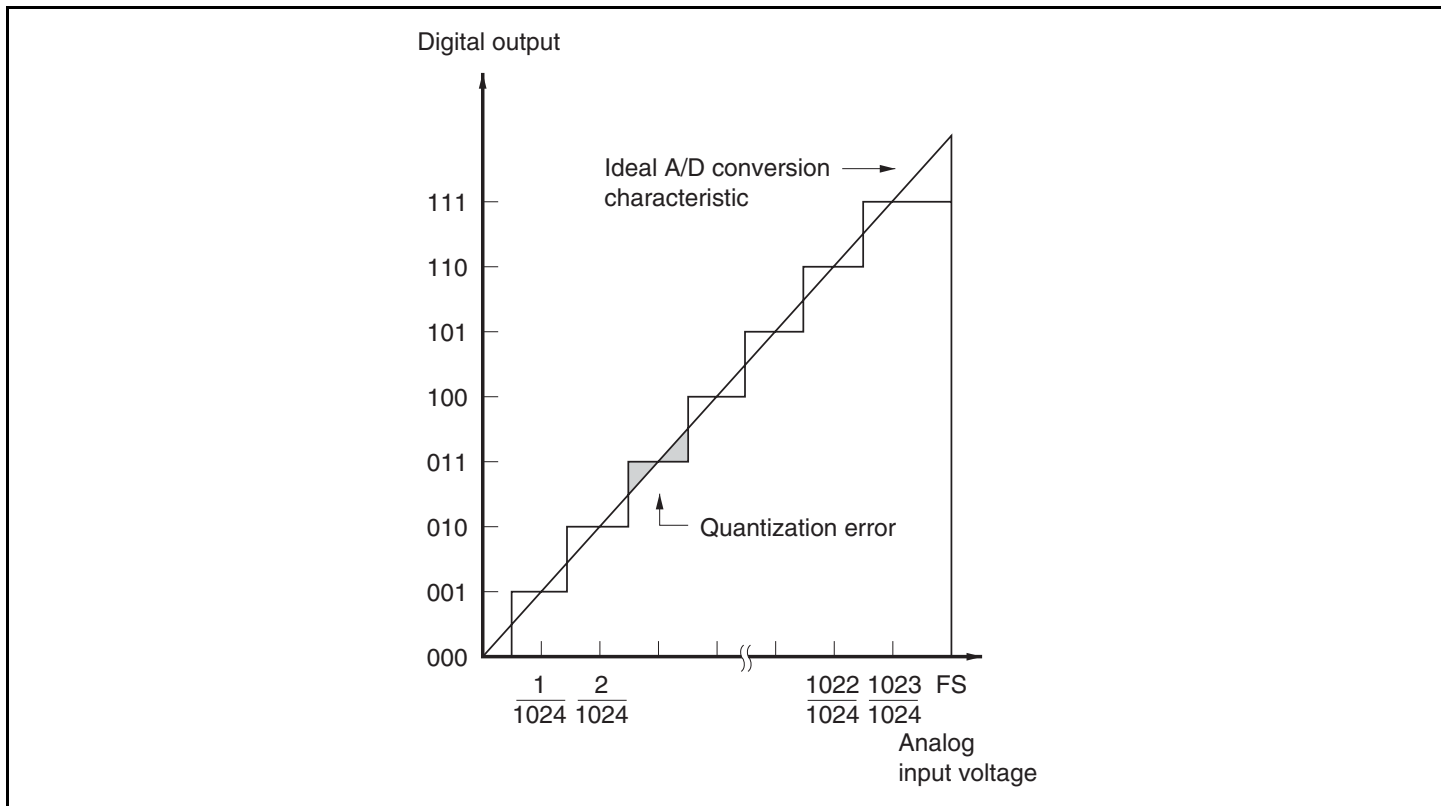
Figure 15.4 A/D Conversion Accuracy Definitions
