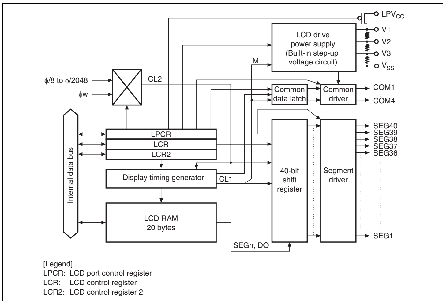
Figure 17.1 Block Diagram of LCD Controller/Driver
