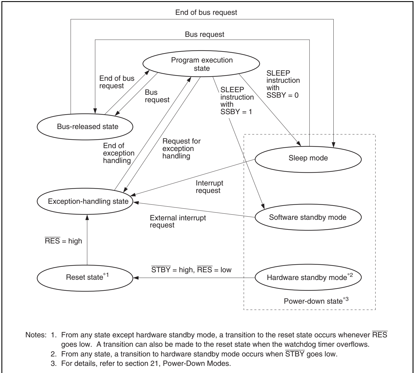
Figure 2.13 State Transitions
