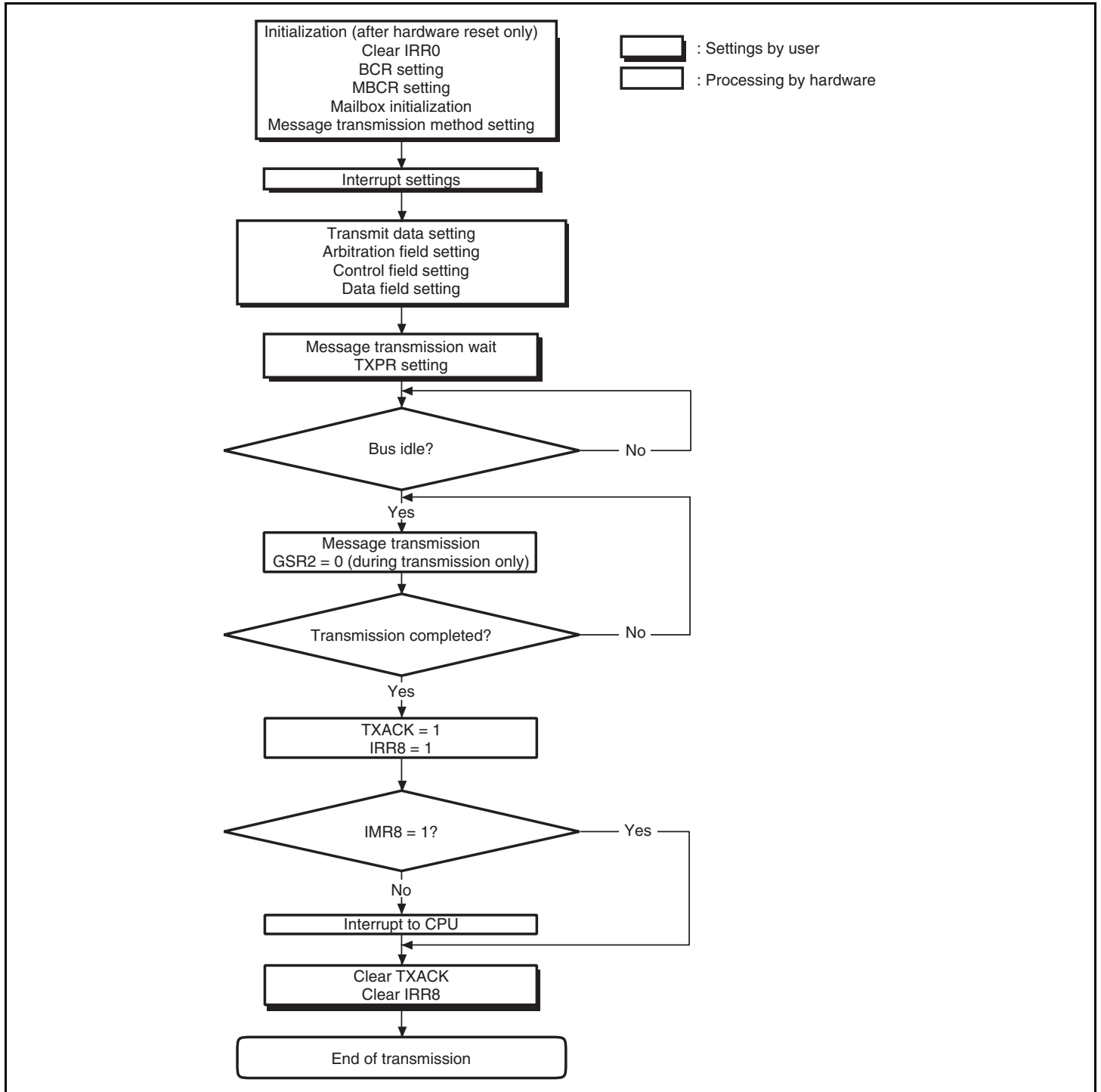
Figure 14.9 Transmission Flowchart
