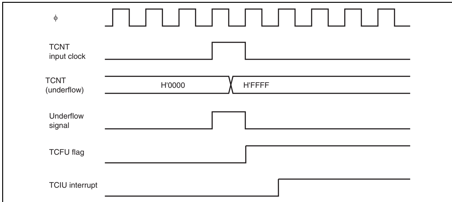
Figure 10.41 TCIU Interrupt Setting Timing
