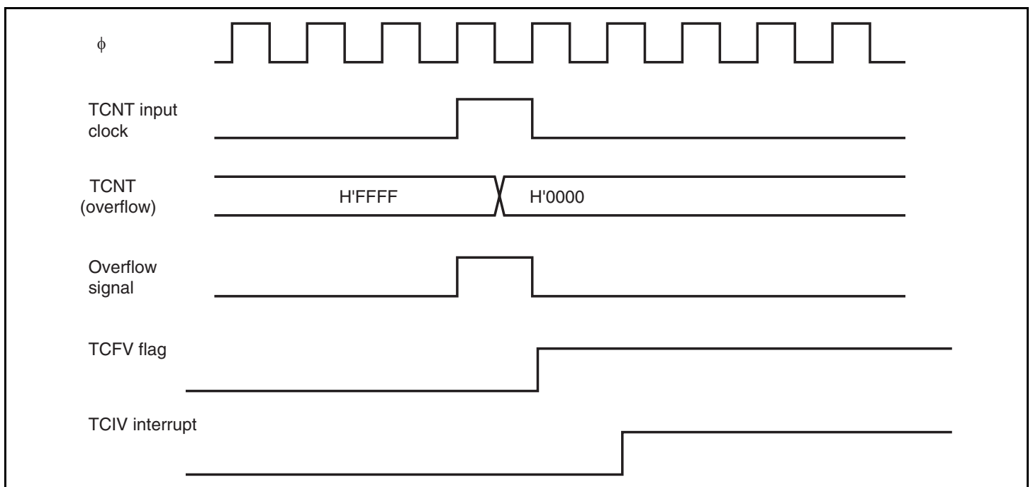
Figure 10.40 TCIV Interrupt Setting Timing
