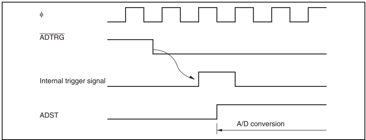
Figure 15.3 External Trigger Input Timing
