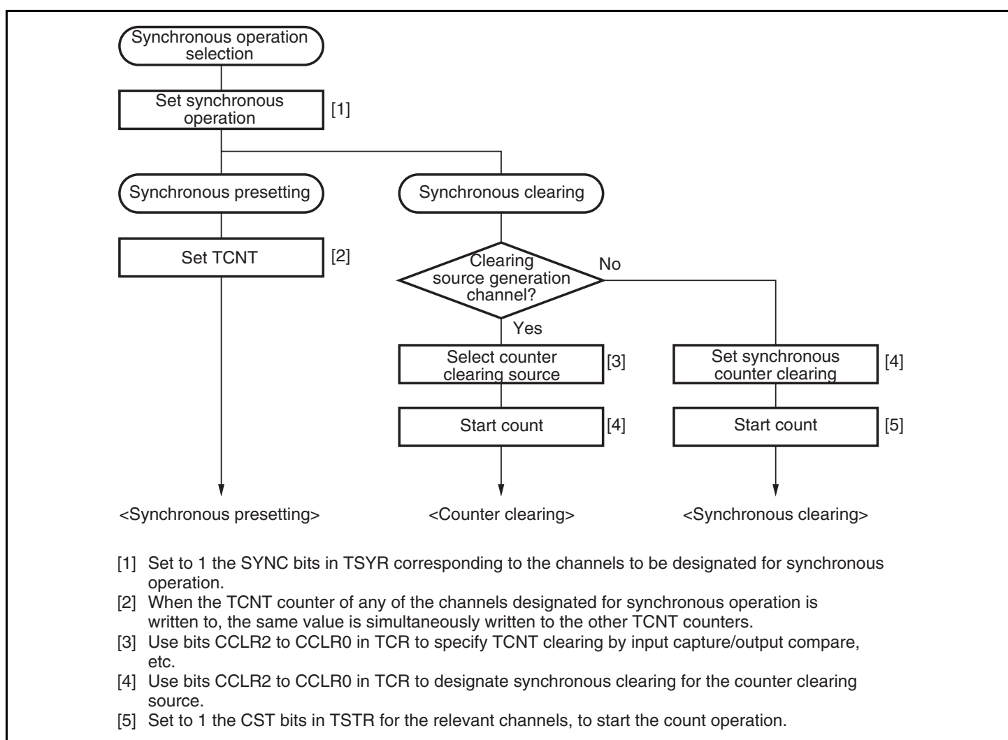
Figure 10.10 Example of Synchronous Operation Setting Procedure
