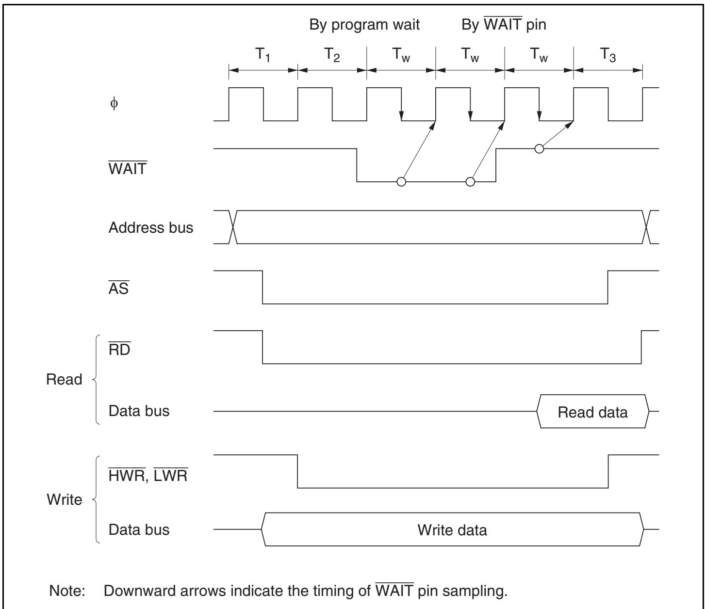
Figure 7.13 Example of Wait State Insertion Timing
