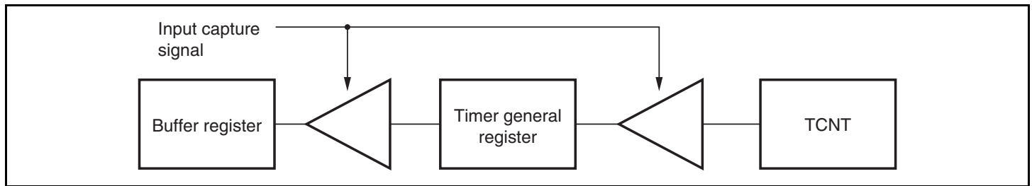
Figure 10.13 Input Capture Buffer Operation
