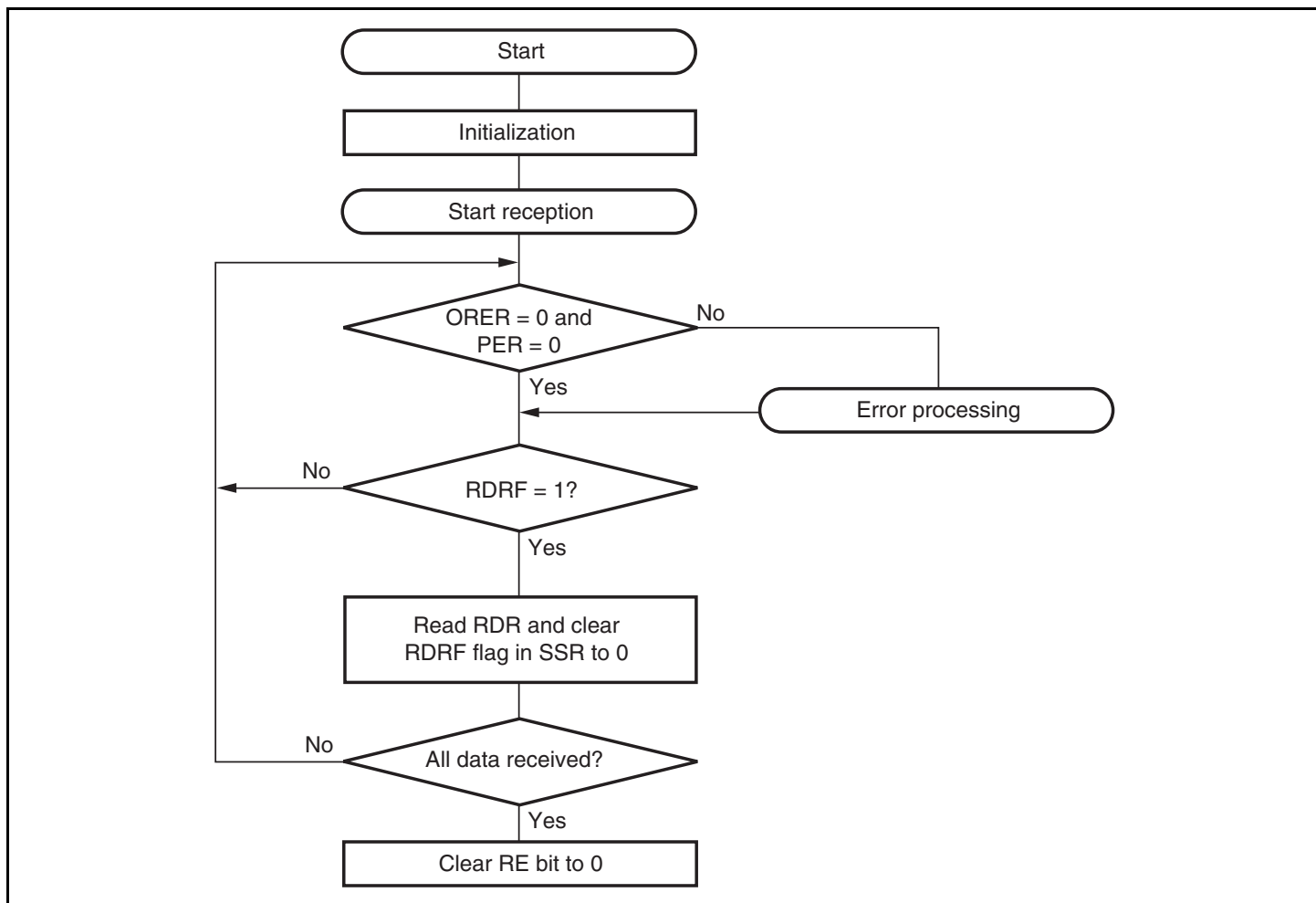
Figure 13.30 Example of Reception Processing Flow
