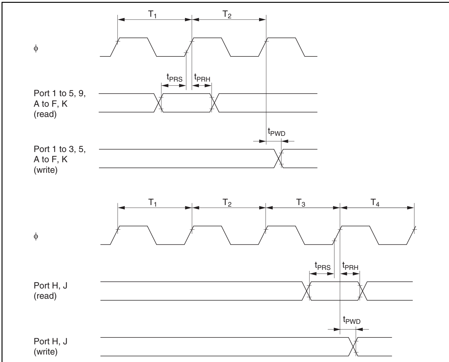
Figure 23.11 I/O Port Input/Output Timing
