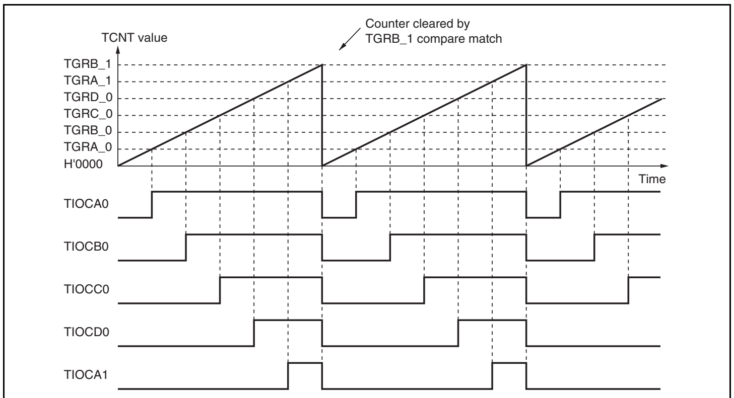
Figure 10.22 Example of PWM Mode Operation (2)
