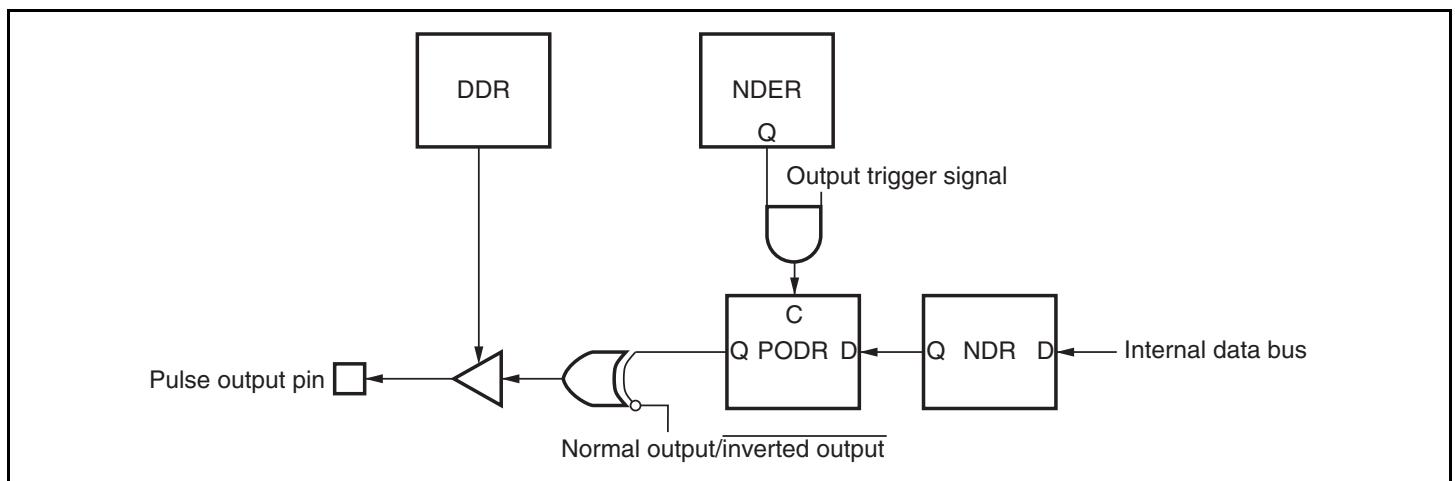
Figure 11.2 PPG Output Operation
