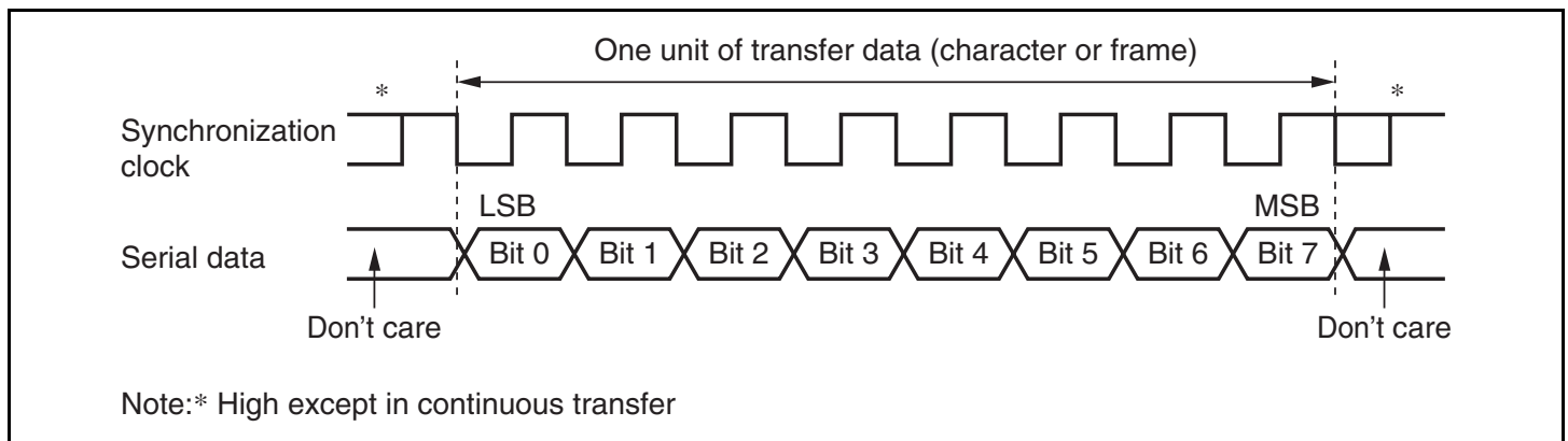
Figure 13.14 Data Format in Synchronous Communication (For LSB-First)
