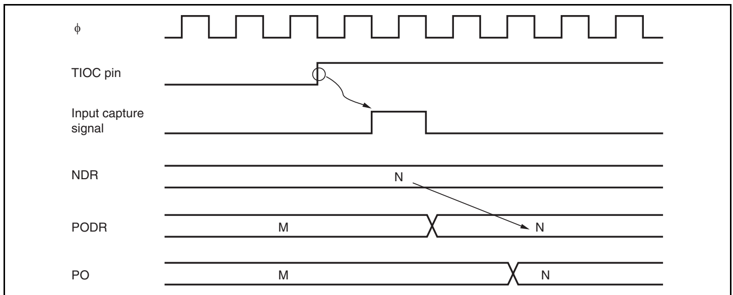
Figure 11.11 Pulse Output Triggered by Input Capture (Example)
