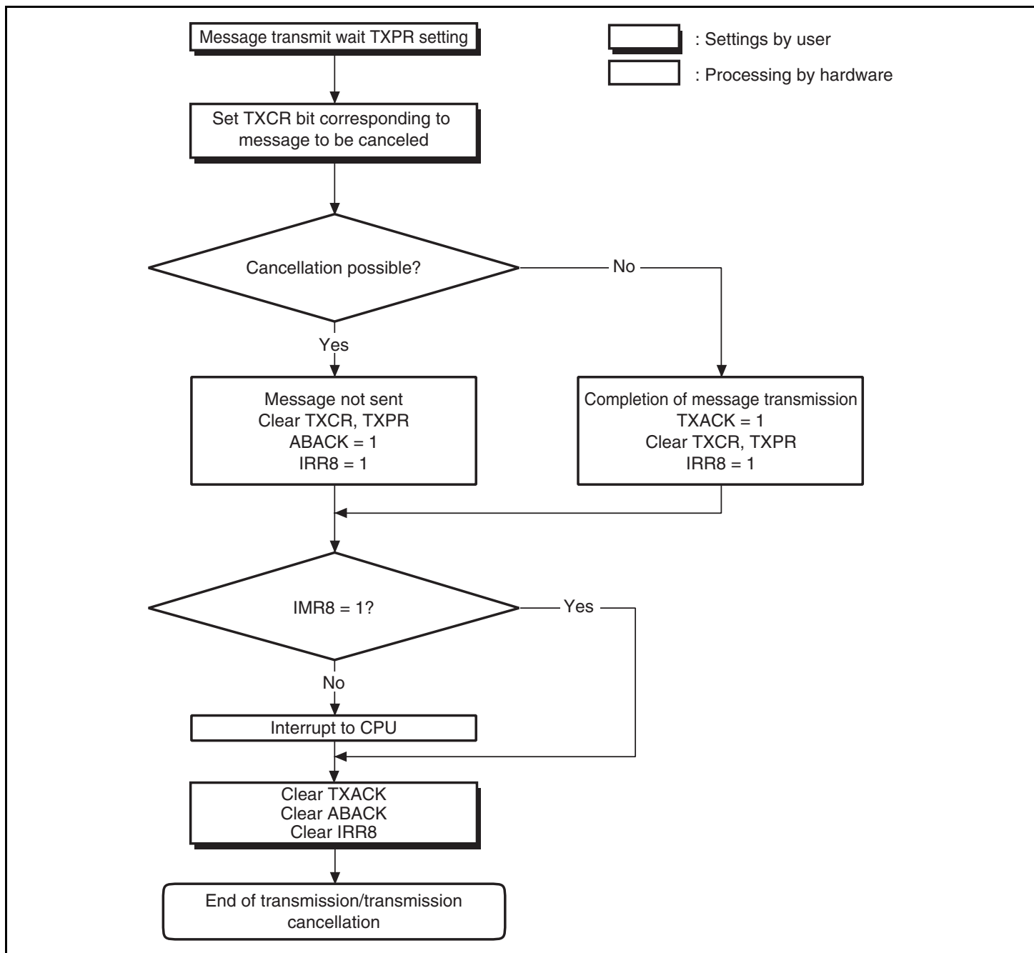
Figure 14.10 Transmit Message Cancellation Flowchart
