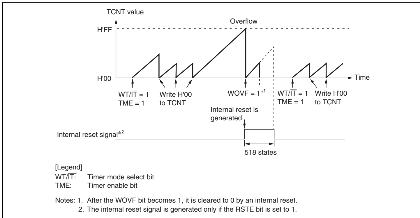
Figure 12.3 (a) WDT_0 Operation in Watchdog Timer Mode
