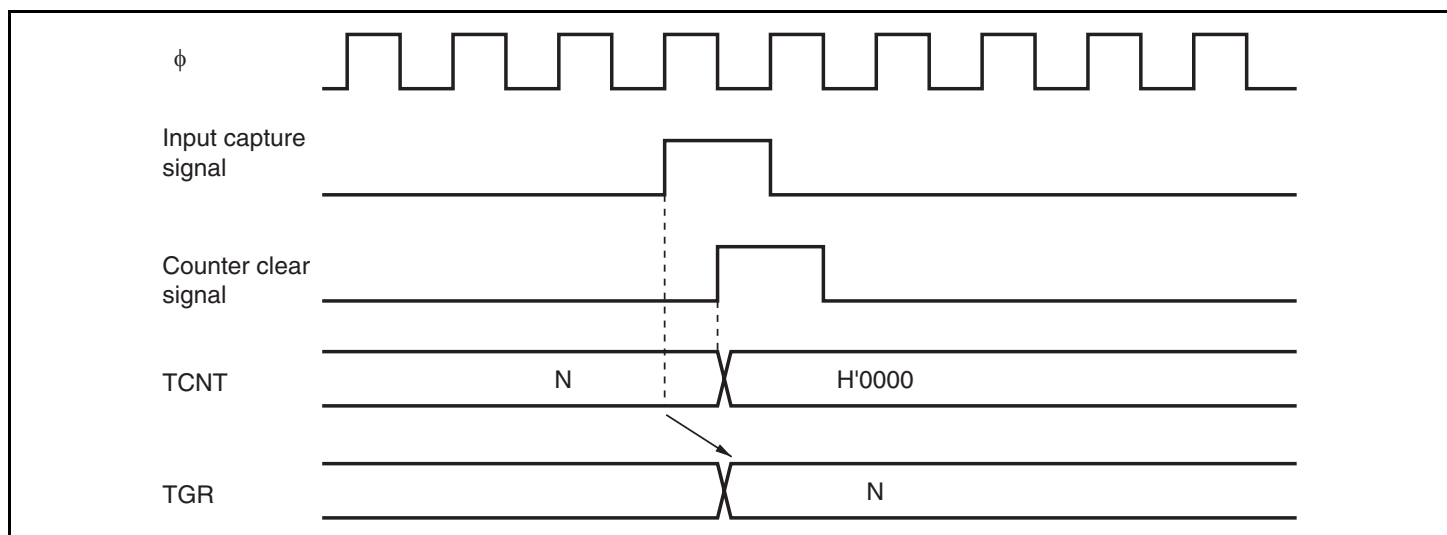
Figure 10.35 Counter Clear Timing (Input Capture)
