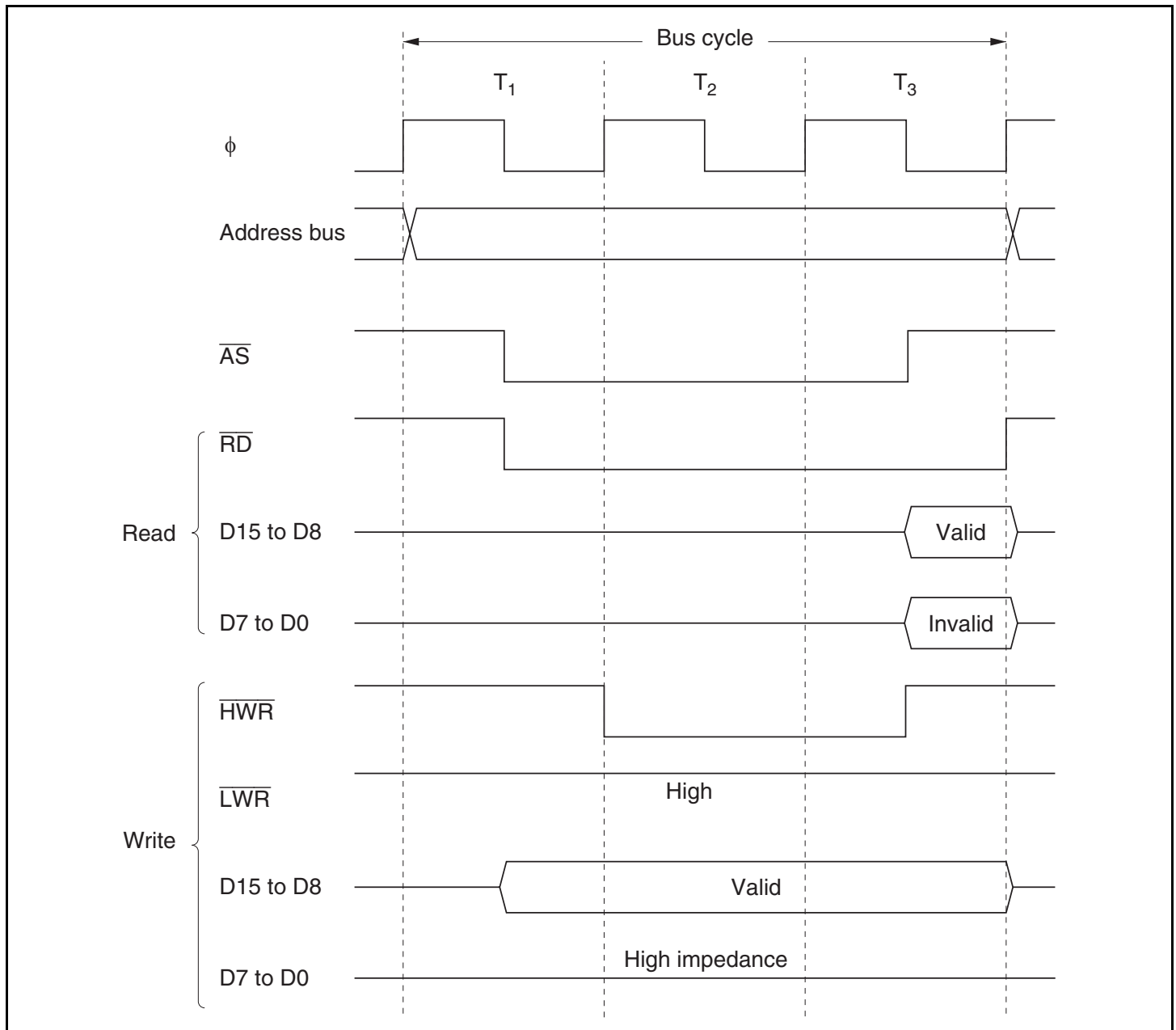
Figure 7.6 Bus Timing for 8-Bit, 3-State Access Space
