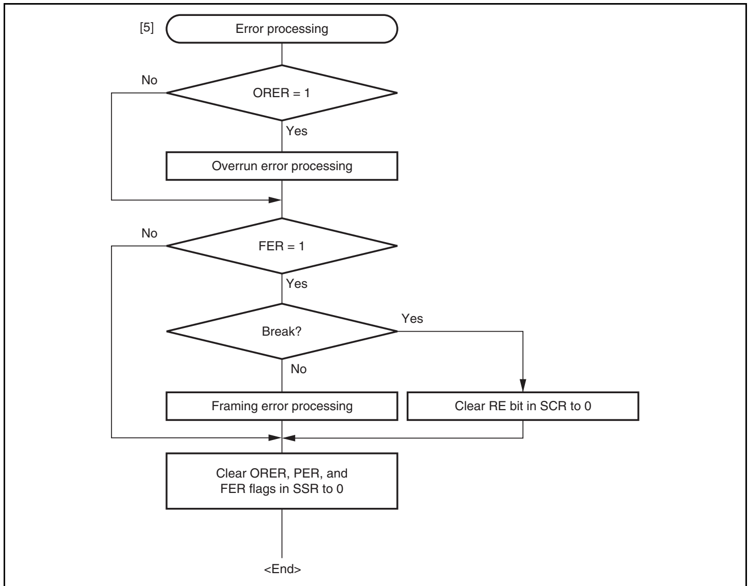
Figure 13.13 Sample Multiprocessor Serial Reception Flowchart (2)
