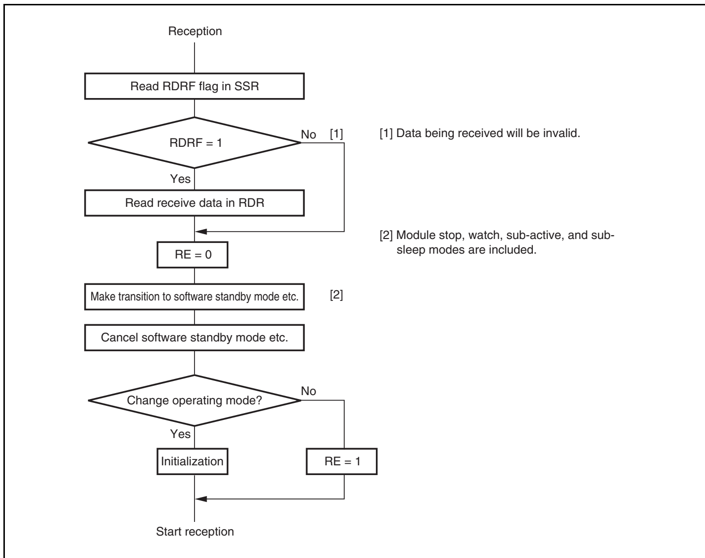
Figure 13.37 Sample Flowchart for Mode Transition during Reception
