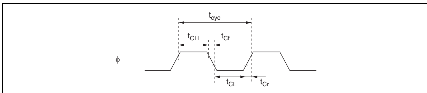
Figure 23.2 System Clock Timing
