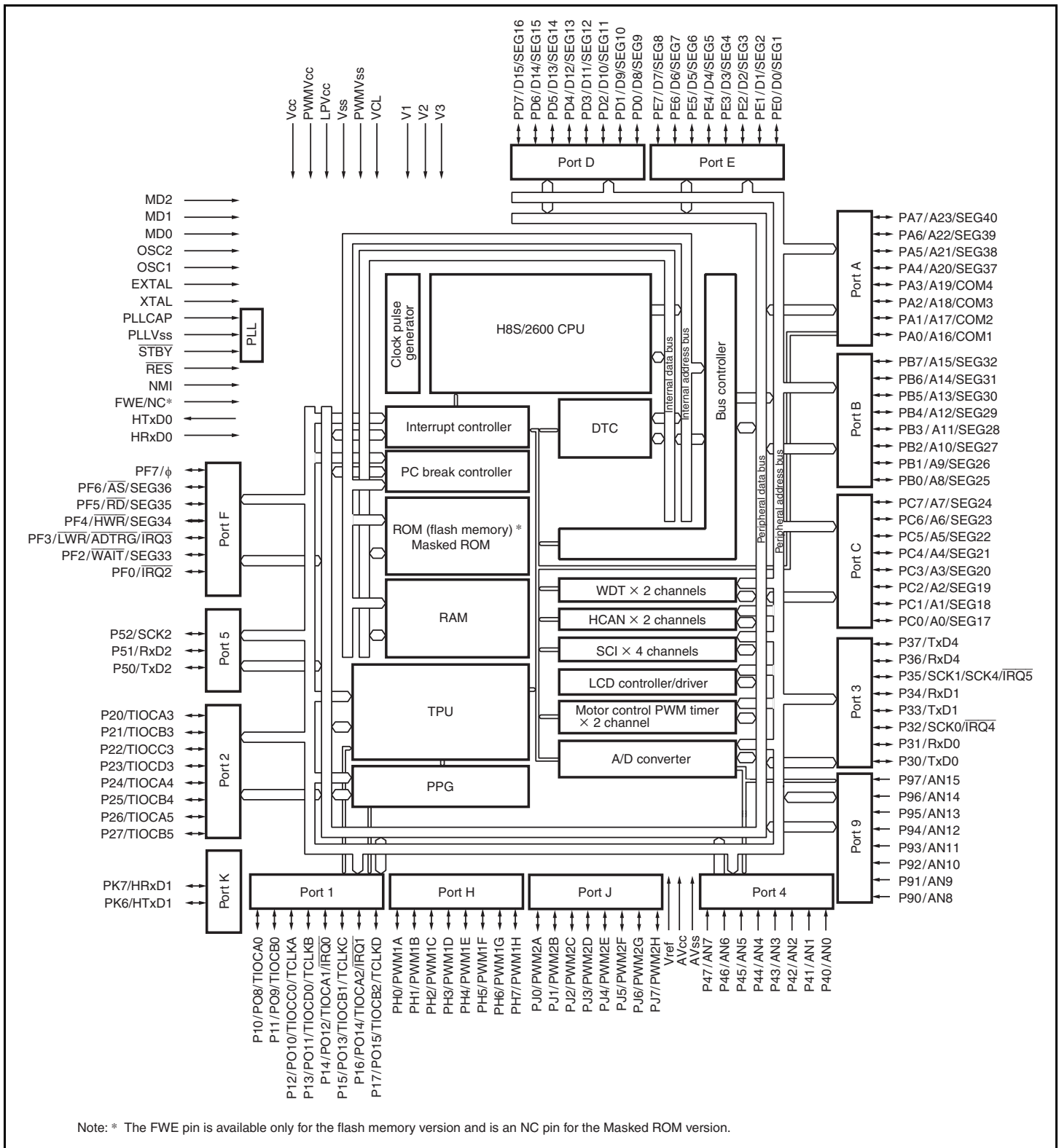
Figure 1.1 Internal Block Diagram
