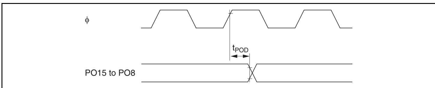
Figure 23.12 PPG Output Timing
