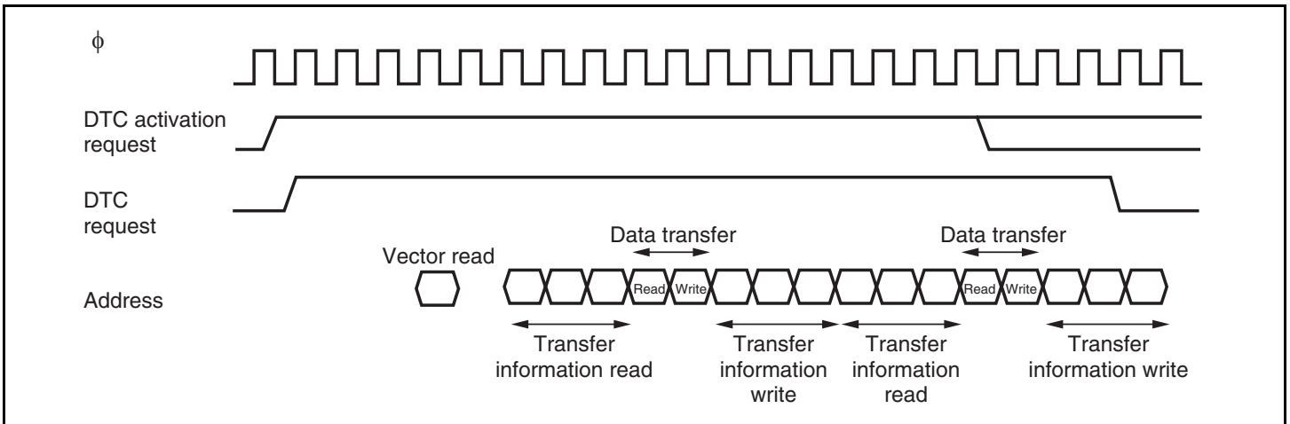
Figure 8.11 DTC Operation Timing (Example of Chain Transfer)
