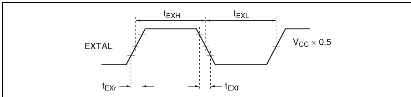
Figure 20.5 External Clock Input Timing
