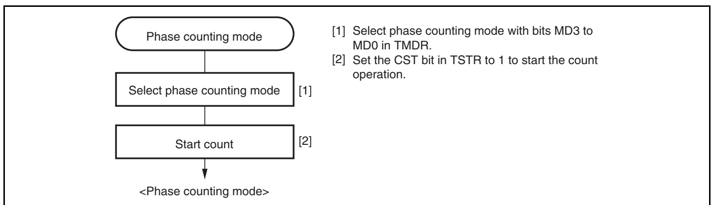
Figure 10.24 Example of Phase Counting Mode Setting Procedure
