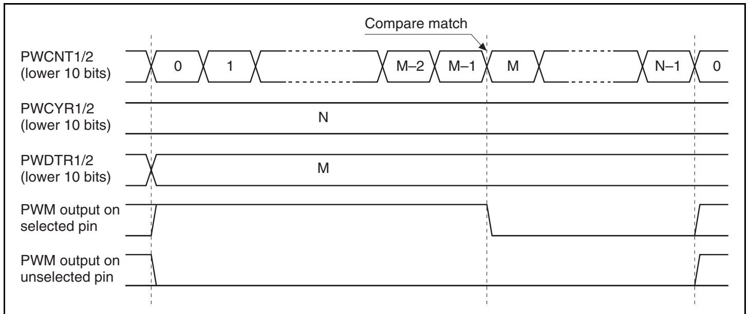
Figure 16.3 Duty Register Compare Match (OPS = 0 in PWPR)
