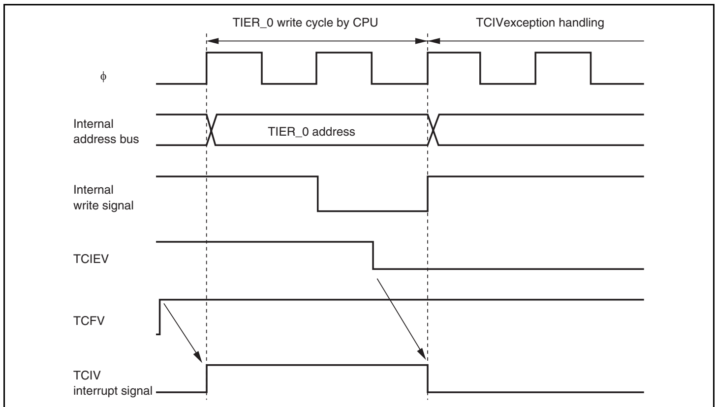
Figure 5.6 Conflict between Interrupt Generation and Disabling
