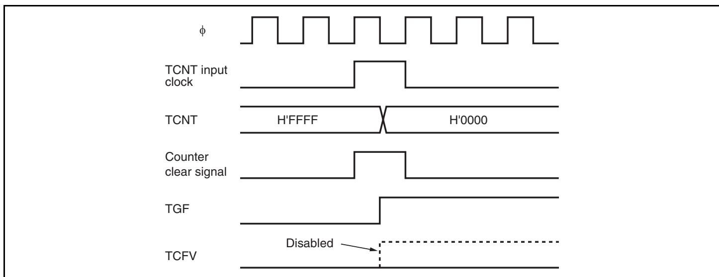
Figure 10.52 Conflict between Overflow and Counter Clearing
