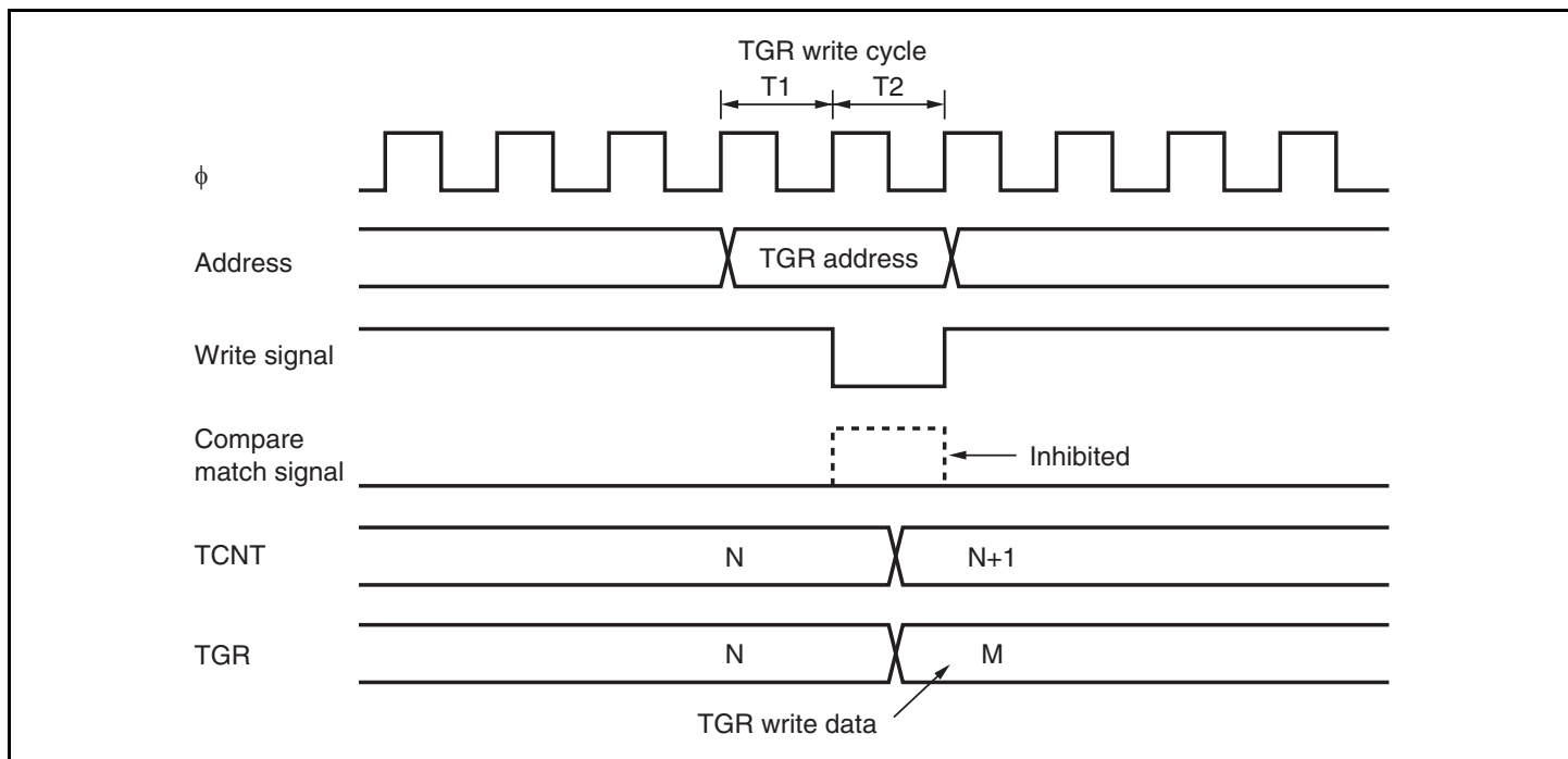
Figure 10.47 Conflict between TGR Write and Compare Match
