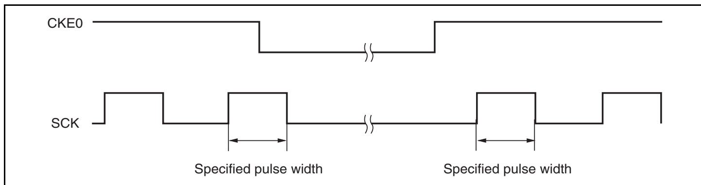
Figure 13.31 Timing for Fixing Clock Output Level
