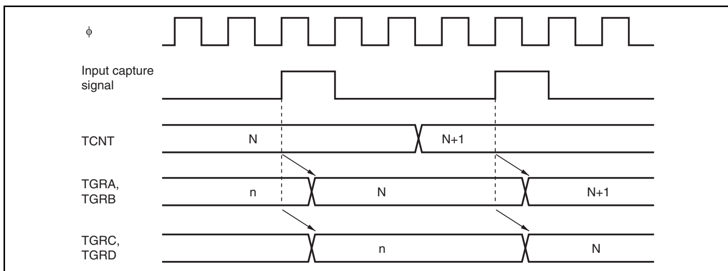
Figure 10.37 Buffer Operation Timing (Input Capture)
