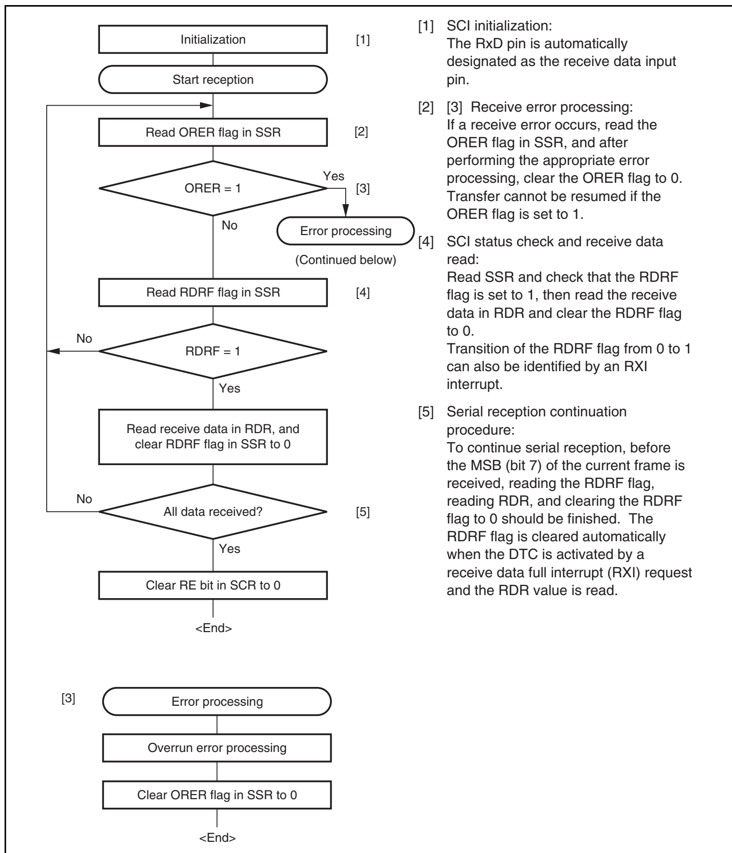
Figure 13.19 Sample Serial Reception Flowchart
