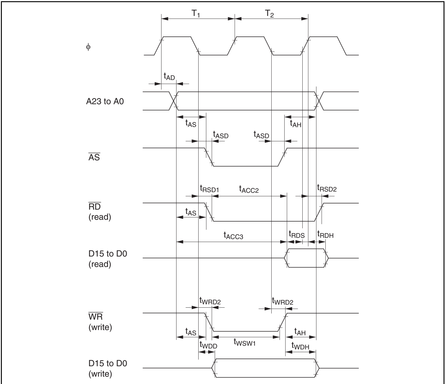
Figure 23.6 Basic Bus Timing (Two-State Access)
