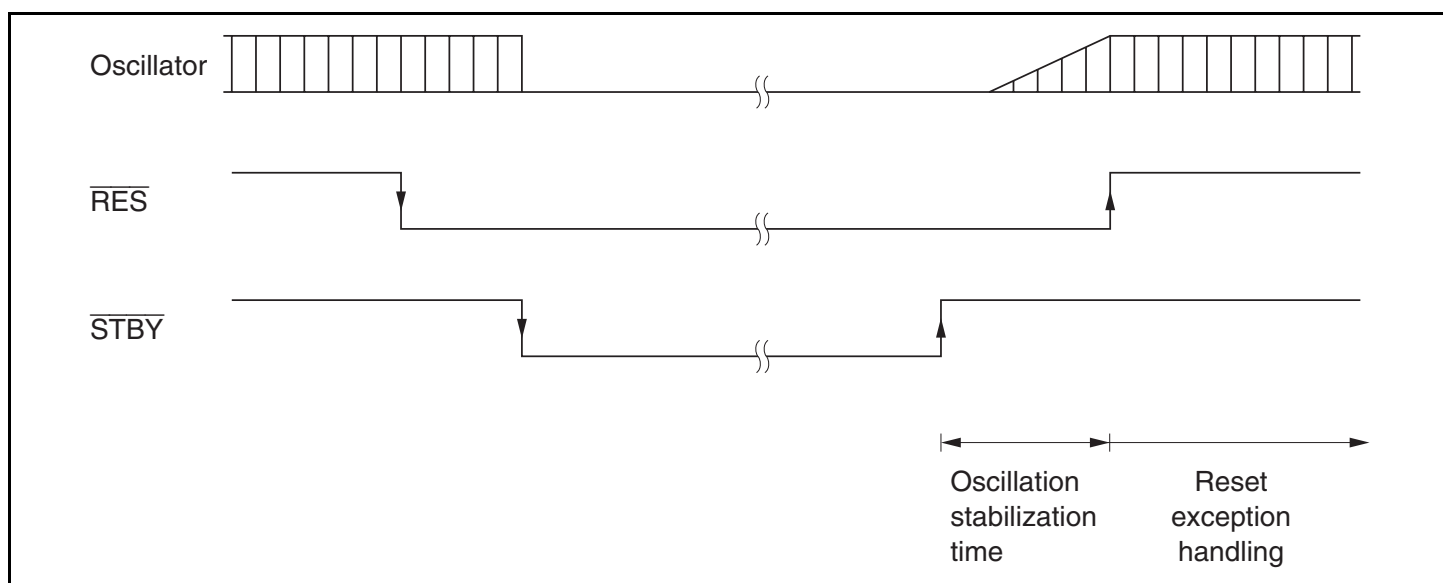
Figure 21.4 Hardware Standby Mode Timing
