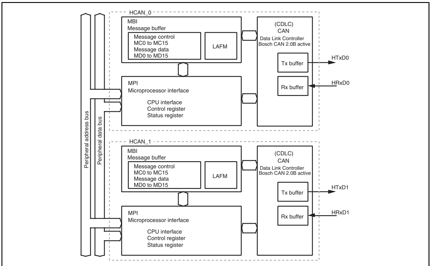
Figure 14.1 HCAN Block Diagram
