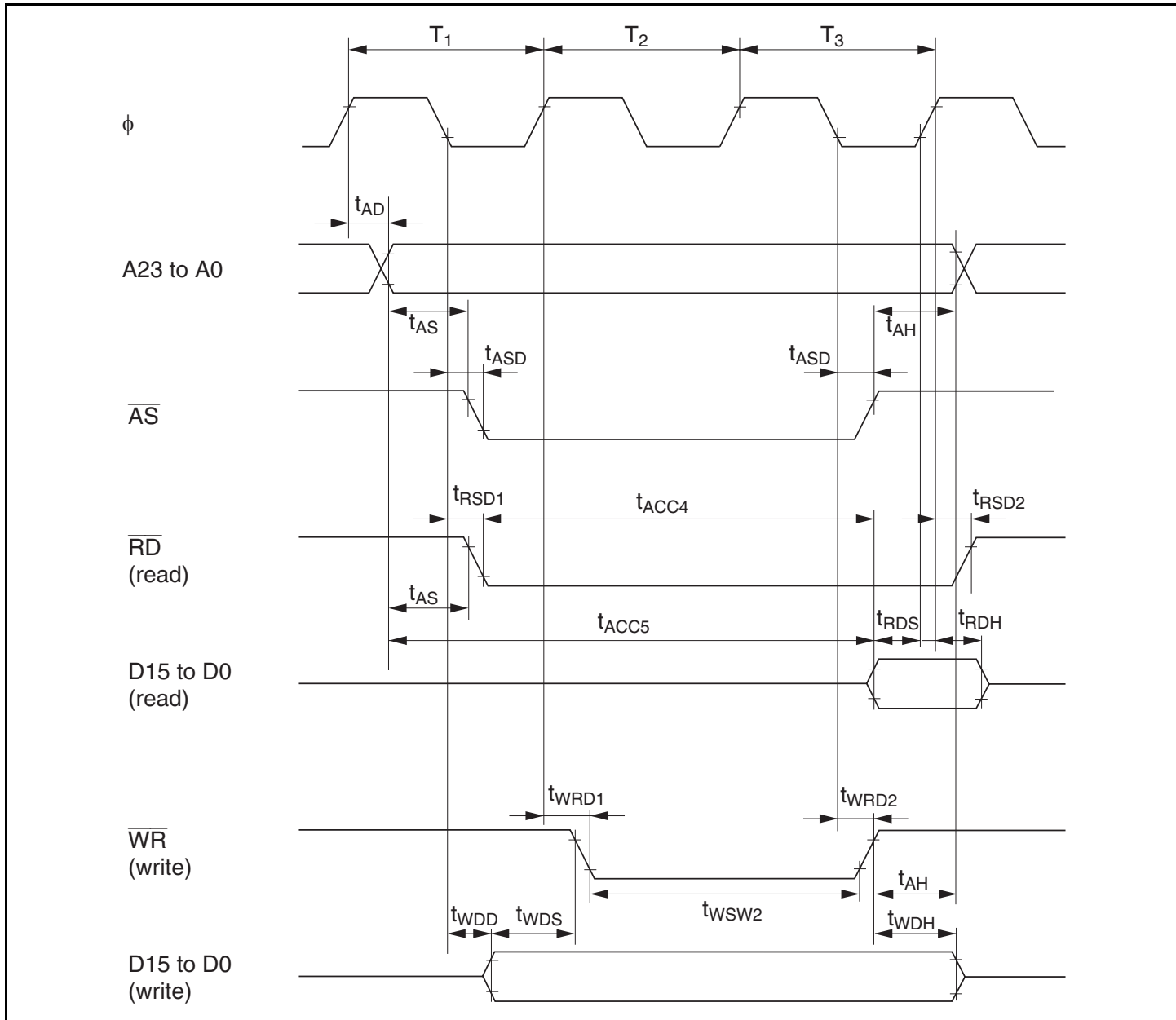
Figure 23.7 Basic Bus Timing (Three-State Access)
