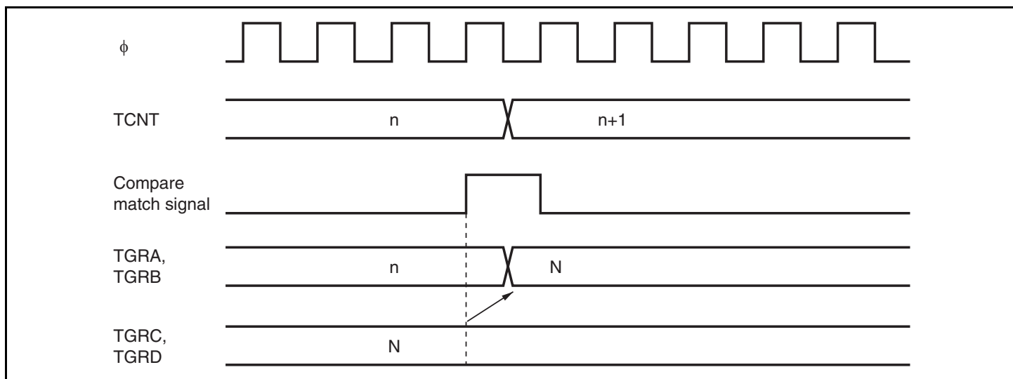
Figure 10.36 Buffer Operation Timing (Compare Match)
