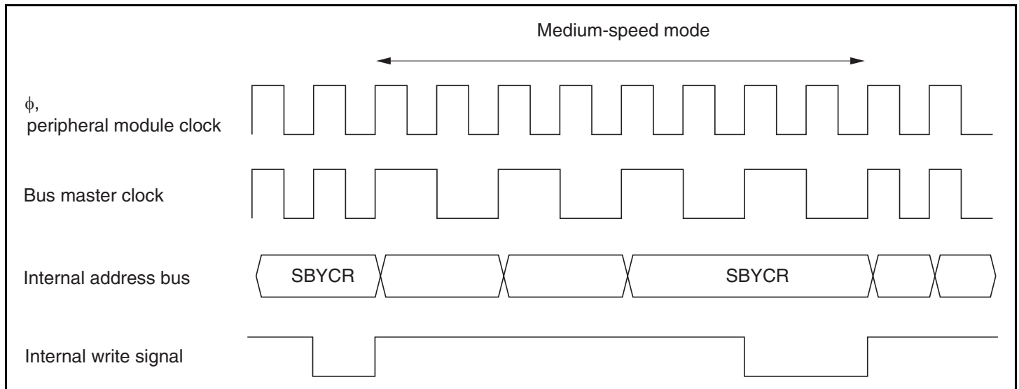
Figure 21.2 Medium-Speed Mode Transition and Clearance Timing
