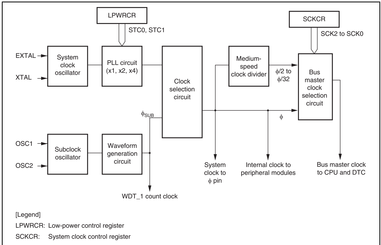
Figure 20.1 Block Diagram of Clock Pulse Generator
