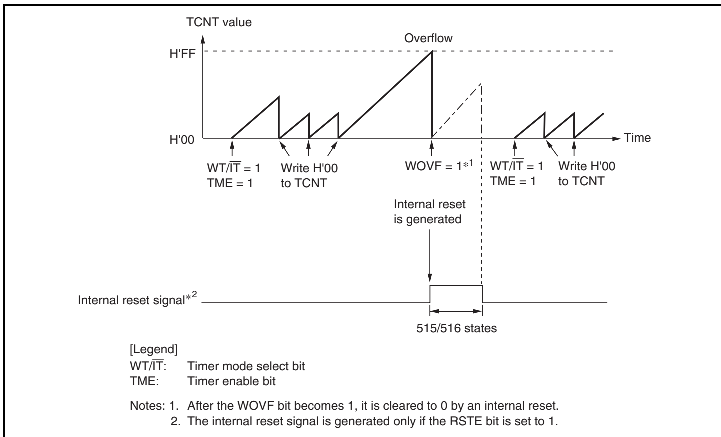
Figure 12.3 (b) WDT_1 Operation in Watchdog Timer Mode
