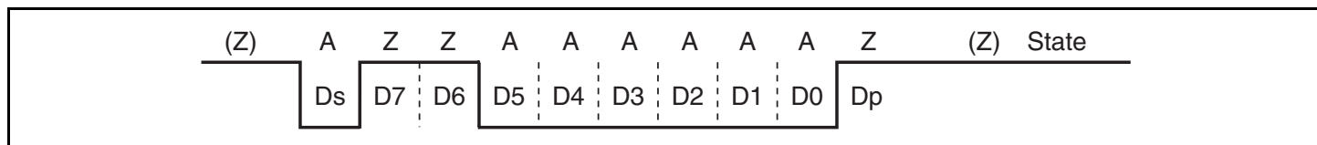
Figure 13.24 Inverse Convention (SDIR = SINV = O/\bar{E} = 1)
