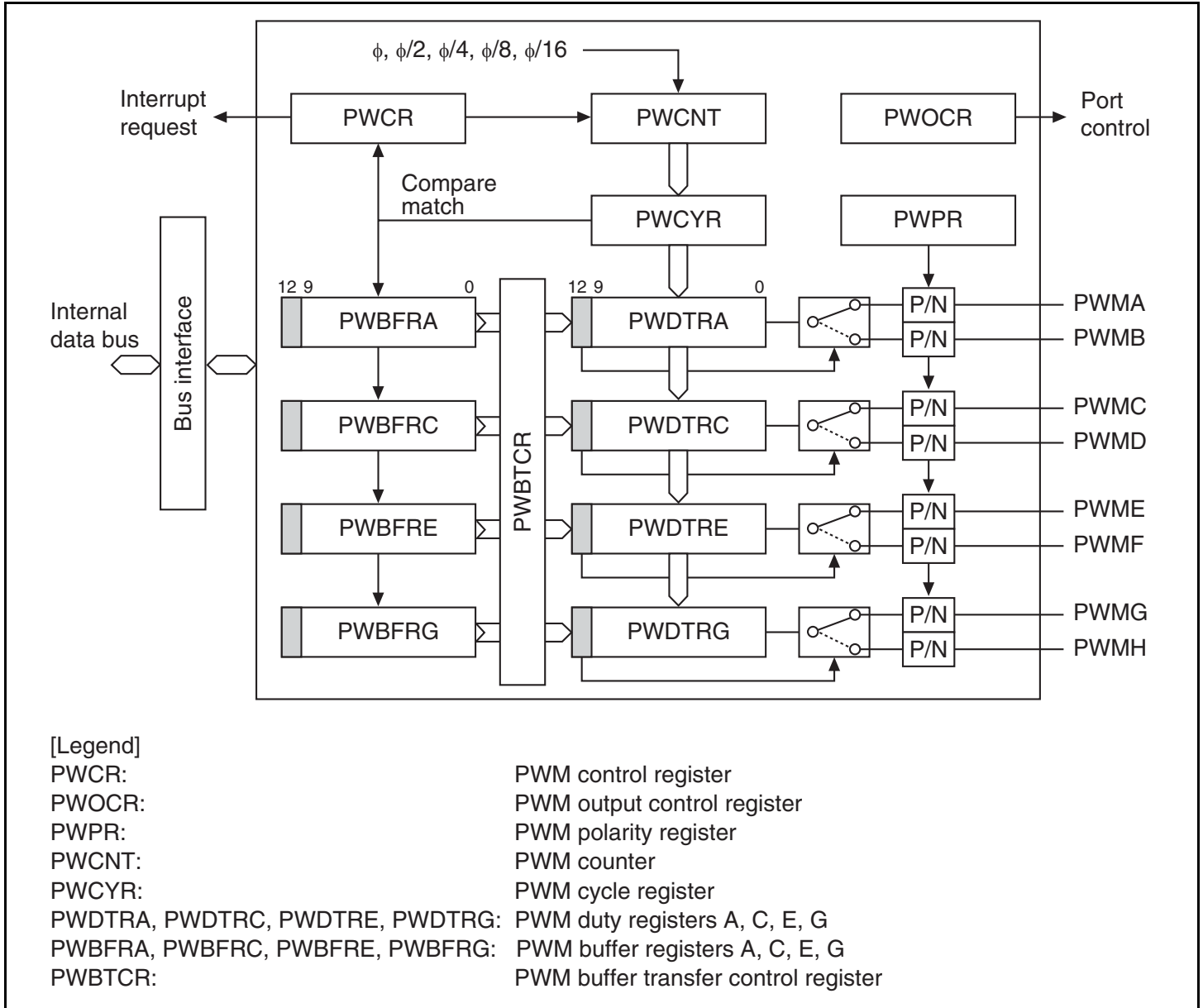
Figure 16.1 Block Diagram of PWM
