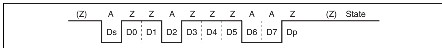
Figure 13.23 Direct Convention (SDIR = SINV = \overline{O/E} = 0 )
