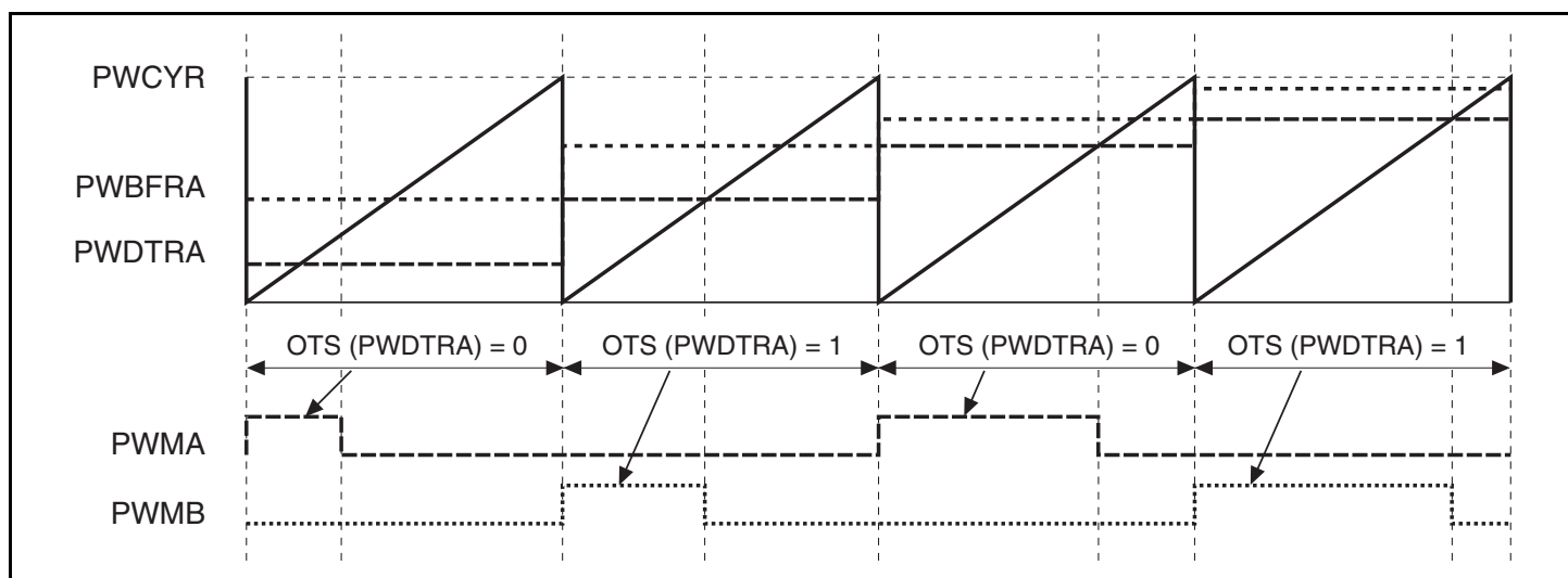
Figure 16.7 PWM Operation
