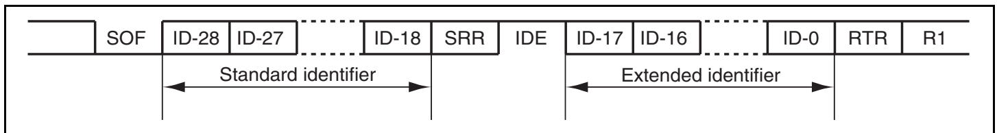
Figure 14.4 Extended Format
