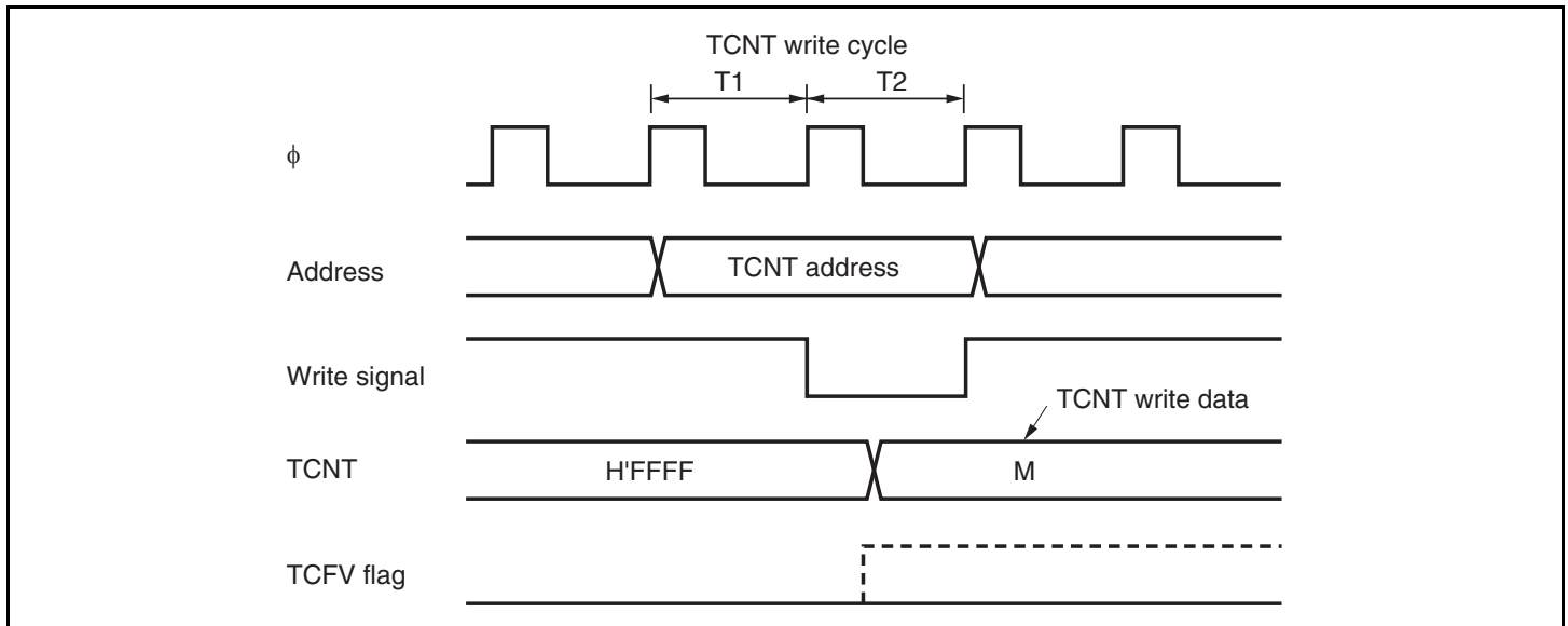
Figure 10.53 Conflict between TCNT Write and Overflow
