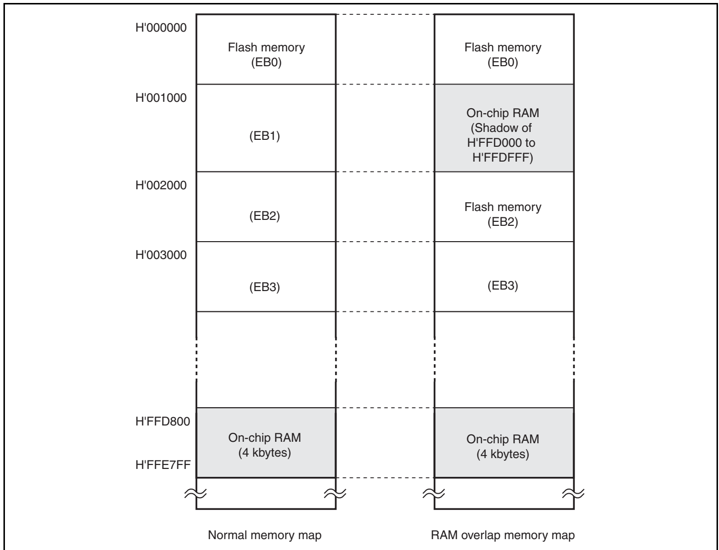
Figure 19.8 Example of RAM Overlap Operation
