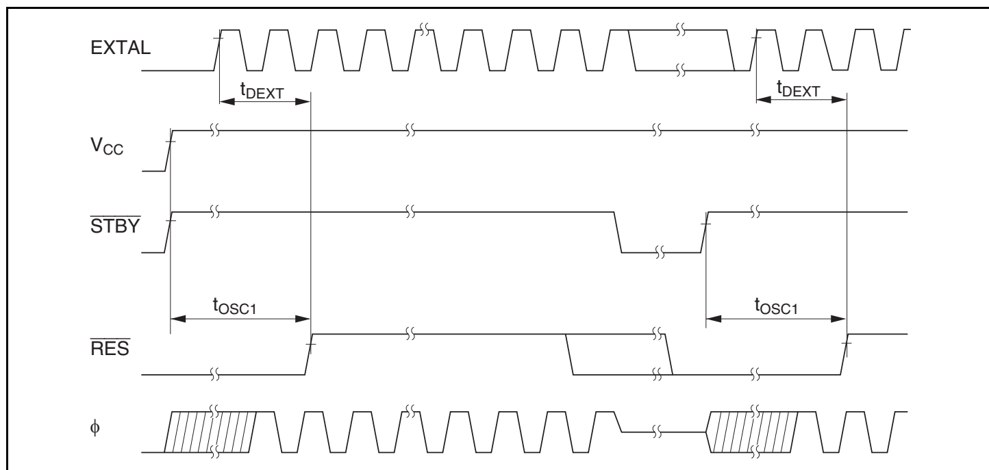
Figure 23.3 Oscillator Settling Timing
