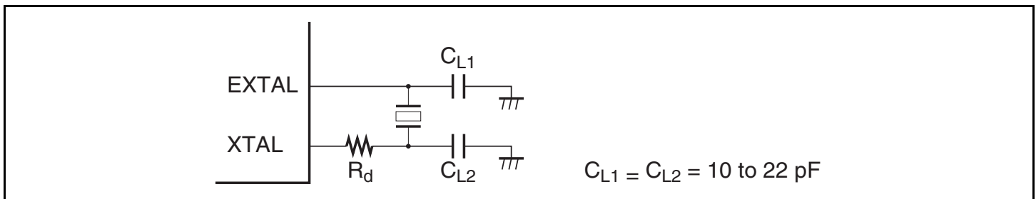
Figure 20.2 Connection of Crystal Resonator (Example)
