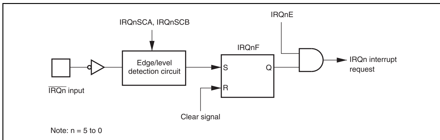
Figure 5.2 Block Diagram of Interrupts IRQ0 to IRQ5
