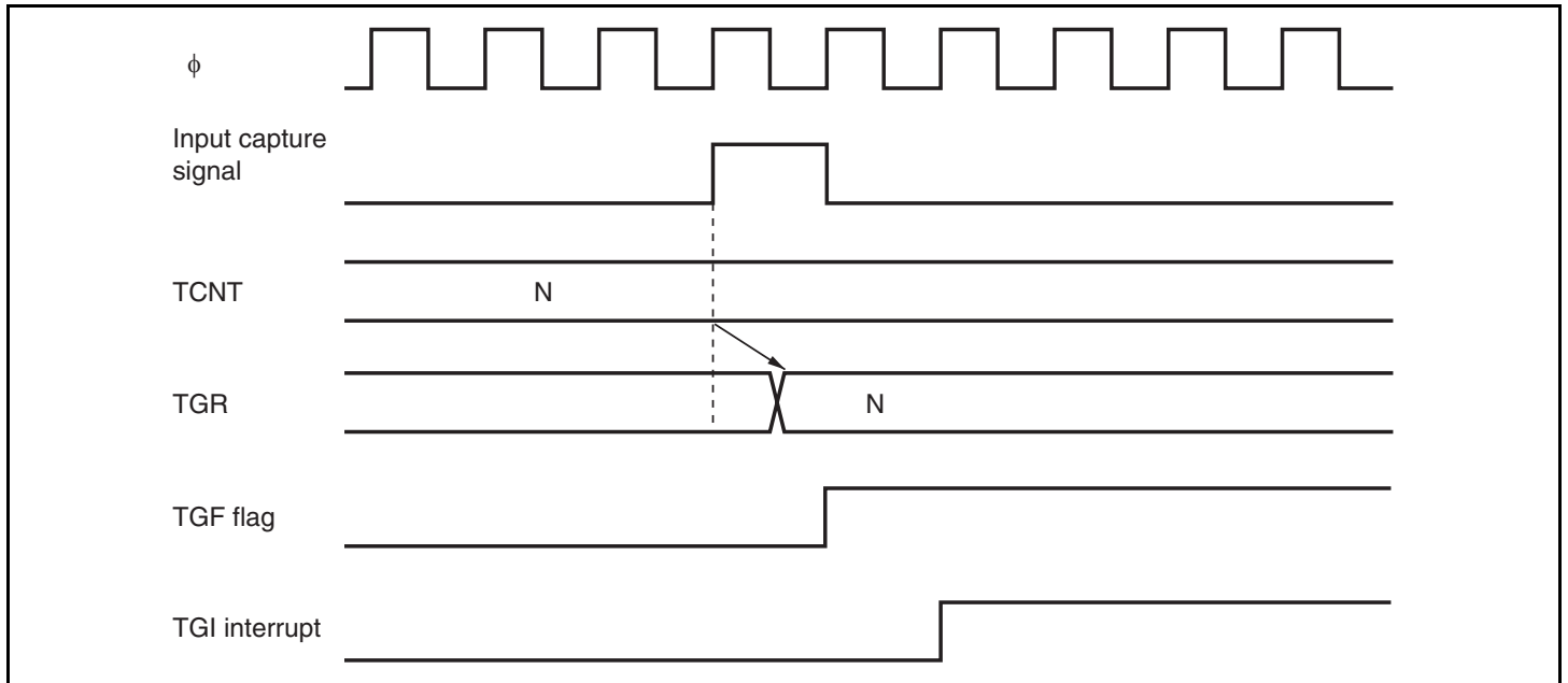
Figure 10.39 TGI Interrupt Timing (Input Capture)
