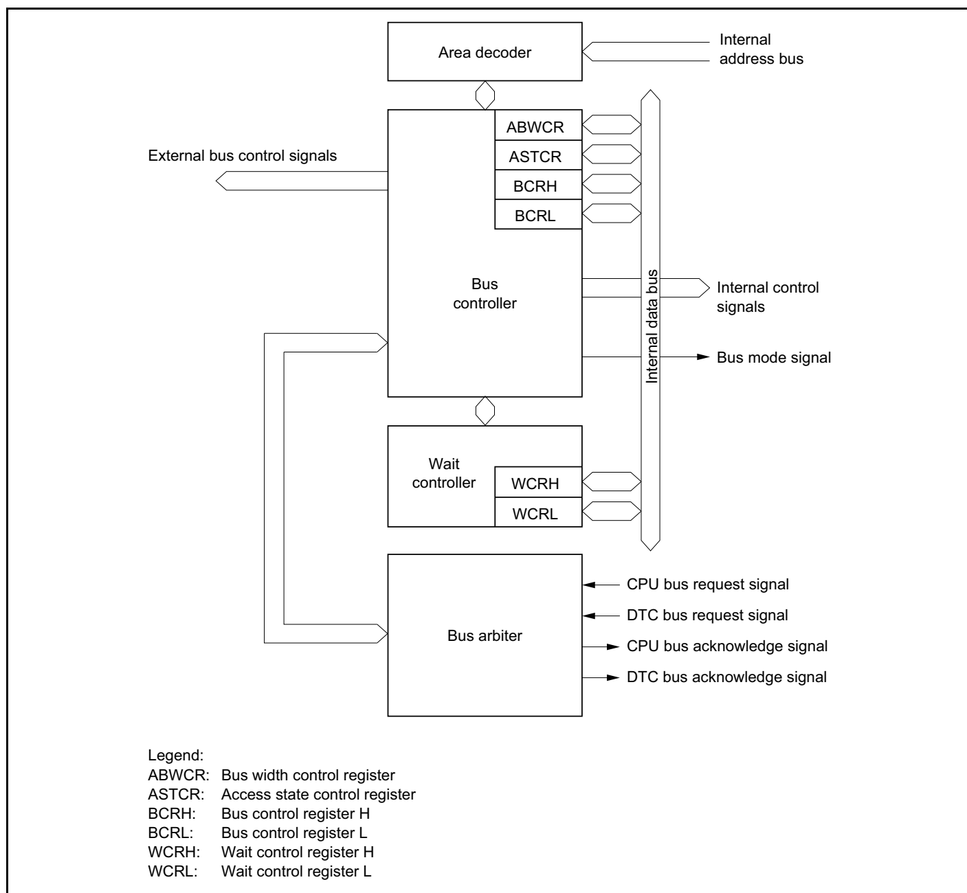
Figure 7-1 Block Diagram of Bus Controller
