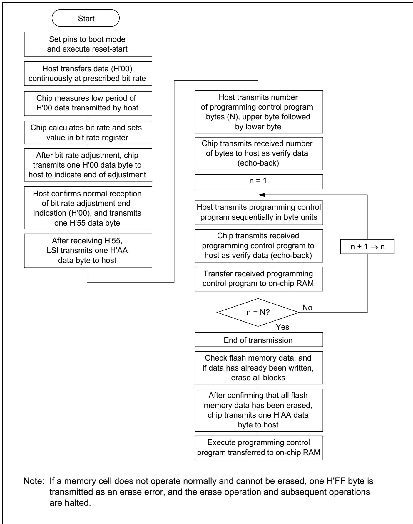
Figure 21A-8 Boot Mode Execution Procedure
