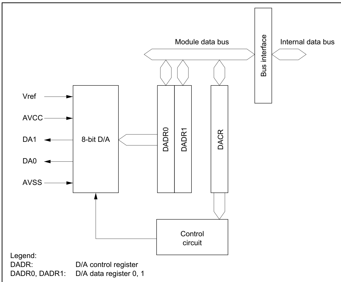
Figure 18-1 Block Diagram of D/A Converter
