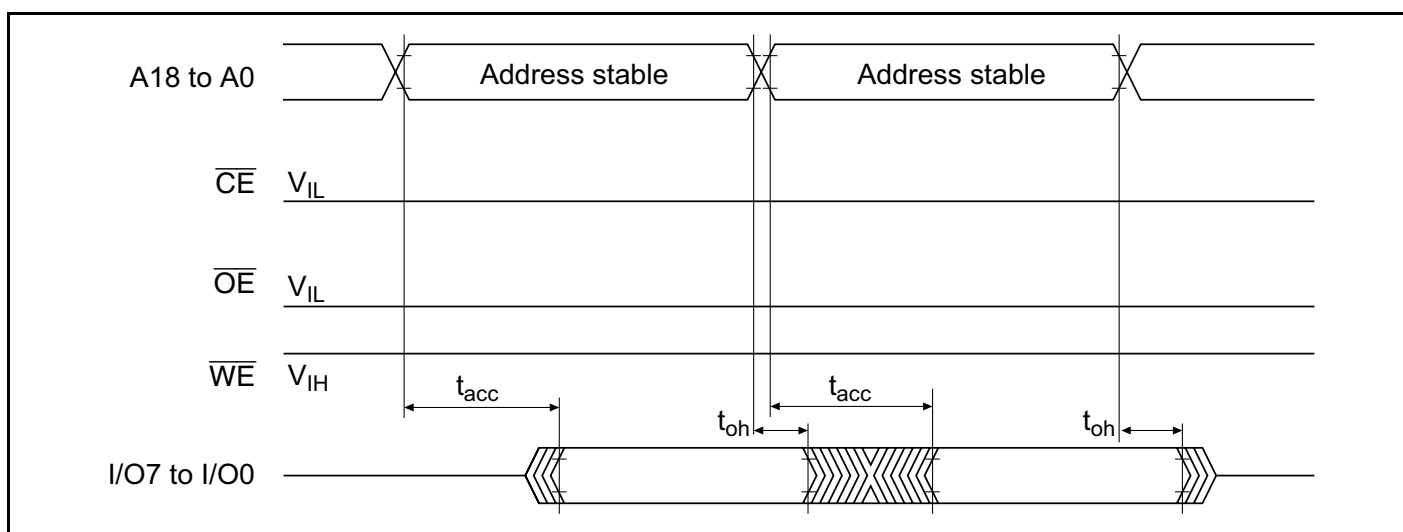
Figure 21A-20 \overline{\text{CE}} and \overline{\text{OE}} Enable State Read Timing Waveforms
