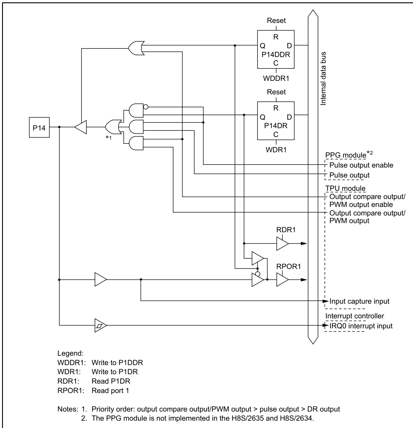
Figure C-1 (c) Port 1 Block Diagram (Pin P14)
