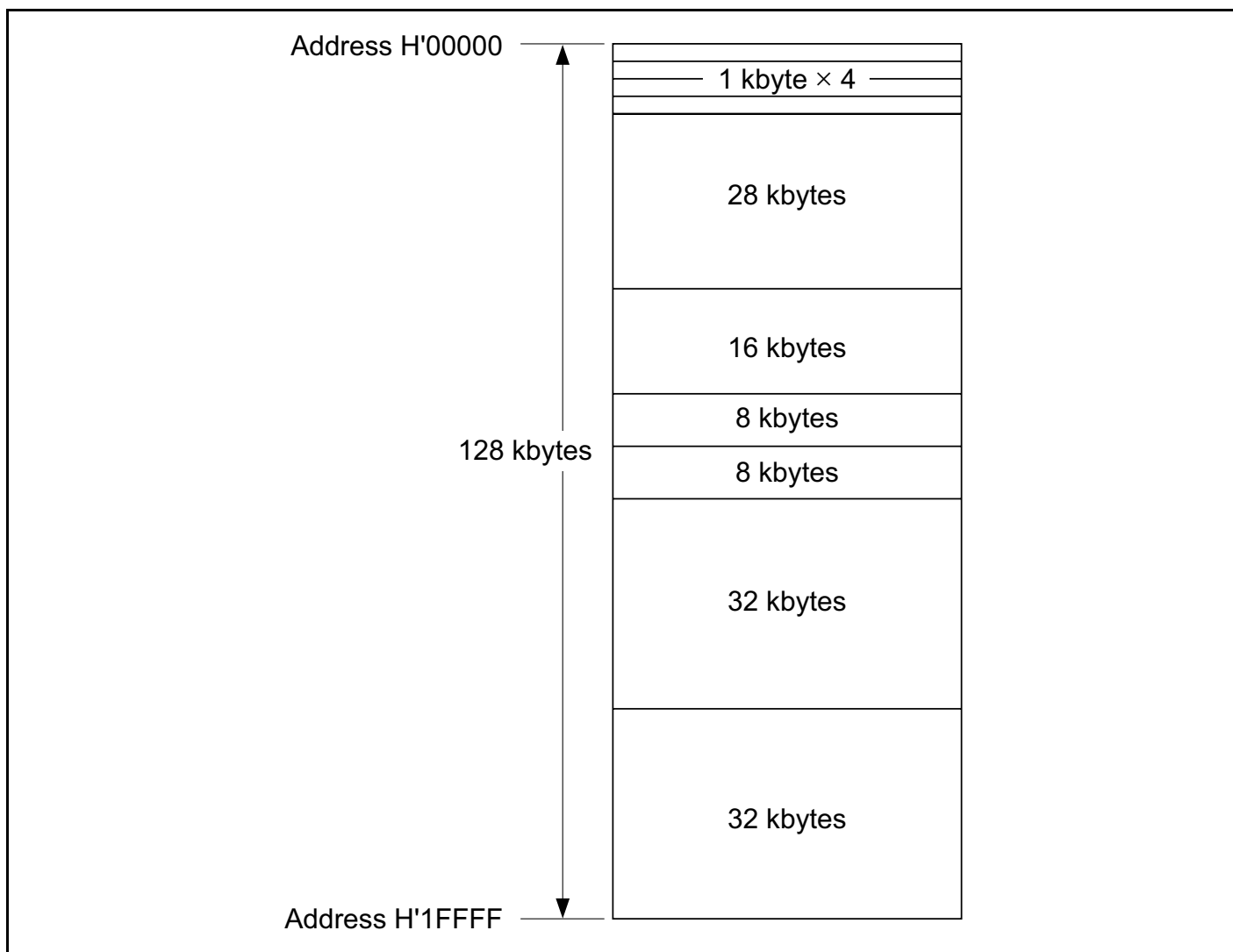
Figure 21A-6 Block Configuration
