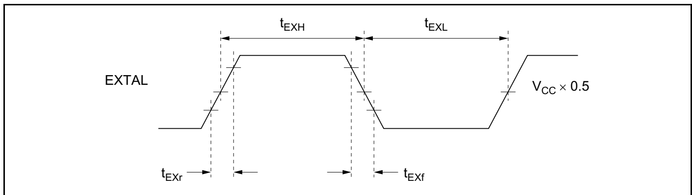
Figure 22A-7 External Clock Input Timing
