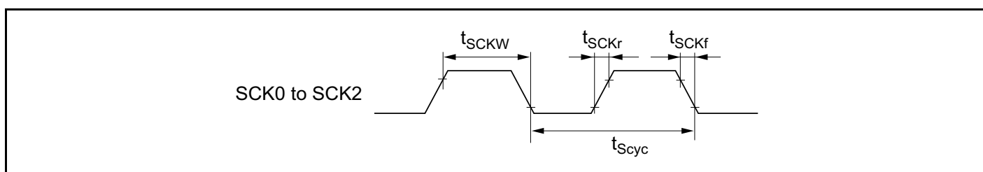
Figure 24-24 SCK Clock Input Timing
