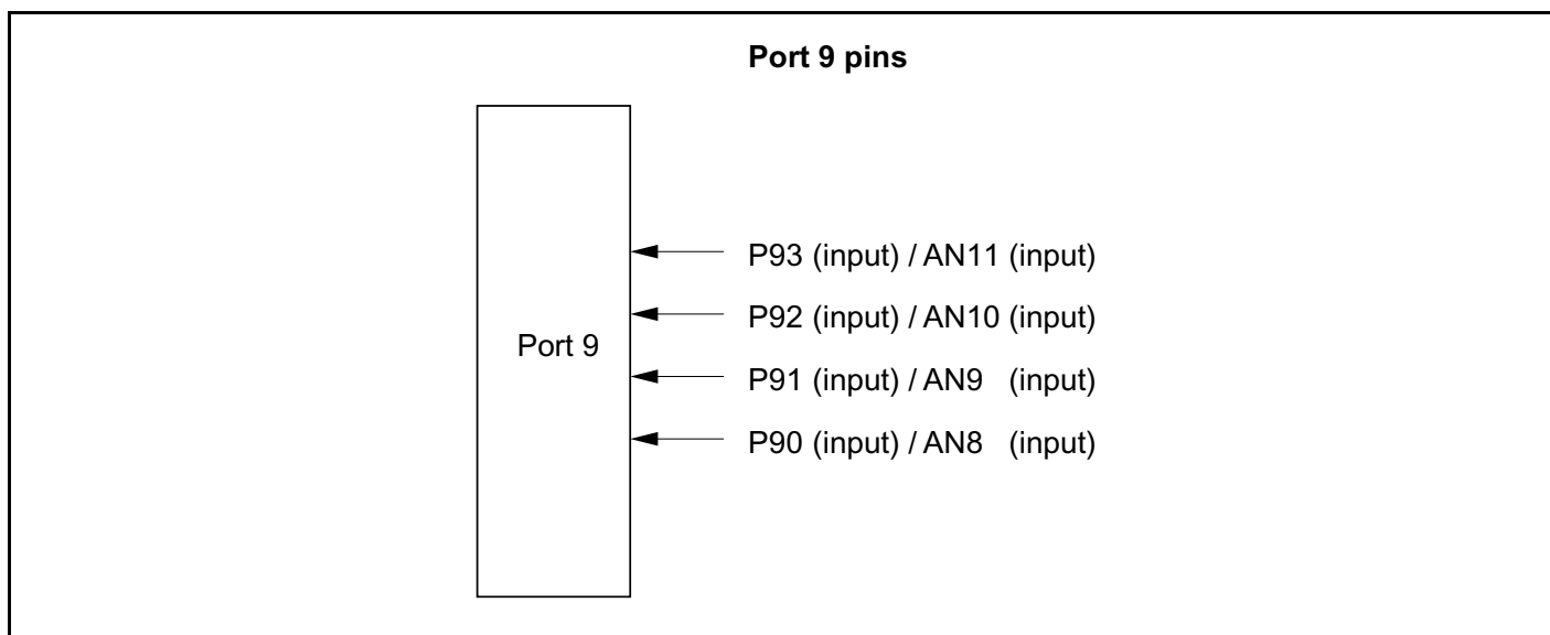
Figure 9-4 Port 9 Pin Functions
