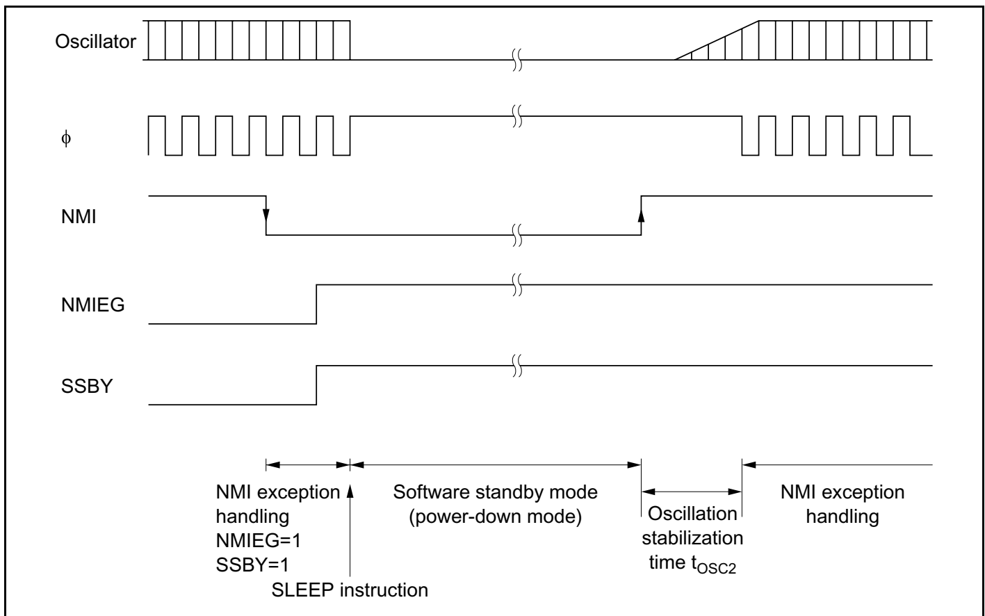
Figure 23B-3 Software Standby Mode Application Example
