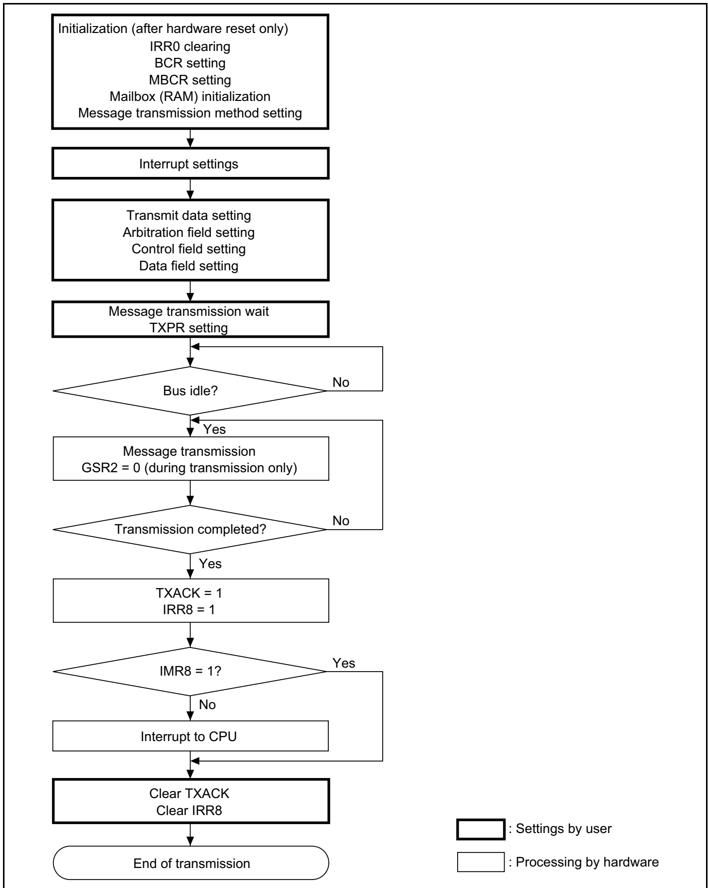
Figure 16-7 Transmission Flowchart
