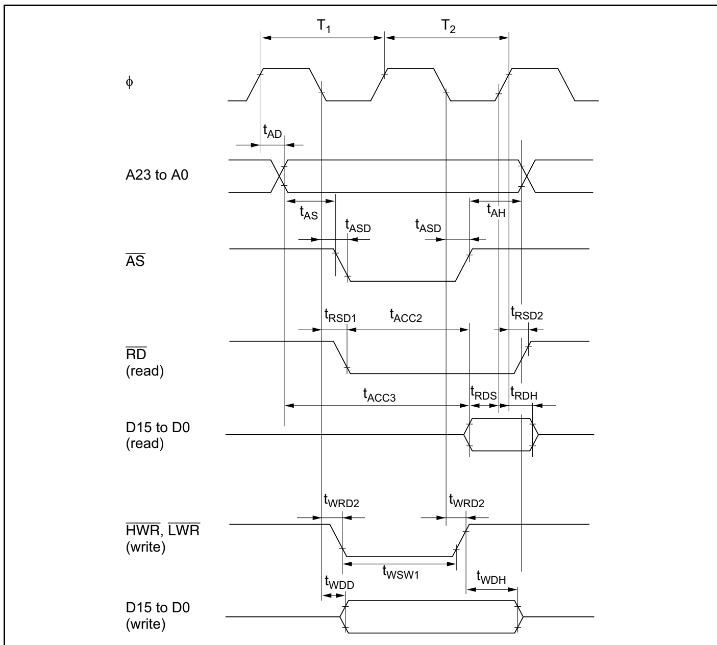
Figure 24-13 Basic Bus Timing (Two-State Access)
