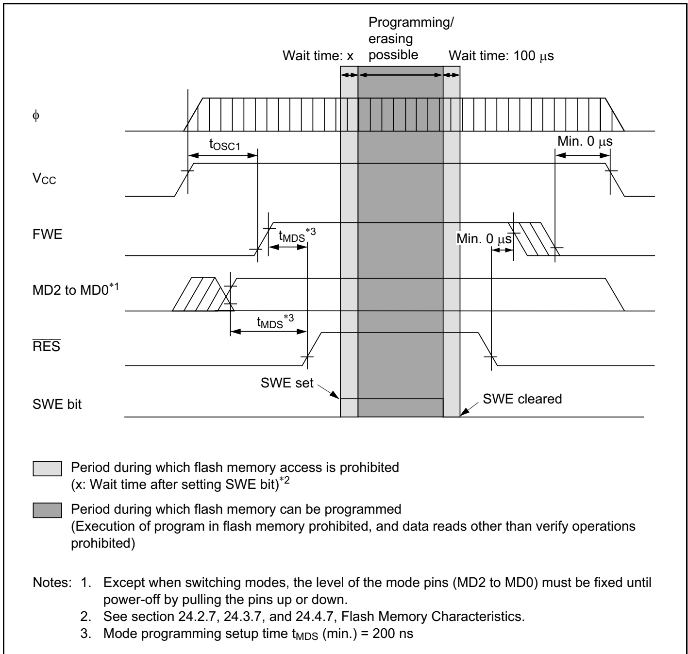
Figure 21C-26 Power-On/Off Timing (Boot Mode)
