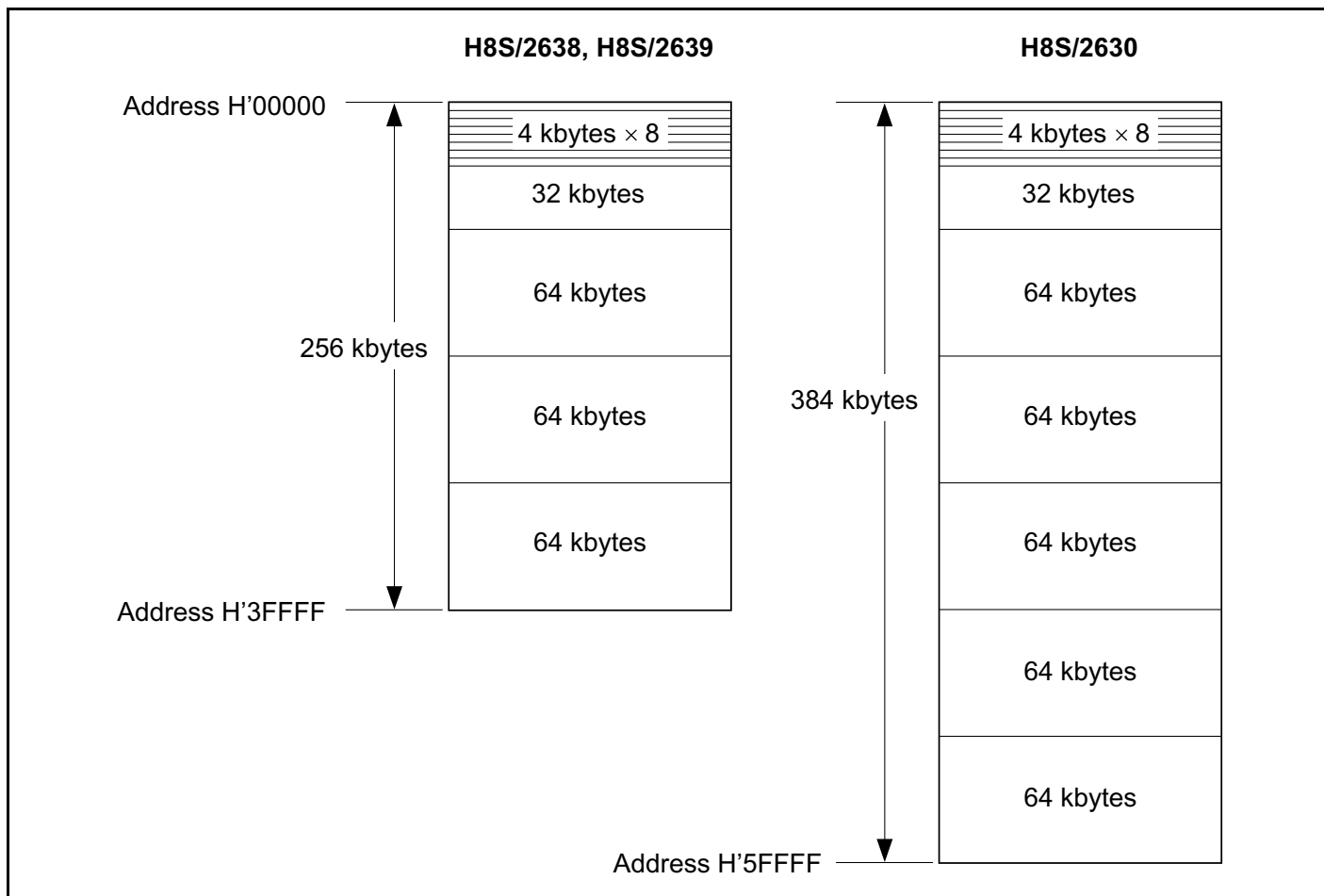
Figure 21B-6 Flash Memory Block Configuration
