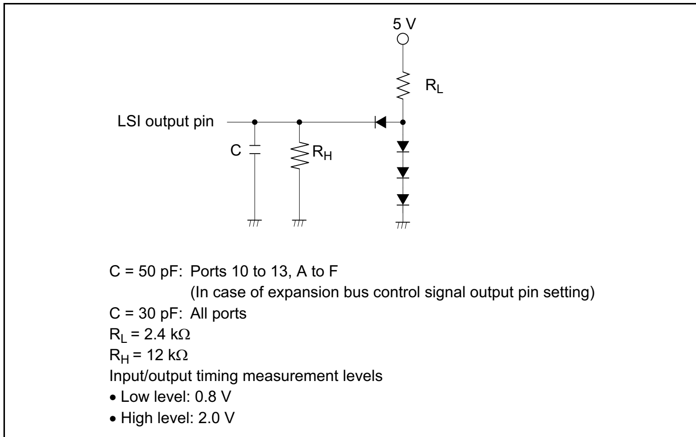
Figure 24-8 Output Load Circuit
