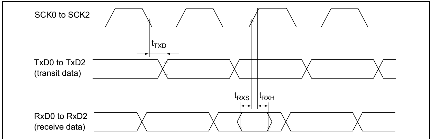
Figure 24-25 SCI Input/Output Timing (Clock Synchronous Mode)
