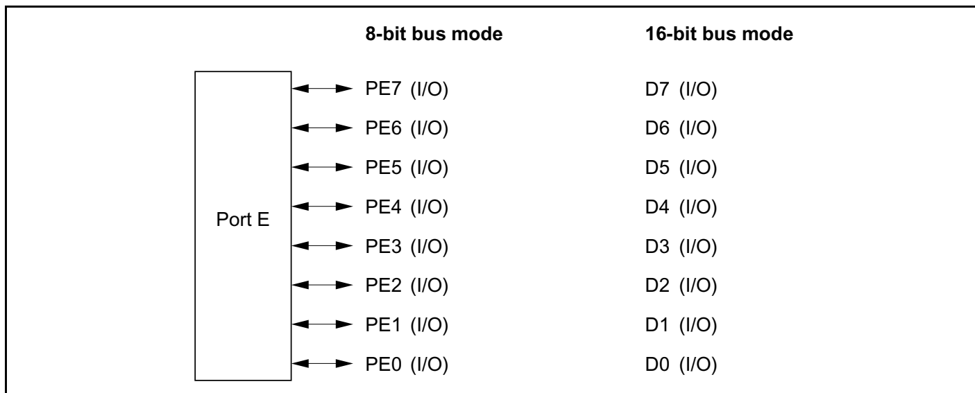
Figure 9-19 Port E Pin Functions (Modes 4 to 6)
