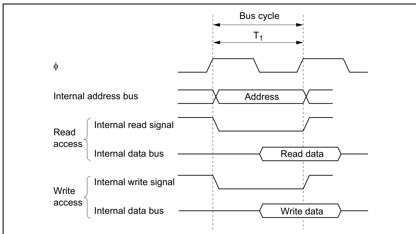
Figure 2-17 On-Chip Memory Access Cycle
