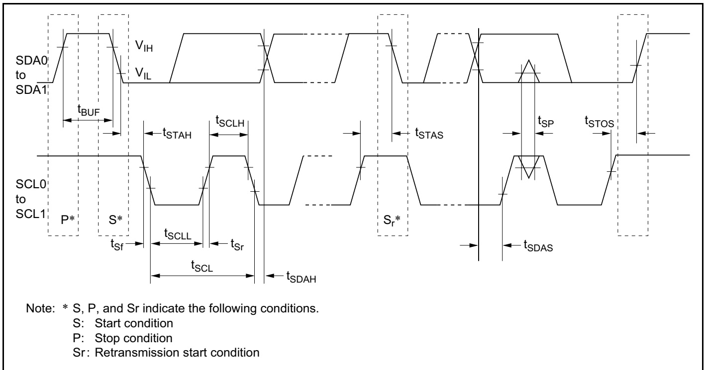
Figure 24-28 I 2 C Bus Interface Input/Output Timing (Option)*
