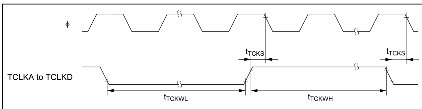
Figure 24-22 TPU Clock Input Timing
