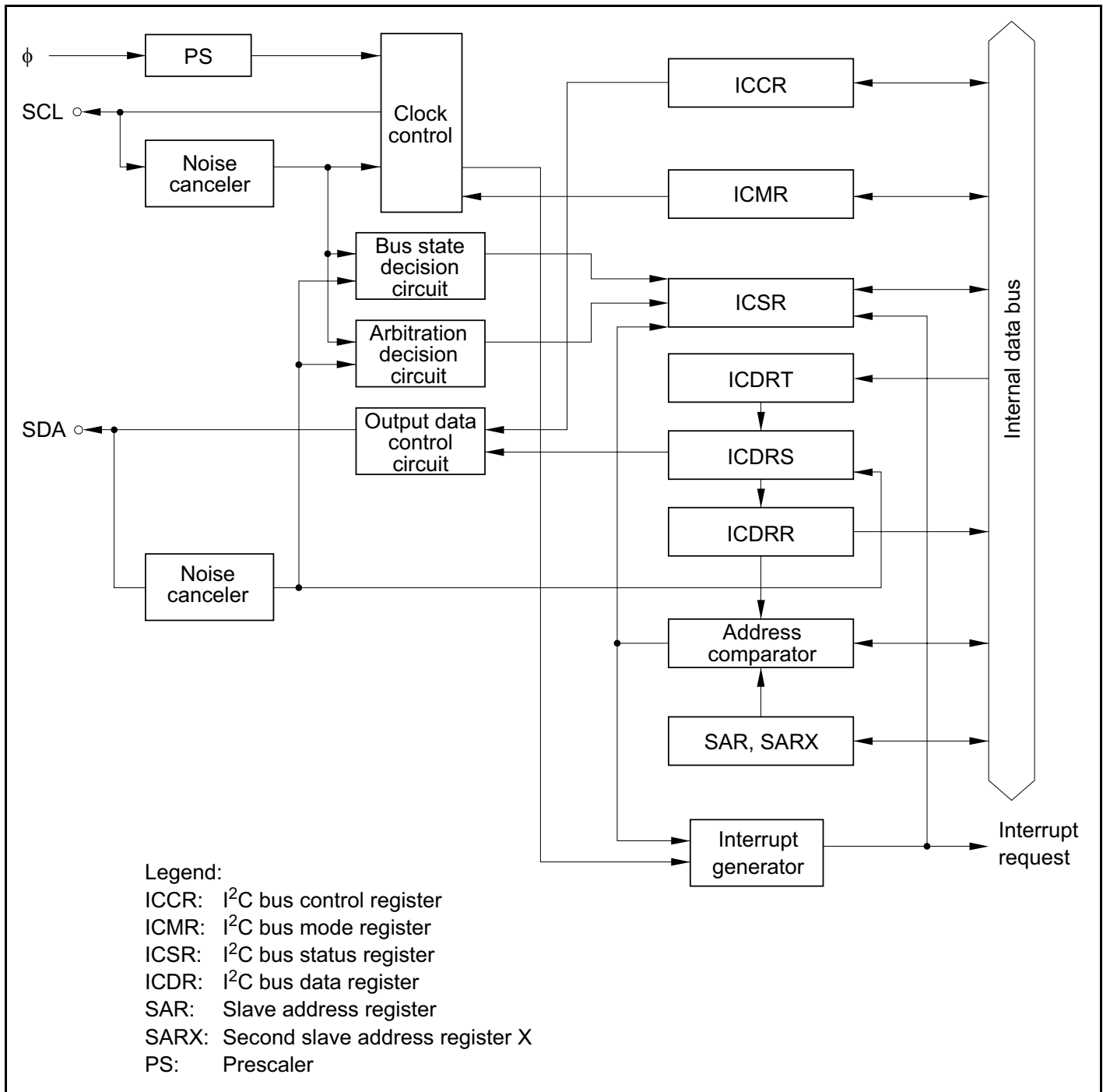
Figure 15-1 Block Diagram of I 2 C Bus Interface
