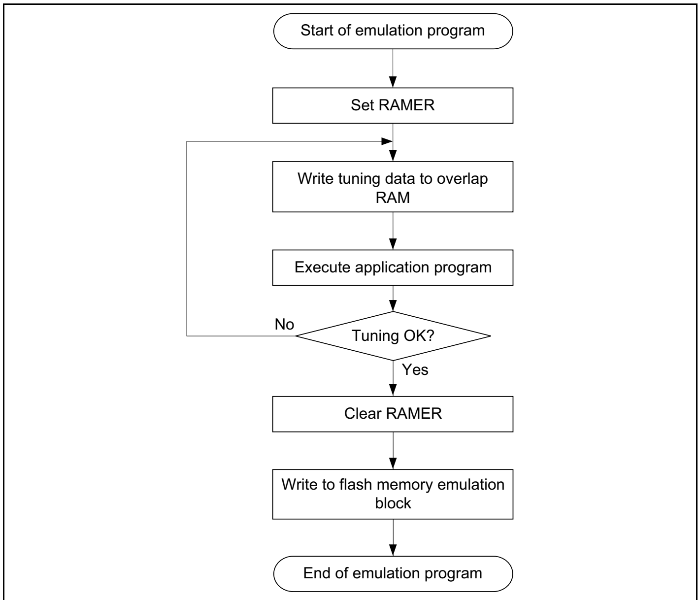
Figure 21C-15 Flowchart for Flash Memory Emulation in RAM
