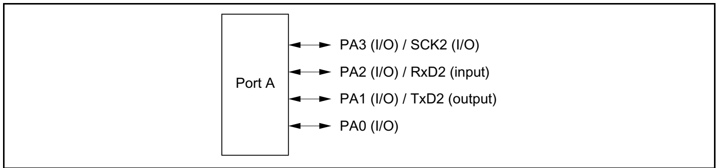
Figure 9-7 Port A Pin Functions (Mode 7)
