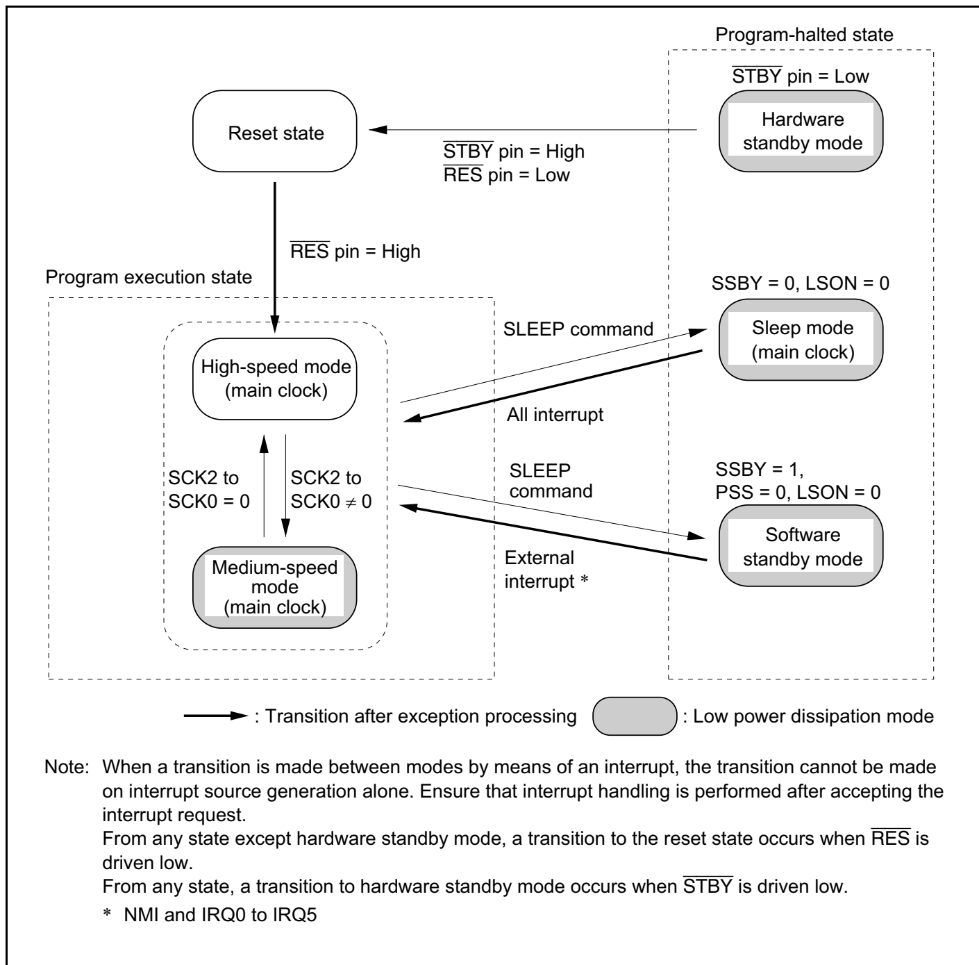
Figure 23A-1 Mode Transition Diagram
