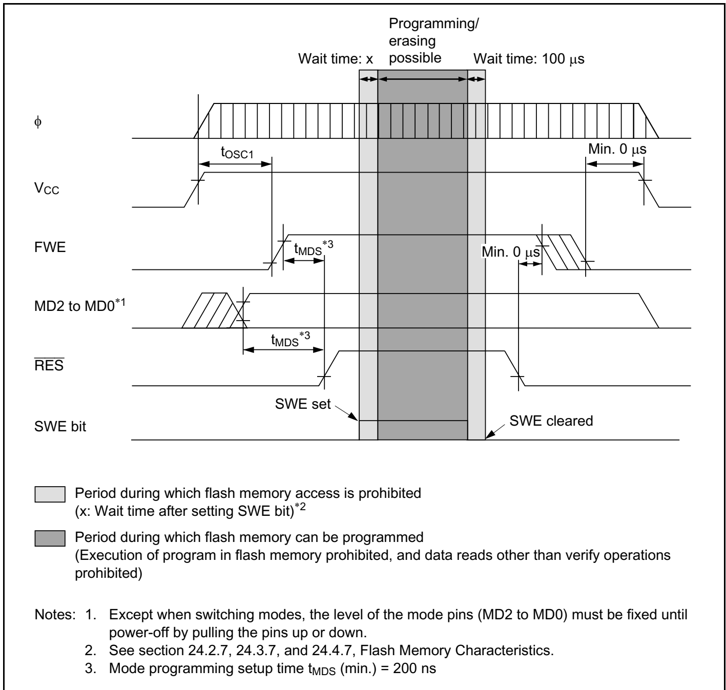
Figure 21B-26 Power-On/Off Timing (Boot Mode)
