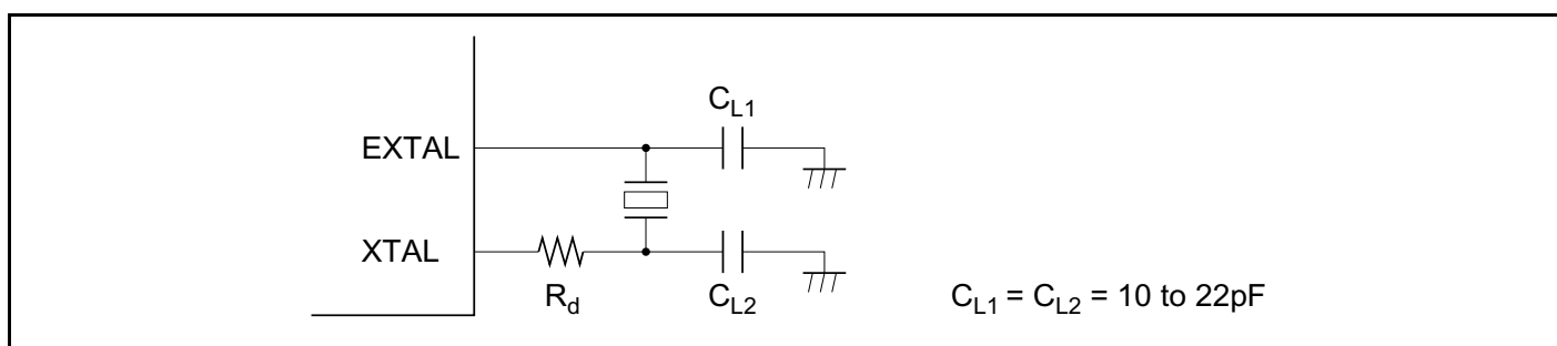
Figure 22A-2 Connection of Crystal Resonator (Example)
