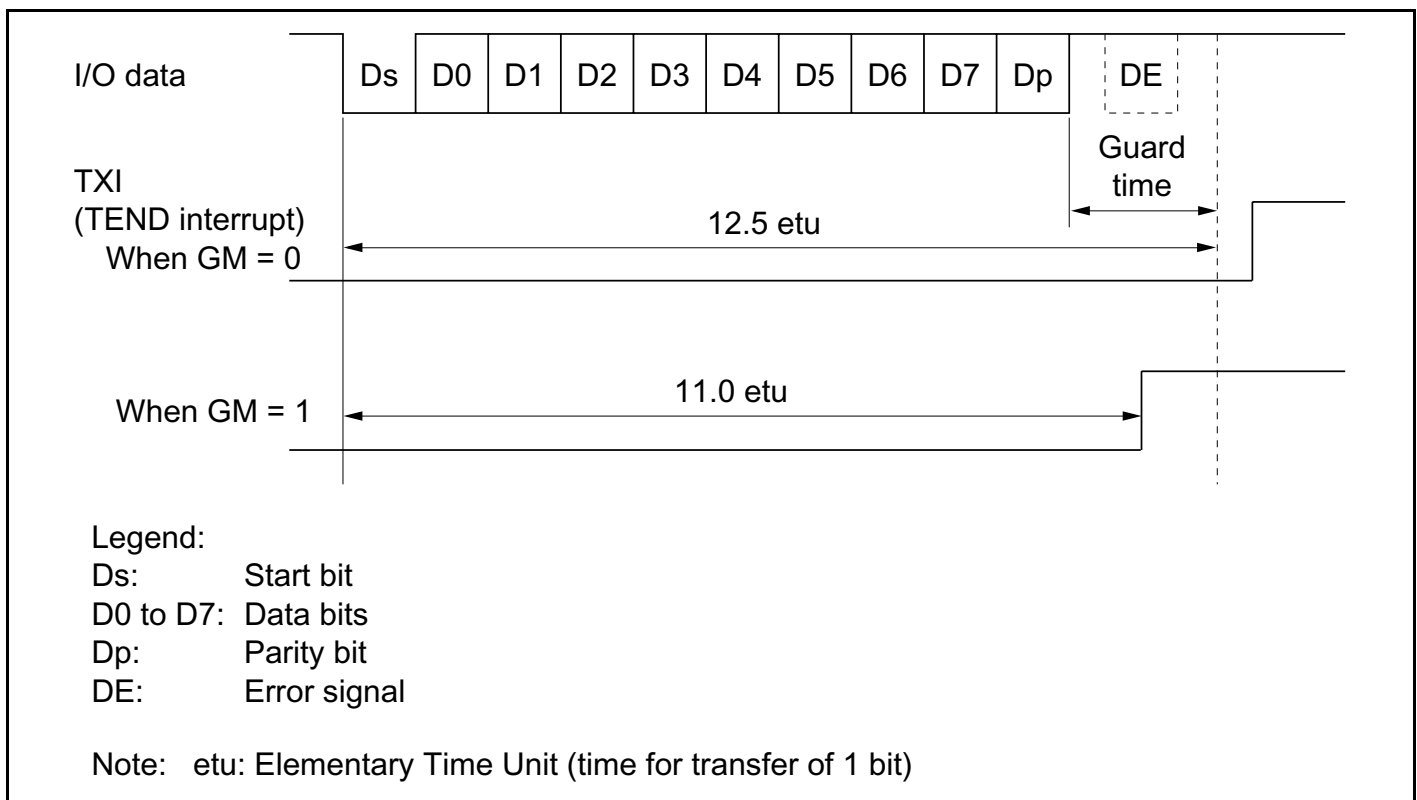
Figure 14-6 TEND Flag Generation Timing in Transmission Operation
