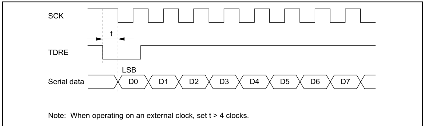
Figure 13-22 Example of Clocked Synchronous Transmission by DTC
