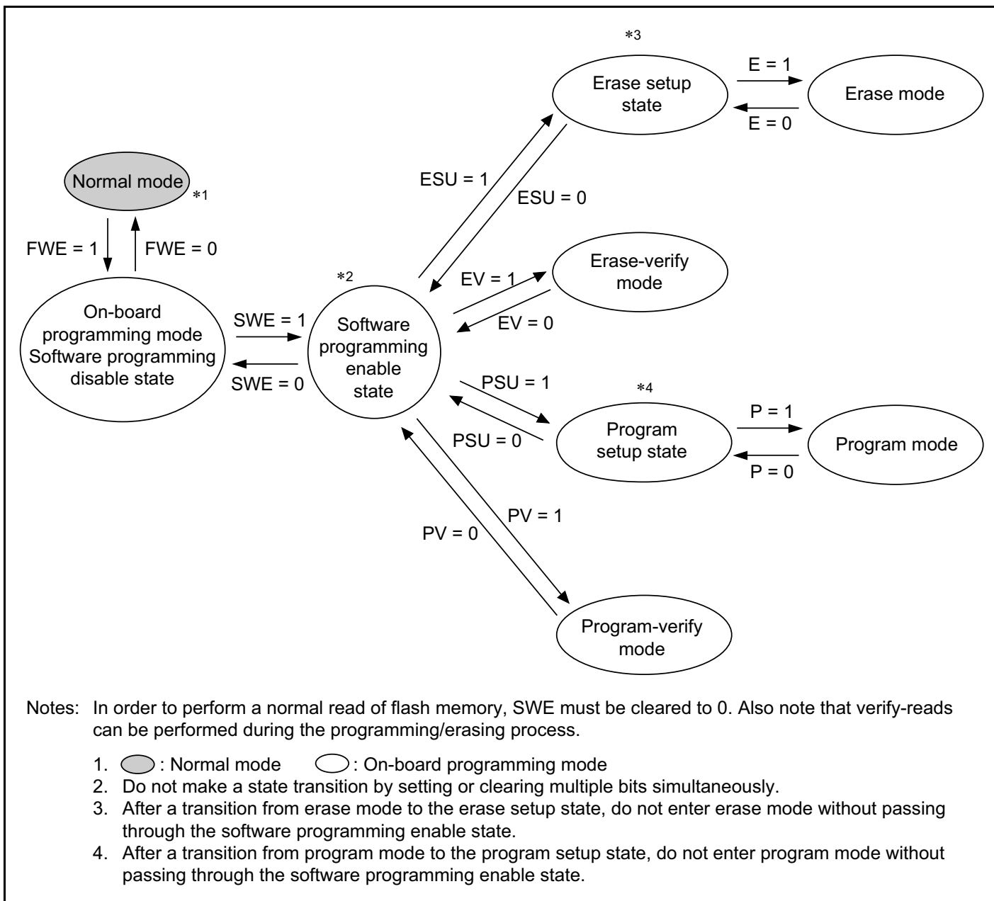
Figure 21A-11 FLMCR1 Bit Settings and State Transitions
