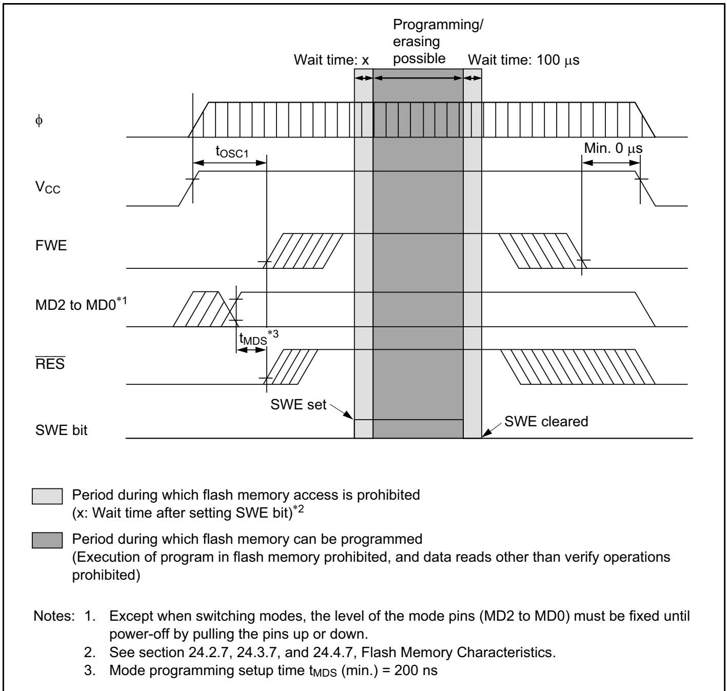
Figure 21C-27 Power-On/Off Timing (User Program Mode)
