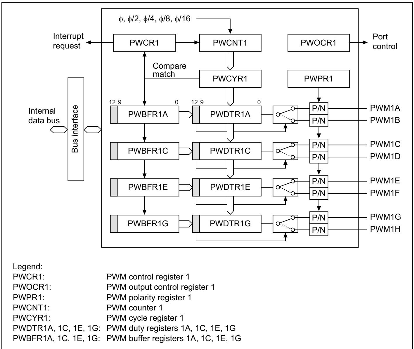
Figure 19-1 Block Diagram of PWM Channel 1
