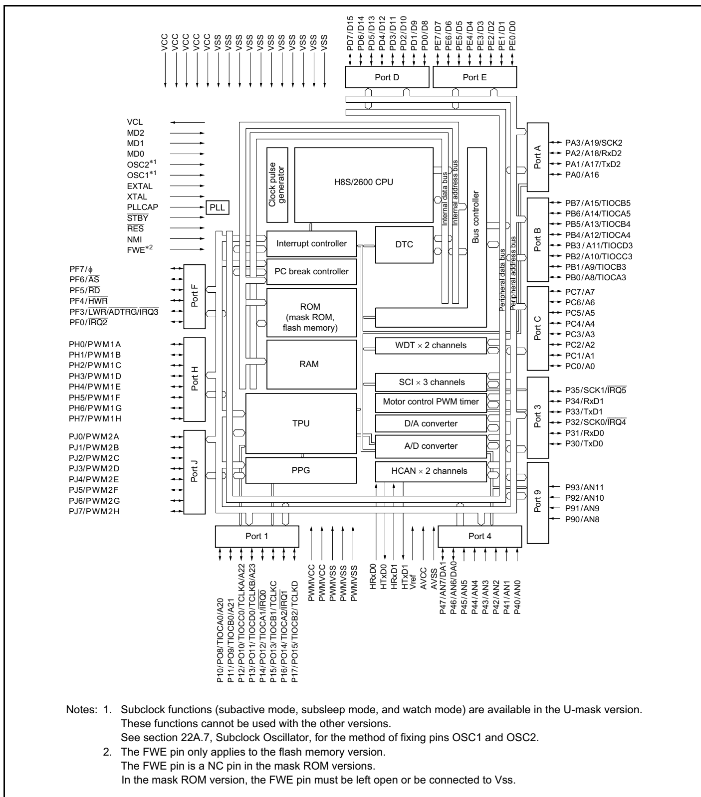
Figure 1-1 (a) Internal Block Diagram of H8S/2636
