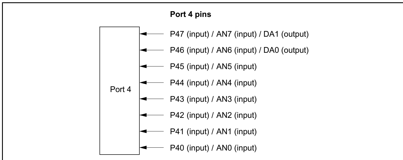
Figure 9-3 Port 4 Pin Functions
