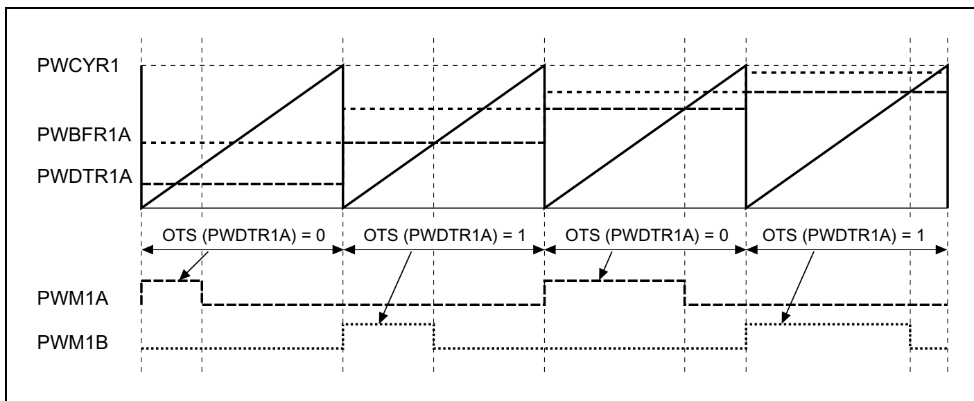
Figure 19-10 PWM Channel 1 Operation
