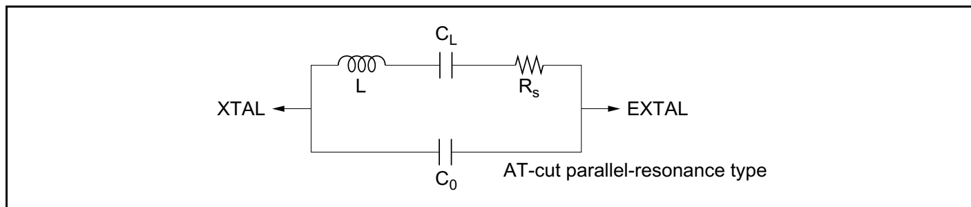
Figure 22A-3 Crystal Resonator Equivalent Circuit
