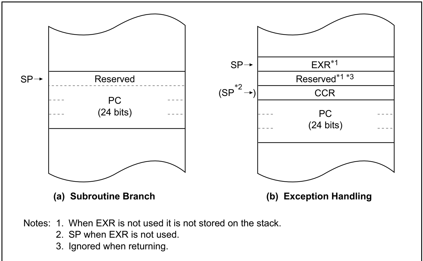
Figure 2-5 Stack Structure in Advanced Mode
