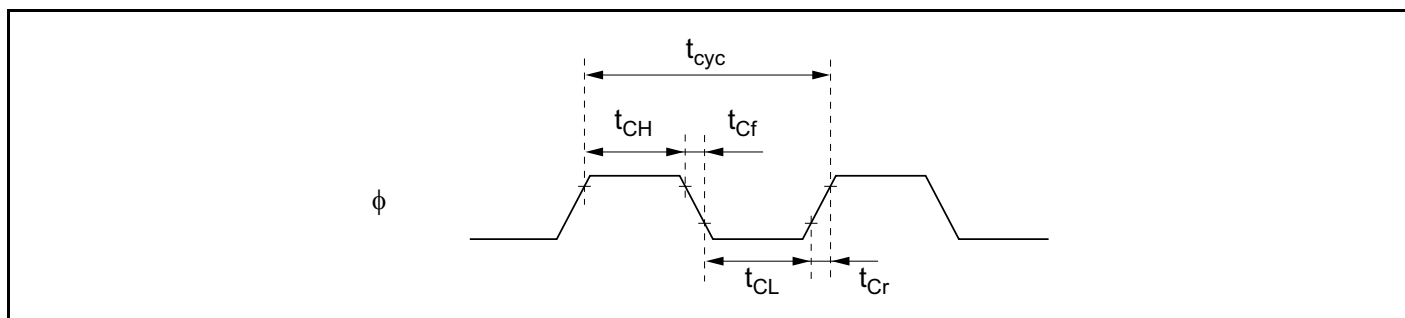
Figure 24-9 System Clock Timing
