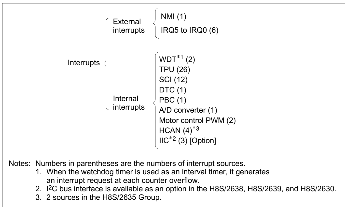
Figure 4-4 Interrupt Sources and Number of Interrupts
