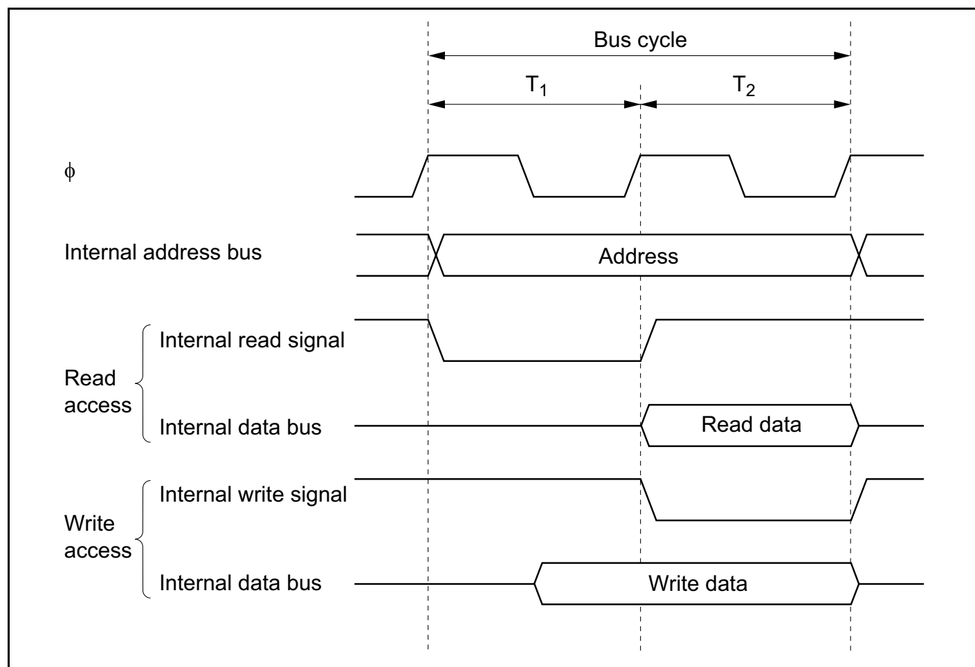
Figure 2-19 On-Chip Supporting Module Access Cycle
