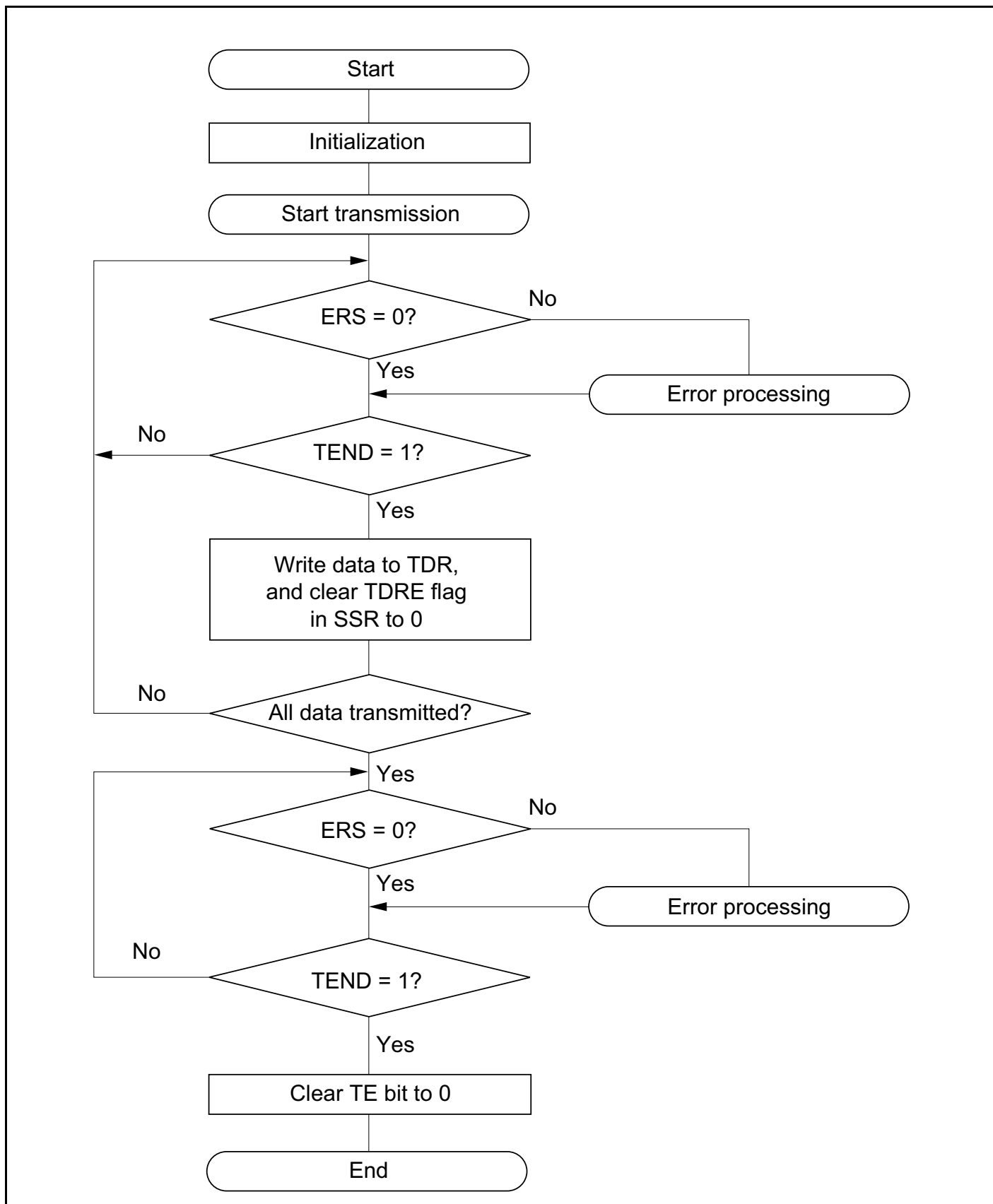
Figure 14-4 Example of Transmission Processing Flow
