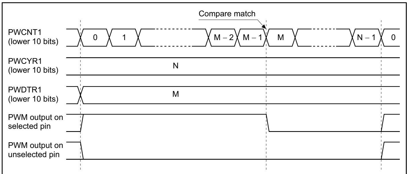
Figure 19-4 Duty Register Compare Match (OPS = 0 in PWPR1)
