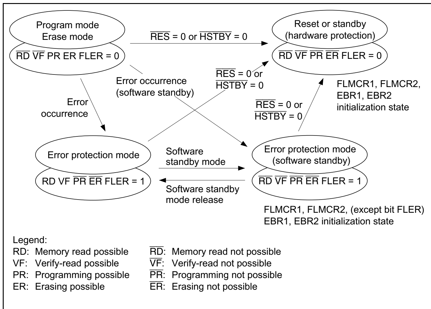
Figure 21B-14 Flash Memory State Transitions
