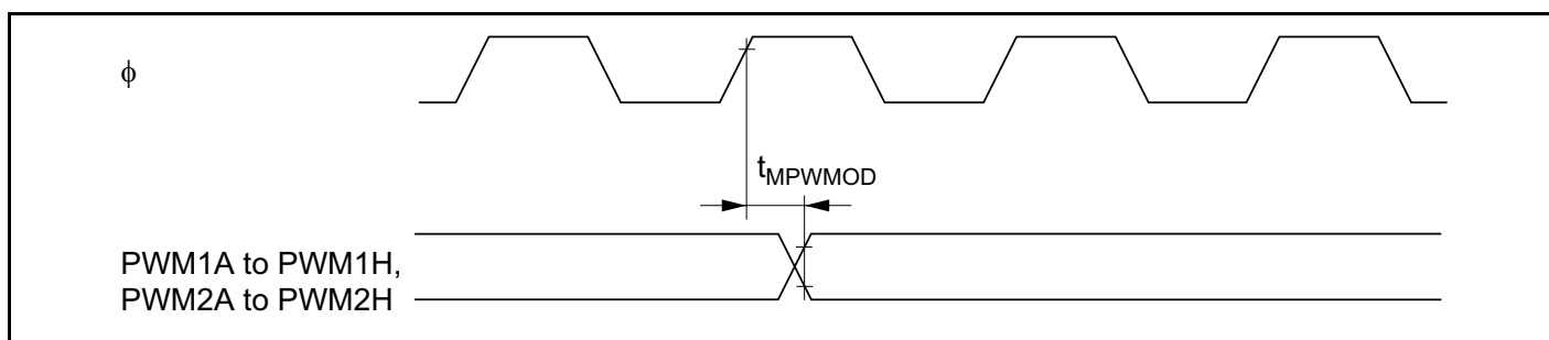
Figure 24-23 Motor Control PWM Output Timing
