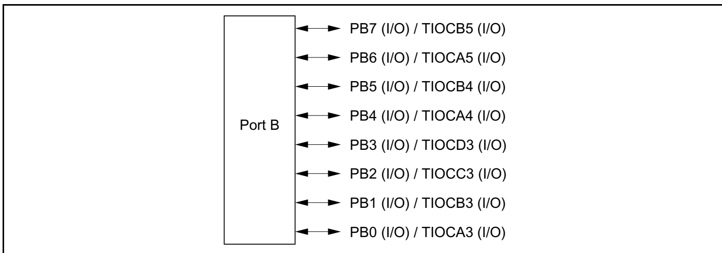
Figure 9-10 Port B Pin Functions (Mode 7)
