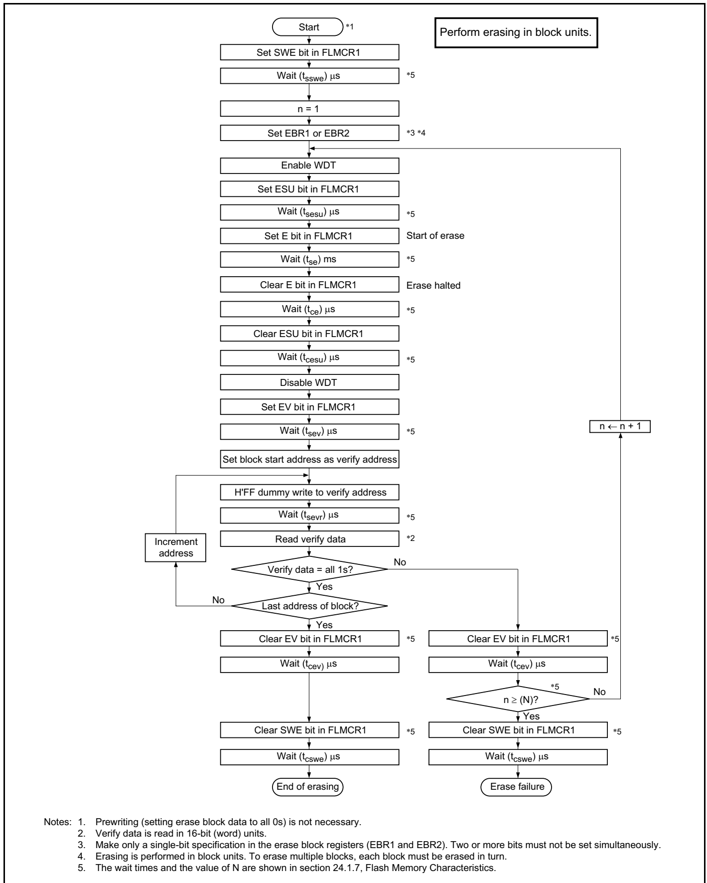
Figure 21A-13 Erase/Erase-Verify Flowchart
