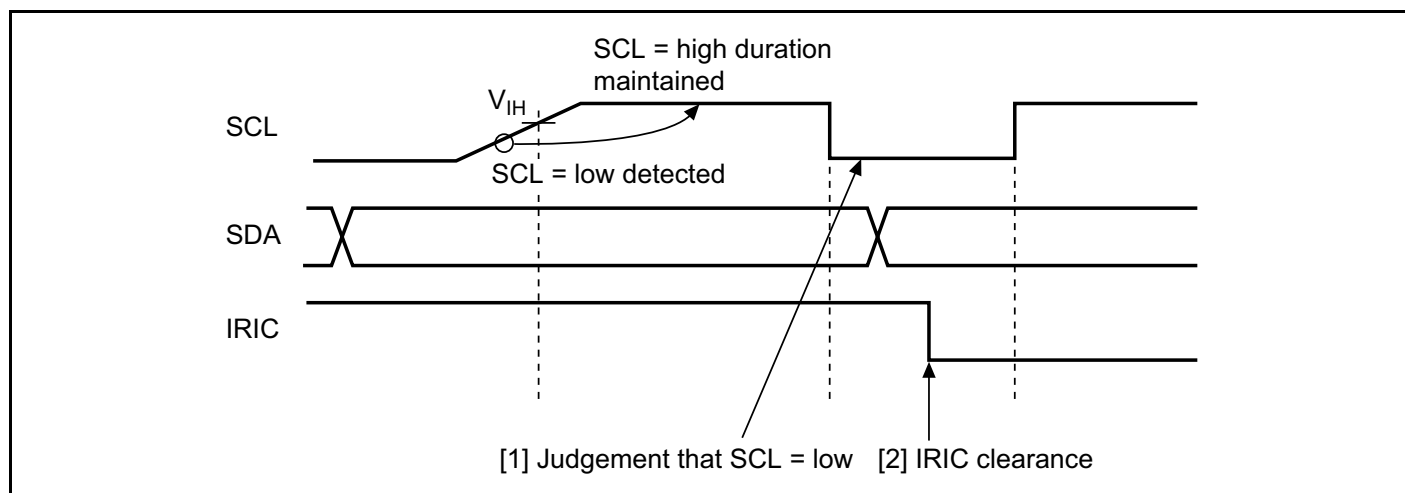
Figure 15-24 IRIC Flag Clearance in WAIT = 1 Status
