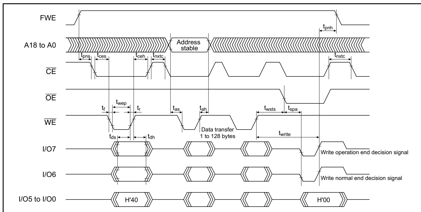
Figure 21A-22 Auto-Program Mode Timing Waveforms
