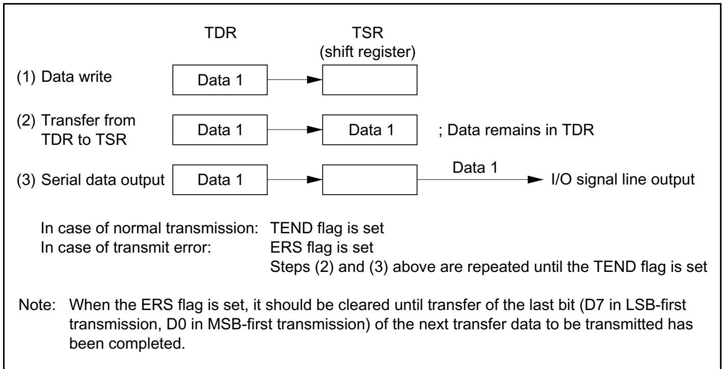
Figure 14-5 Relation Between Transmit Operation and Internal Registers
