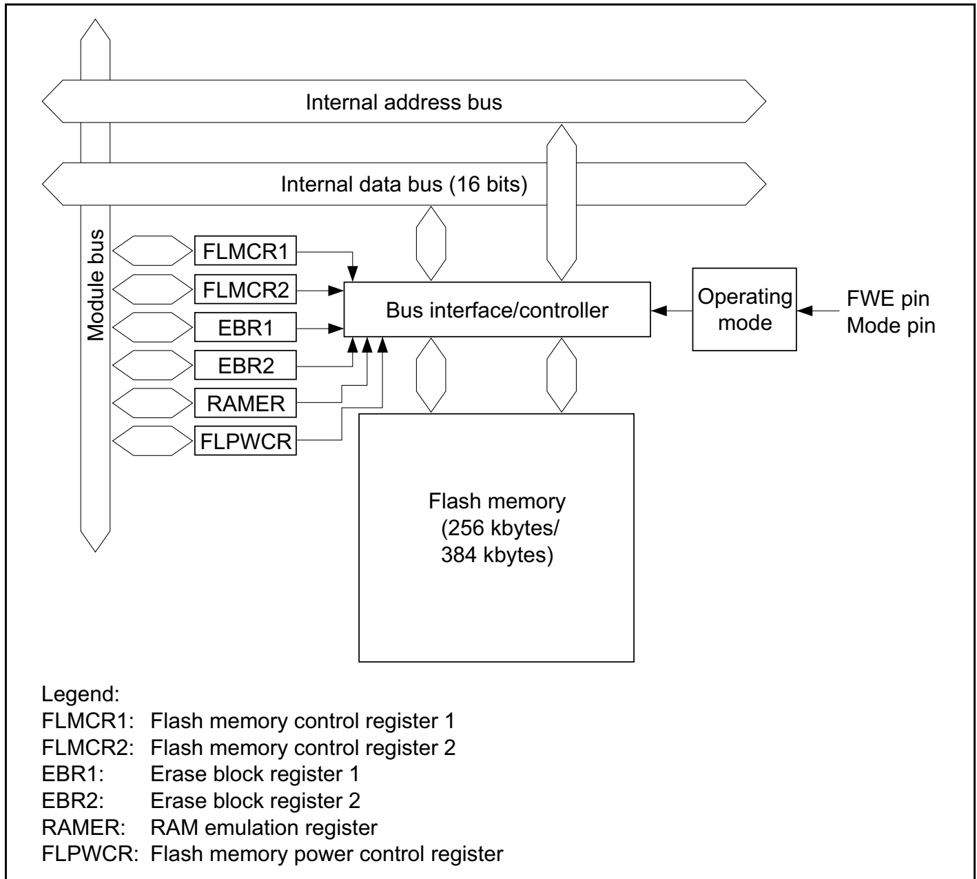
Figure 21B-2 Block Diagram of Flash Memory
