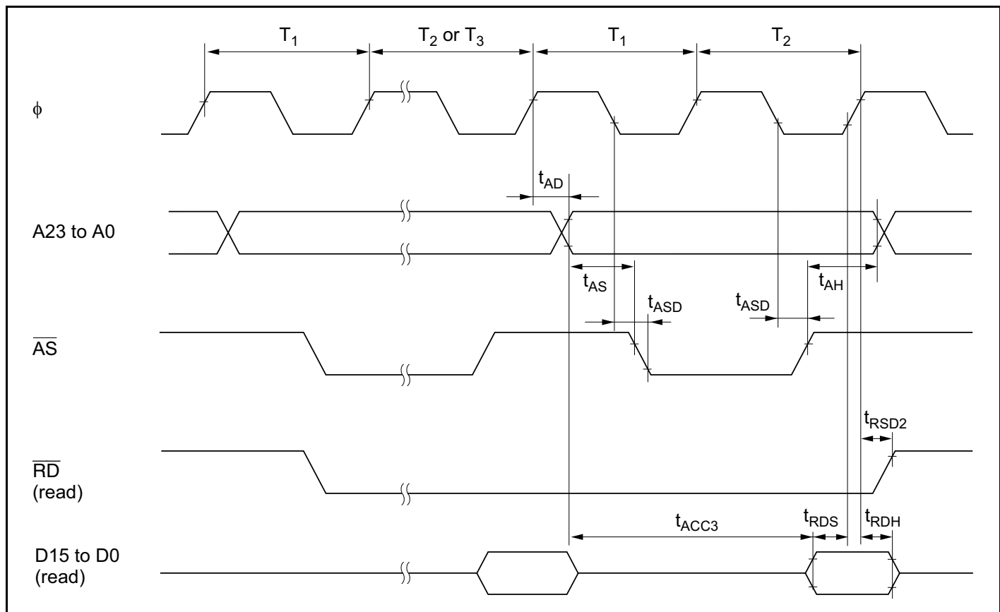
Figure 24-16 Burst ROM Access Timing (Two-State Access)
