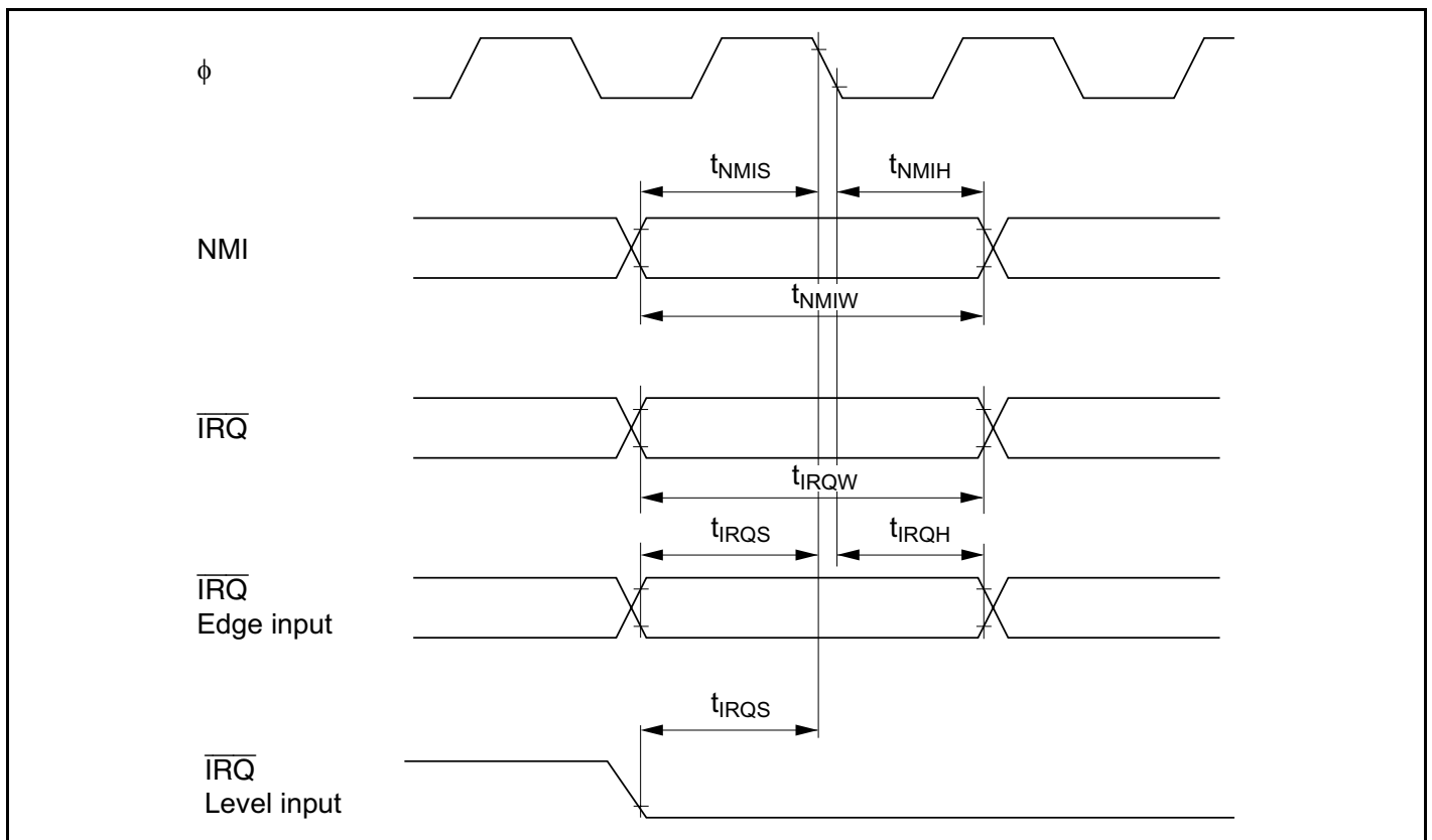
Figure 24-12 Interrupt Input Timing
