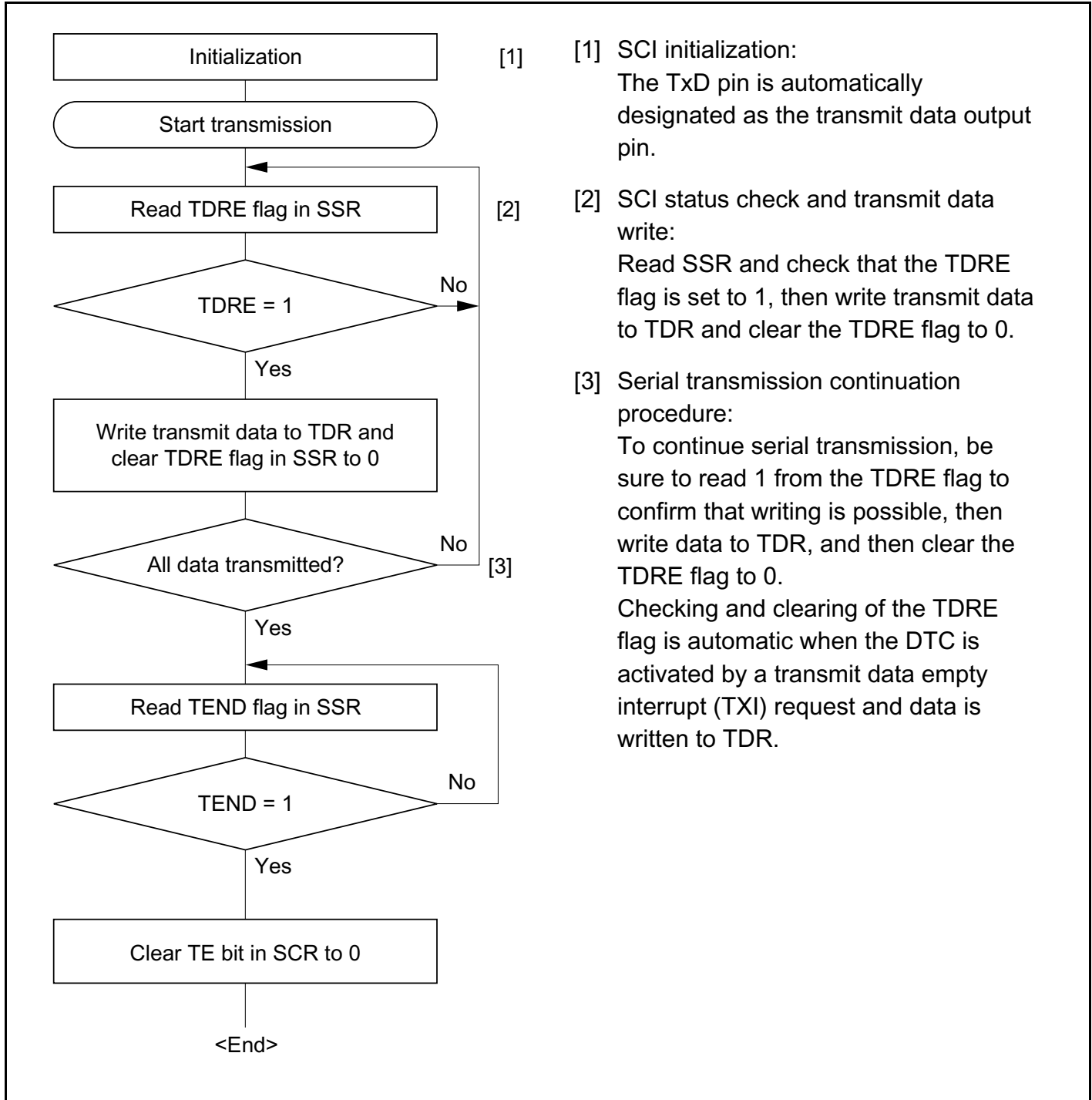
Figure 13-16 Sample Serial Transmission Flowchart
