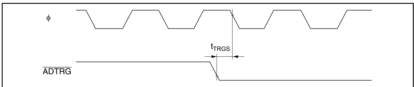
Figure 24-26 A/D Converter External Trigger Input Timing
