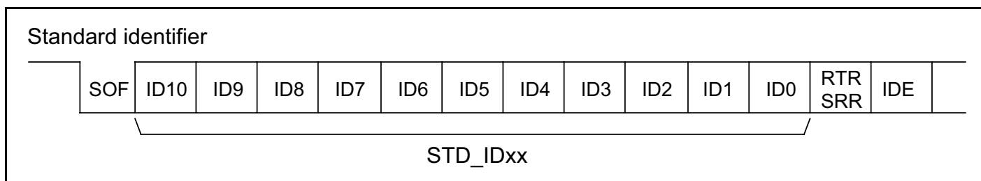
Figure 16-2 Standard identifier
