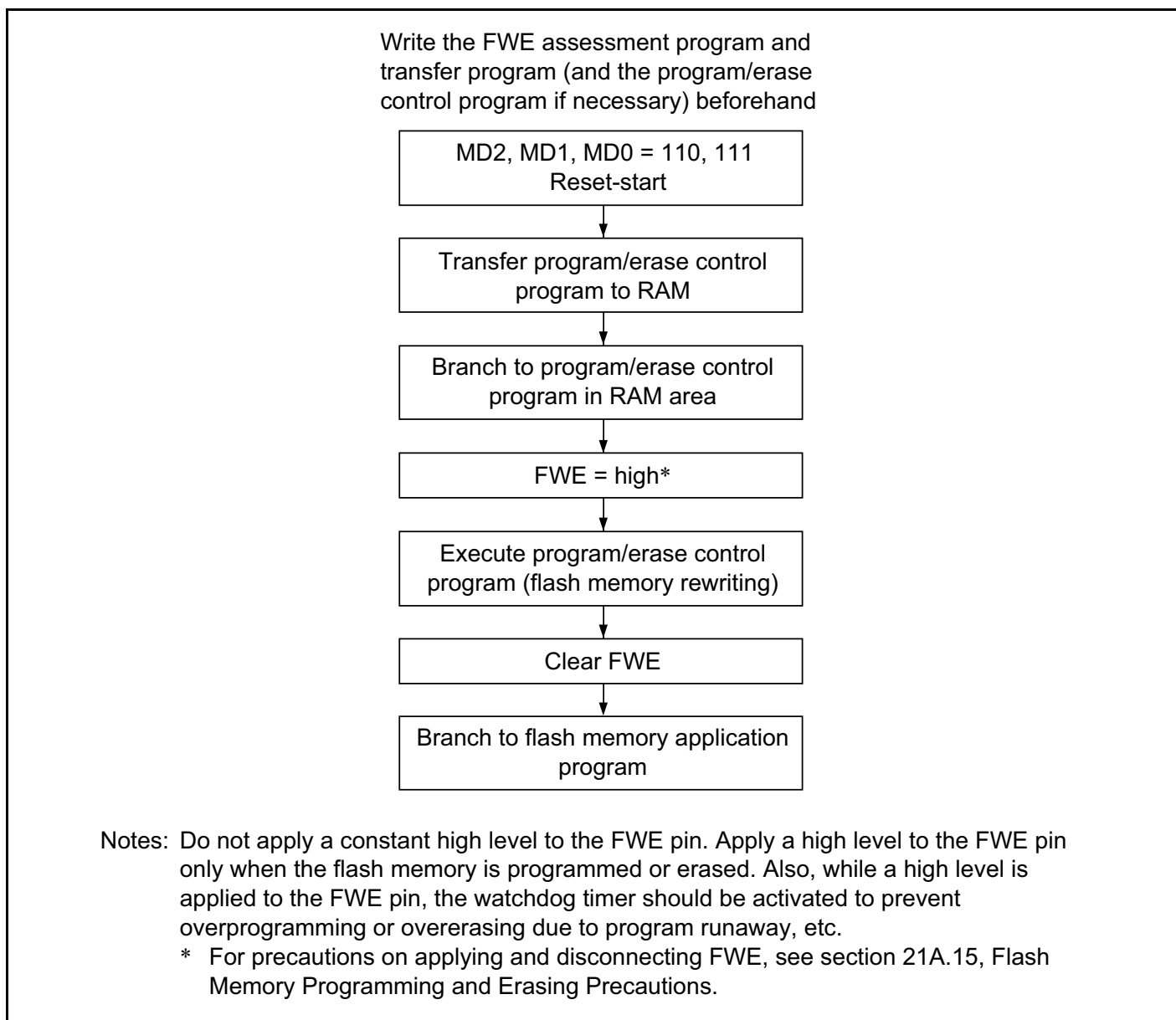
Figure 21A-10 User Program Mode Execution Procedure
