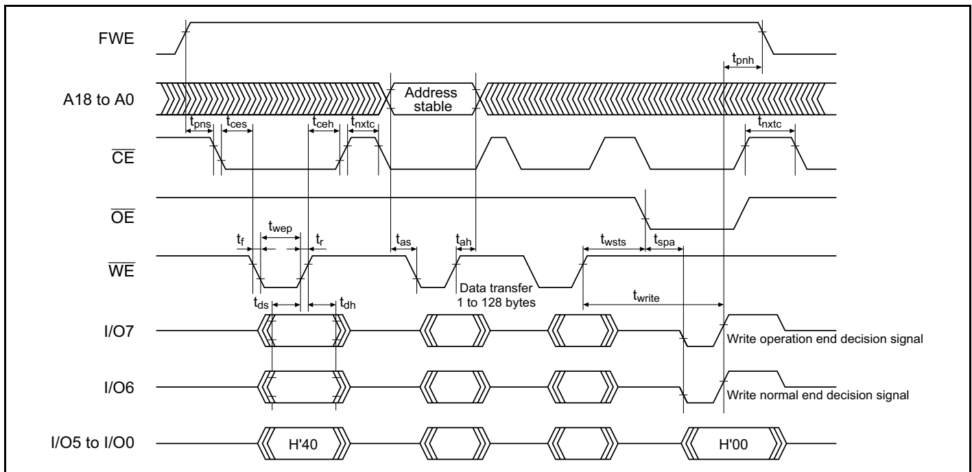
Figure 21C-22 Auto-Program Mode Timing Waveforms
