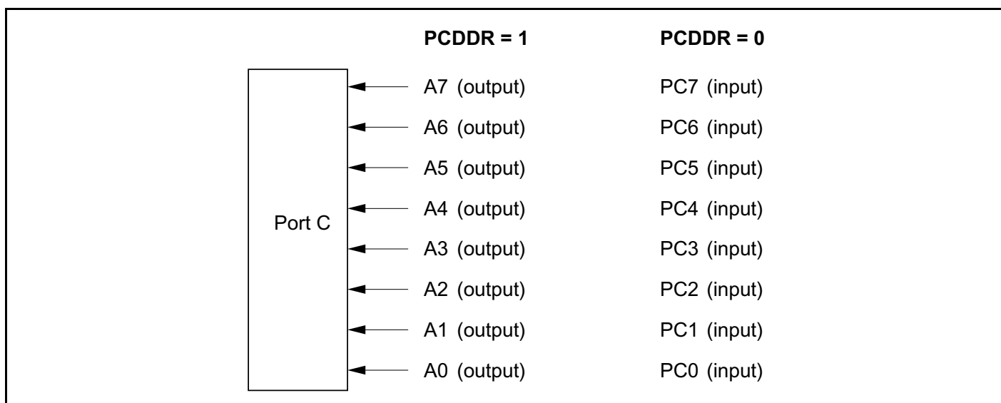
Figure 9-13 Port C Pin Functions (Mode 6)
