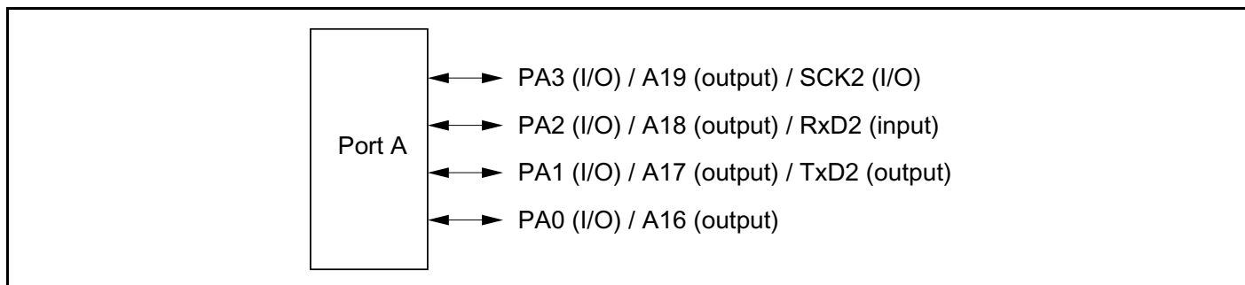
Figure 9-6 Port A Pin Functions (Modes 4 to 6)
