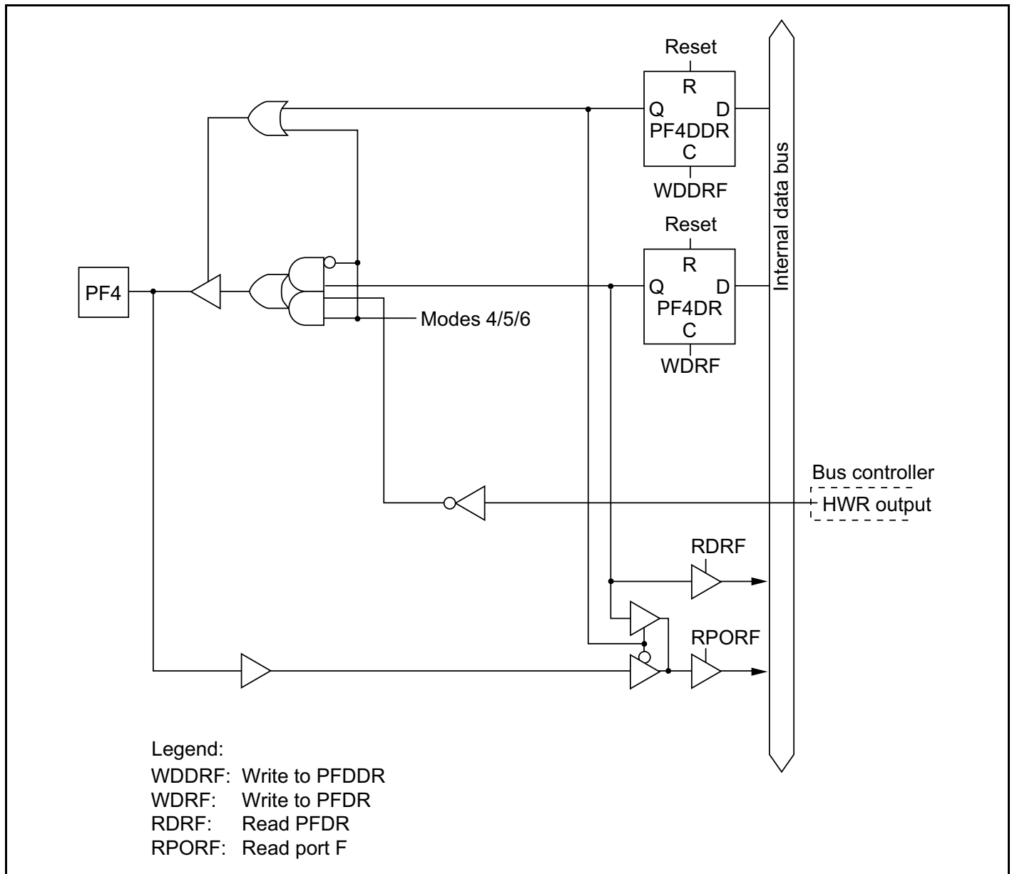
Figure C-10 (c) Port F Block Diagram (Pin PF4)
