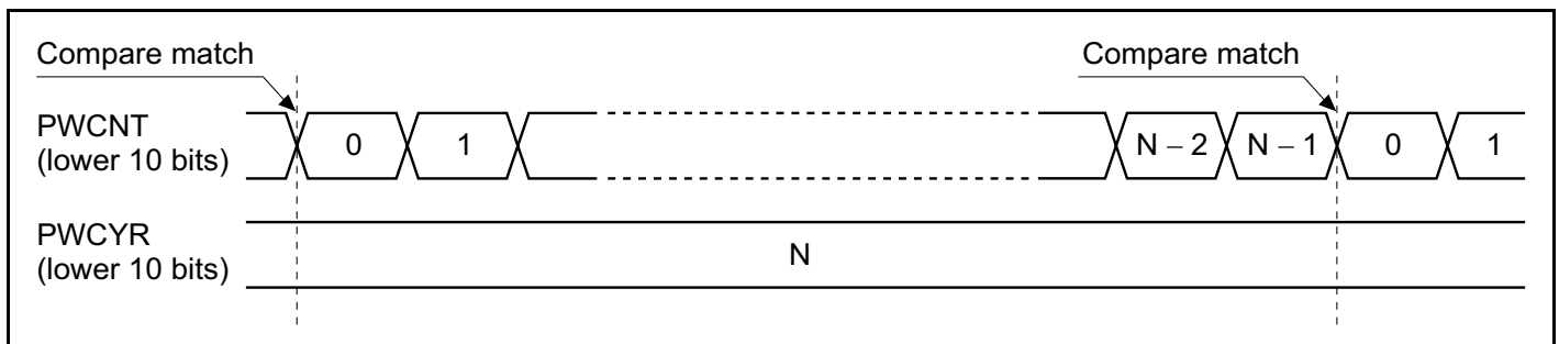
Figure 19-3 Cycle Register Compare Match
