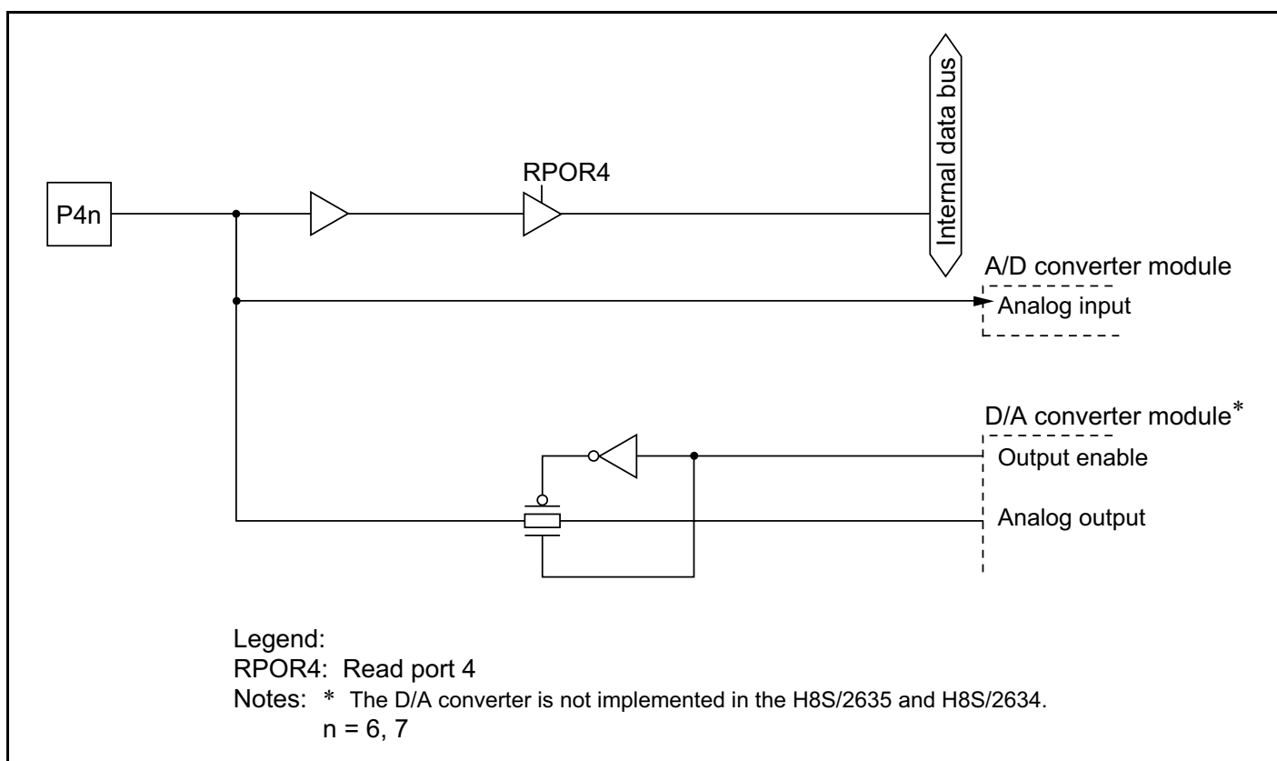
Figure C-3 (b) Port 4 Block Diagram (Pins P46, P47)
