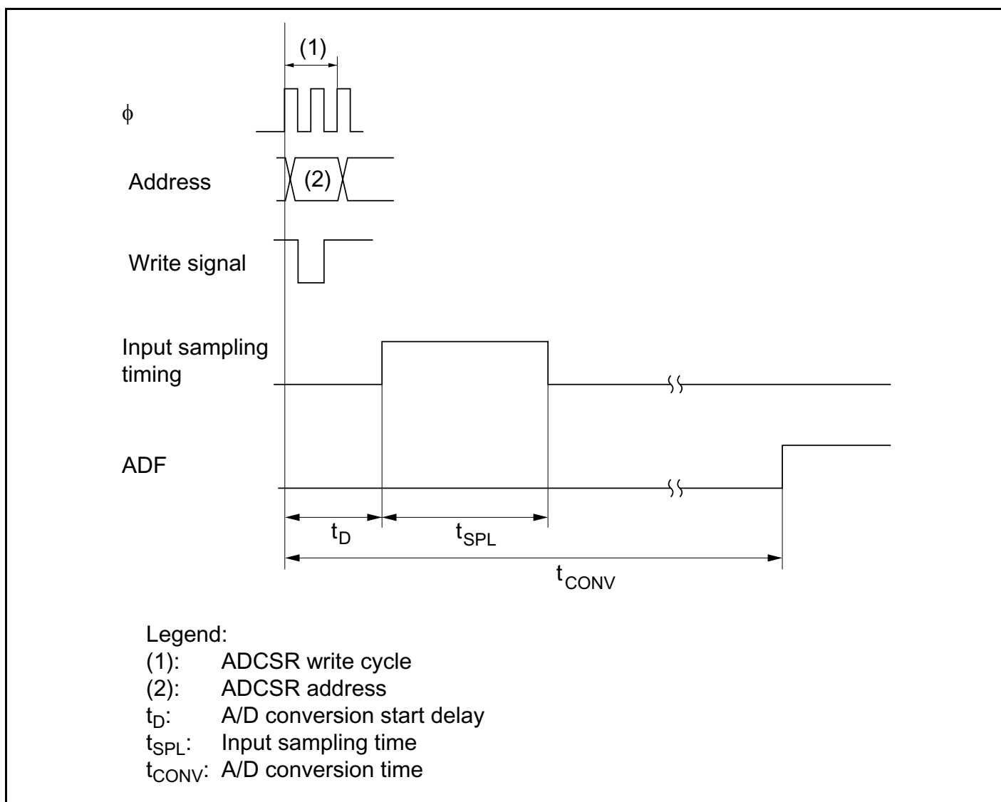
Figure 17-5 A/D Conversion Timing
