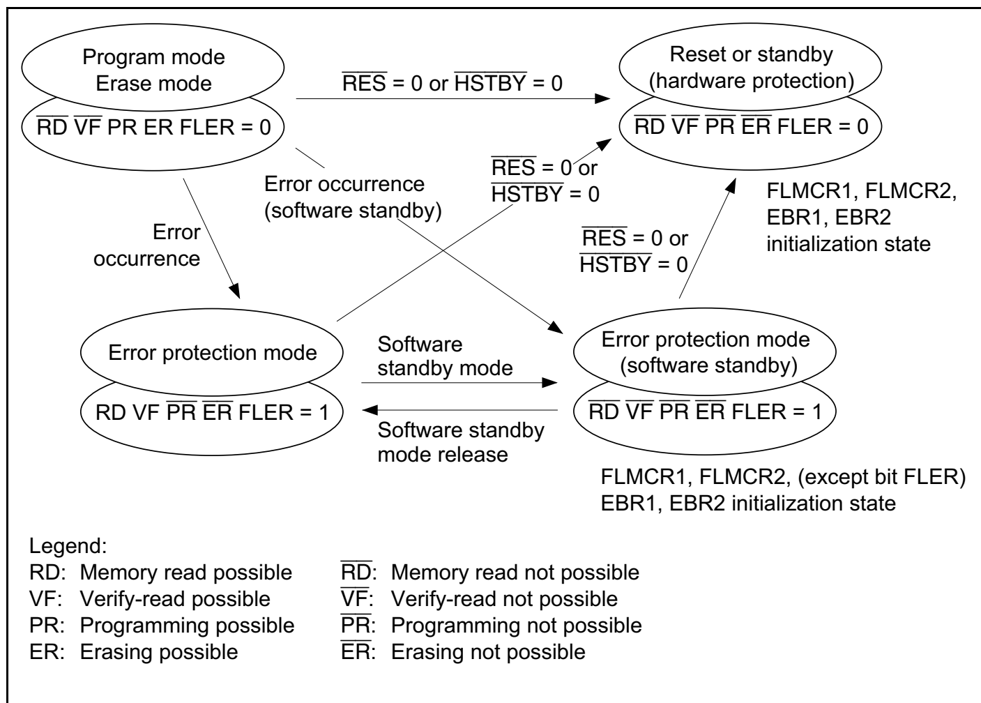
Figure 21C-14 Flash Memory State Transitions
