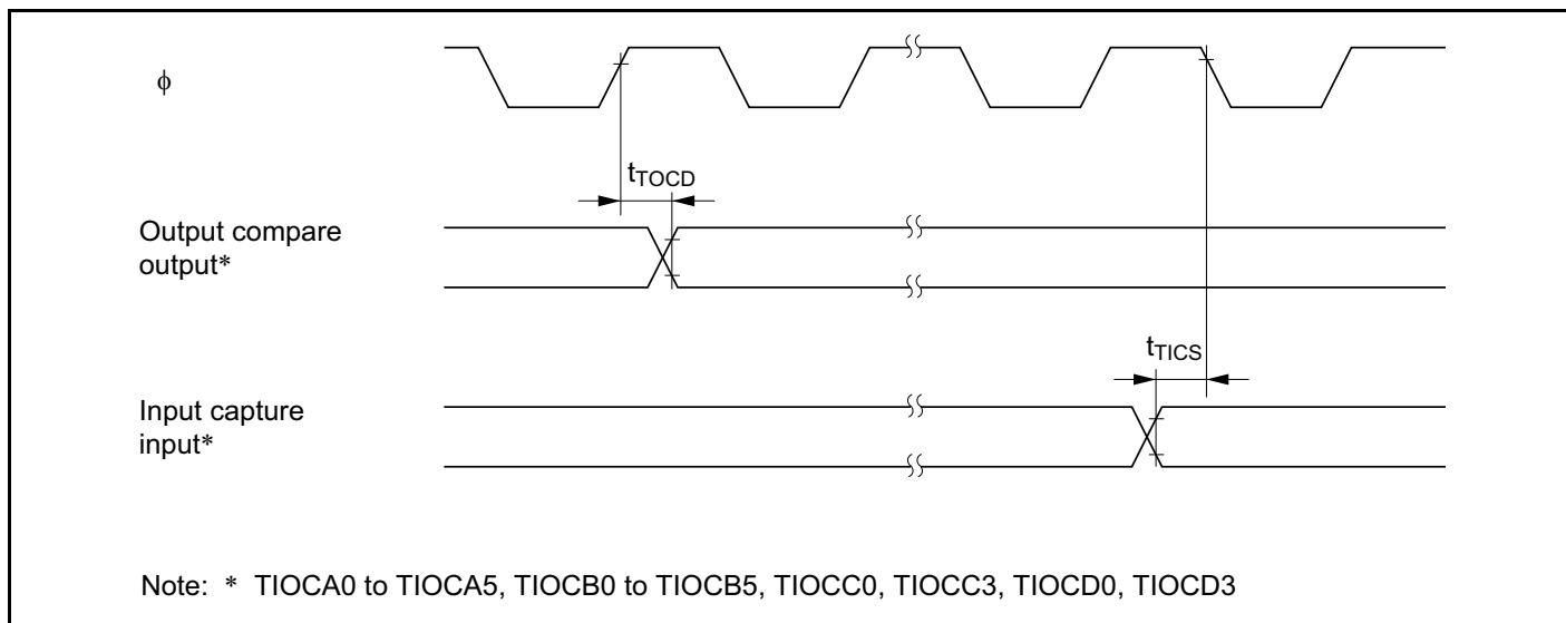
Figure 24-21 TPU Input/Output Timing
