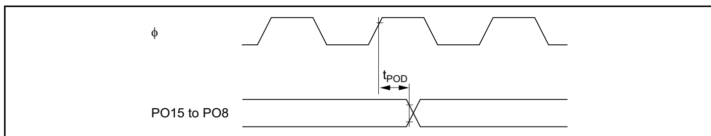
Figure 24-20 PPG Output Timing*
