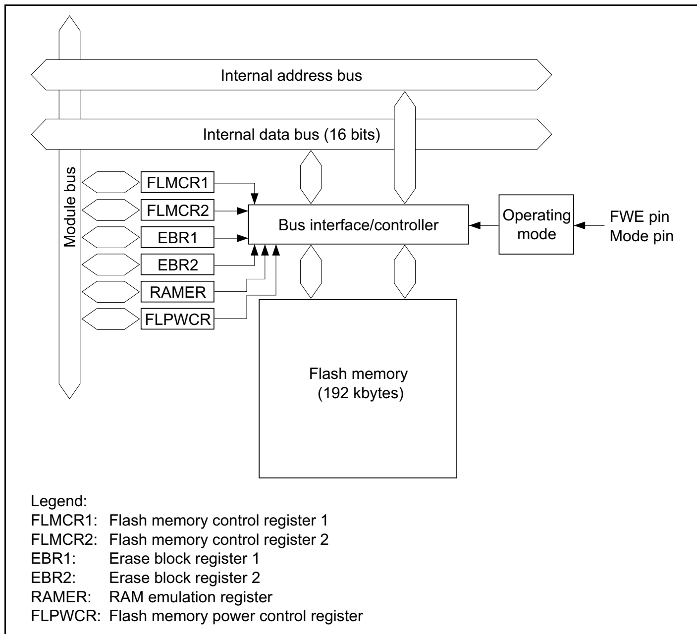
Figure 21C-2 Block Diagram of Flash Memory
