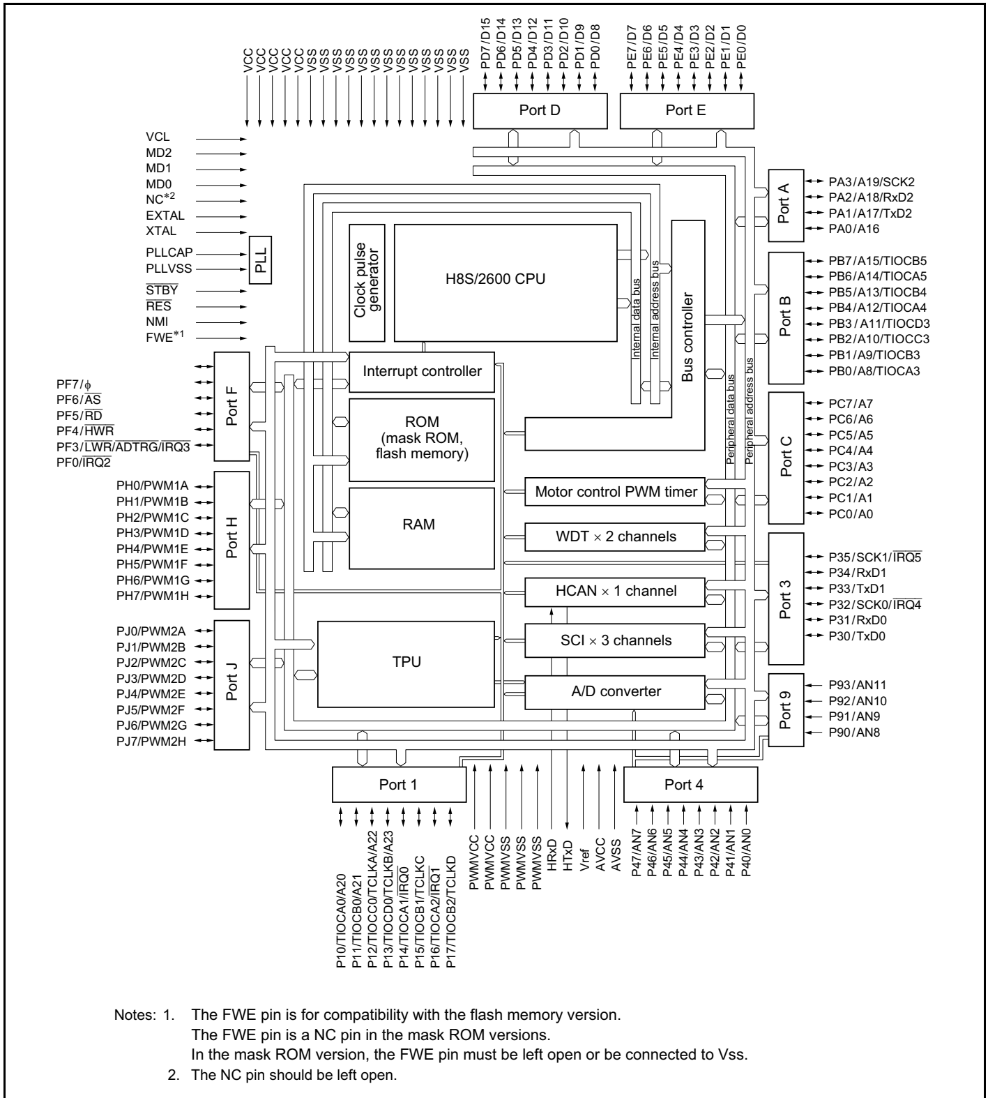
Figure 1-1 (c) Internal Block Diagram of H8S/2635 Group
