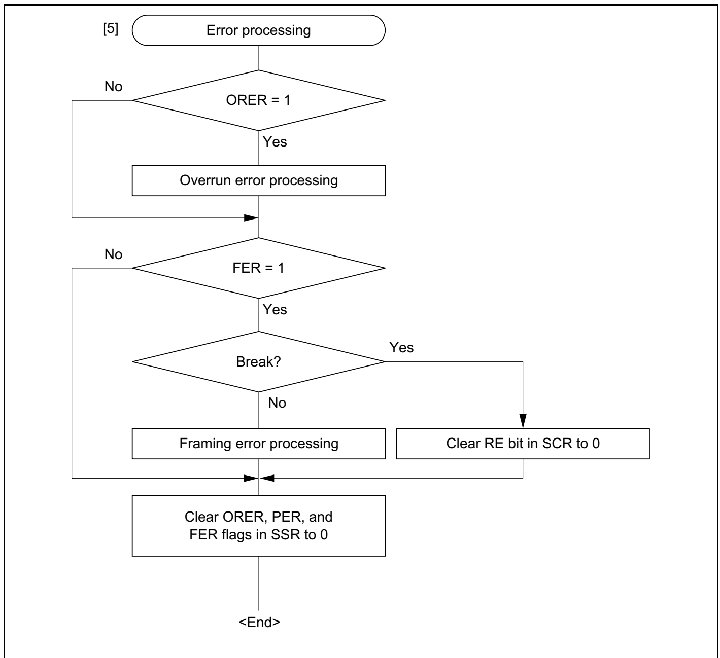
Figure 13-12 Sample Multiprocessor Serial Reception Flowchart (cont)
