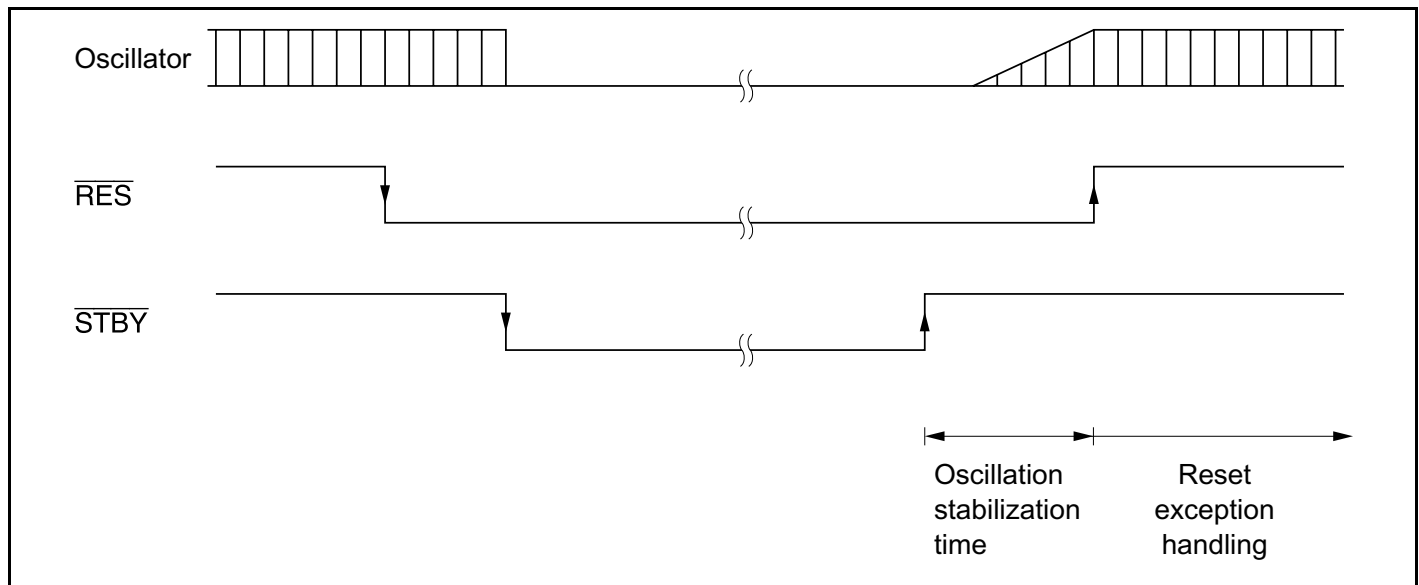
Figure 23B-4 Hardware Standby Mode Timing
