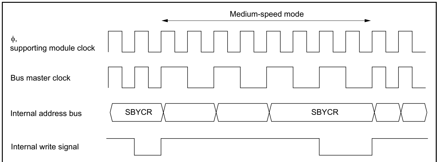
Figure 23A-2 Medium-Speed Mode Transition and Clearance Timing
