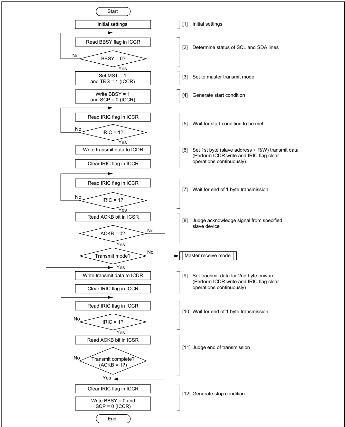
Figure 15-7 Flowchart for Master Transmit Mode (Example)
