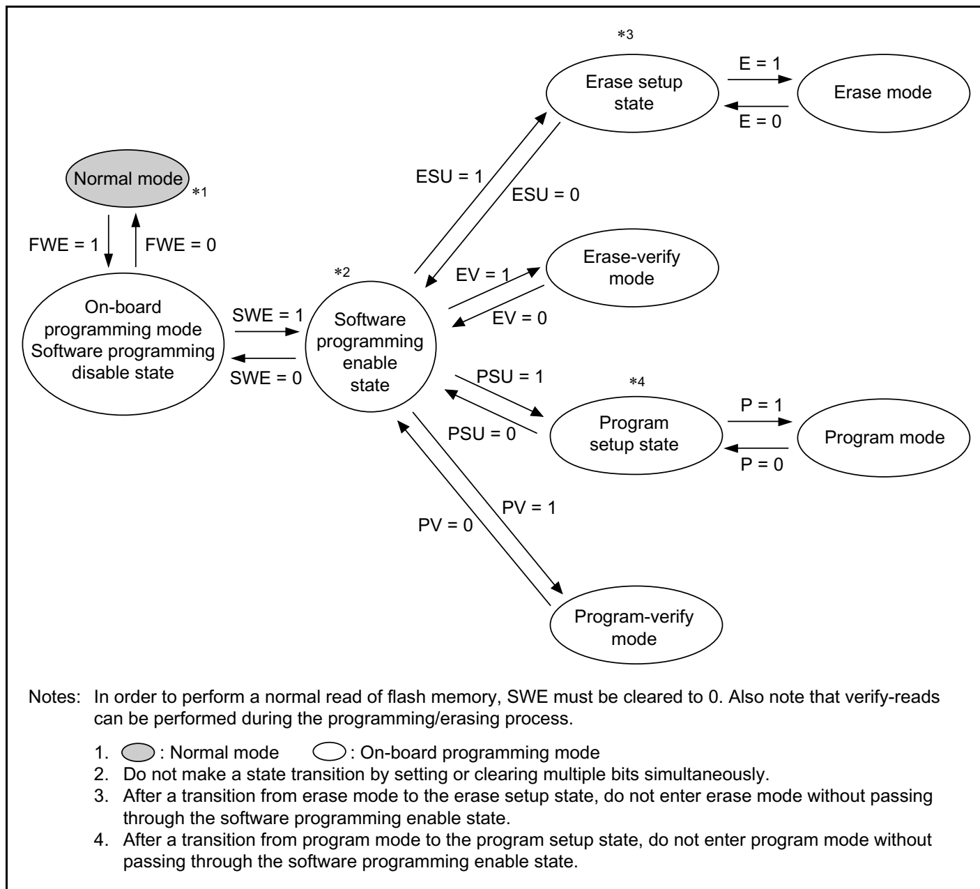
Figure 21B-11 FLMCR1 Bit Settings and State Transitions
