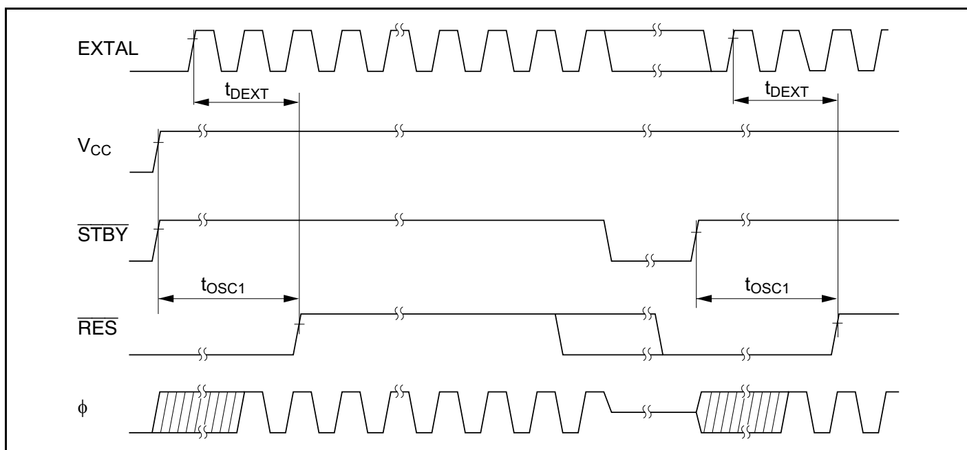
Figure 24-10 Oscillator Settling Timing
