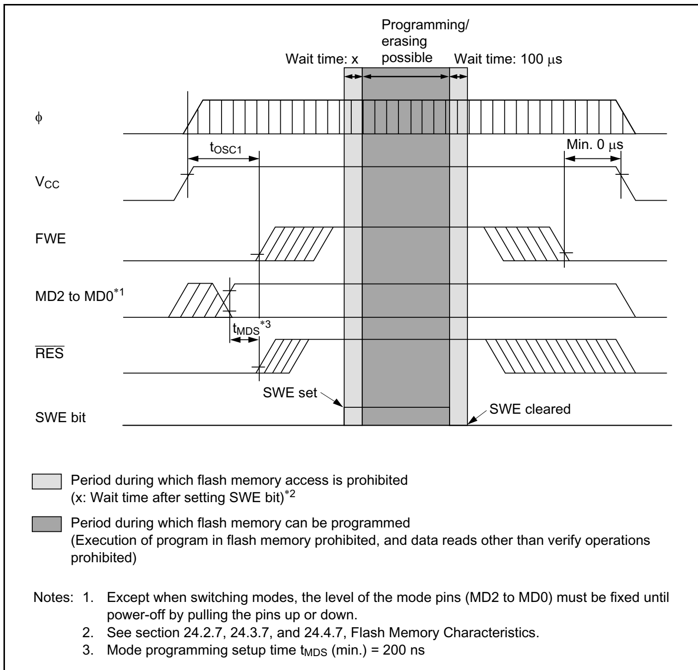
Figure 21B-27 Power-On/Off Timing (User Program Mode)
