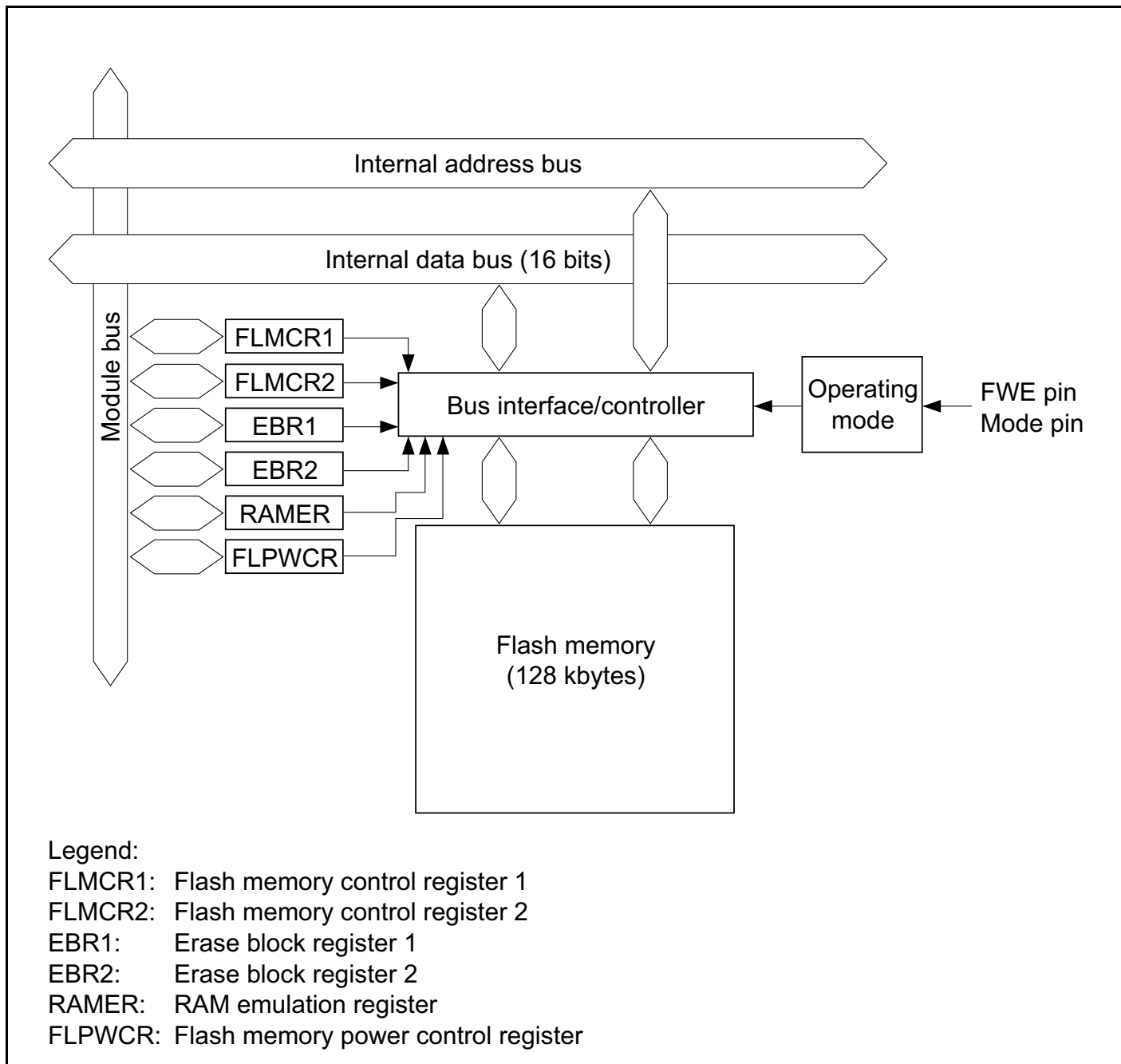
Figure 21A-2 Block Diagram of Flash Memory
