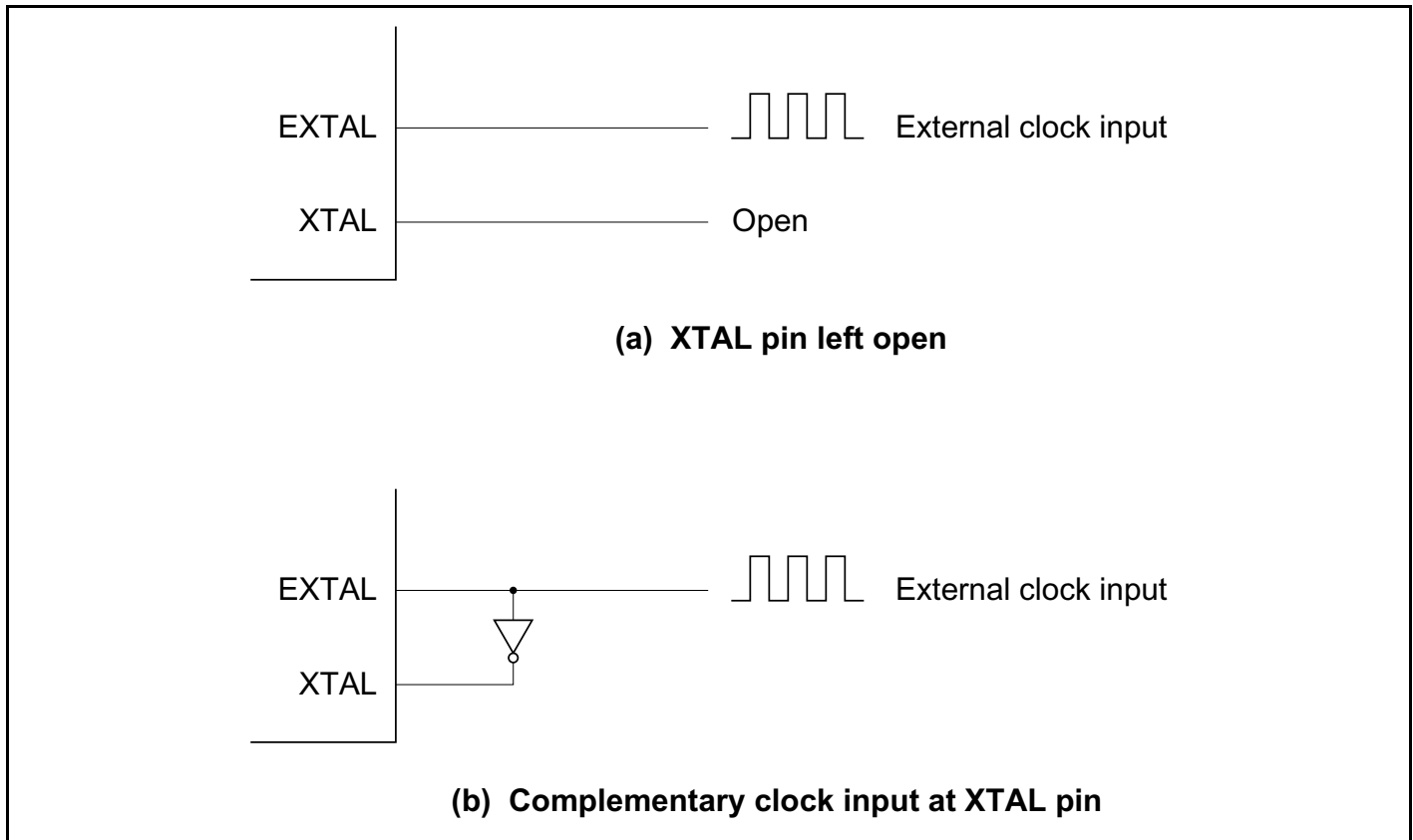
Figure 22A-6 External Clock Input (Examples)
