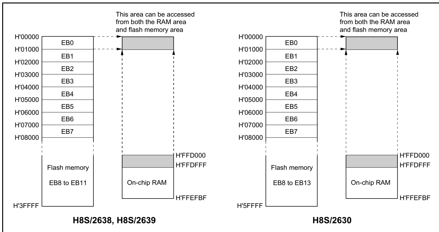
Figure 21B-16 Example of RAM Overlap Operation
