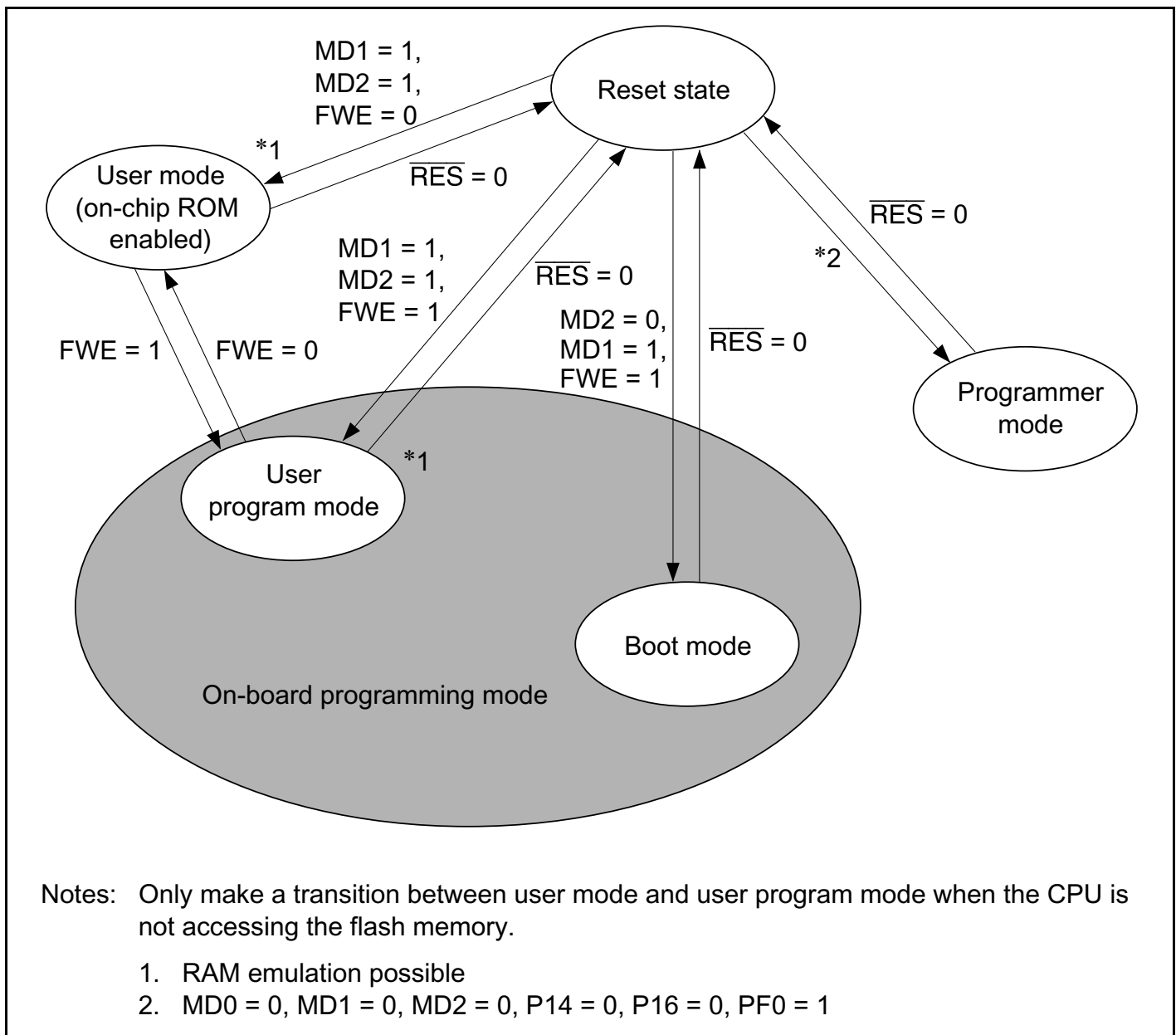
Figure 21A-3 Flash Memory State Transitions
