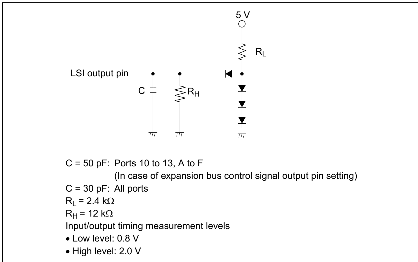
Figure 24-6 Output Load Circuit
