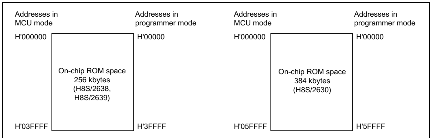
Figure 21B-17 On-Chip ROM Memory Map
