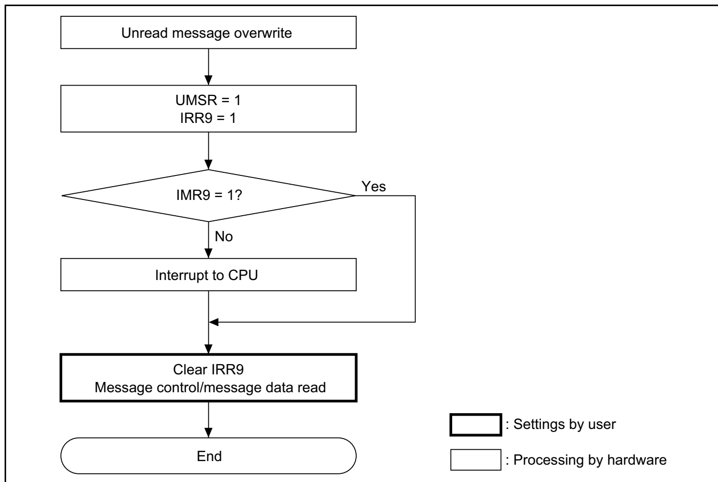
Figure 16-10 Unread Message Overwrite Flowchart
