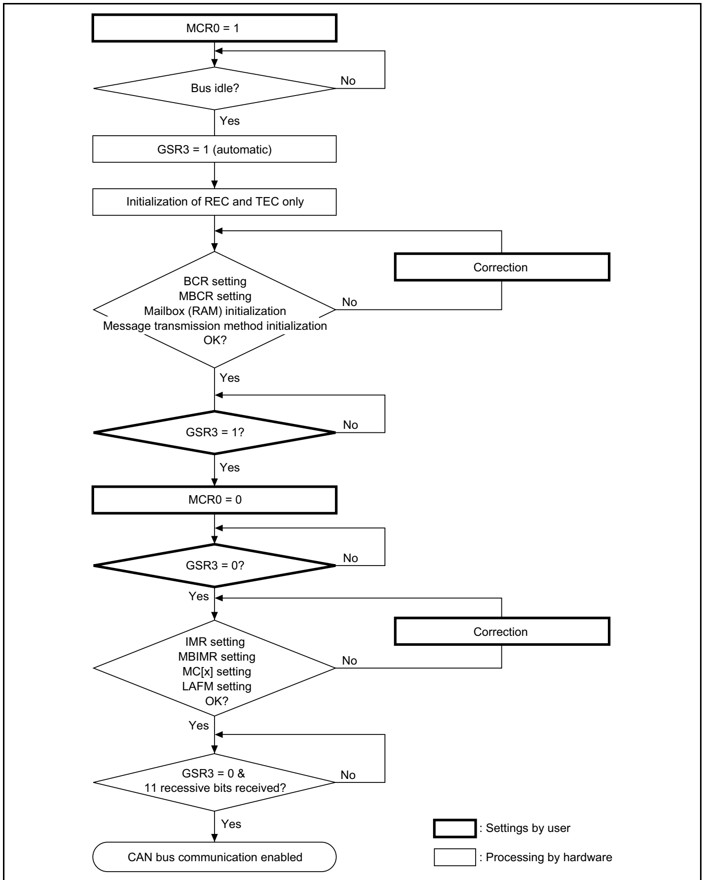
Figure 16-5 Software Reset Flowchart
