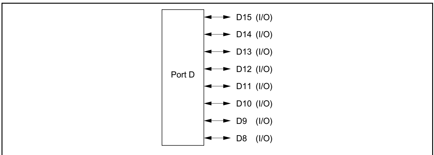
Figure 9-16 Port D Pin Functions (Modes 4 to 6)
