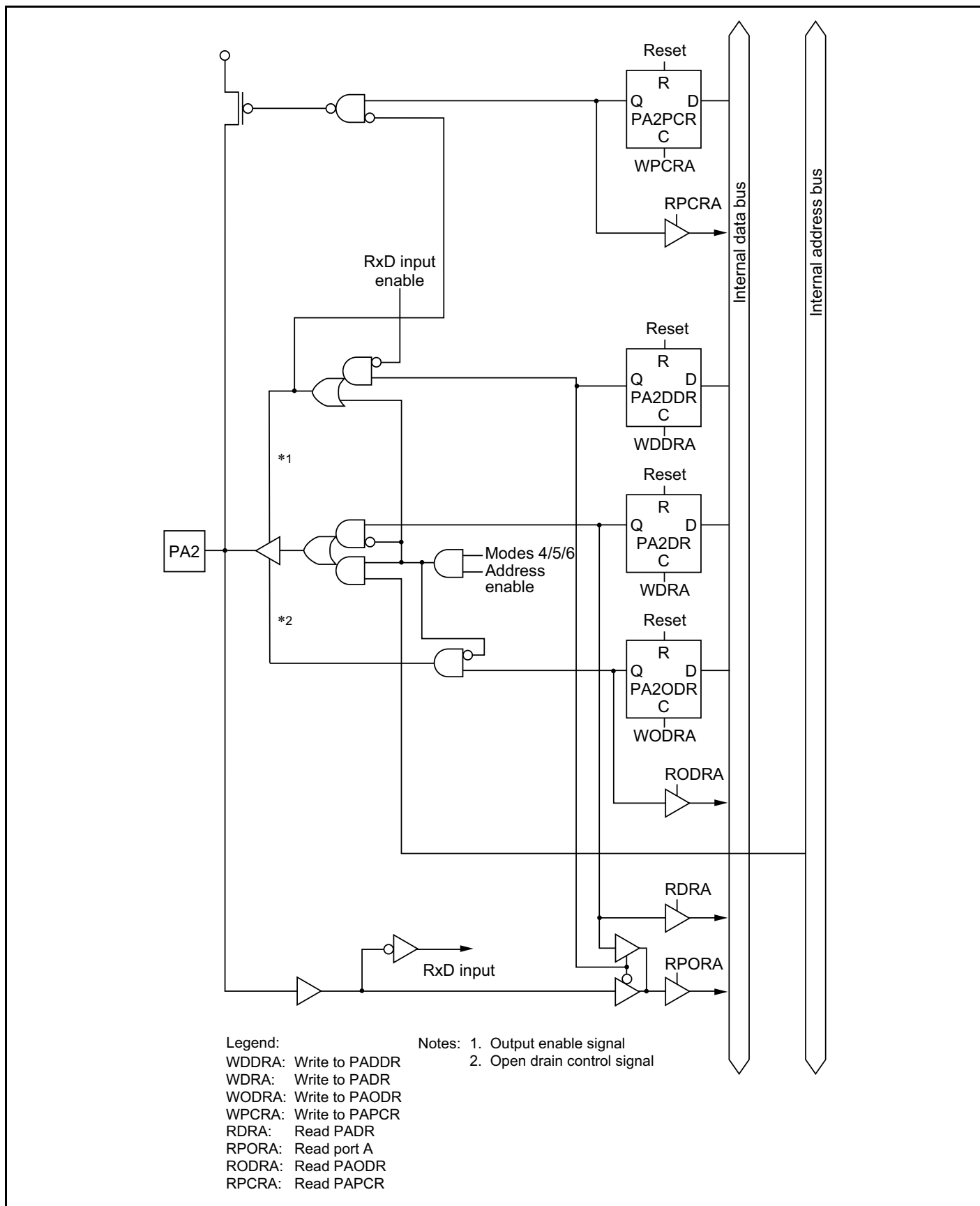
Figure C-5 (c) Port A Block Diagram (Pin PA2)
