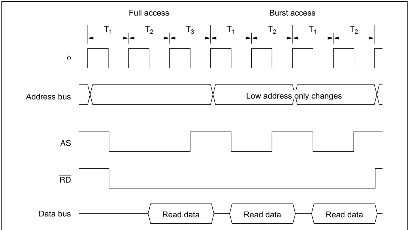
Figure 7-14 (a) Example Burst ROM Access Timing ( AST0 = BRSTS1 = 1 )
