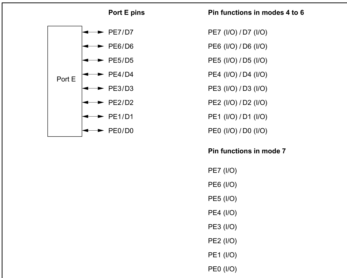
Figure 9-18 Port E Pin Functions
