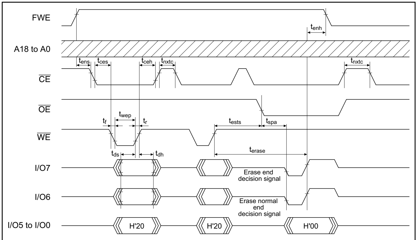
Figure 21B-23 Auto-Erase Mode Timing Waveforms
