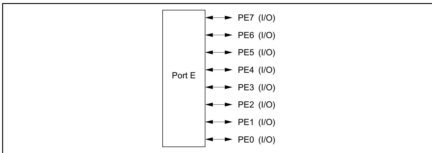
Figure 9-20 Port E Pin Functions (Mode 7)
