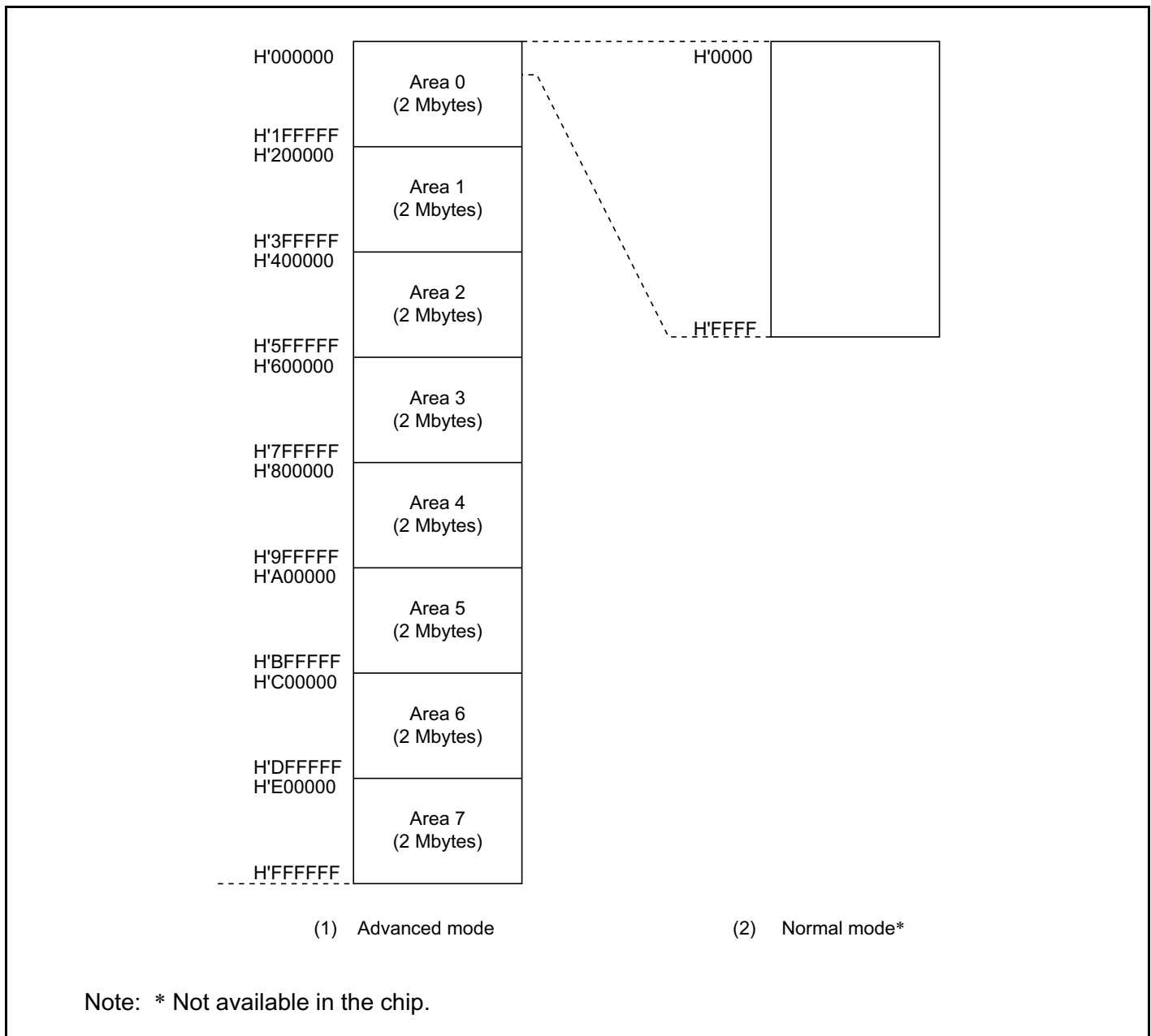
Figure 7-2 Overview of Area Partitioning
