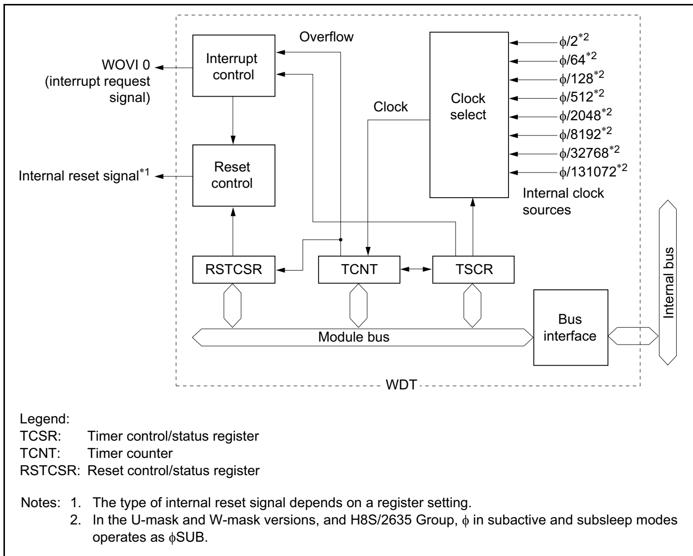
Figure 12-1 (a) Block Diagram of WDT0
