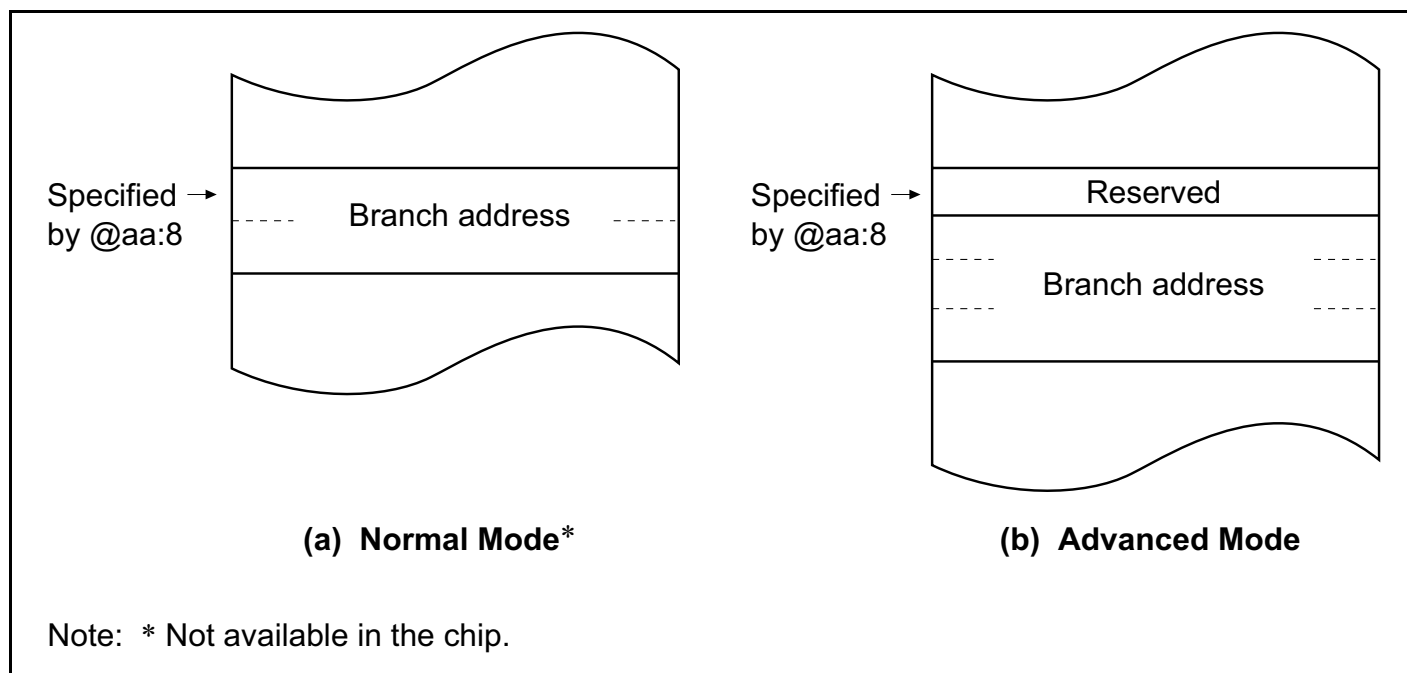
Figure 2-13 Branch Address Specification in Memory Indirect Mode
