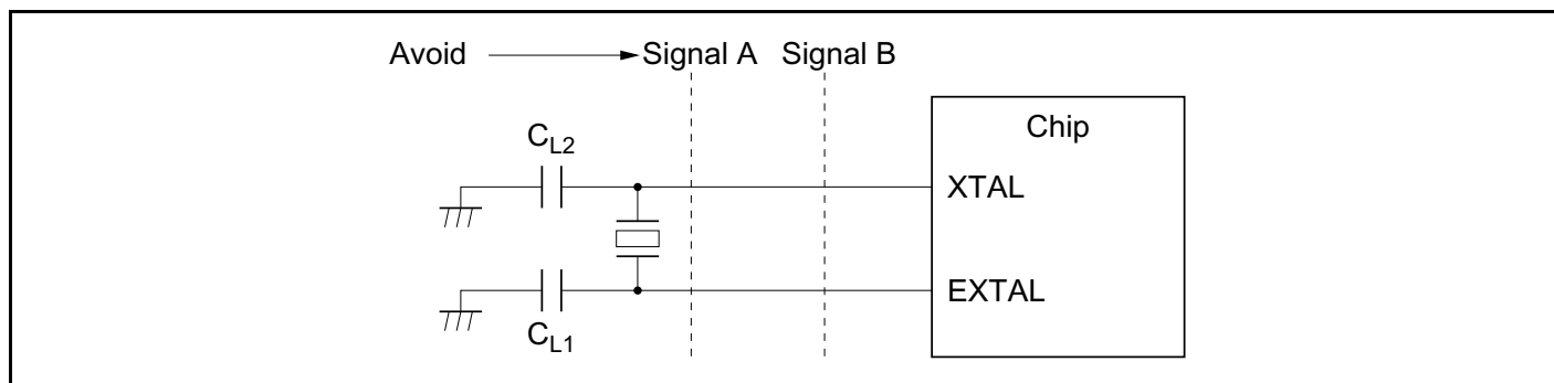
Figure 22A-4 Example of Incorrect Board Design
