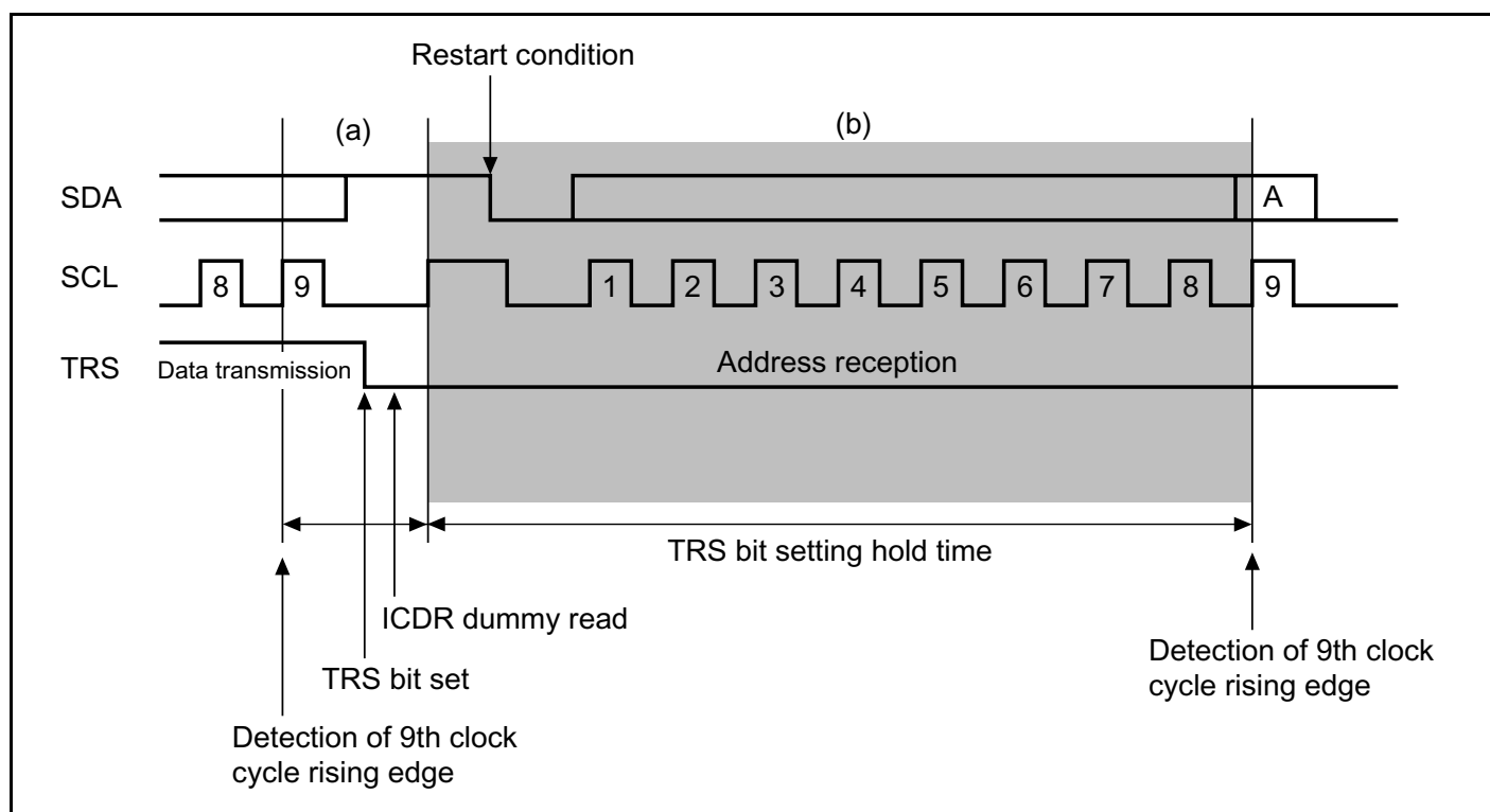
Figure 15-26 TRS Bit Setting Timing in Slave Mode
