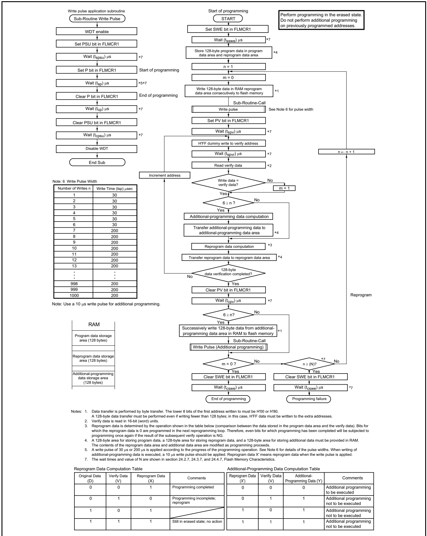
Figure 21C-12 Program/Program-Verify Flowchart
