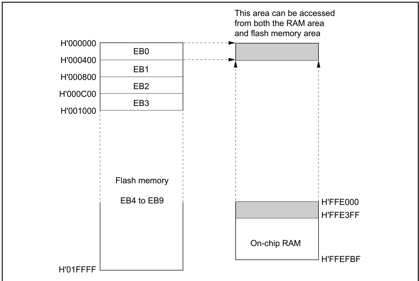
Figure 21A-16 Example of RAM Overlap Operation
