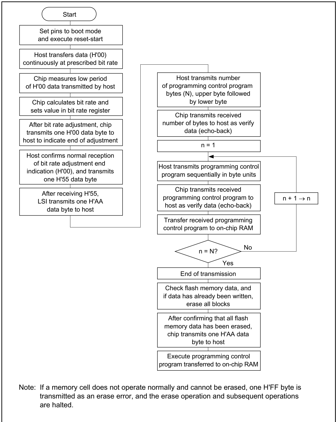
Figure 21B-8 Boot Mode Execution Procedure
