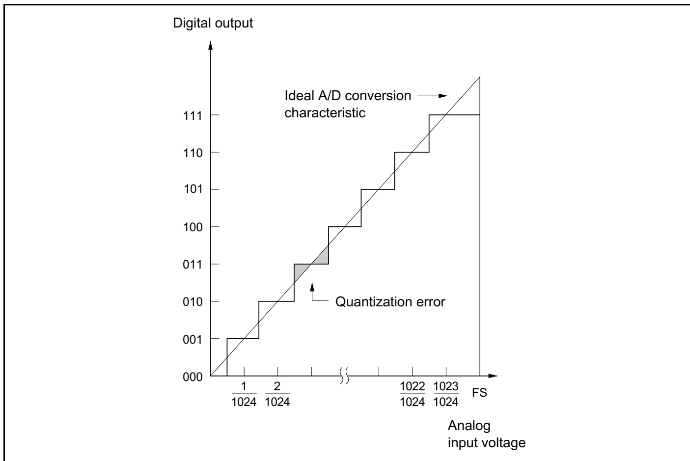
Figure 17-9 A/D Conversion Precision Definitions (1)
