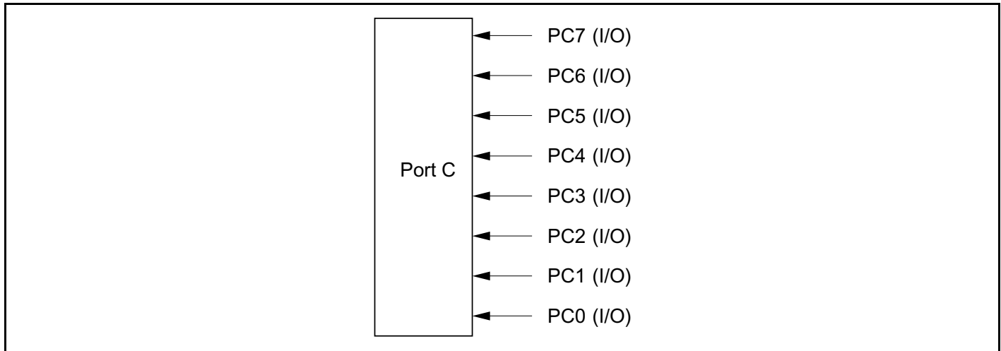
Figure 9-14 Port C Pin Functions (Mode 7)
