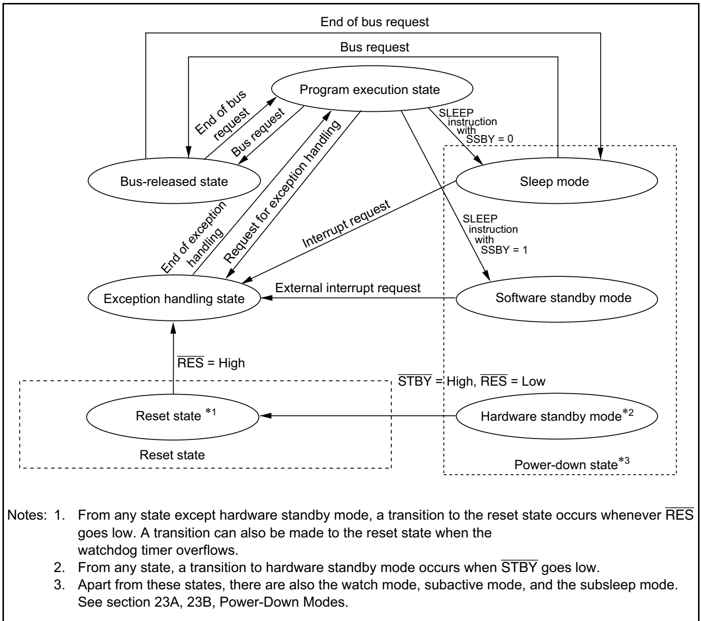
Figure 2-15 State Transitions
