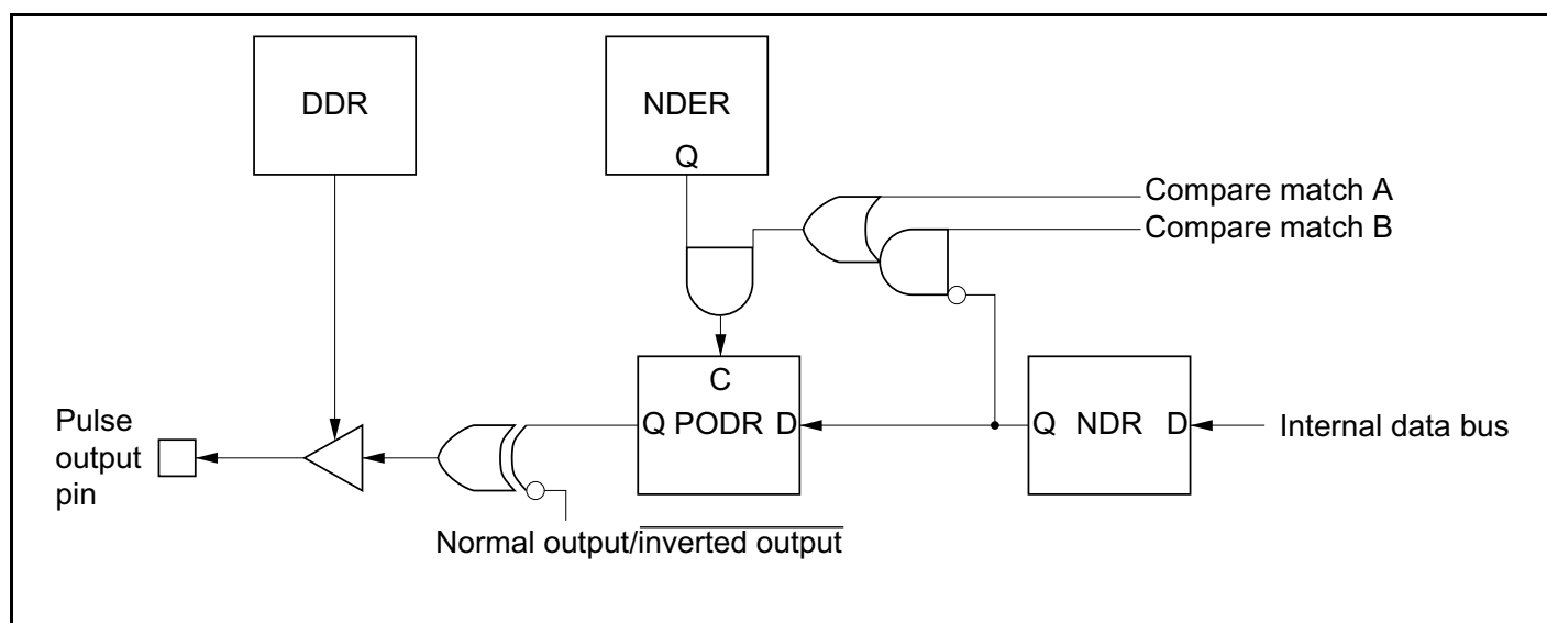
Figure 11-10 Non-Overlapping Pulse Output
