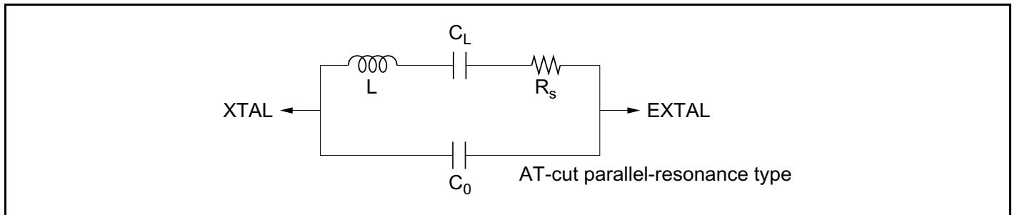
Figure 22B-3 Crystal Resonator Equivalent Circuit
