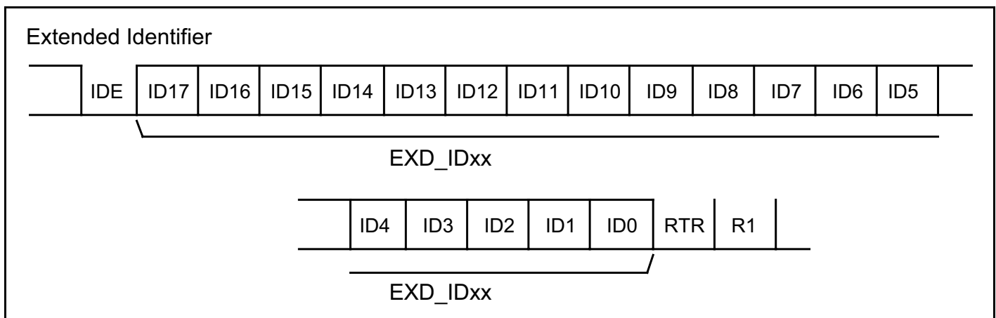
Figure 16-3 Extended identifier
