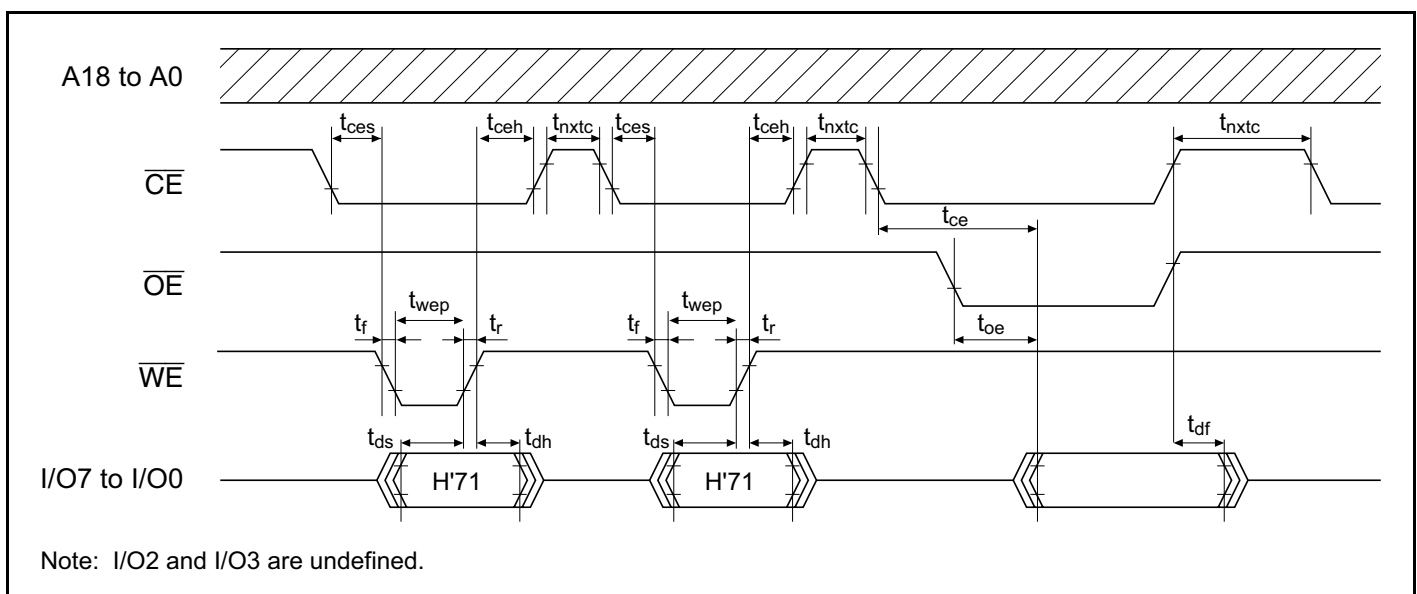
Figure 21A-24 Status Read Mode Timing Waveforms
