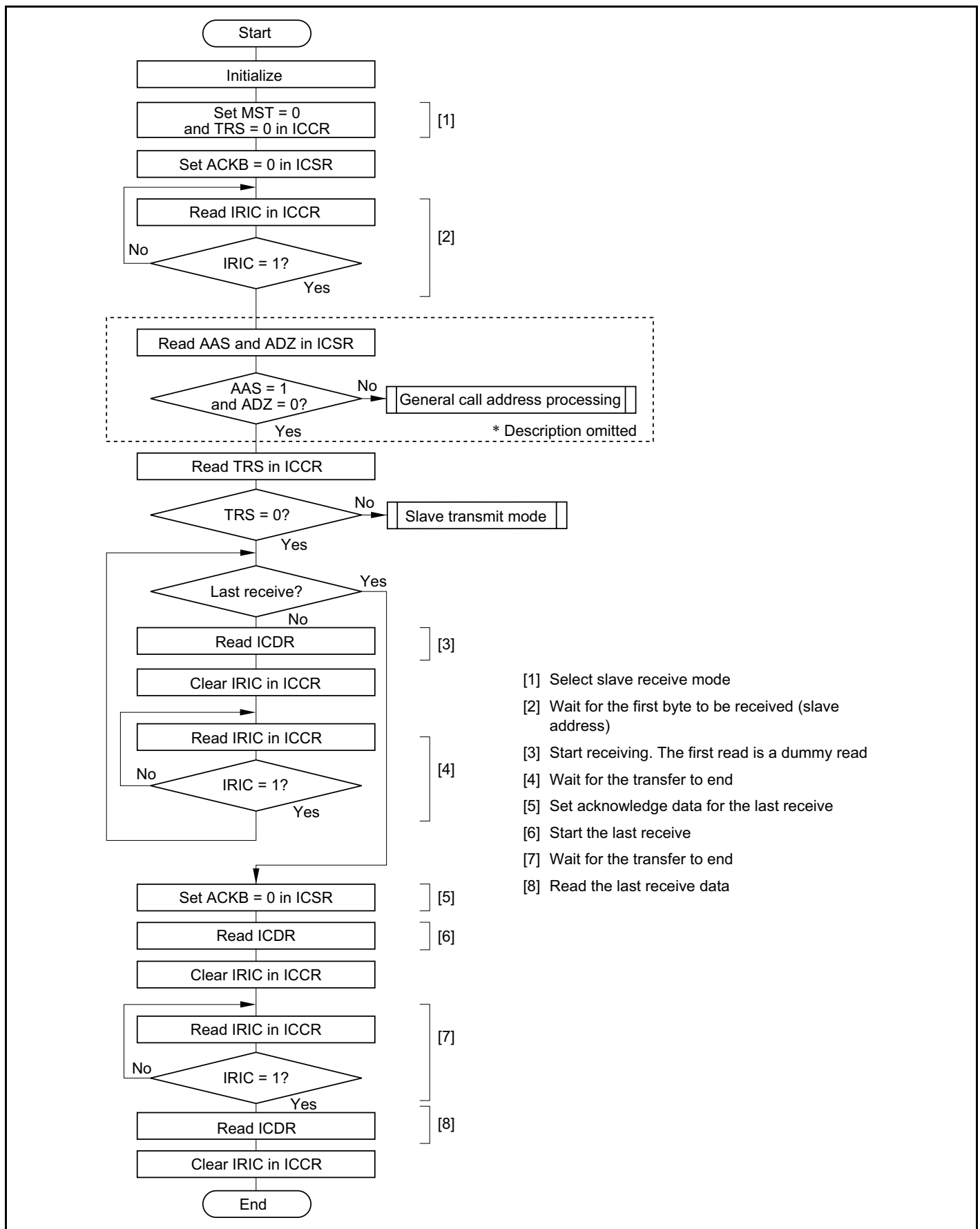
Figure 15-14 Flowchart for Slave Transmit Mode (Example)
