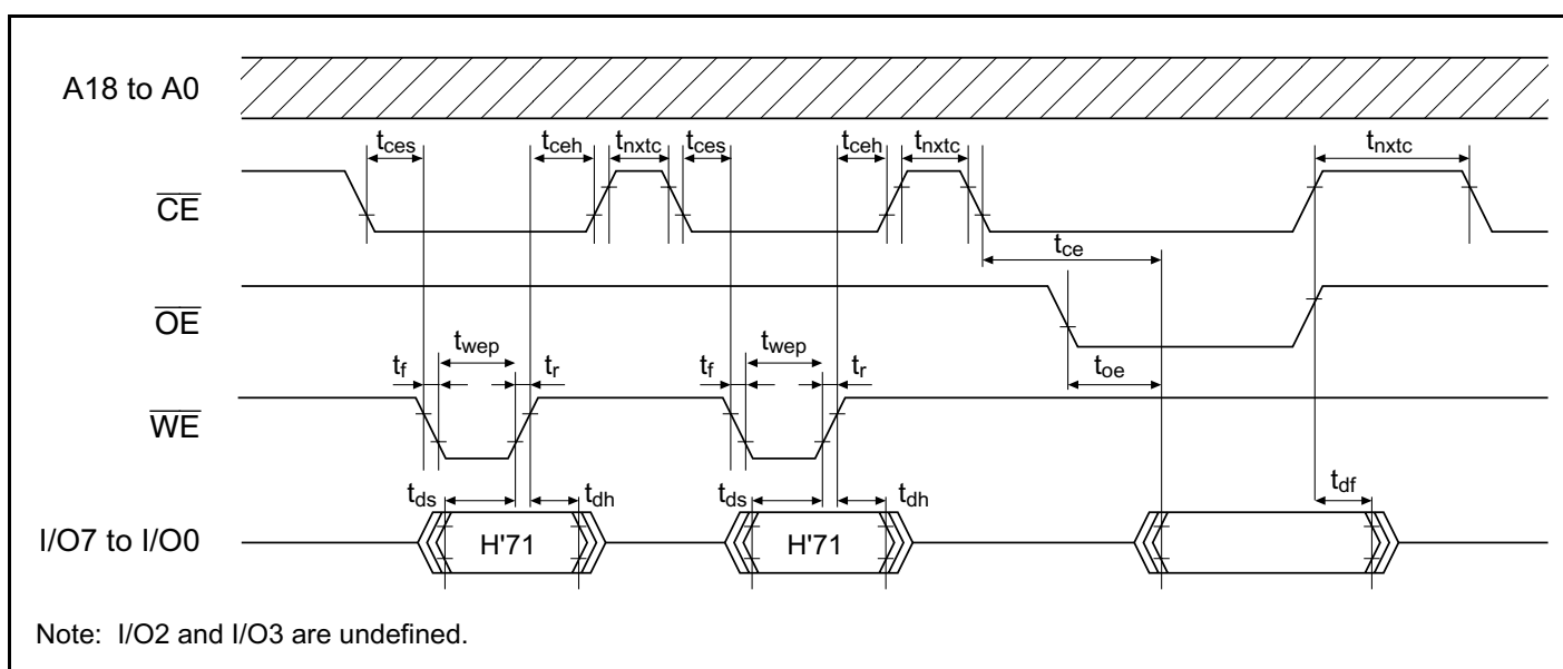
Figure 21B-24 Status Read Mode Timing Waveforms
