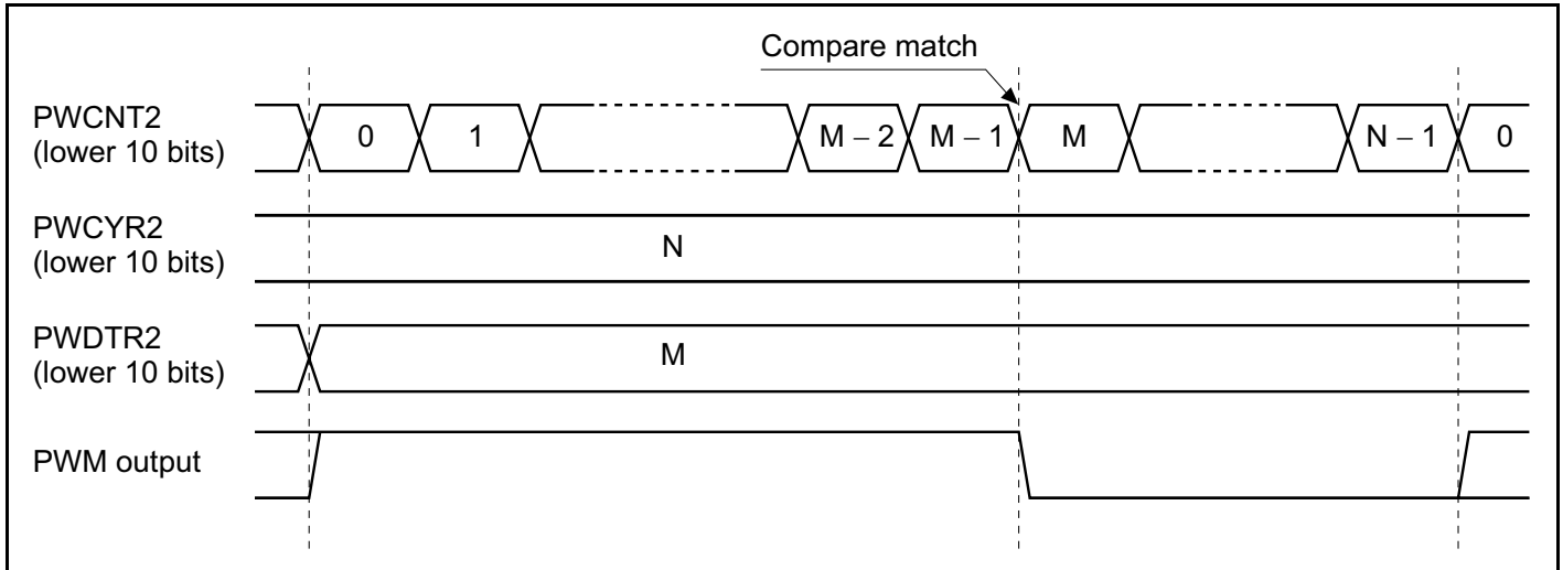
Figure 19-6 Duty Register Compare Match (OPS = 0 in PWPR2)
