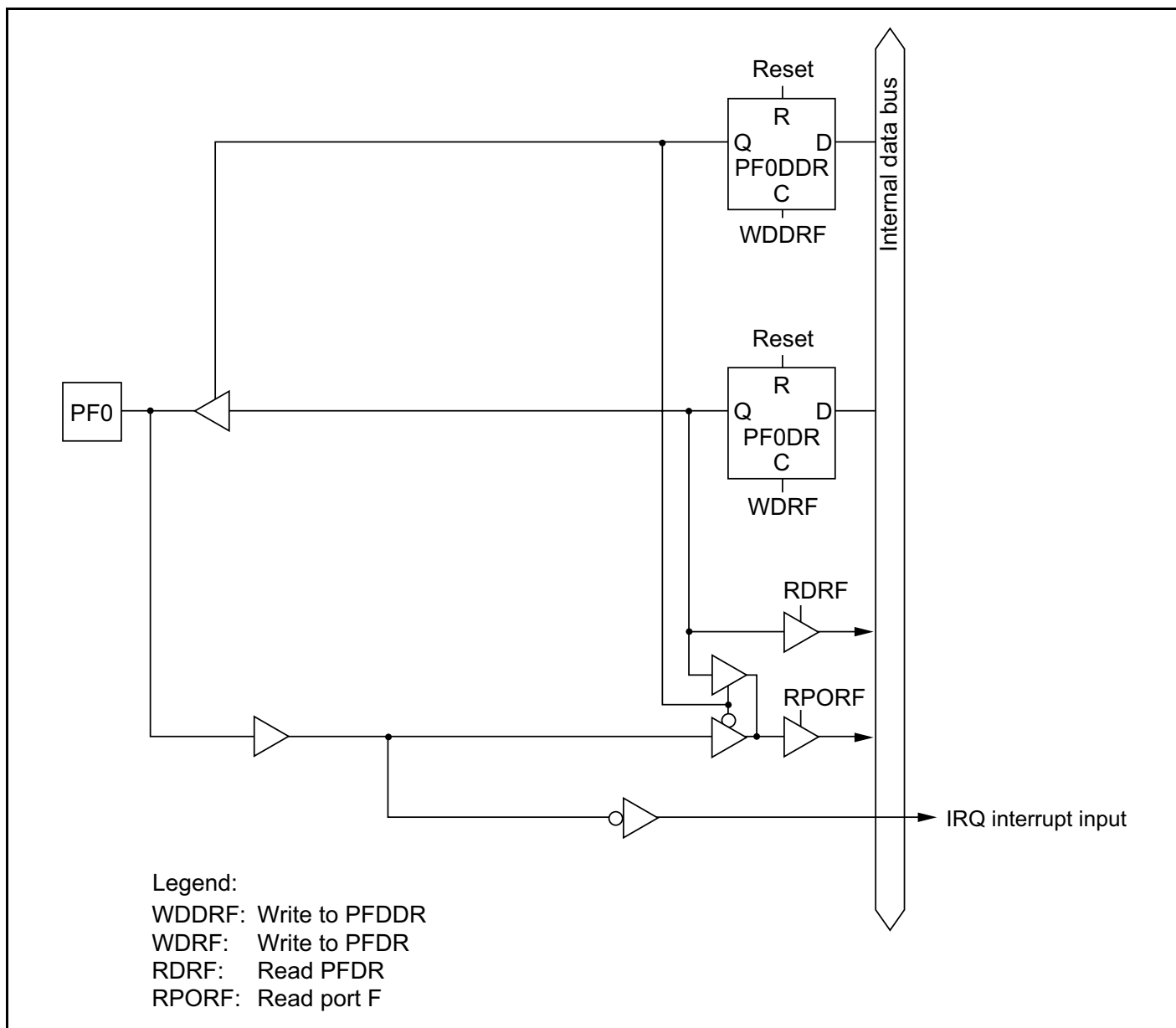
Figure C-10 (a) Port F Block Diagram (Pin PF0)
