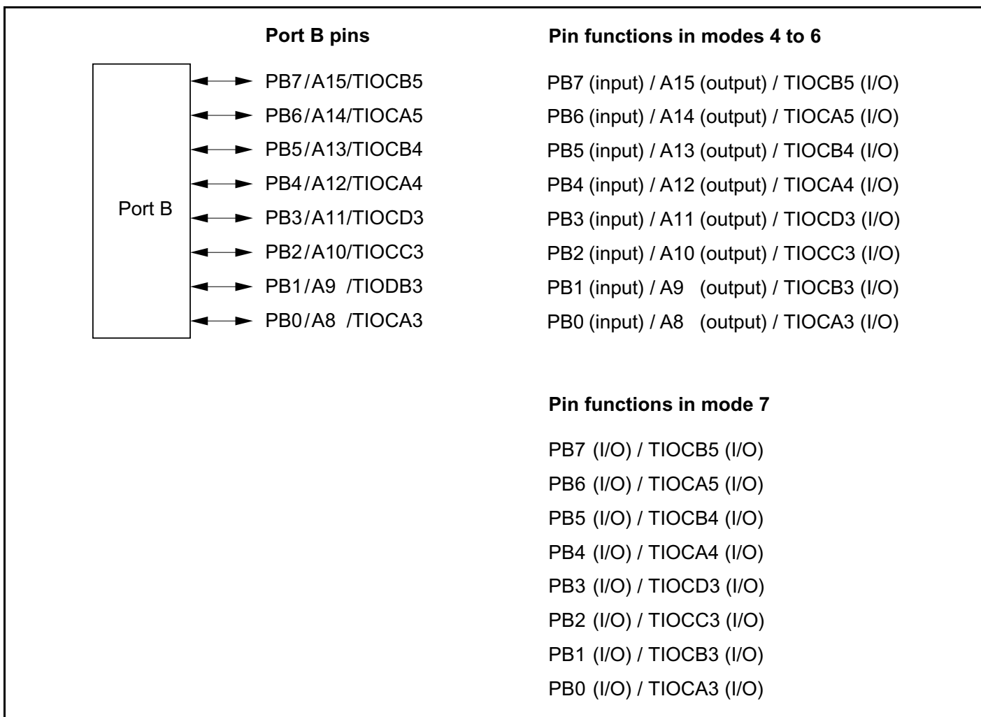
Figure 9-8 Port B Pin Functions
