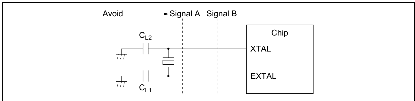
Figure 22B-4 Example of Incorrect Board Design
