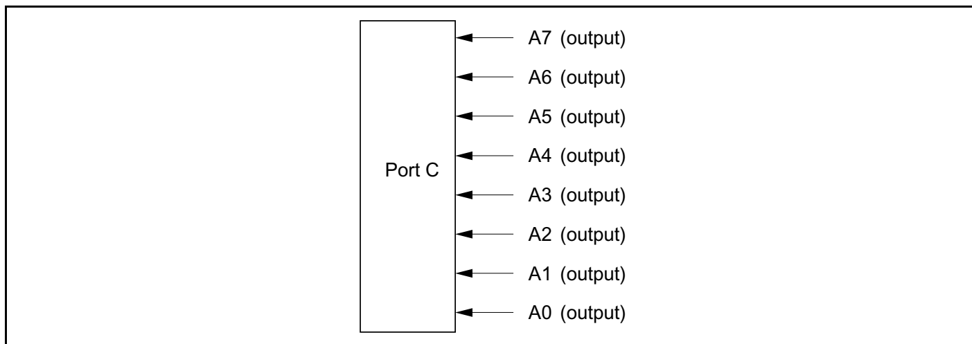
Figure 9-12 Port C Pin Functions (Modes 4 and 5)
