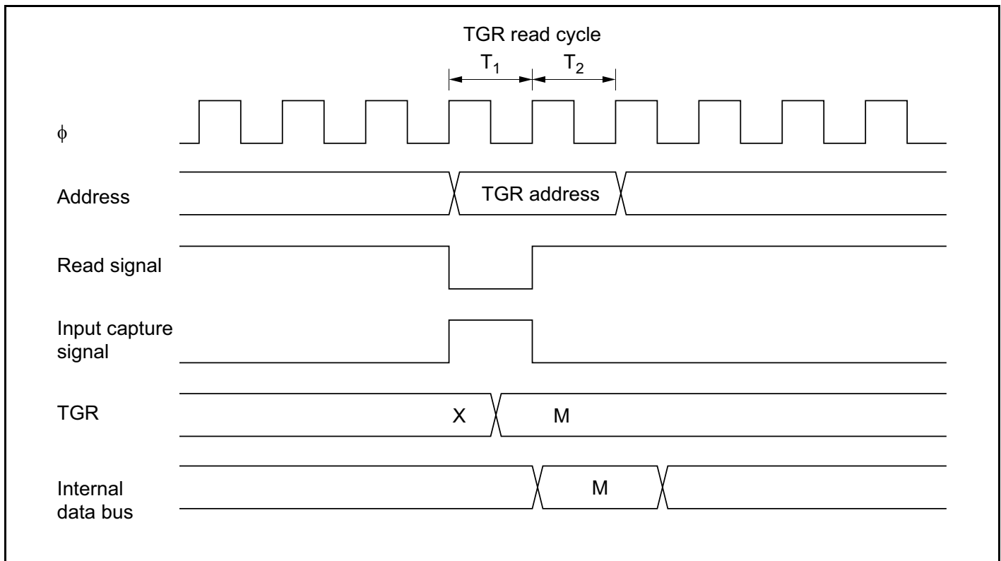
Figure 10-53 Contention between TGR Read and Input Capture
