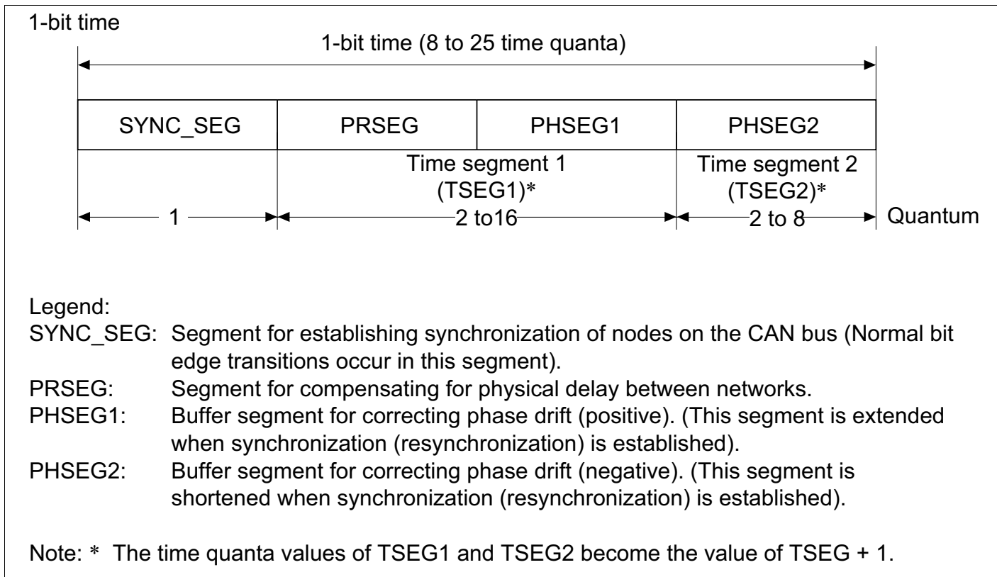
Figure 16-6 Detailed Description of One Bit
