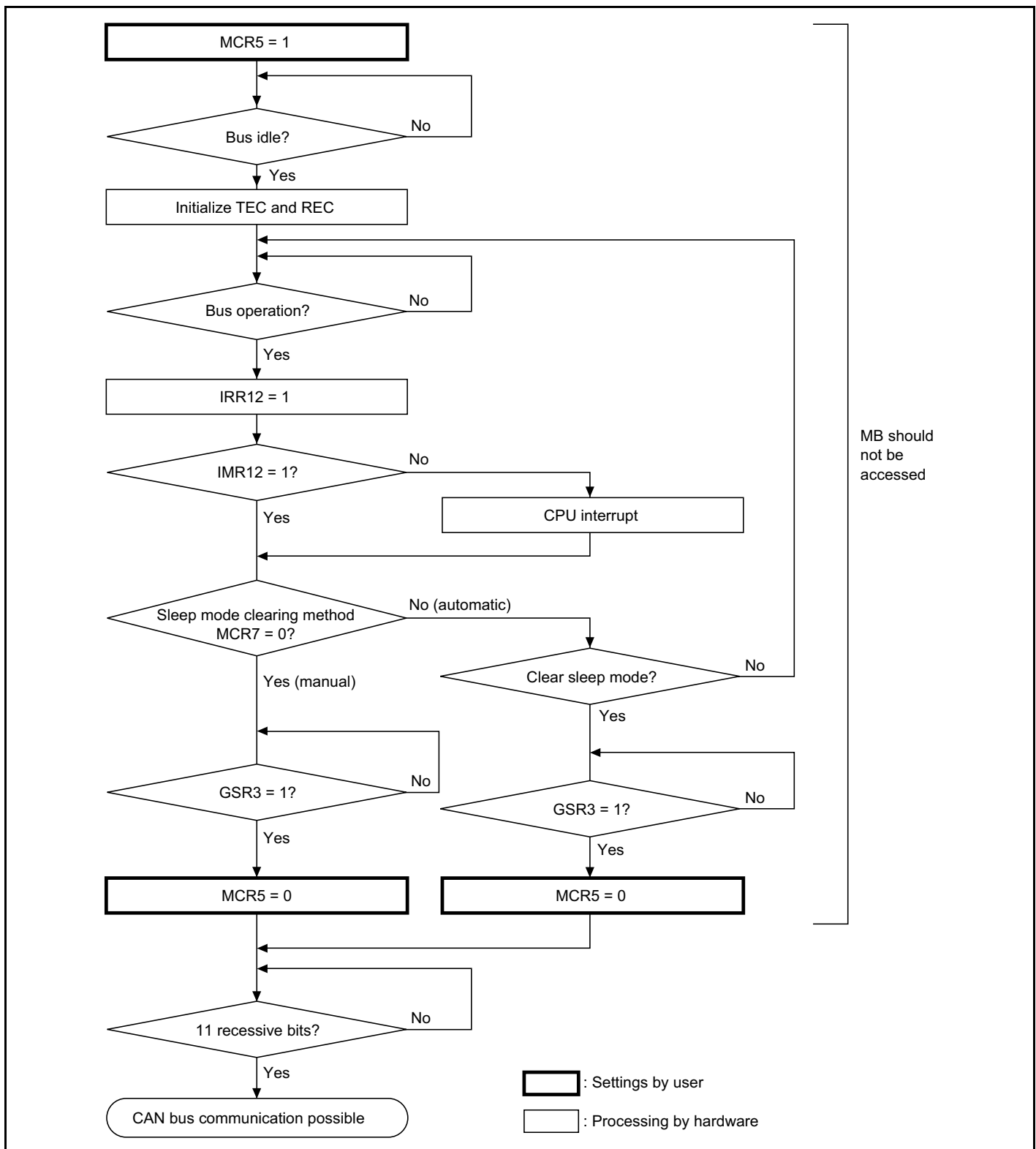
Figure 16-11 HCAN Sleep Mode Flowchart
