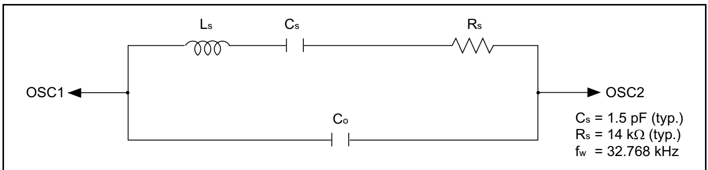
Figure 22A-9 Equivalence Circuit for 32.768kHz Oscillator
