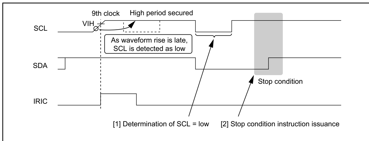
Figure 15-23 Timing of Stop Condition Issuance
