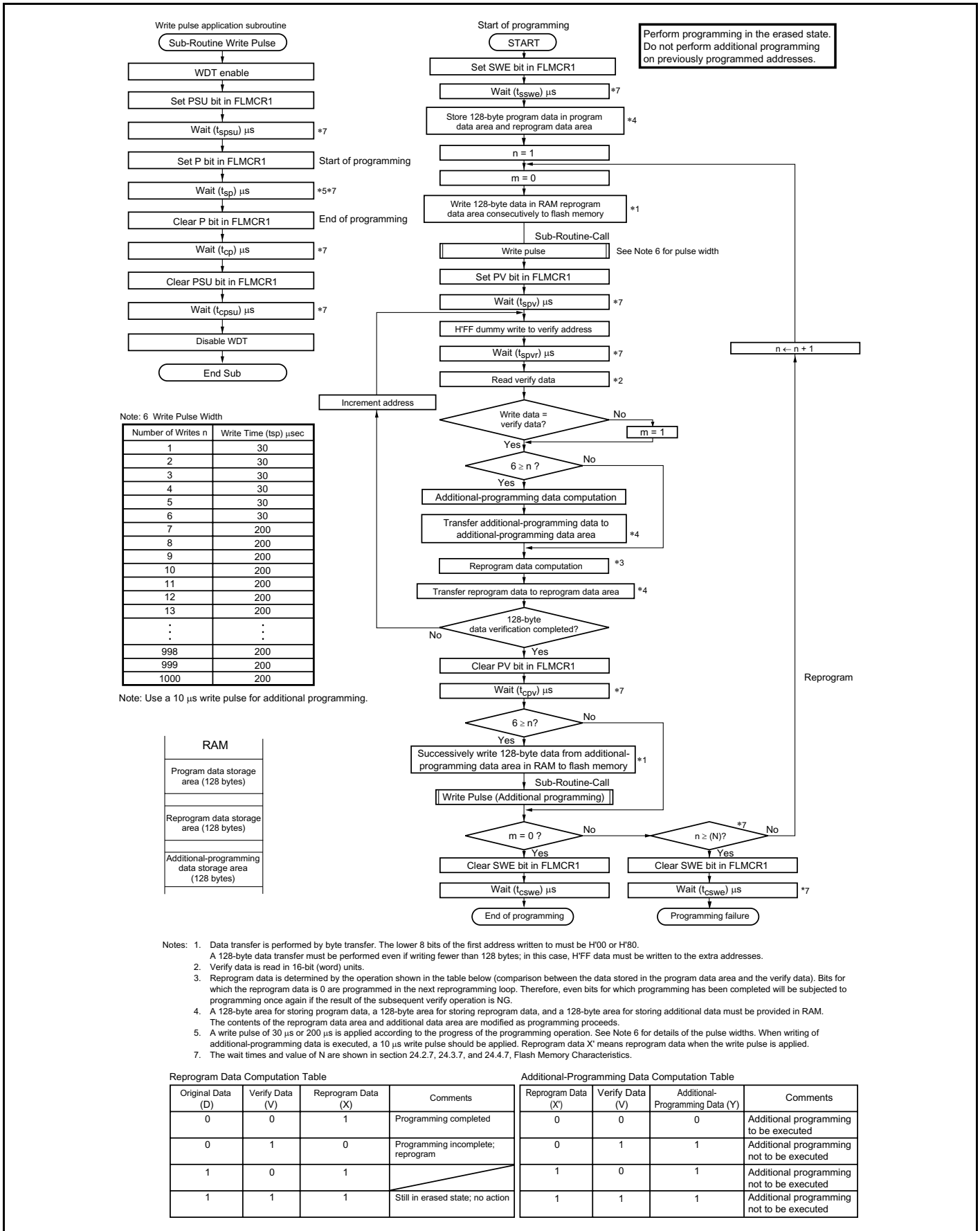
Figure 21B-12 Program/Program-Verify Flowchart
