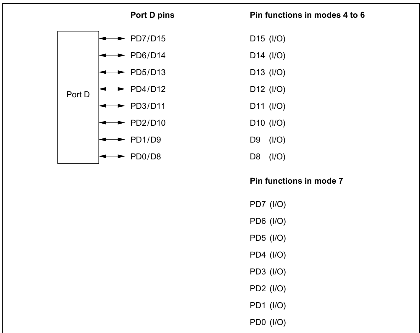
Figure 9-15 Port D Pin Functions
