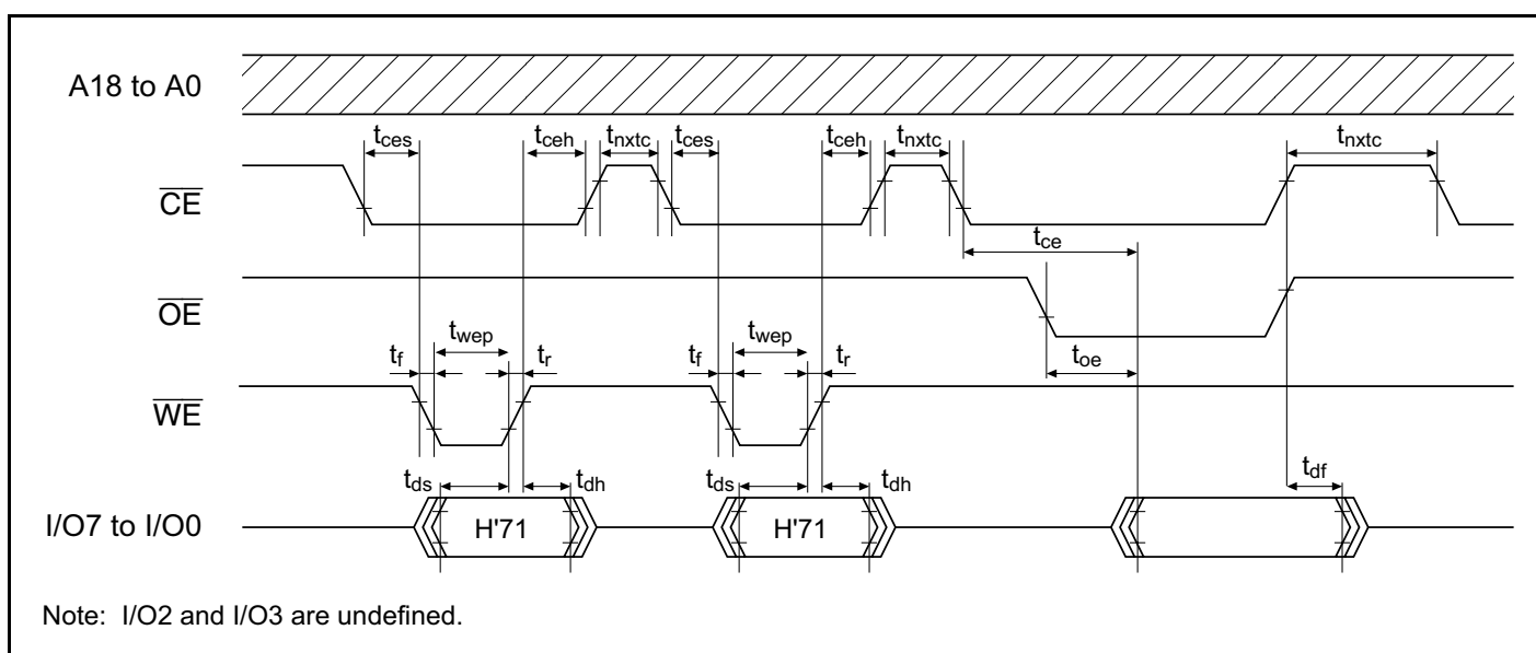
Figure 21C-24 Status Read Mode Timing Waveforms
