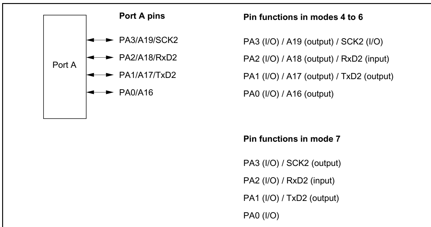
Figure 9-5 Port A Pin Functions
