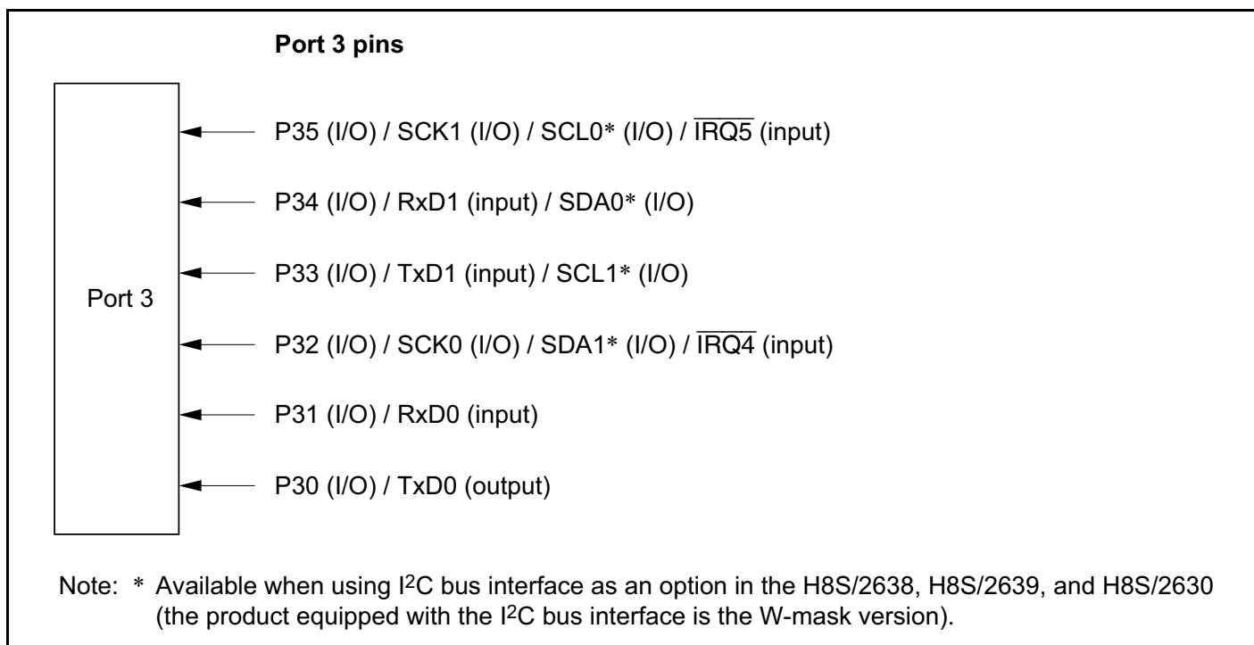
Figure 9-2 Port 3 Pin Functions
