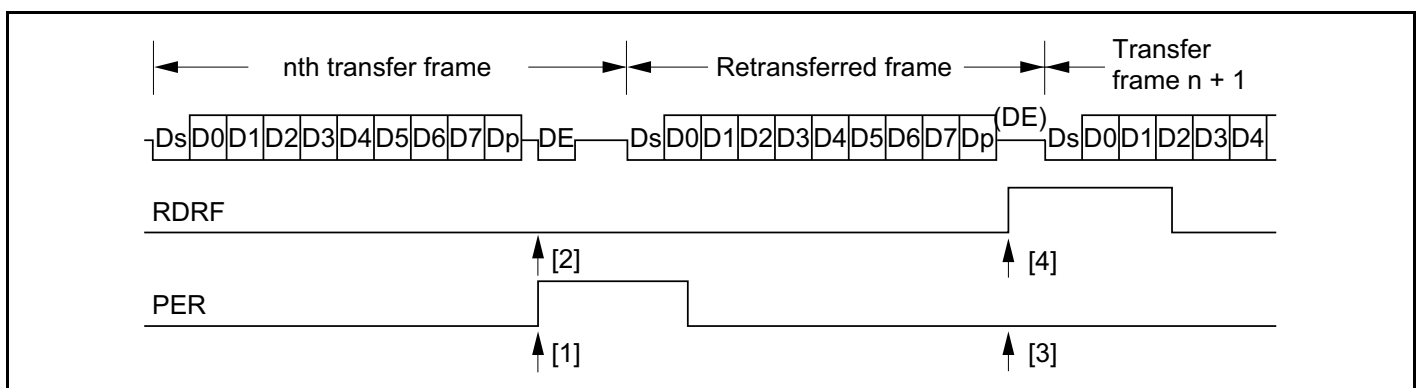
Figure 14-11 Retransfer Operation in SCI Receive Mode
