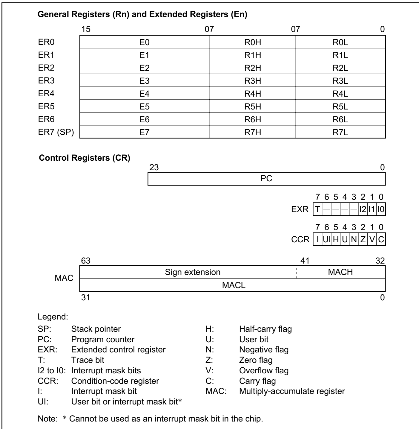
Figure 2-7 CPU Registers
