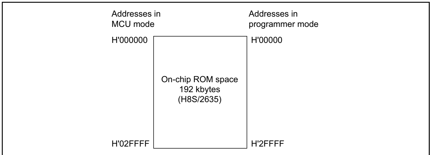
Figure 21C-17 On-Chip ROM Memory Map
