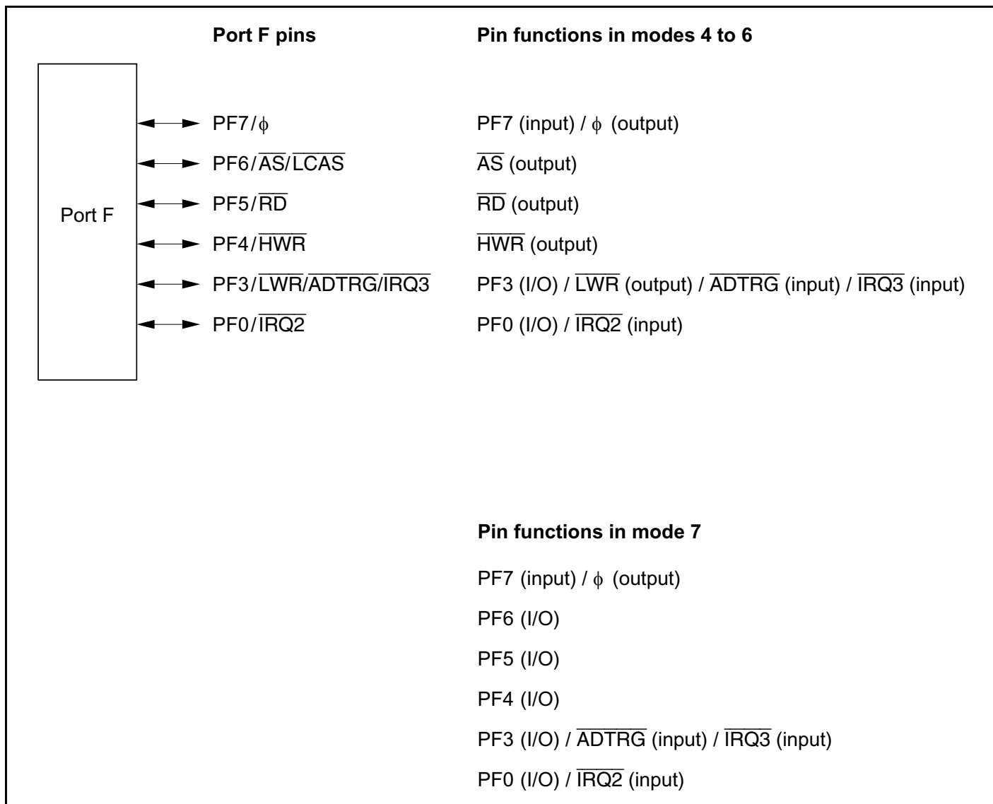
Figure 9-21 Port F Pin Functions
