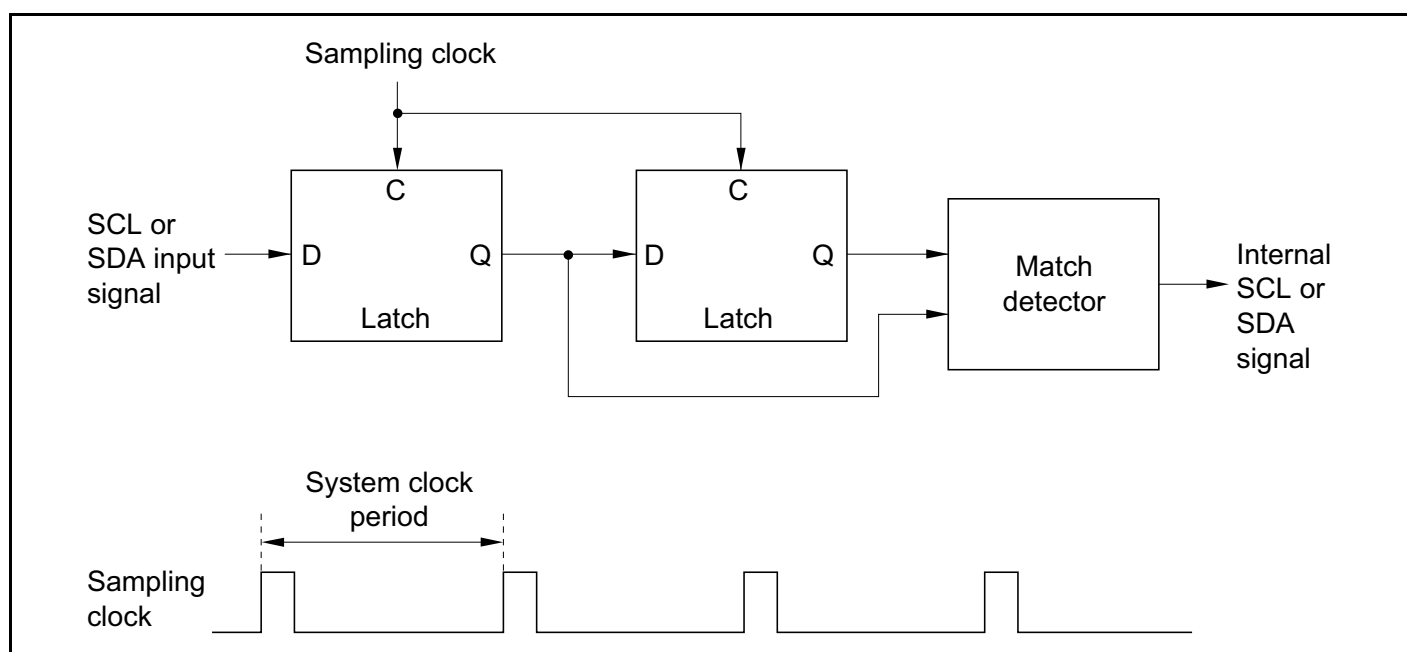
Figure 15-20 Block Diagram of Noise Canceler
