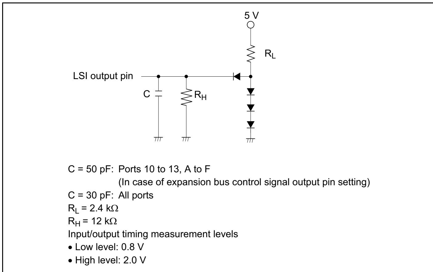
Figure 24-4 Output Load Circuit
