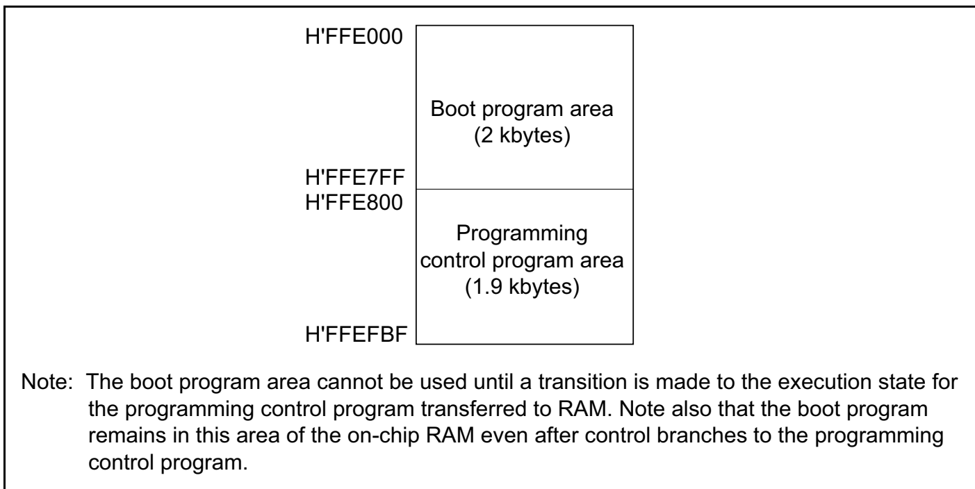
Figure 21A-9 RAM Areas in Boot Mode
