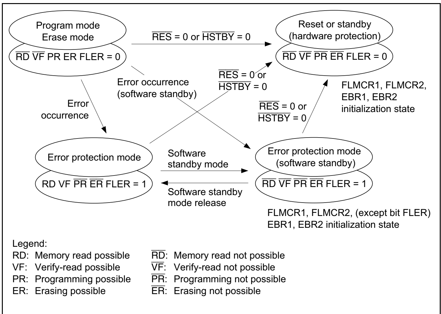
Figure 21A-14 Flash Memory State Transitions
