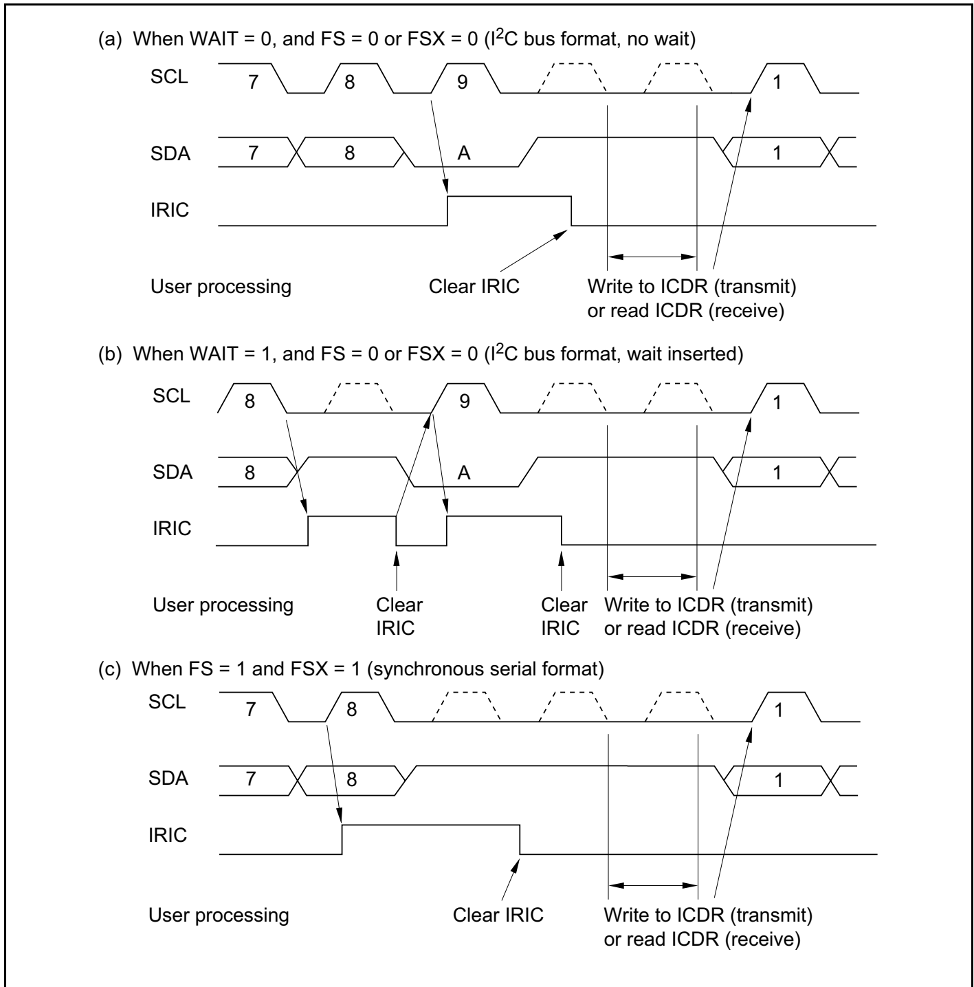
Figure 15-19 IRIC Setting Timing and SCL Control
