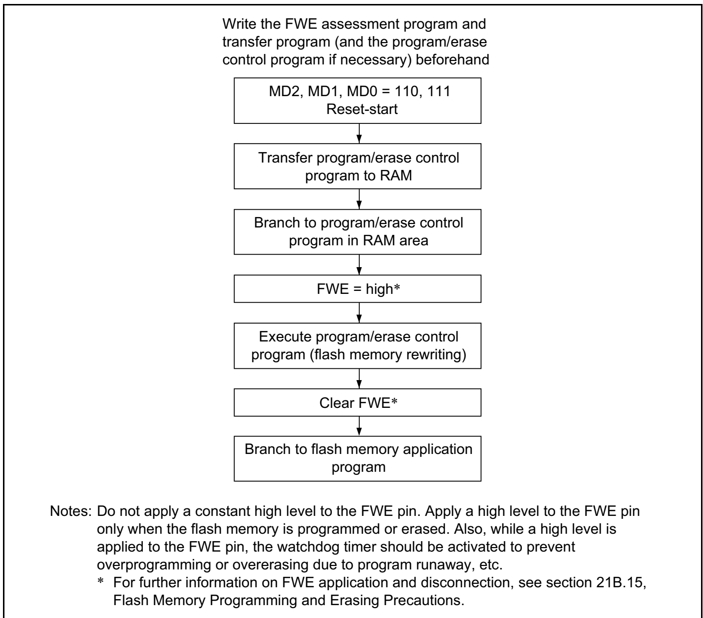
Figure 21C-10 User Program Mode Execution Procedure
