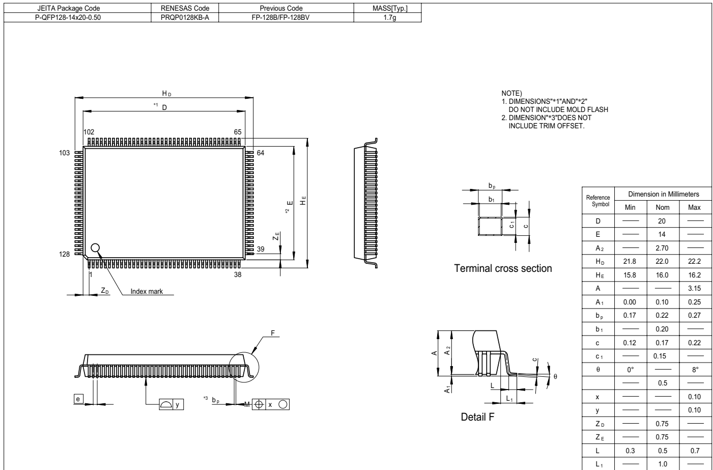
Figure G-1 FP-128B Package Dimensions
