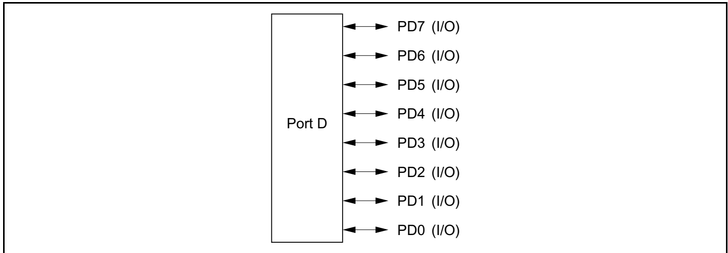
Figure 9-17 Port D Pin Functions (Mode 7)
