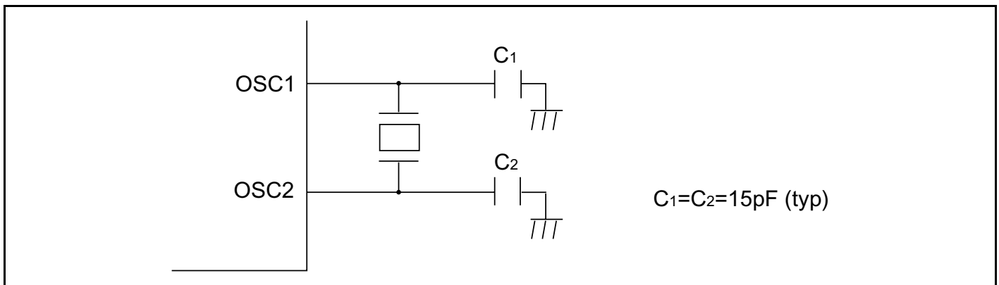
Figure 22A-8 Example Connection of 32.768kHz Quartz Oscillator
