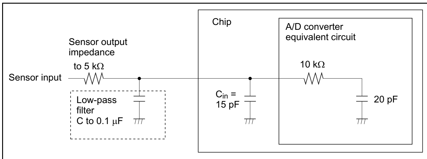
Figure 17-11 Example of Analog Input Circuit
