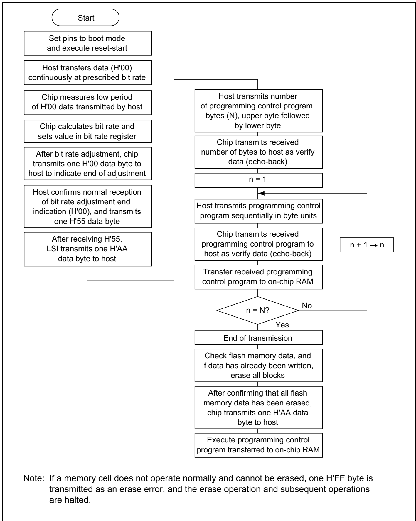
Figure 21C-8 Boot Mode Execution Procedure
