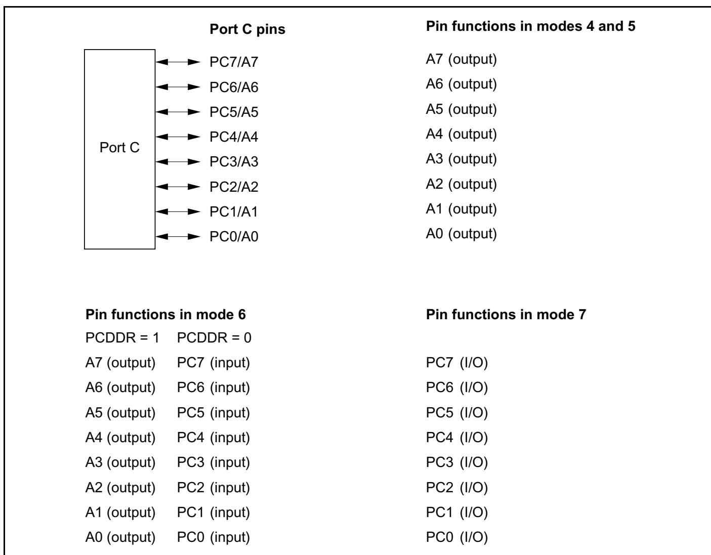
Figure 9-11 Port C Pin Functions
