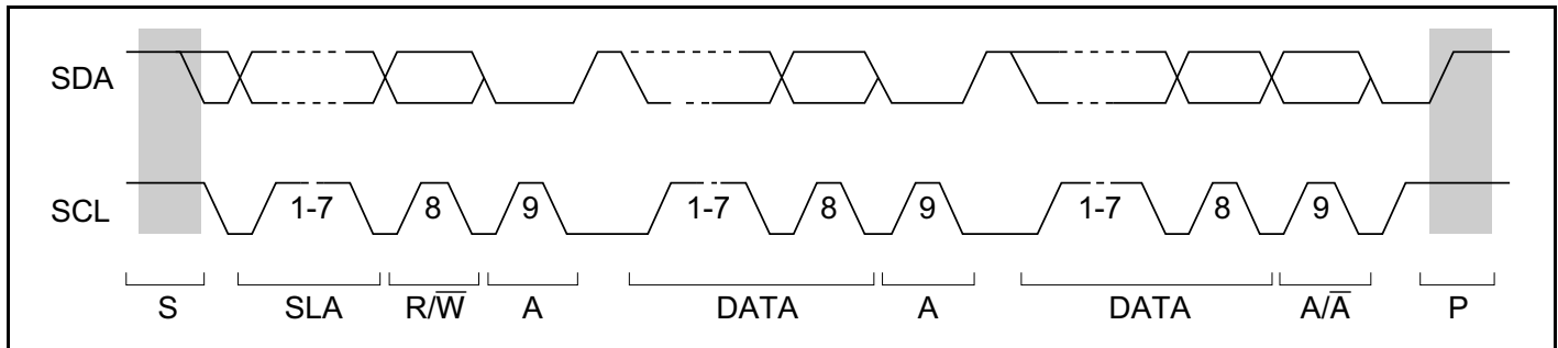
Figure 15-5 I 2 C Bus Timing
