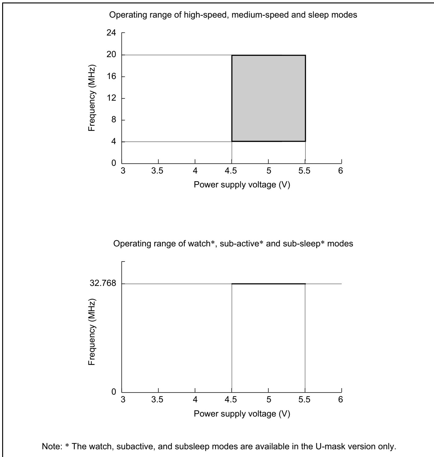
Figure 24-1 Power Supply Voltage and Operating Ranges
