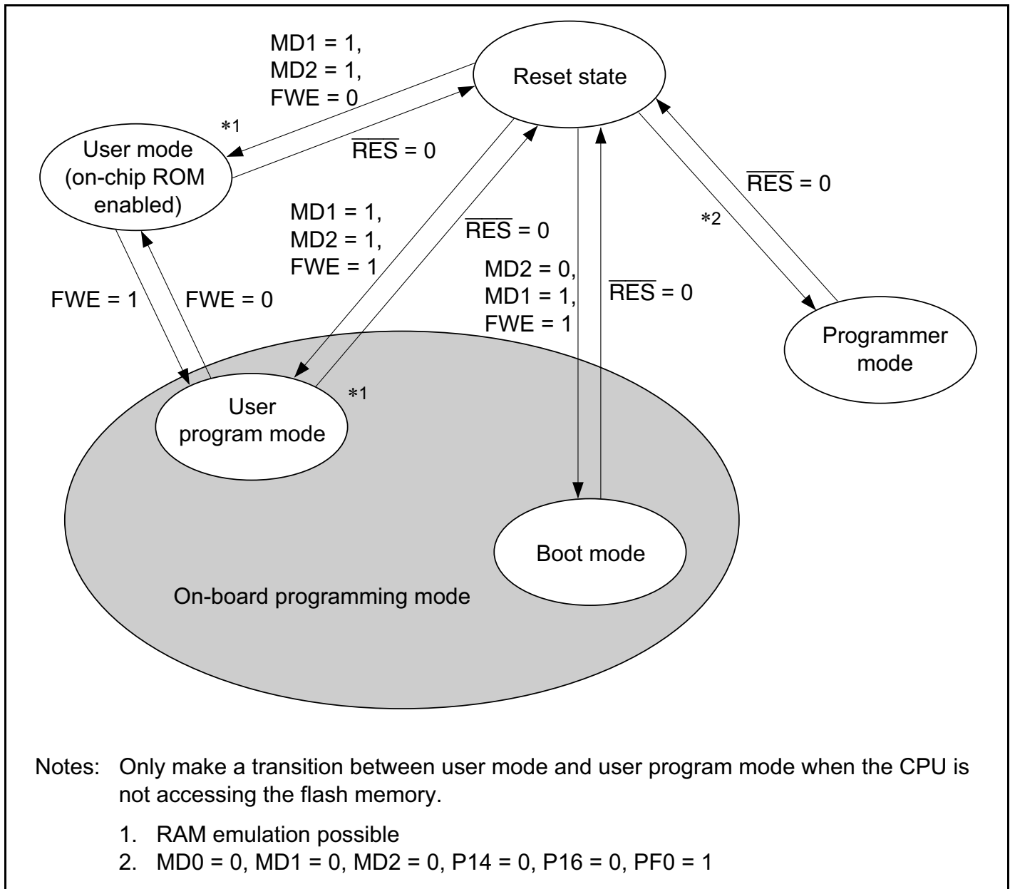
Figure 21C-3 Flash Memory State Transitions
