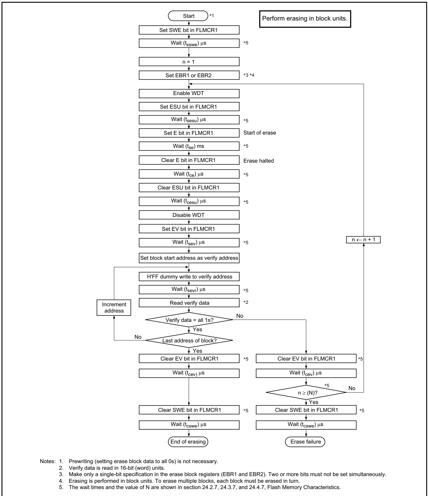
Figure 21C-13 Erase/Eraser-Verify Flowchart
