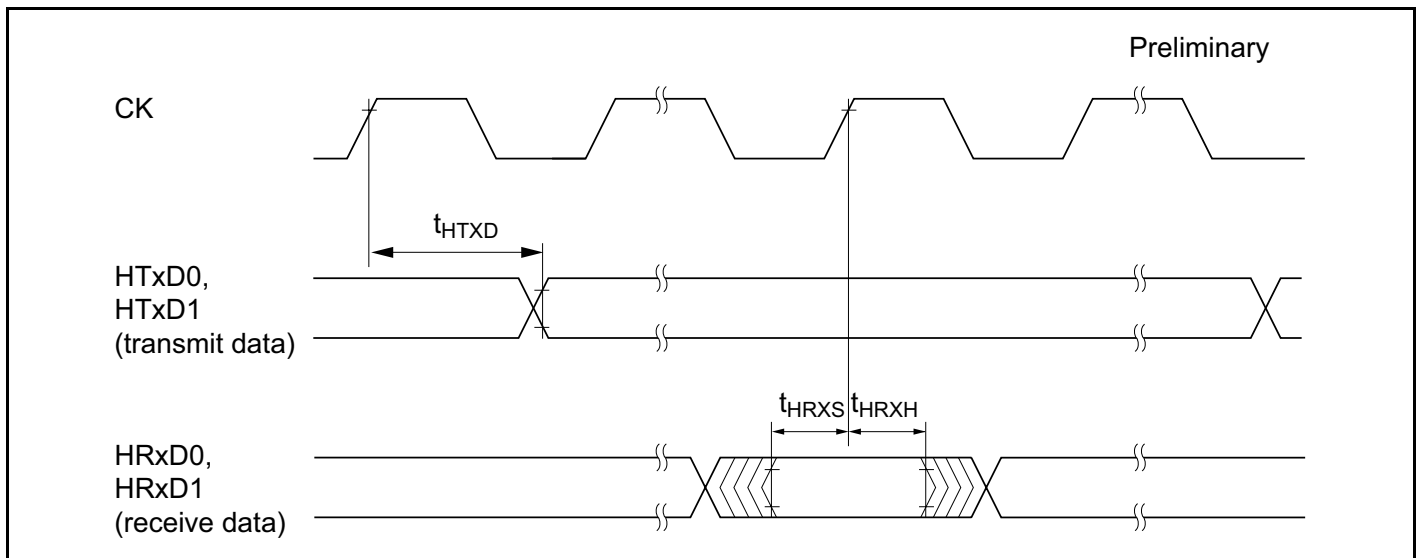
Figure 24-27 HCAN Input/Output Timing
