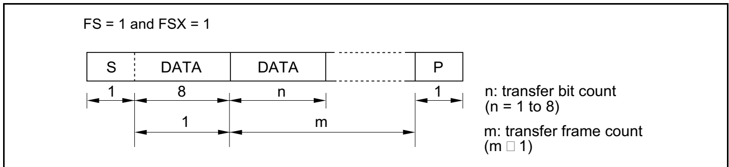
Figure 15-4 I 2 C Bus Data Format (Serial Format)
