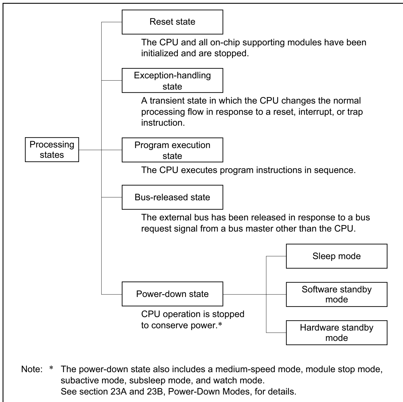
Figure 2-14 Processing States
