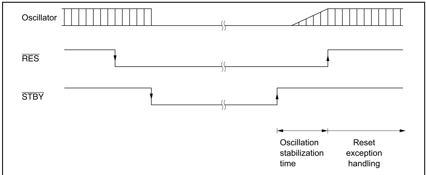
Figure 23A-4 Hardware Standby Mode Timing
