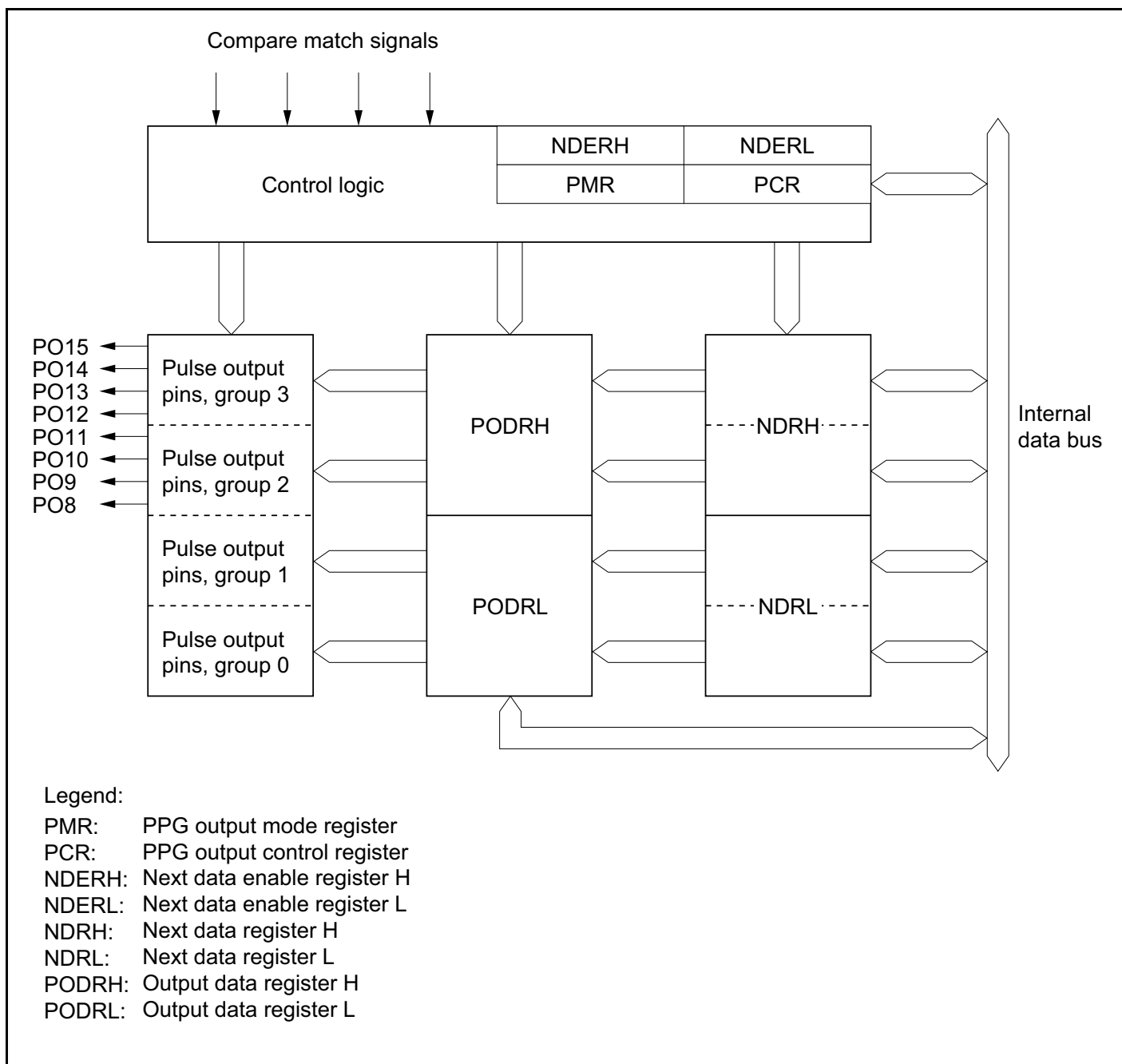
Figure 11-1 Block Diagram of PPG
