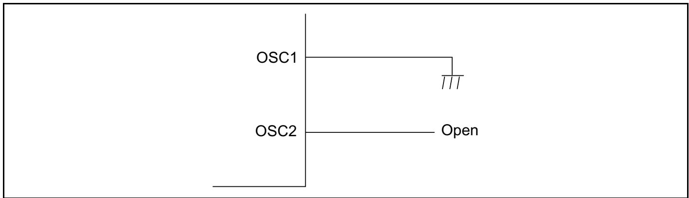
Figure 22A-10 Pin Handling when Subclock not Required
