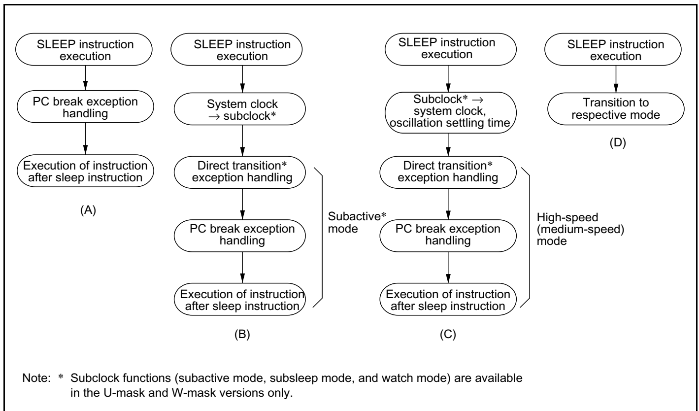
Figure 6-2 Operation in Power-Down Mode Transitions
