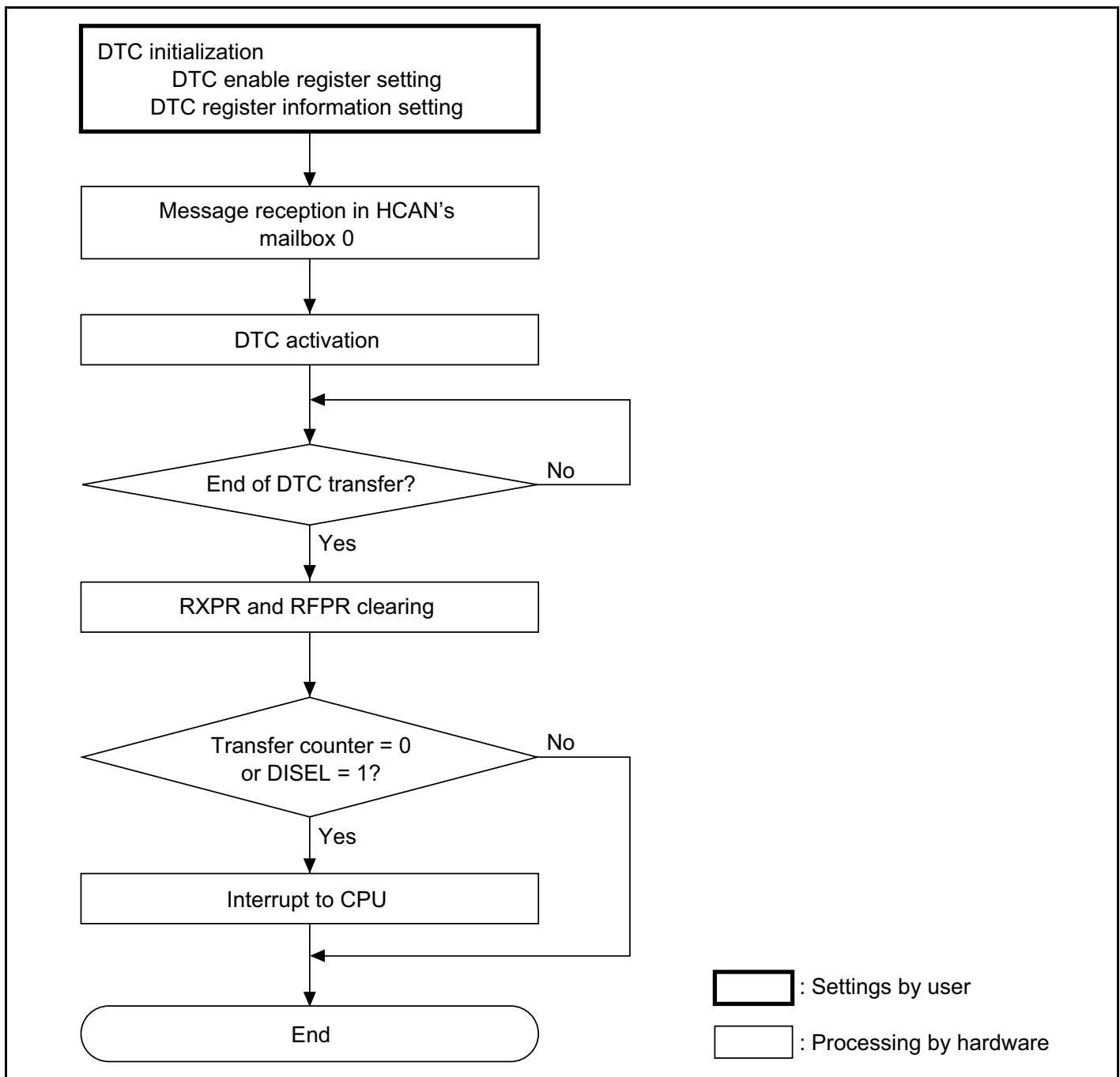
Figure 16-13 DTC Transfer Flowchart
