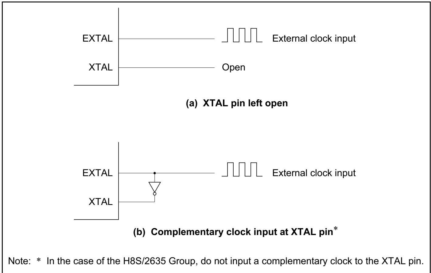
Figure 22B-6 External Clock Input (Examples)
