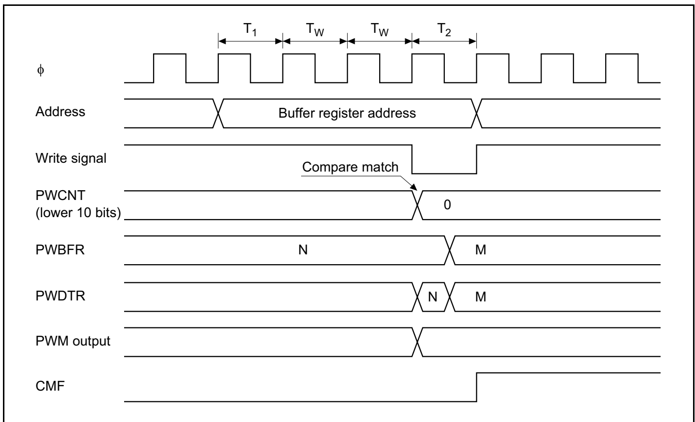
Figure 19-12 PWM Channel 1 Operation
