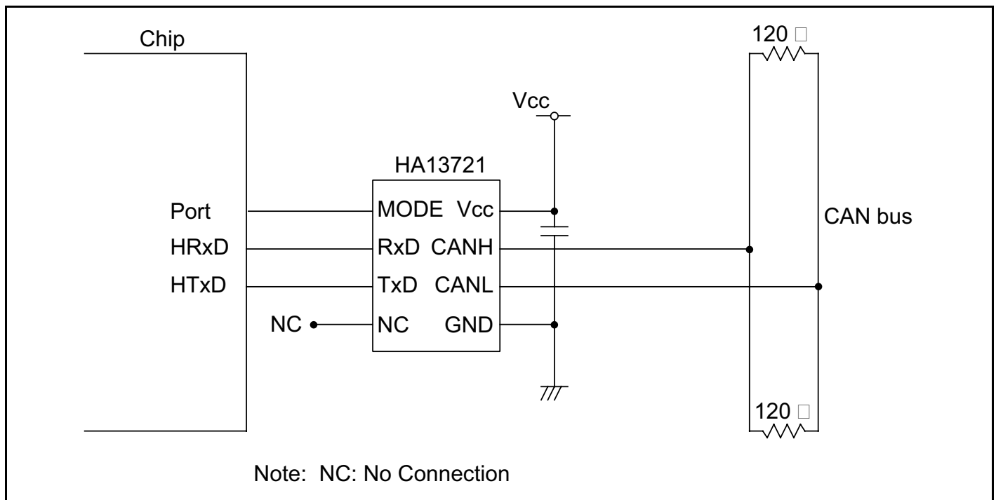
Figure 16-14 High-Speed Interface Using HA13721
