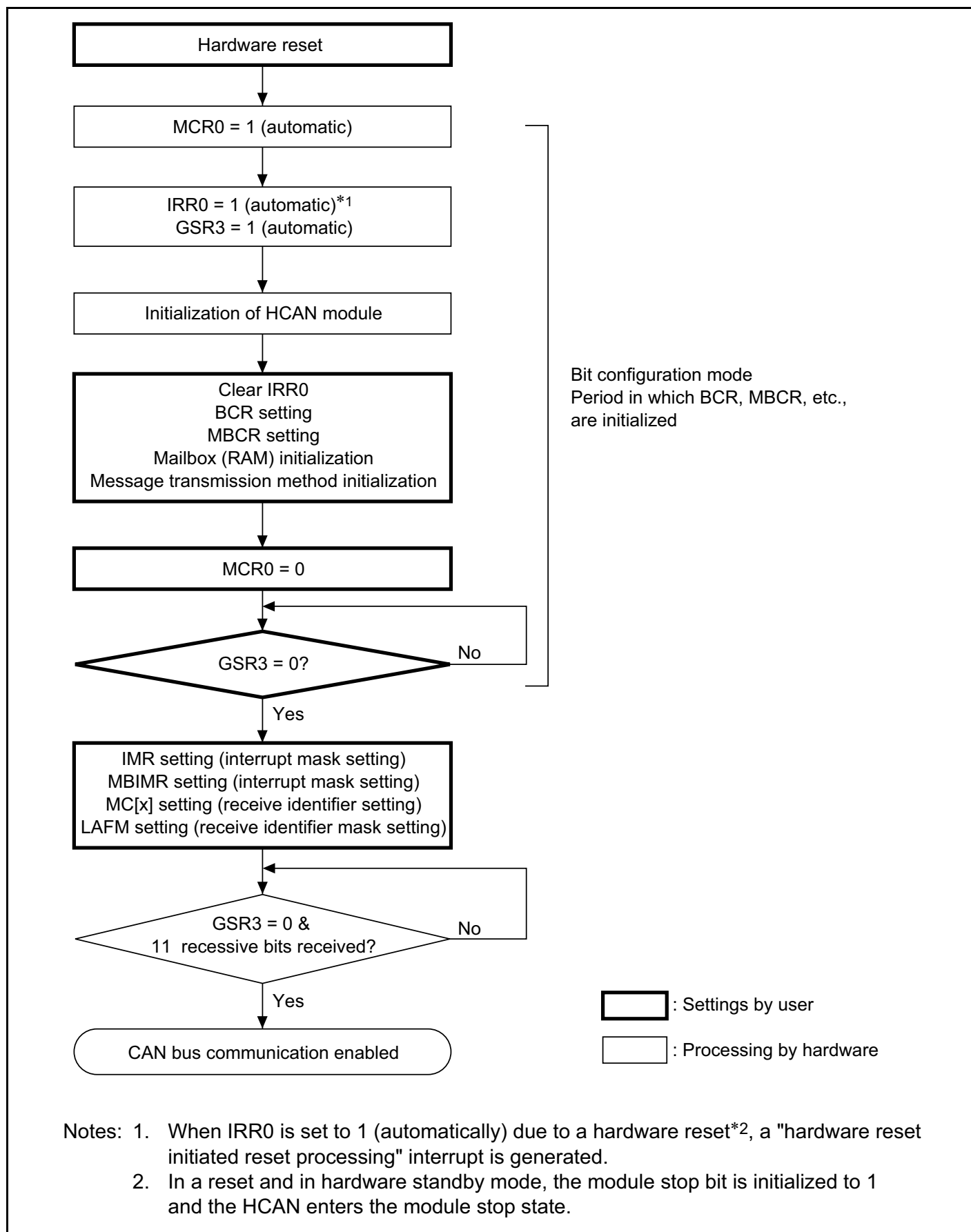
Figure 16-4 Hardware Reset Flowchart
