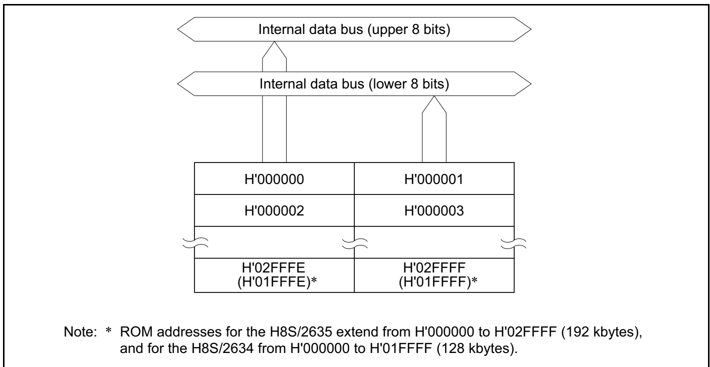
Figure 21C-1 Block Diagram of ROM 192 kbytes (128 kbytes)*
