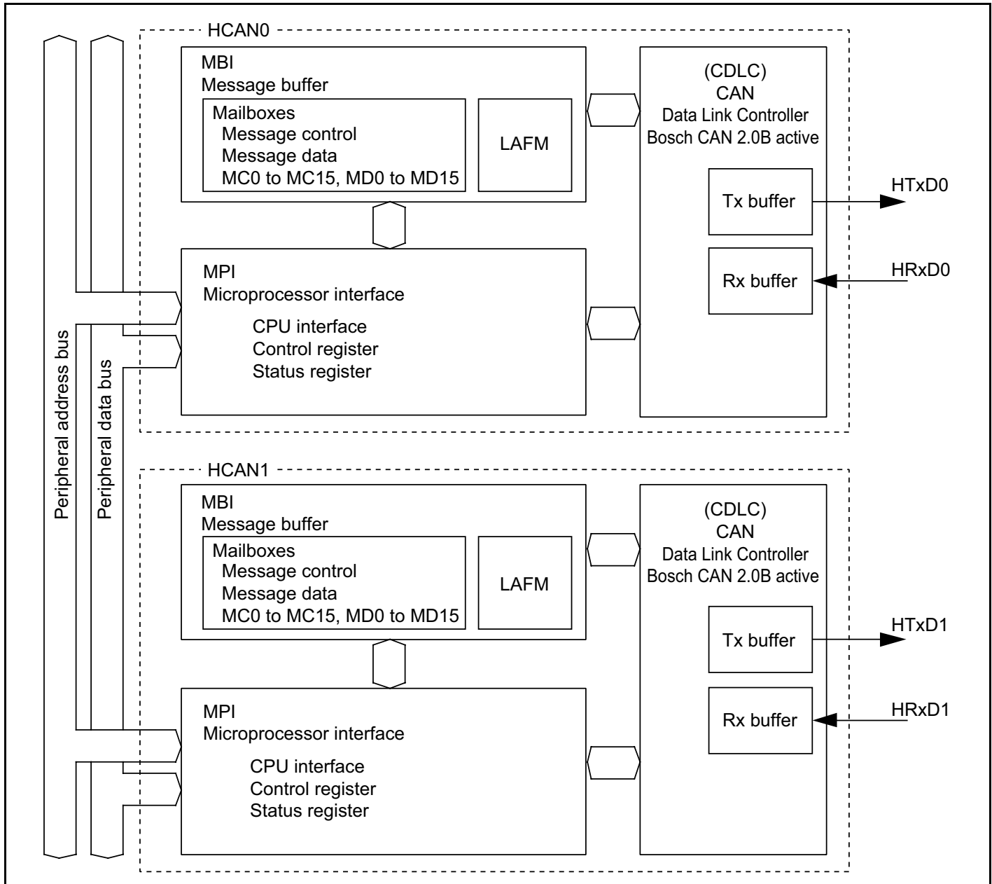
Figure 16-1 HCAN Block Diagram
