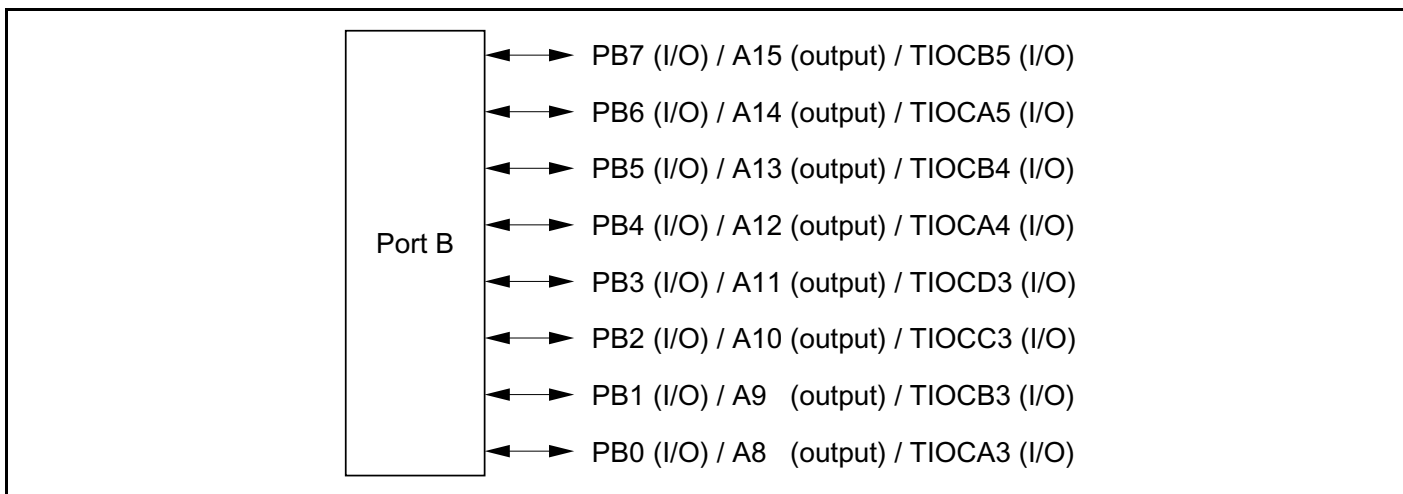
Figure 9-9 Port B Pin Functions (Modes 4 to 6)
