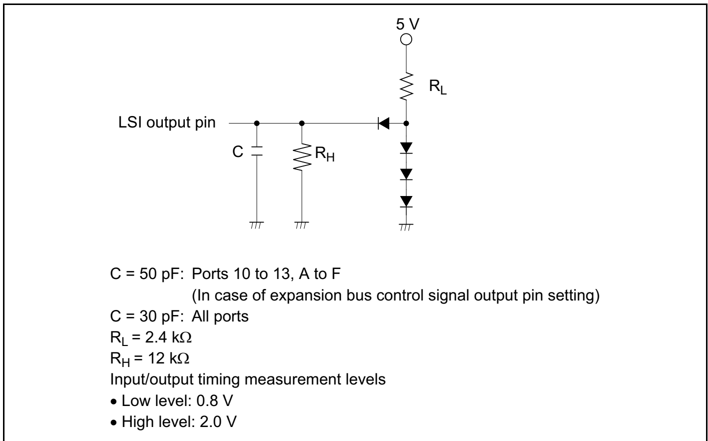
Figure 24-2 Output Load Circuit
