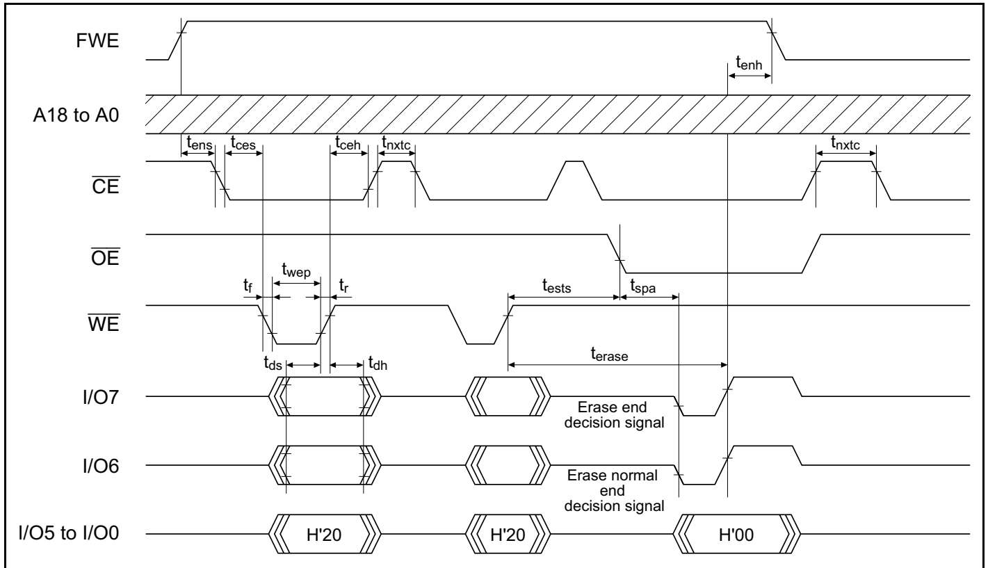
Figure 21C-23 Auto-Erase Mode Timing Waveforms
