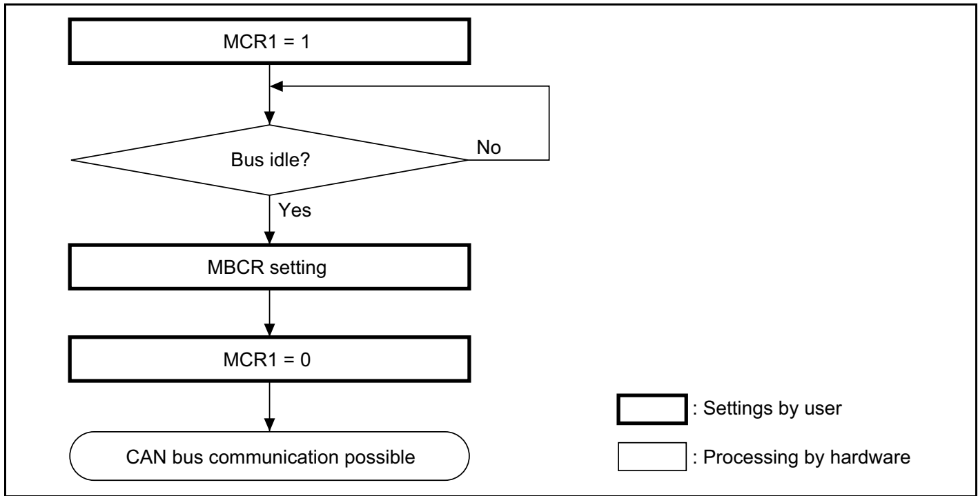
Figure 16-12 HCAN Halt Mode Flowchart
