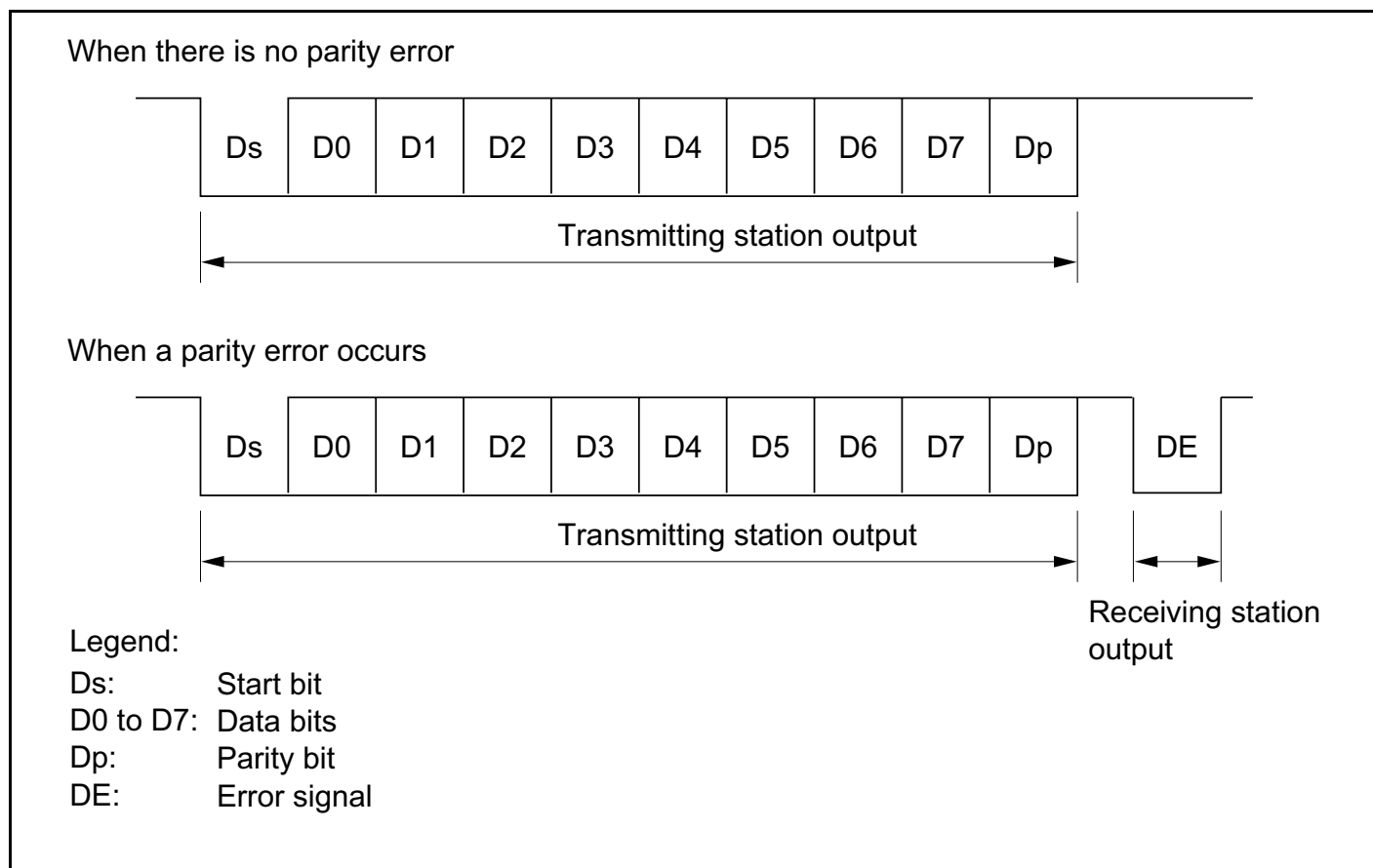
Figure 14-3 Normal Smart Card Interface Data Format
