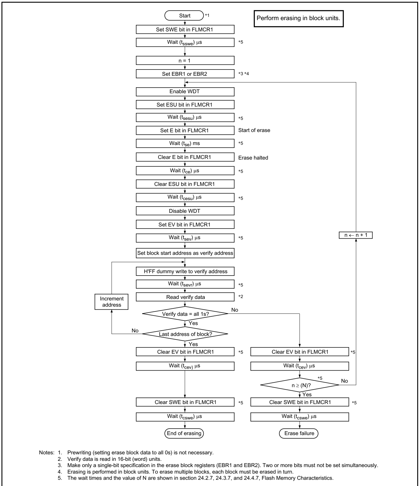
Figure 21B-13 Erase/Eraser-Verify Flowchart
