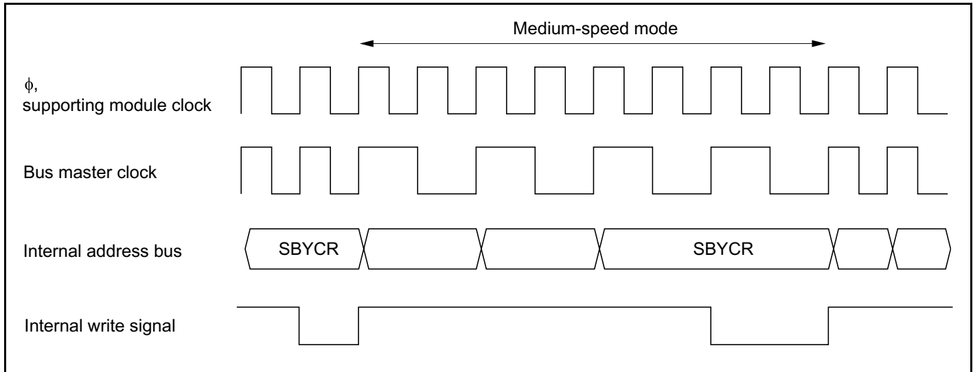
Figure 23B-2 Medium-Speed Mode Transition and Clearance Timing
