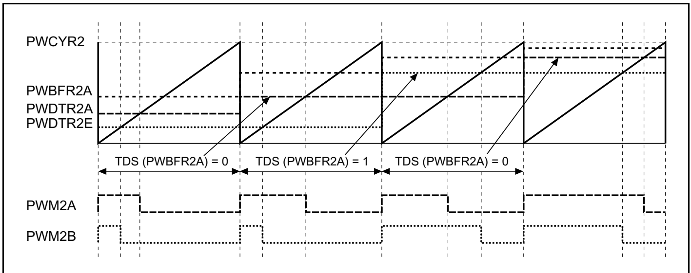
Figure 19-11 PWM Channel 2 Operation
