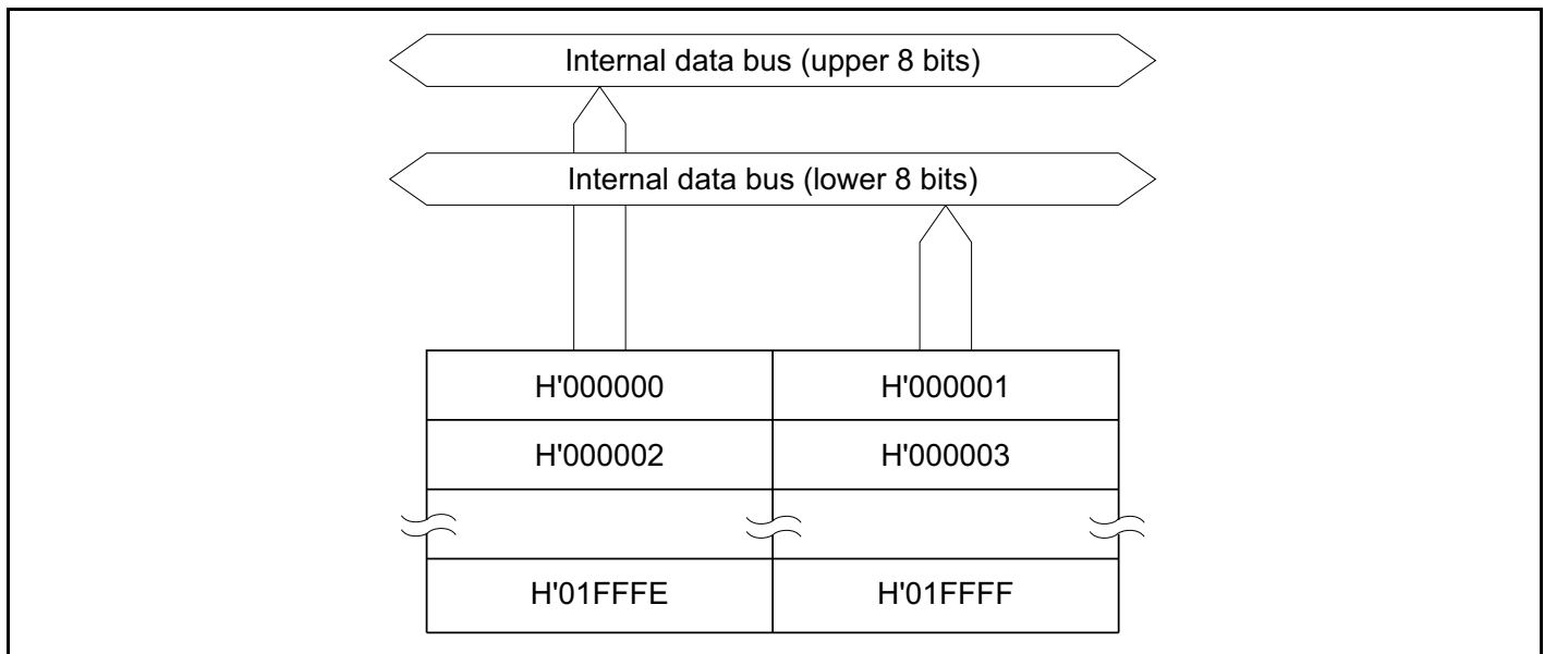
Figure 21A-1 Block Diagram of ROM (128 kbytes)
