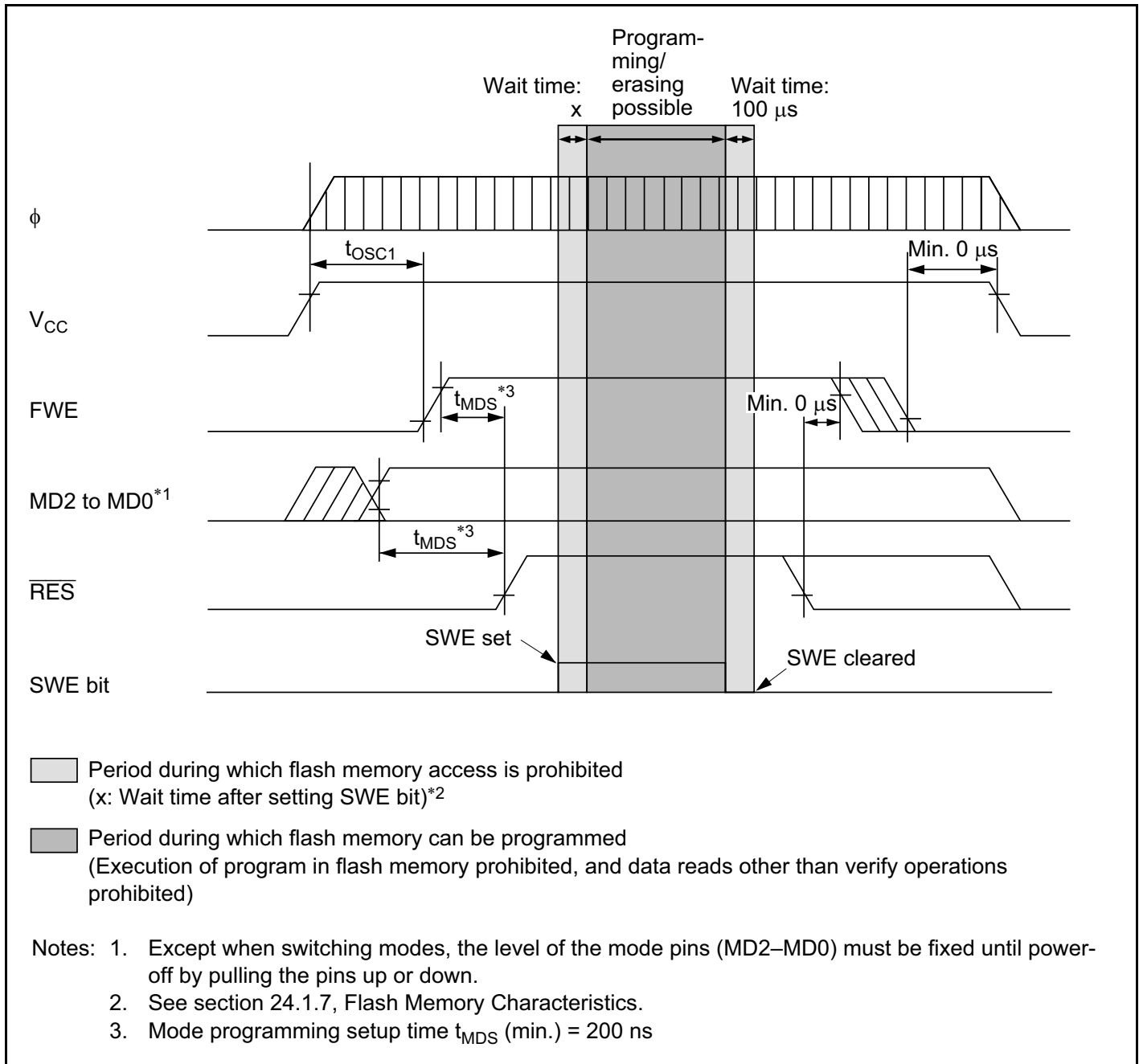
Figure 21A-26 Power-On/Off Timing (Boot Mode)
