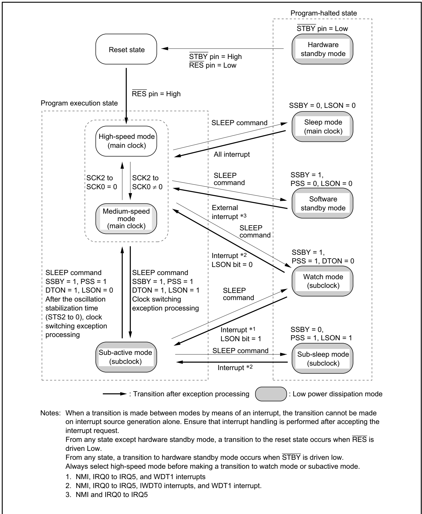
Figure 23B-1 Mode Transition Diagram
