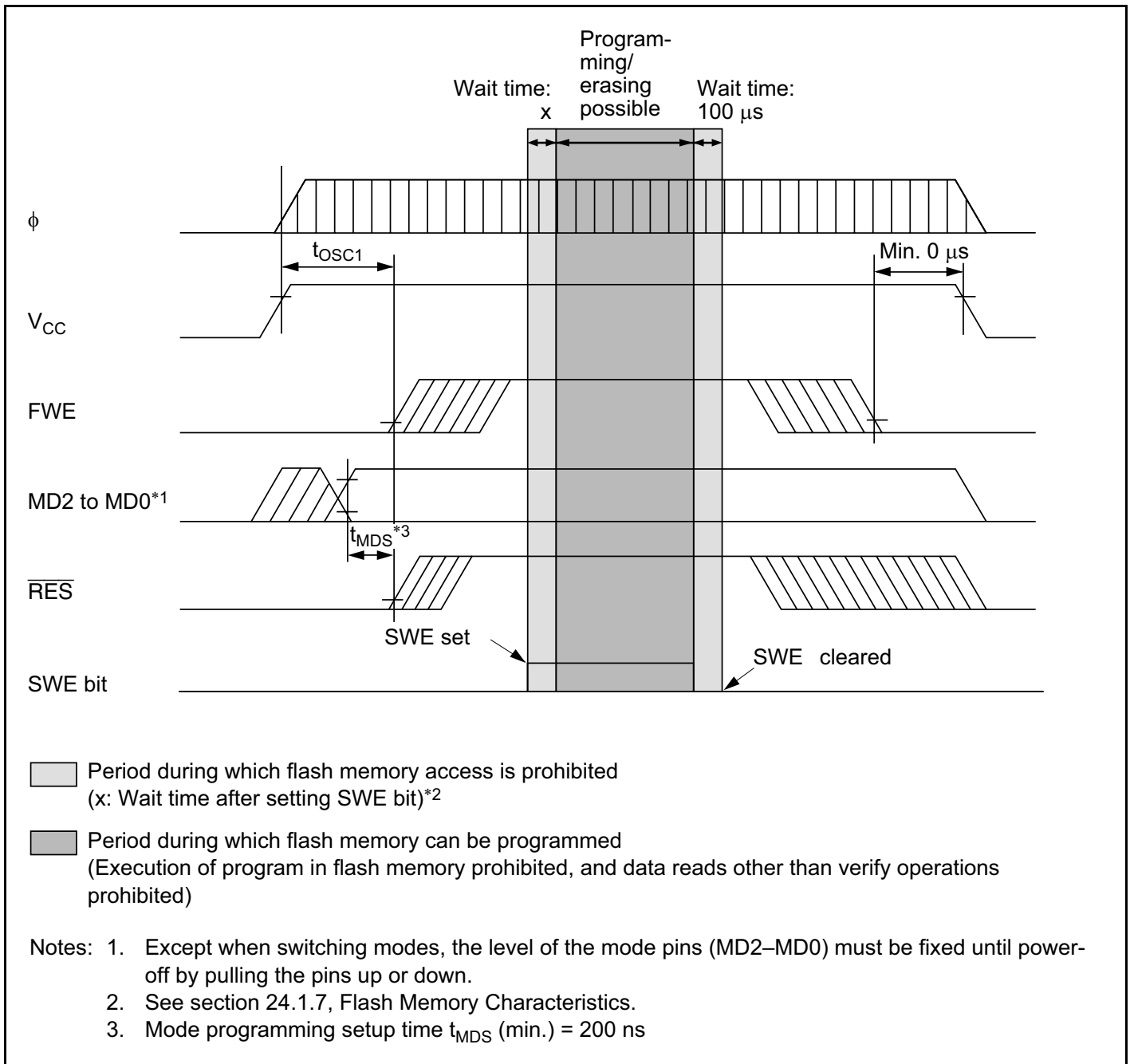
Figure 21A-27 Power-On/Off Timing (User Program Mode)
