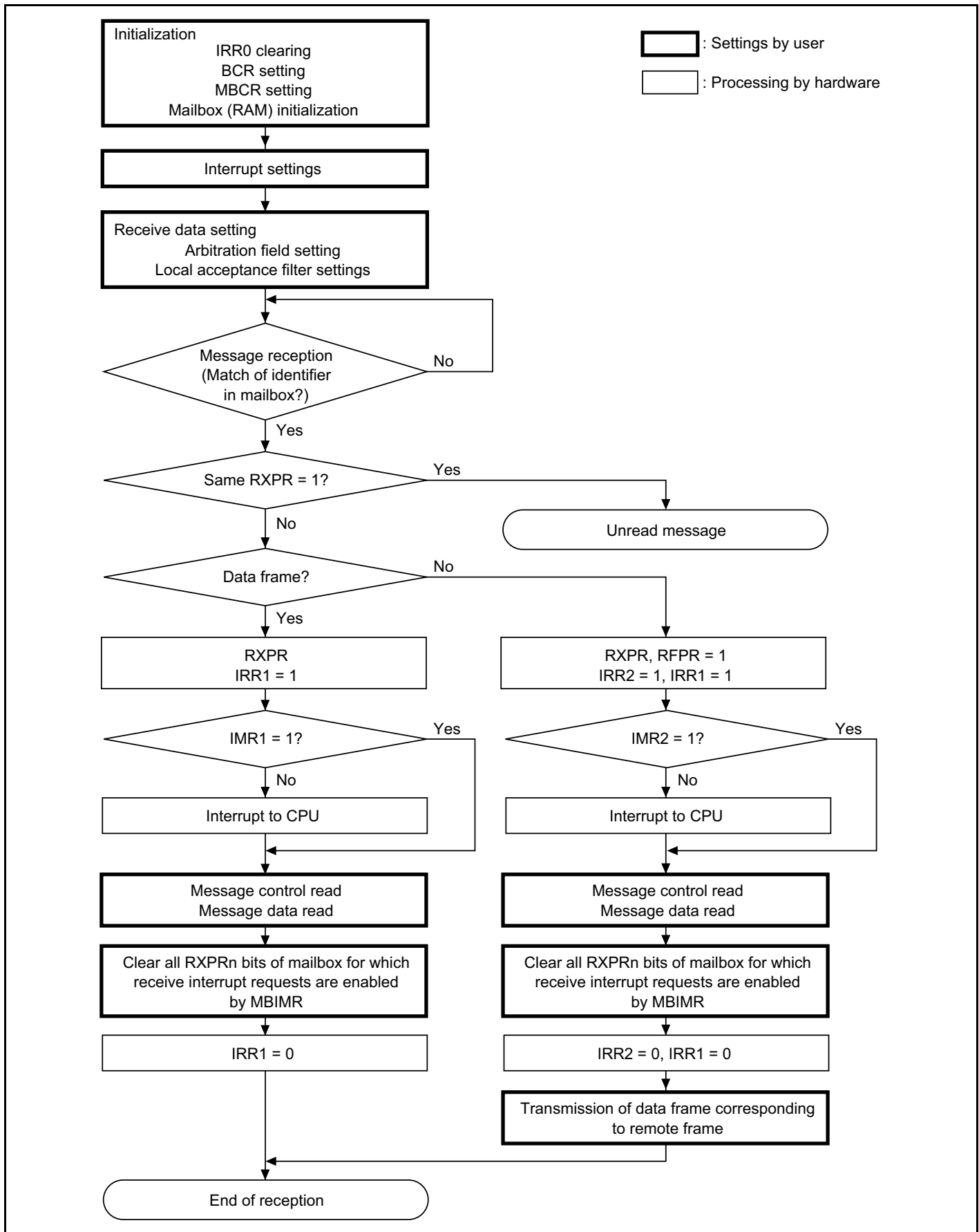
Figure 16-9 Reception Flowchart
