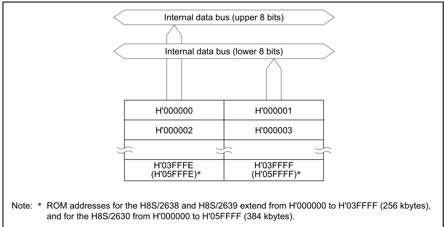
Figure 21B-1 Block Diagram of ROM 256 kbytes (384 kbytes)*
