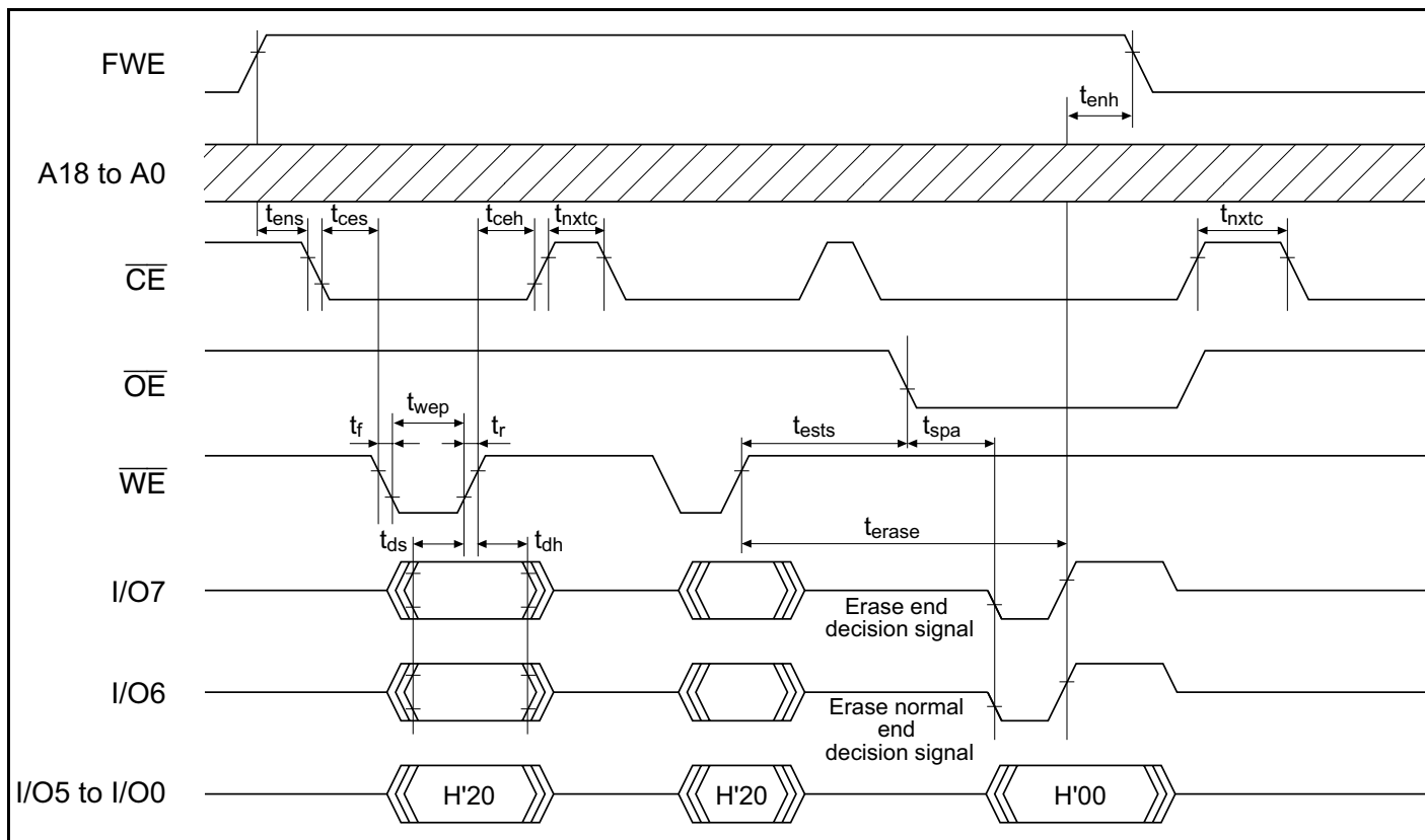
Figure 21A-23 Auto-Erase Mode Timing Waveforms
