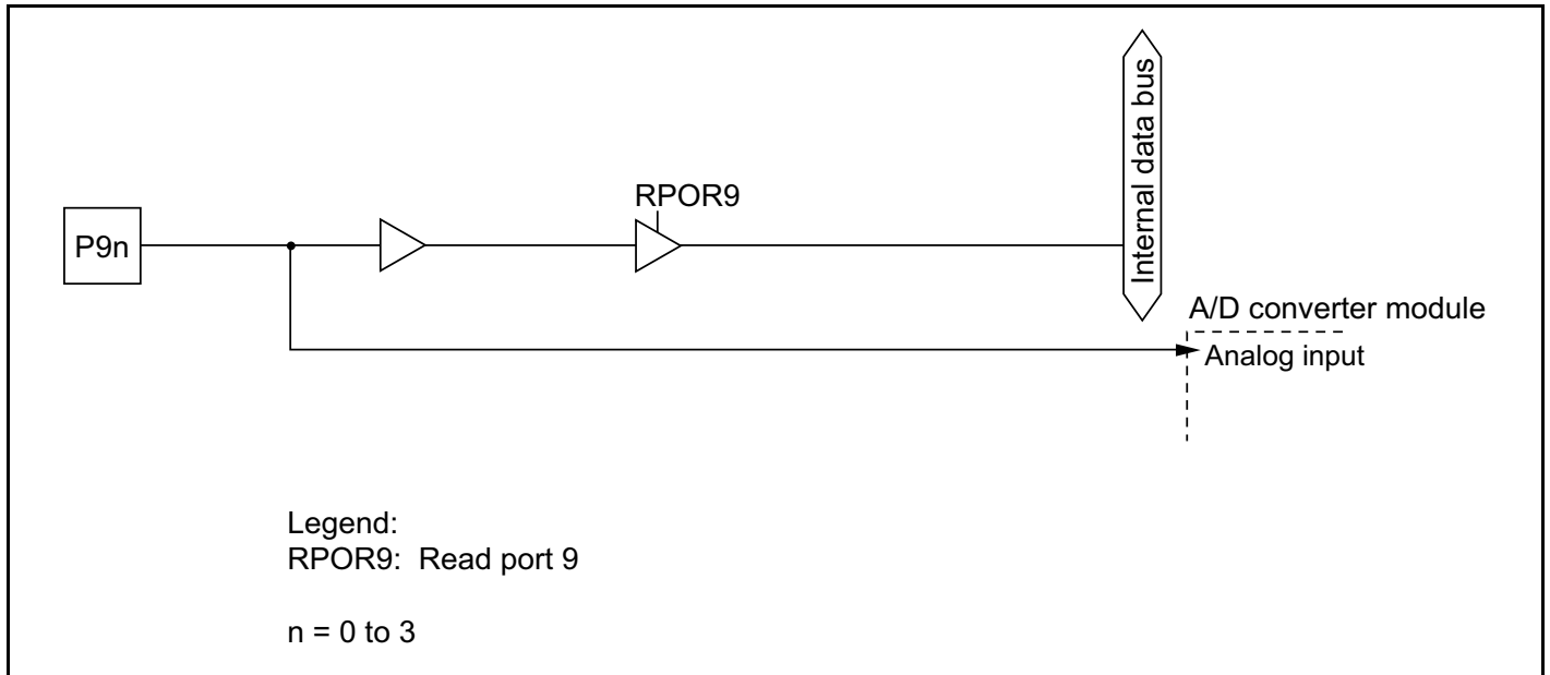
Figure C-4 Port 9 Block Diagram (Pins P90 to P93)
