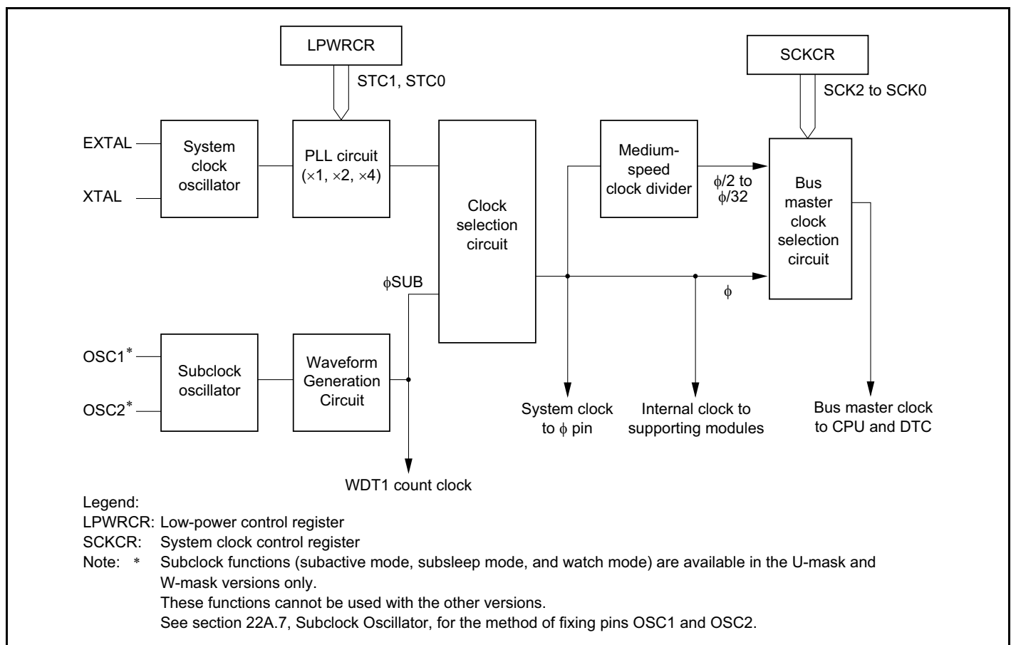
Figure 22A-1 Block Diagram of Clock Pulse Generator
