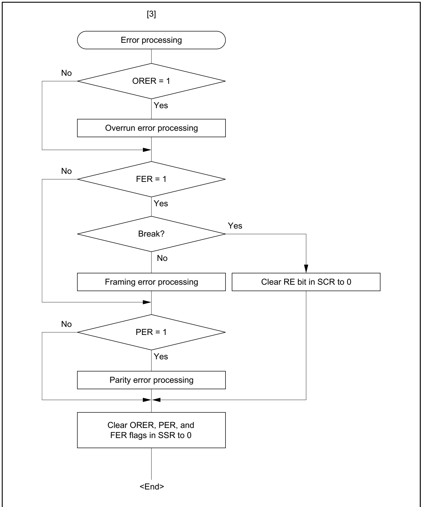
Figure 13-7 Sample Serial Reception Data Flowchart (cont)
