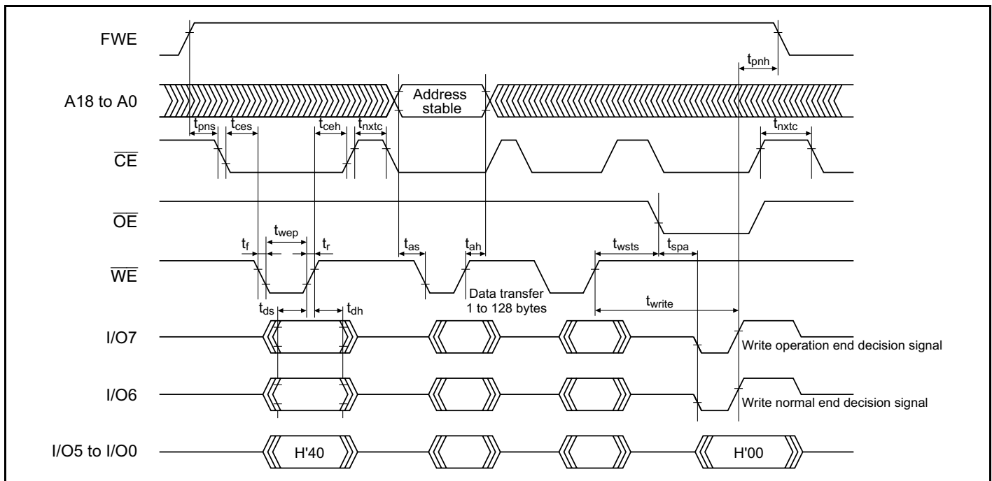
Figure 21B-22 Auto-Program Mode Timing Waveforms
