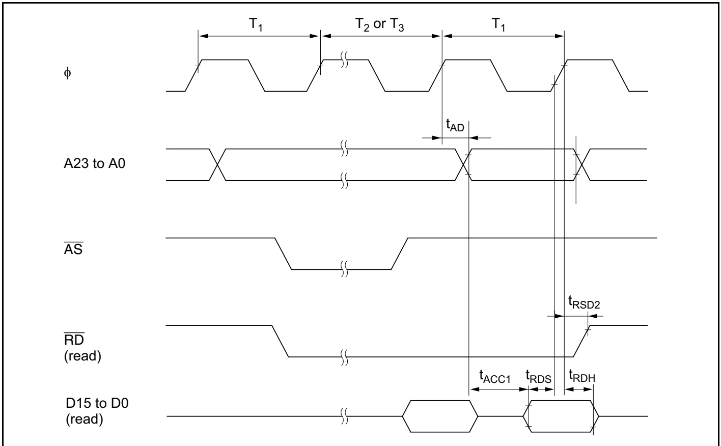
Figure 24-17 Burst ROM Access Timing (One-State Access)
