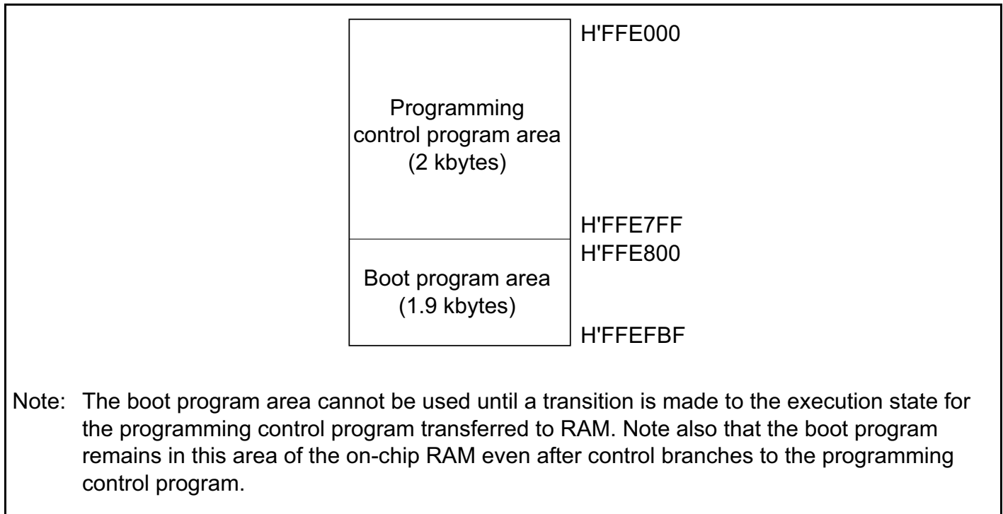
Figure 21C-9 RAM Areas in Boot Mode
