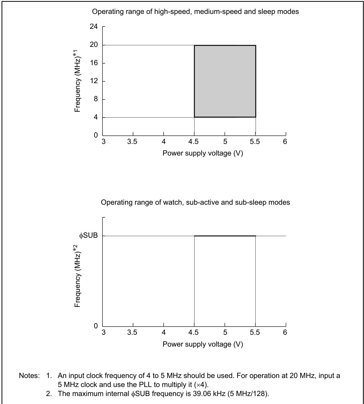
Figure 24-5 Power Supply Voltage and Operating Ranges
