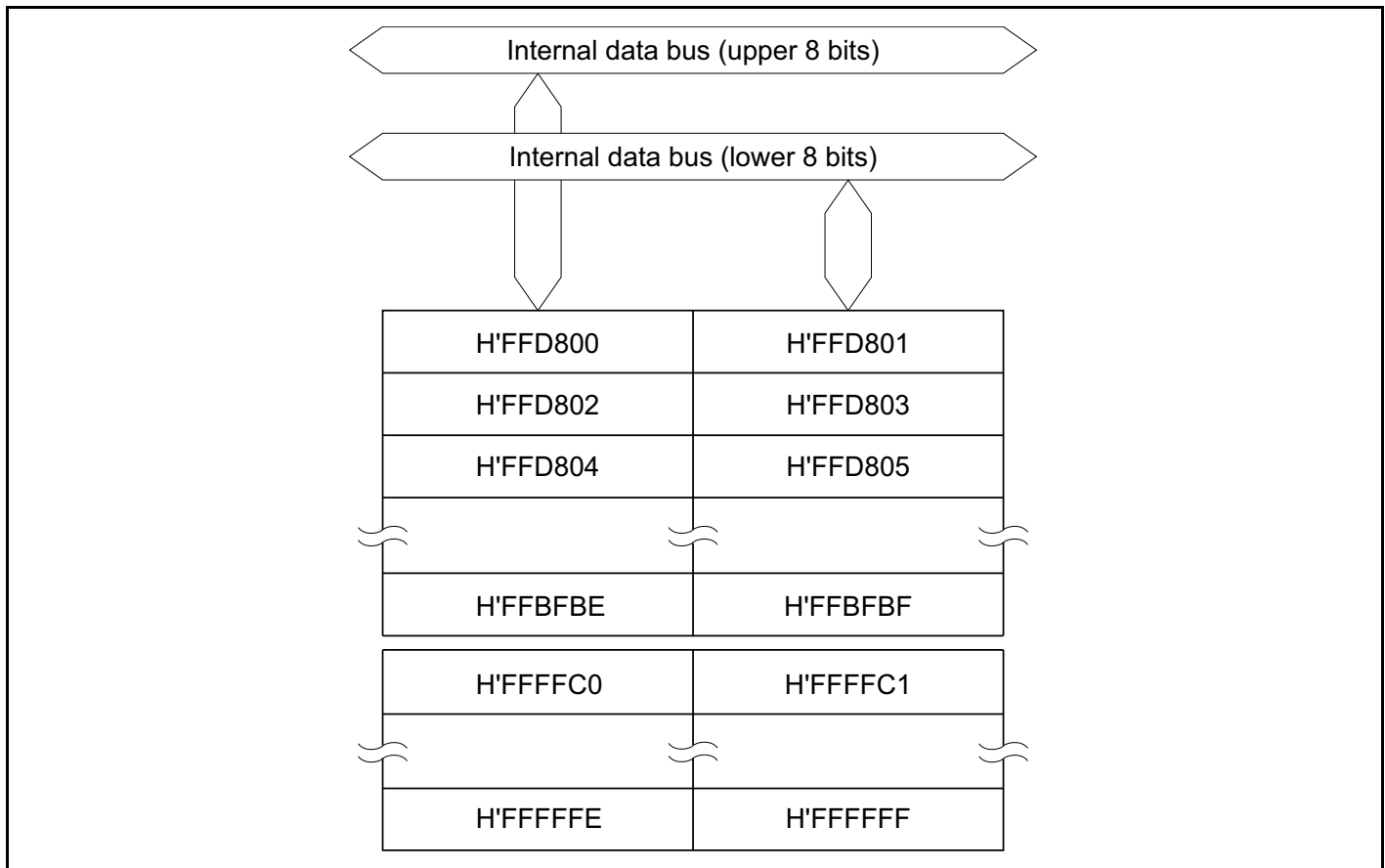
Figure 20-1 (c) Block Diagram of RAM (H8S/2635 Group)
