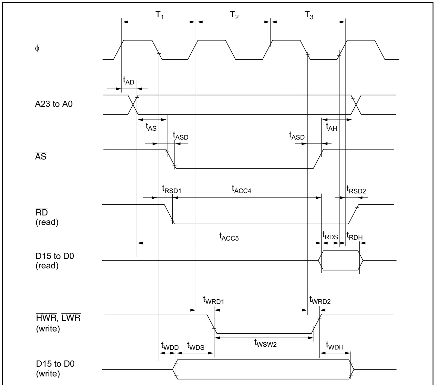
Figure 24-14 Basic Bus Timing (Three-State Access)
