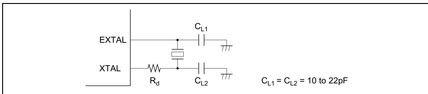
Figure 22B-2 Connection of Crystal Resonator (Example)
