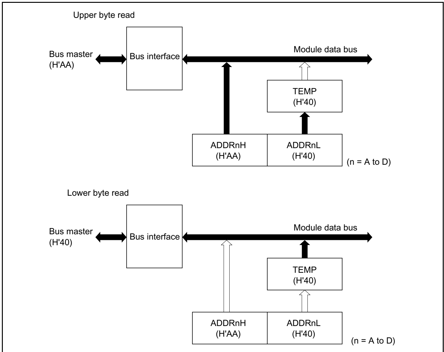
Figure 17-2 ADDR Access Operation (Reading H'AA40)
