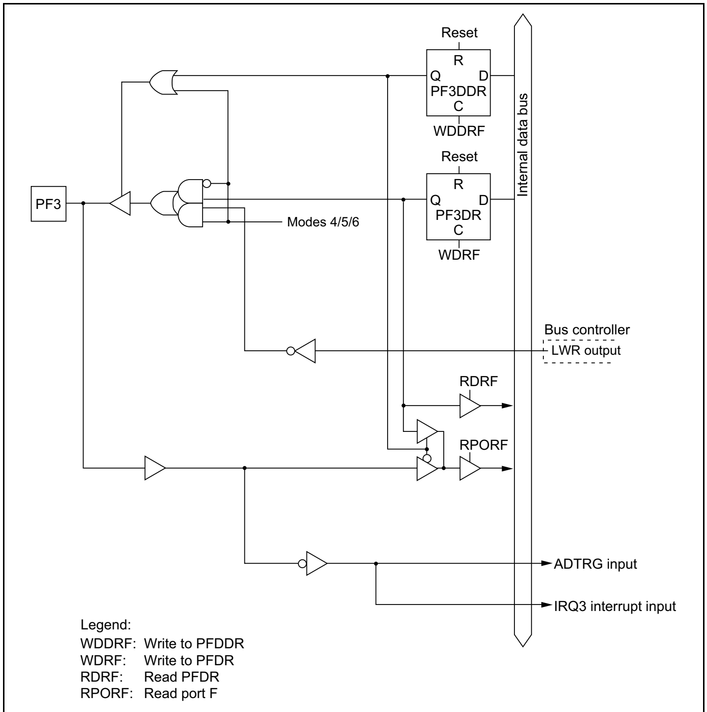
Figure C-10 (b) Port F Block Diagram (Pin PF3)
