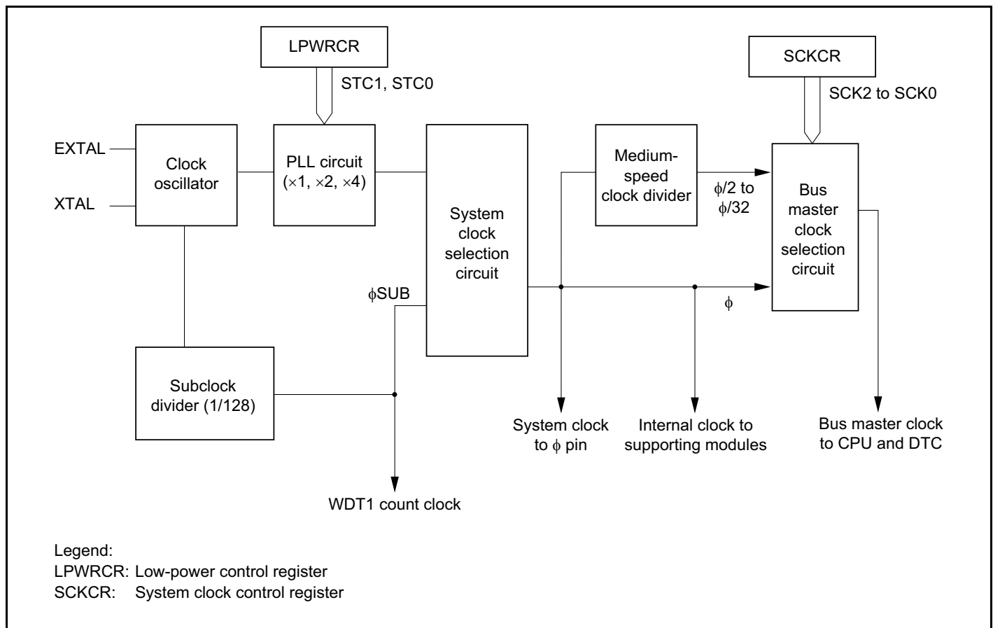
Figure 22B-1 Block Diagram of Clock Pulse Generator
