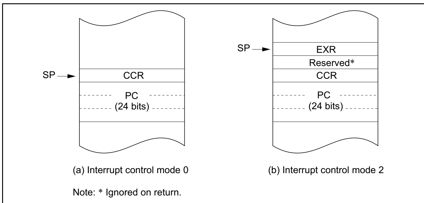
Figure 4-5 (2) Stack Status after Exception Handling (Advanced Modes)
