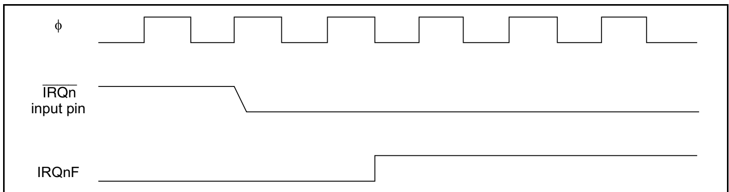
Figure 5-3 Timing of Setting IRQnF
