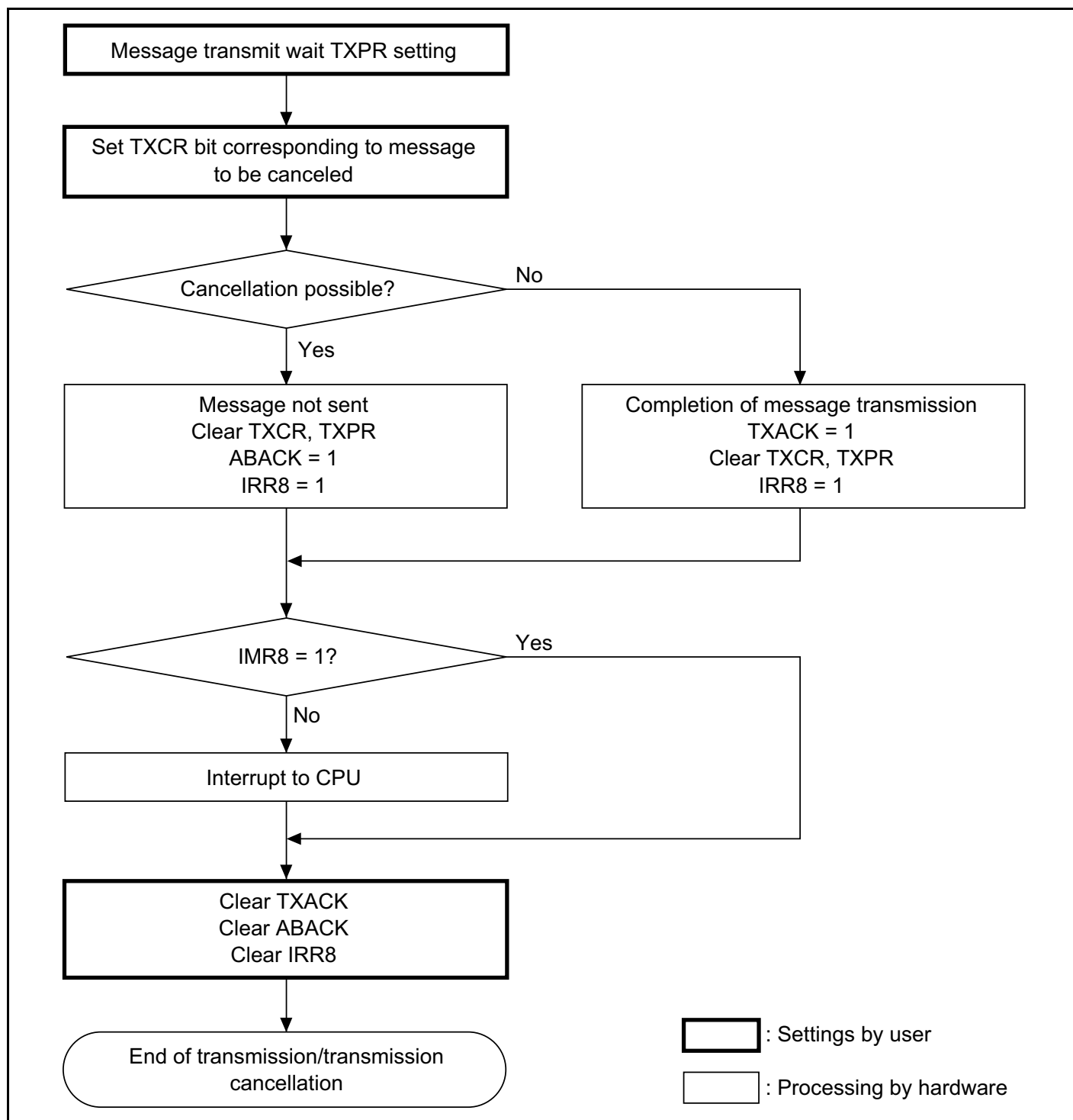
Figure 16-8 Transmit Message Cancellation Flowchart
