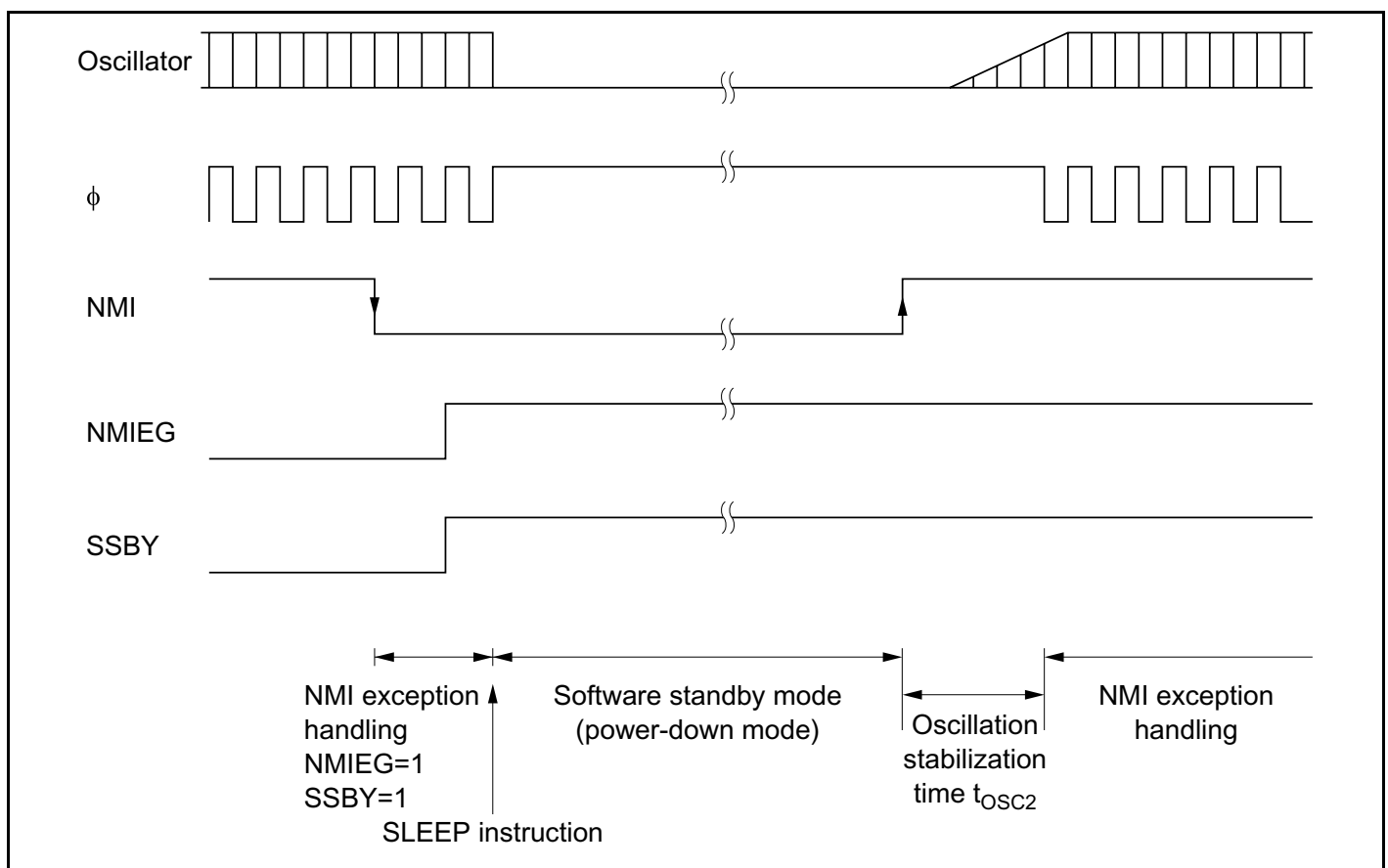
Figure 23A-3 Software Standby Mode Application Example
