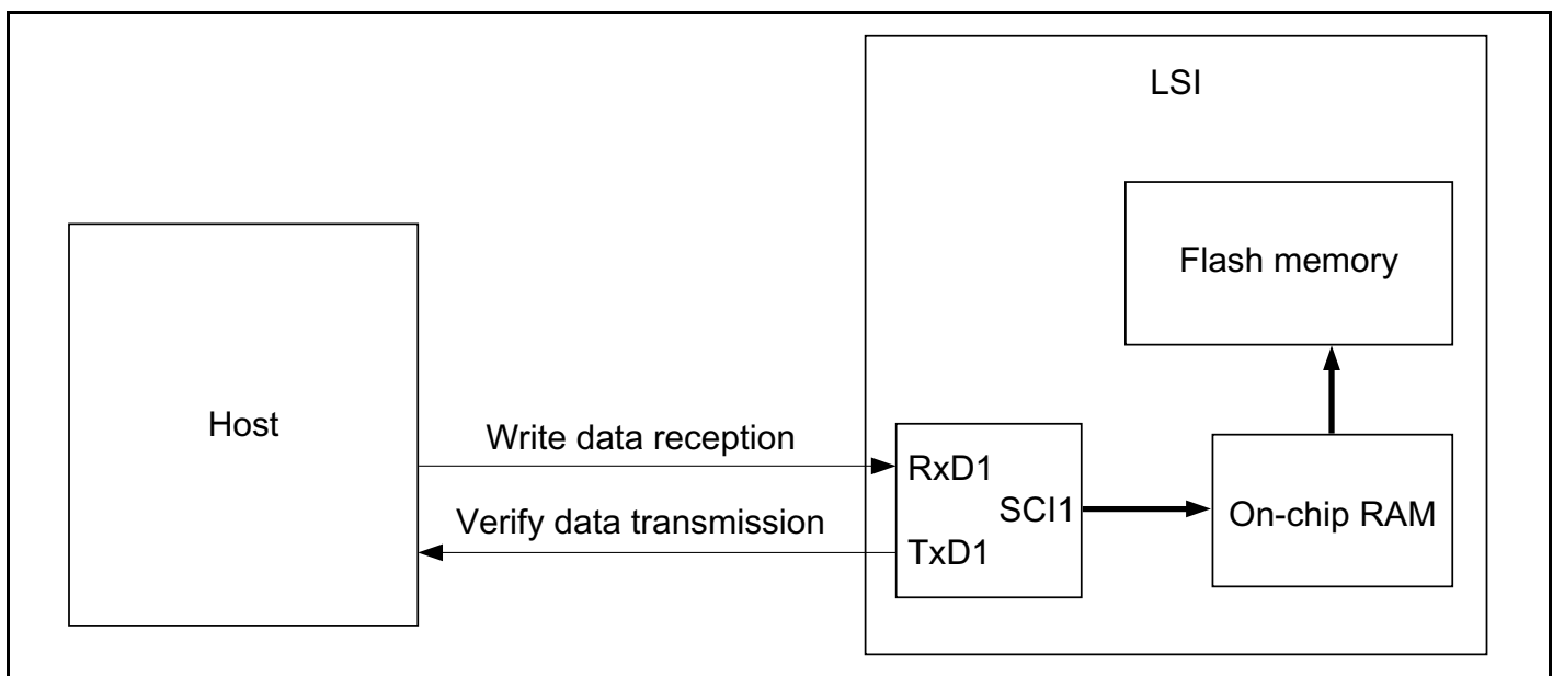
Figure 21A-7 System Configuration in Boot Mode
