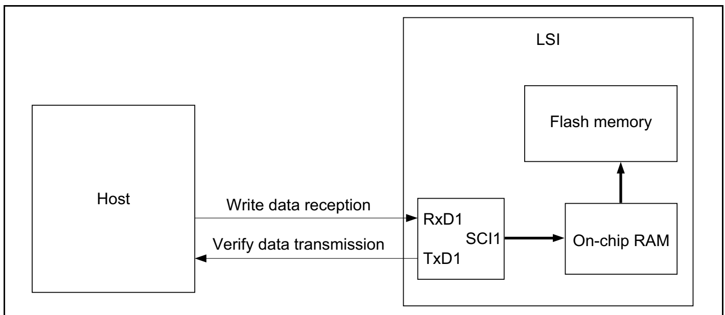
Figure 21C-7 System Configuration in Boot Mode
