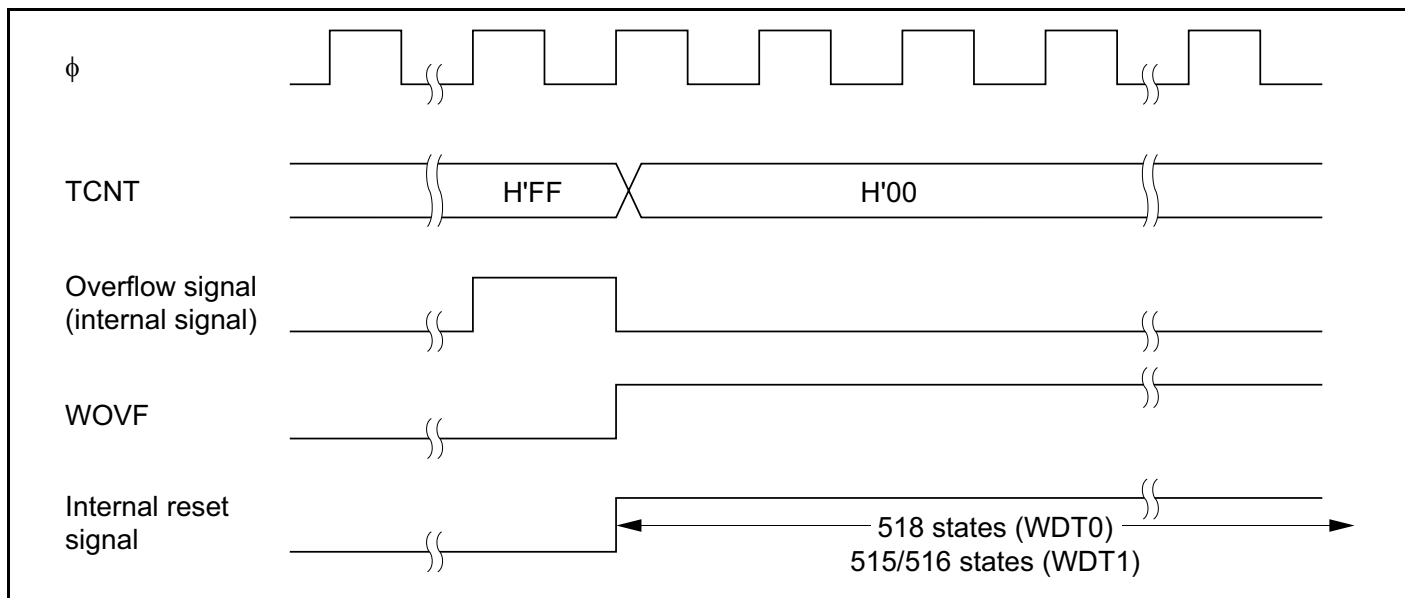
Figure 12-7 Timing of Setting of WOVF
