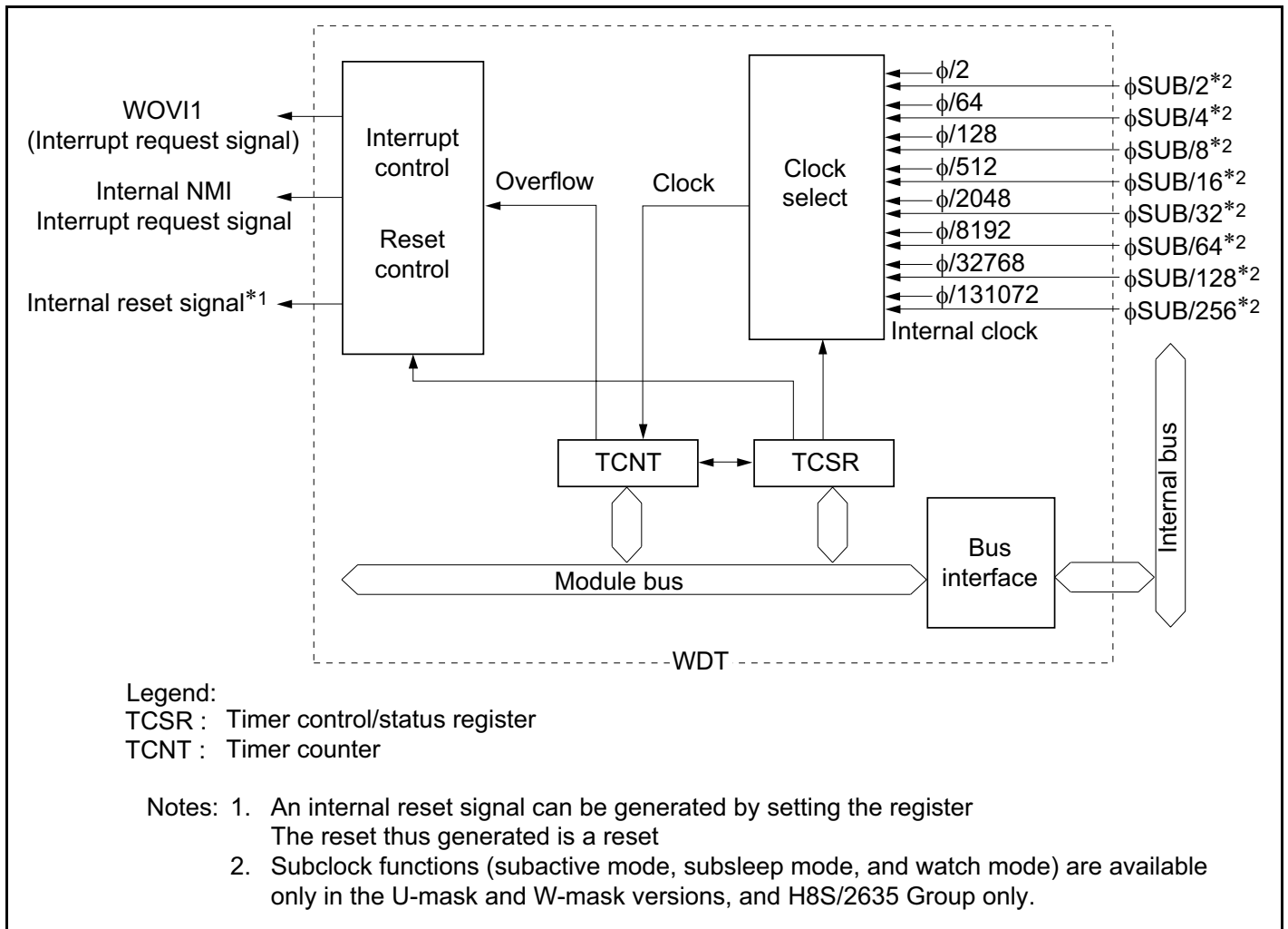
Figure 12-1 (b) Block Diagram of WDT1
