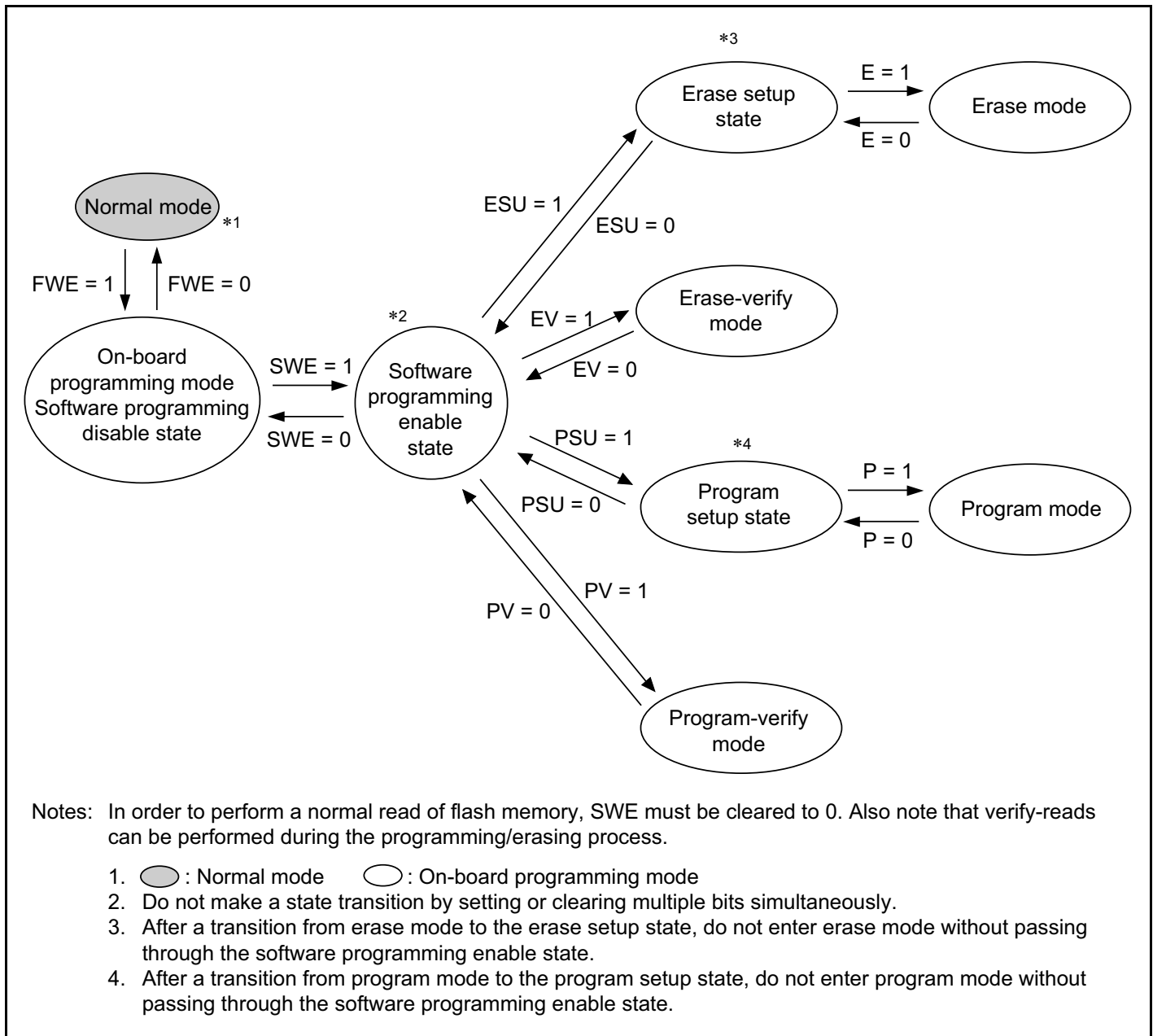
Figure 21C-11 FLMCR1 Bit Settings and State Transitions
