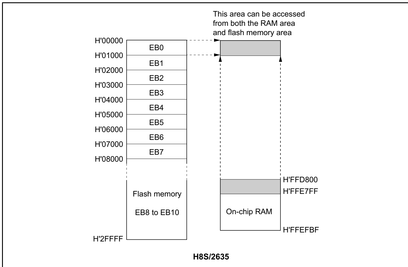
Figure 21C-16 Example of RAM Overlap Operation
