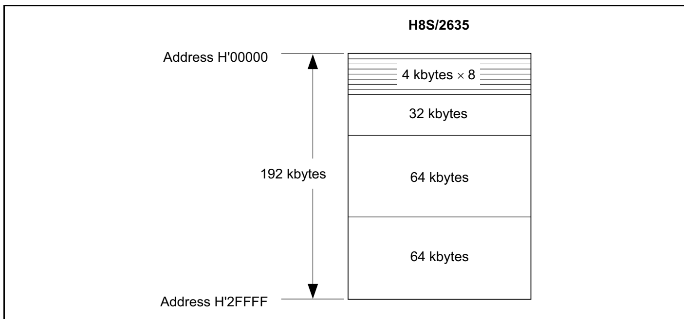
Figure 21C-6 Flash Memory Block Configuration
