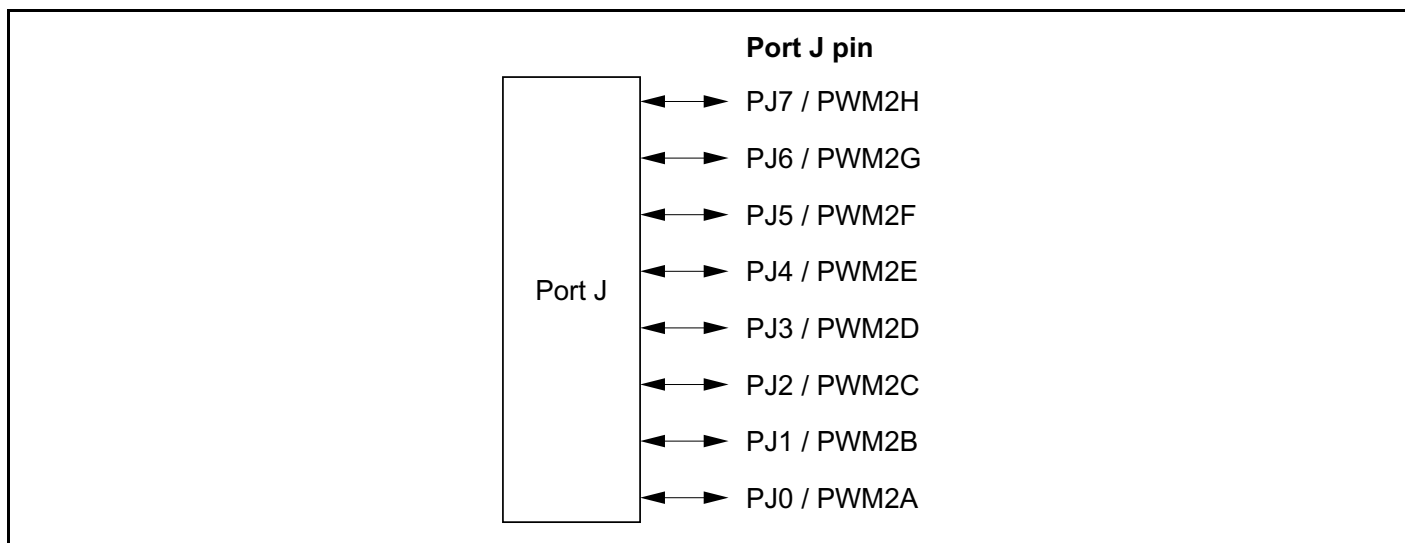
Figure 9-23 Port J Pin Functions
