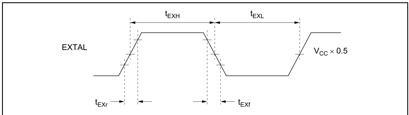
Figure 22B-7 External Clock Input Timing
