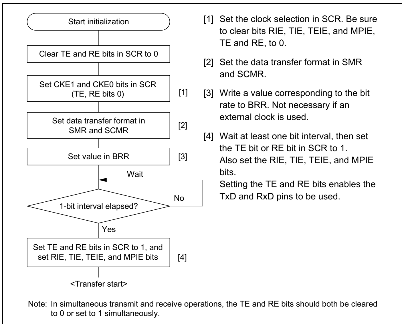
Figure 13-15 Sample SCI Initialization Flowchart
