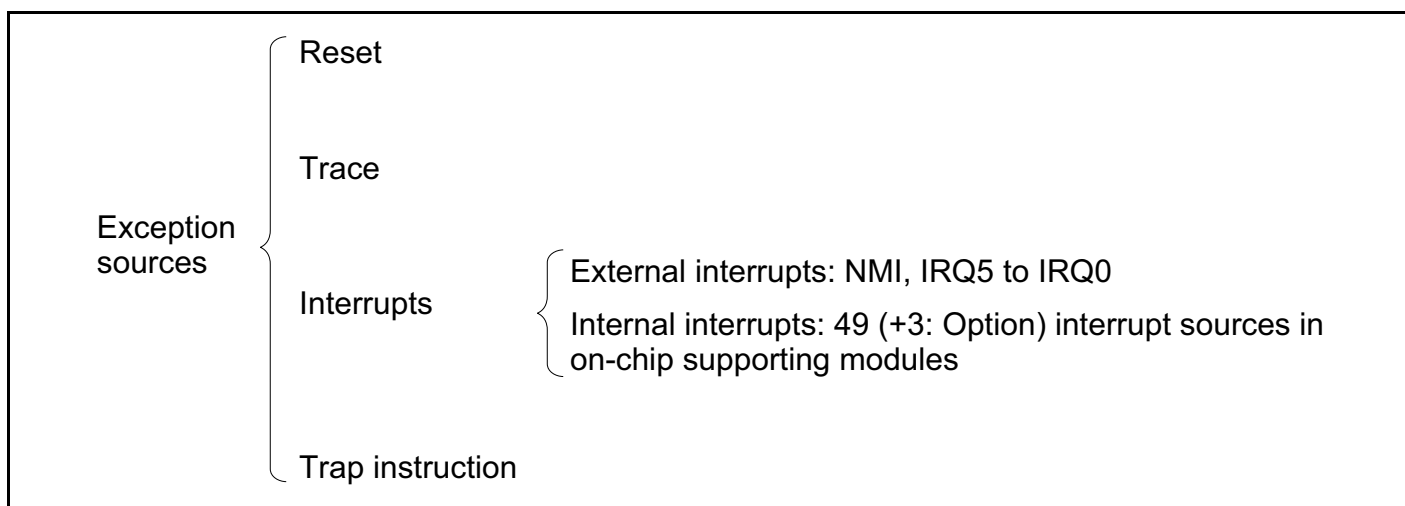
Figure 4-1 Exception Sources
