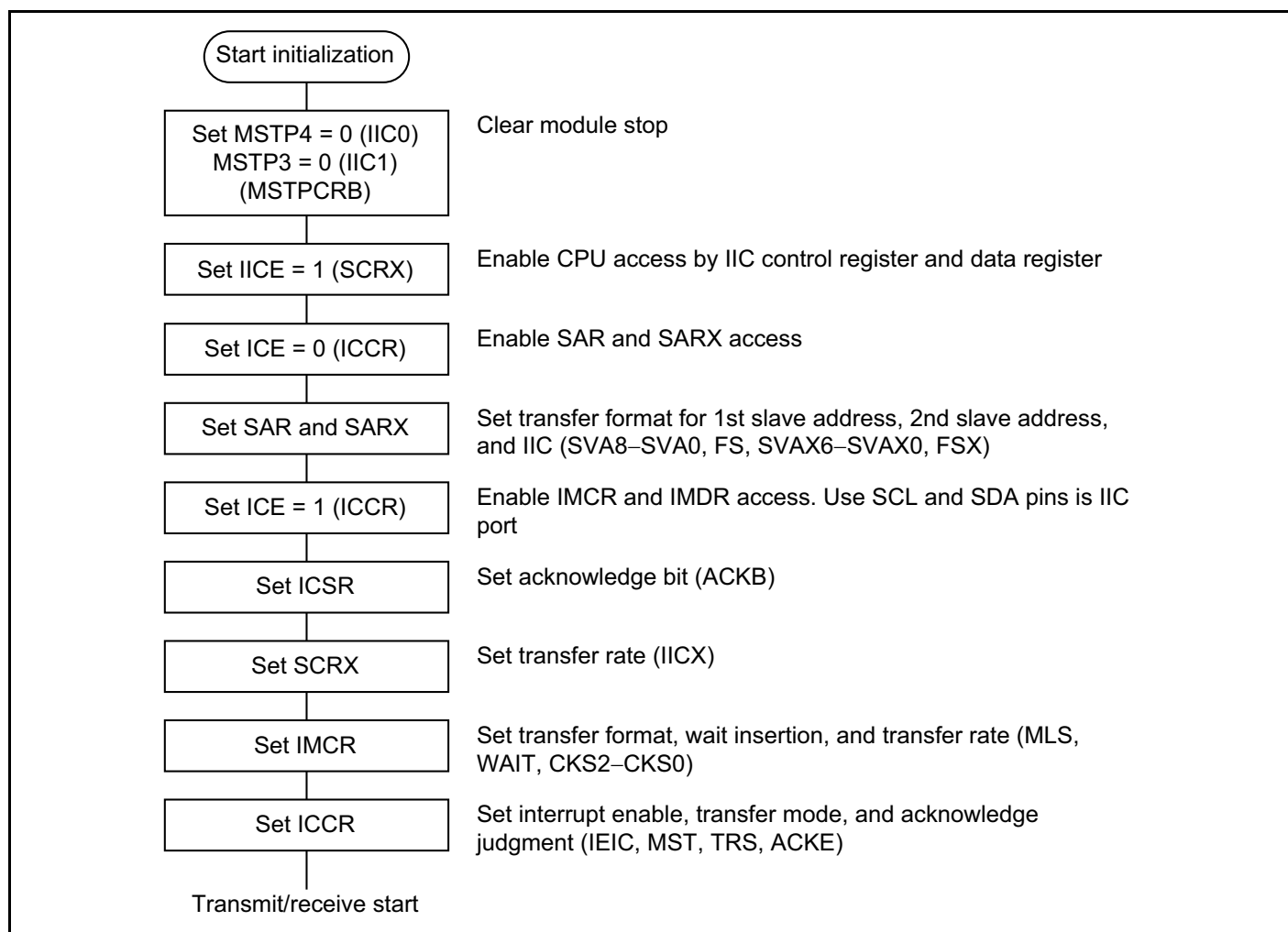
Figure 15-6 Flowchart for IIC Initialization (Example)
