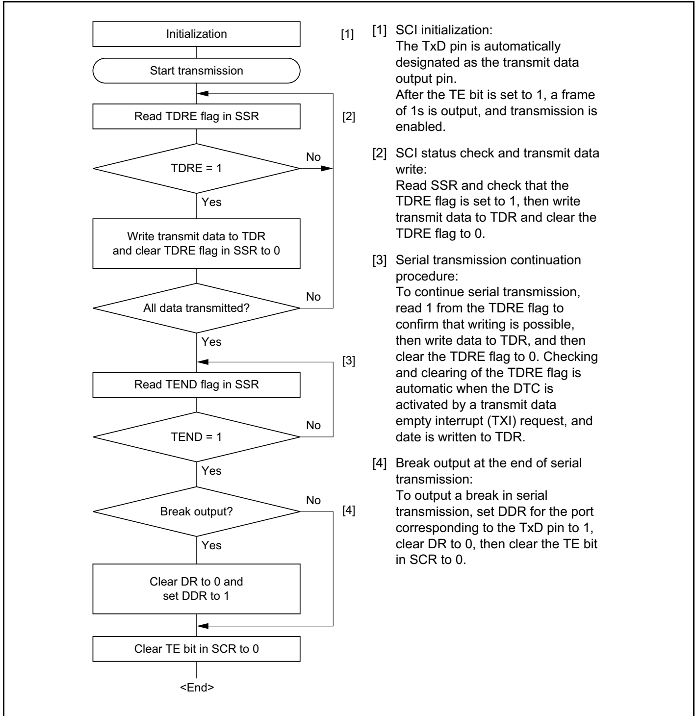
Figure 13-5 Sample Serial Transmission Flowchart
