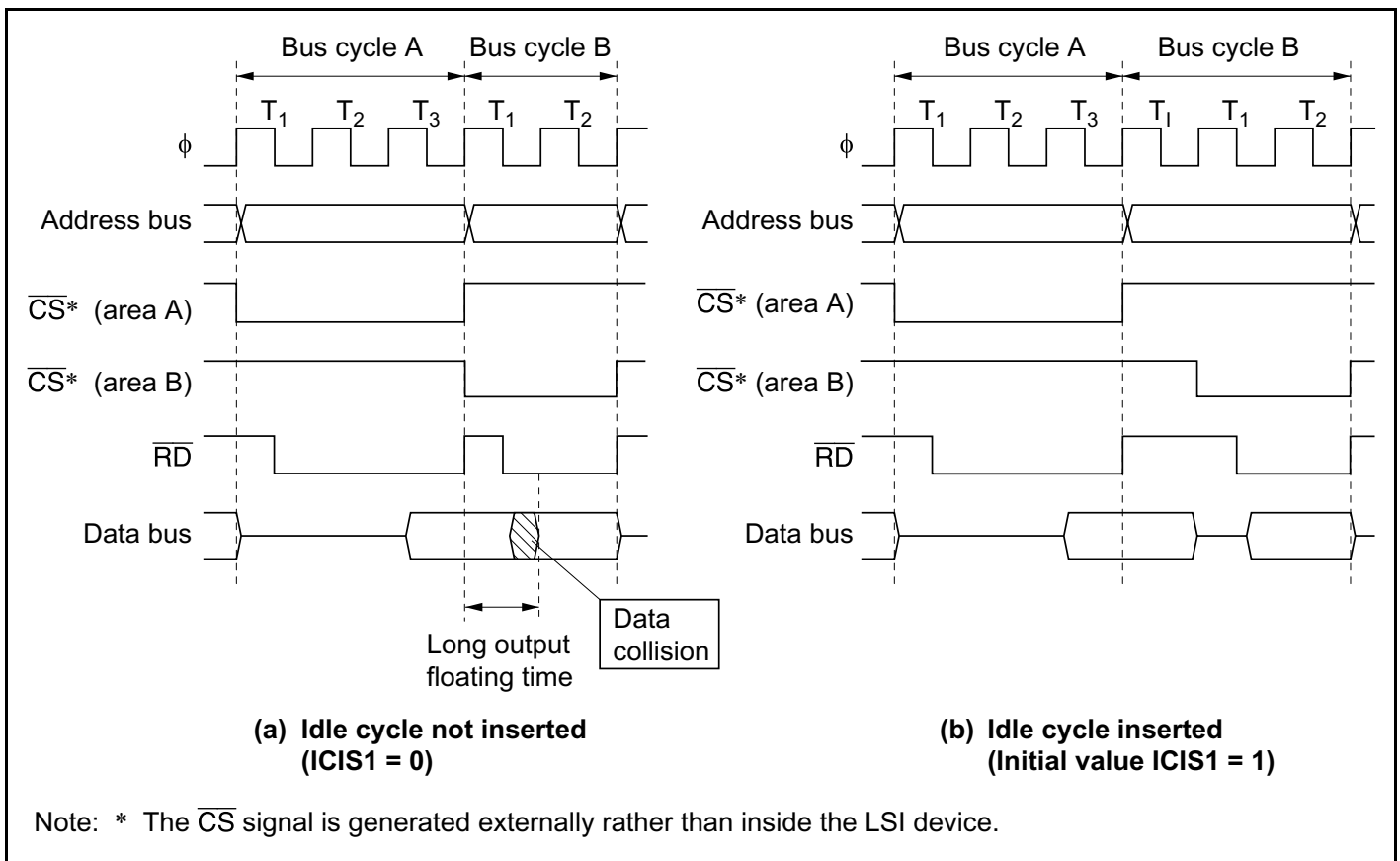
Figure 7-15 Example of Idle Cycle Operation (1)
