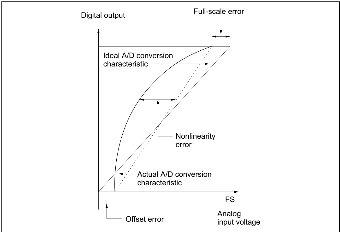
Figure 17-10 A/D Conversion Precision Definitions (2)
