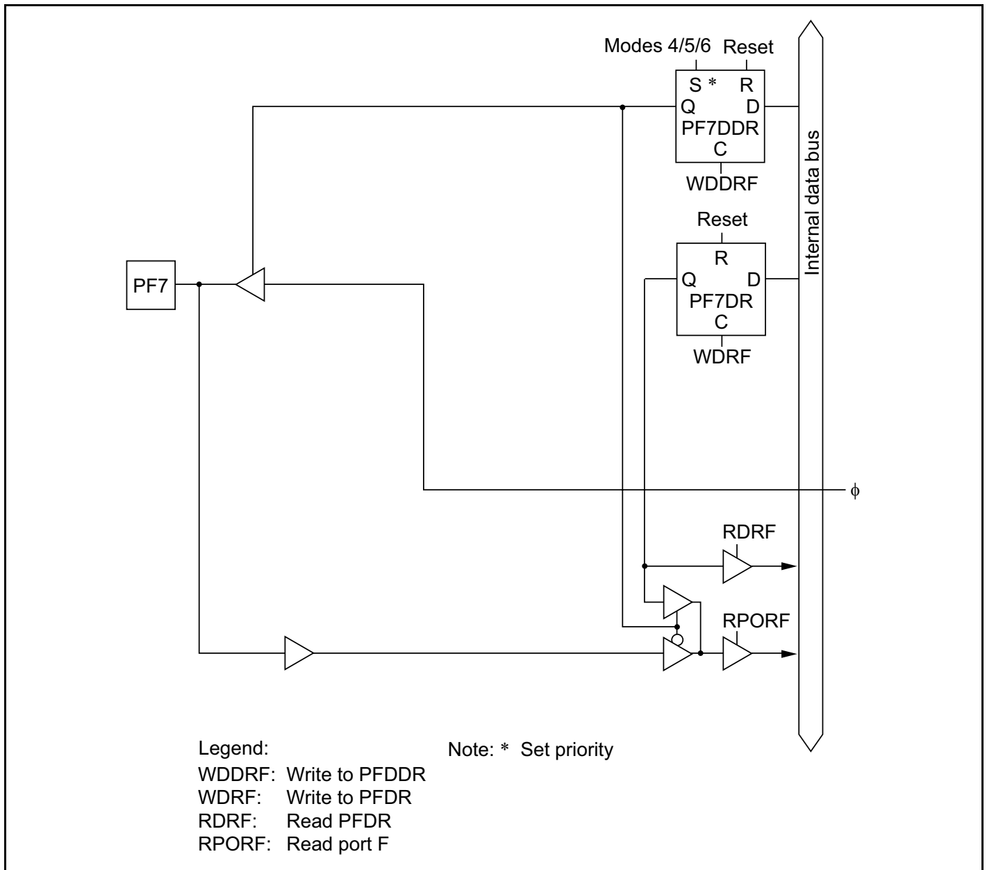
Figure C-10 (f) Port F Block Diagram (Pin PF7)
