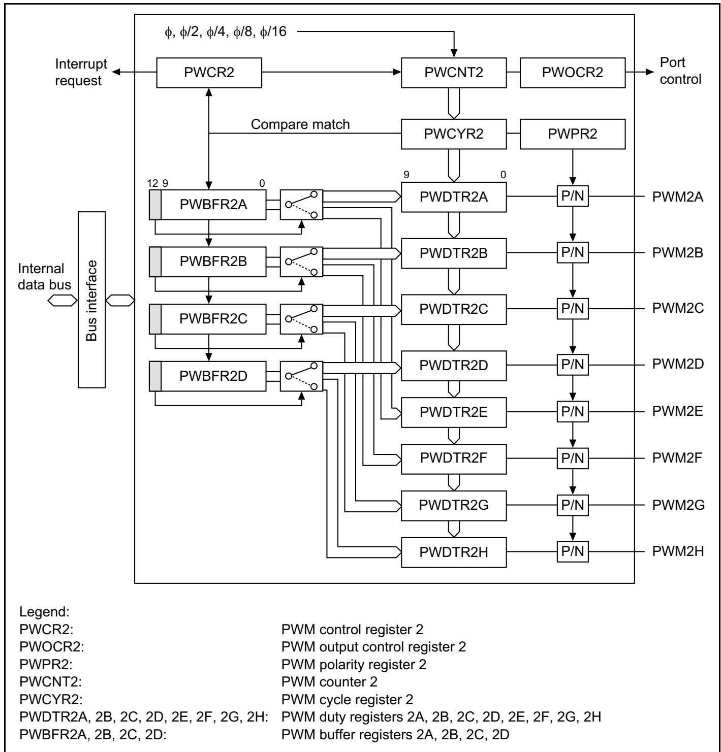
Figure 19-2 Block Diagram of PWM Channel 2
