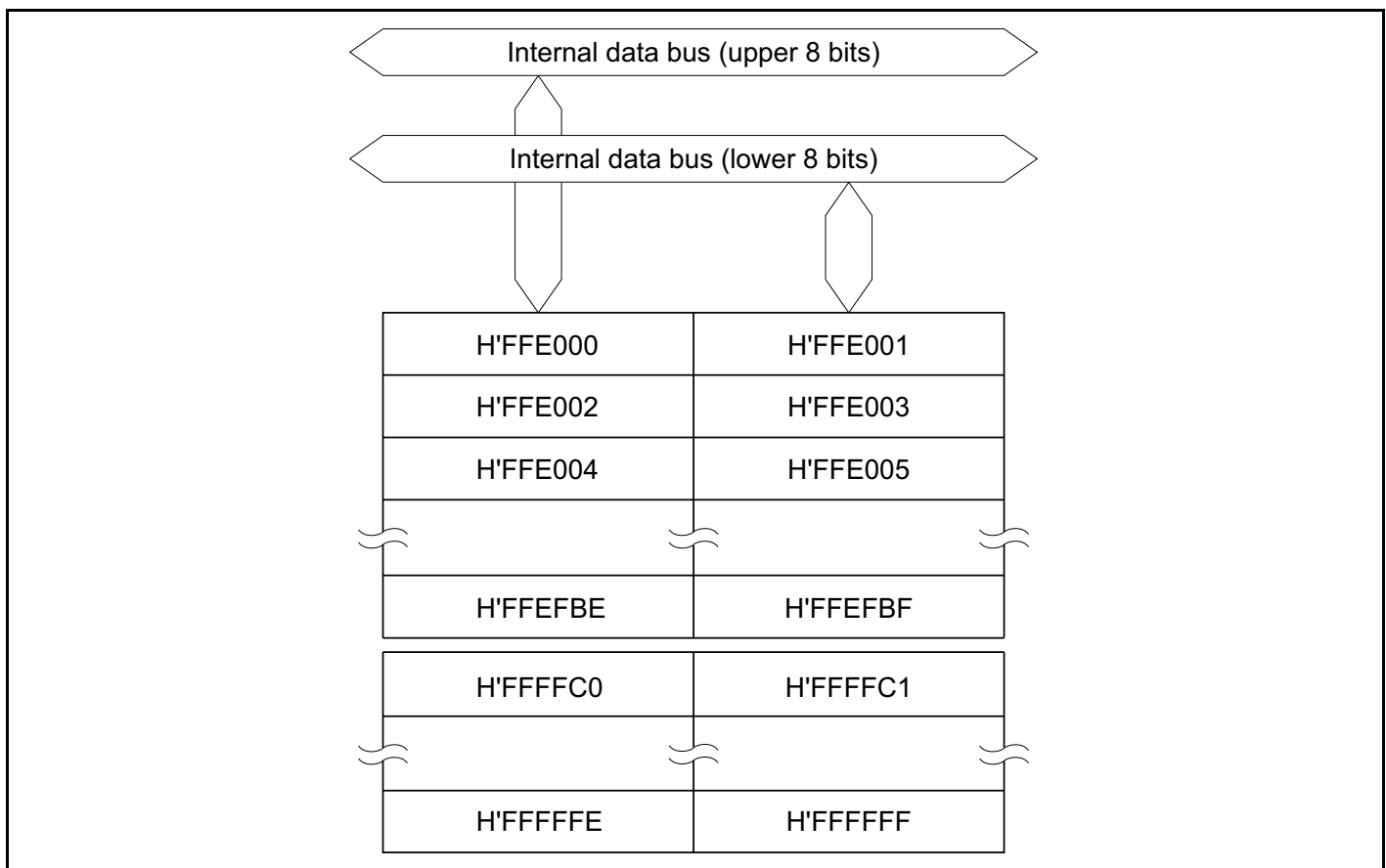
Figure 20-1 (a) Block Diagram of RAM (H8S/2636)
