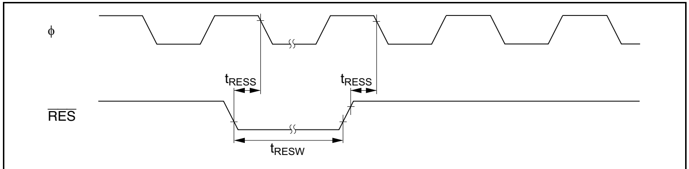
Figure 24-11 Reset Input Timing
