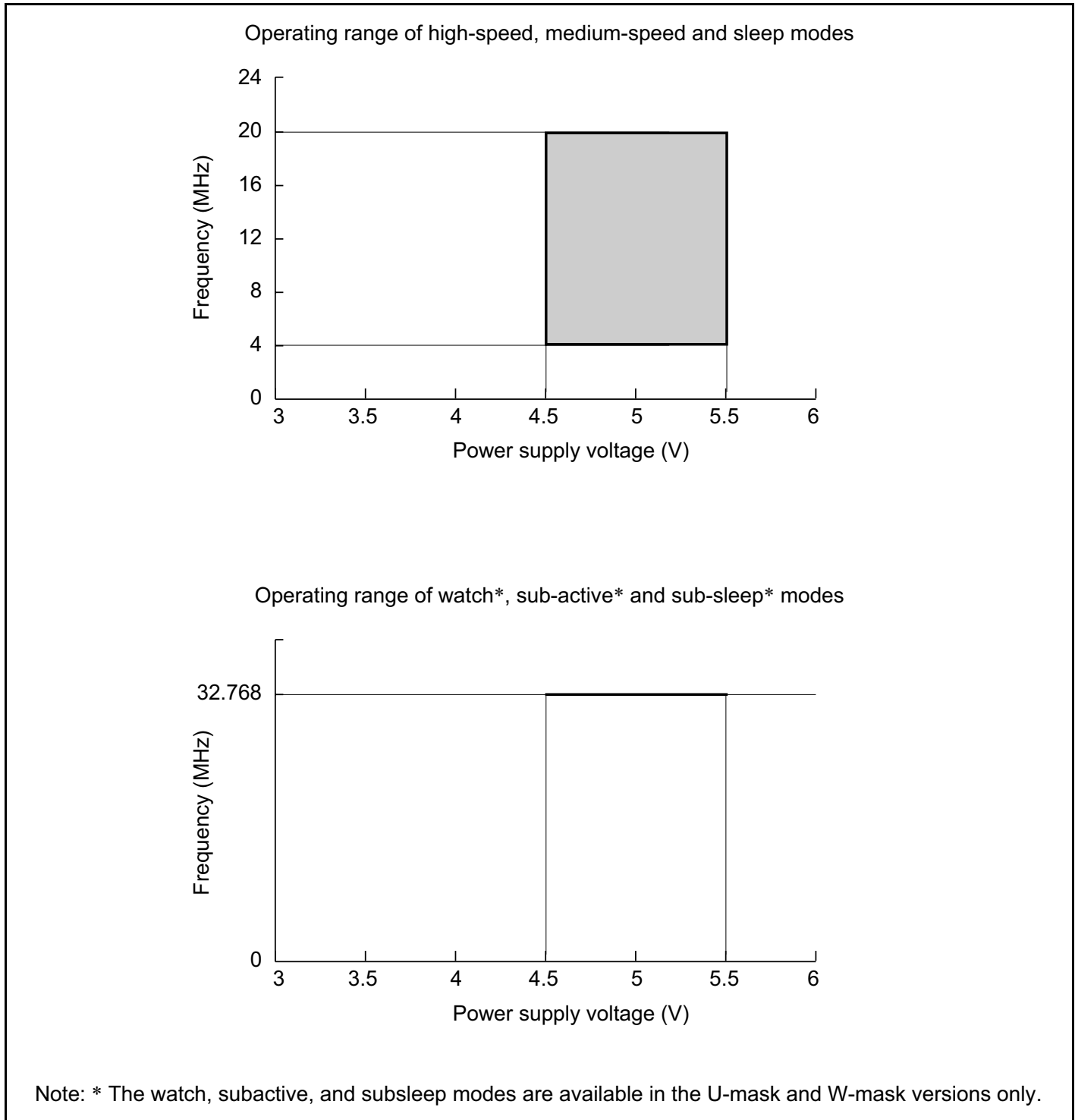
Figure 24-3 Power Supply Voltage and Operating Ranges
