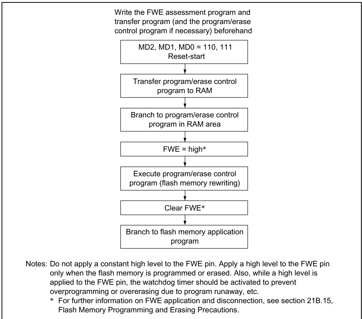
Figure 21B-10 User Program Mode Execution Procedure
