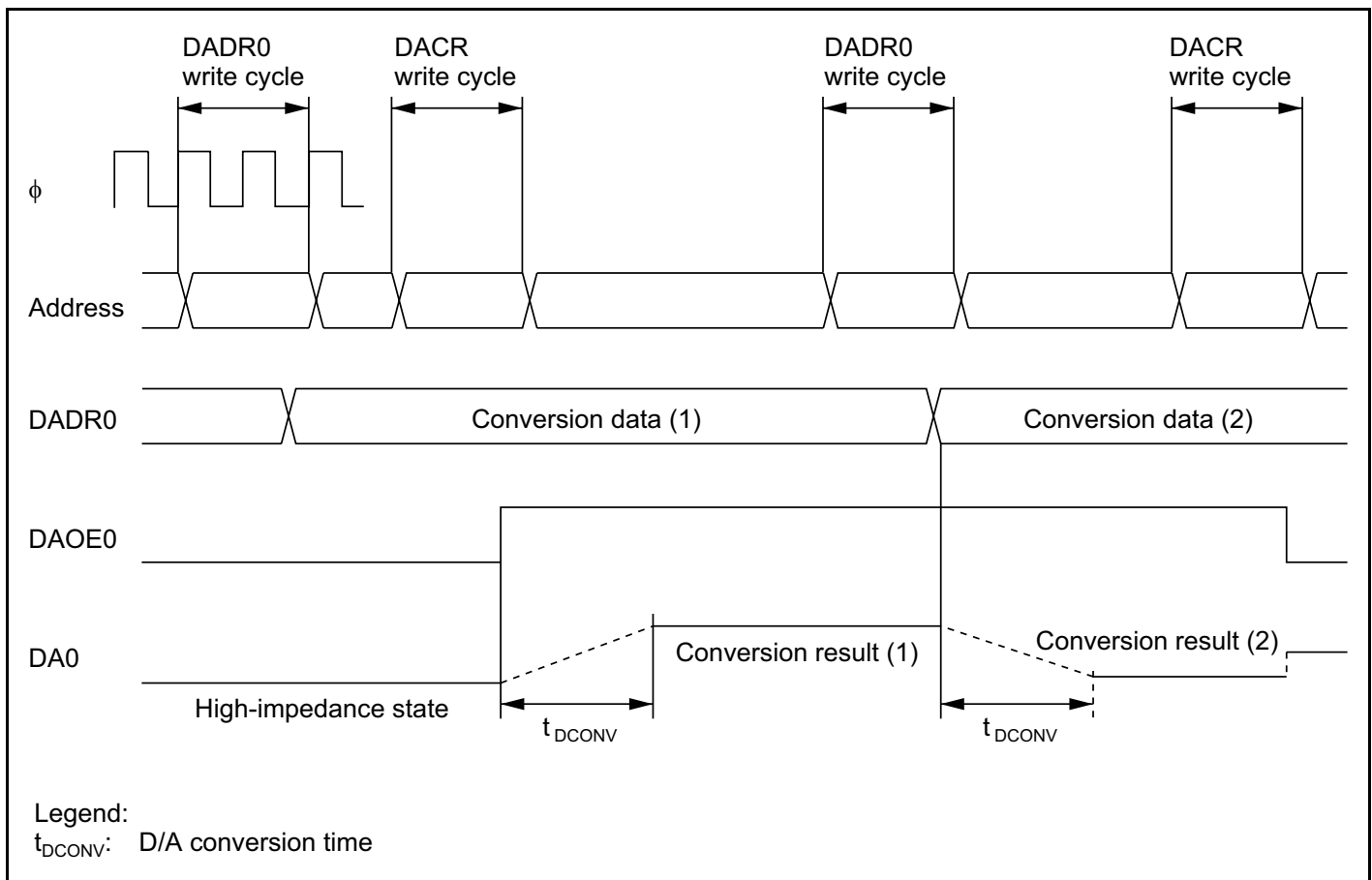
Figure 18-2 D/A Conversion (Example)
