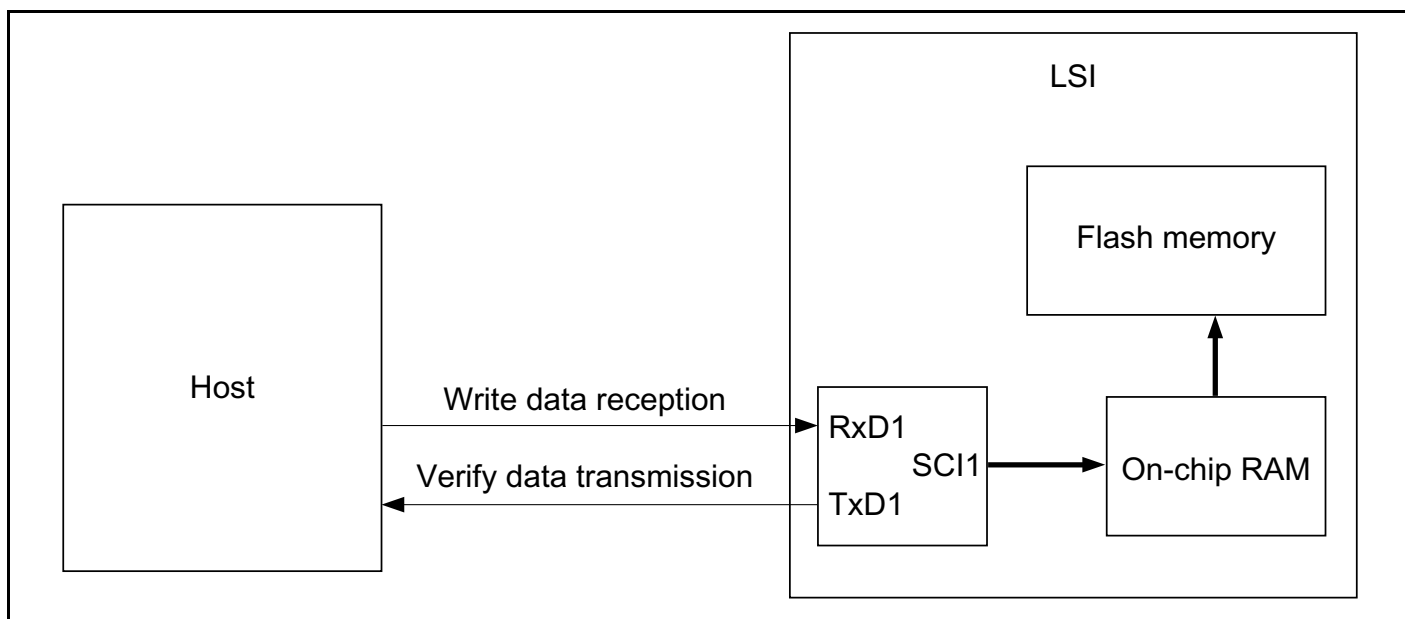
Figure 21B-7 System Configuration in Boot Mode
