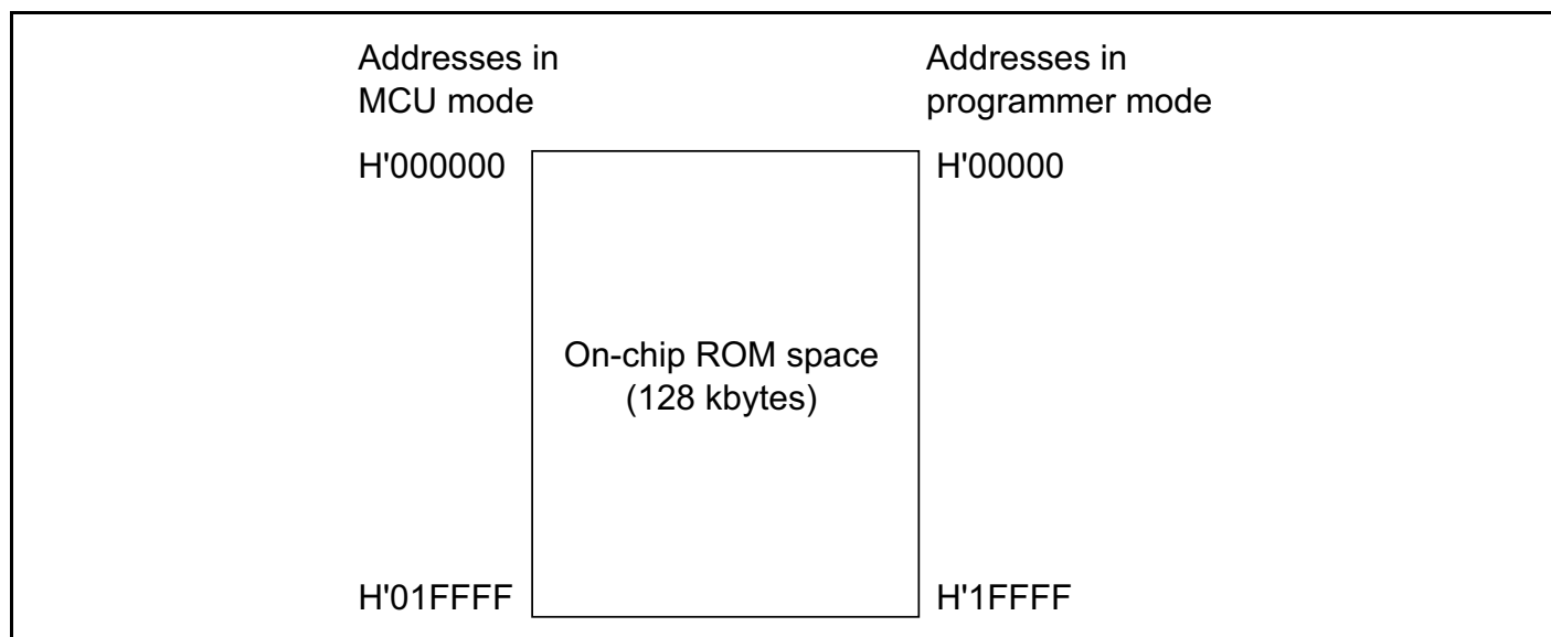
Figure 21A-17 On-Chip ROM Memory Map
