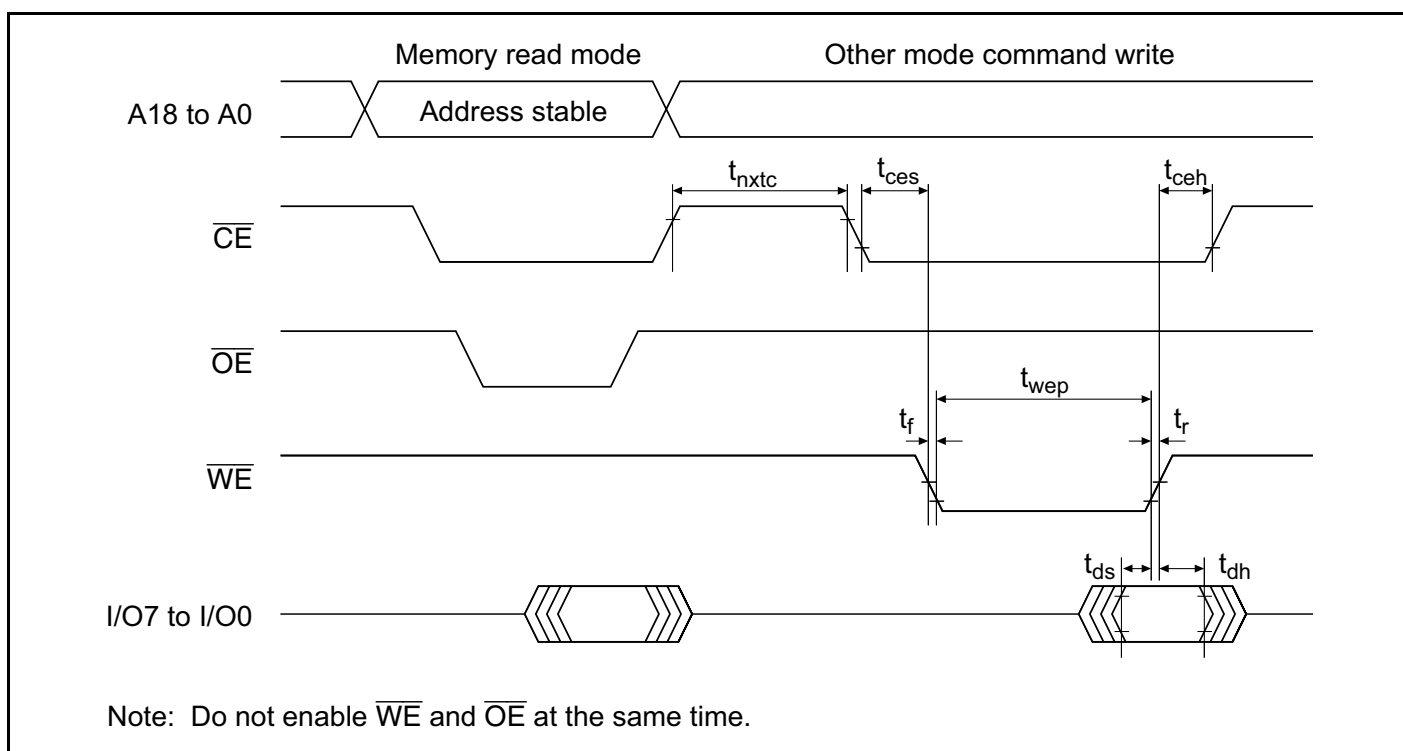
Figure 21C-19 Timing Waveforms in Transition from Memory Read Mode to Another Mode
