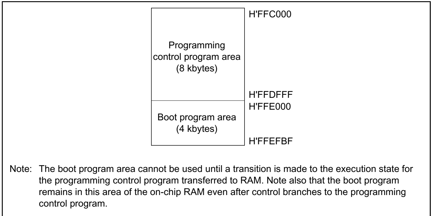
Figure 21B-9 RAM Areas in Boot Mode
