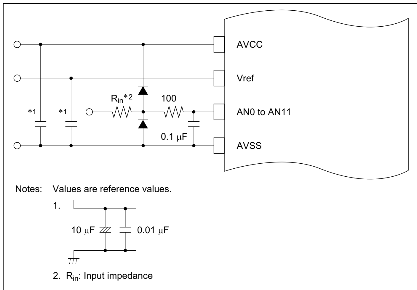
Figure 17-7 Example of Analog Input Protection Circuit
