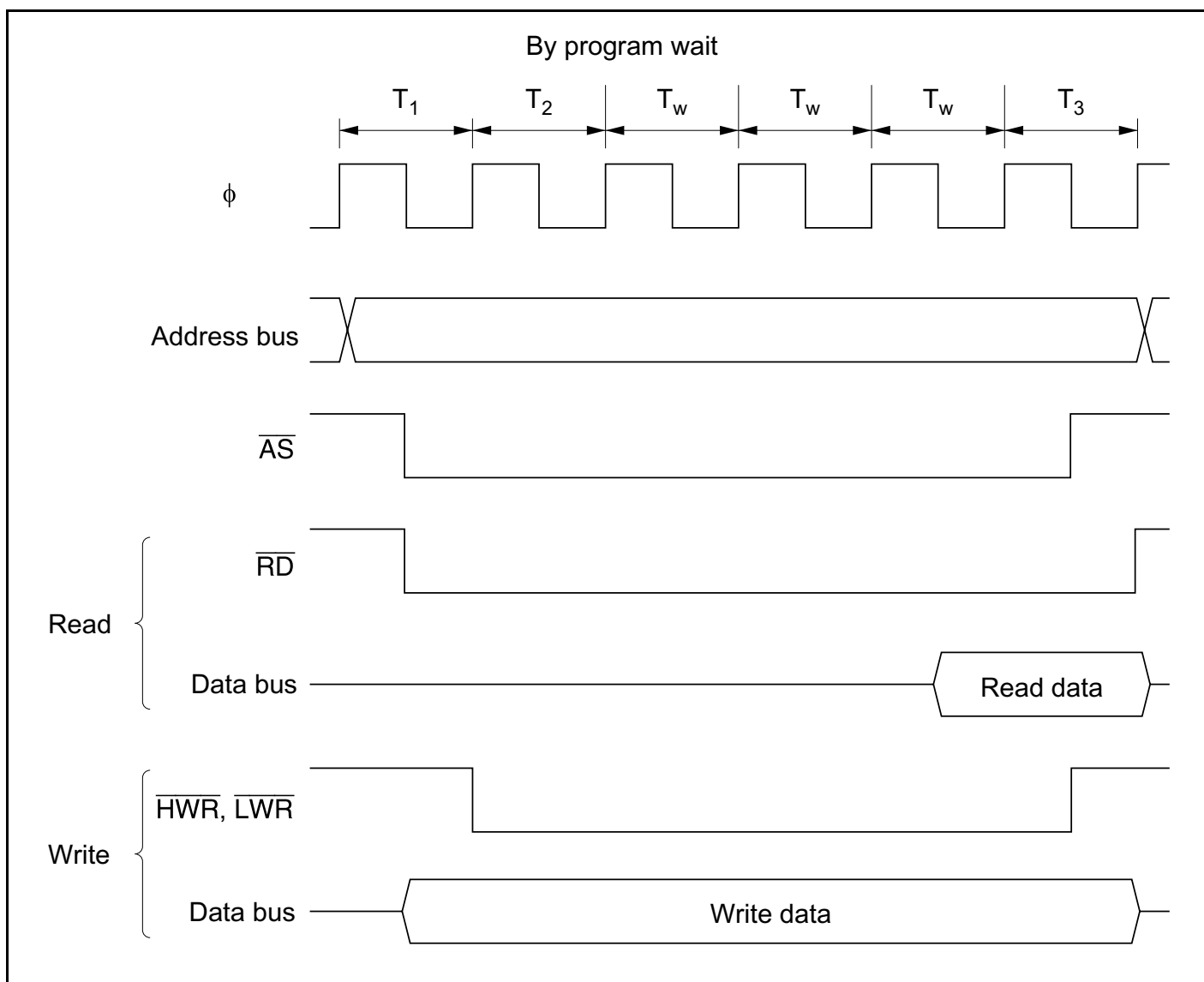
Figure 7-13 Example of Wait State Insertion Timing
