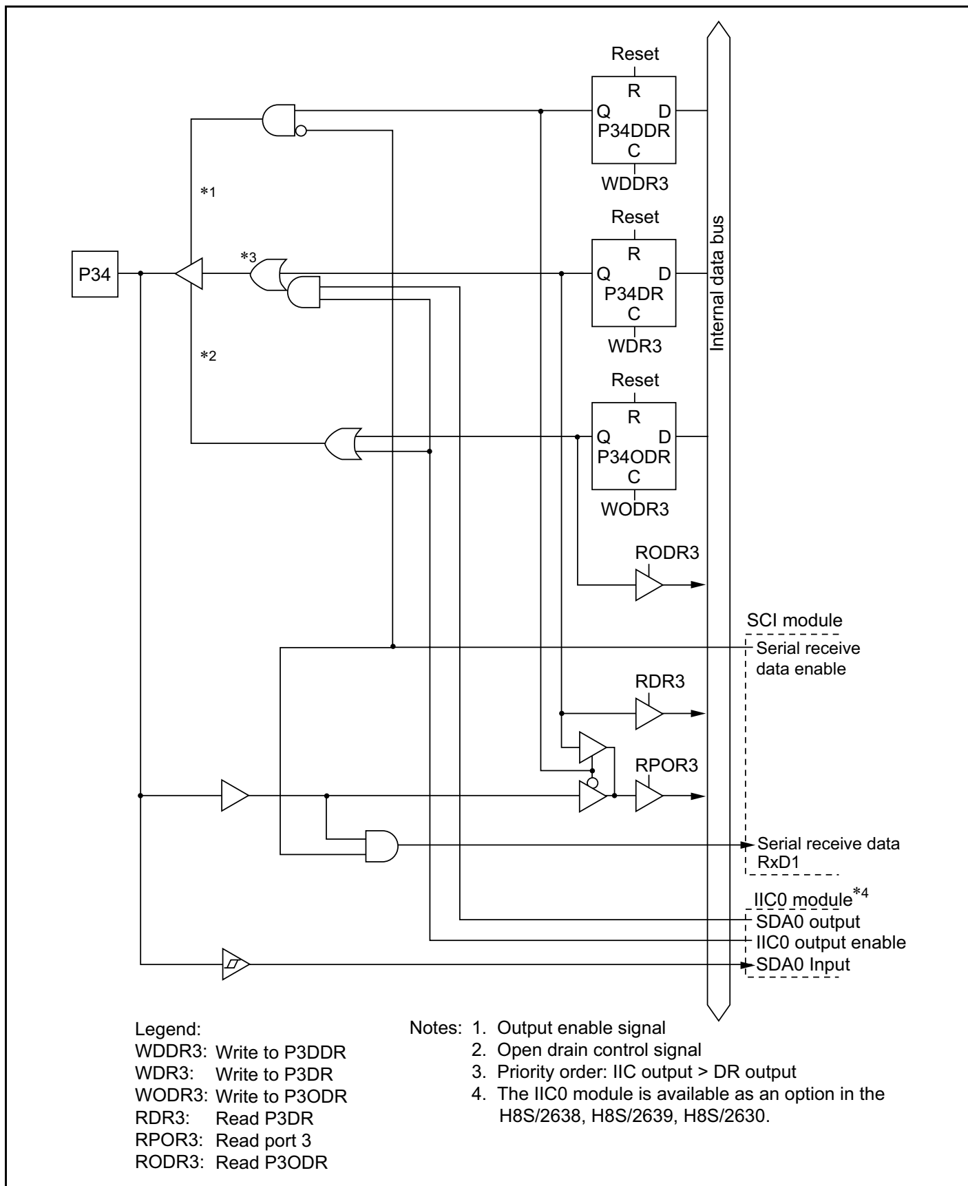
Figure C-2 (e) Port 3 Block Diagram (Pin P34)
