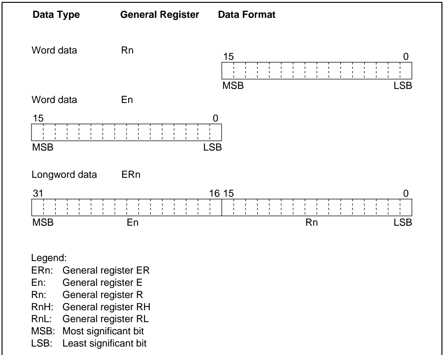
Figure 2.10 General Register Data Formats (cont)
