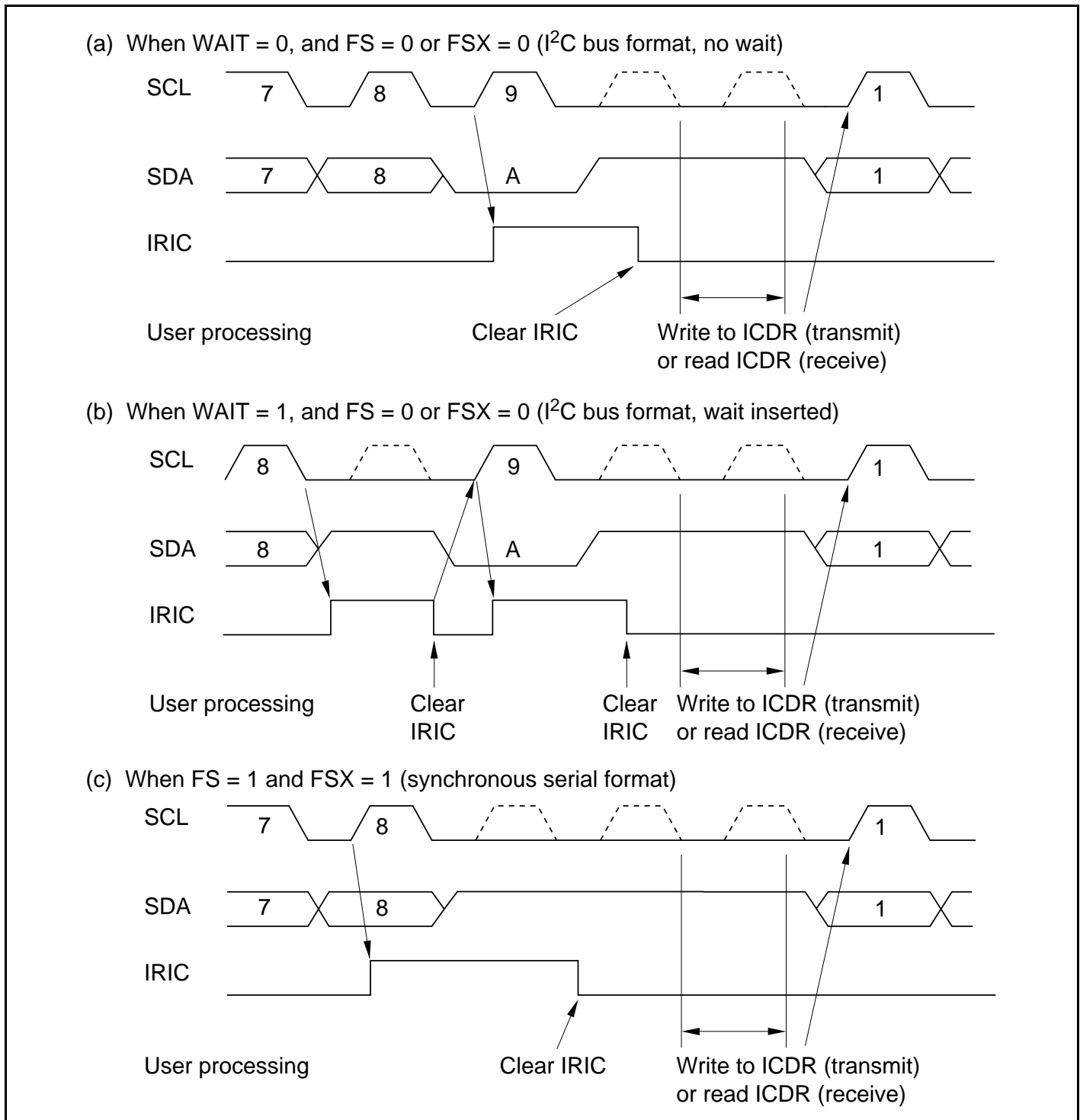
Figure 16.12 IRIC Setting Timing and SCL Control
