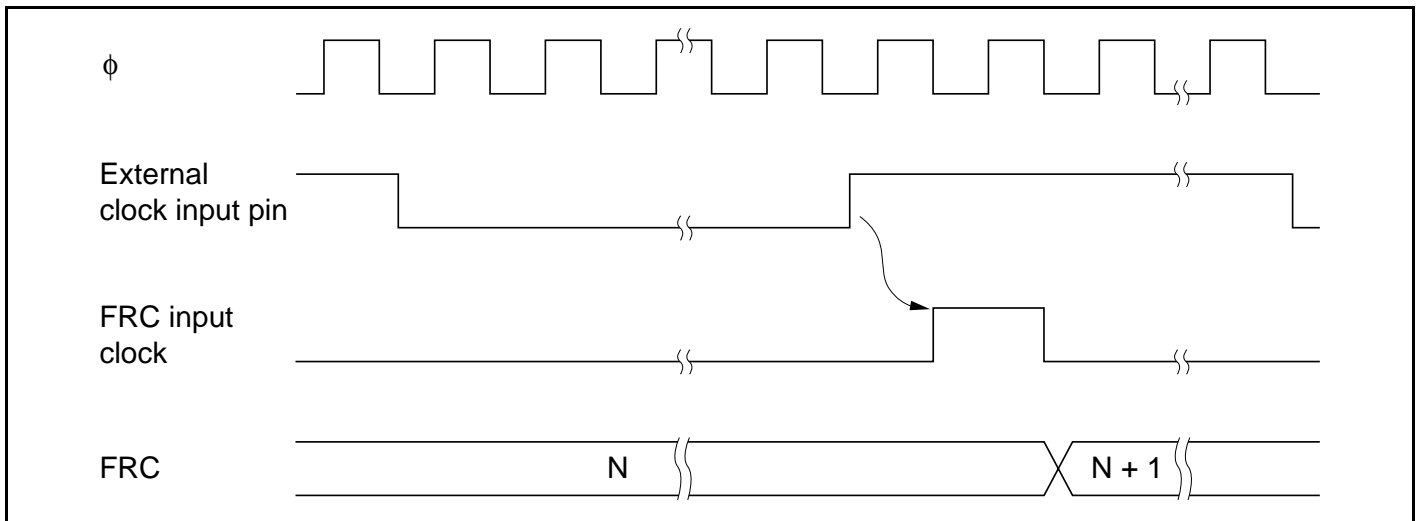
Figure 11.4 Increment Timing with External Clock Source
