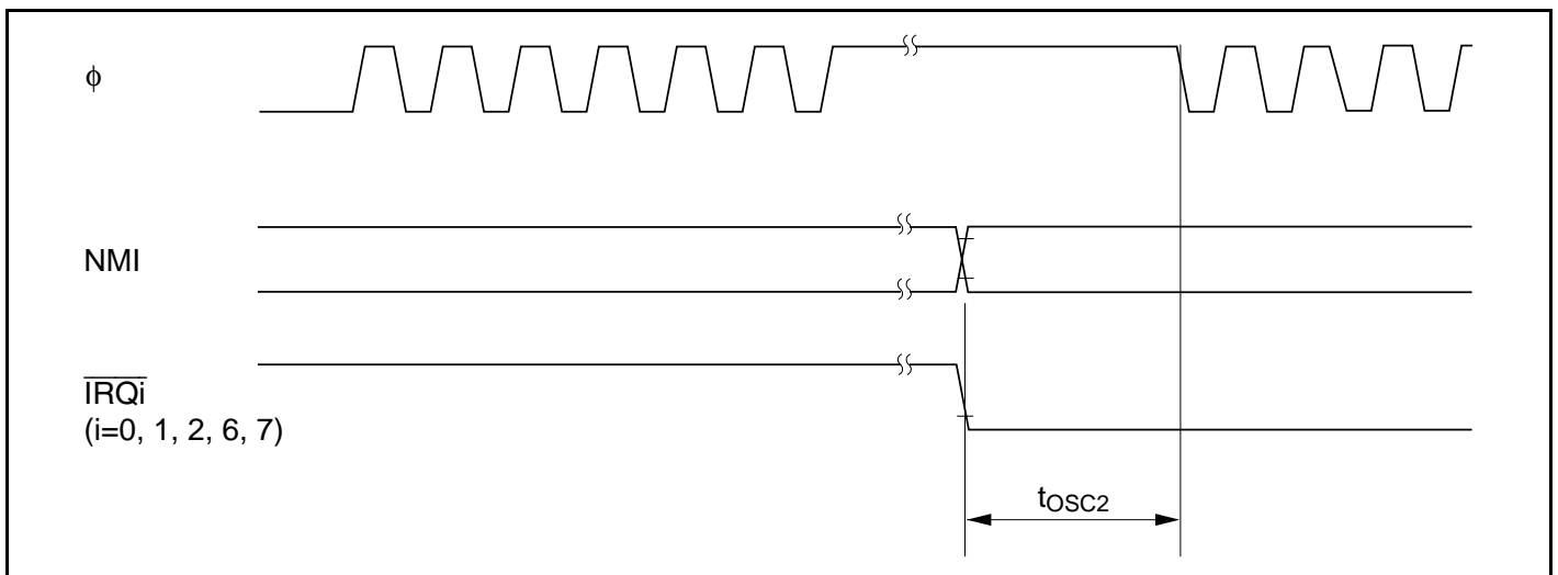
Figure 25.7 Oscillation Settling Timing (Exiting Software Standby Mode)
