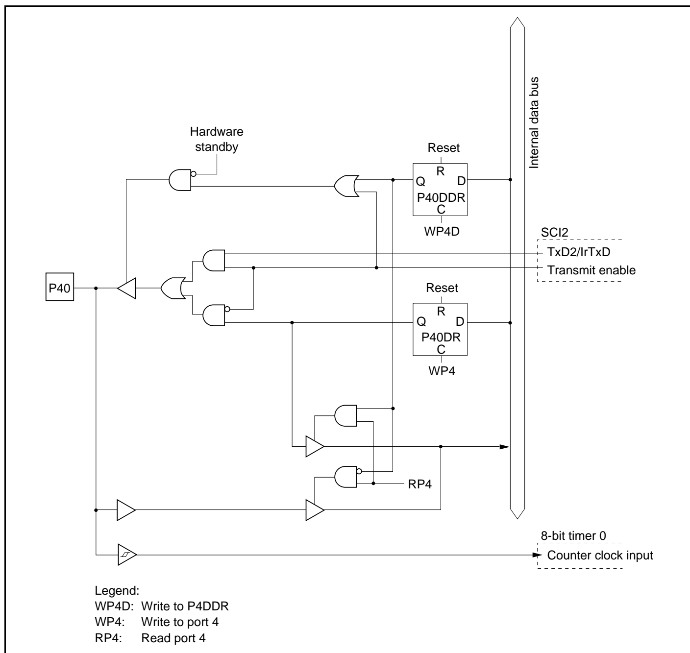
Figure C.6 Port 4 Block Diagram (Pin P40)
