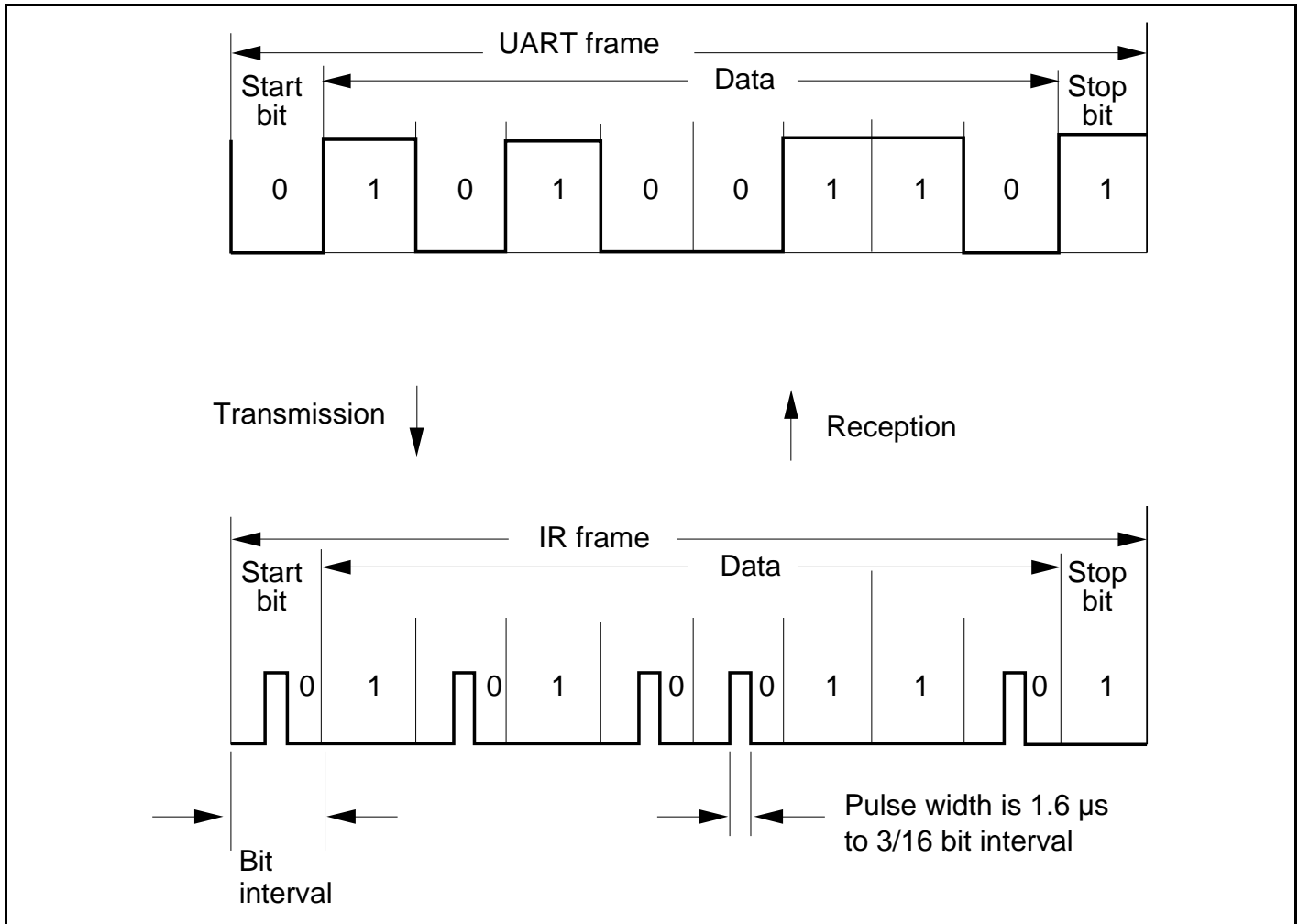
Figure 15.22 IrDA Transmit/Receive Operations
