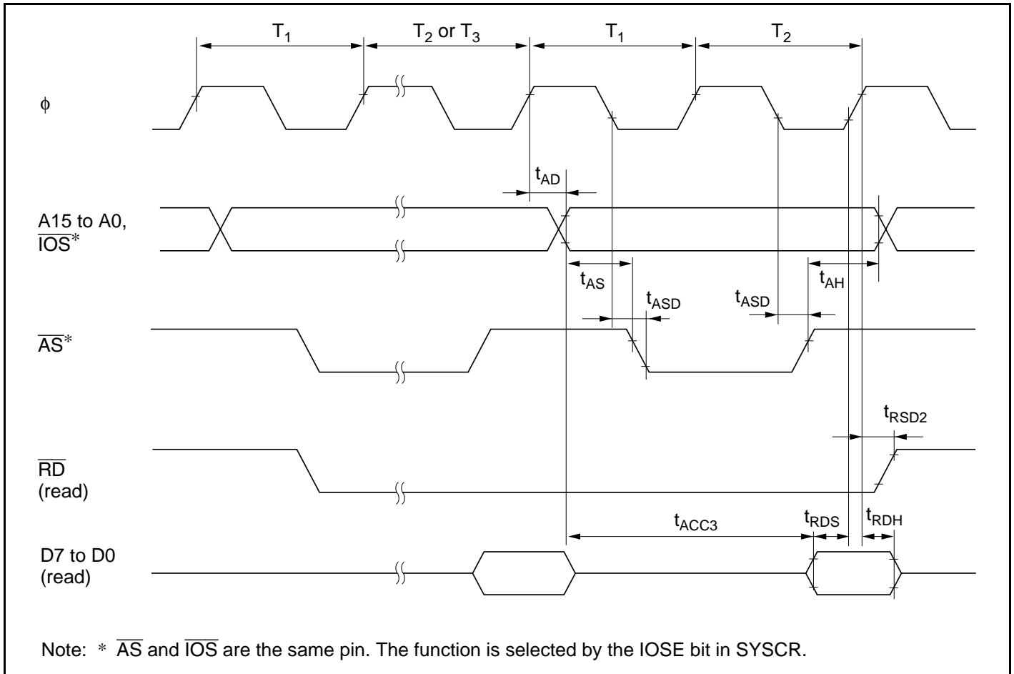
Figure 25.13 Burst ROM Access Timing (Two-State Access)
