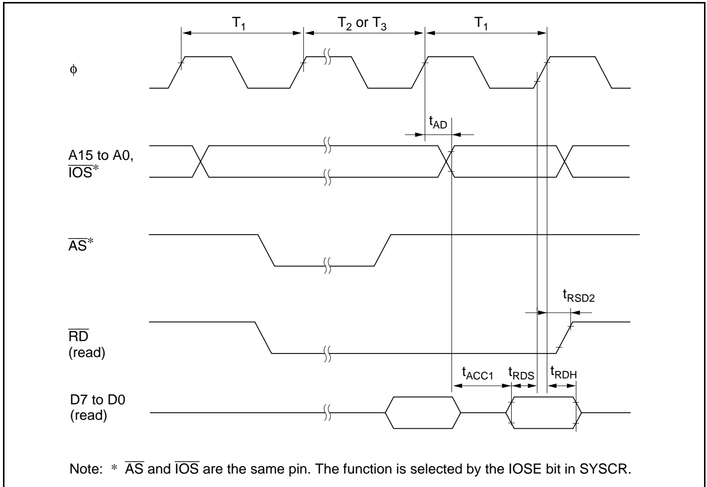
Figure 25.14 Burst ROM Access Timing (One-State Access)
