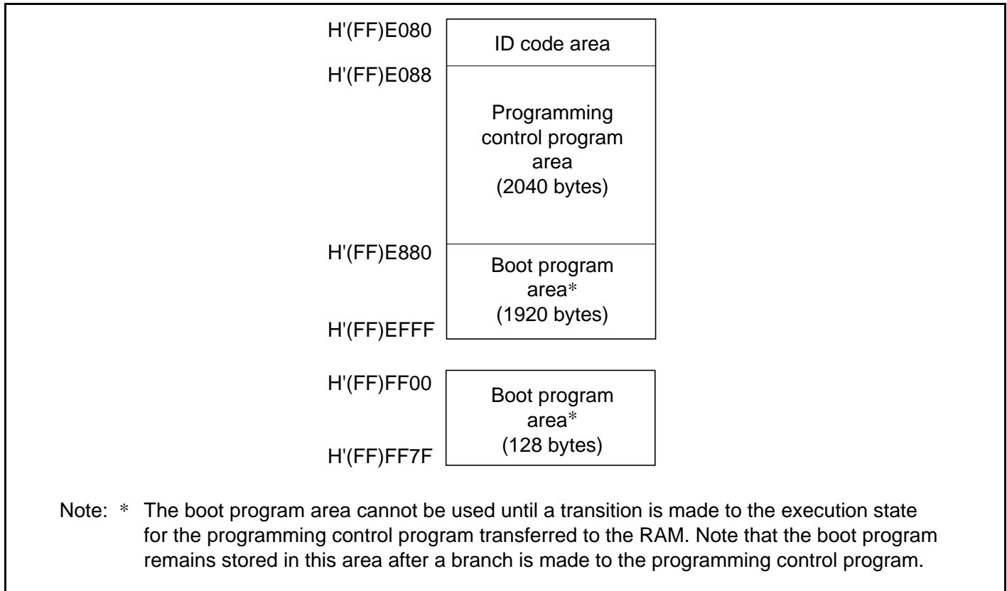
Figure 22.10 RAM Areas in Boot Mode
