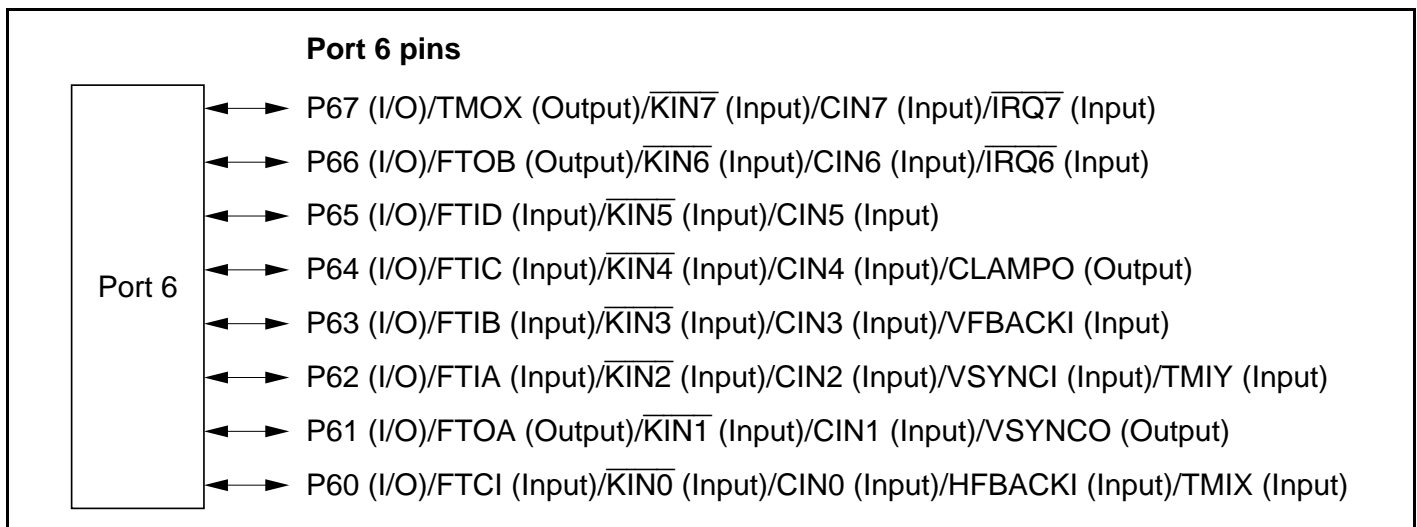
Figure 8.14 Port 6 Pin Functions
