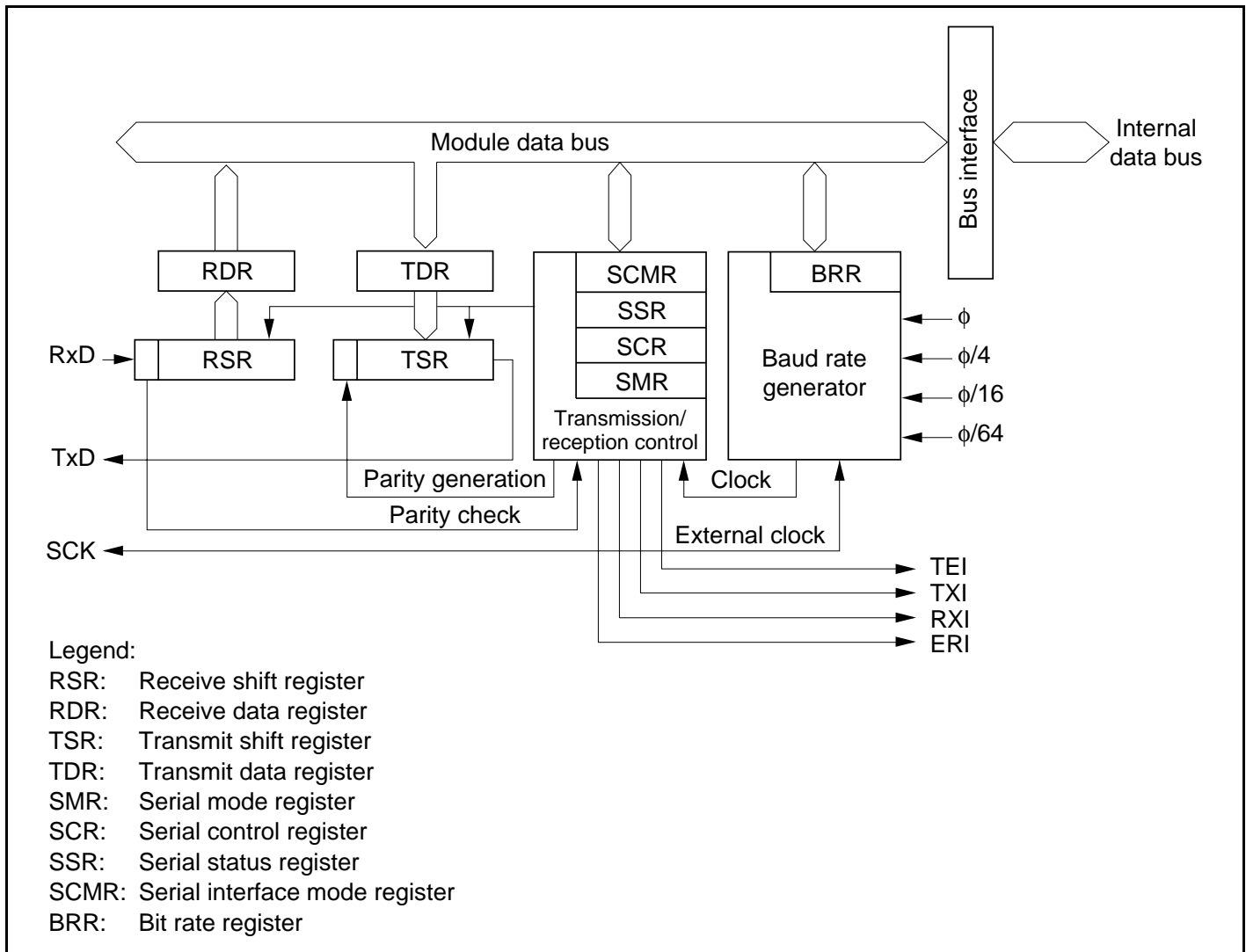
Figure 15.1 Block Diagram of SCI
