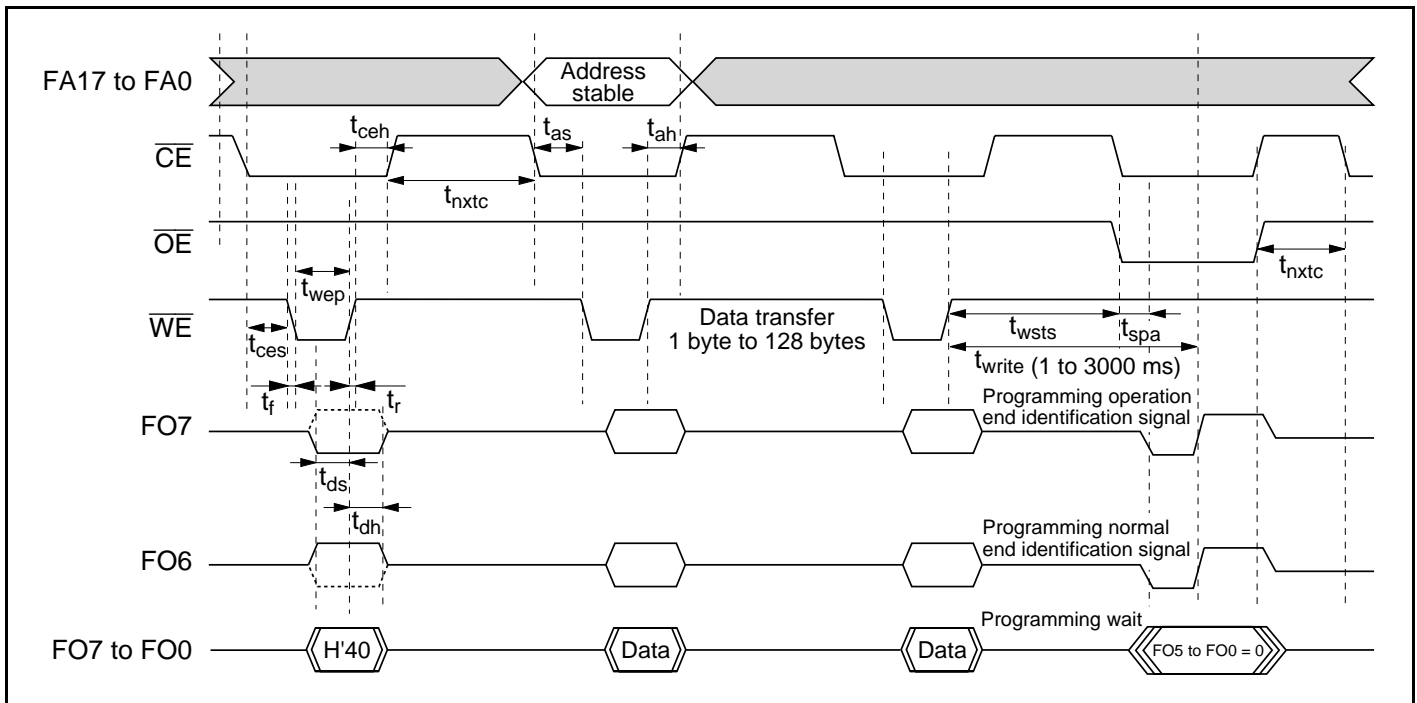
Figure 22.20 Auto-Program Mode Timing Waveforms
