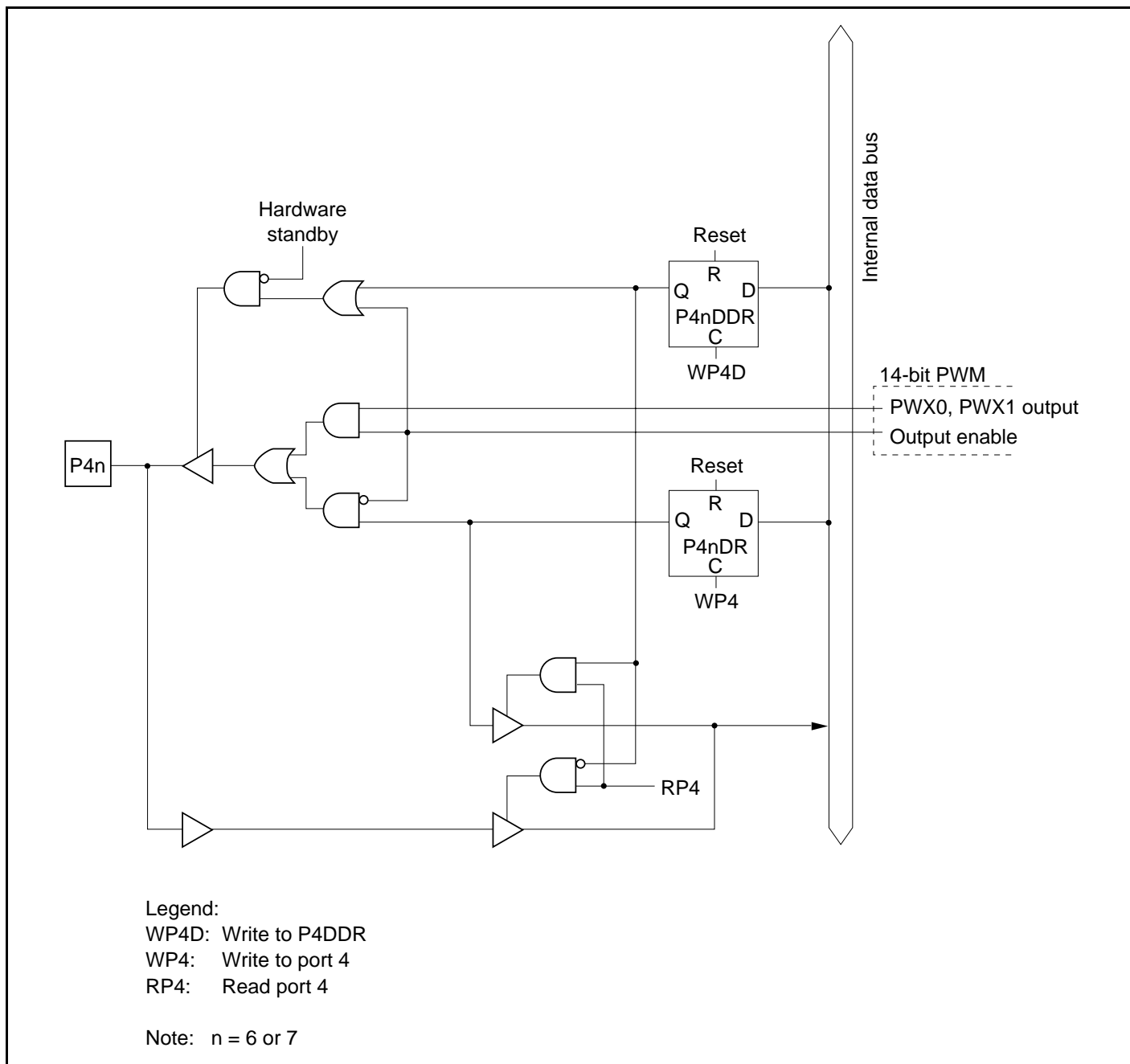
Figure C.12 Port 4 Block Diagram (Pins P46, P47)
