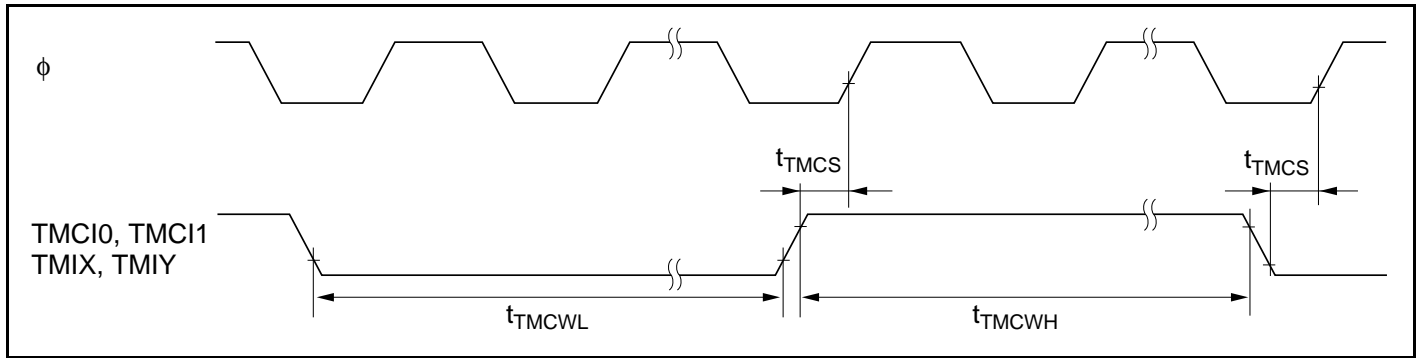
Figure 25.19 8-Bit Timer Clock Input Timing
