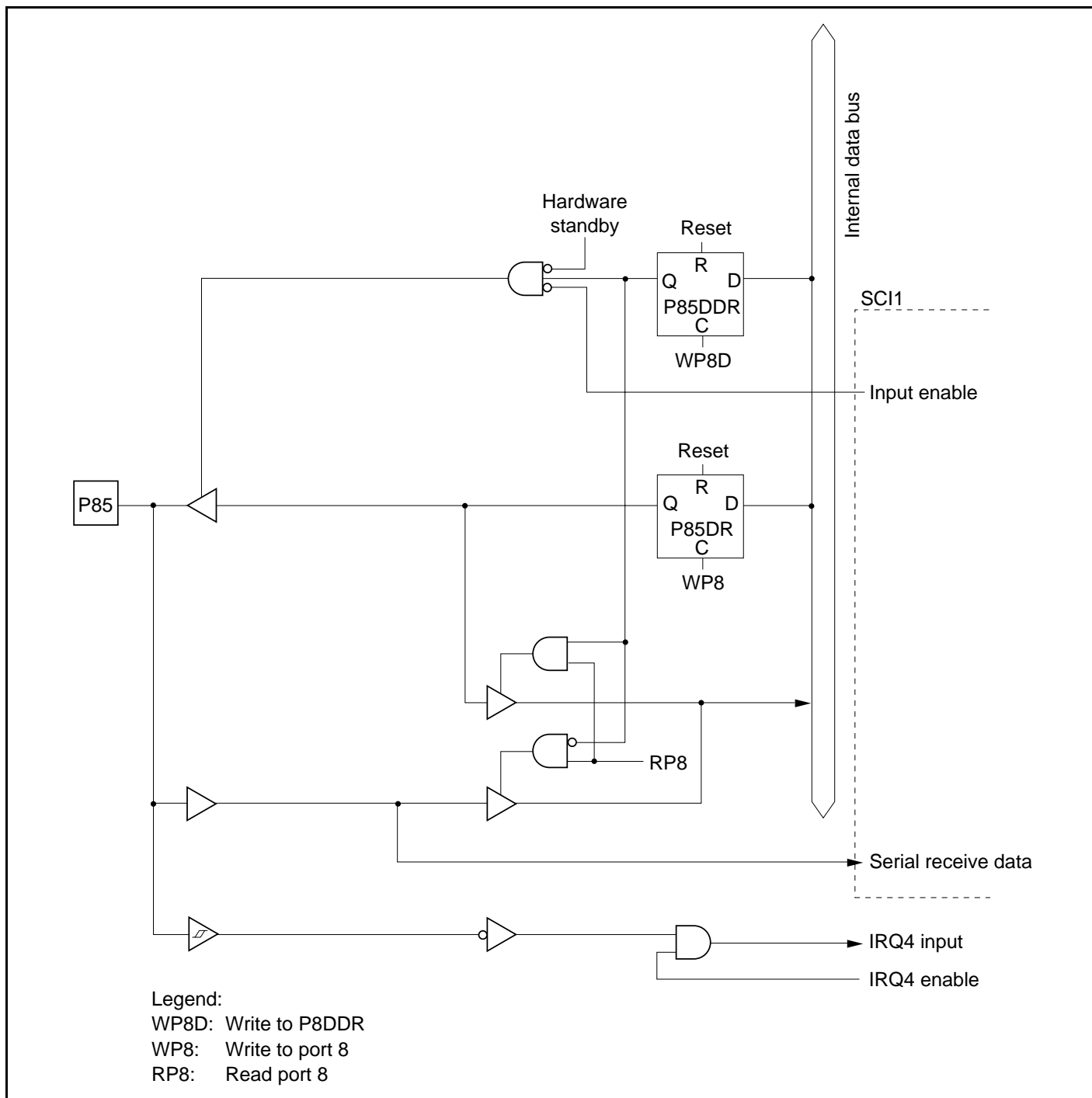
Figure C.27 Port 8 Block Diagram (Pin P85)
