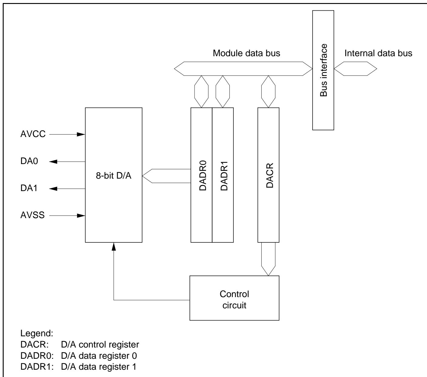
Figure 18.1 Block Diagram of D/A Converter
