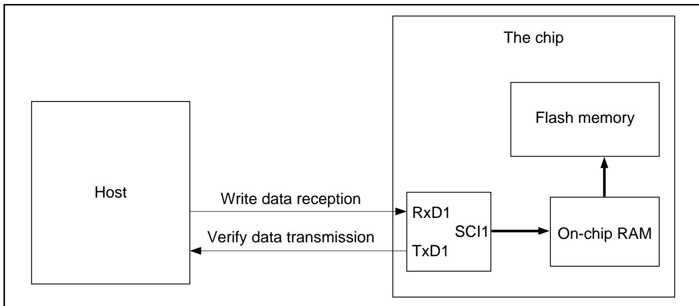
Figure 21.7 System Configuration in Boot Mode
