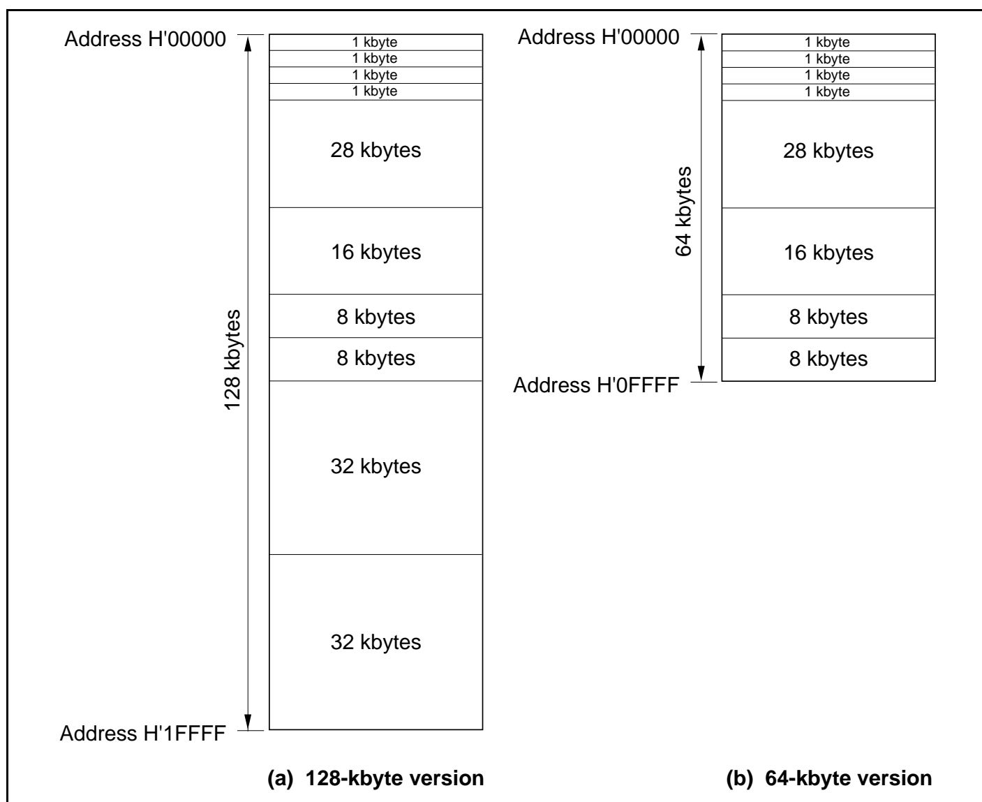
Figure 21.6 Flash Memory Block Configuration
