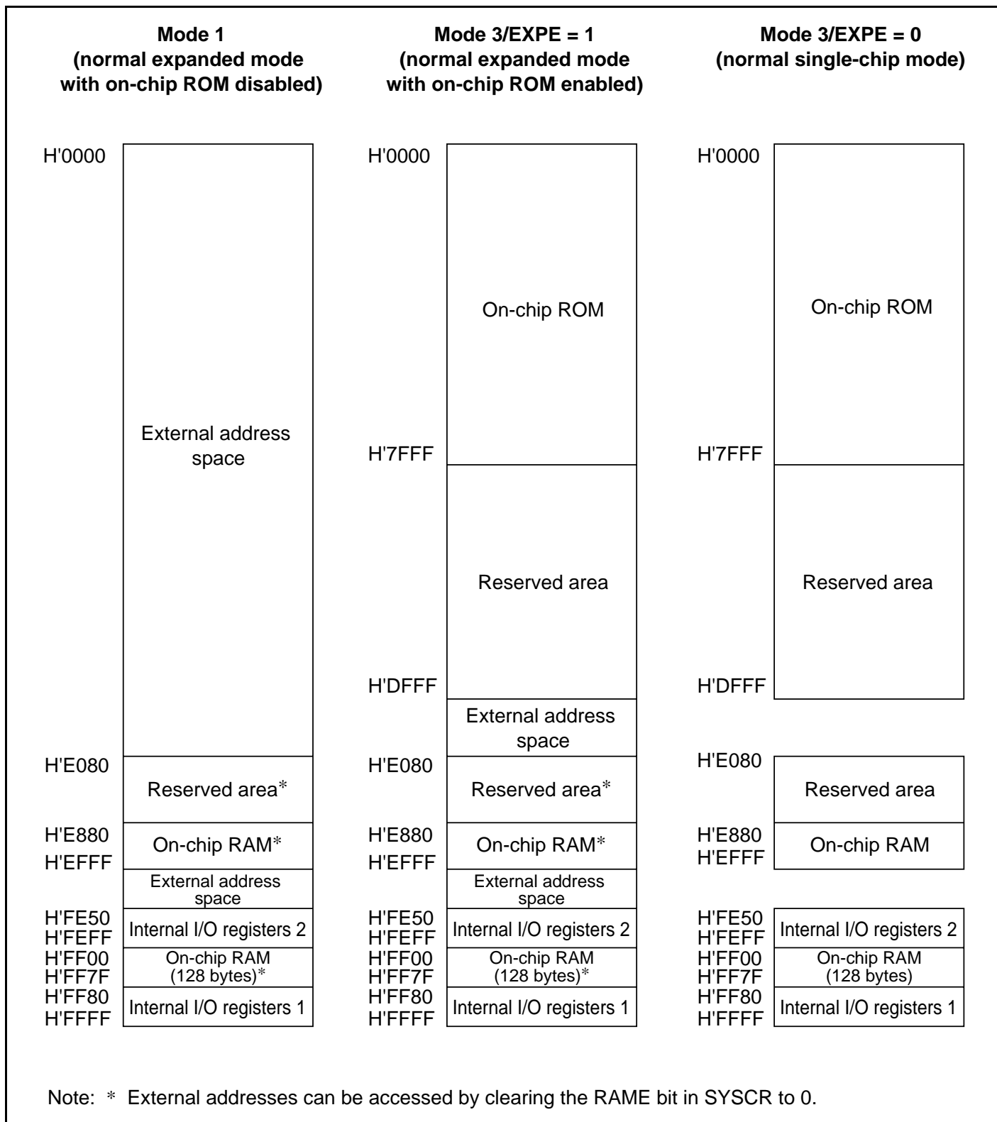
Figure 3.5 H8S/2130 Memory Map in Each Operating Mode
