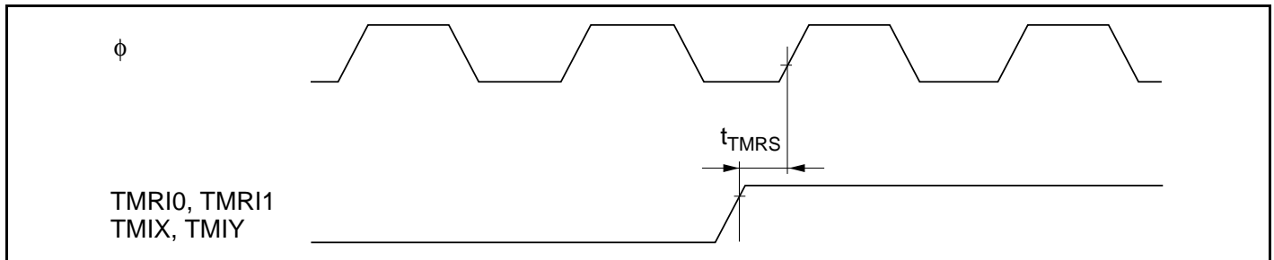
Figure 25.20 8-Bit Timer Reset Input Timing
