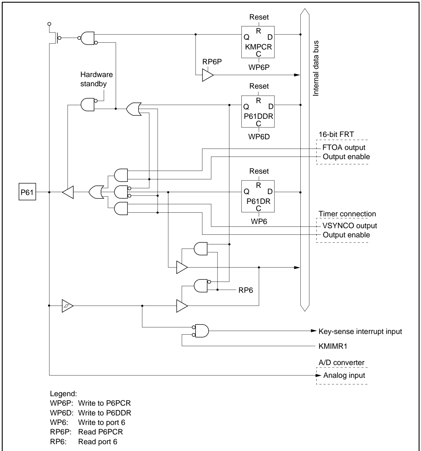
Figure C.17 Port 6 Block Diagram (Pin P61)
