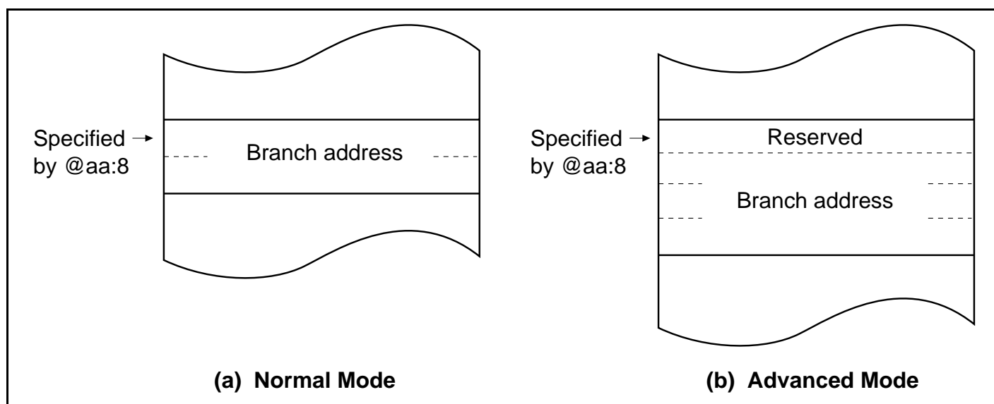
Figure 2.13 Branch Address Specification in Memory Indirect Mode
