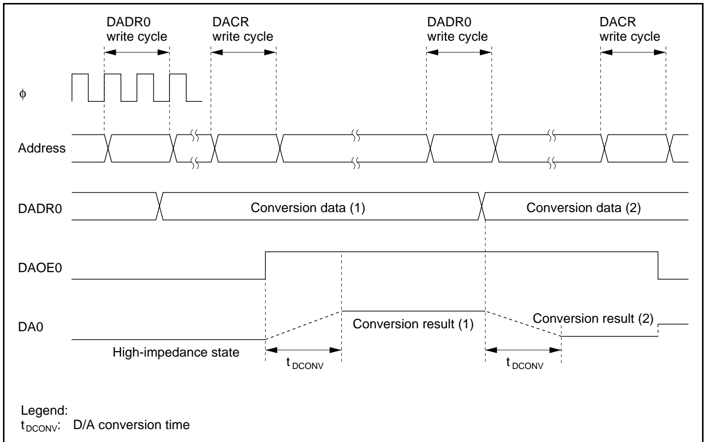
Figure 18.2 D/A Conversion (Example)
