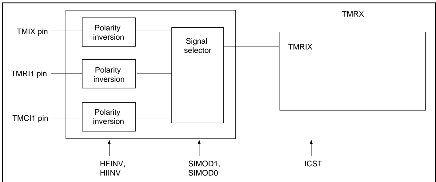
Figure 12.11 Switching of Input Capture Signal
