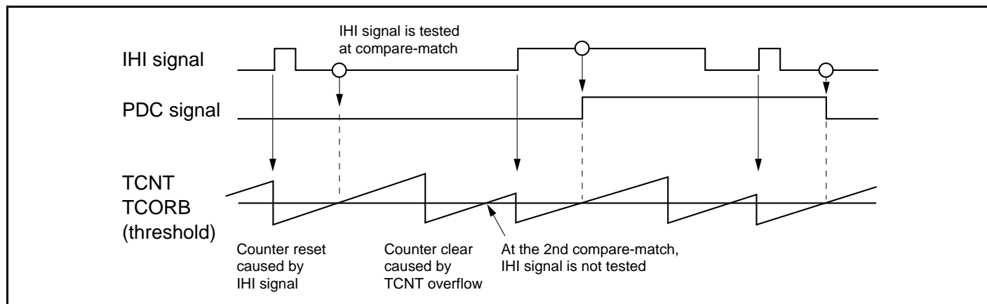
Figure 13.2 Timing Chart for PWM Decoding
