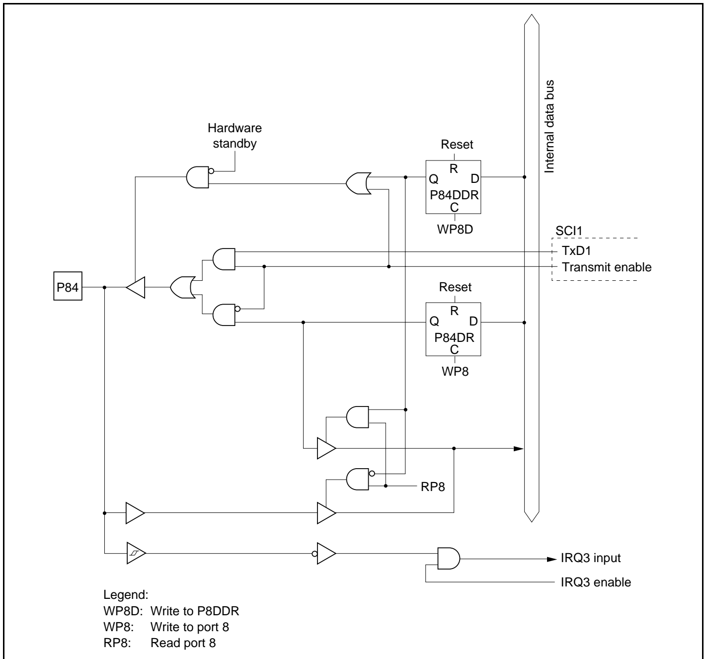
Figure C.26 Port 8 Block Diagram (Pin P84)
