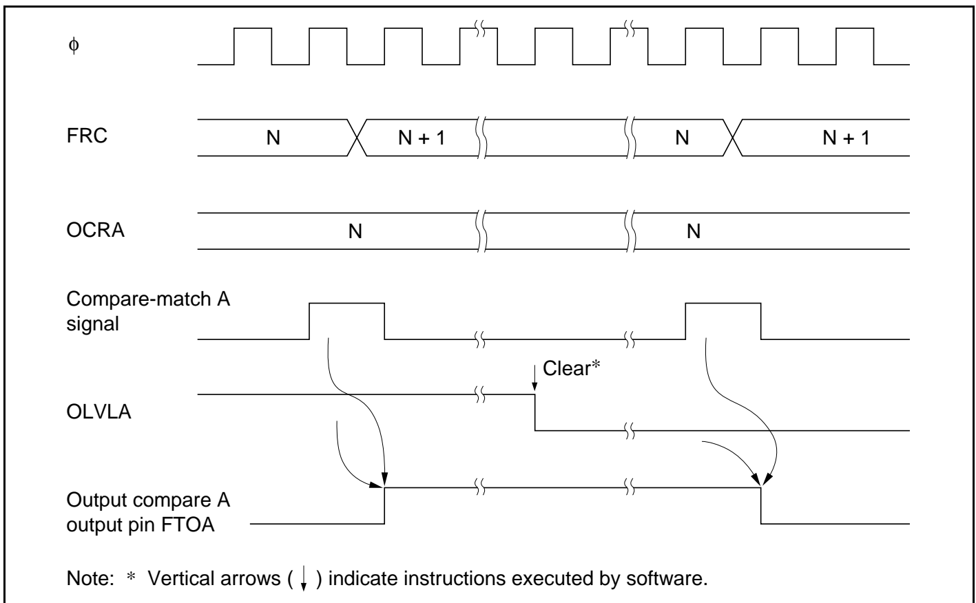
Figure 11.5 Timing of Output Compare A Output
