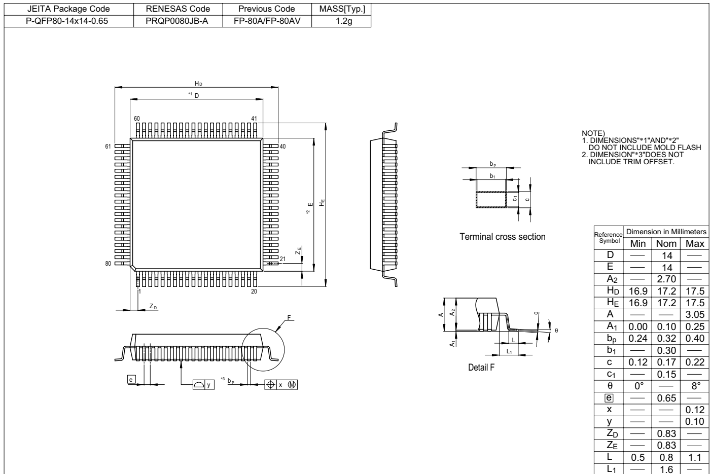
Figure G.1 Package Dimensions (FP-80A)
