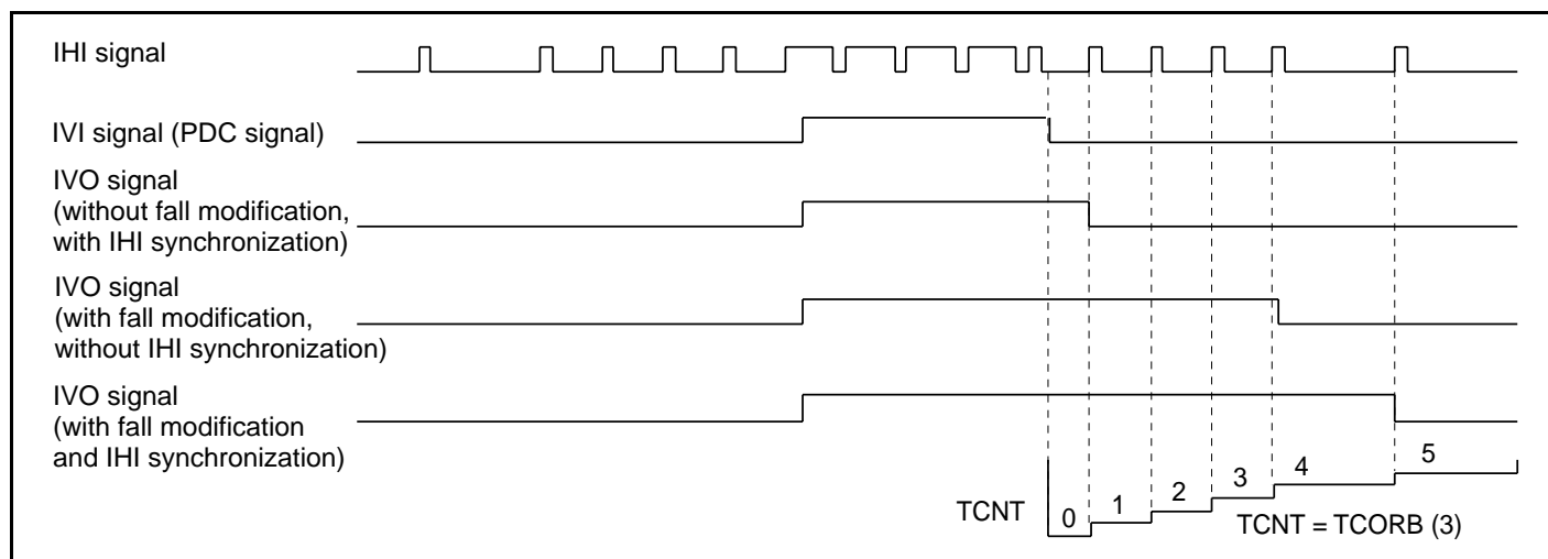
Figure 13.7 Fall Modification/IHI Synchronization Timing Chart
