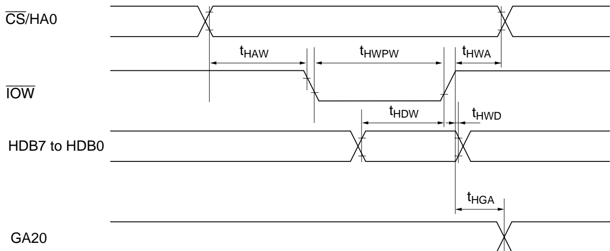
Figure 25.25 Host Interface Timing
