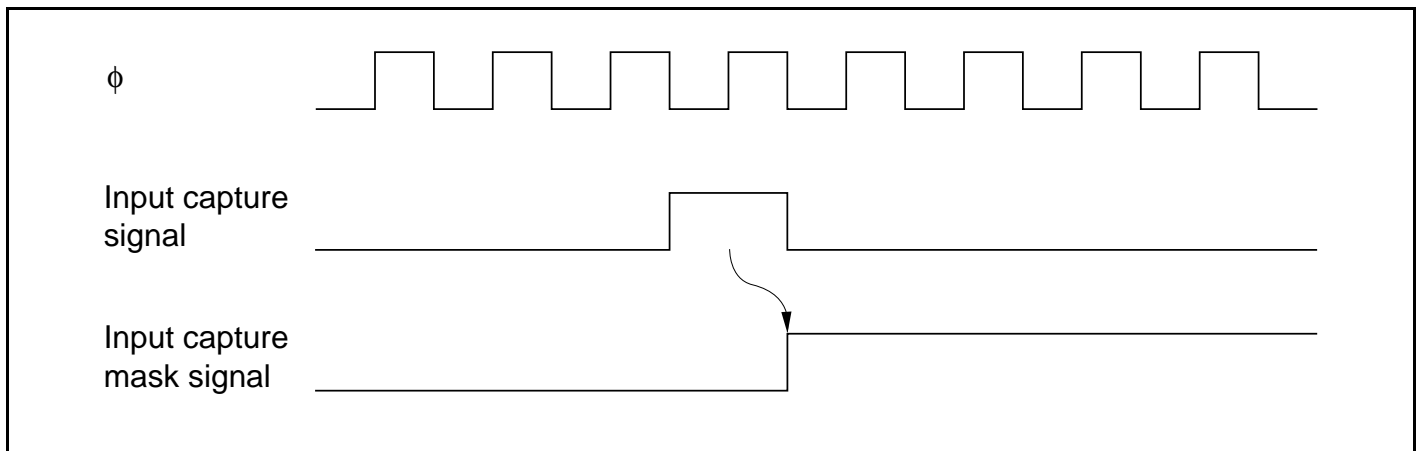
Figure 11.15 Input Capture Mask Signal Setting Timing
