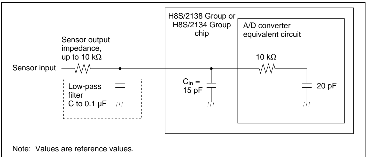
Figure 19.11 Example of Analog Input Circuit
