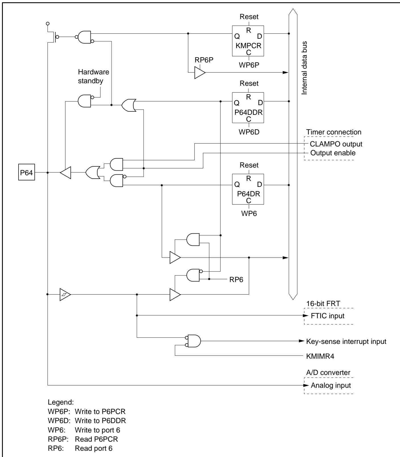
Figure C.18 Port 6 Block Diagram (Pin P64)
