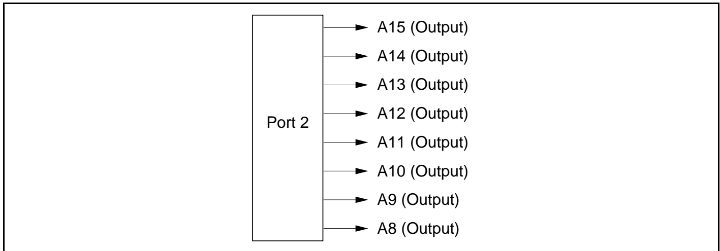
Figure 8.6 Port 2 Pin Functions (Mode 1)
