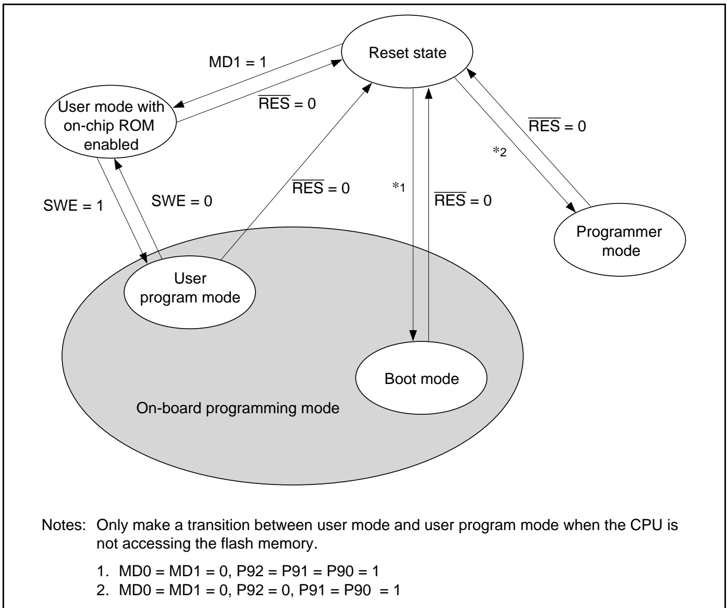
Figure 22.3 Flash Memory Mode Transitions
