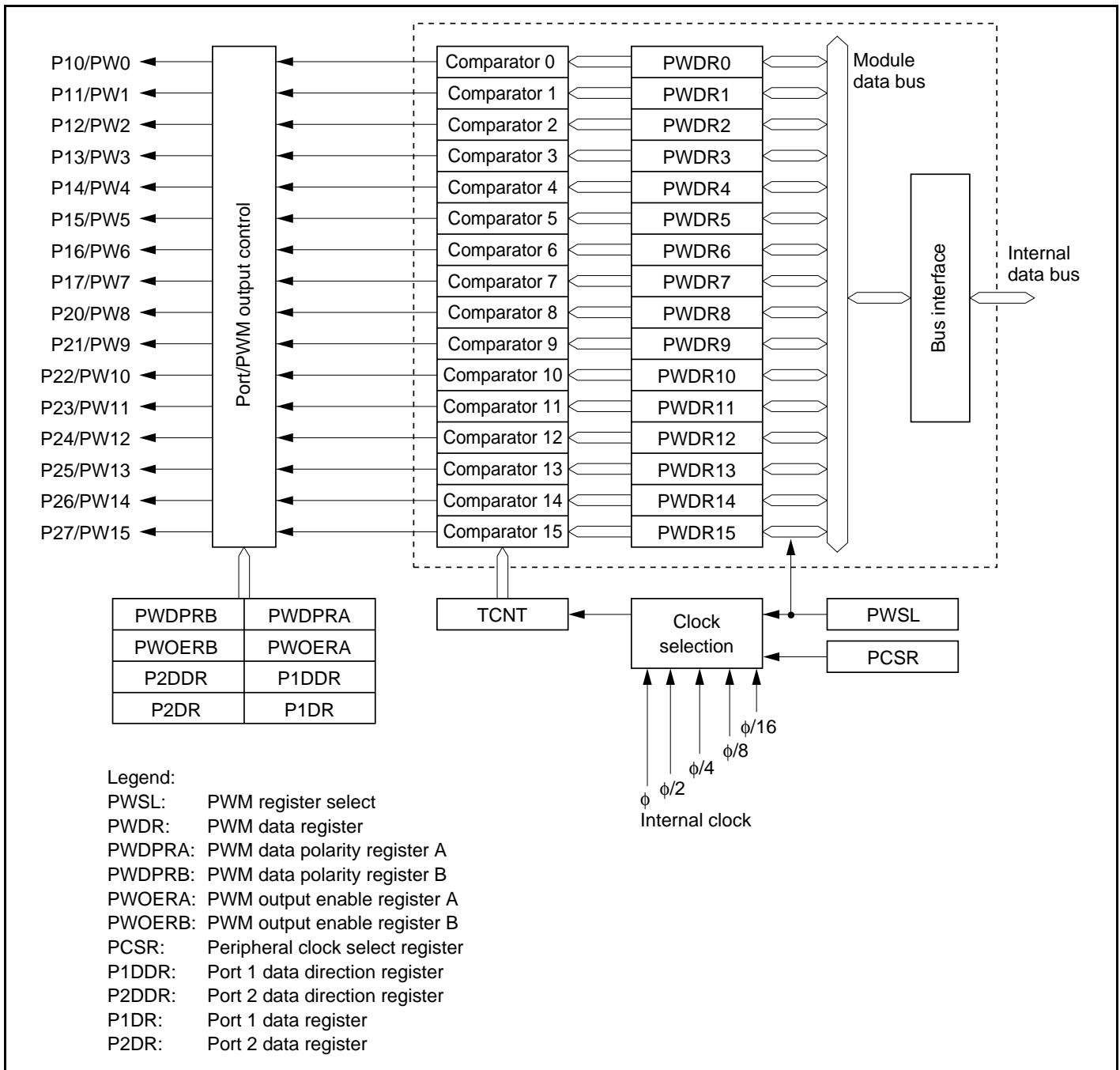
Figure 9.1 Block Diagram of PWM Timer Module
