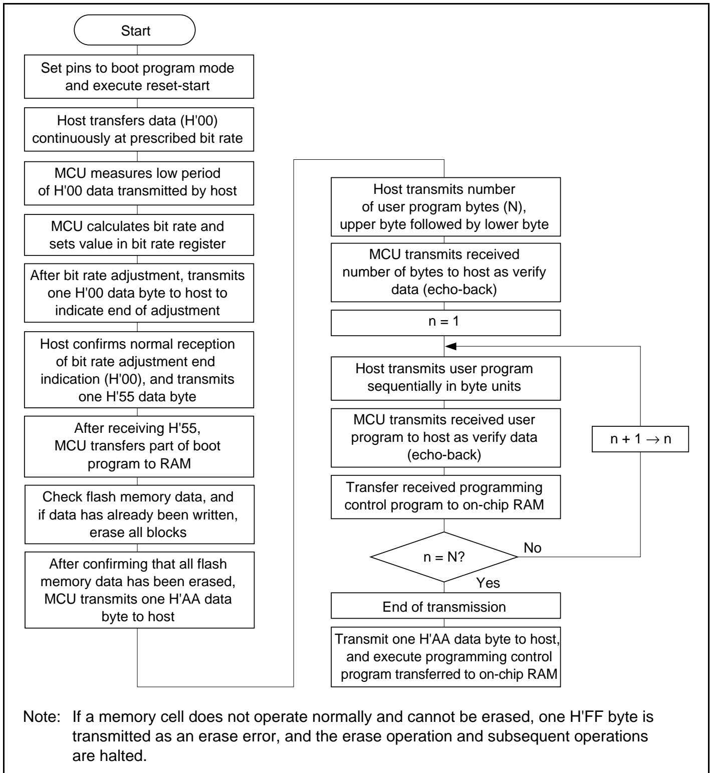
Figure 21.8 Boot Mode Execution Procedure
