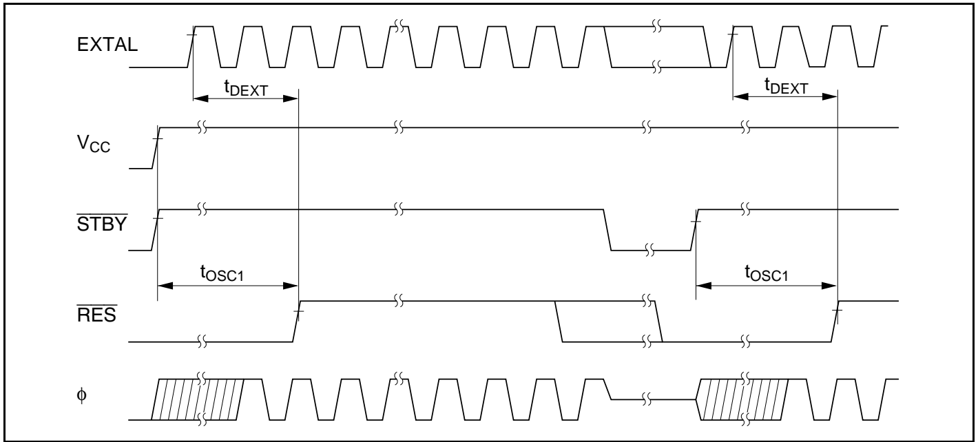
Figure 25.6 Oscillation Settling Timing
