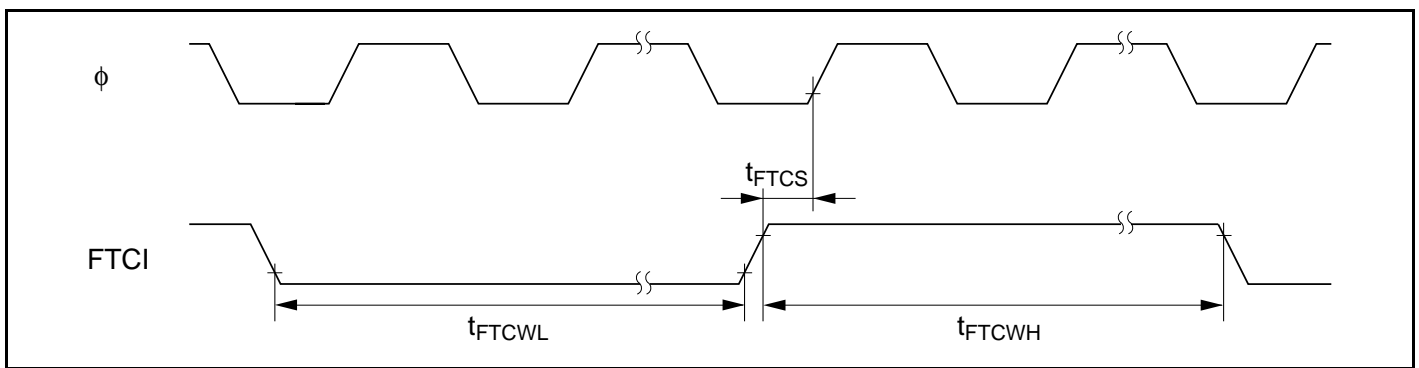
Figure 25.17 FRT Clock Input Timing
