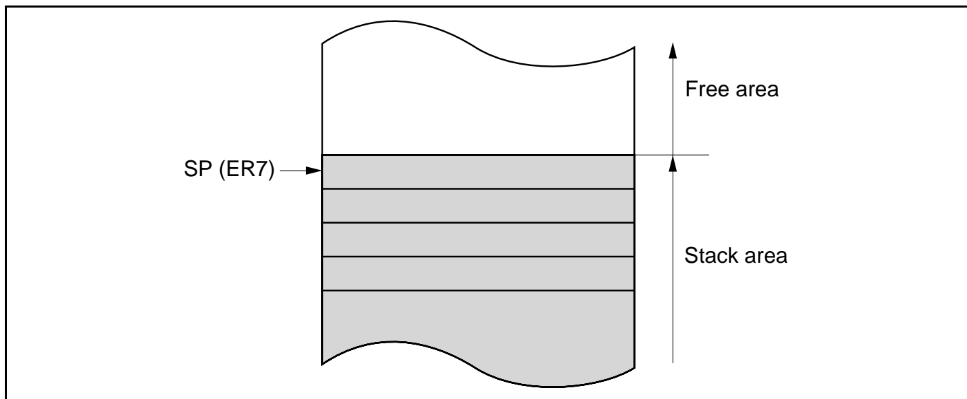
Figure 2.9 Stack
