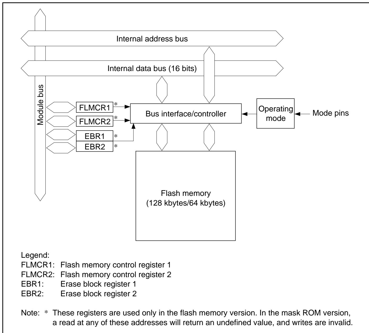
Figure 21.2 Block Diagram of Flash Memory
