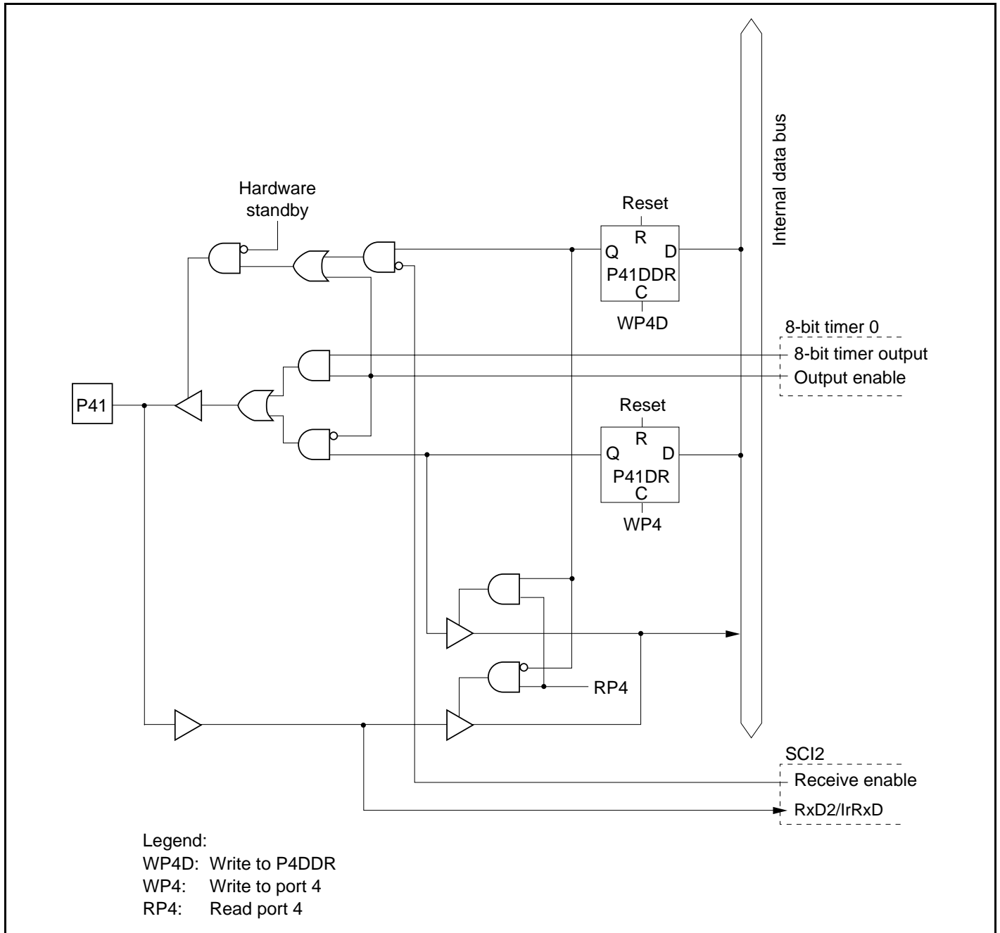
Figure C.7 Port 4 Block Diagram (Pin P41)
