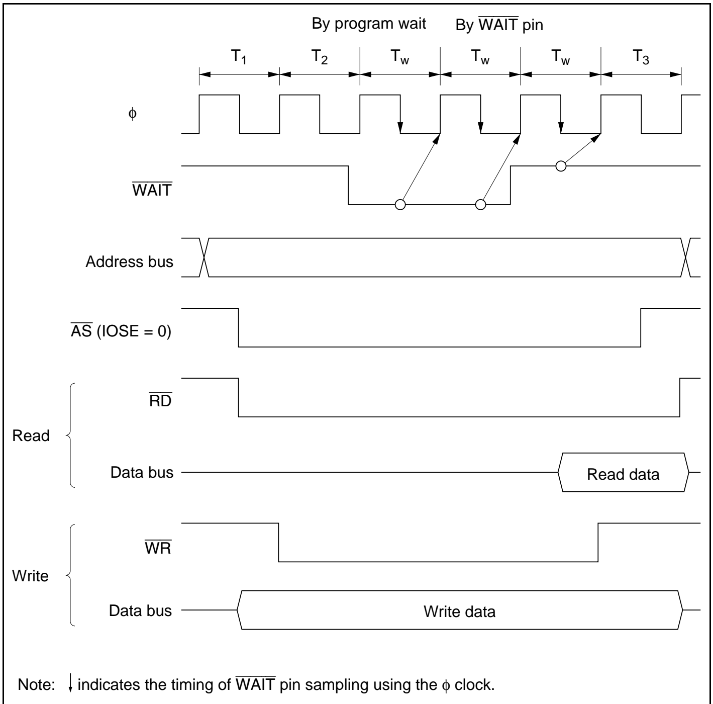
Figure 6.7 Example of Wait State Insertion Timing
