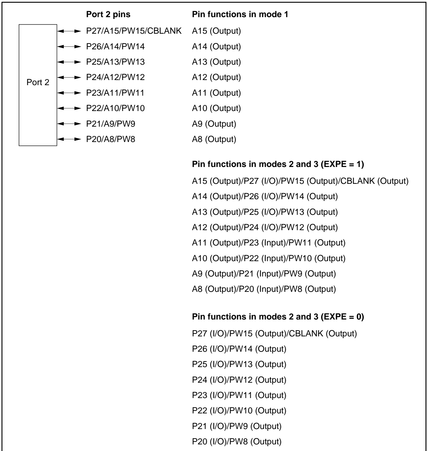
Figure 8.5 Port 2 Pin Functions
