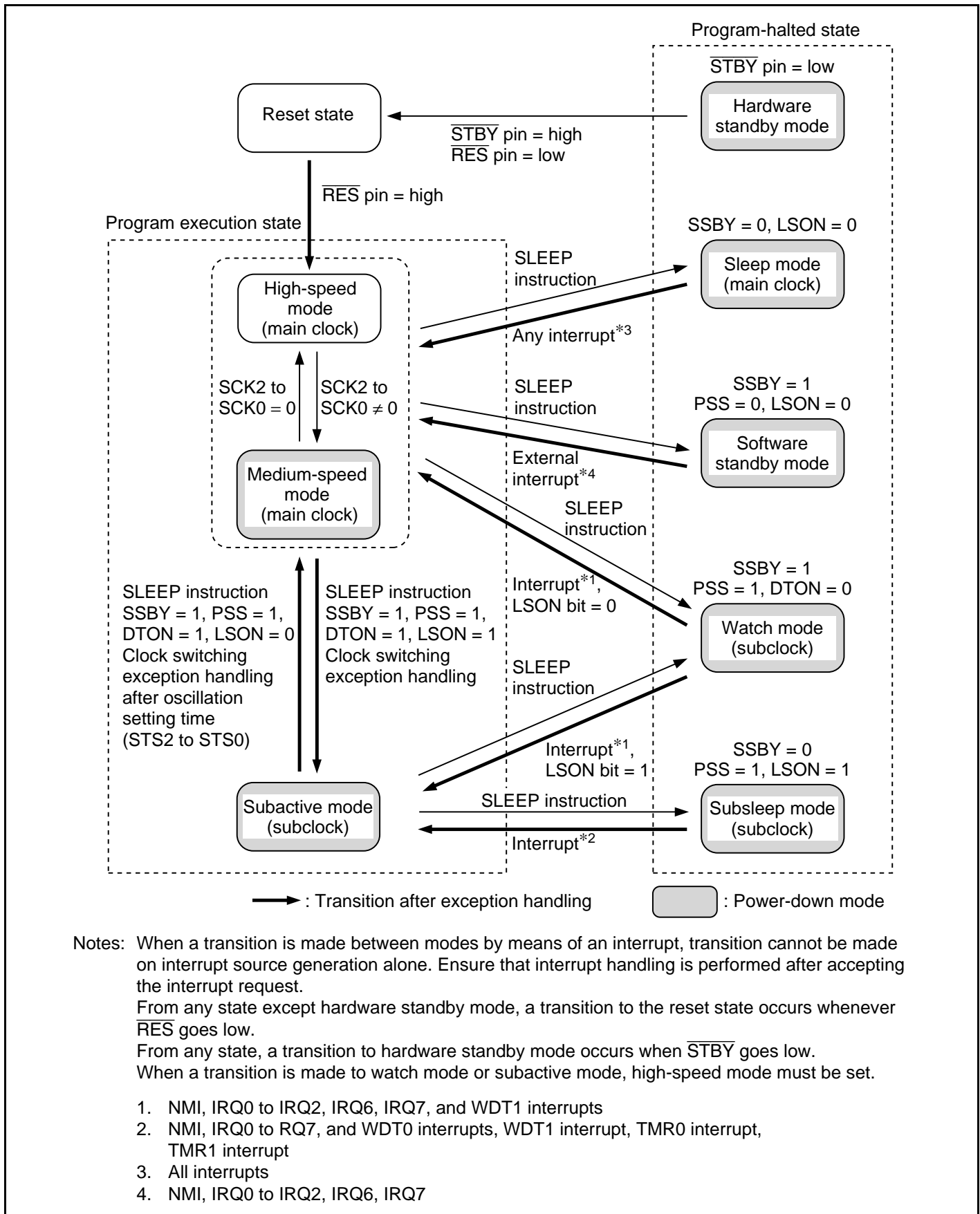
Figure 24.1 Mode Transitions
