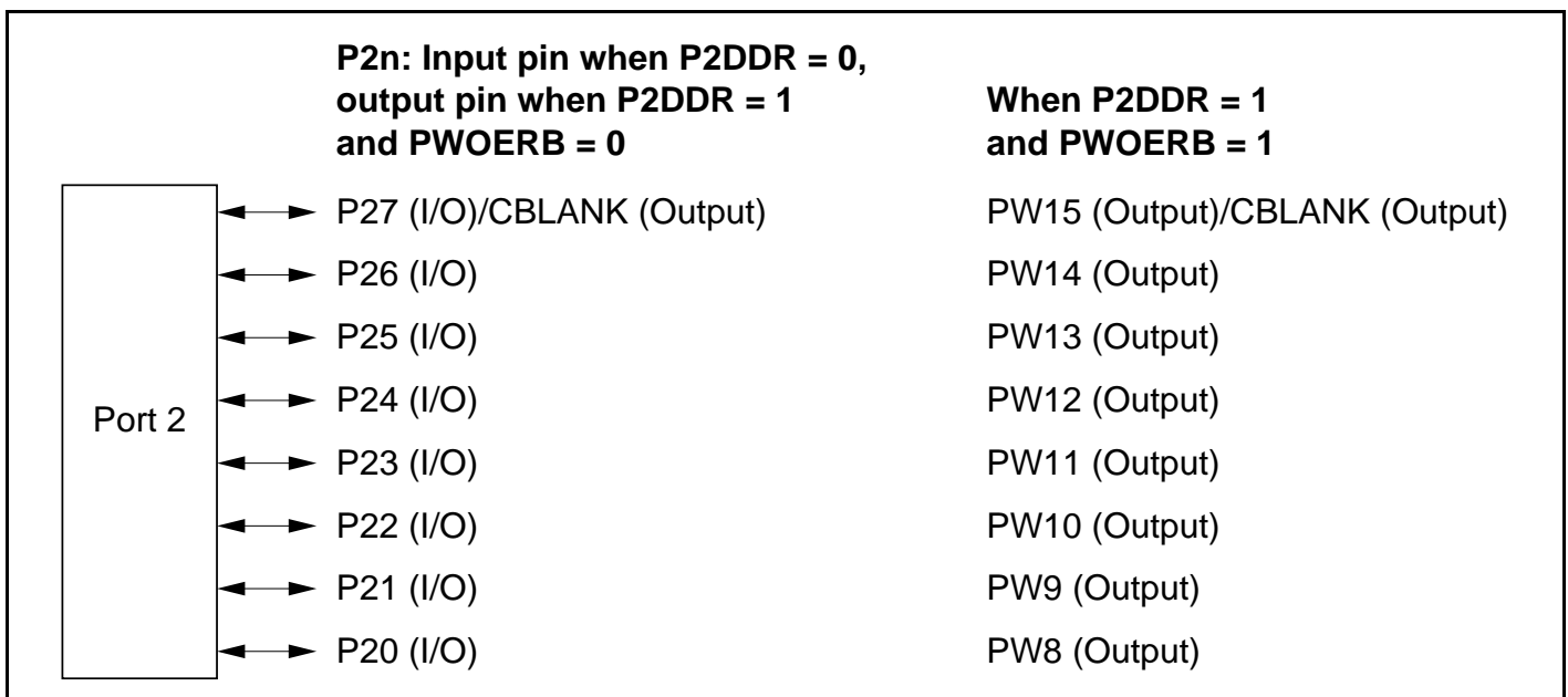
Figure 8.8 Port 2 Pin Functions (Modes 2 and 3 (EXPE = 0))
