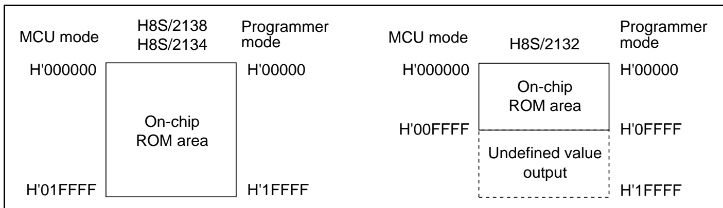
Figure 21.15 Memory Map in Programmer Mode
