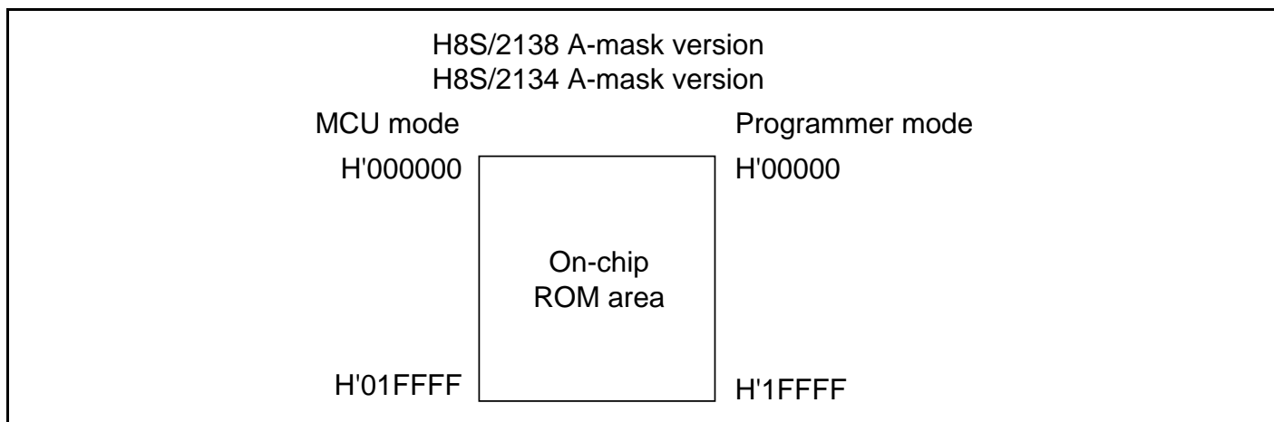
Figure 22.15 Memory Map in Programmer Mode
