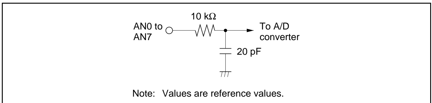
Figure 19.8 Analog Input Pin Equivalent Circuit
