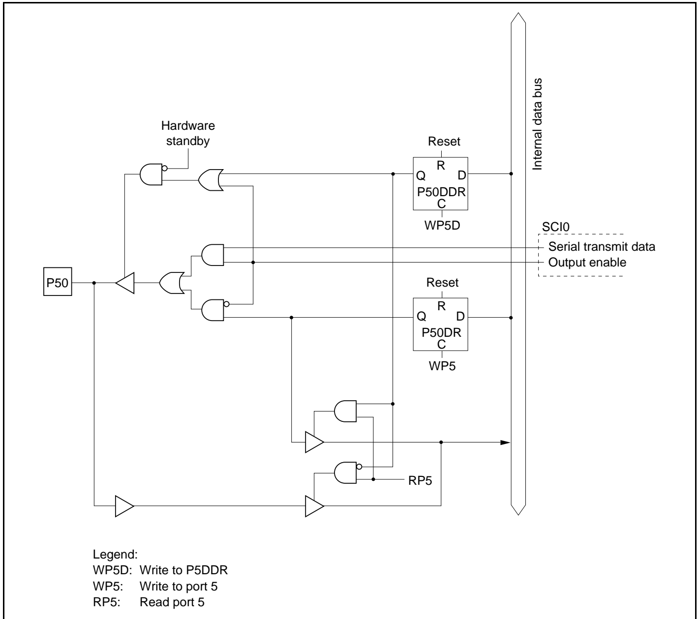
Figure C.13 Port 5 Block Diagram (Pin P50)
