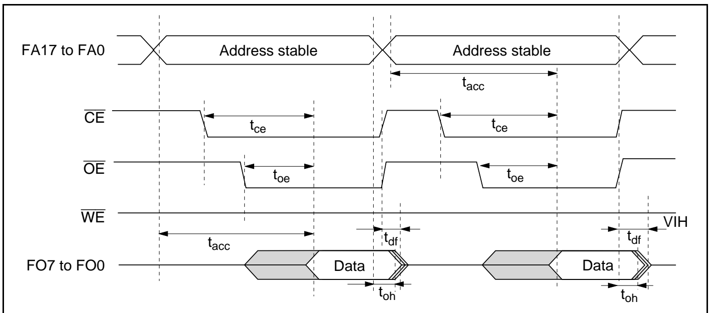
Figure 21.19 Timing Waveforms for \overline{\text{CE}}/\overline{\text{OE}} Clocked Read
