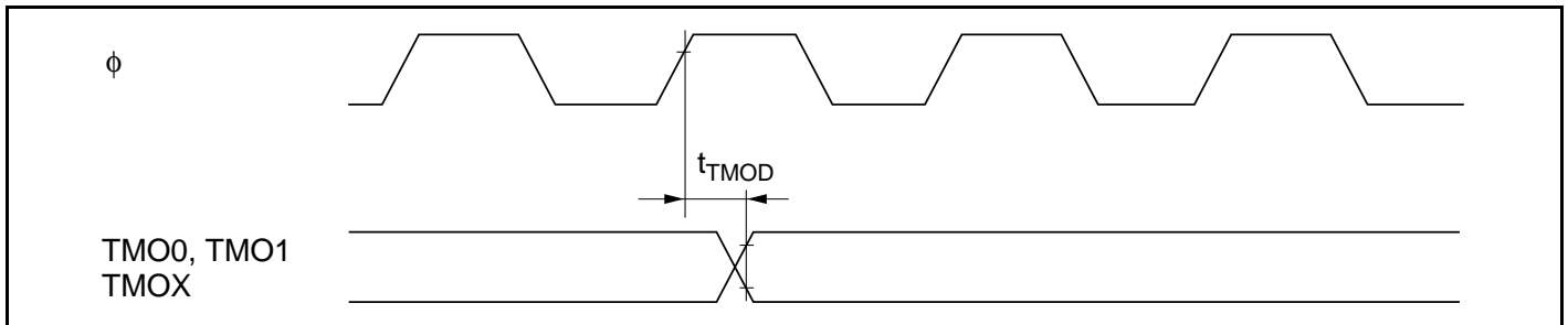
Figure 25.18 8-Bit Timer Output Timing
