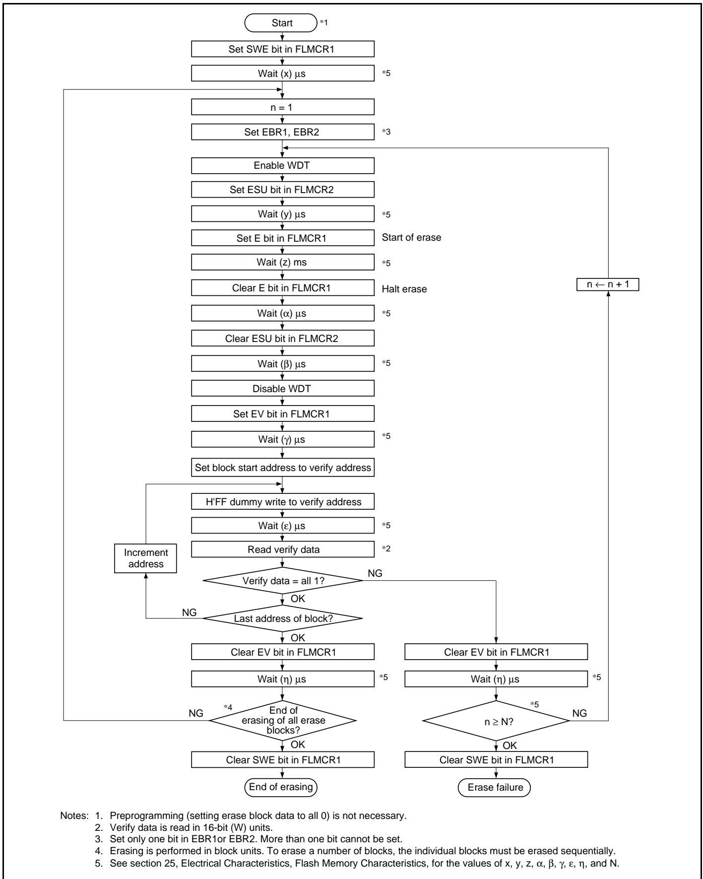
Figure 21.13 Erase/Erase-Verify Flowchart (Single-Block Erase)
