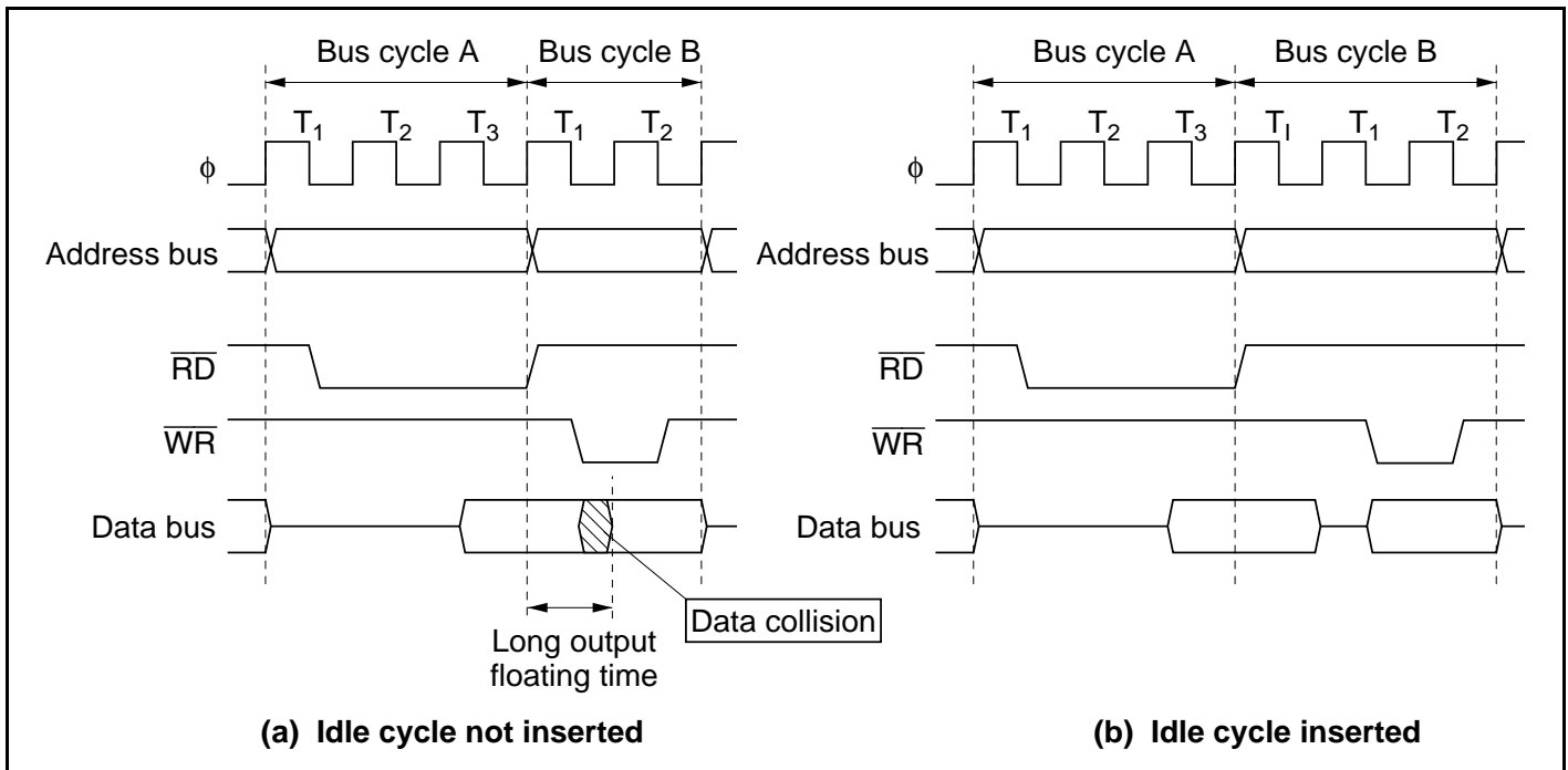
Figure 6.9 Example of Idle Cycle Operation
