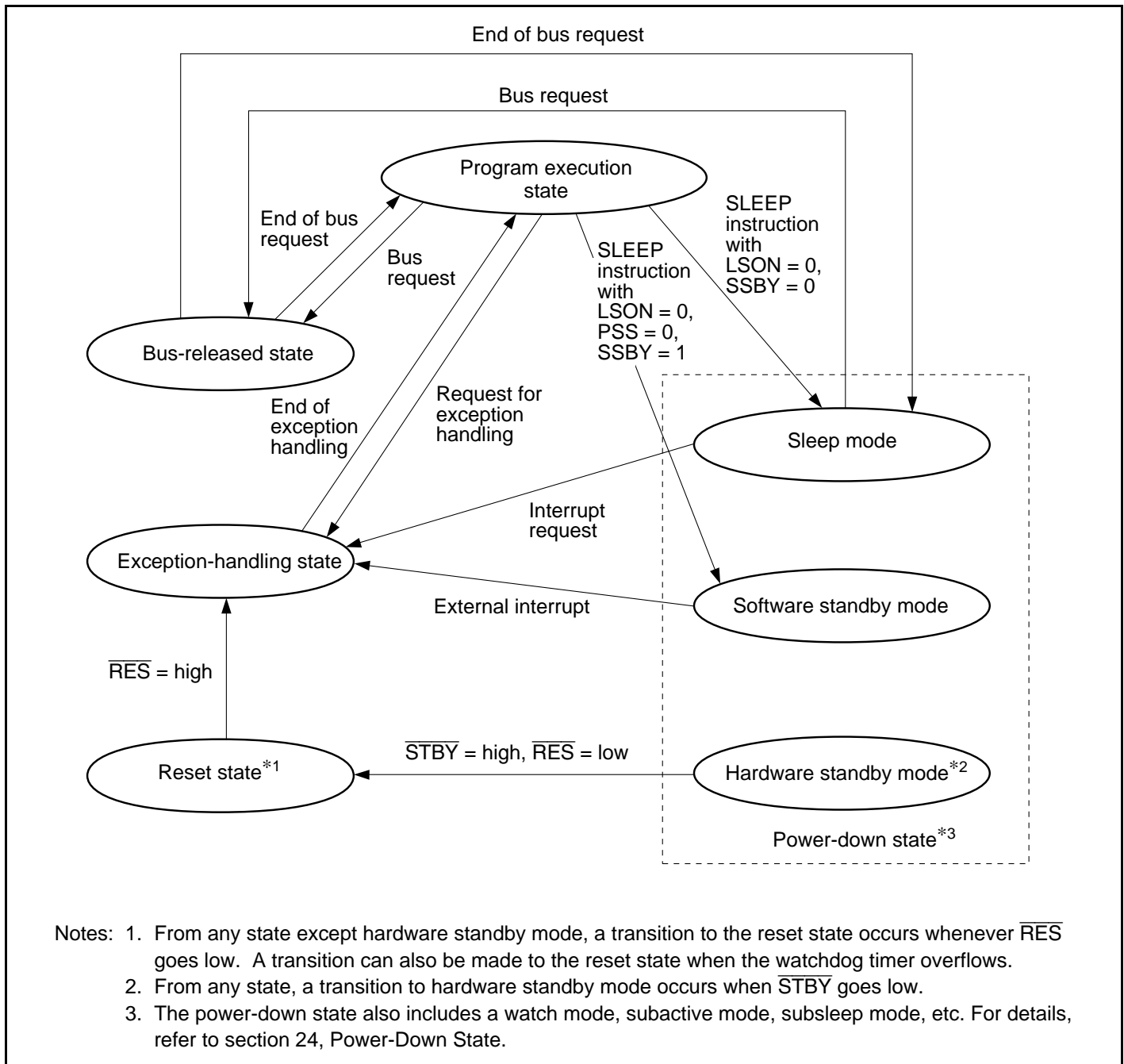
Figure 2.15 State Transitions
