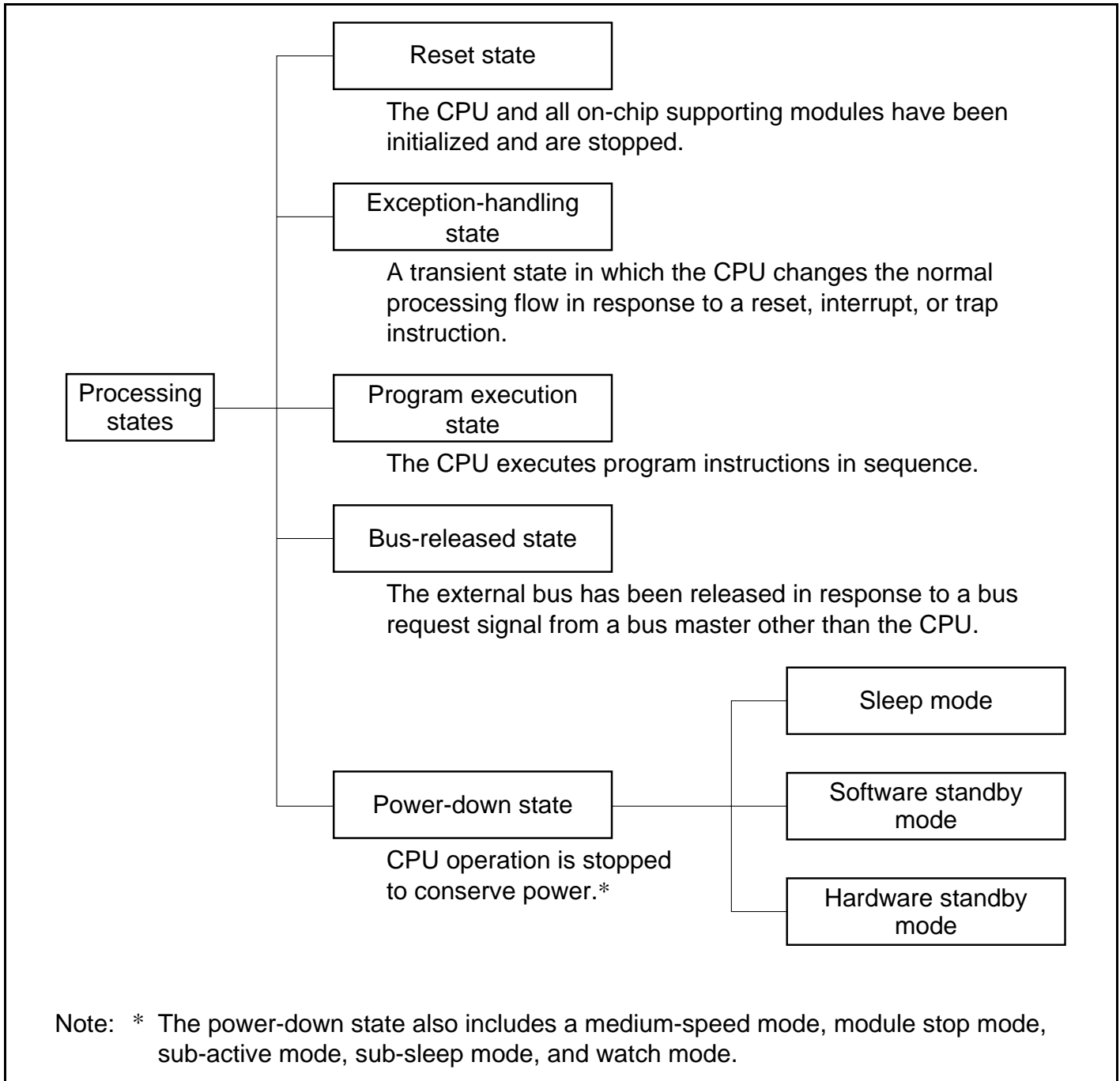
Figure 2.14 Processing States
