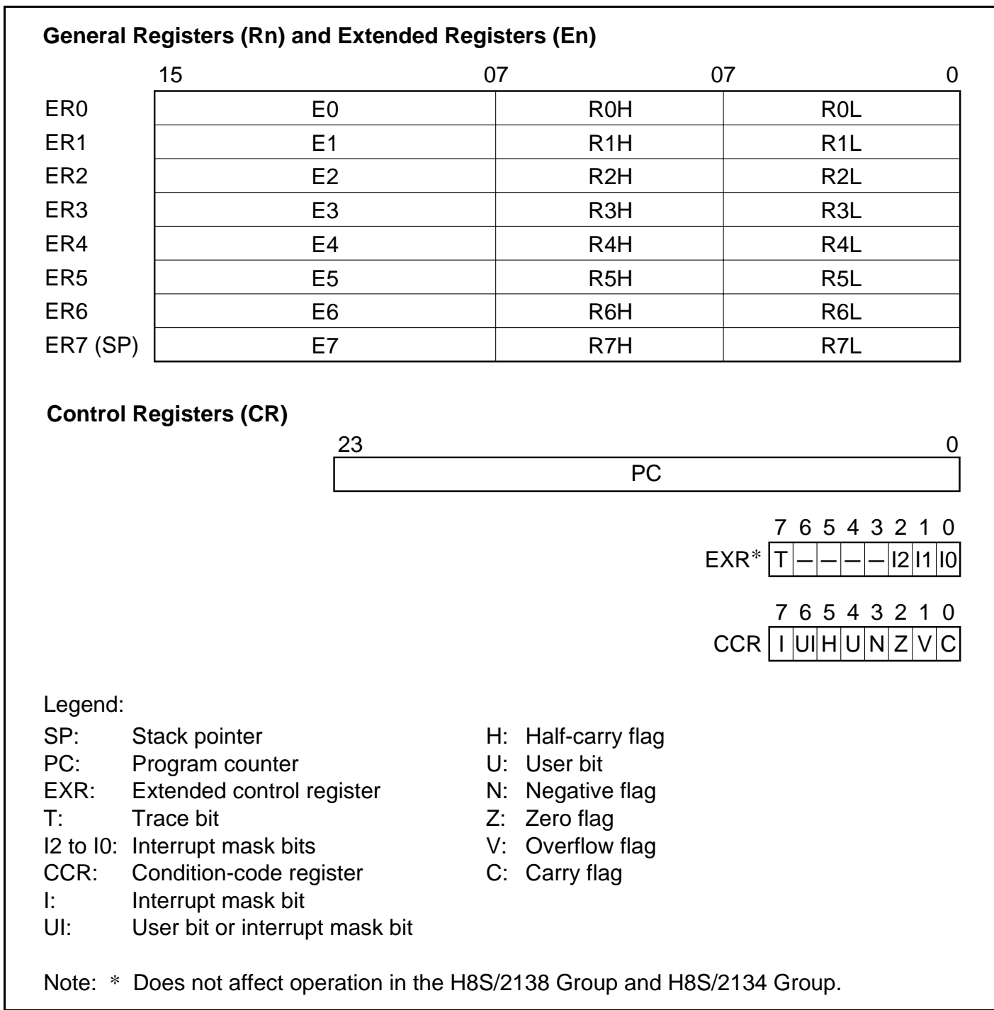
Figure 2.7 CPU Registers
