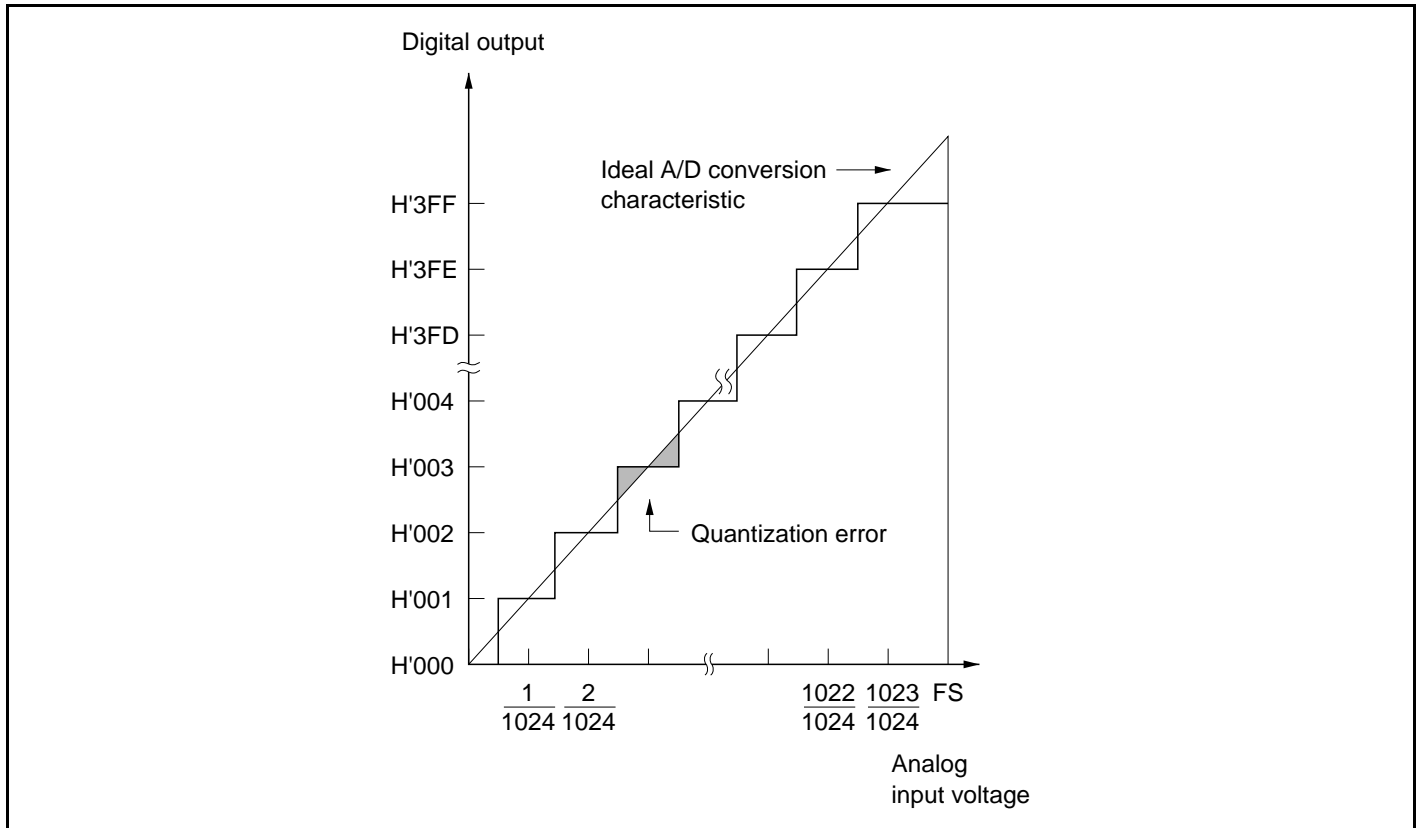
Figure 19.9 A/D Conversion Precision Definitions (1)
