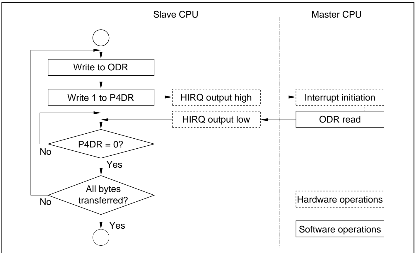
Figure 17.3 HIRQ Output Flowchart
