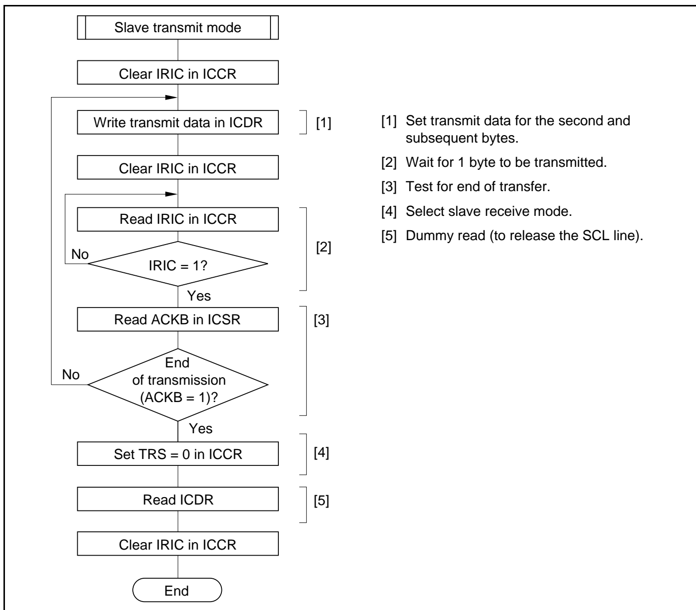
Figure 16.17 Flowchart for Slave Transmit Mode (Example)
