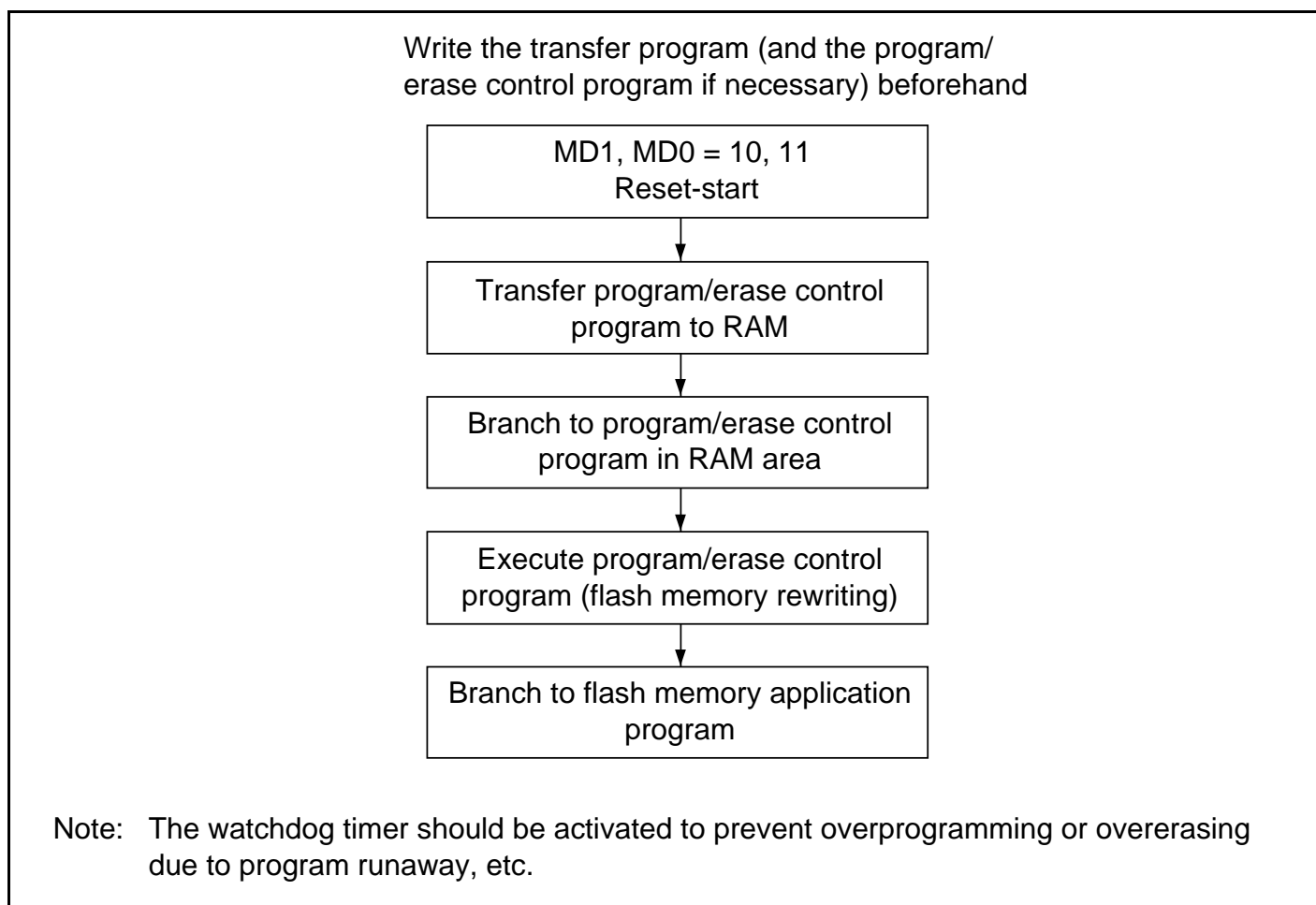
Figure 21.11 User Program Mode Execution Procedure
