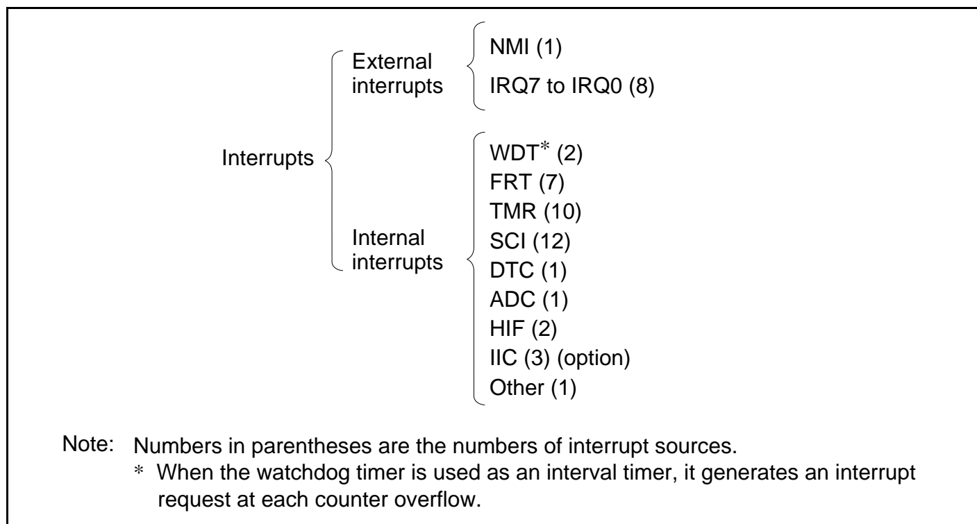
Figure 4.4 Interrupt Sources and Number of Interrupts
