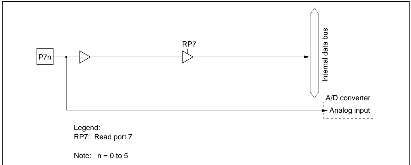
Figure C.21 Port 7 Block Diagram (Pins P70 to P75)
