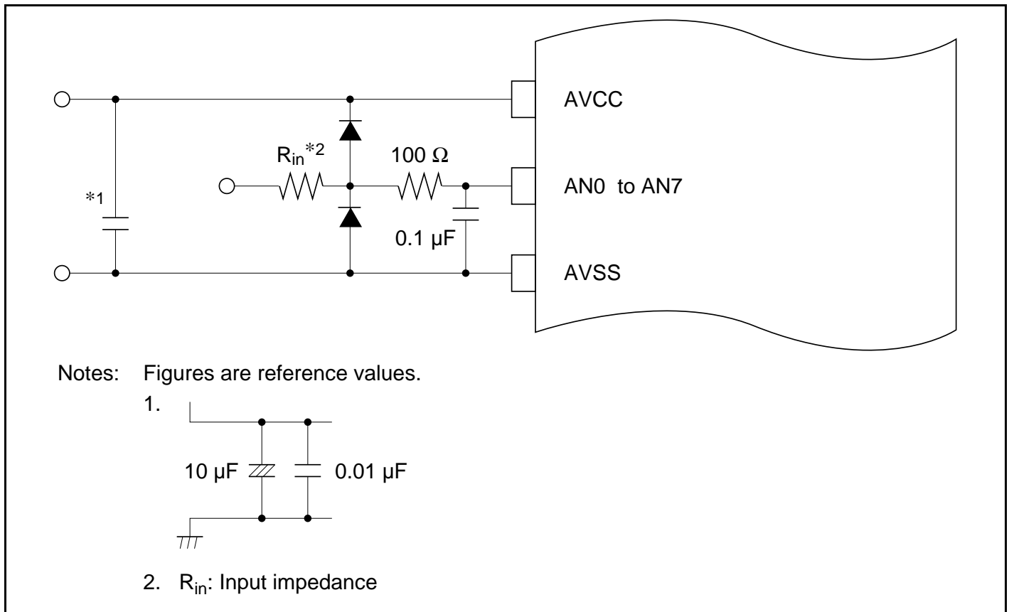
Figure 19.7 Example of Analog Input Protection Circuit
