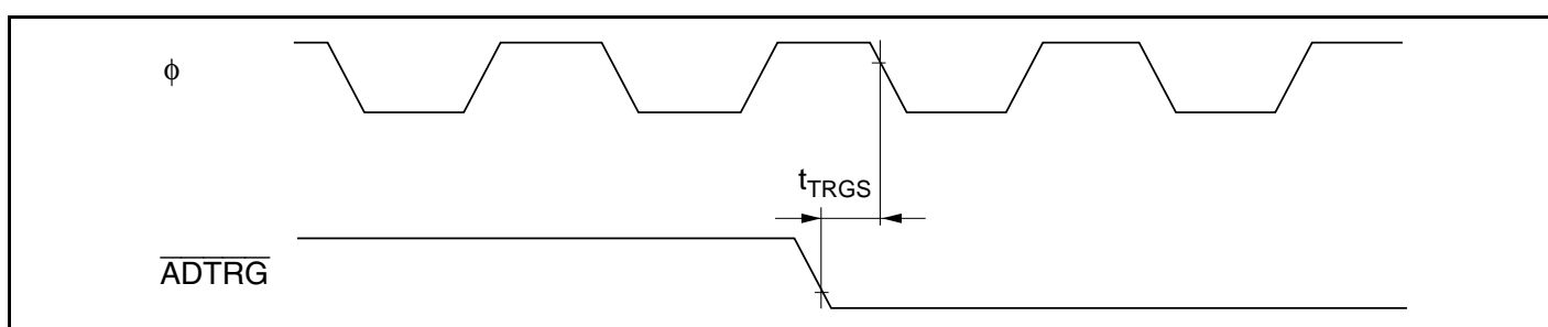
Figure 25.24 A/D Converter External Trigger Input Timing
