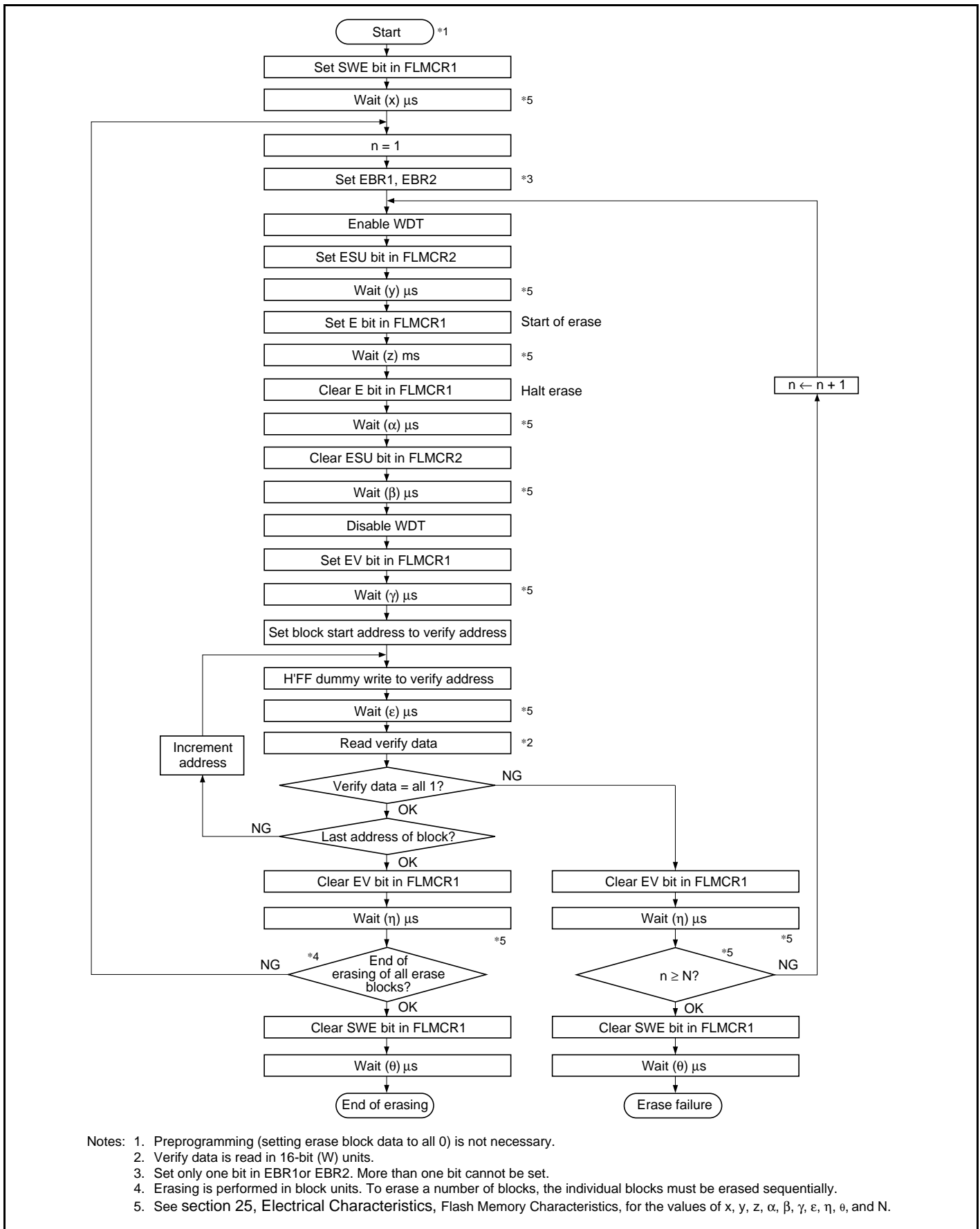
Figure 22.13 Erase/Erase-Verify Flowchart (Single-Block Erase)
