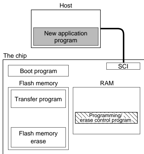
Figure 22.5 User Program Mode (Example)
