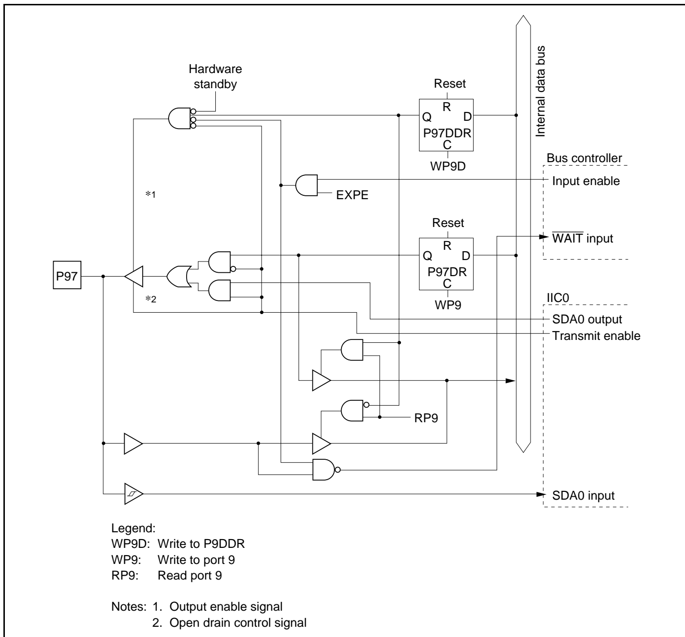
Figure C.33 Port 9 Block Diagram (Pin P97)
