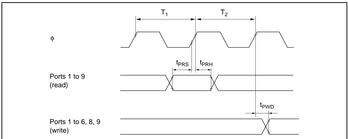
Figure 25.15 I/O Port Input/Output Timing
