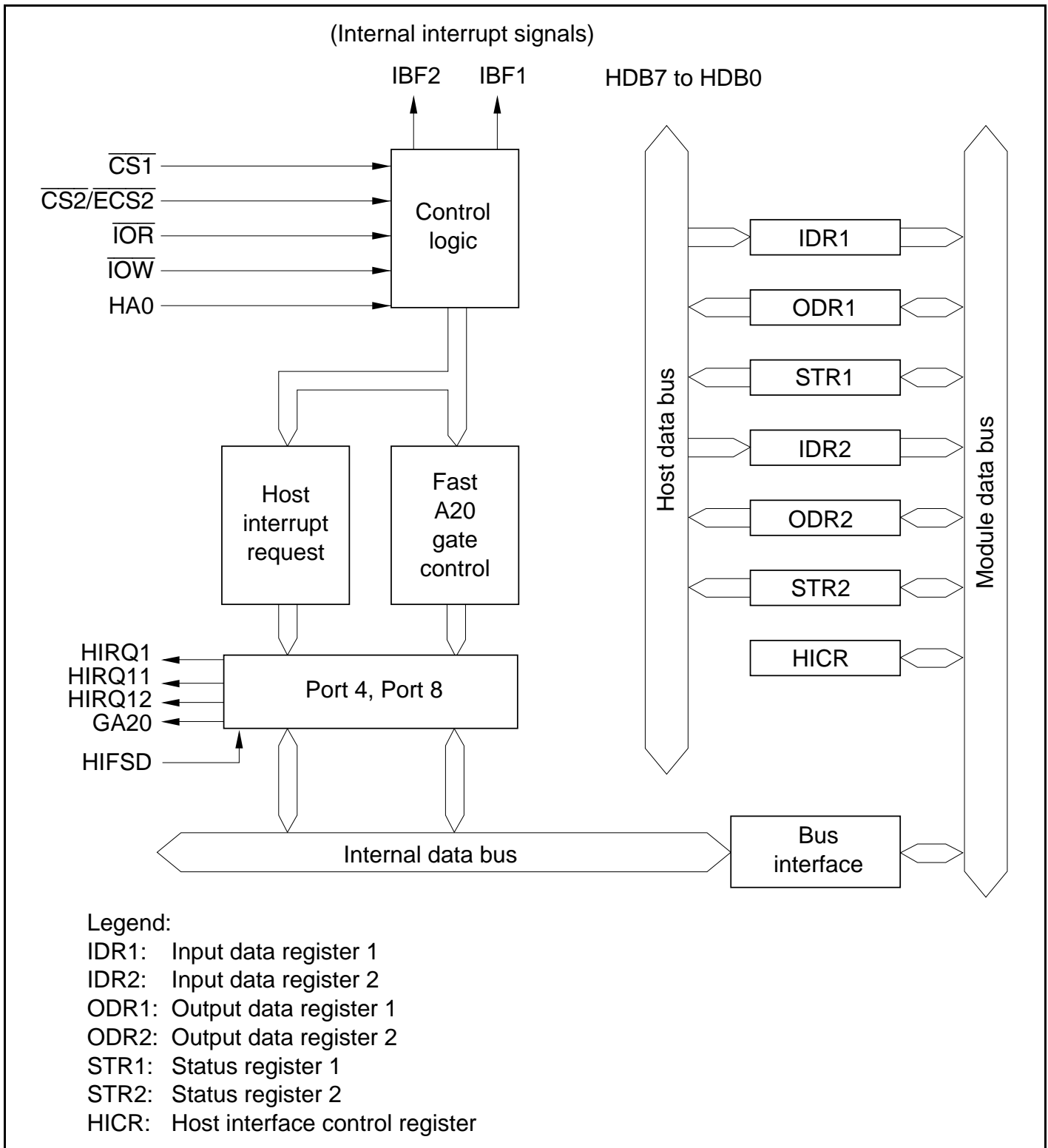
Figure 17.1 Block Diagram of Host Interface
