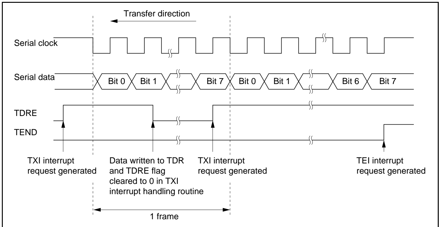
Figure 15.17 Example of SCI Operation in Transmission
