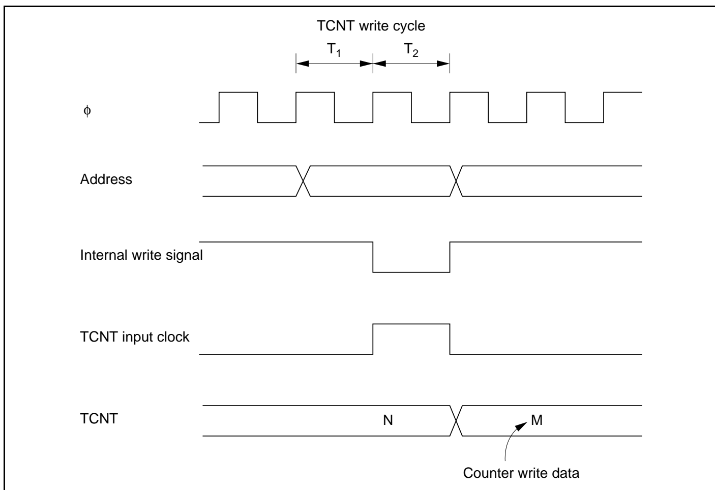
Figure 14.6 Contention between TCNT Write and Increment
