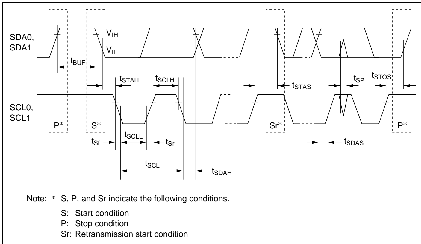
Figure 25.26 I 2 C Bus Interface Input/Output Timing (Option)
