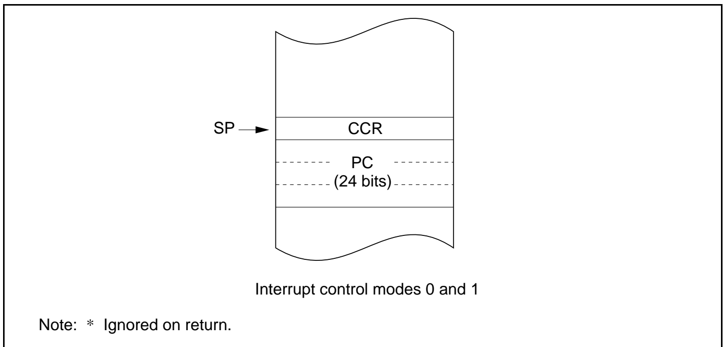
Figure 4.5 (2) Stack Status after Exception Handling (Advanced Mode)
