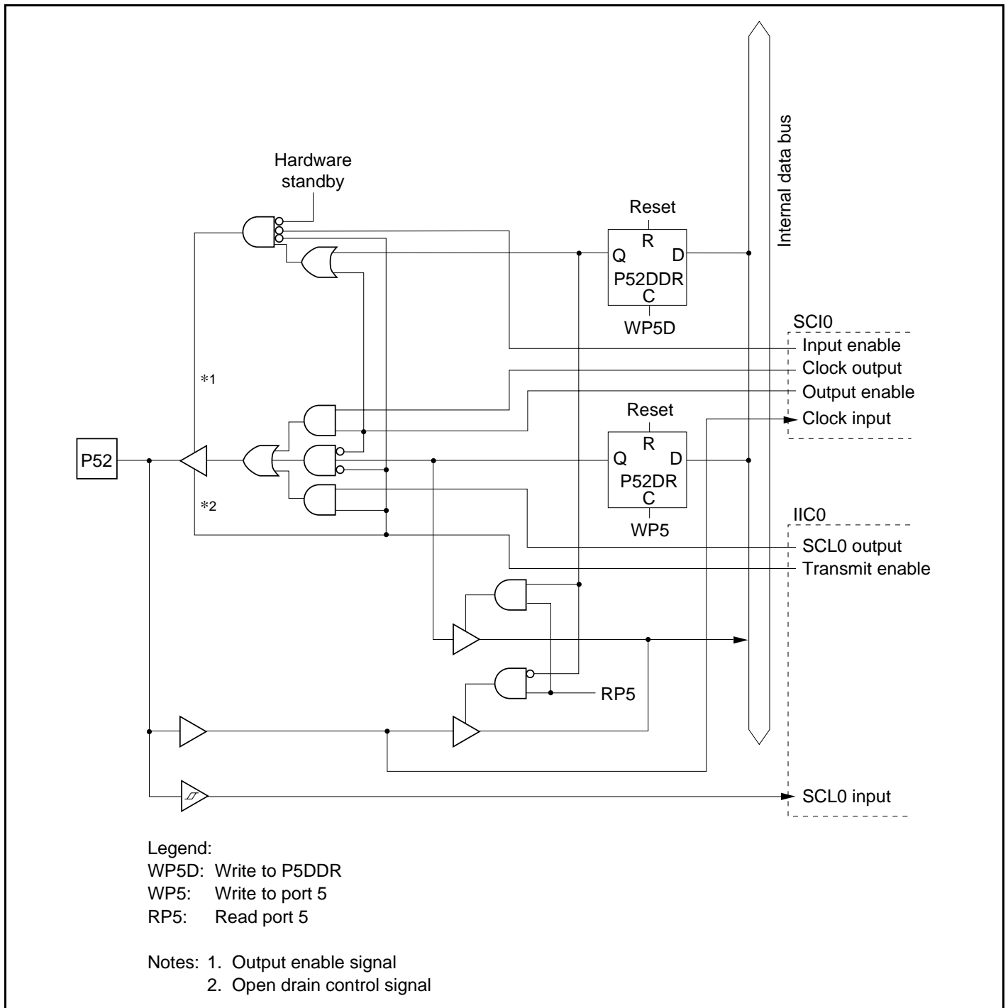
Figure C.15 Port 5 Block Diagram (Pin P52)
