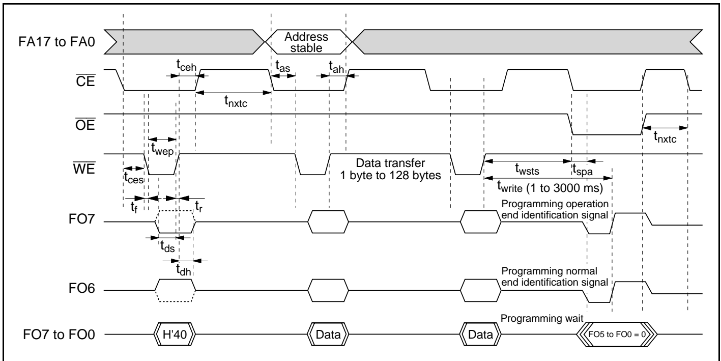
Figure 21.20 Auto-Program Mode Timing Waveforms
