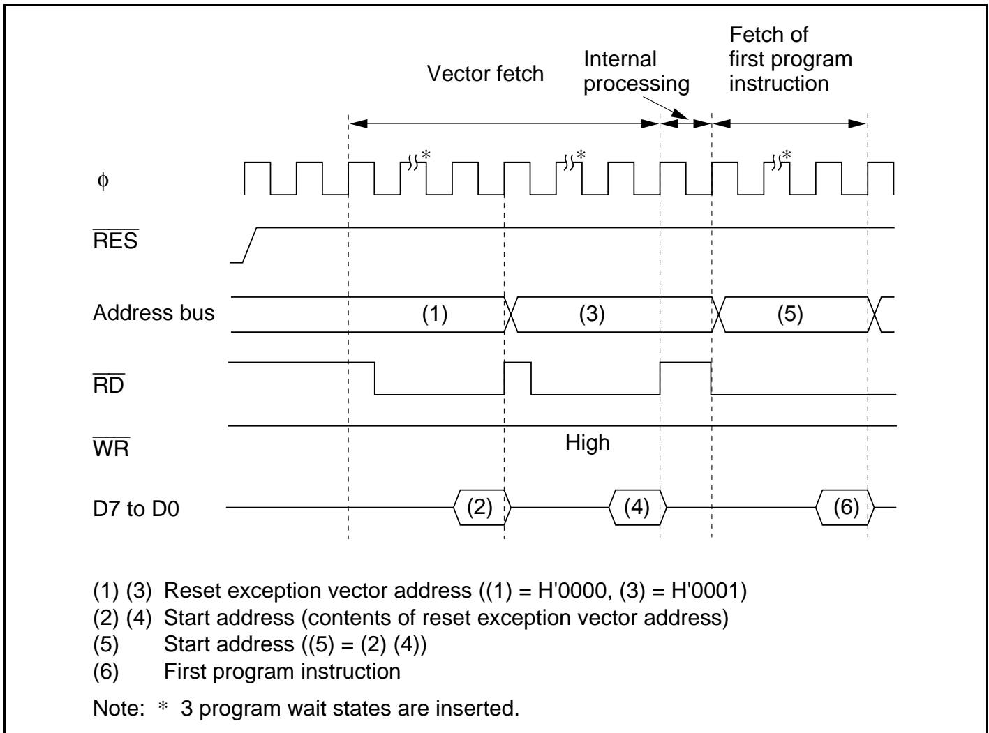
Figure 4.3 Reset Sequence (Mode 1)
