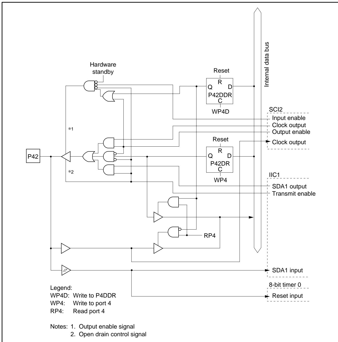
Figure C.8 Port 4 Block Diagram (Pin P42)
