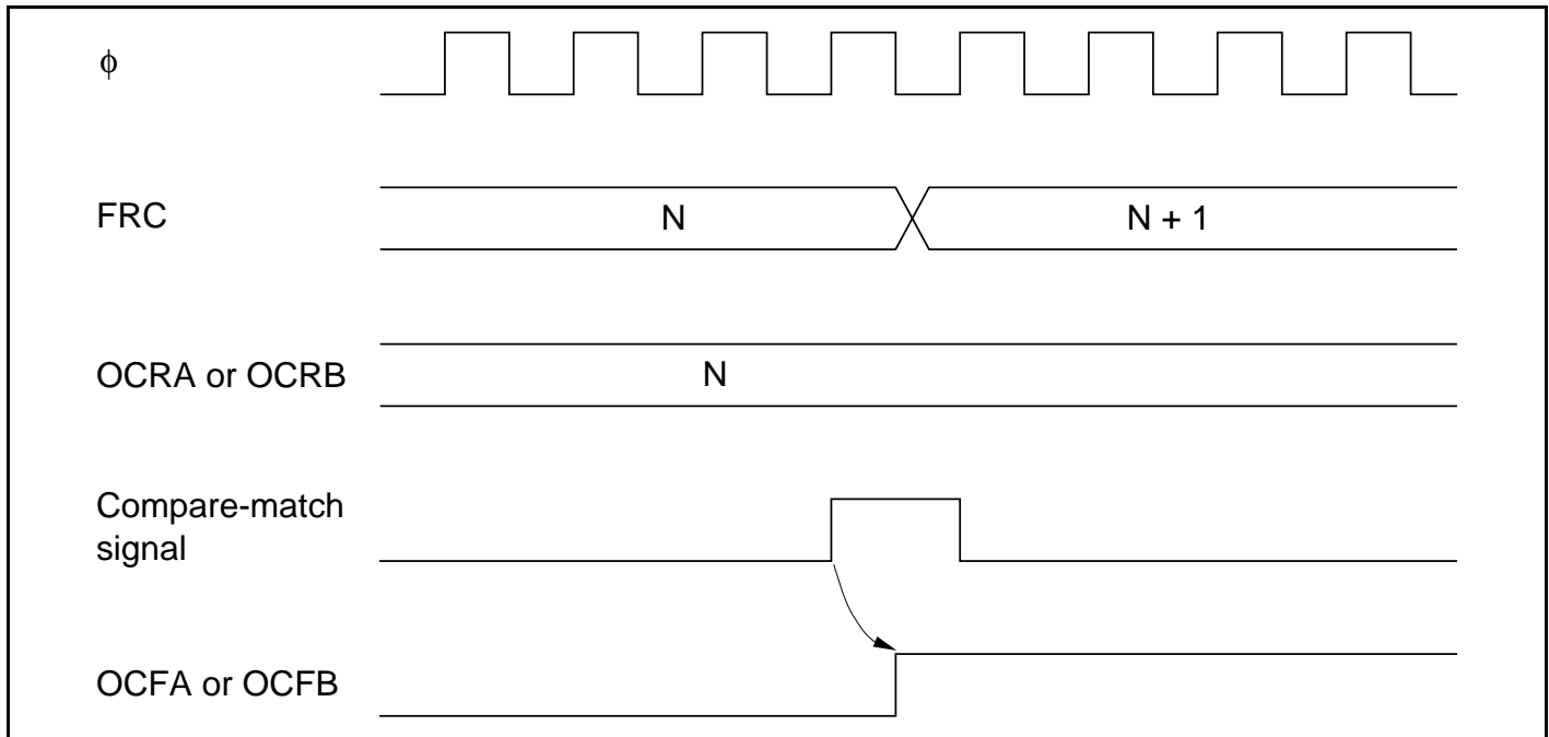
Figure 11.12 Setting of Output Compare Flag (OCFA, OCFB)
