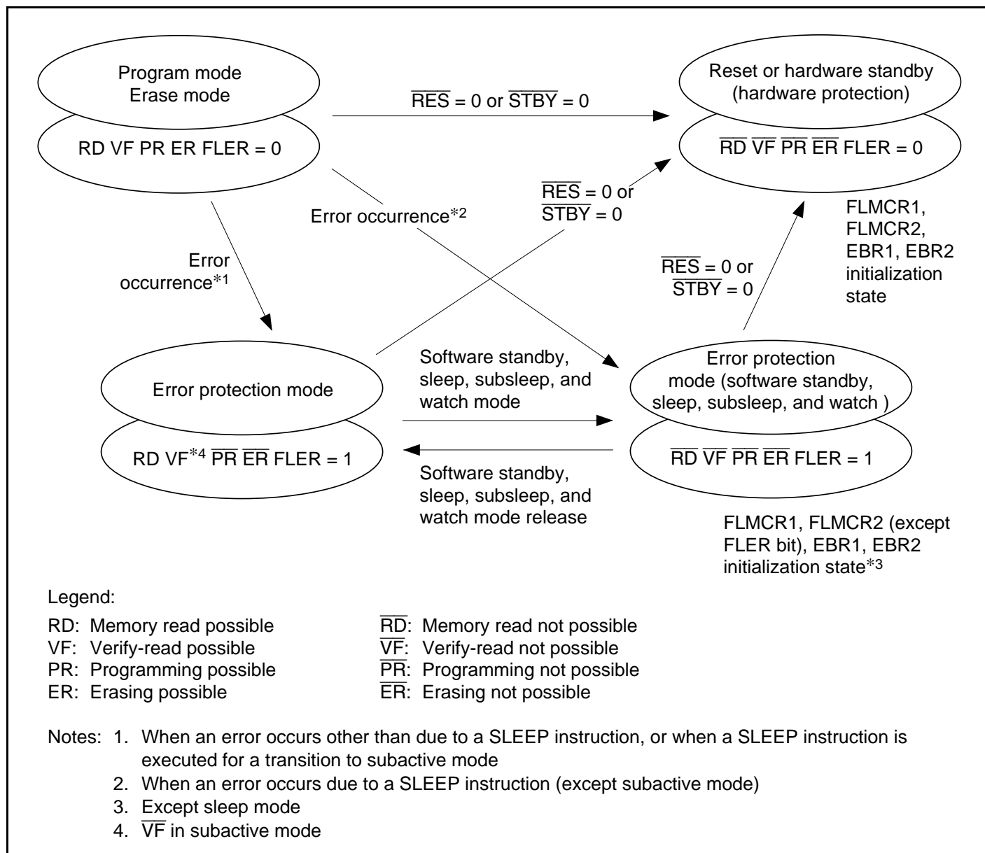
Figure 21.14 Flash Memory State Transitions
