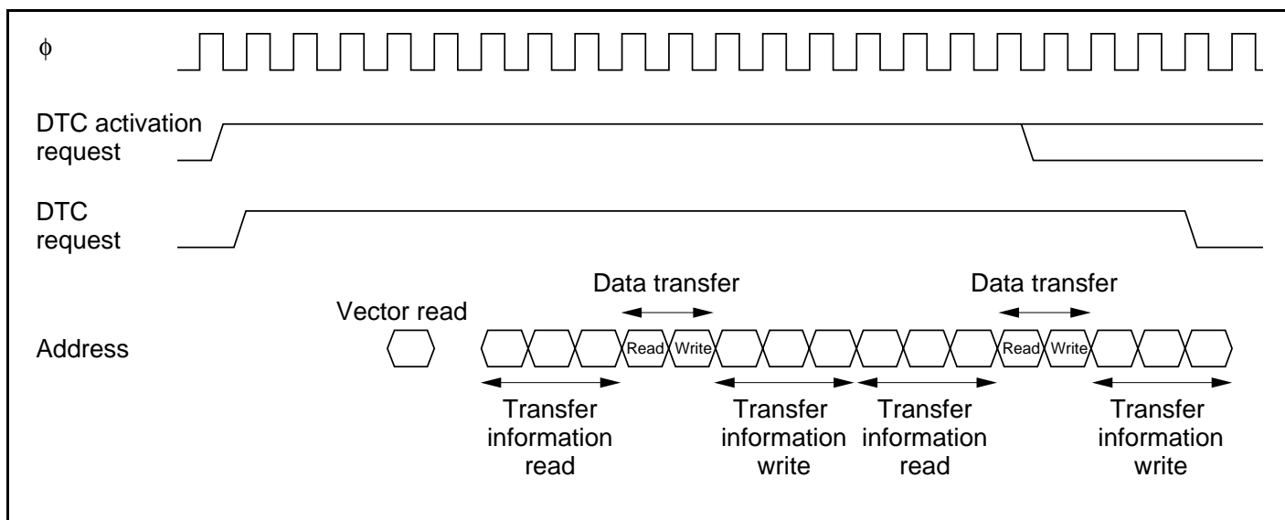
Figure 7.12 DTC Operation Timing (Chain Transfer)
