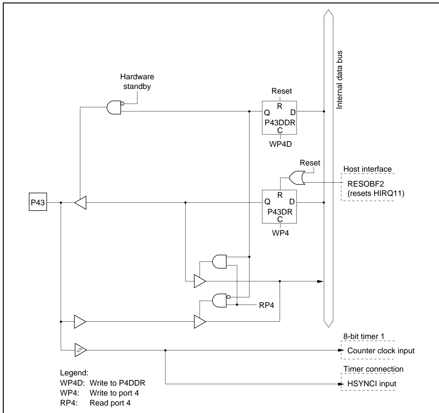
Figure C.9 Port 4 Block Diagram (Pin P43)
