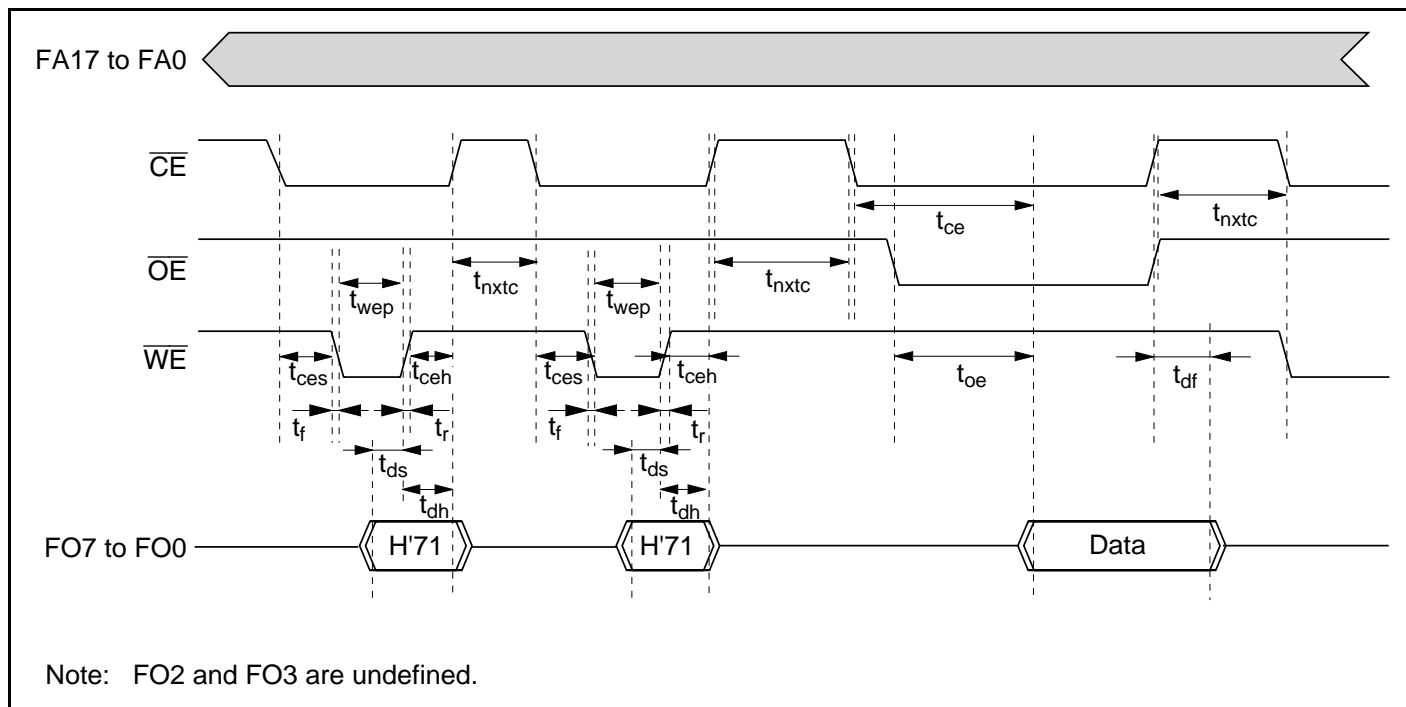
Figure 21.22 Status Read Mode Timing Waveforms
