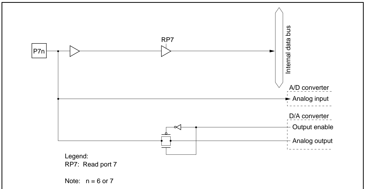
Figure C.22 Port 7 Block Diagram (Pins P76, P77)
