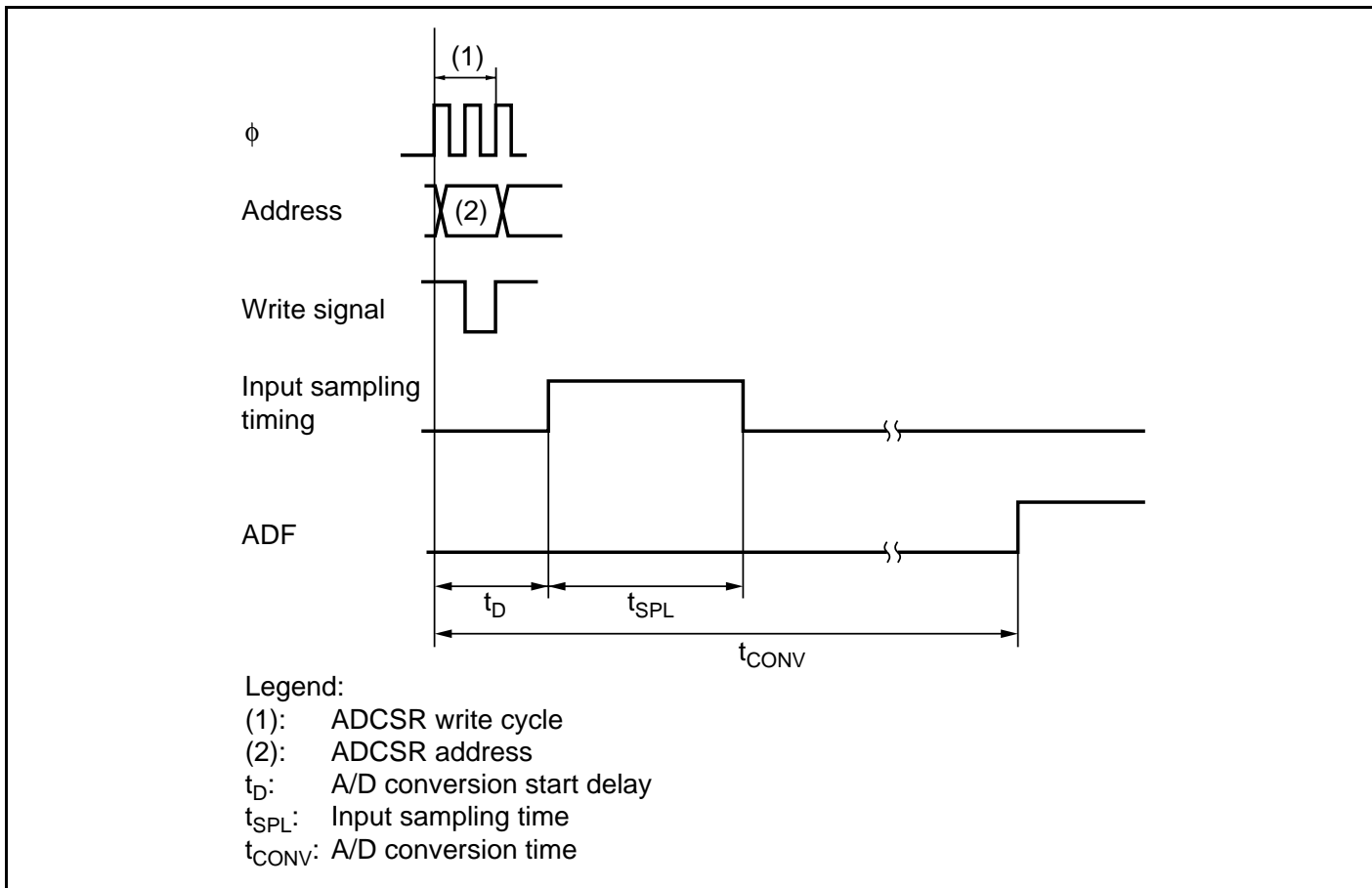
Figure 19.5 A/D Conversion Timing
