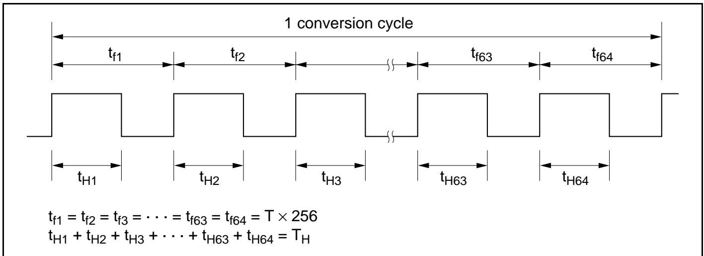
Figure 10.4 (4) Output Waveform
