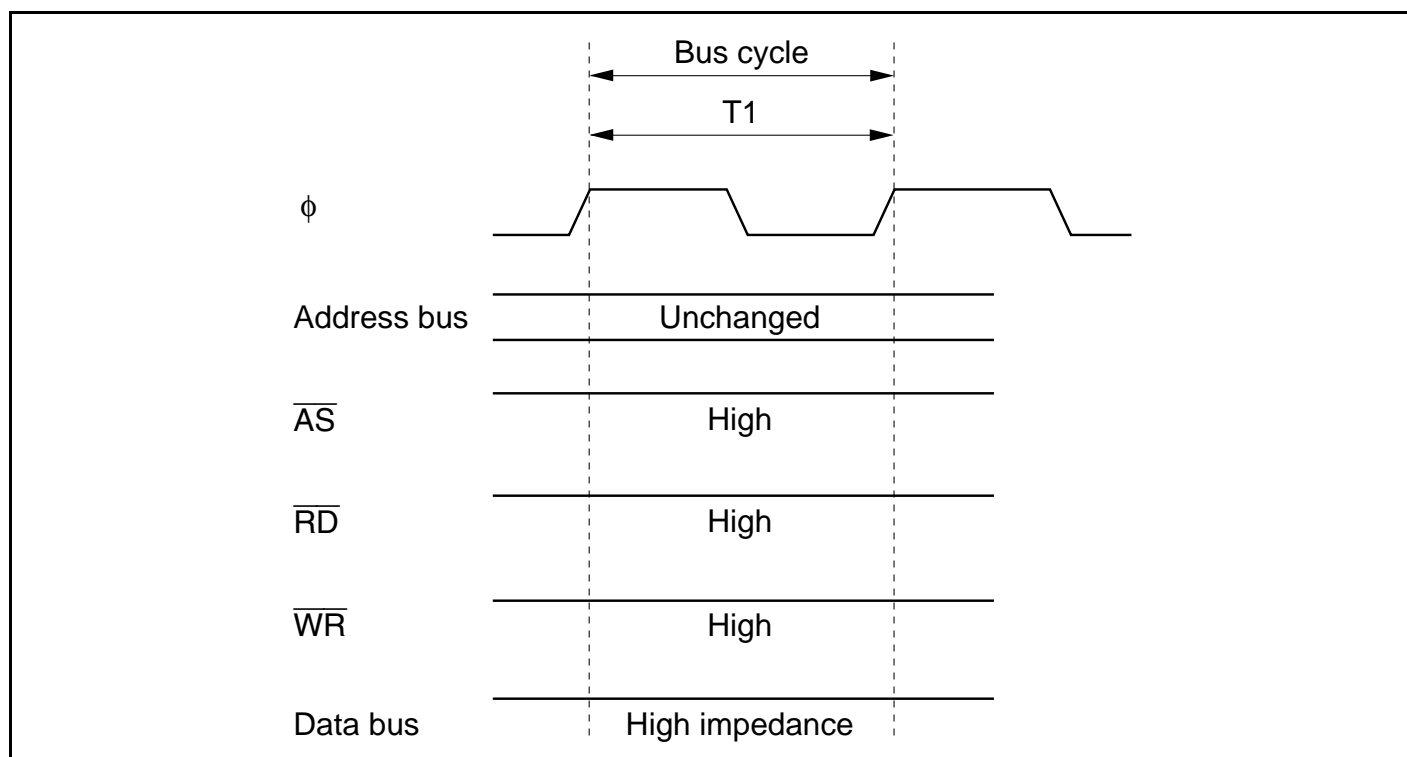
Figure 2.18 Pin States during On-Chip Memory Access
