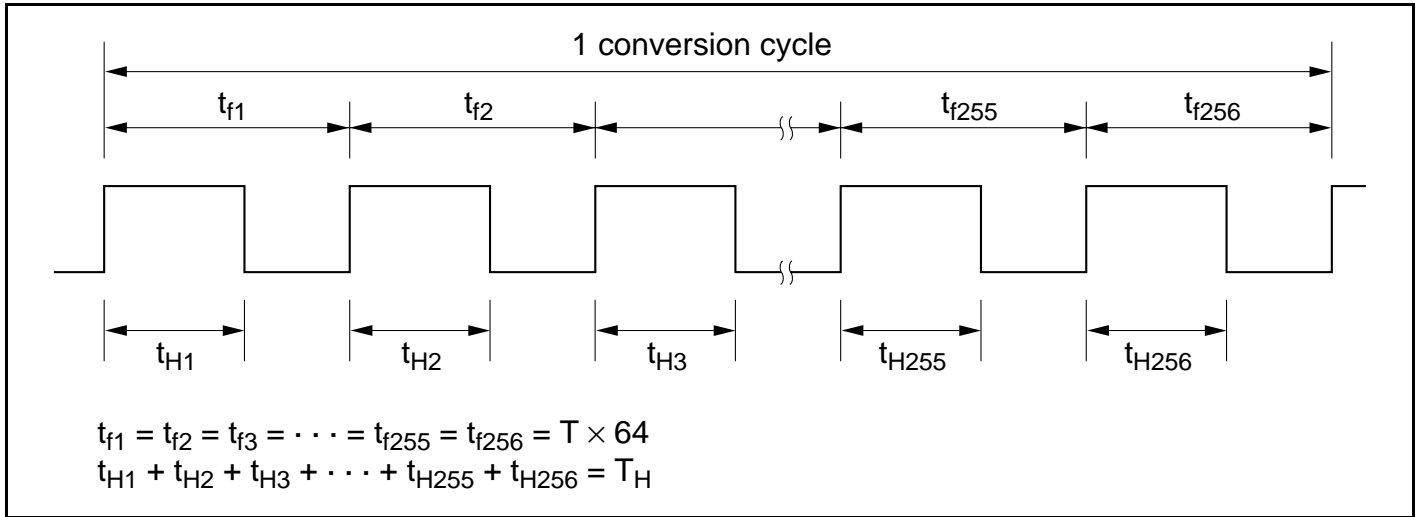
Figure 10.4 (3) Output Waveform
