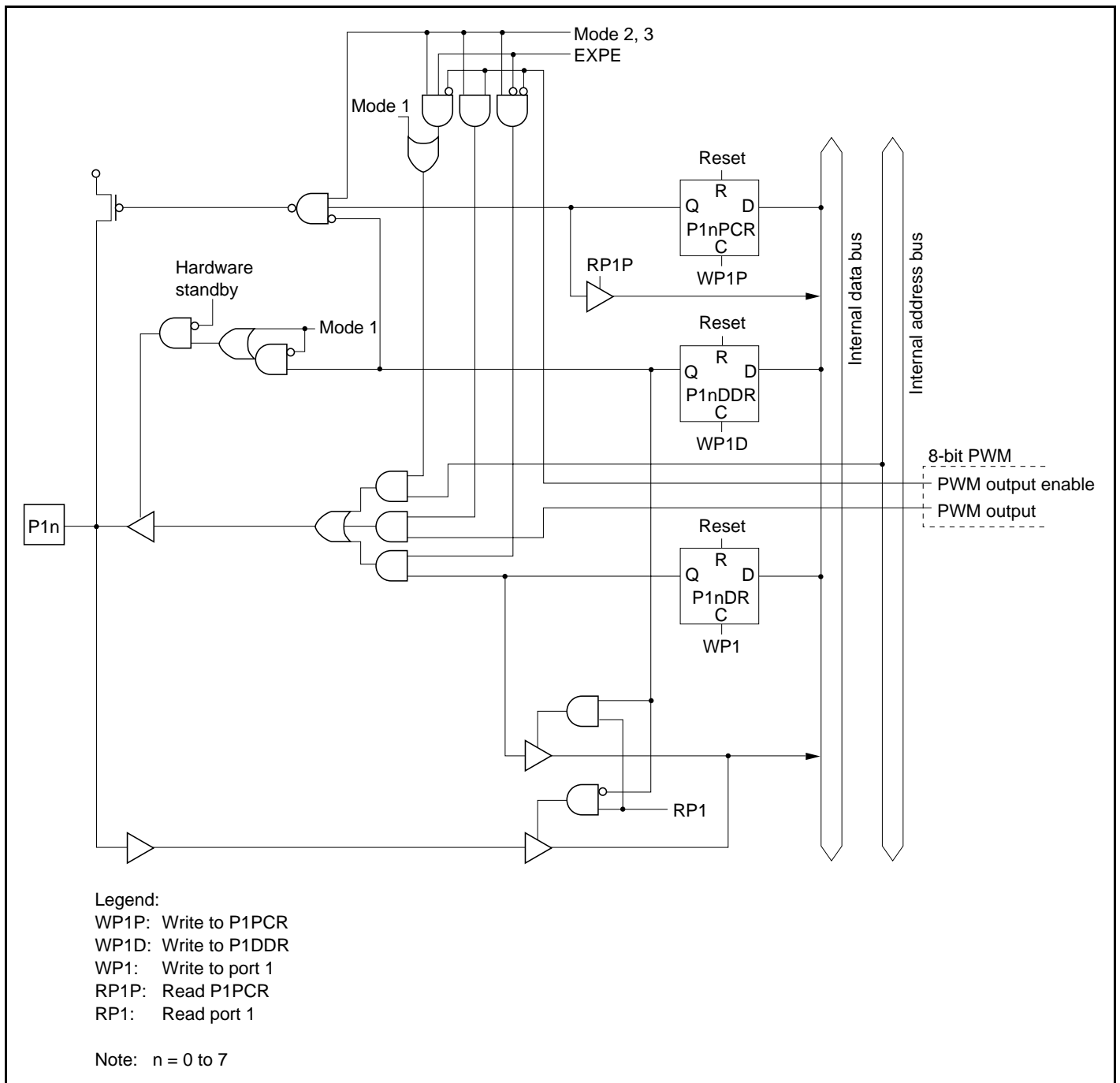
Figure C.1 Port 1 Block Diagram
