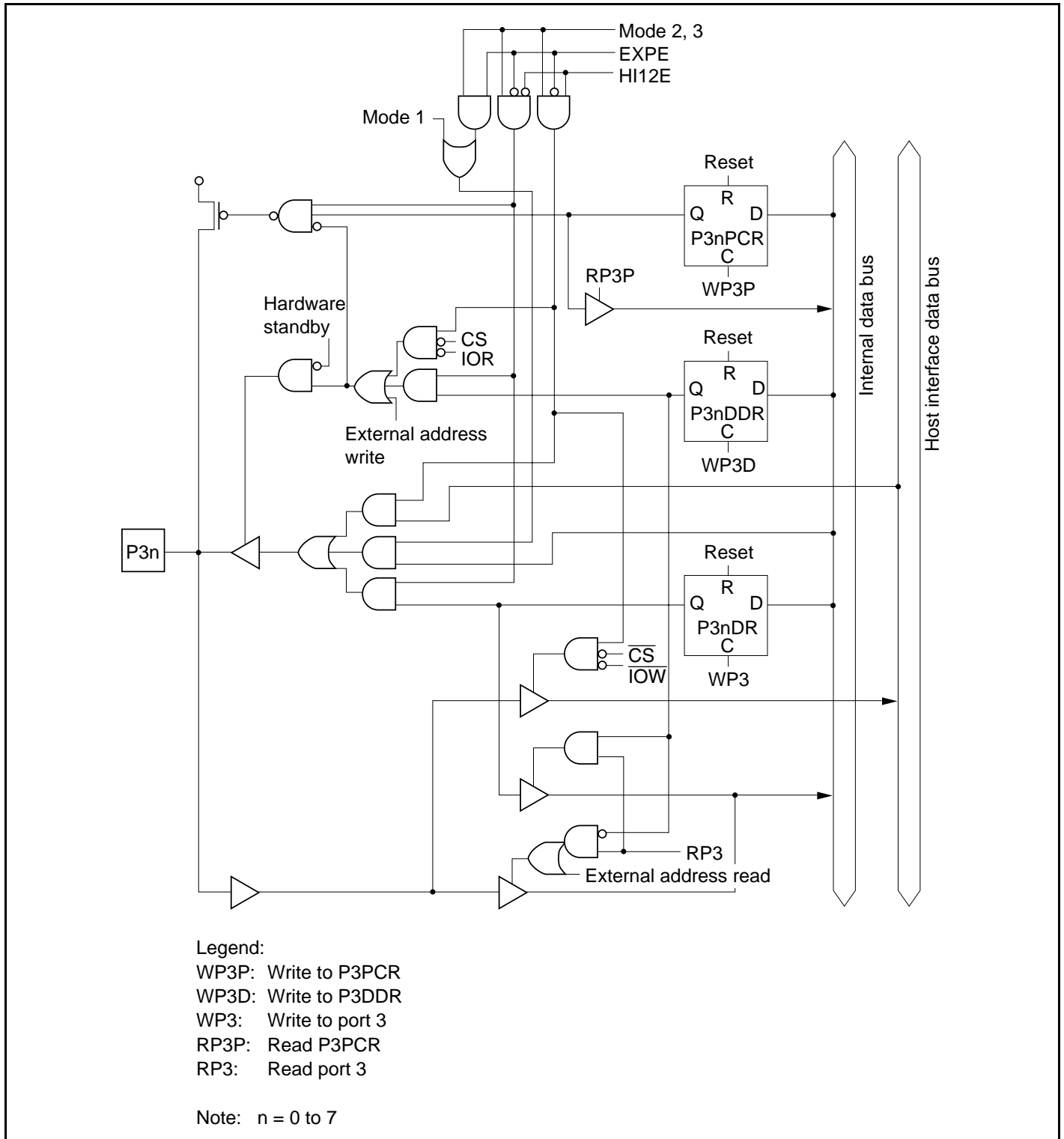
Figure C.5 Port 3 Block Diagram
