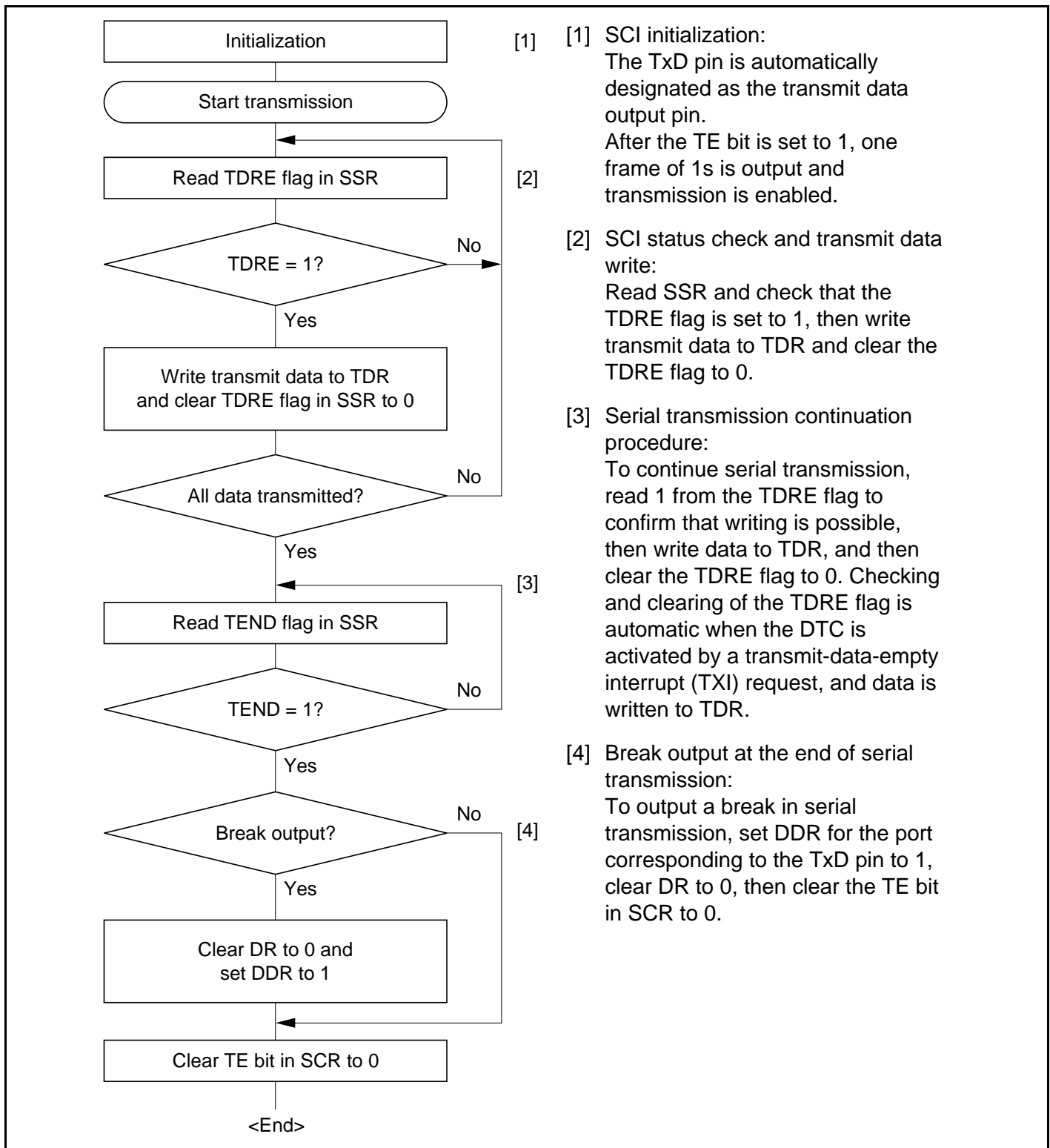
Figure 15.5 Sample Serial Transmission Flowchart
