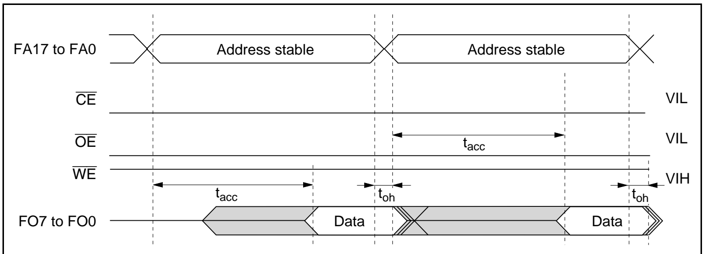
Figure 21.18 Timing Waveforms for \overline{\text{CE}}/\overline{\text{OE}} Enable State Read
