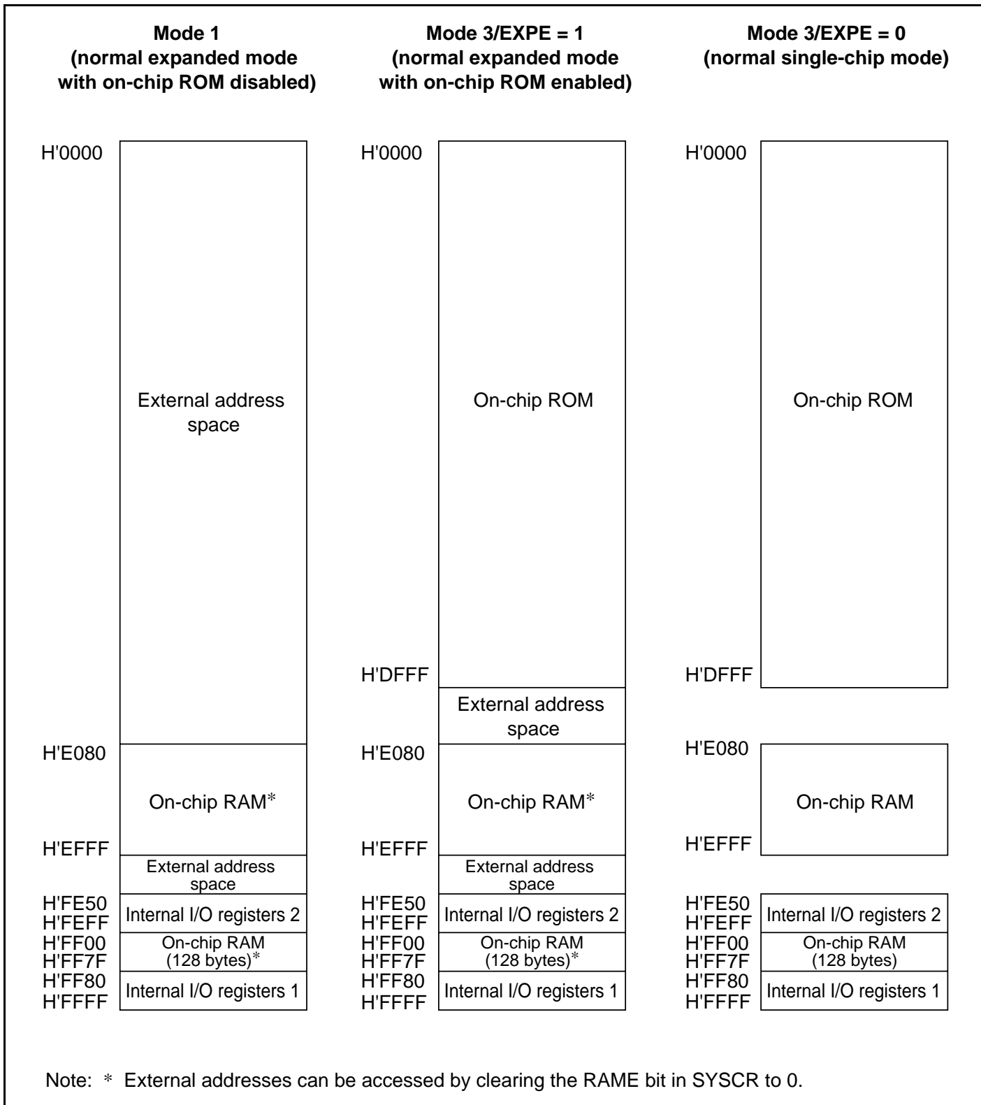
Figure 3.3 H8S/2133 Memory Map in Each Operating Mode
