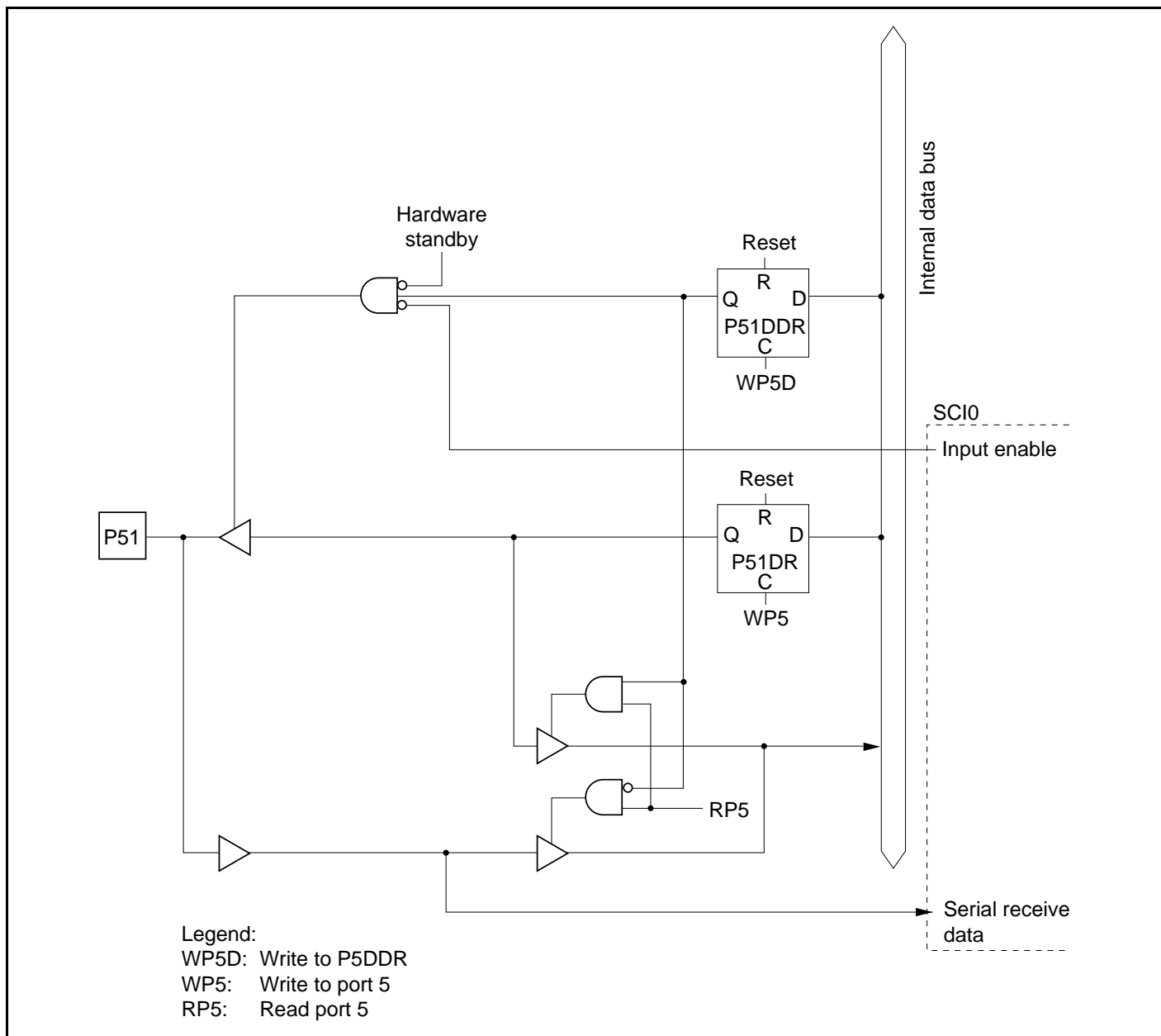
Figure C.14 Port 5 Block Diagram (Pin P51)
