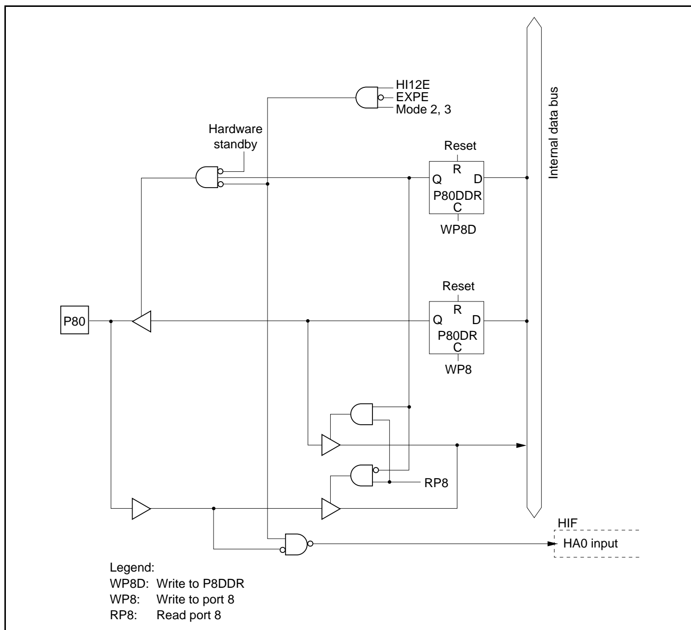
Figure C.23 Port 8 Block Diagram (Pin P80)
