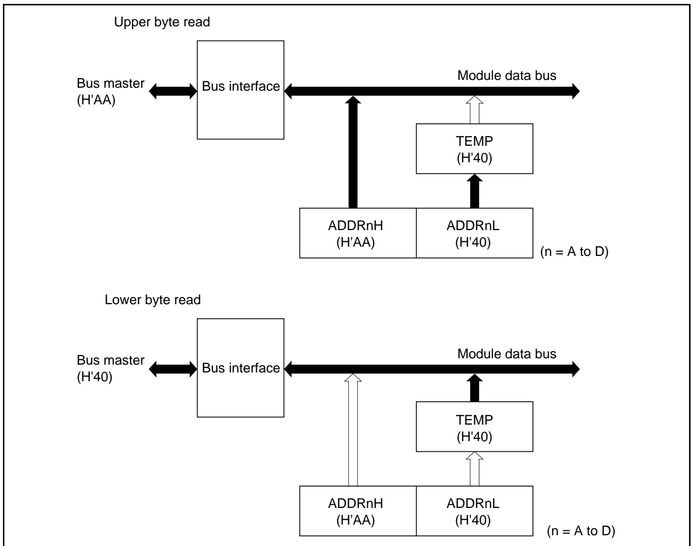
Figure 19.2 ADDR Access Operation (Reading H'AA40)
