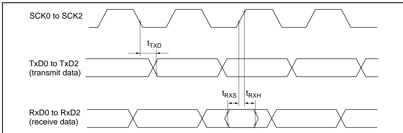
Figure 25.23 SCI Input/Output Timing (Synchronous Mode)
