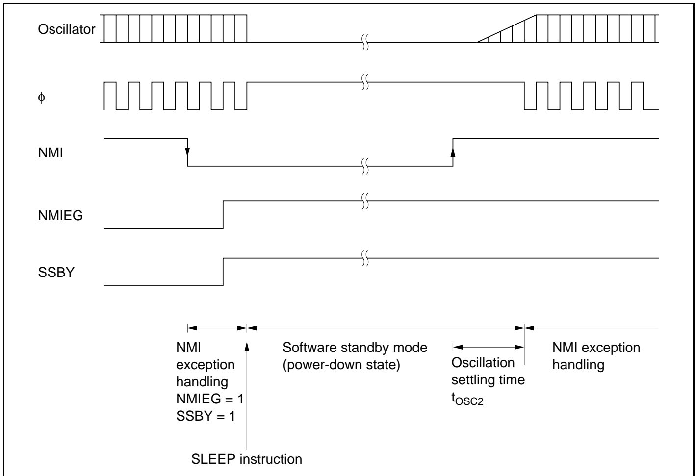
Figure 24.3 Software Standby Mode Application Example
