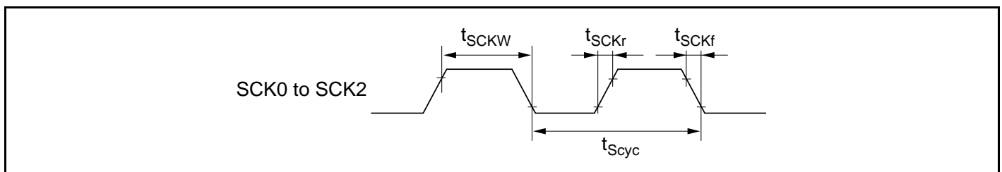
Figure 25.22 SCK Clock Input Timing
