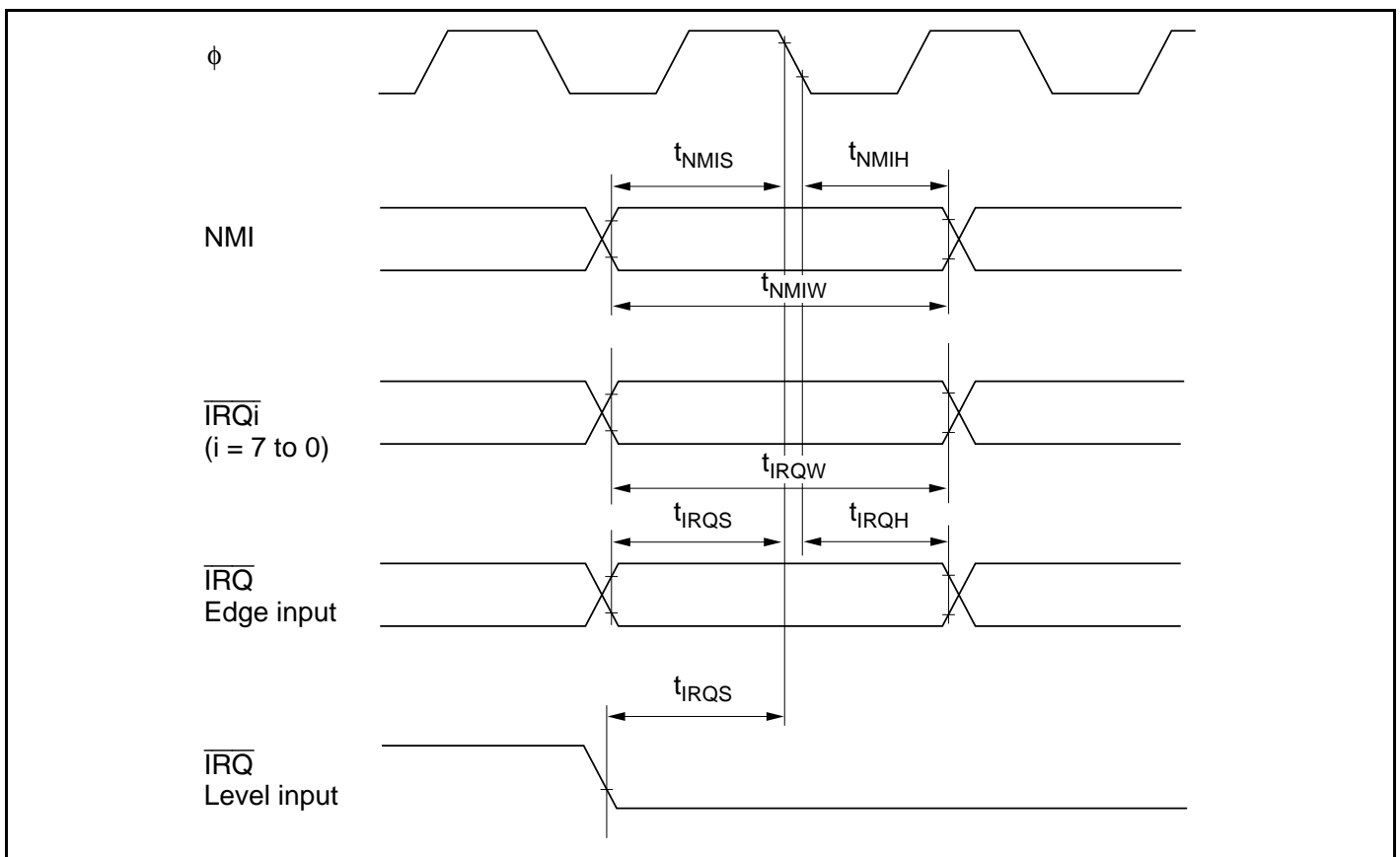
Figure 25.9 Interrupt Input Timing
