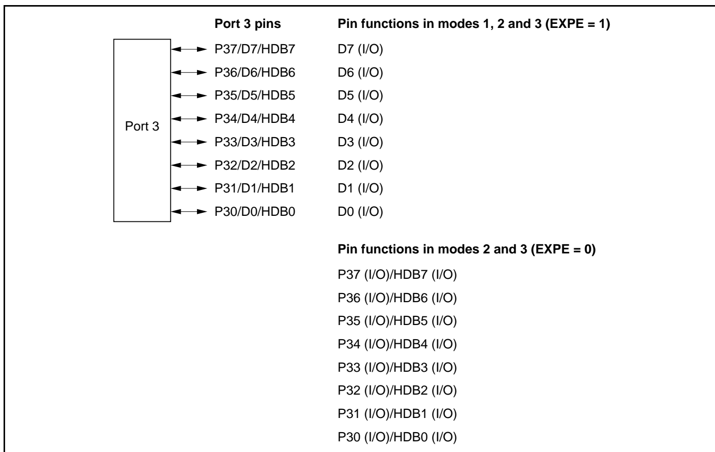
Figure 8.9 Port 3 Pin Functions
