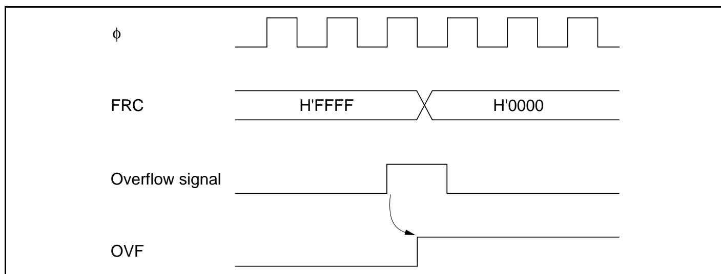
Figure 11.13 Setting of Overflow Flag (OVF)
