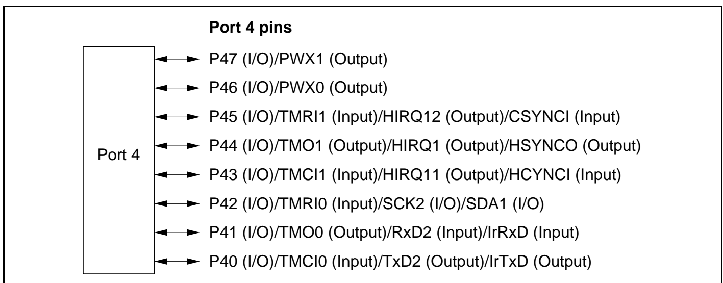
Figure 8.12 Port 4 Pin Functions
