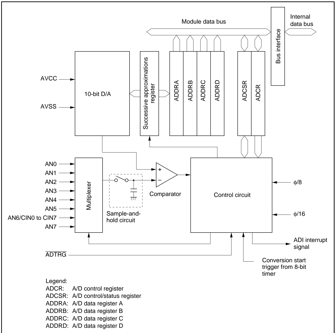
Figure 19.1 Block Diagram of A/D Converter
