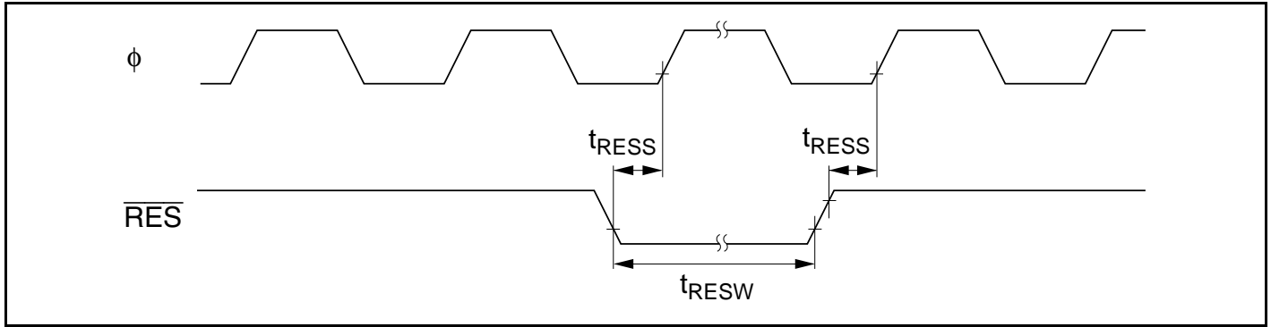
Figure 25.8 Reset Input Timing
