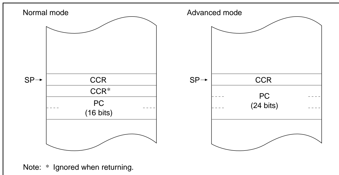
Figure 2.16 Stack Structure after Exception Handling (Examples)
