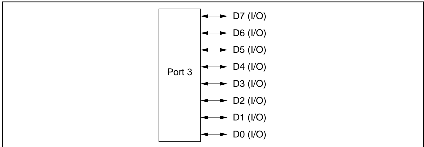
Figure 8.10 Port 3 Pin Functions (Modes 1, 2, and 3 (EXPE = 1))
