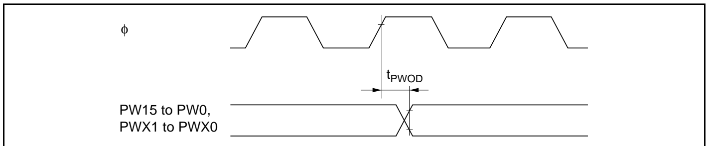
Figure 25.21 PWM, PWMX Output Timing
