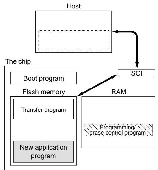
Figure 21.5 User Program Mode (Example)
