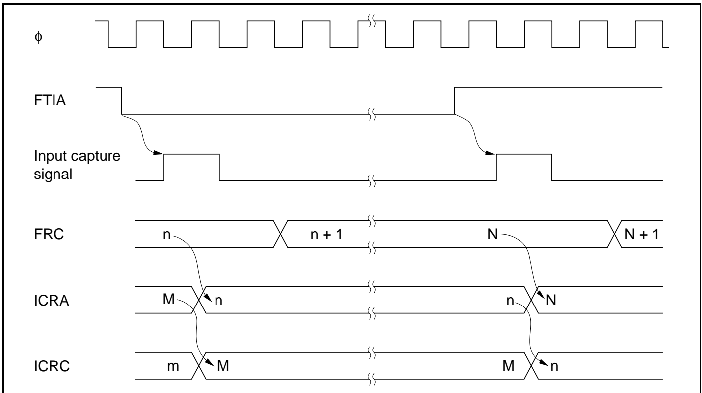
Figure 11.9 Buffered Input Capture Timing (Usual Case)
