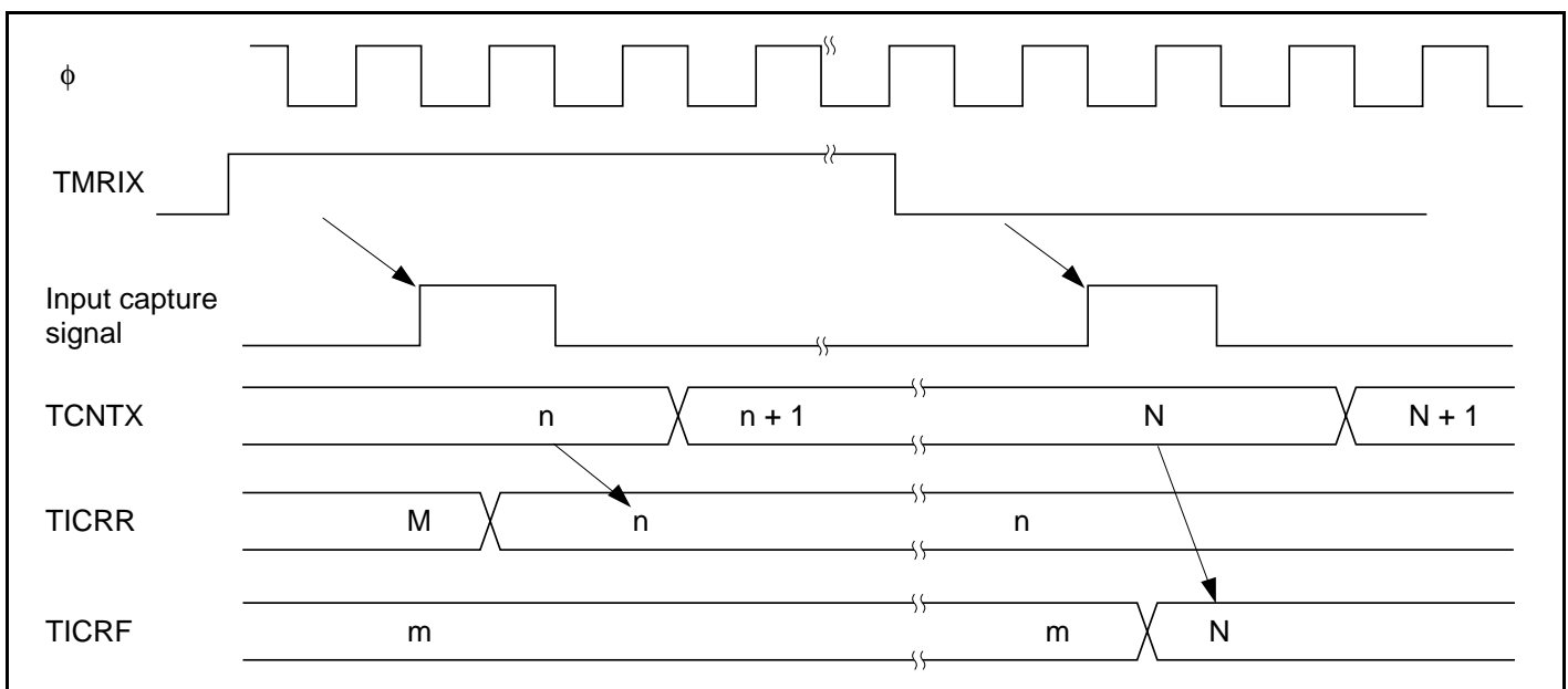
Figure 12.9 Timing of Input Capture Operation
