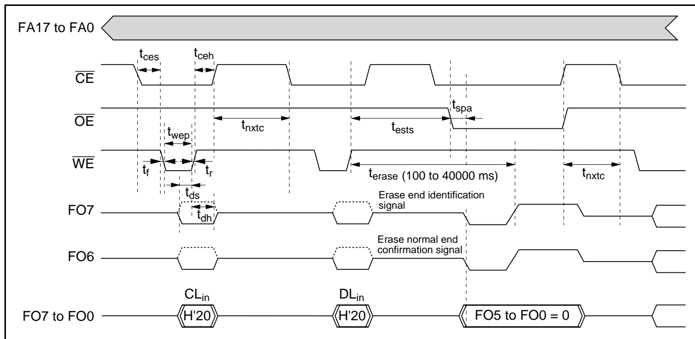
Figure 21.21 Auto-Erase Mode Timing Waveforms
