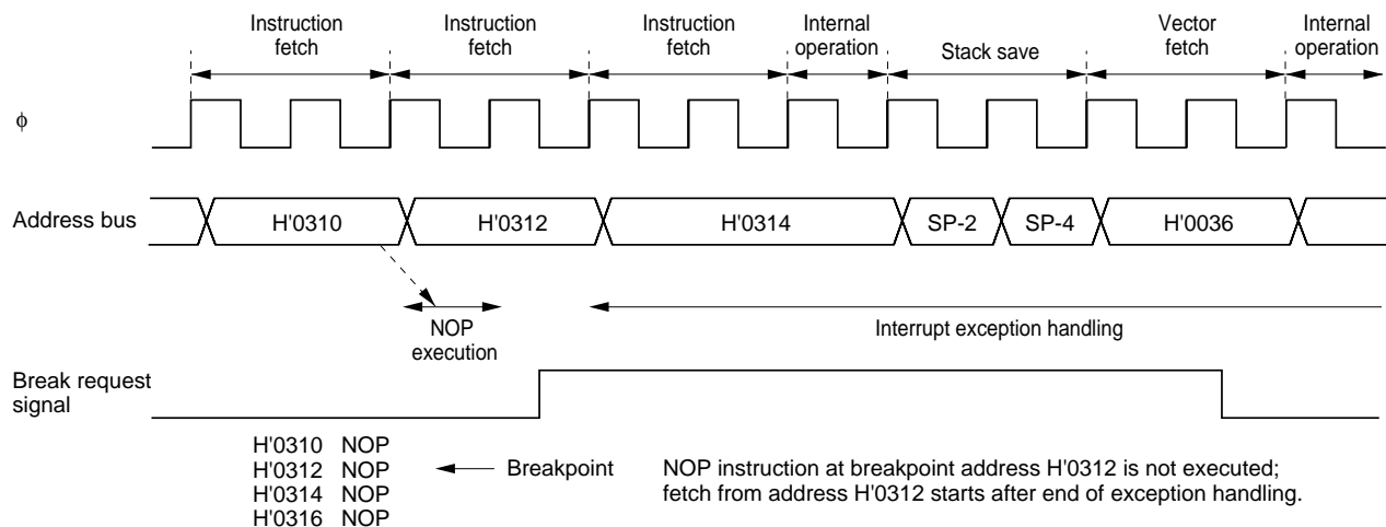
Figure 5.6 Examples of Address Break Timing
