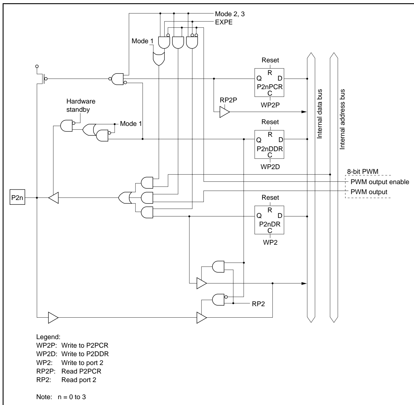
Figure C.2 Port 2 Block Diagram (Pins P20 to P23)
