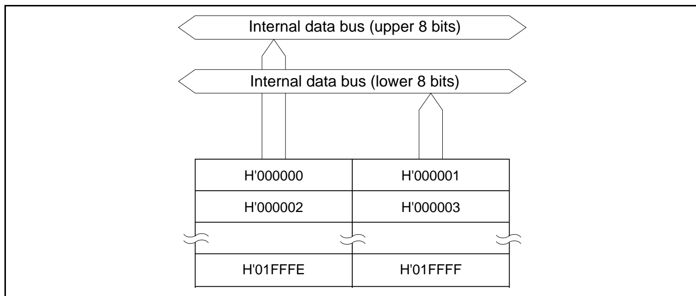
Figure 21.1 ROM Block Diagram (H8S/2138, H8S/2134)
