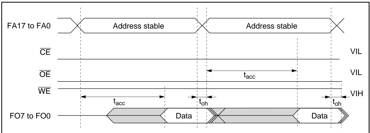
Figure 22.18 Timing Waveforms for \overline{\text{CE}}/\overline{\text{OE}} Enable State Read
