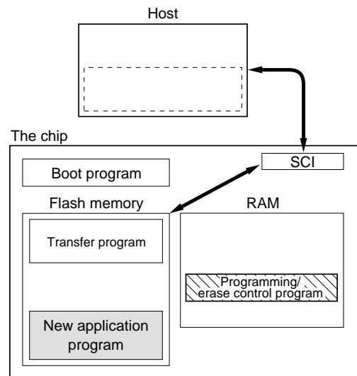
Figure 22.5 User Program Mode (Example)
