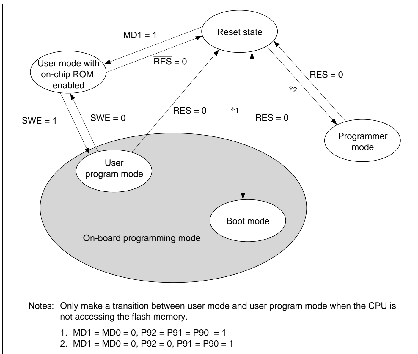
Figure 21.3 Flash Memory Mode Transitions
