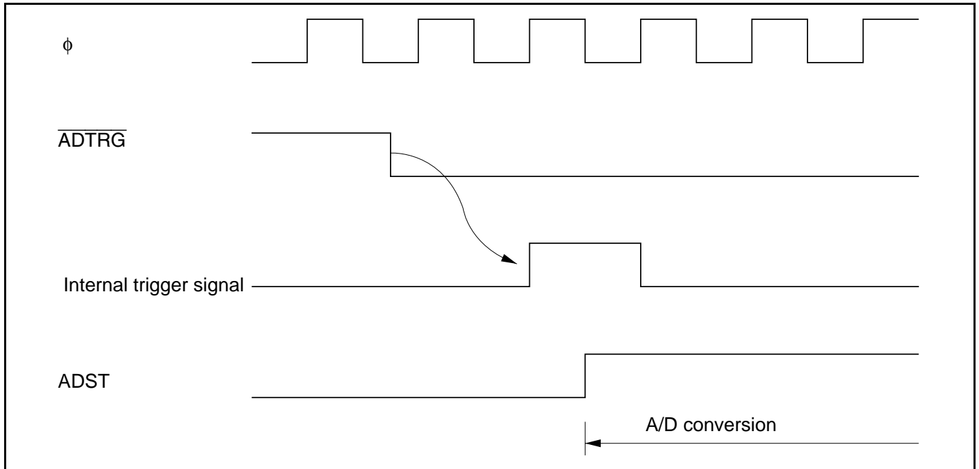
Figure 19.6 External Trigger Input Timing
