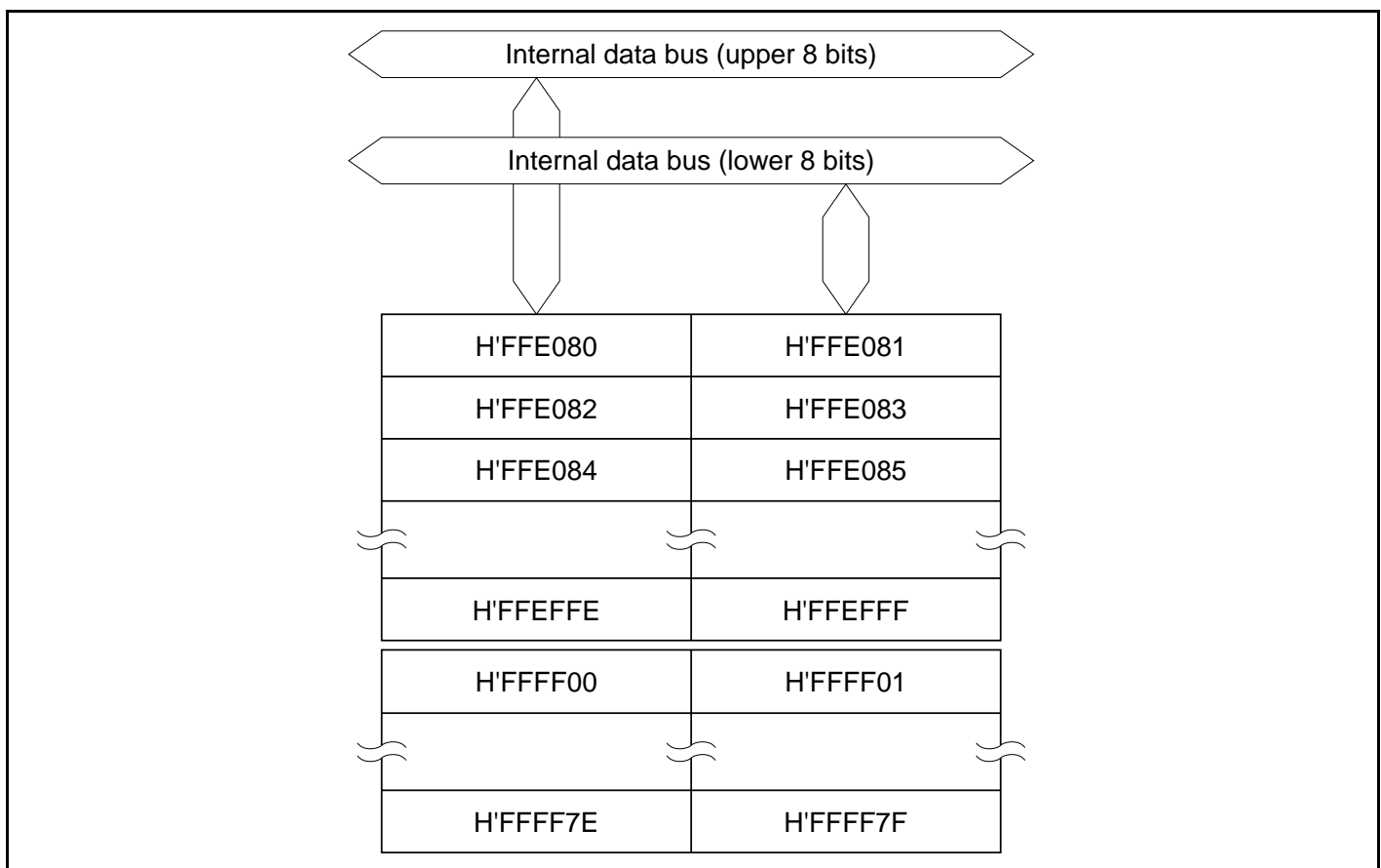
Figure 20.1 Block Diagram of RAM (H8S/2138, H8S/2134, H8S/2133)
