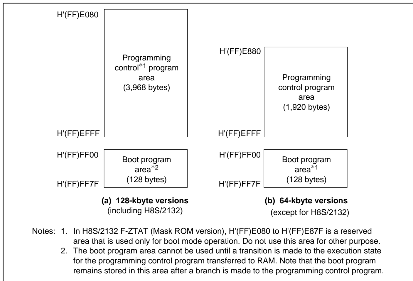
Figure 21.10 RAM Areas in Boot Mode
