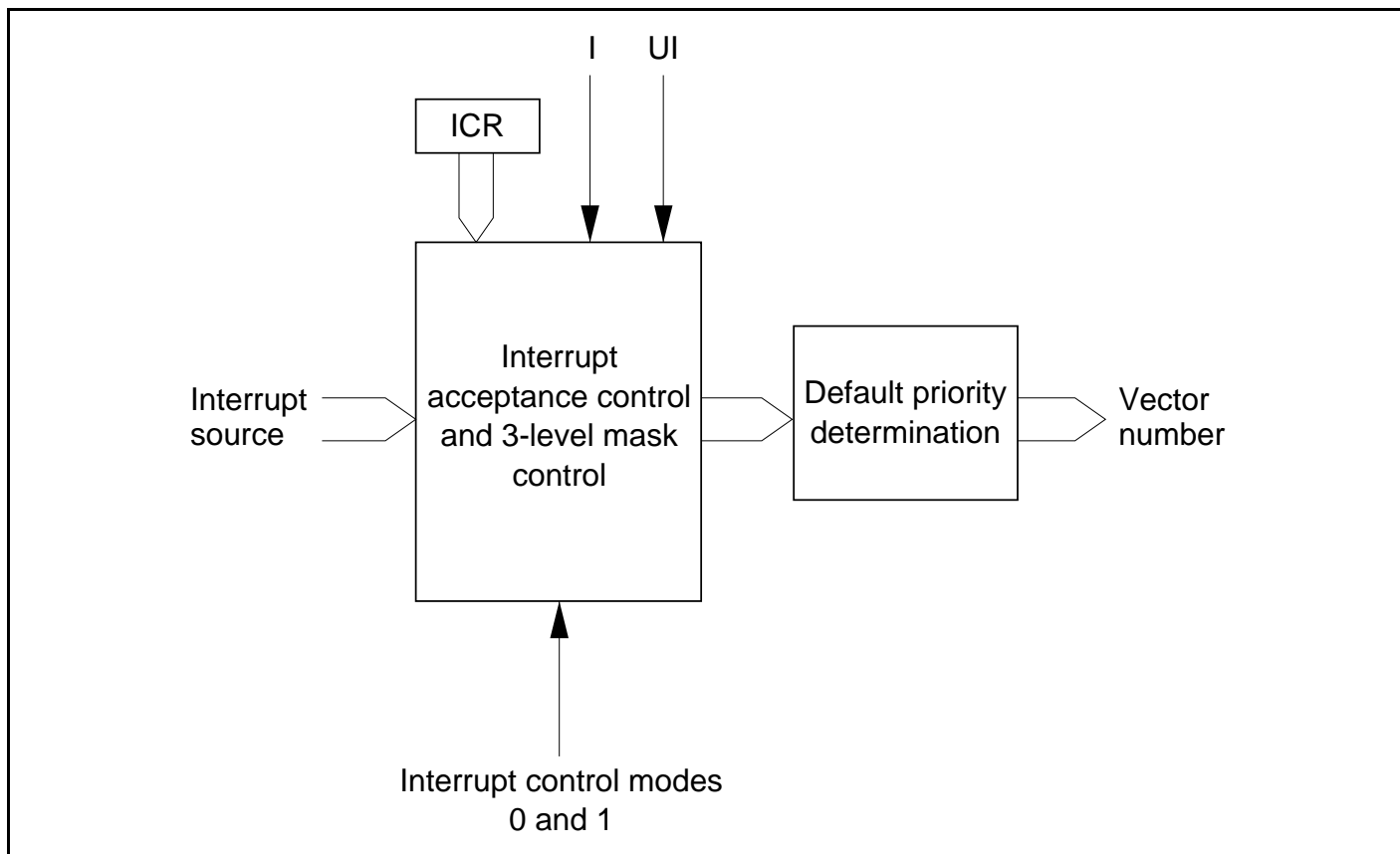
Figure 5.7 Block Diagram of Interrupt Control Operation
