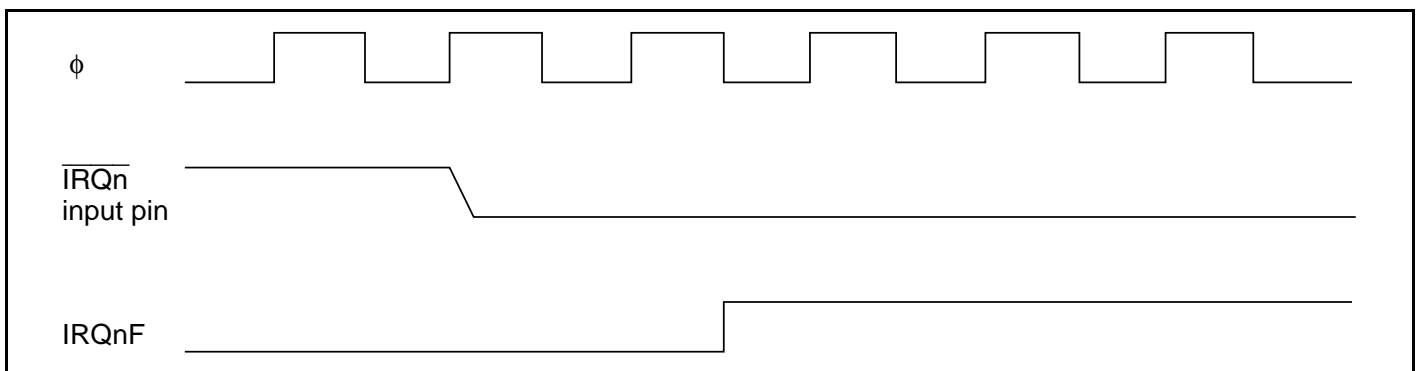
Figure 5.4 Timing of \text{IRQnF} Setting
