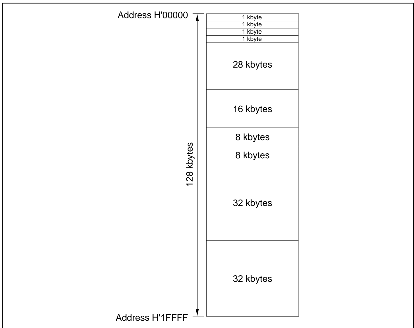
Figure 22.6 Flash Memory Block Configuration
