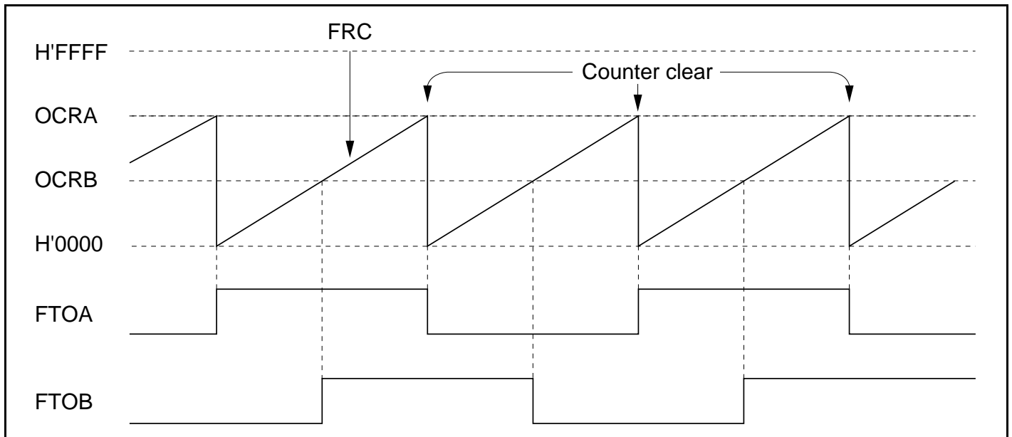
Figure 11.17 Pulse Output (Example)
