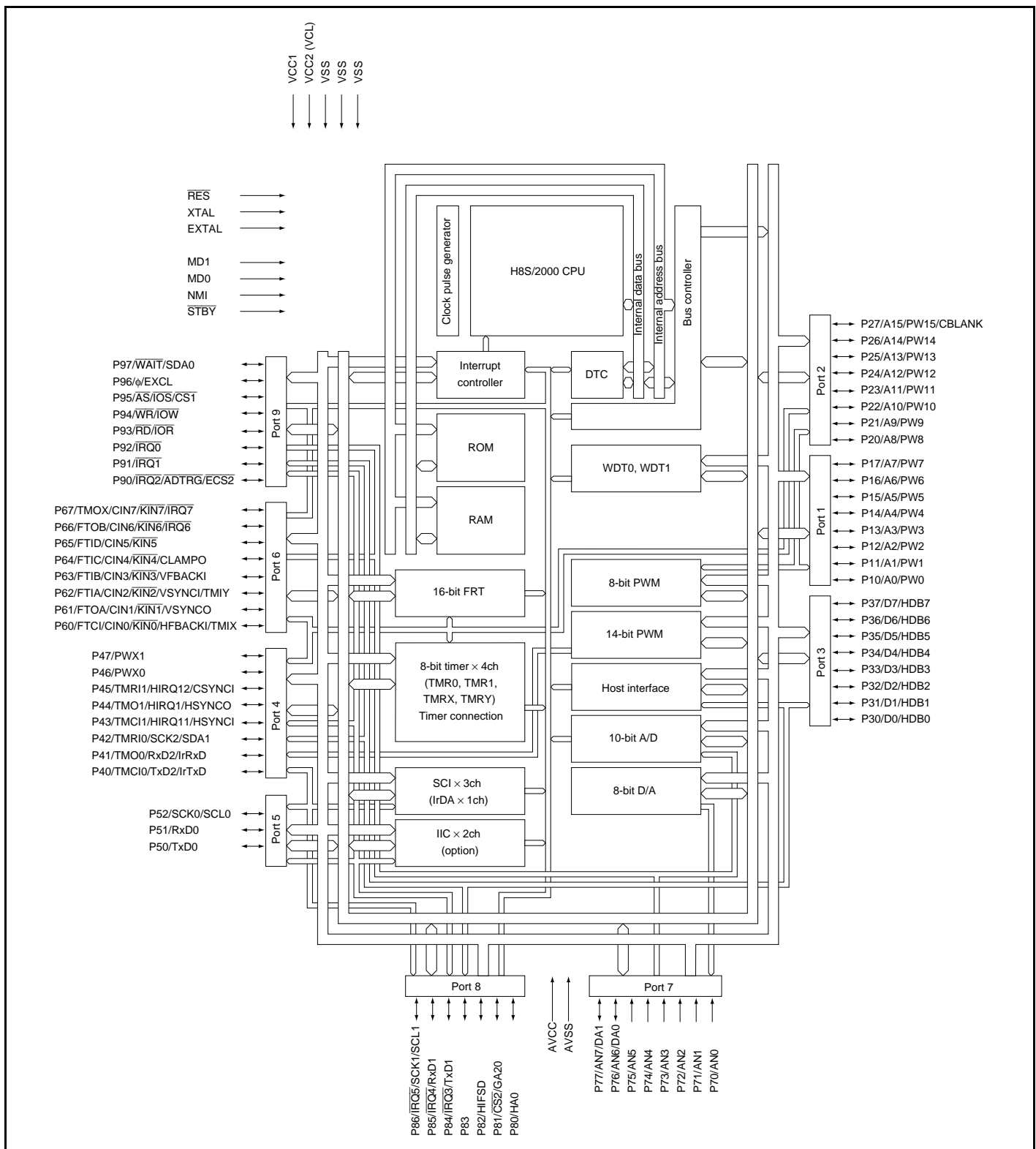
Figure 1.1 Internal Block Diagram of H8S/2138 Group
