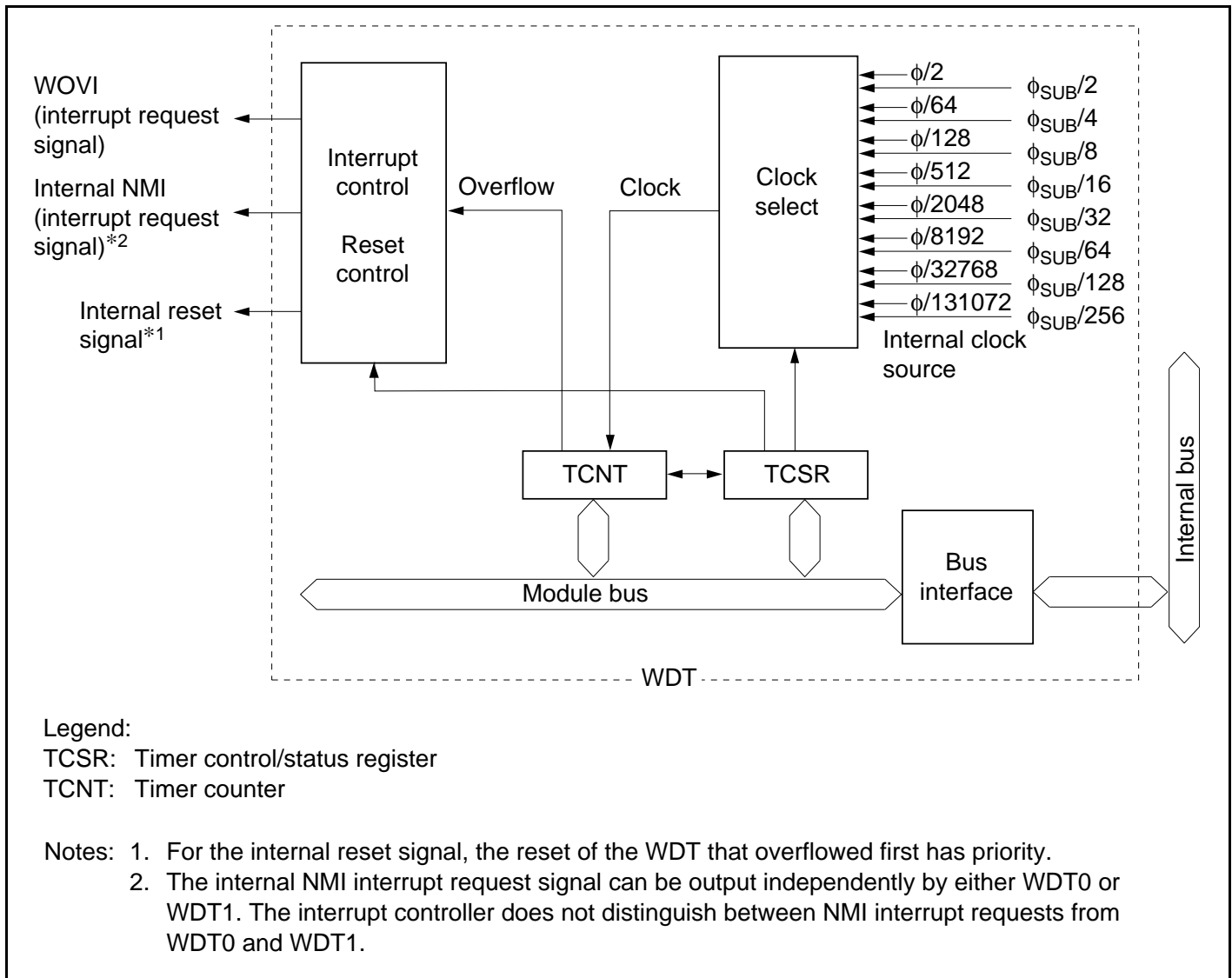
Figure 14.1 (b) Block Diagram of WDT1
