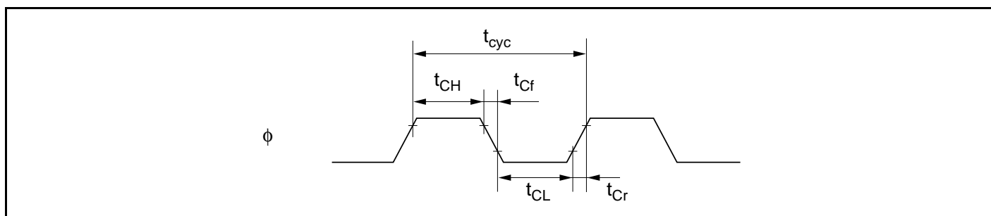
Figure 25.5 System Clock Timing
