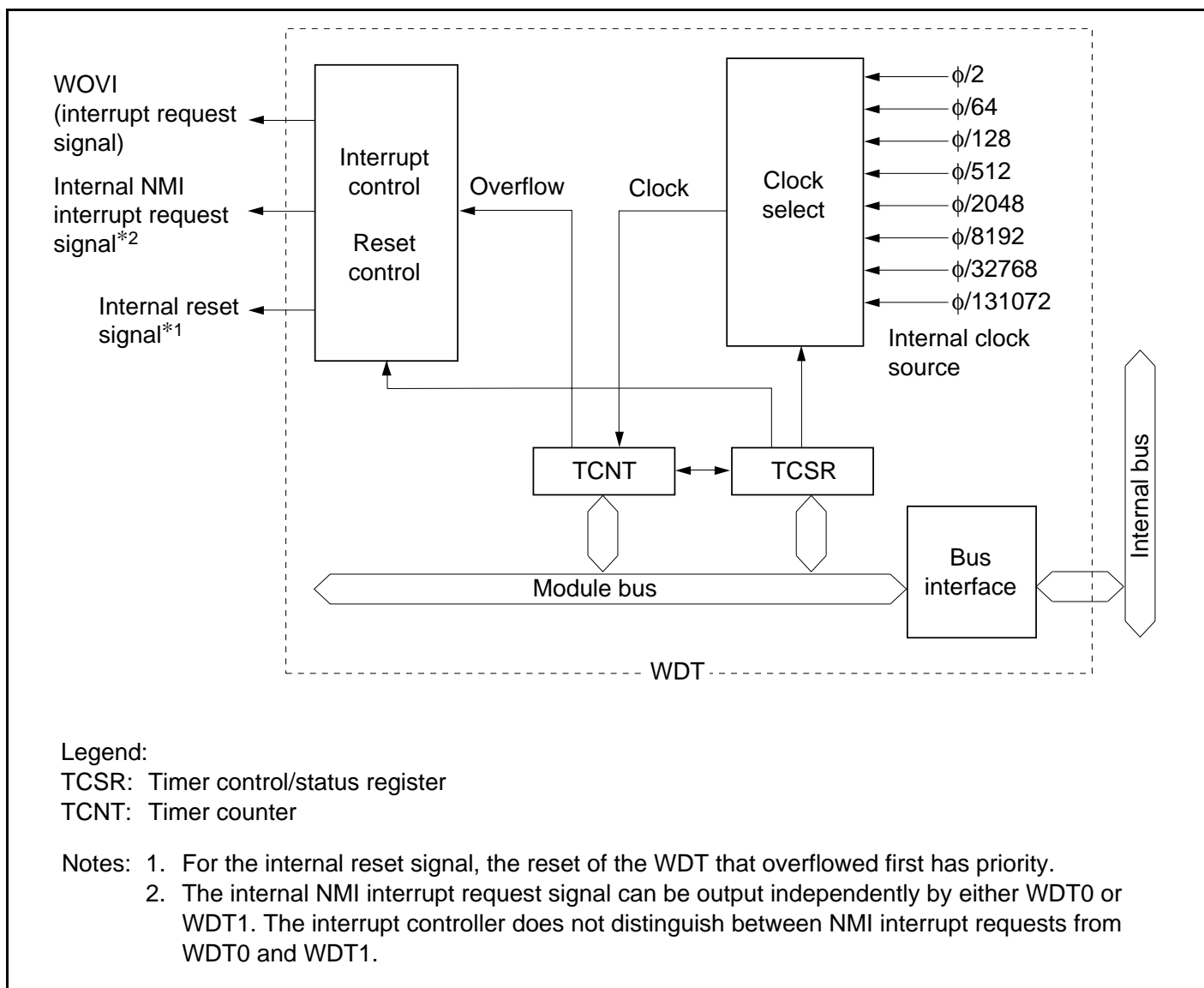
Figure 14.1 (a) Block Diagram of WDT0
