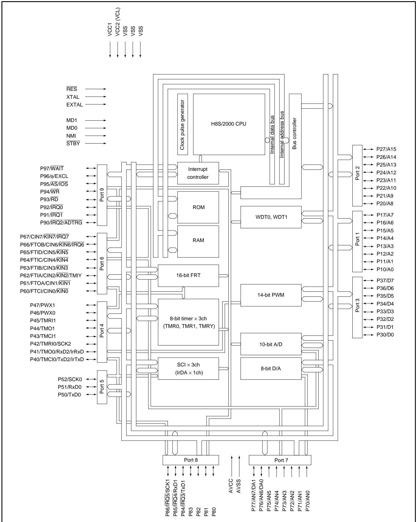
Figure 1.2 Internal Block Diagram of H8S/2134 Group
