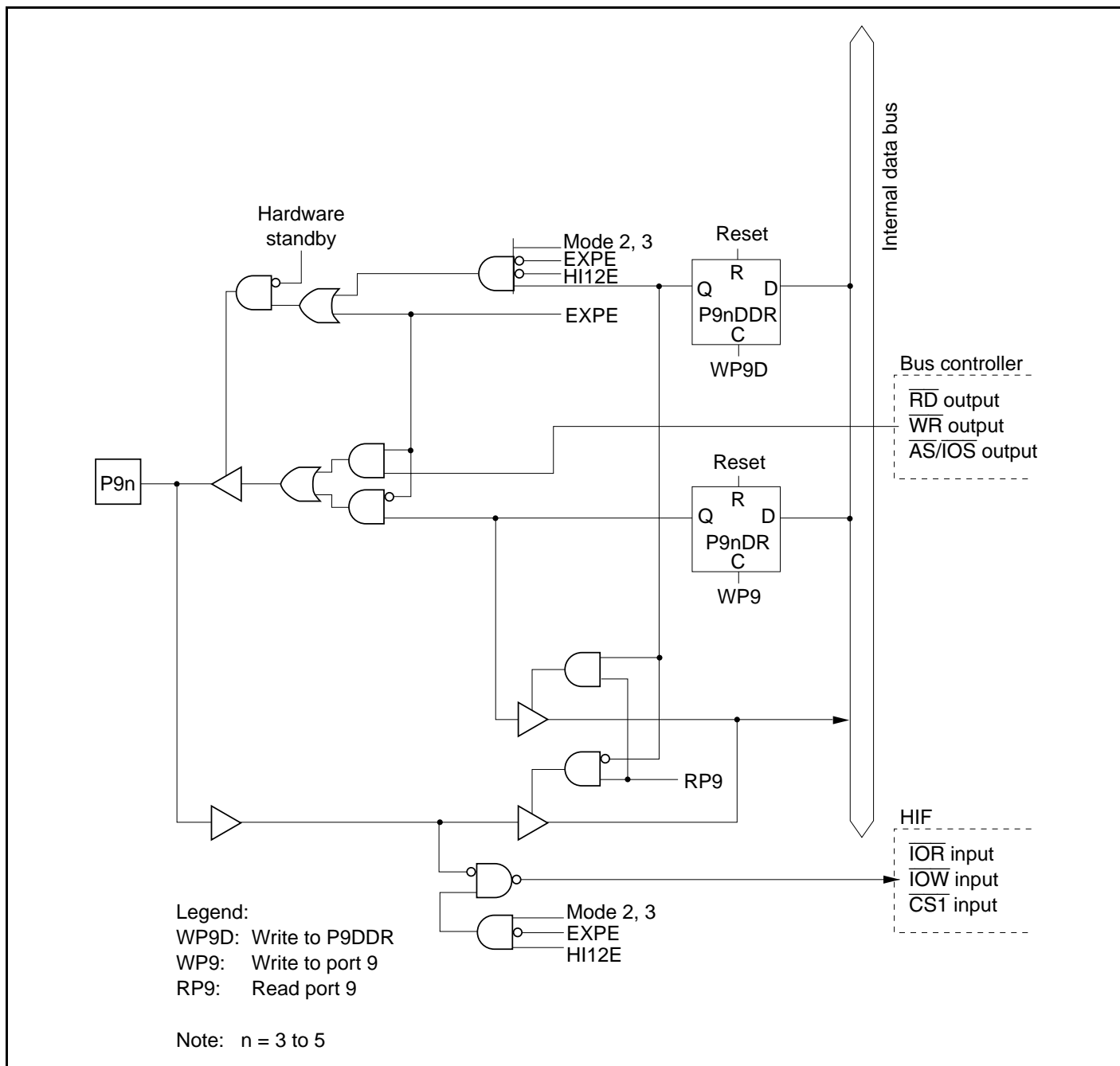
Figure C.31 Port 9 Block Diagram (Pins P93 to P95)
