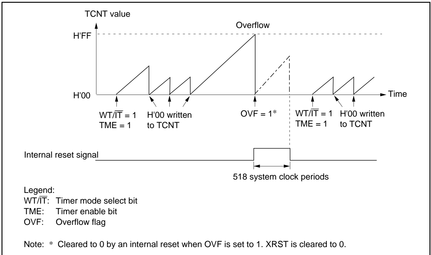
Figure 14.3 Operation in Watchdog Timer Mode
