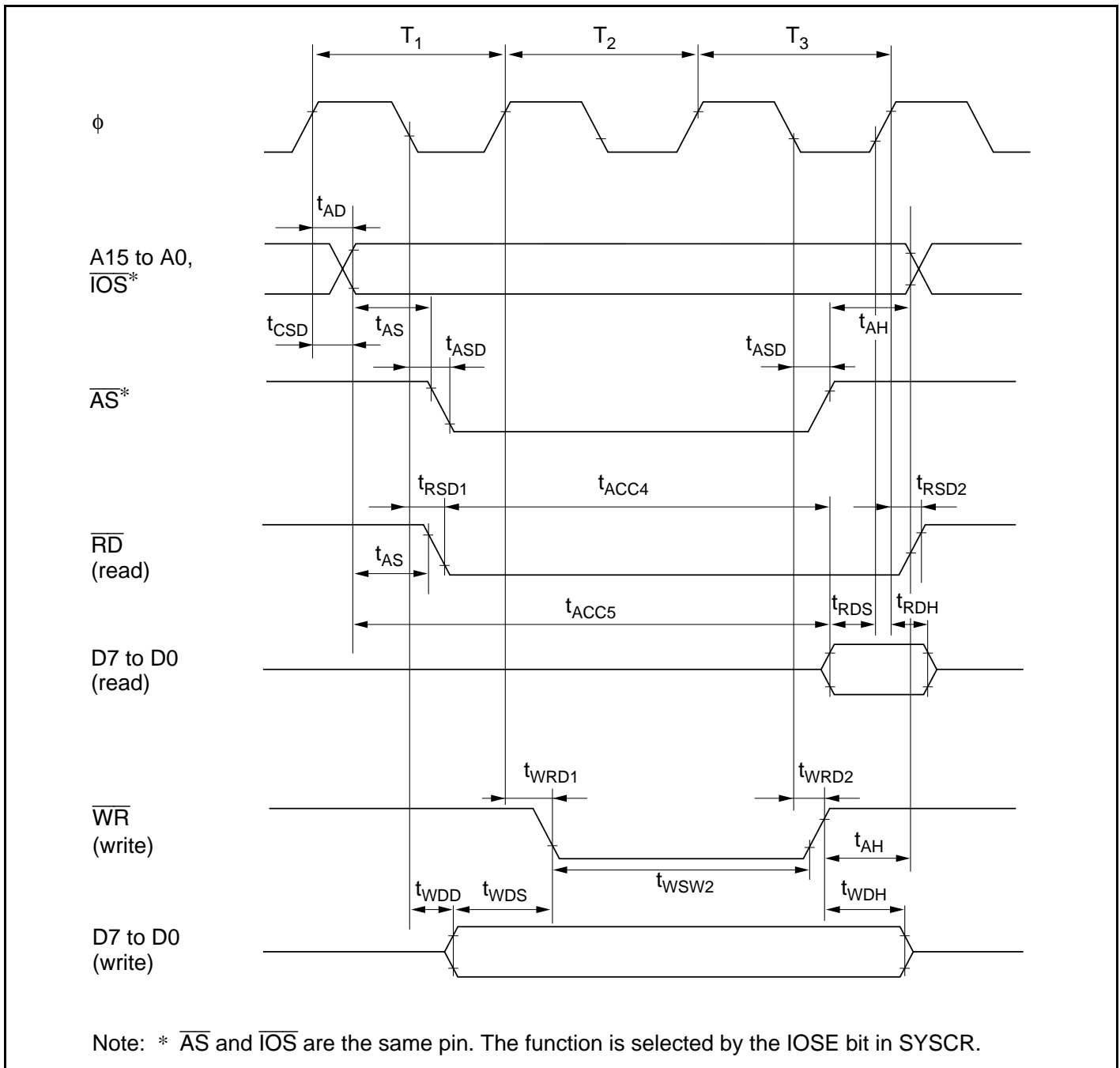
Figure 25.11 Basic Bus Timing (Three-State Access)
