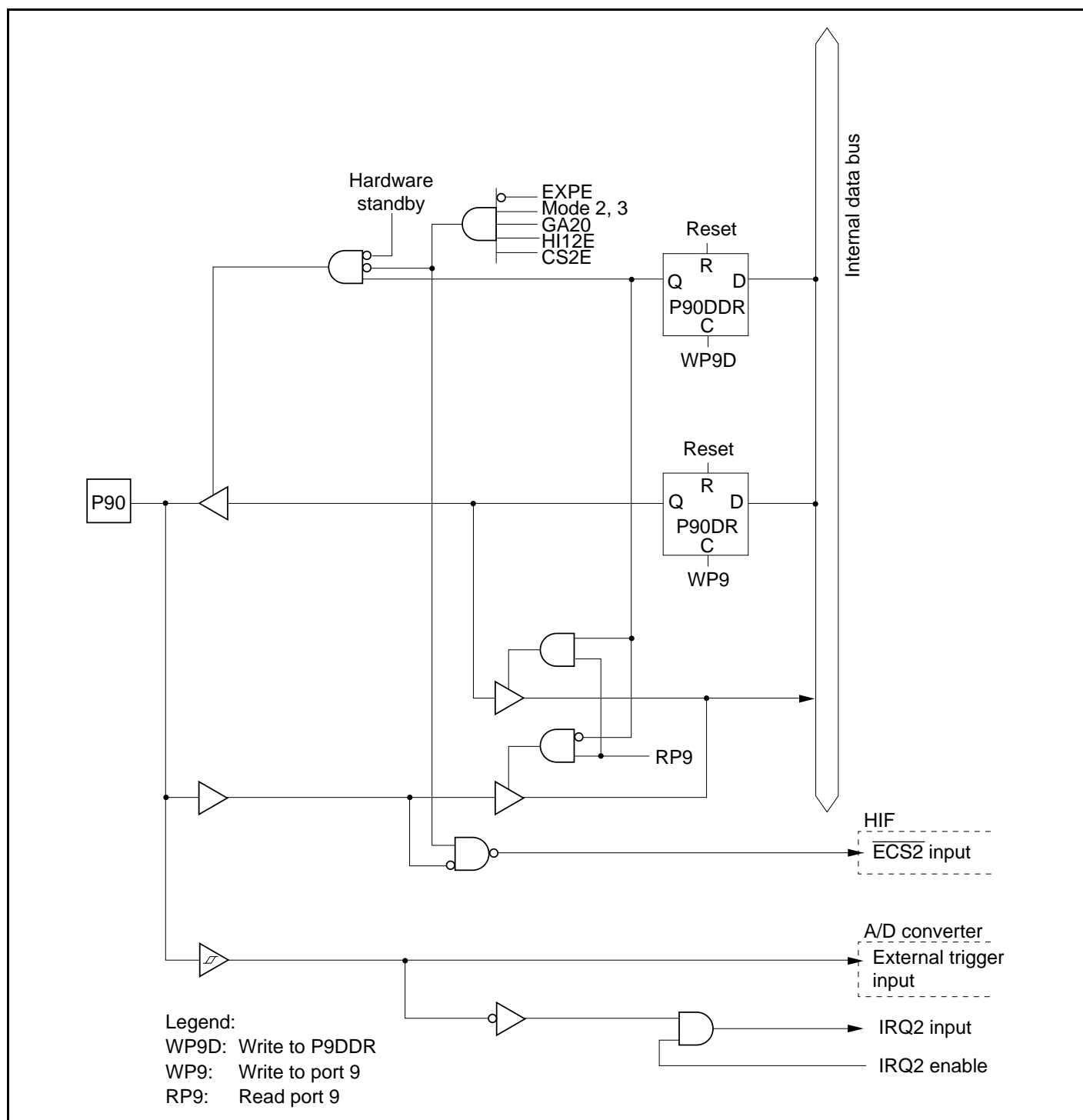
Figure C.29 Port 9 Block Diagram (Pin P90)
