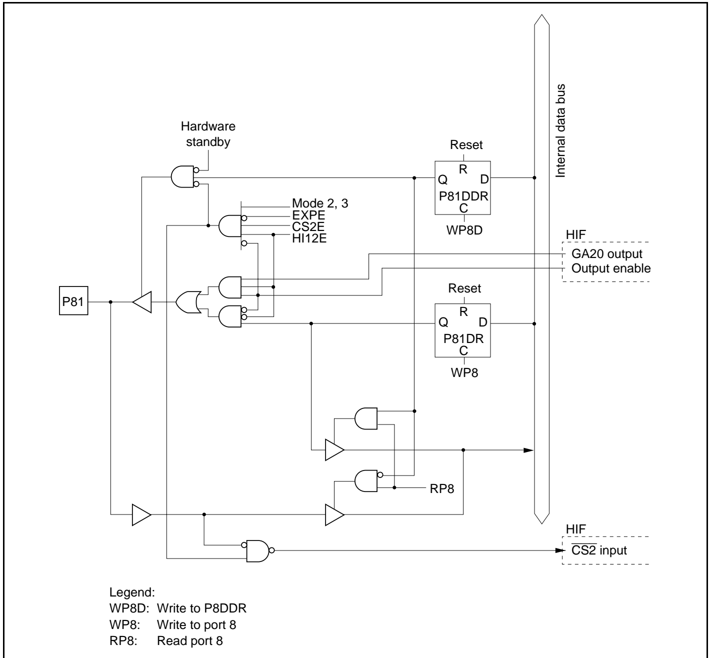
Figure C.24 Port 8 Block Diagram (Pin P81)
