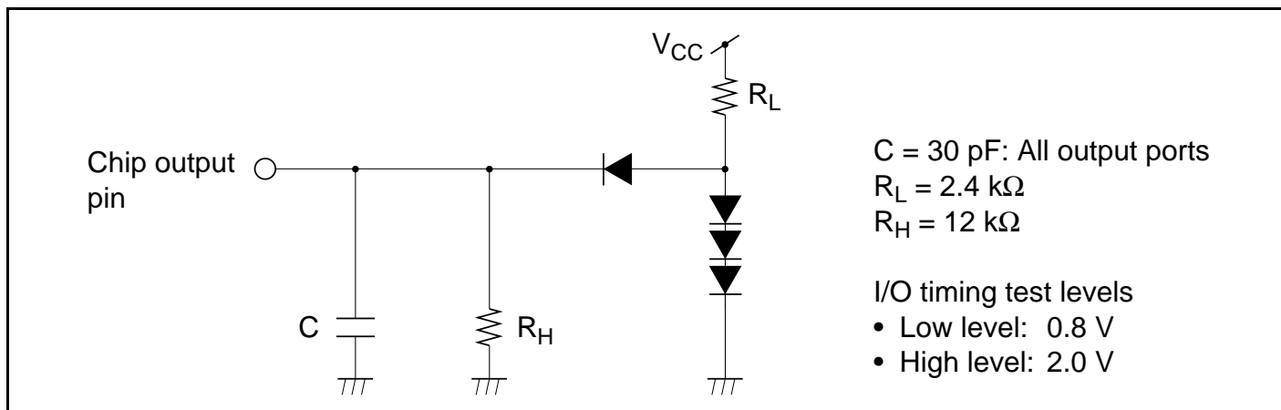
Figure 25.4 Output Load Circuit
