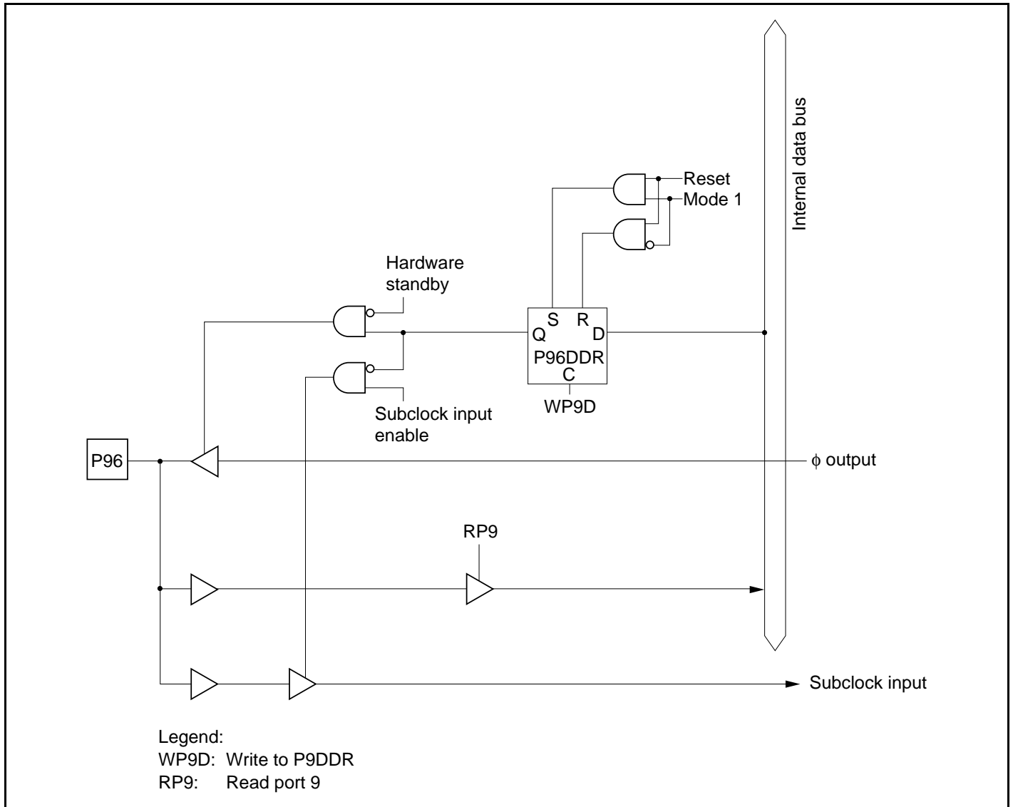
Figure C.32 Port 9 Block Diagram (Pin P96)
