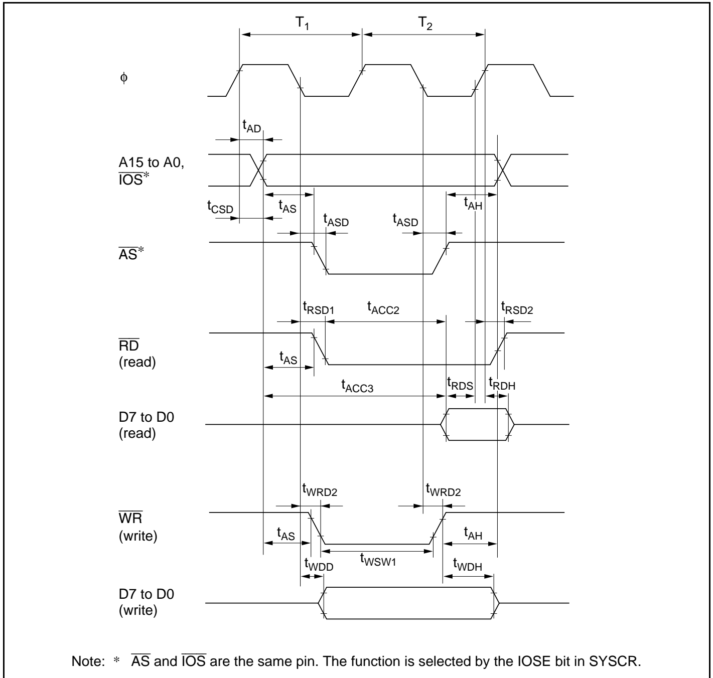
Figure 25.10 Basic Bus Timing (Two-State Access)
