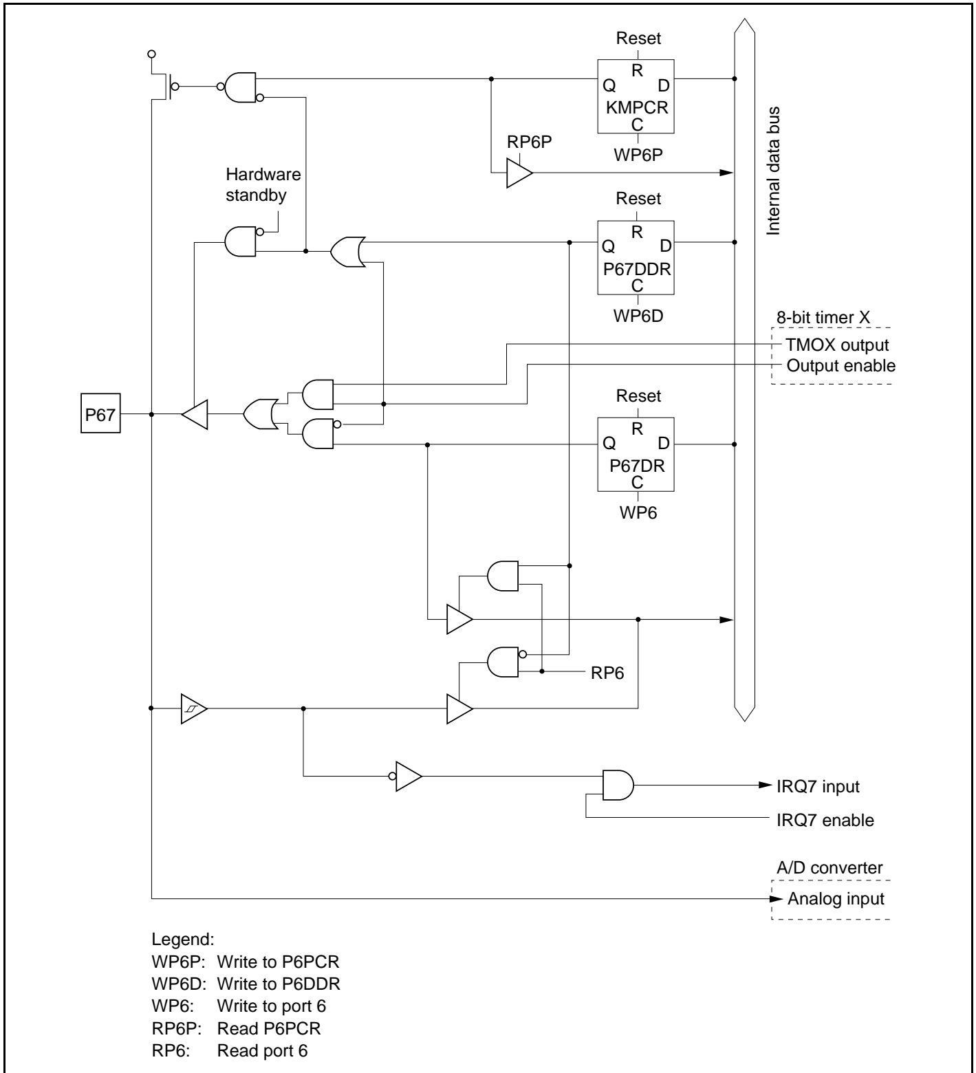
Figure C.20 Port 6 Block Diagram (Pin P67)
