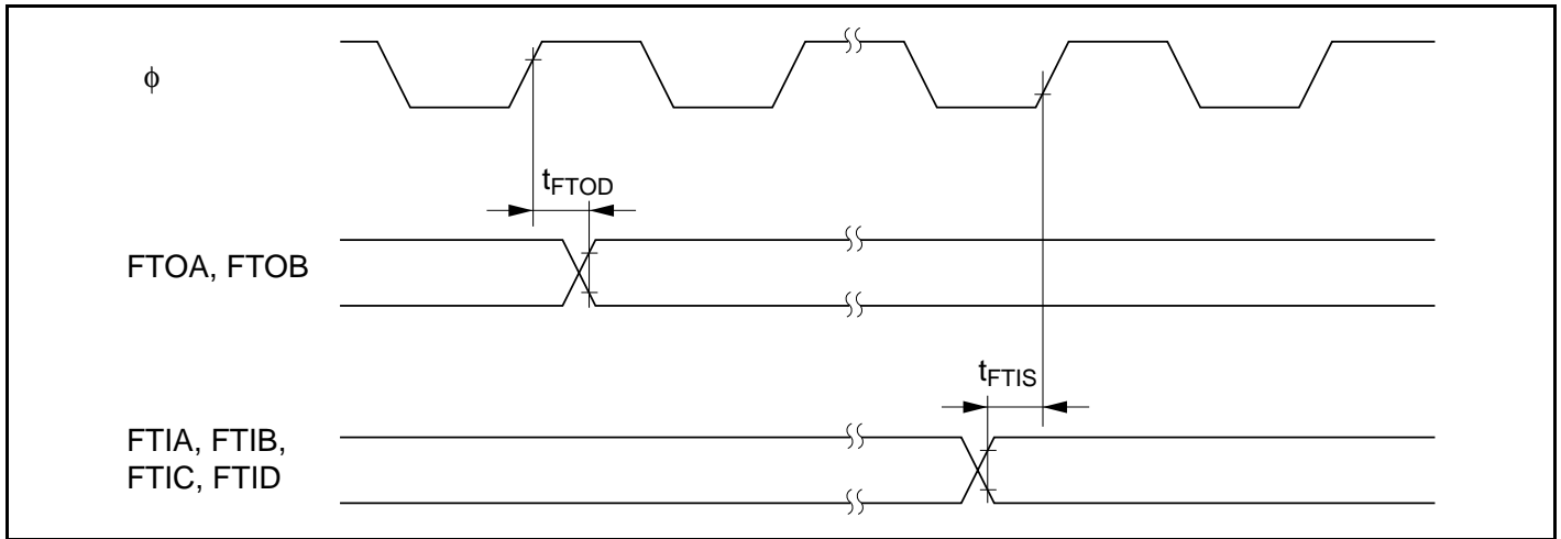
Figure 25.16 FRT Input/Output Timing
