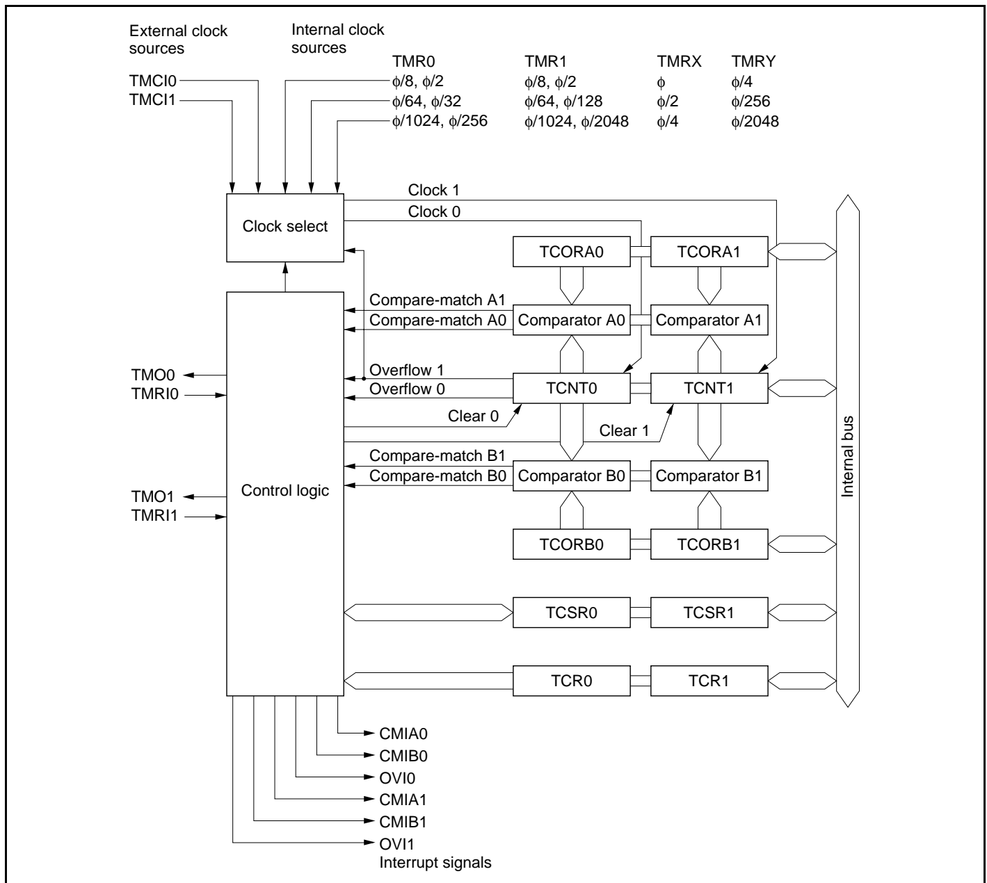
Figure 12.1 Block Diagram of 8-Bit Timer Module
