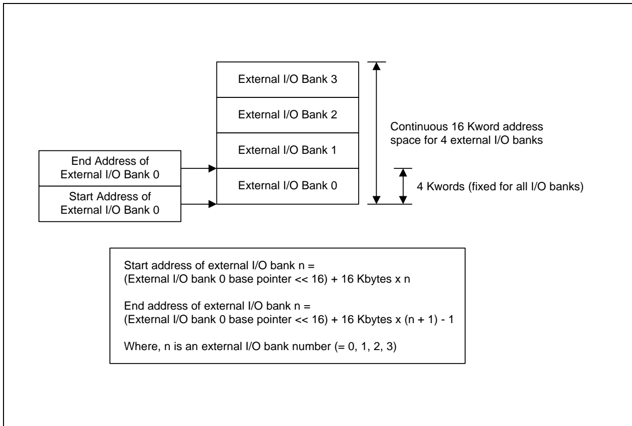
Figure 4-38. External I/O Bank Address Map
