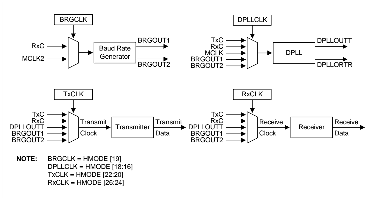
Figure 8-4. Clock Usage Method Diagram
