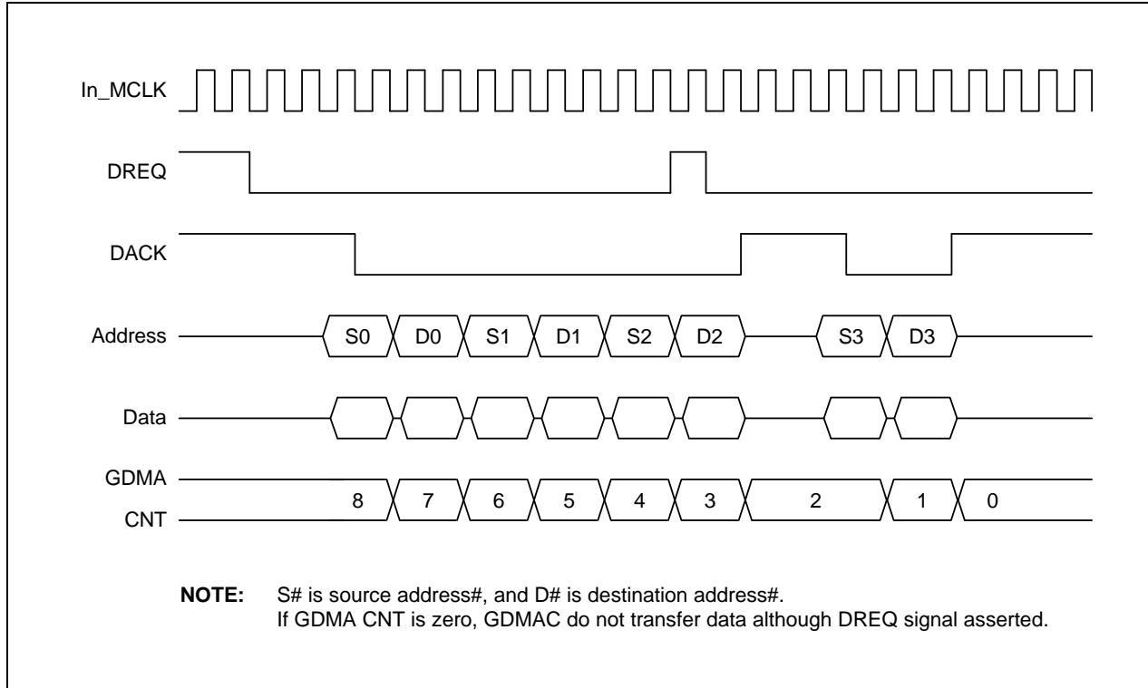
Figure 9-15. Demand and One Data Burst Mode Timing
