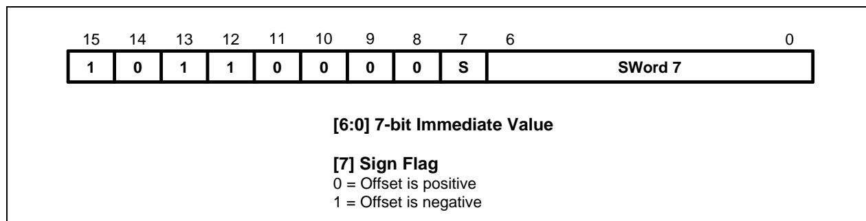
Figure 3-42. Format 13
