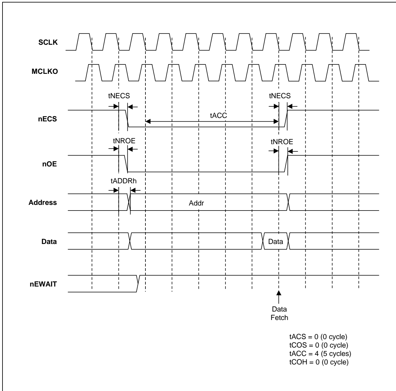
Figure 4-11. External I/O Read Timing 1
