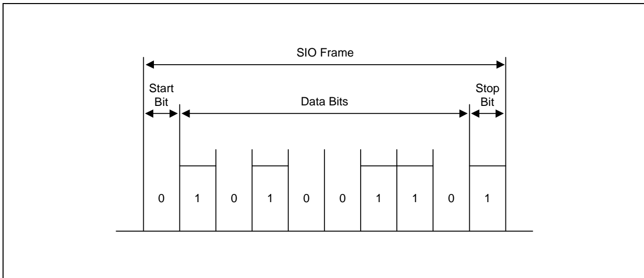
Figure 10-13. Serial I/O Frame Timing Diagram (Normal UART)
