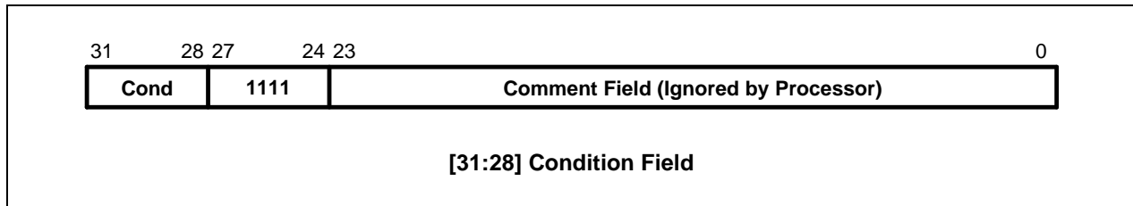
Figure 3-24. Software Interrupt Instruction
