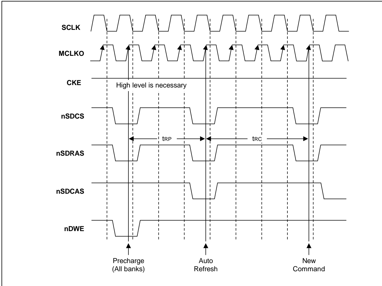
Figure 4-40. Auto Refresh Cycle of SDRAM
