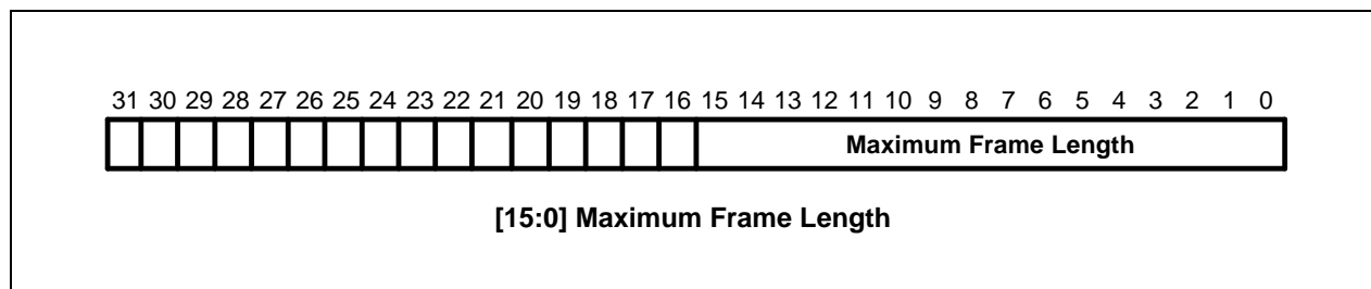
Figure 8-27. Maximum Frame Length Register
