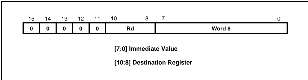
Figure 3-35. Format 6
