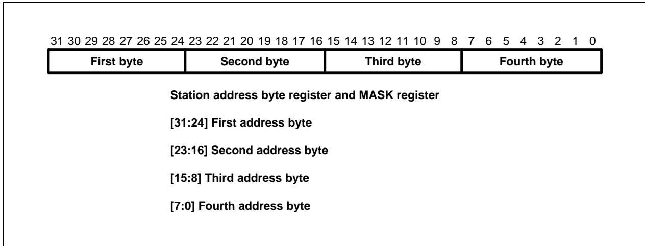
Figure 8-24. HDLC Station Address and HMASK Register
