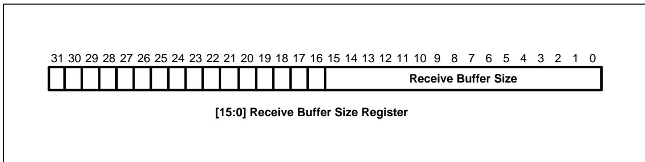
Figure 8-28. DMA Receive Buffer Size Register
