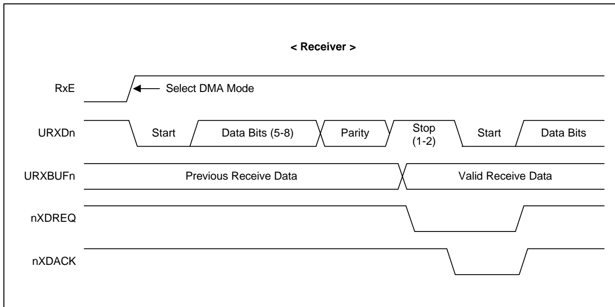
Figure 10-12. DMA-Based Serial I/O Timing Diagram (Rx Only)
