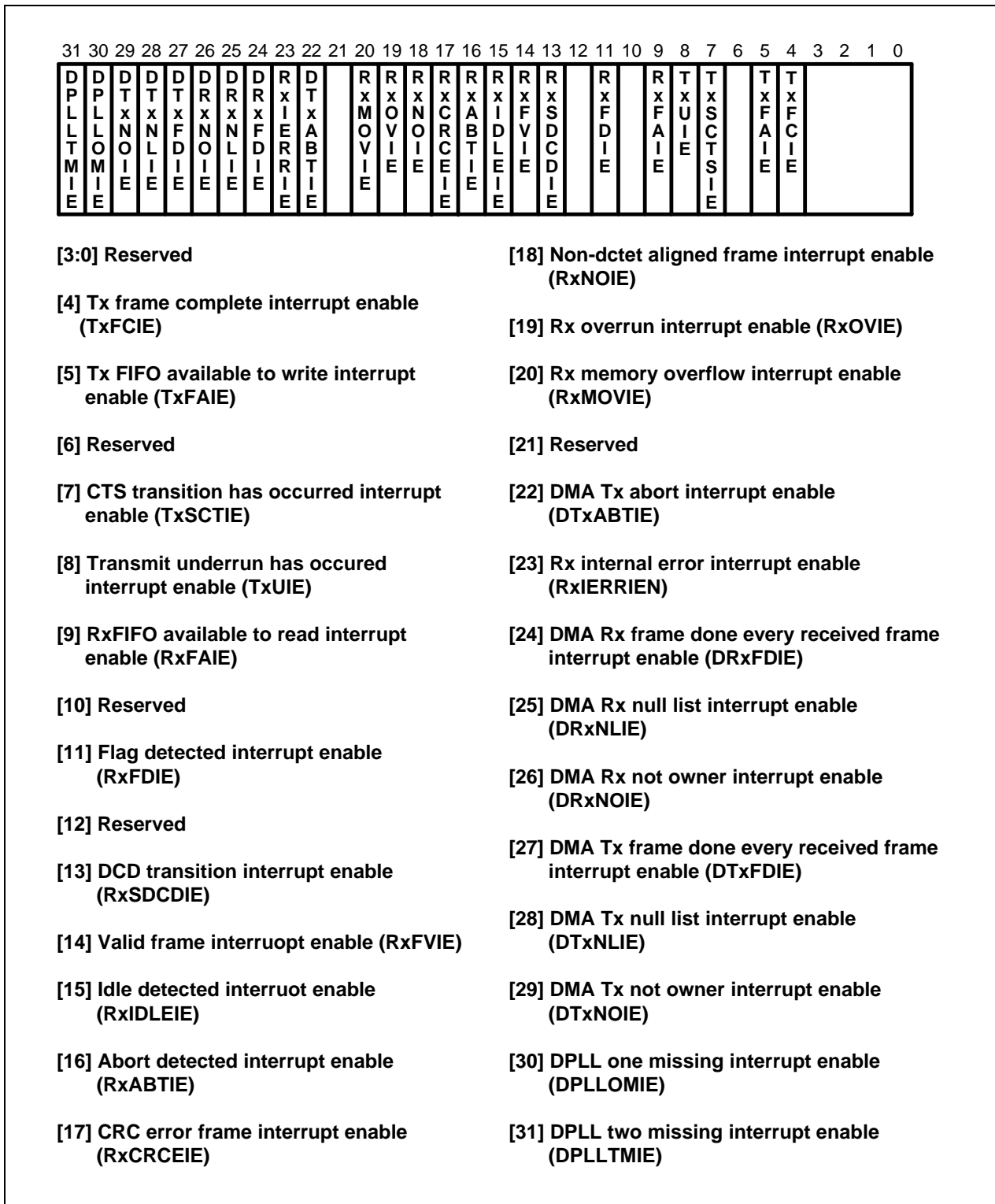
Figure 8-18. HDLC Interrupt Enable Register
