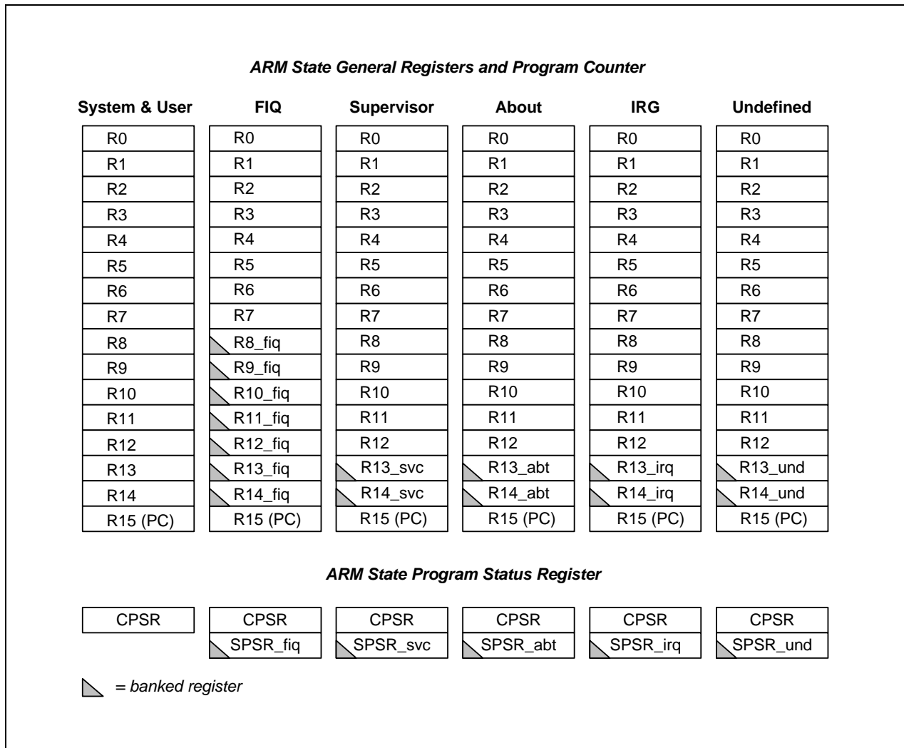
Figure 2-3. Register Organization in ARM State
