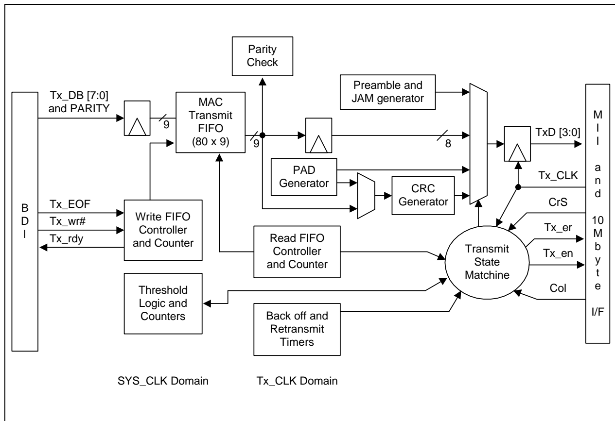
Figure 7-3. MAC Transmit Function Blocks
