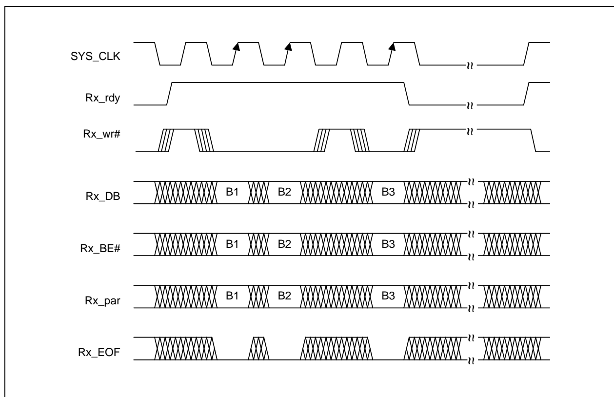
Figure 7-17. BDI Transmit Data Timing
