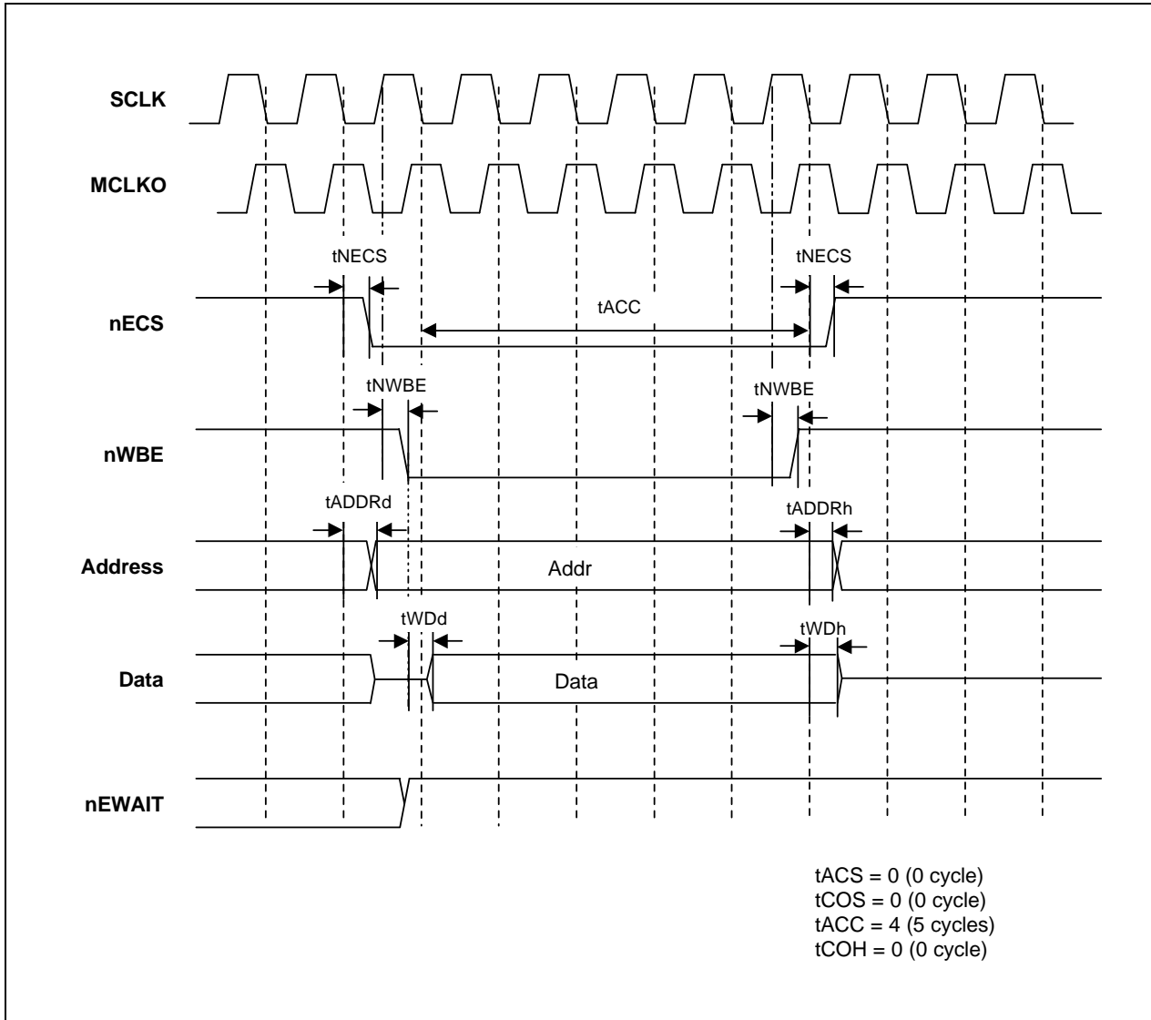
Figure 4-14. External I/O Write Timing 1
