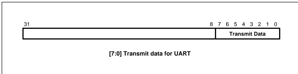
Figure 10-5. UART Transmit Buffer Registers
