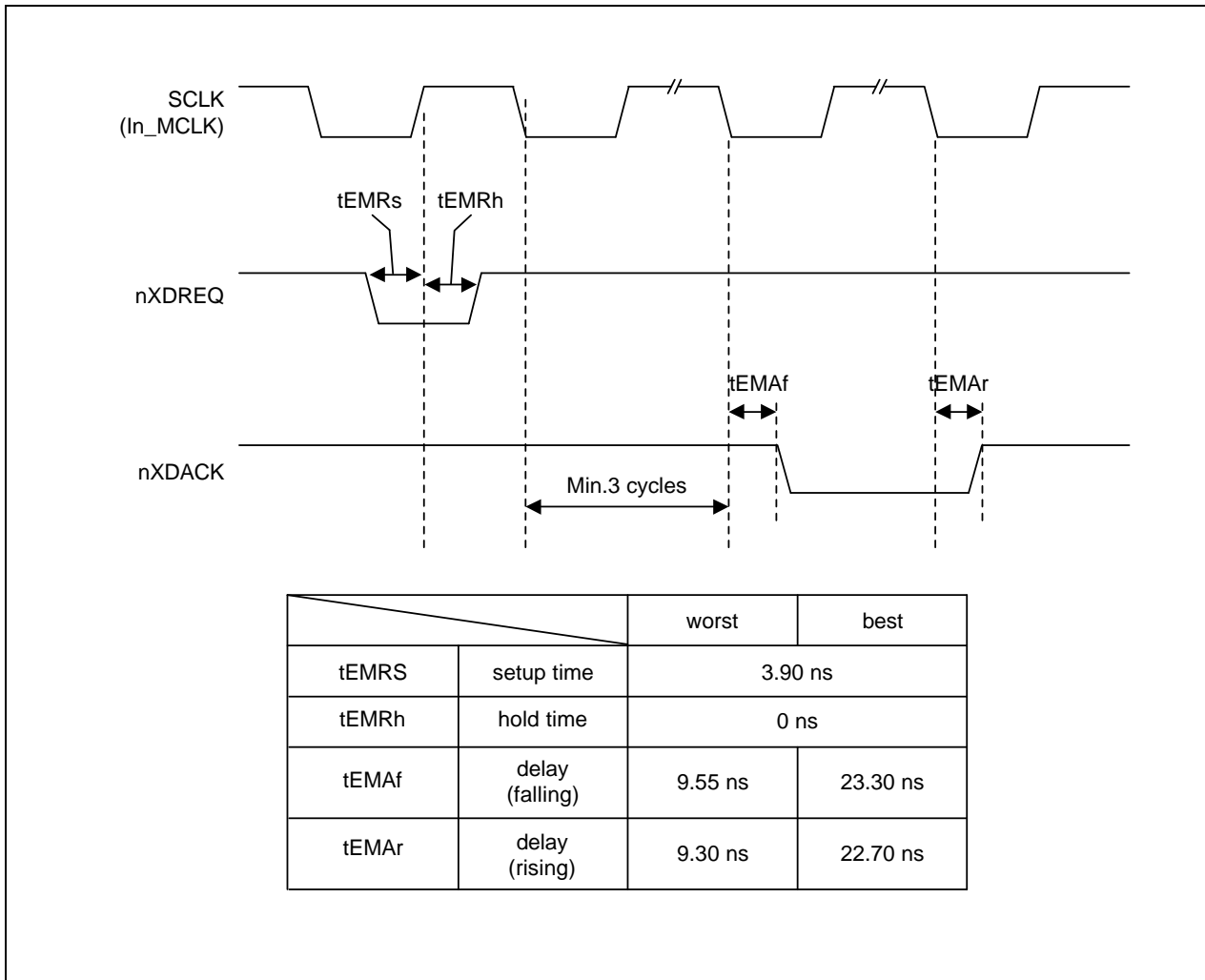
Figure 9-8. External DMA Requests Detailed Timing (S3C4510X)
