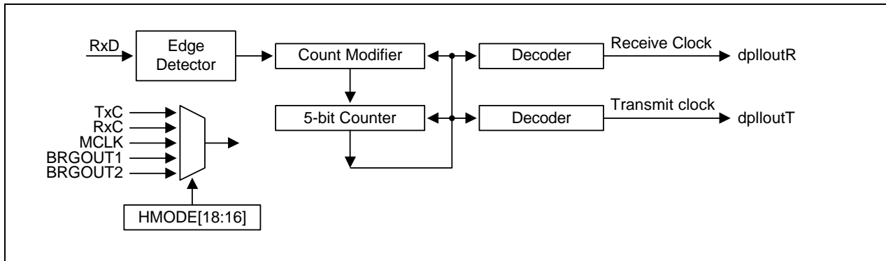
Figure 8-3. DPLL Block Diagram
