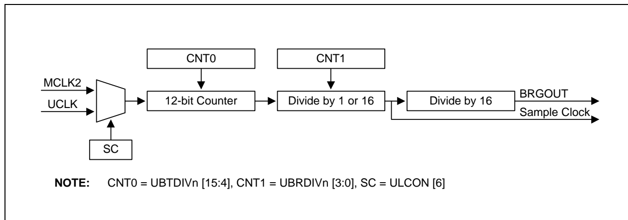
Figure 10-9. UART Baud Rate Generator (BRG)
