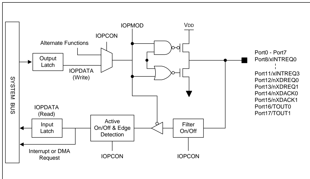
Figure 12-1. I/O Port Function Diagram
