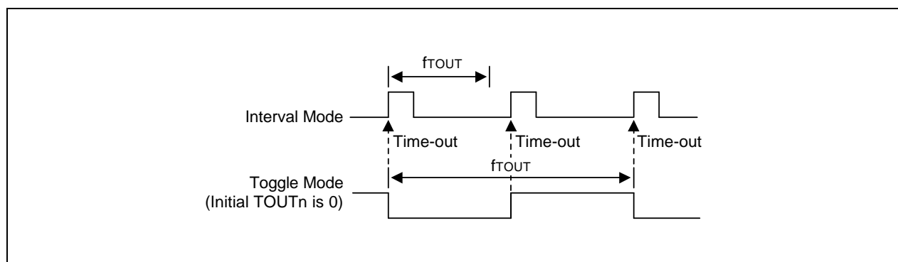
Figure 11-1. Timer Output Signal Timing
