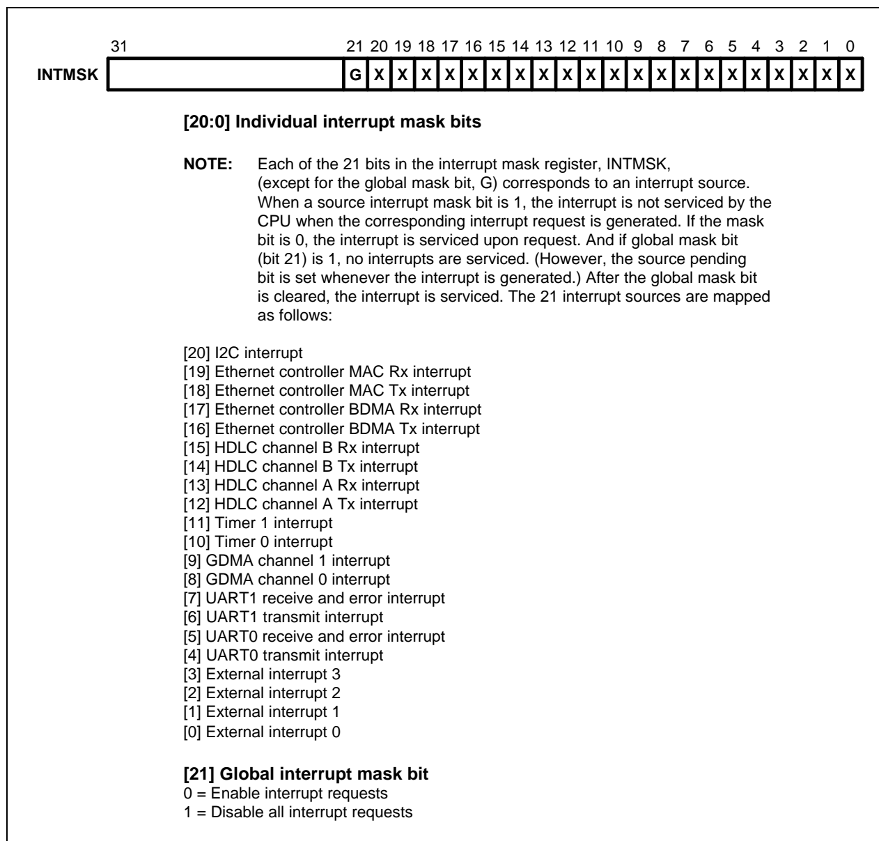
Figure 13-3. Interrupt Mask Register (INTMSK)
