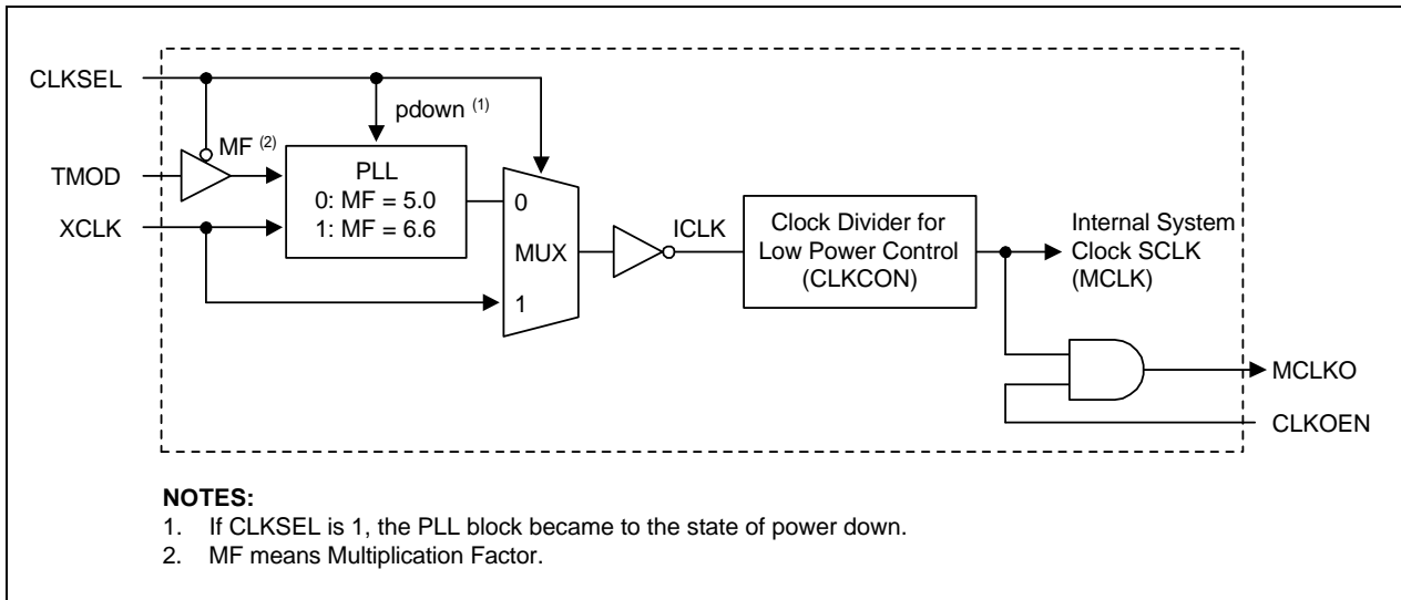
Figure 4-8. System Clock Circuit
