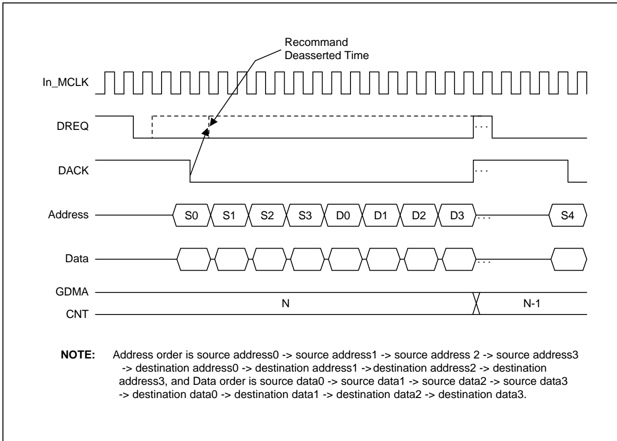
Figure 9-12. Single and Four Data Burst Mode Timing
