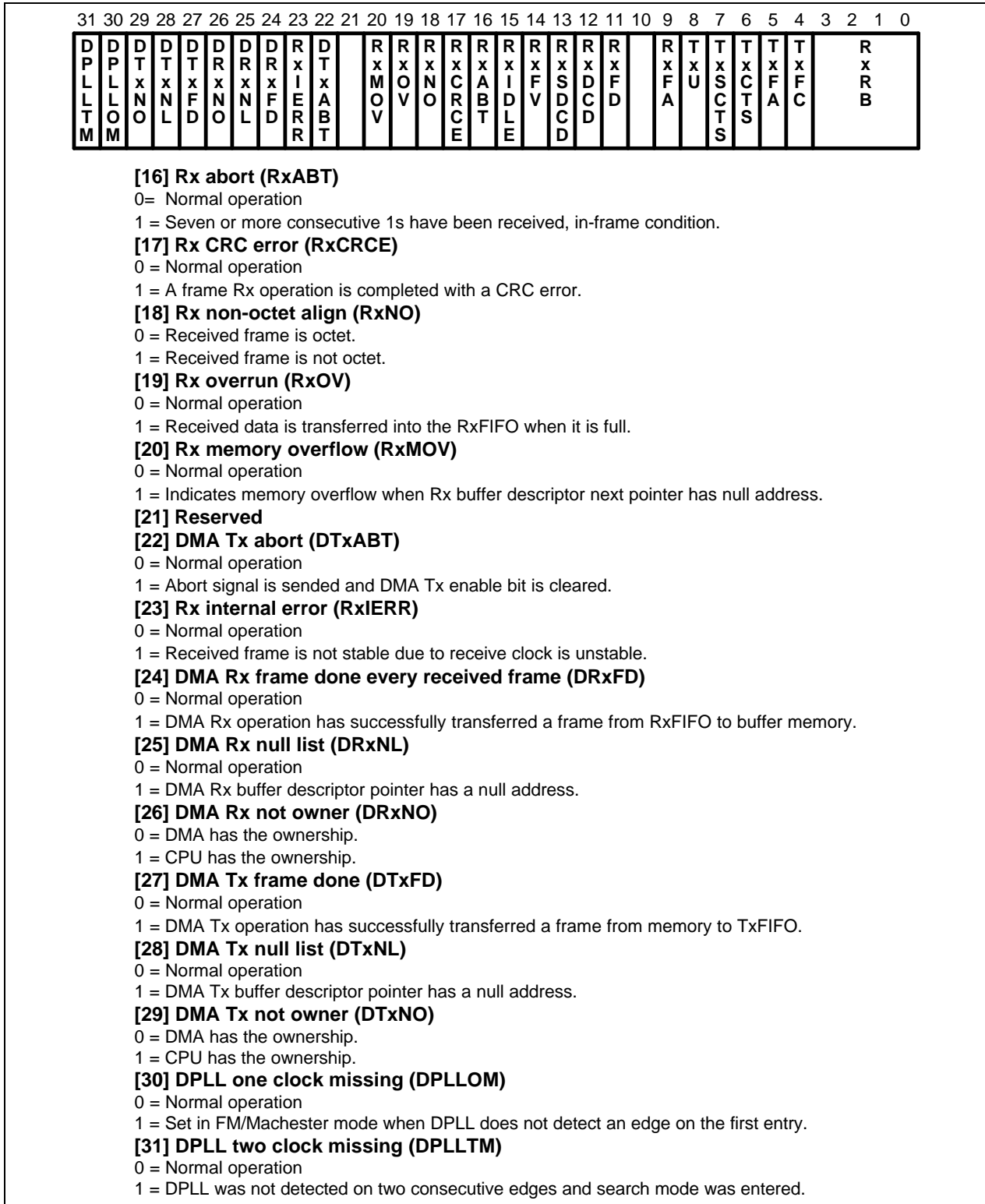
Figure 8-17. HDLC Status Register (Continued)
