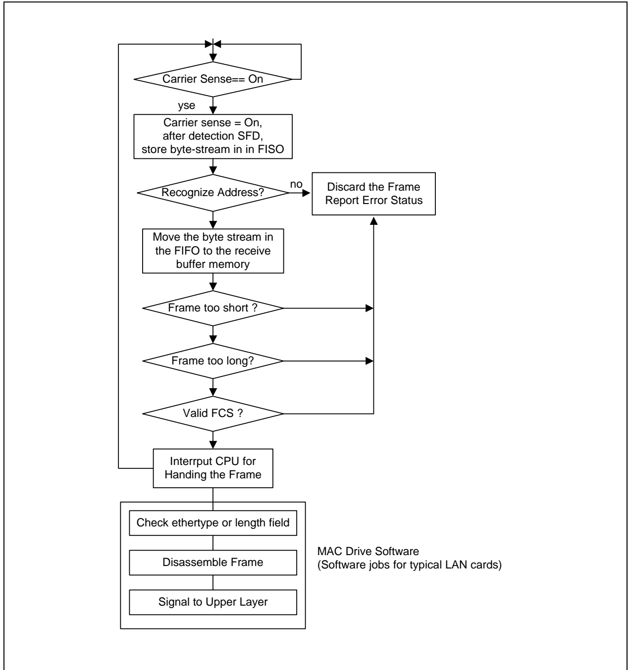
Figure 7-24. CSMA/CD Receive Operation
