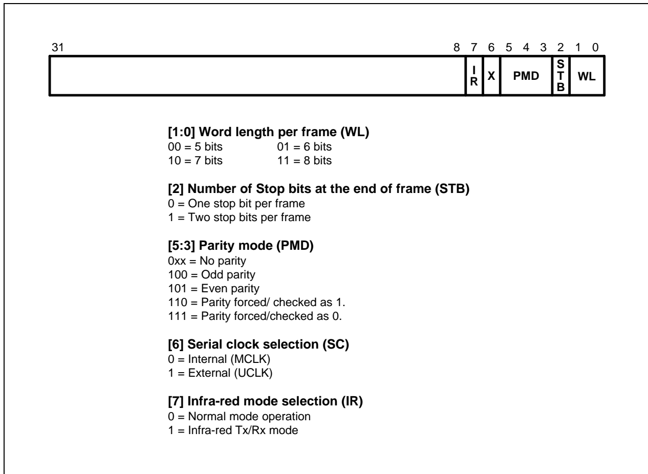
Figure 10-2. UART Line Control Registers
