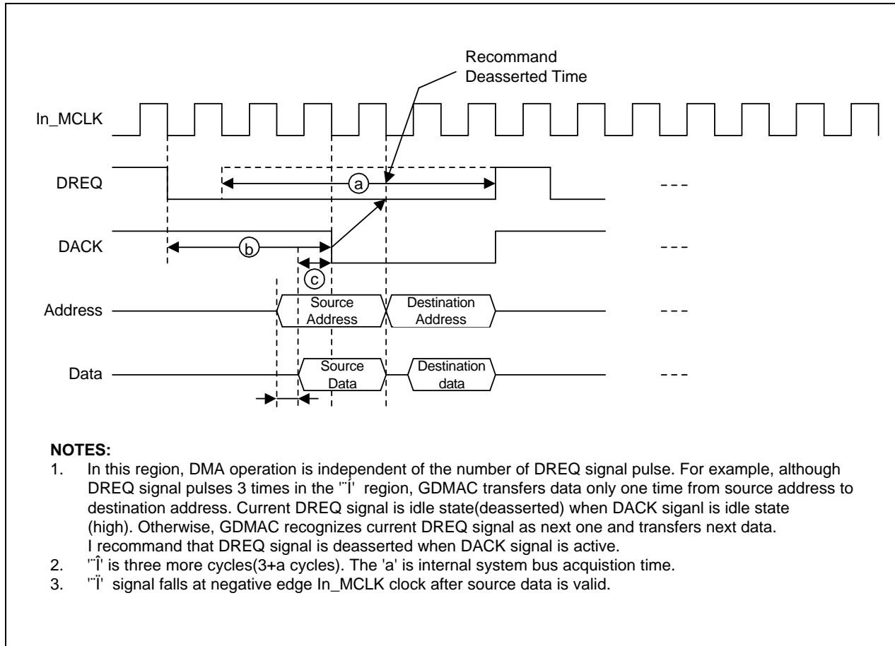
Figure 9-11. Single and One Data Burst Mode Timing
