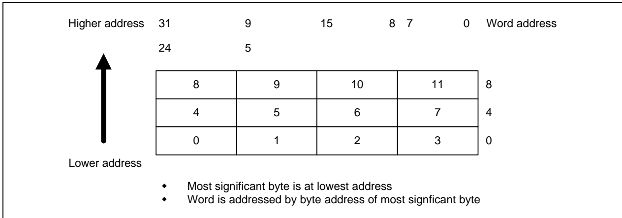
Figure 2-1. Big-Endian Addresses of Bytes within Words
