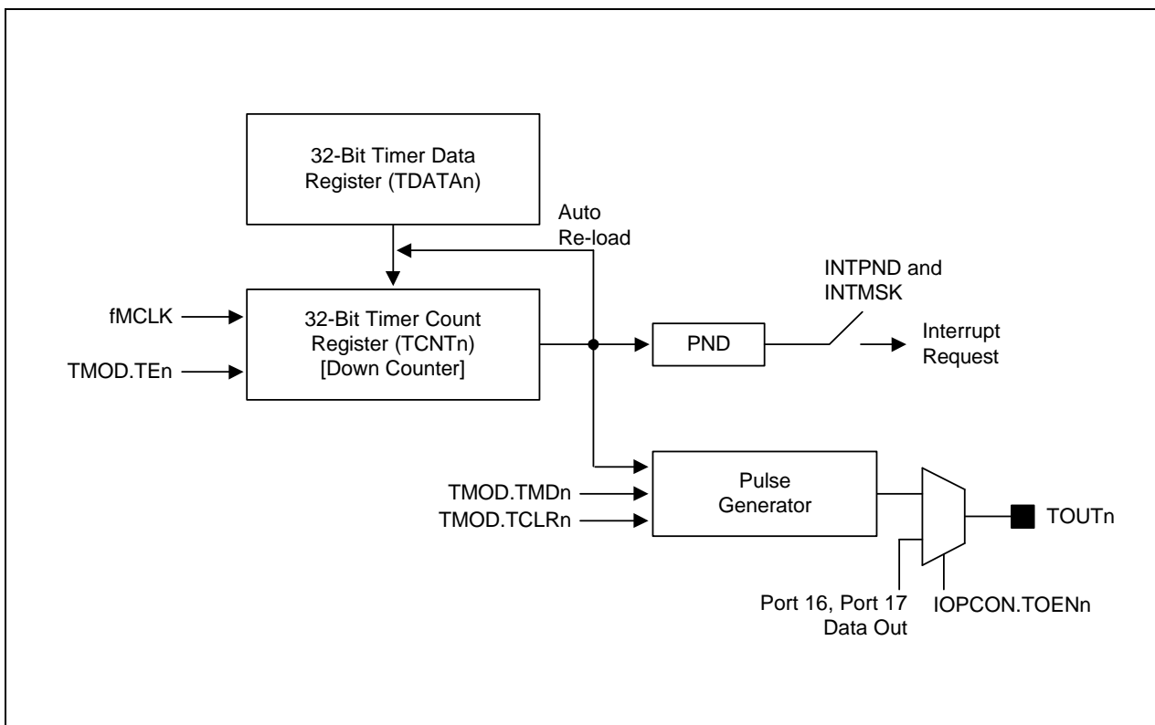
Figure 11-2. 32-Bit Timer Block Diagram
