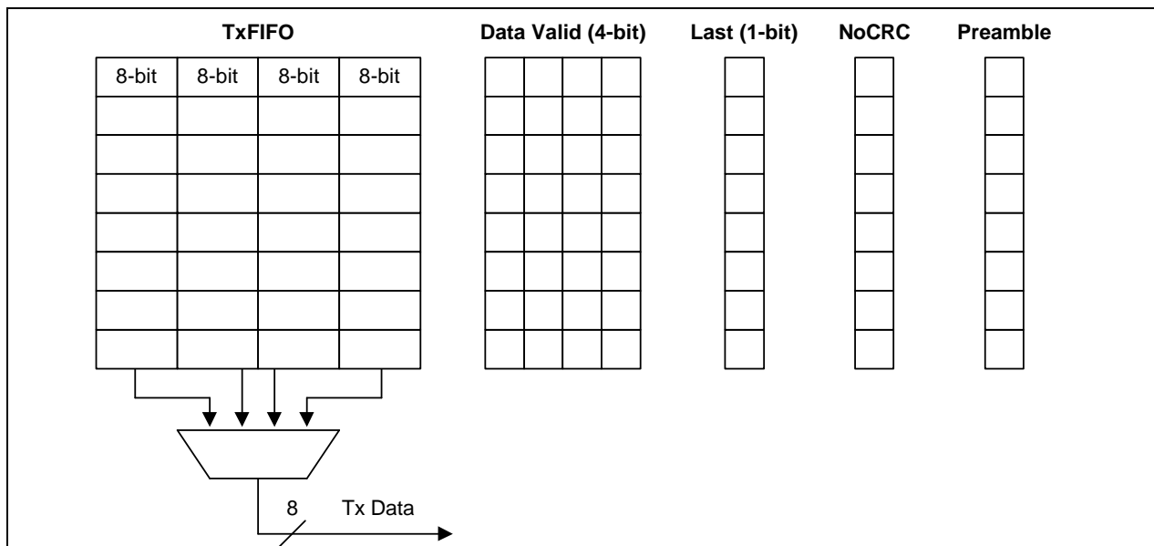
Figure 8-19. HDLC Tx FIFO Function Diagram
