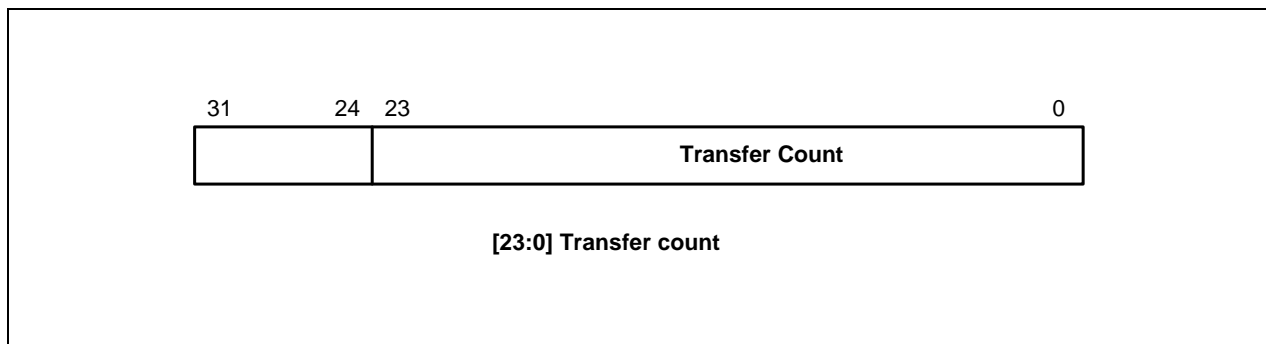
Figure 9-4. DMA Transfer Count Register
