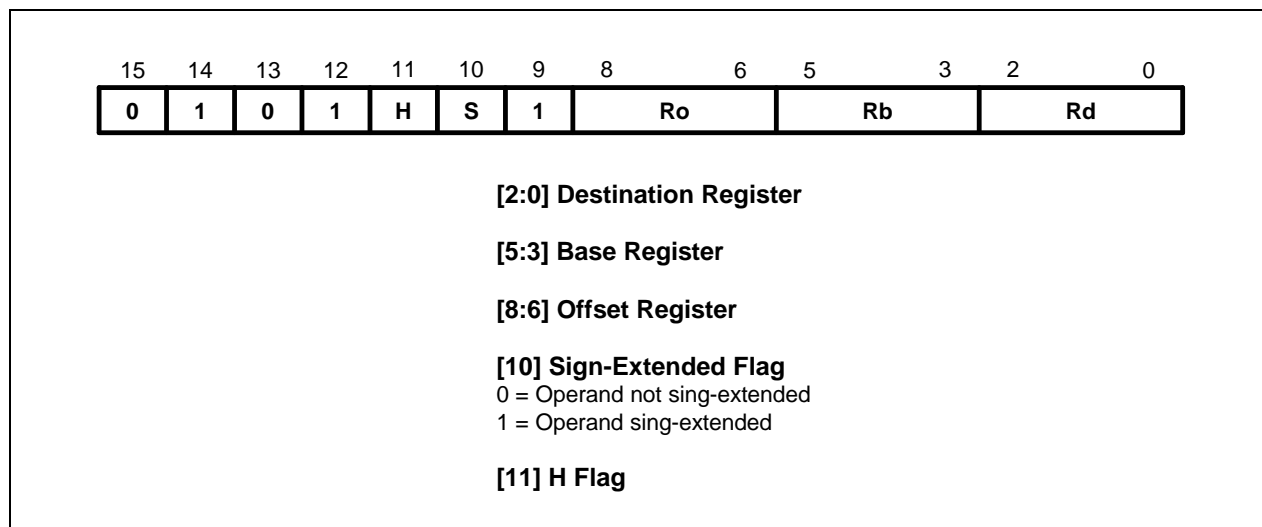
Figure 3-37. Format 8
