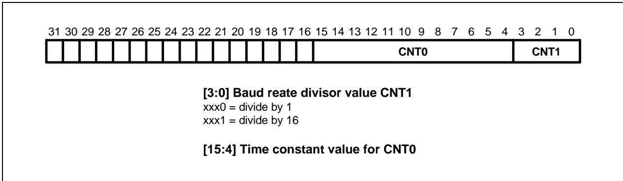
Figure 10-7. UART Baud Rate Divisor Registers
