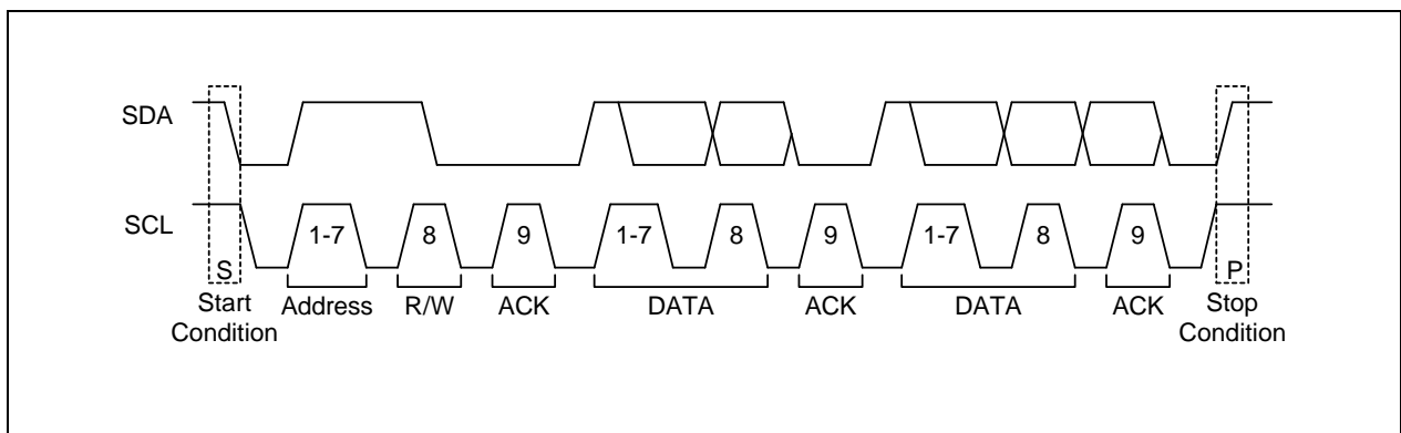
Figure 6-2. Start and Stop Conditions
