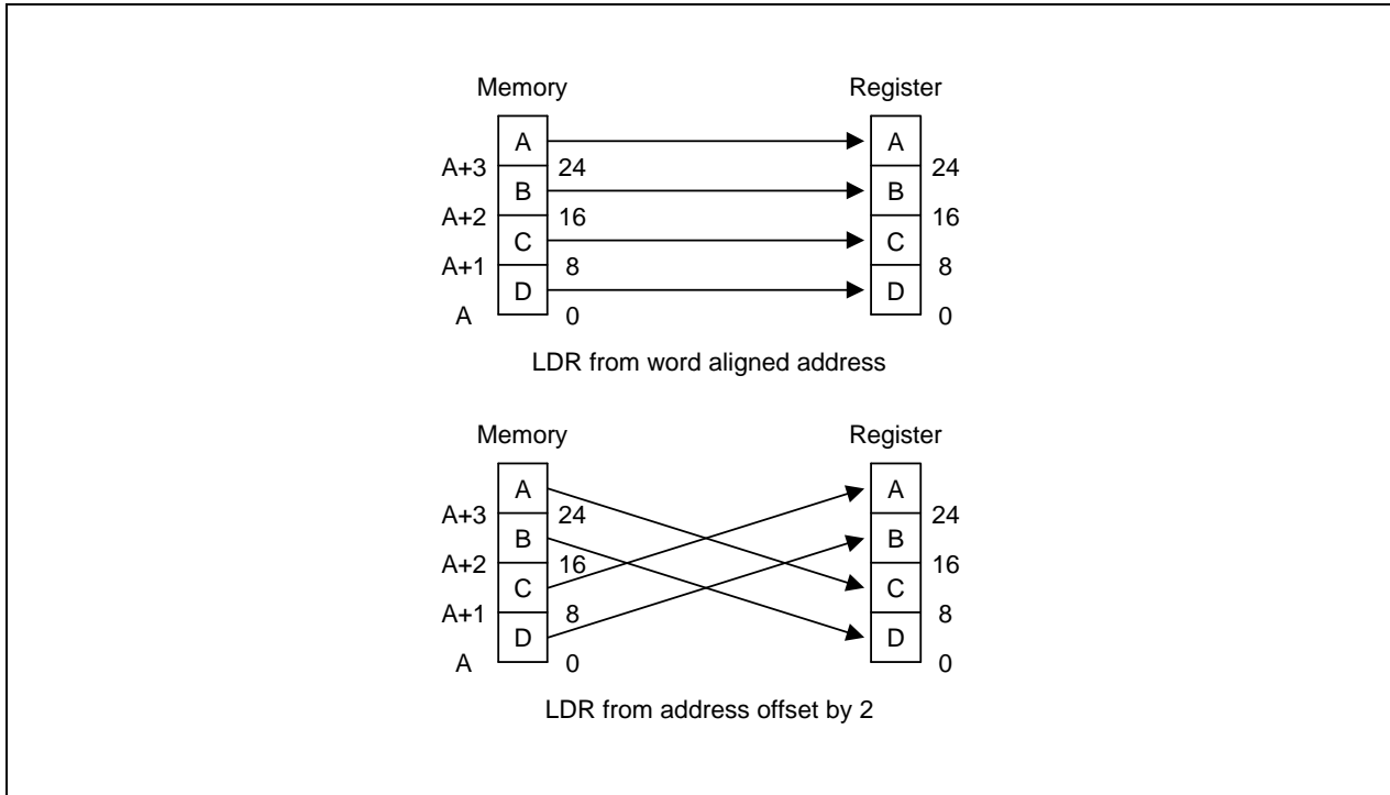
Figure 3-15. Little-Endian Offset Addressing
