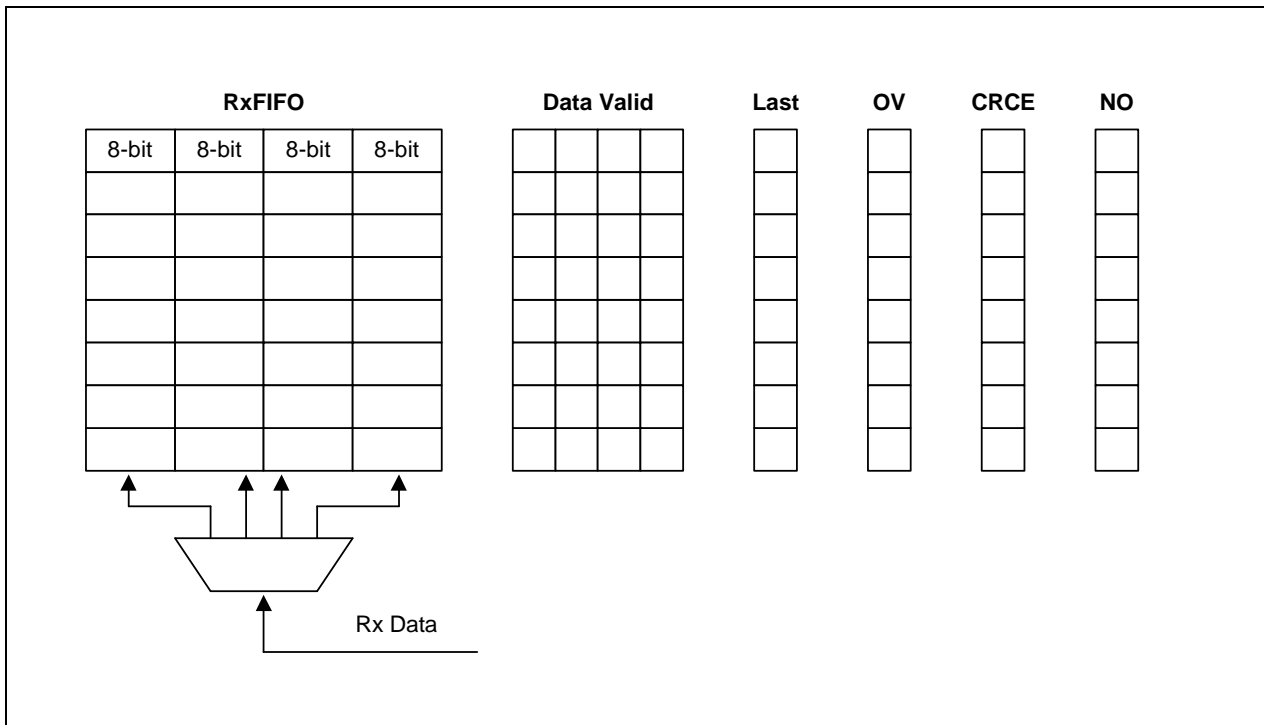
Figure 8-20. HDLC Rx FIFO Function Diagram
