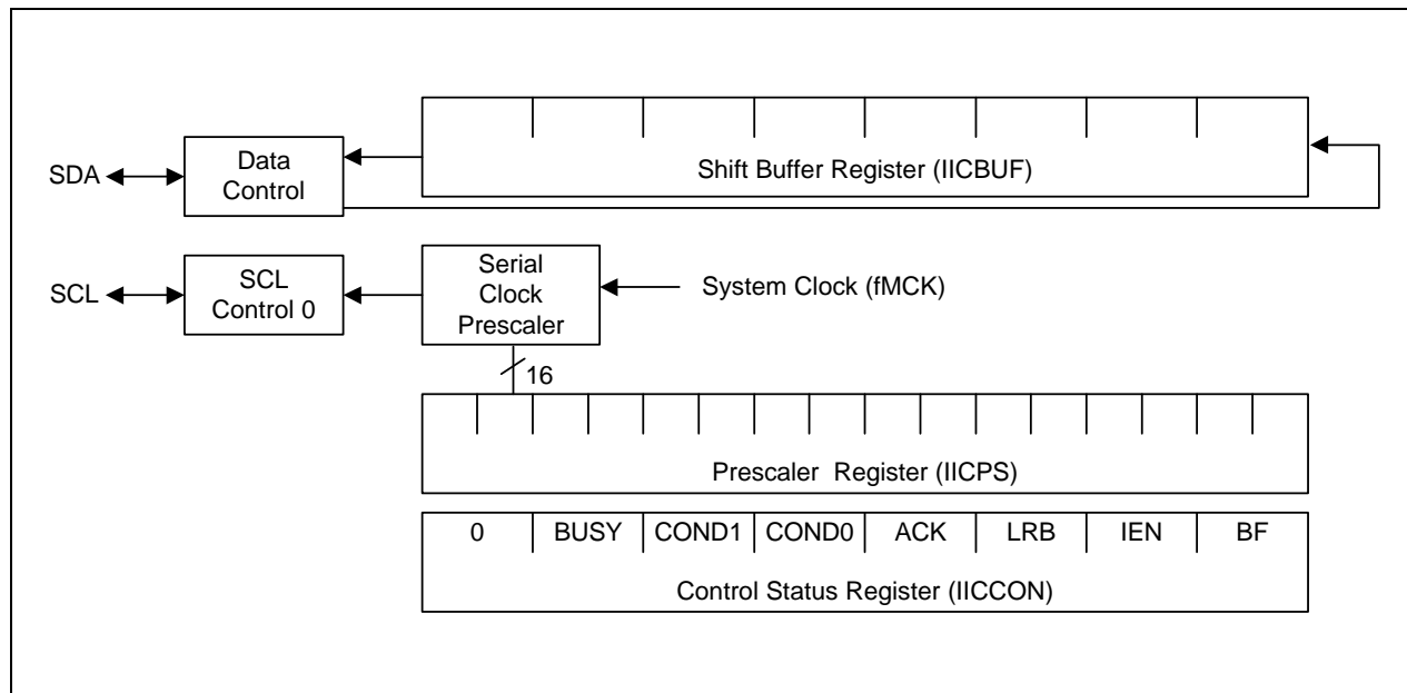
Figure 6-1. I 2 C BUS Block Diagram
