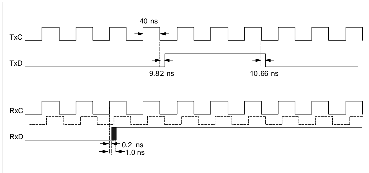
Figure 8-6. Data Encoding Methods and Timing Diagrams
