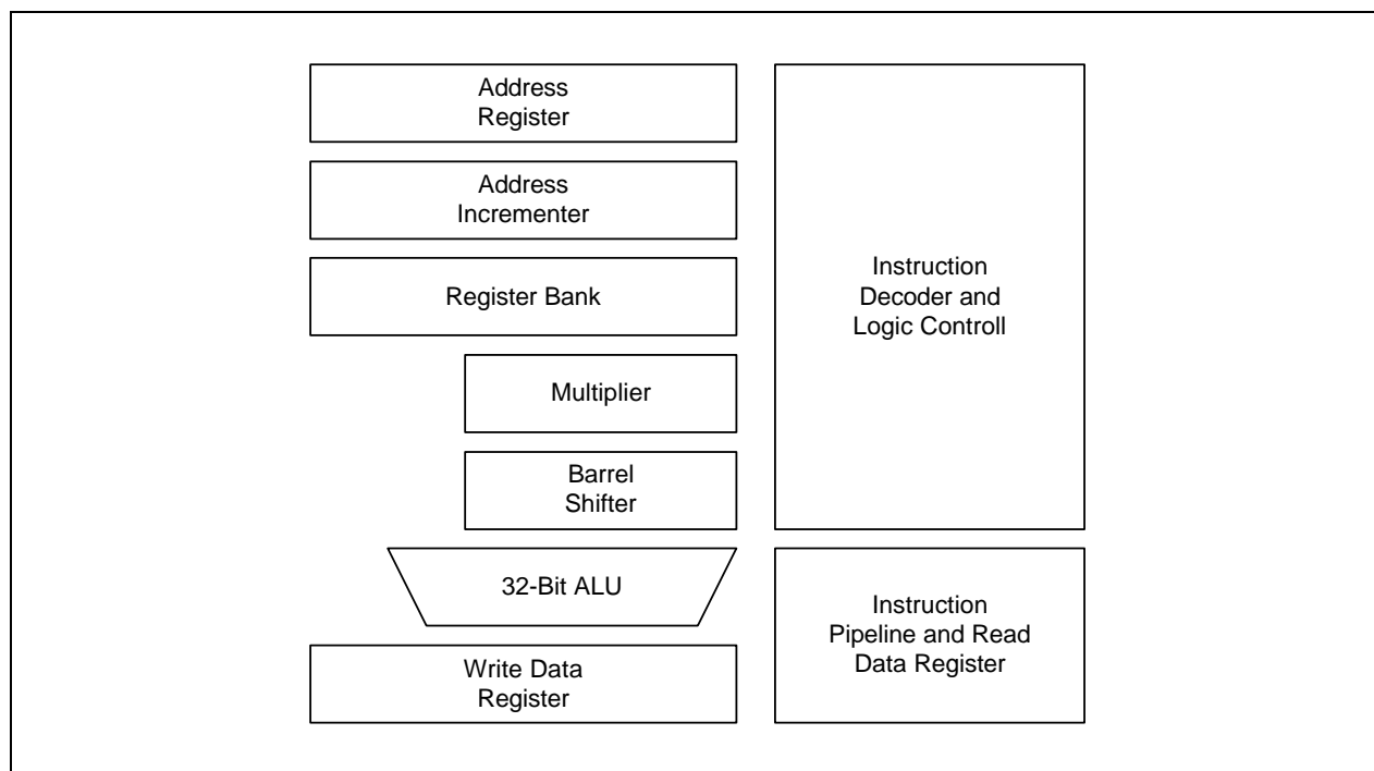
Figure 1-4. ARM7TDMI Core Block Diagram
