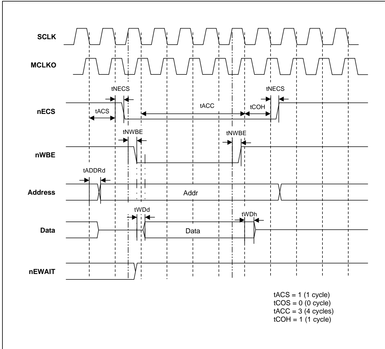
Figure 4-15. External I/O Write Timing 2
