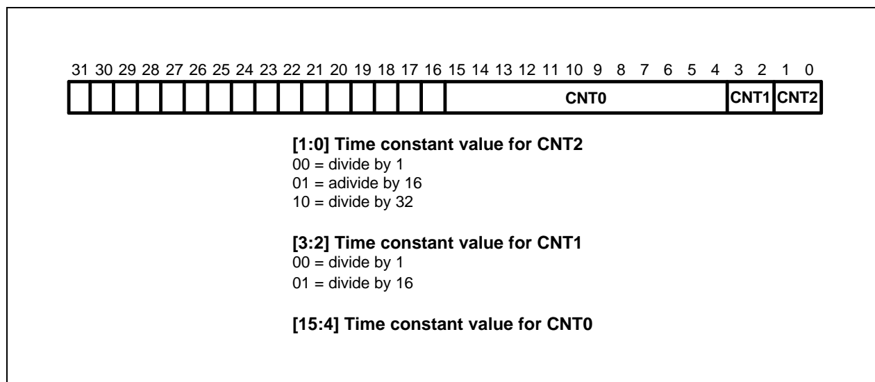
Figure 8-21. HDLC BRG Time Constant Register
