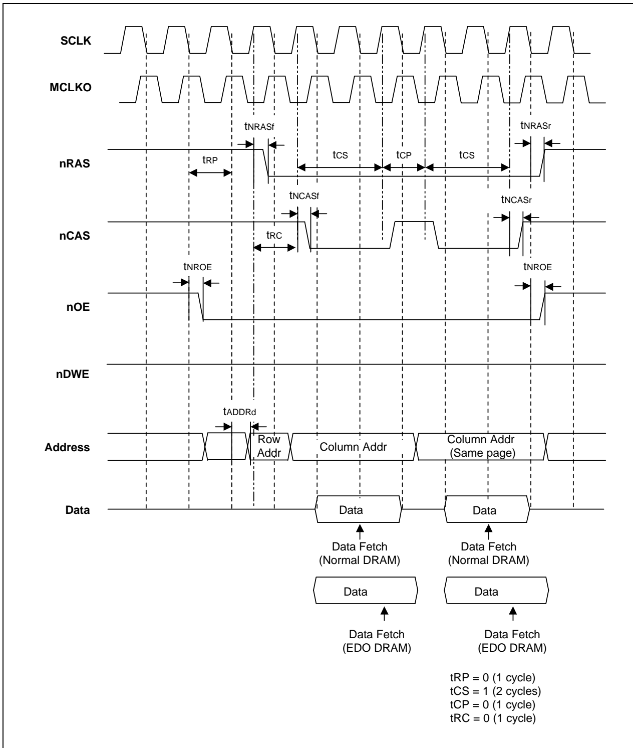
Figure 4-30. EDO/FP DRAM Bank Read Timing (Page Mode)
