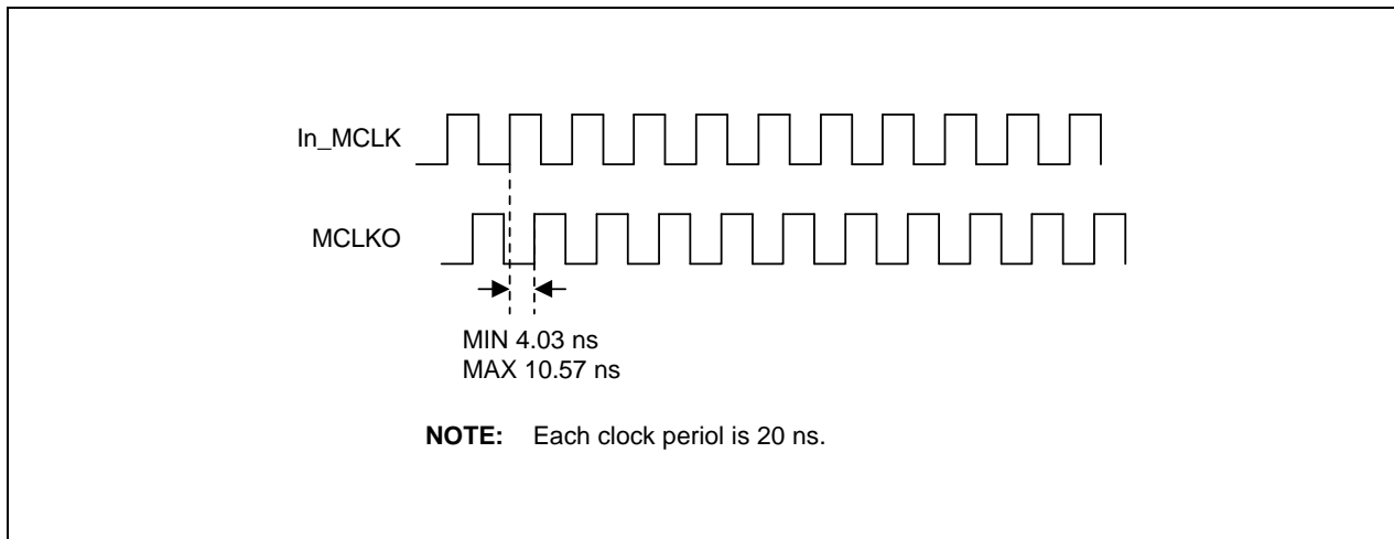
Figure 9-10. MCLKO and SCLK (In_MCLK)
