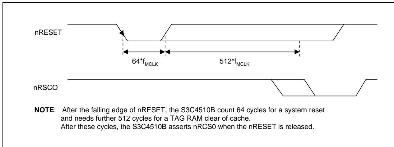
Figure 1-3. Reset Timing Diagram
