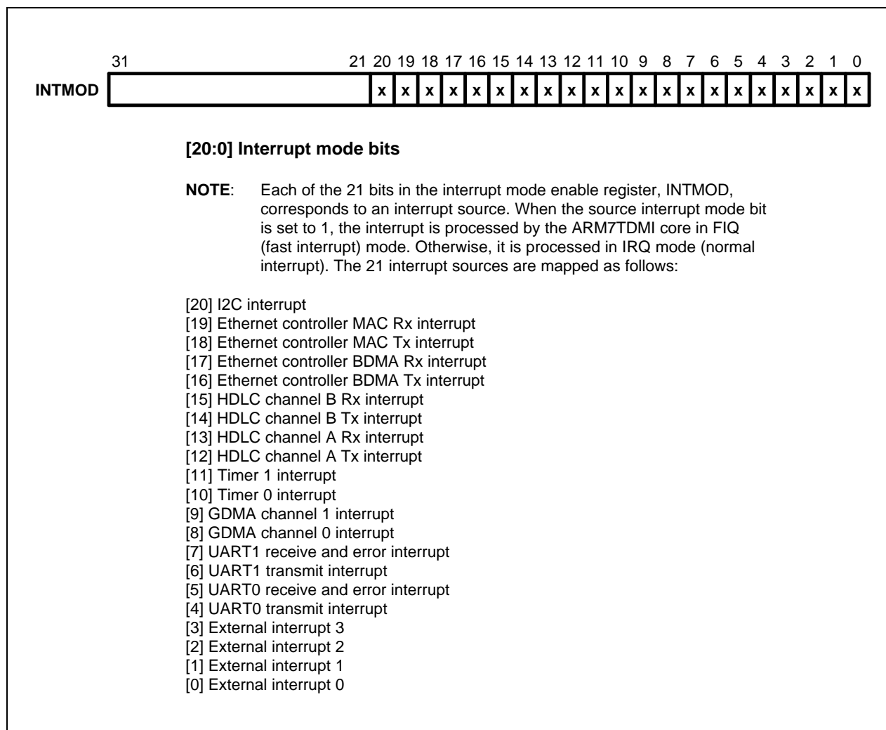
Figure 13-1. Interrupt Mode Register (INTMOD)
