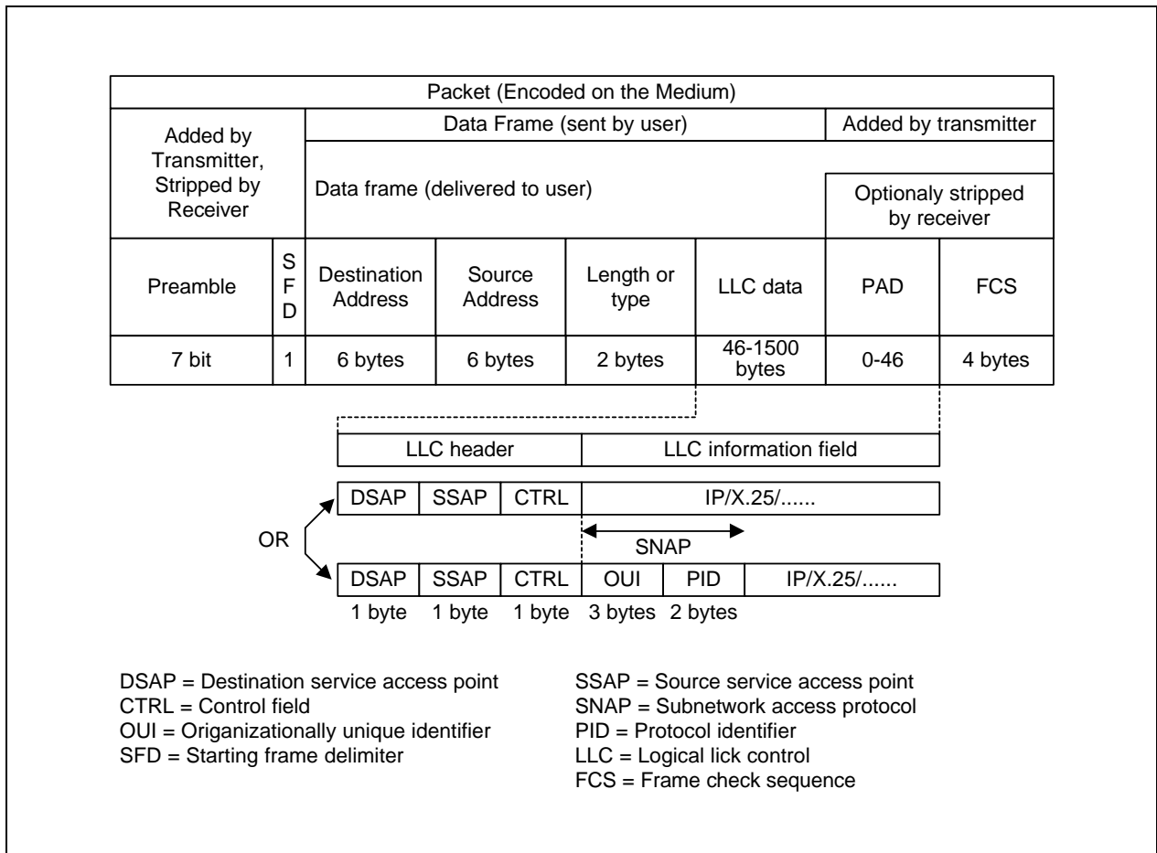
Figure 7-15. Fields of an IEEE802.3/Ethernet Packet (Frame)
