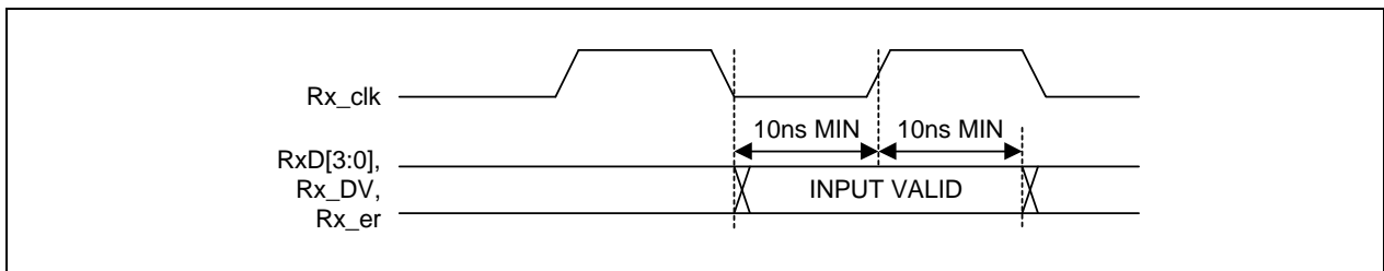
Figure 7-26. Receive Signal Timing Relationship at MII
