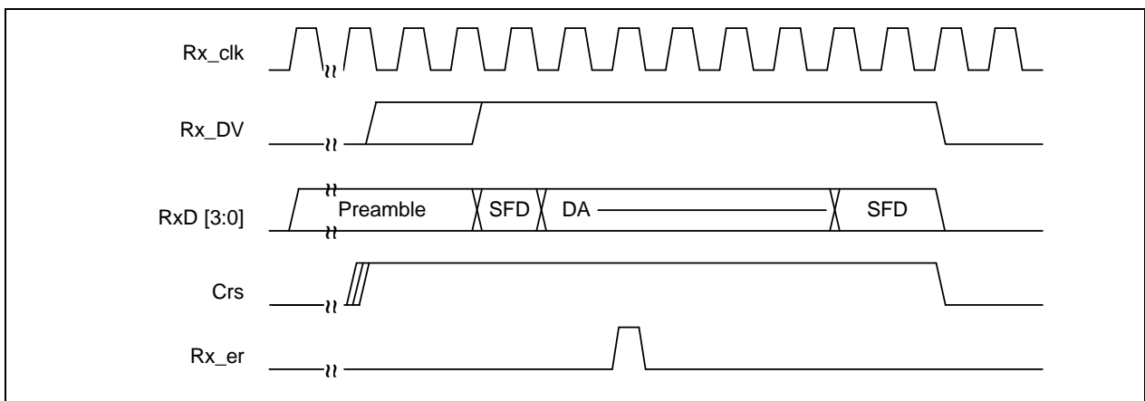
Figure 7-23. Receiving Frame with Error
