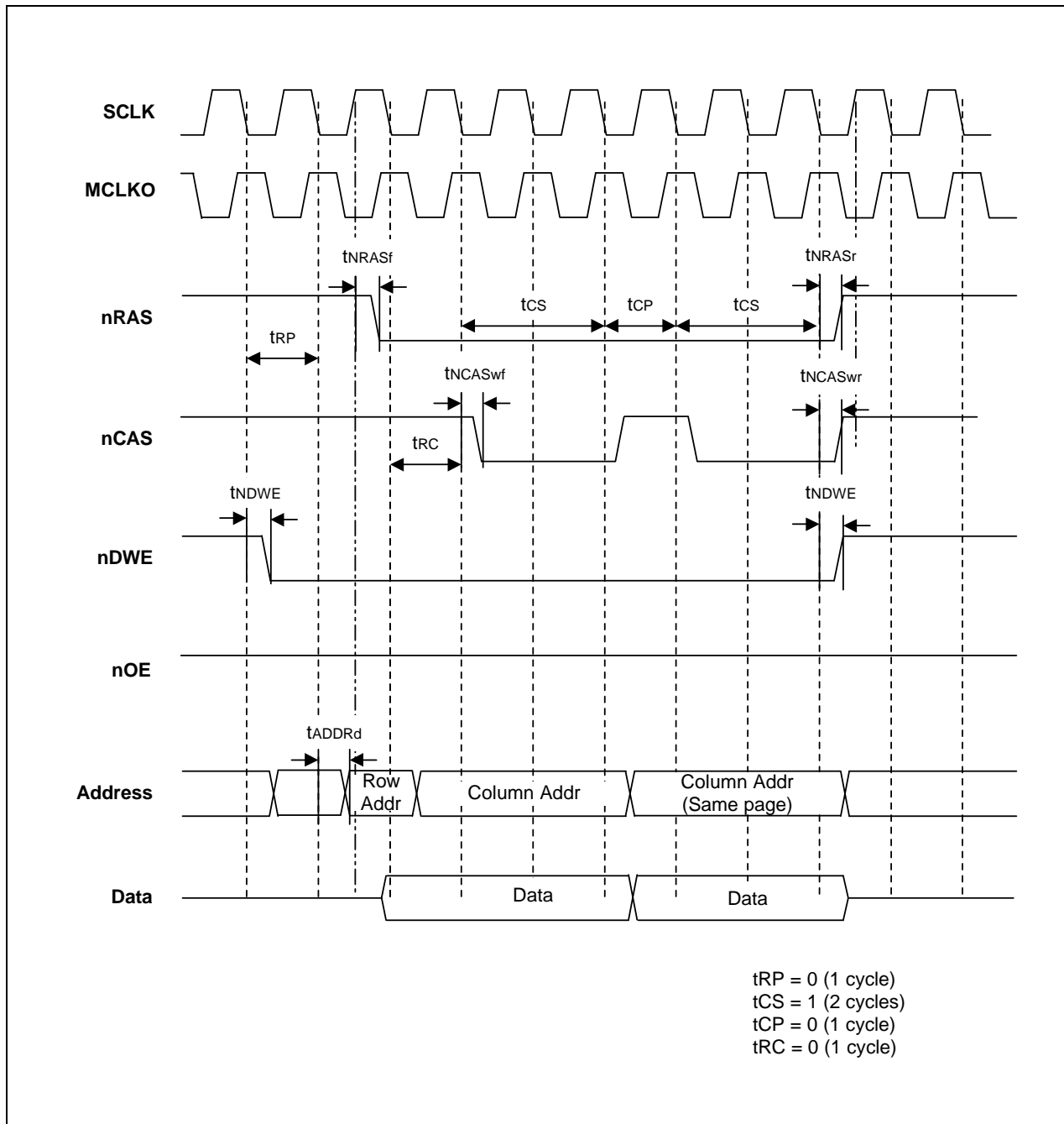
Figure 4-31. EDO/FP DRAM Bank Write Timing (Page Mode)
