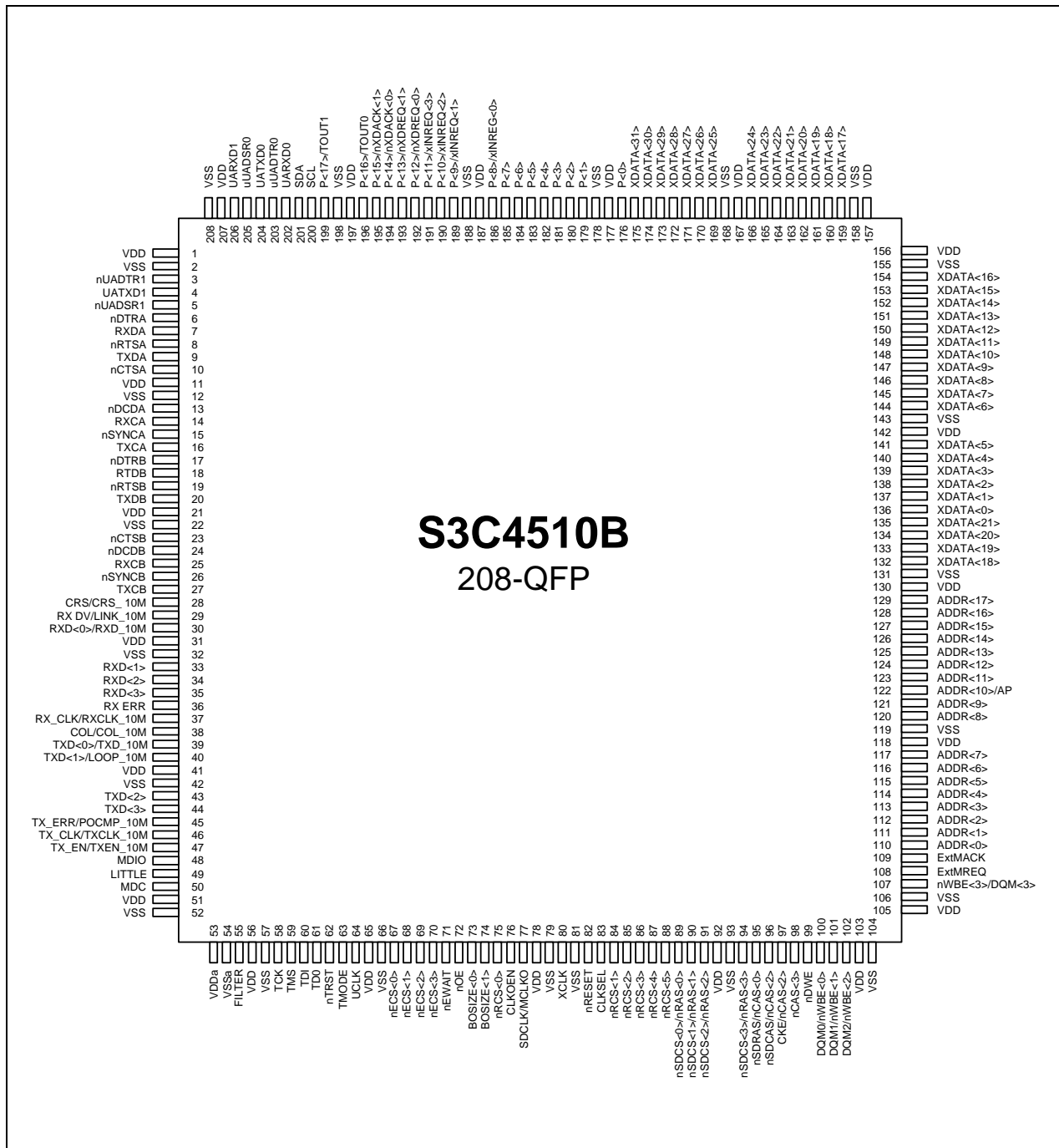
Figure 1-2. S3C4510B Pin Assignment Diagram
