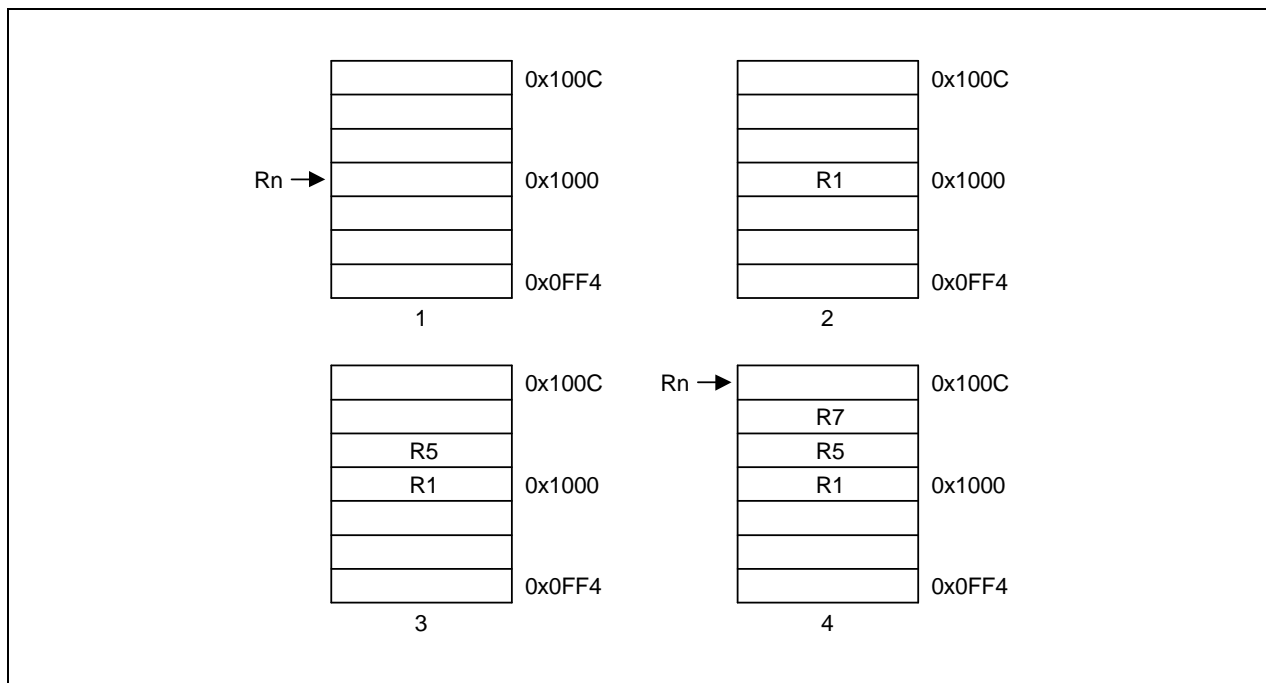
Figure 3-19. Post-Increment Addressing
