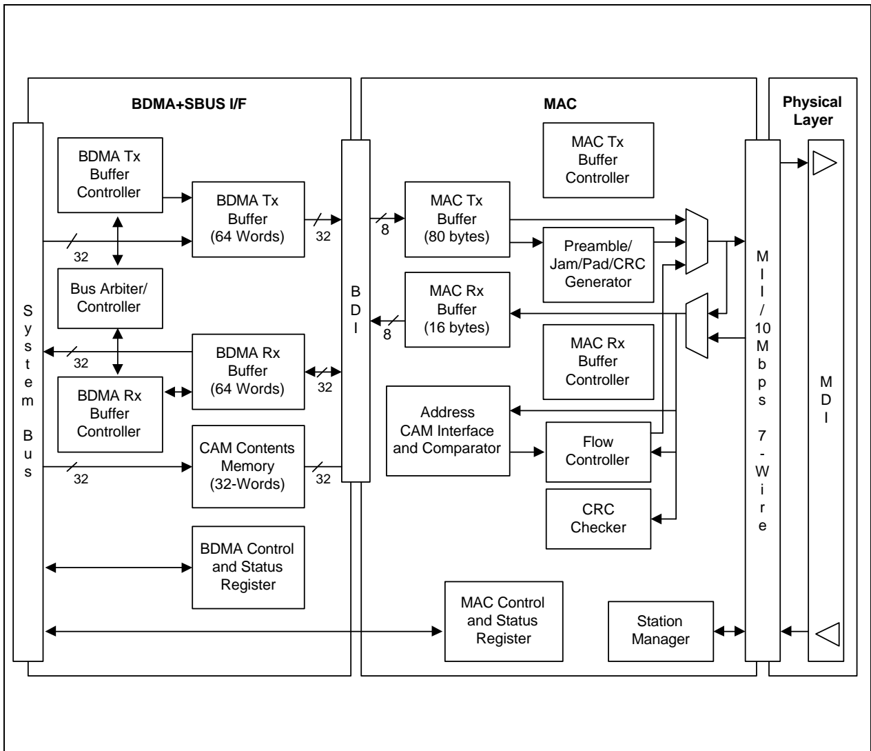
Figure 7-1. Ethernet System Flow Control
