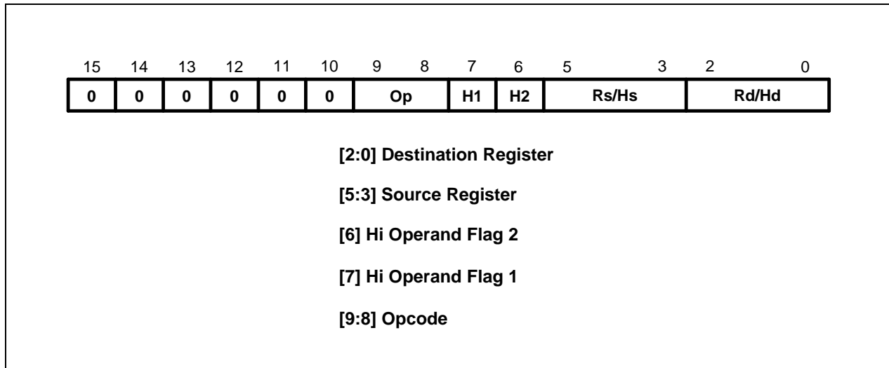
Figure 3-34. Format 5
