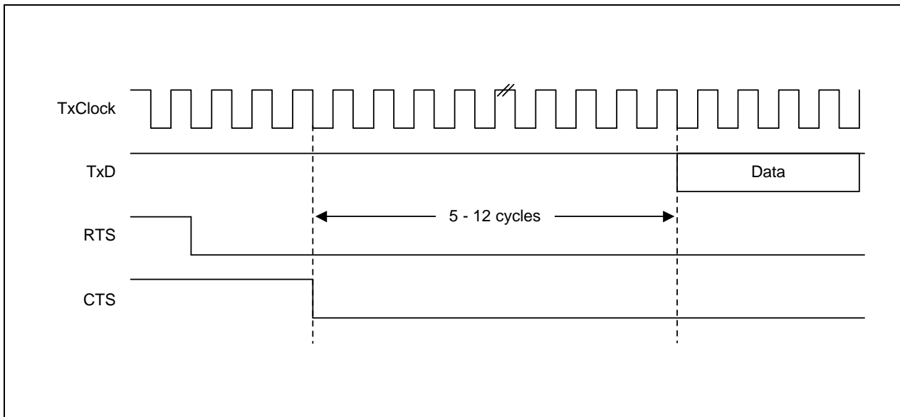
Figure 8-9. CTS Delayed on
