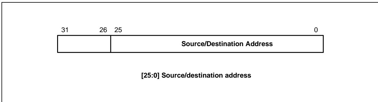
Figure 9-3. GDMA Source/Destination Address Register
