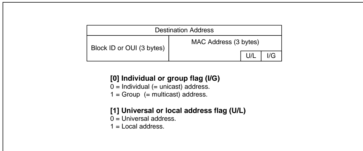
Figure 7-16. Destination Address Format
