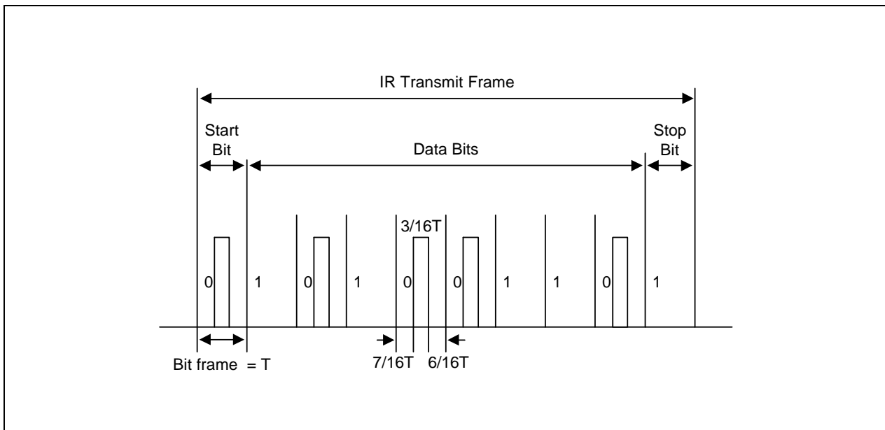
Figure 10-14. Infra-Red Transmit Mode Frame Timing Diagram
