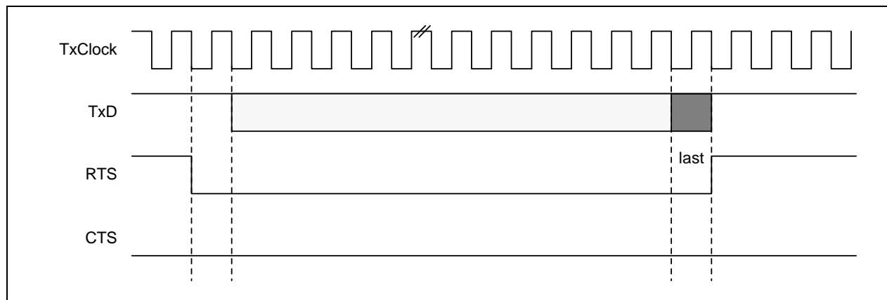
Figure 8-7. nCTS Already Asserted
