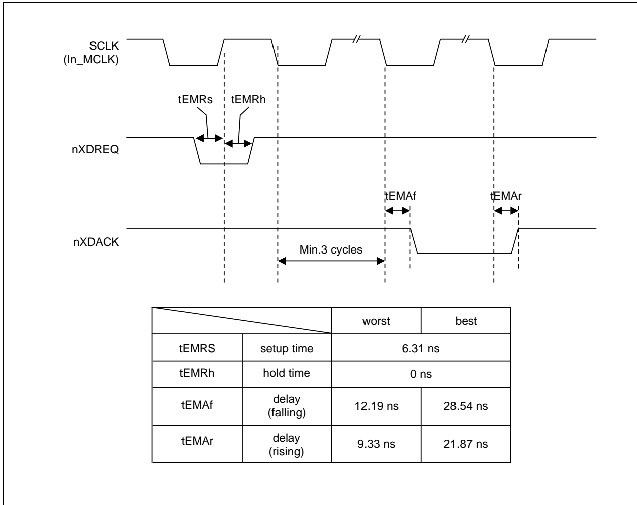
Figure 9-9. External DMA Requests Detailed Timing (S3C4510B)
