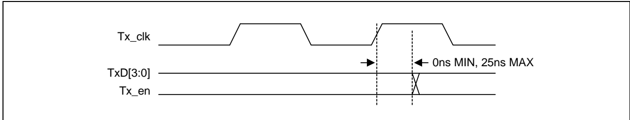
Figure 7-25. Transmit Signal Timing Relationship at MII
