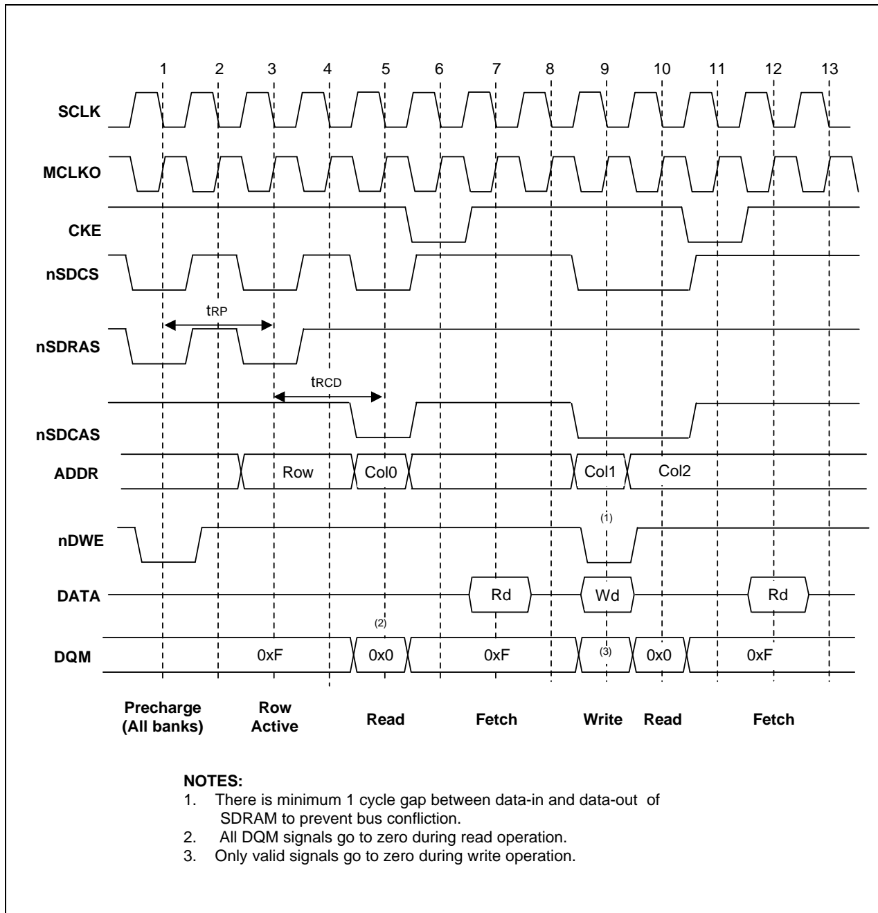
Figure 4-35. Non-burst, Read-Write-Read Cycles @CAS Latency = 2, Burst Length = 1
