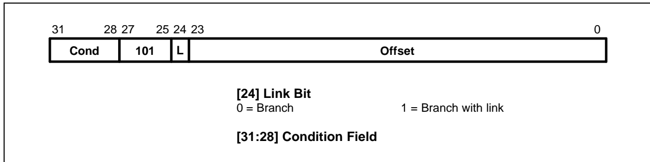
Figure 3-3. Branch Instructions
