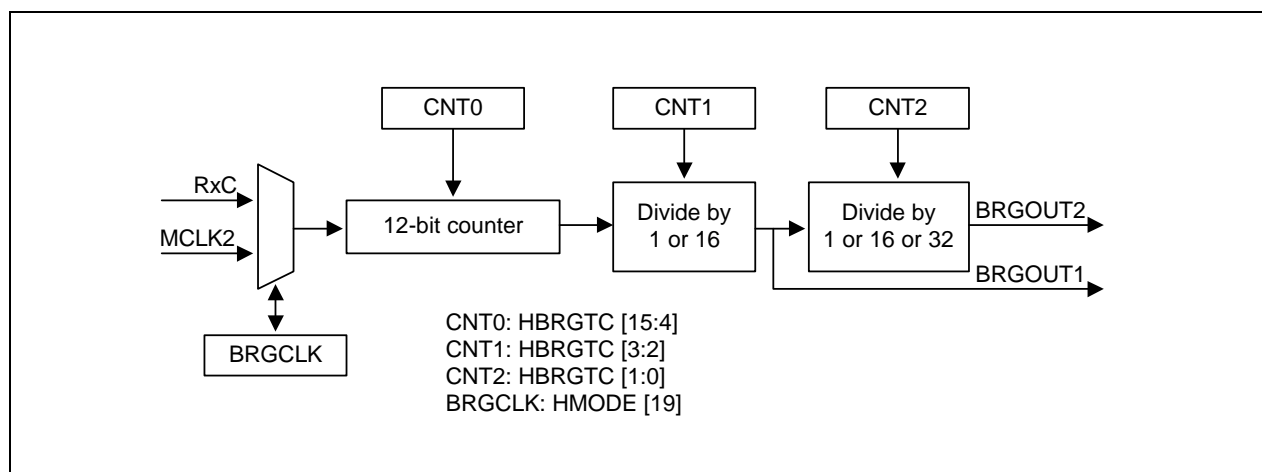
Figure 8-2. Baud Rate Generator Block Diagram
