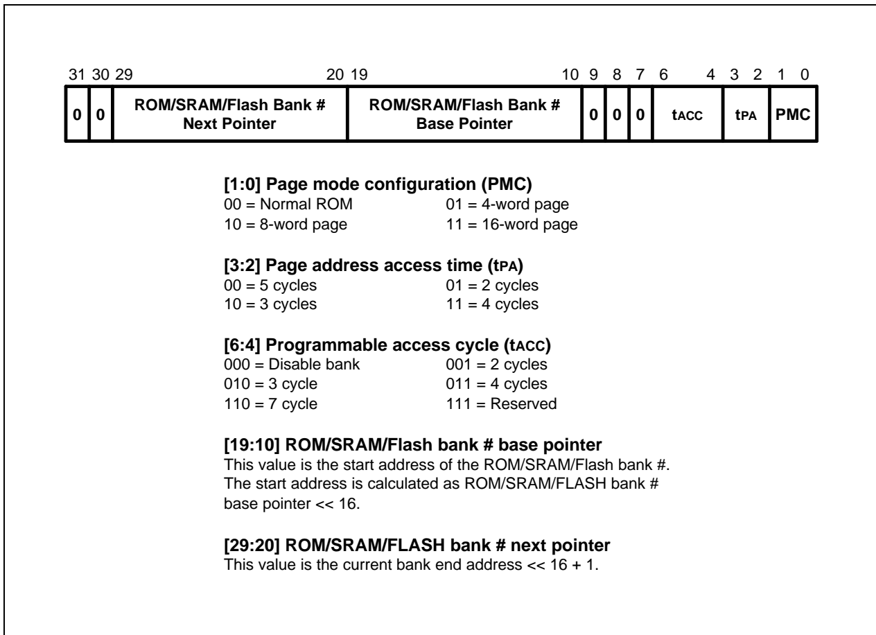
Figure 4-18. ROM/SRAM/FLASH Control Registers (ROMCON0–ROMCON5)
