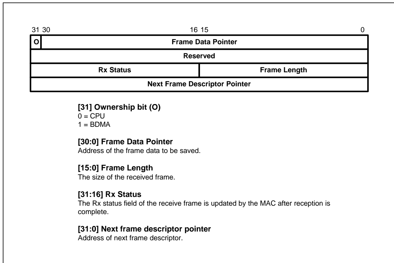
Figure 7-6. Data Structure of Rx Frame Descriptor
