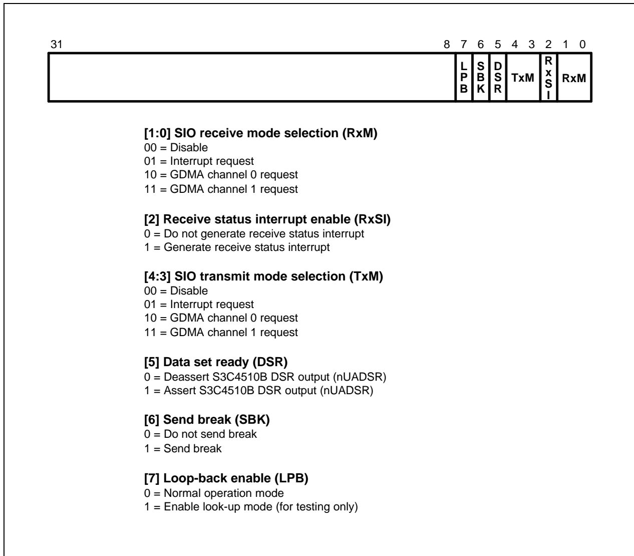
Figure 10-3. UART Control Registers
