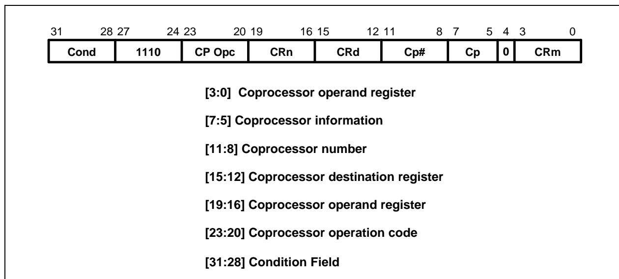
Figure 3-25. Coprocessor Data Operation Instruction
