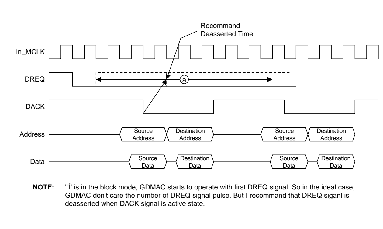
Figure 9-13. Block and One Data Burst Mode Timing
