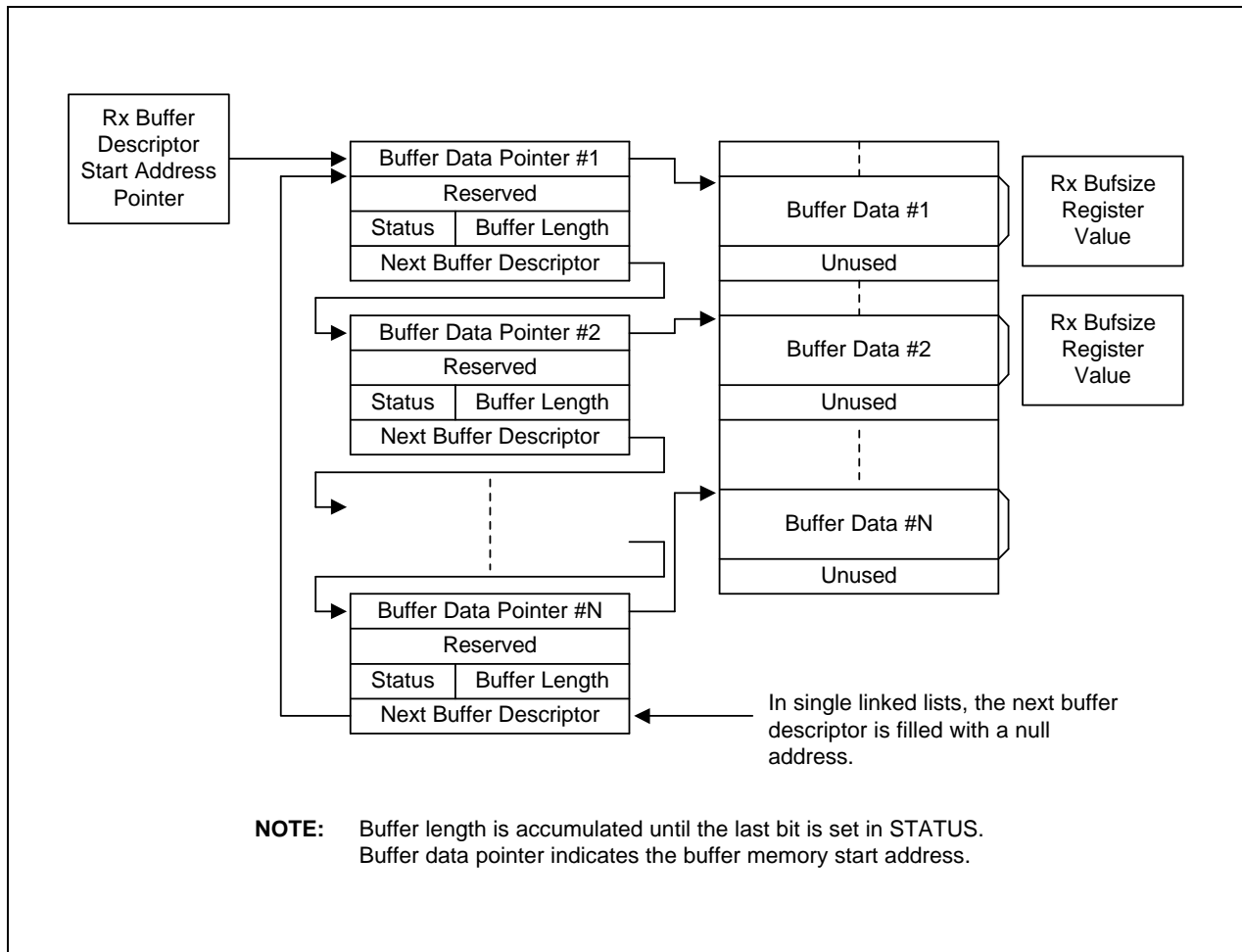
Figure 8-12. Data Structure of the Receive Data Buffer
