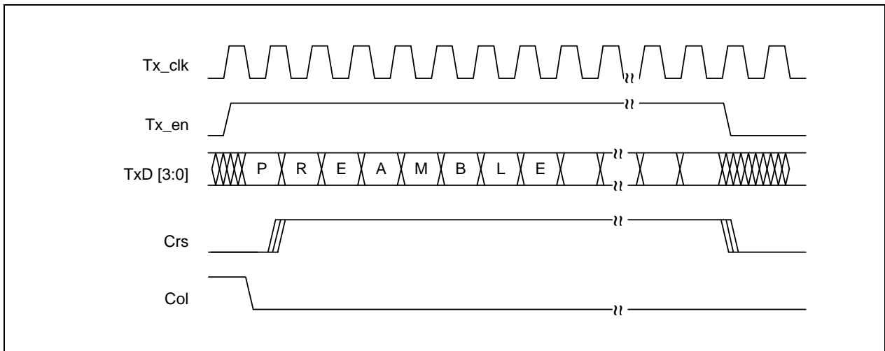
Figure 7-19. Timing for Transmit without Collision
