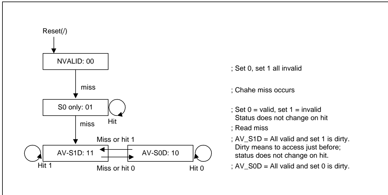
Figure 5-2. Cache Replace Algorithm State Diagram
