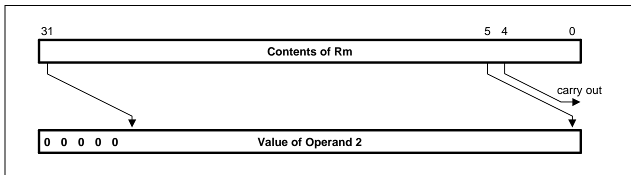
Figure 3-7. Logical Shift Right
