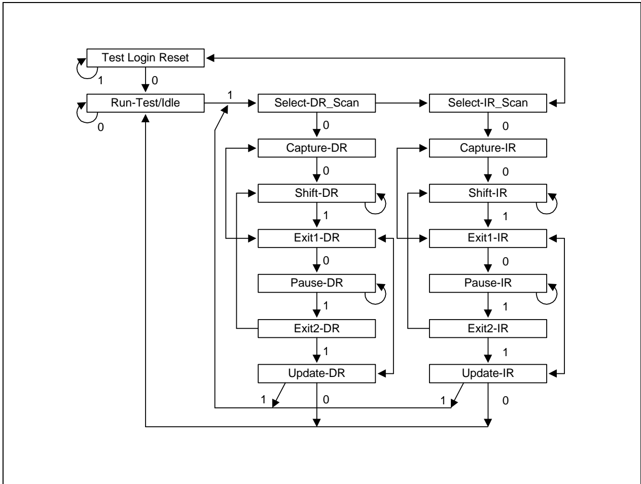
Figure A-1. TAP Controller State Machine
