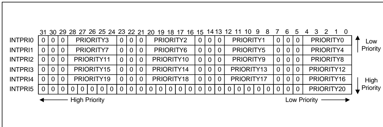
Figure 13-4. Interrupt Priority Register (INTPRI n )
