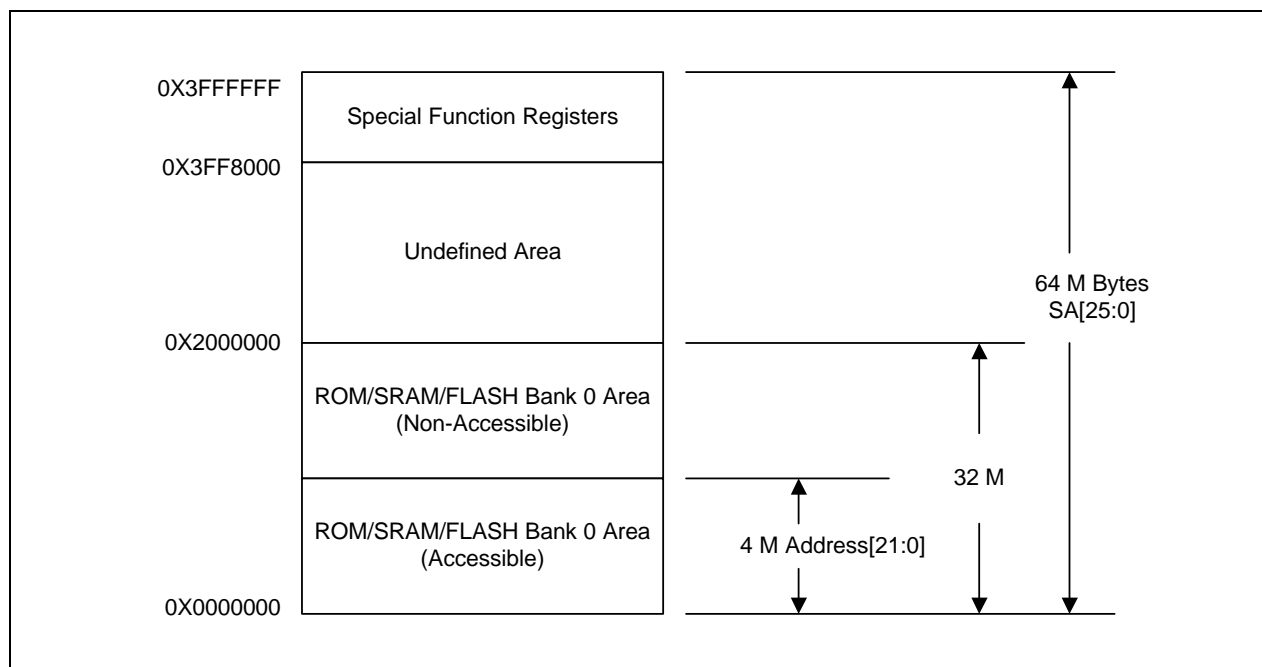
Figure 4-2. Initial System Memory Map (After Reset)
