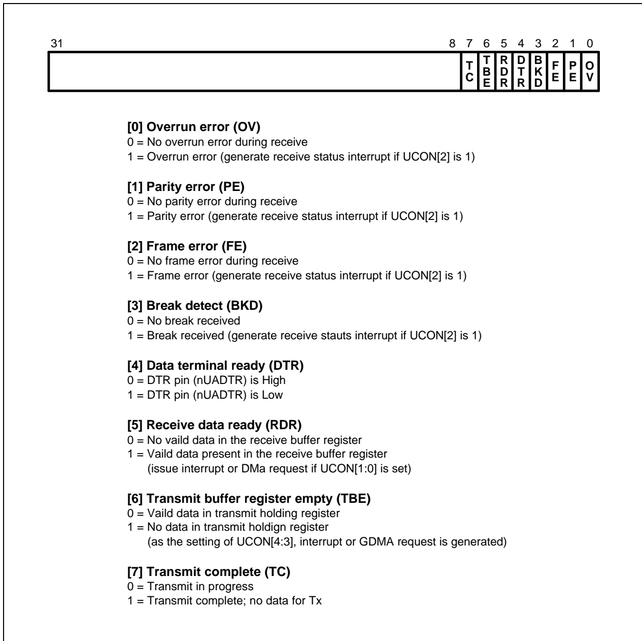
Figure 10-4. UART Status Registers
