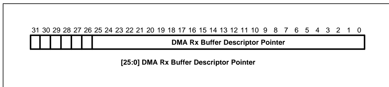
Figure 8-26. DMA Rx Buffer Descriptor Pointer
