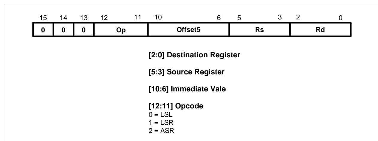
Figure 3-30. Format 1
