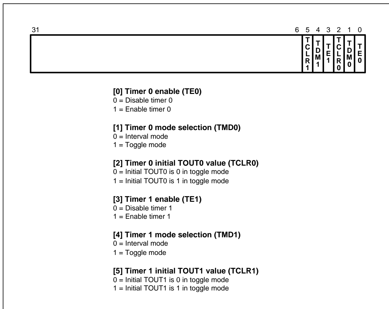
Figure 11-3. Timer Mode Register (TMOD)
