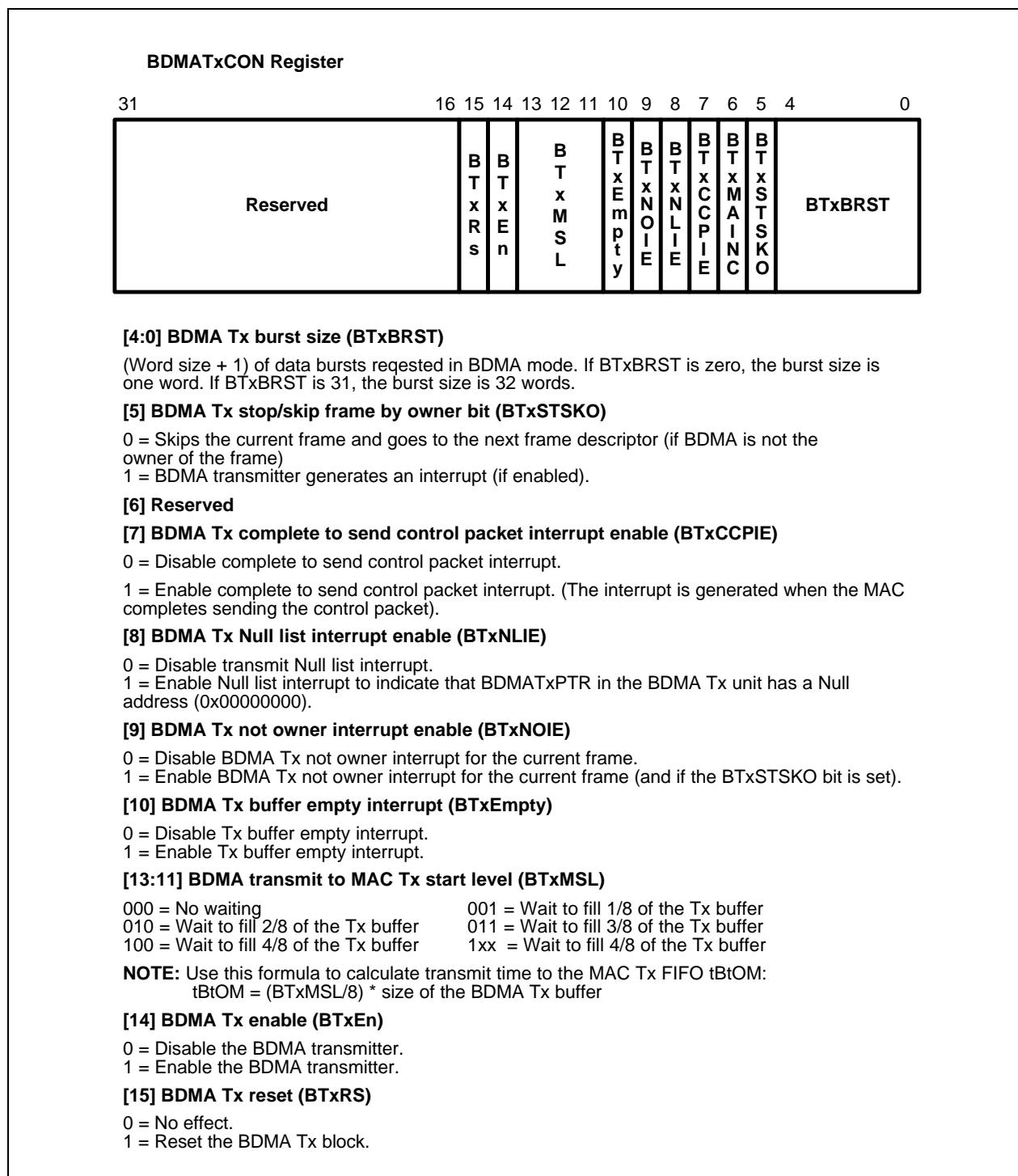
Figure 7-12. Buffered DMA Transmit Control Register
