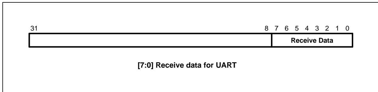
Figure 10-6. UART Receive Buffer Registers
