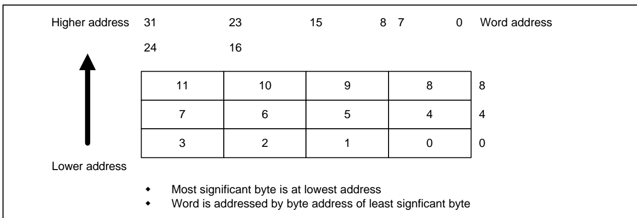
Figure 2-2. Little-Endian Addresses of Bytes Words
