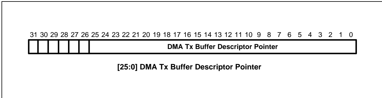
Figure 8-25. DMA Tx Buffer Descriptor Pointer
