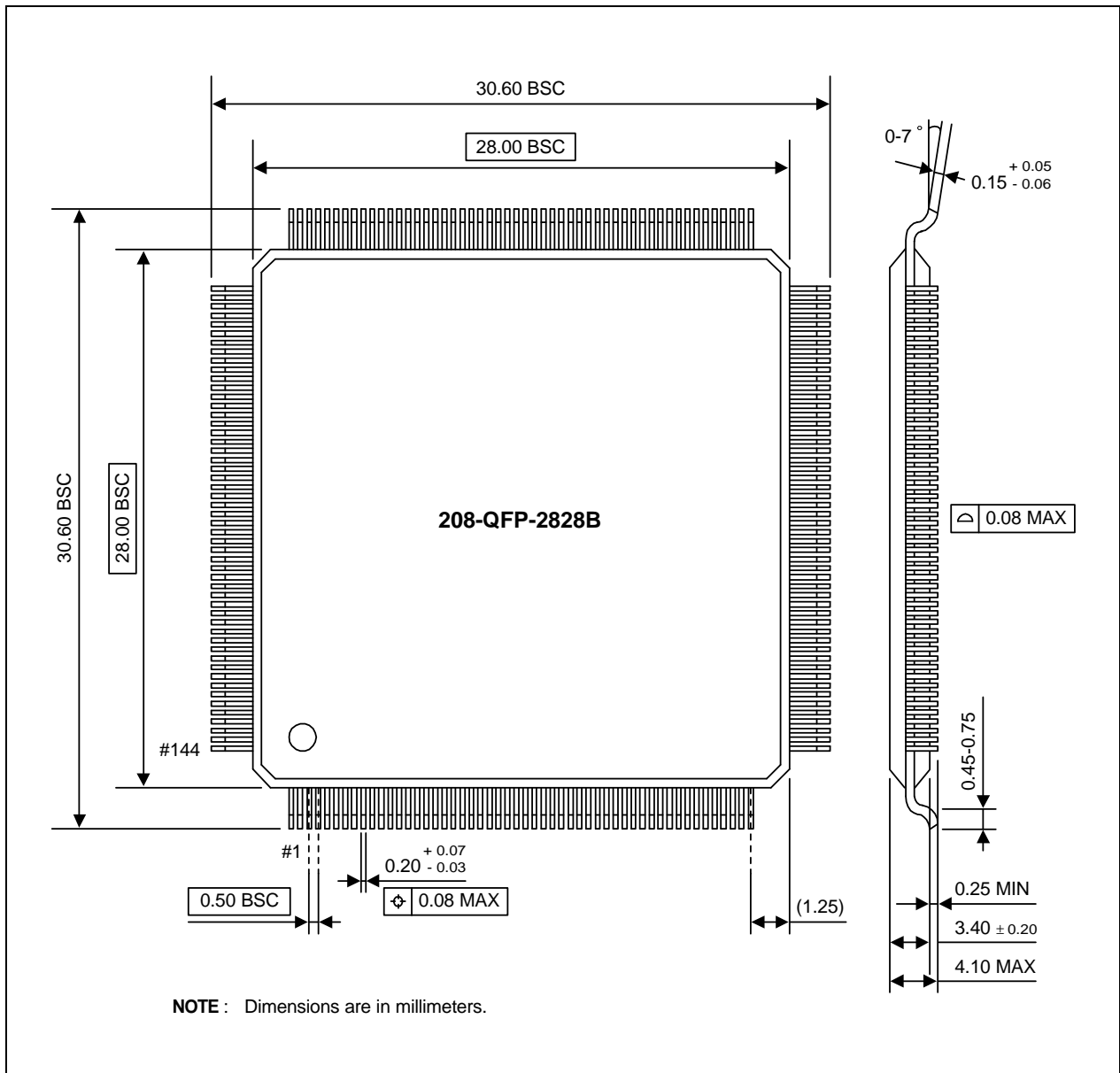
Figure 15-1. 208-QFP-2828B Package Dimensions
