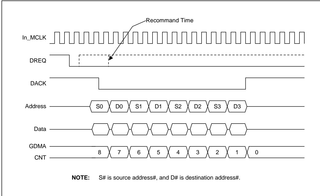
Figure 9-14. Continuous and One Burst Mode Timing
