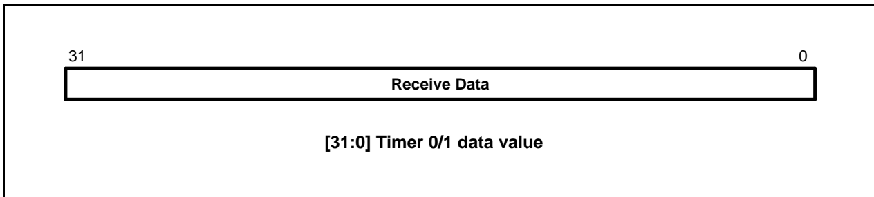
Figure 11-4. Timer Data Registers (TDATA0, TDATA1)
