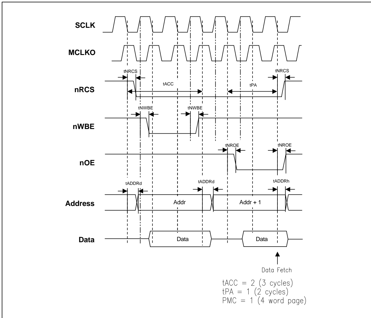
Figure 4-24. ROM/SRAM/Flash Write and Read Access Timing
