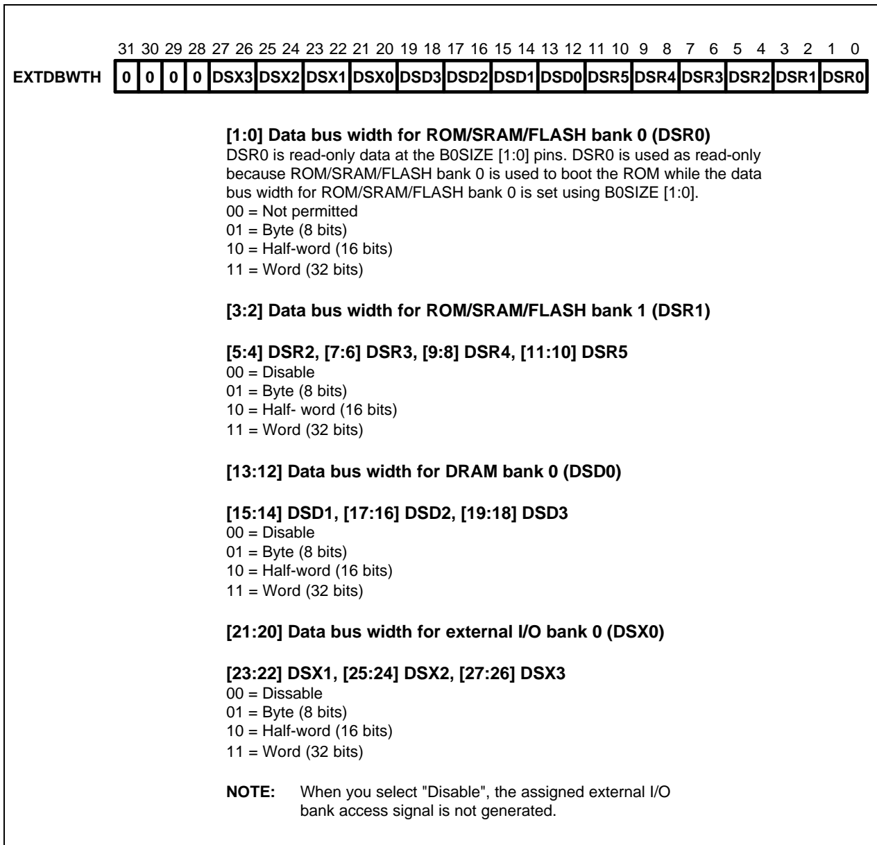
Figure 4-17. Data Bus Width Register (EXTDBWTH)
