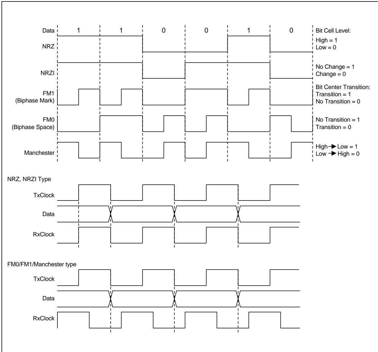
Figure 8-5. Data Encoding Methods and Timing Diagrams
