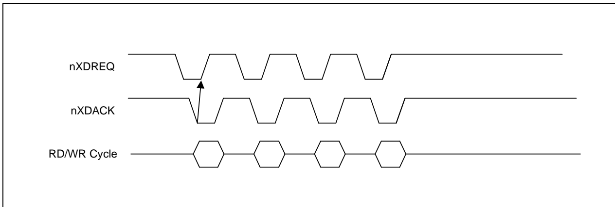
Figure 9-5. External DMA Requests (Single Mode)
