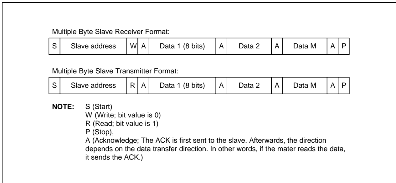
Figure 6-3. Data Transfer Format
