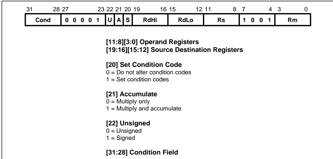
Figure 3-13. Multiply Long Instructions
