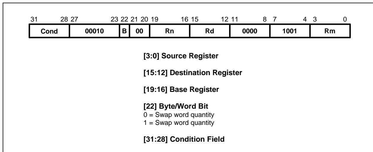
Figure 3-23. Swap Instruction
