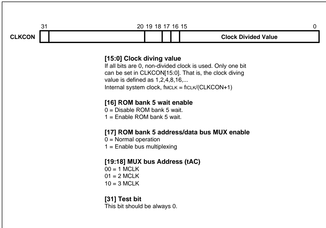
Figure 4-7. Clock Control Register (CLKCON)
