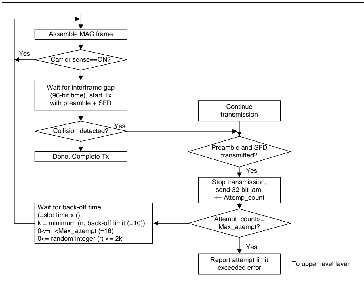
Figure 7-18. CSMA/CD Transmit Operation
