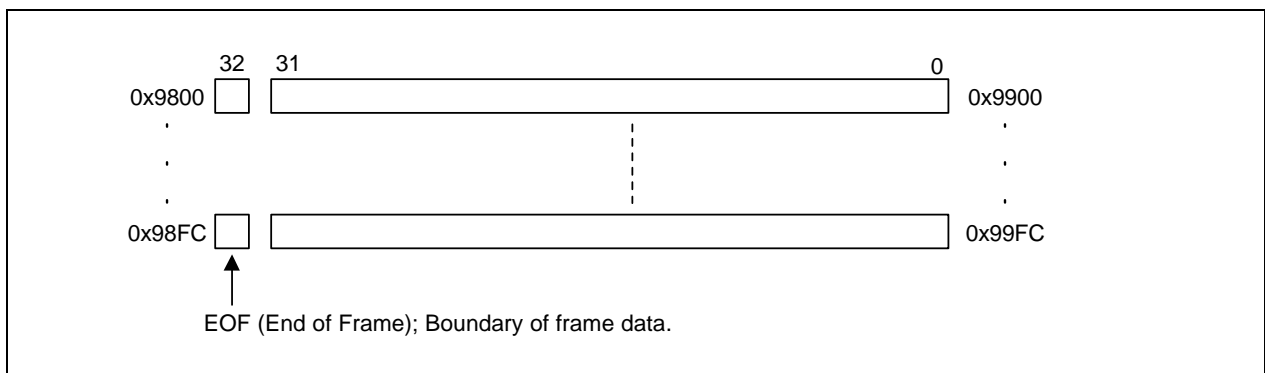
Figure 7-11. End of Frame Bit
