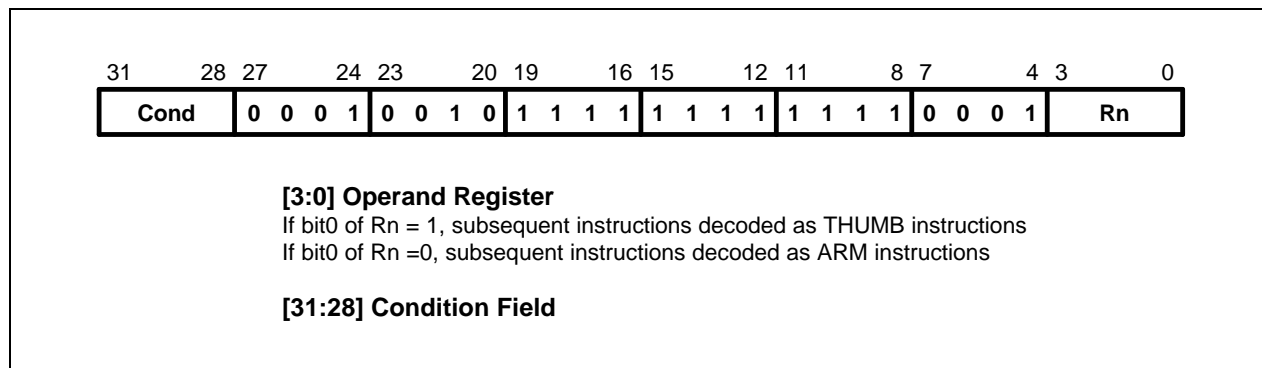
Figure 3-2. Branch and Exchange Instructions
