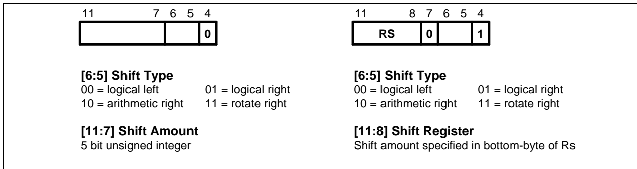
Figure 3-5. ARM Shift Operations
