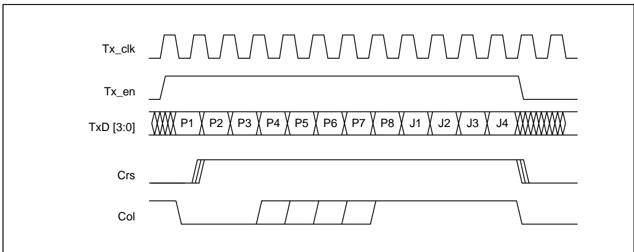
Figure 7-20. Timing for Transmit with Collision in Preamble
