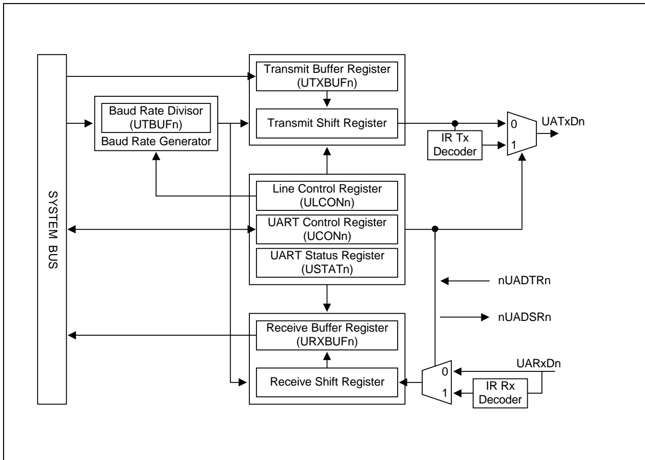
Figure 10-1. Serial I/O Block Diagram
