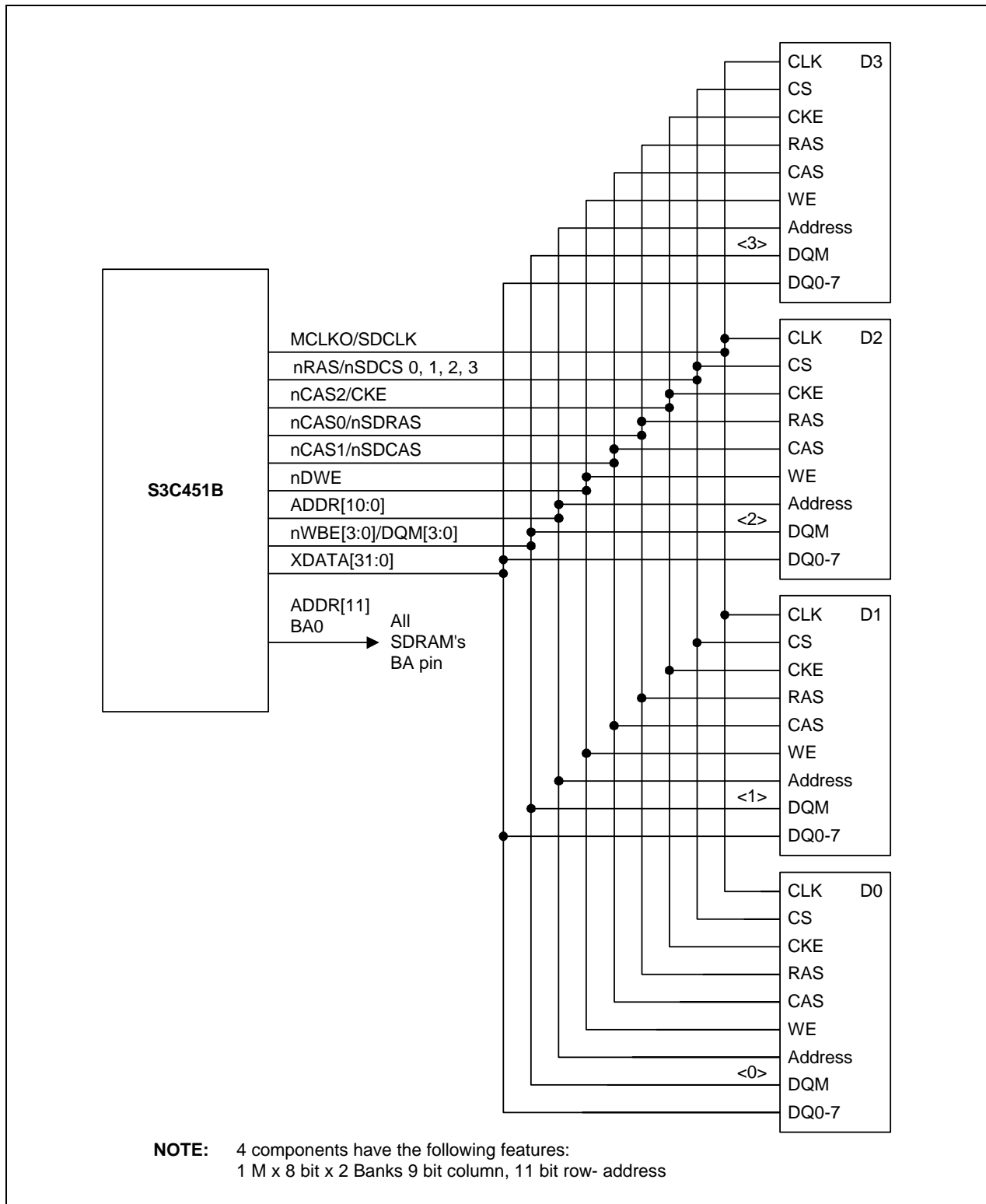
Figure 4-36. SDRAM Application Example
