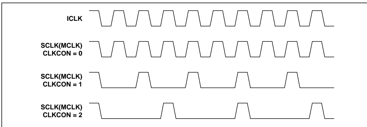
Figure 4-9. Divided System Clocks Timing Diagram
