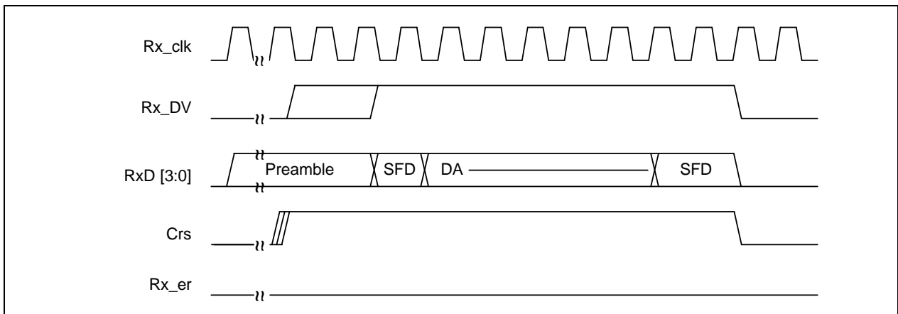
Figure 7-22. Receiving Frame without Error
