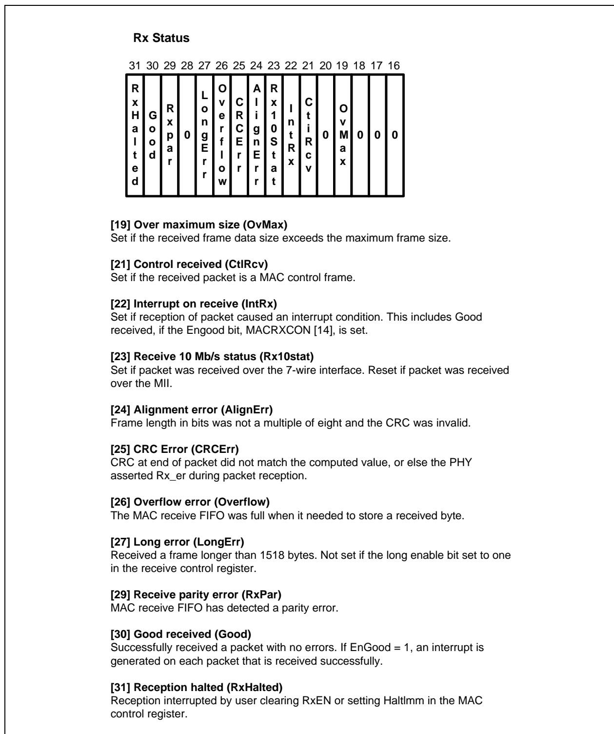
Figure 7-8. Rx Descriptor Status Bits
