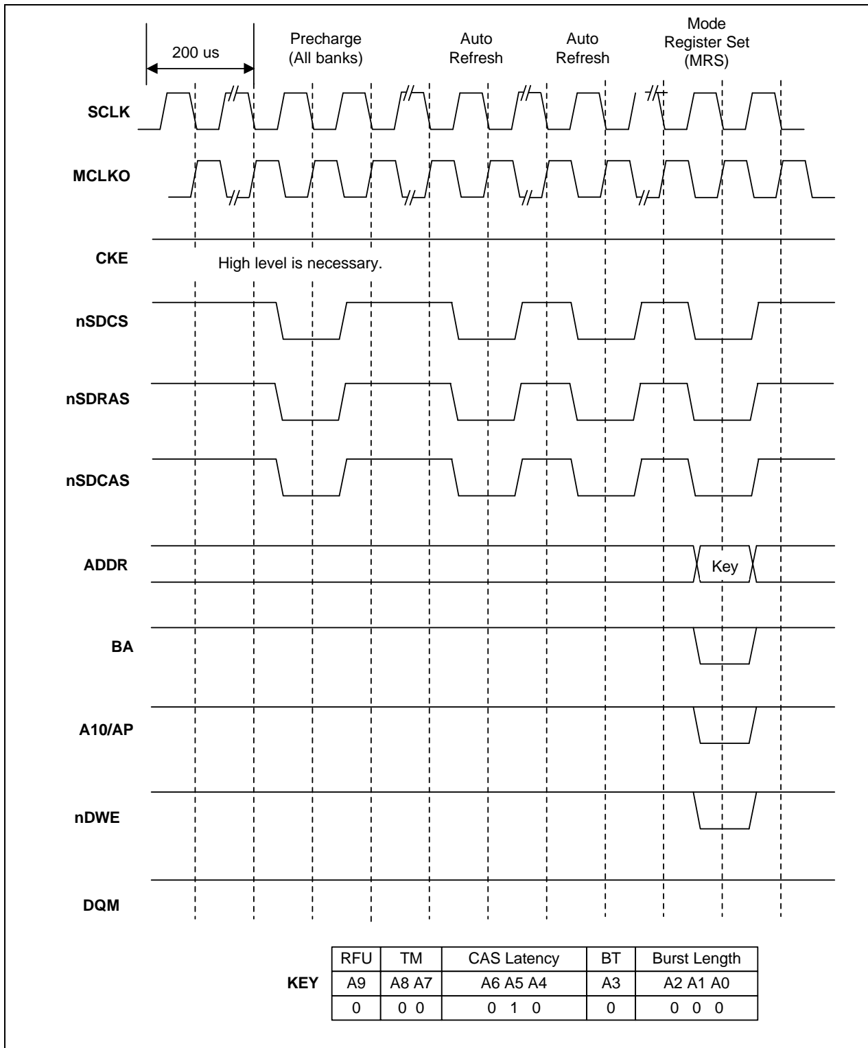
Figure 4-34. SDRAM Power-up Sequence
