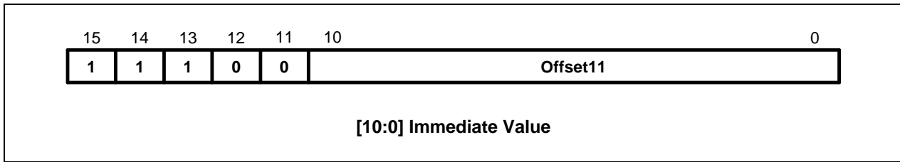
Figure 3-47. Format 18
