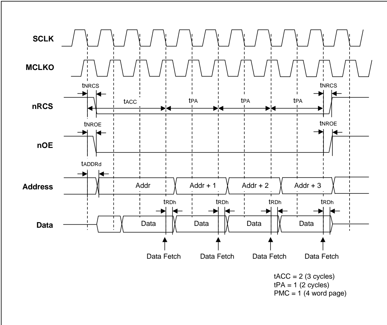
Figure 4-20. ROM/SRAM/Flash Page Read Access Timing
