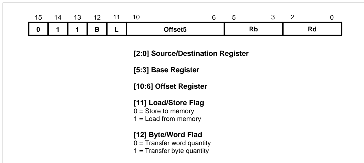
Figure 3-38. Format 9
