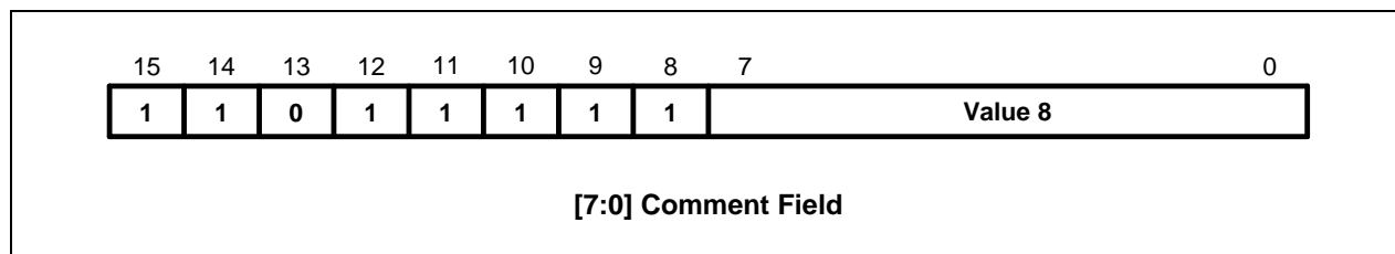
Figure 3-46. Format 17
