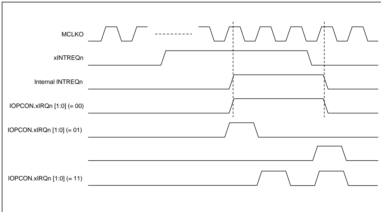
Figure 12-5. External Interrupt Request Timing (Active High)
