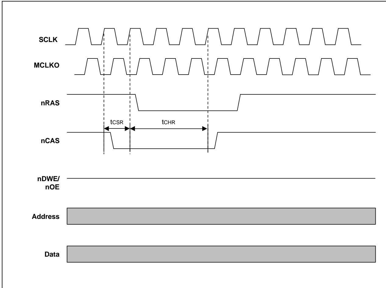
Figure 4-39. EDO/FP DRAM Refresh Timing
