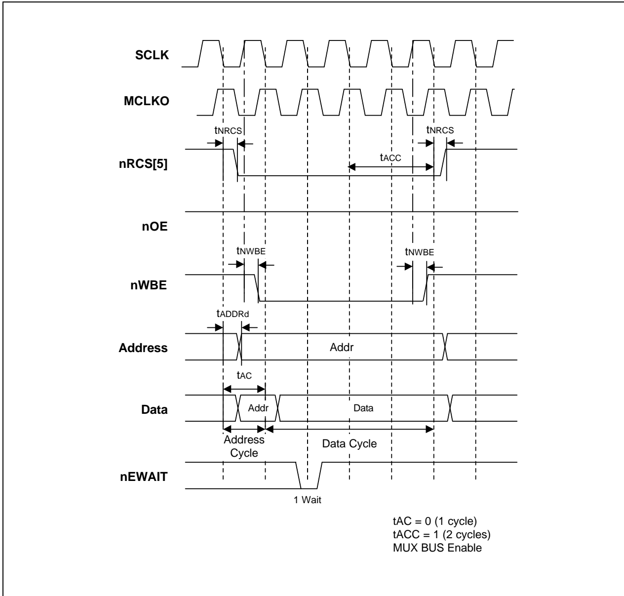
Figure 4-27. ROM/SRAM/FLASH Bank 5 Write Timing with nEWAIT Access Timing
