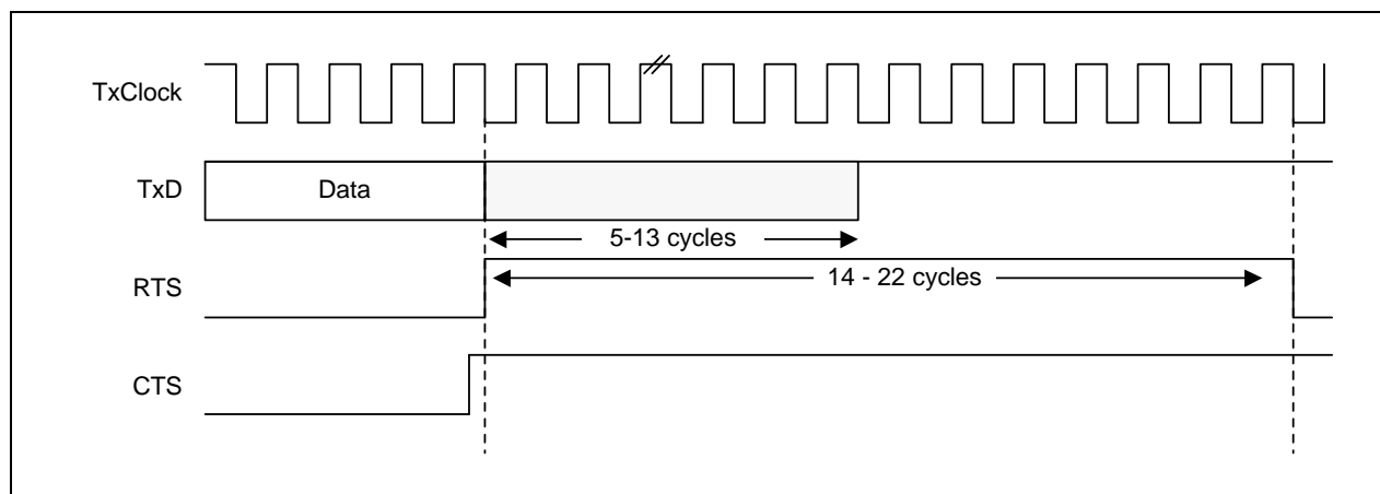
Figure 8-8. CTS Lost during Transmission
