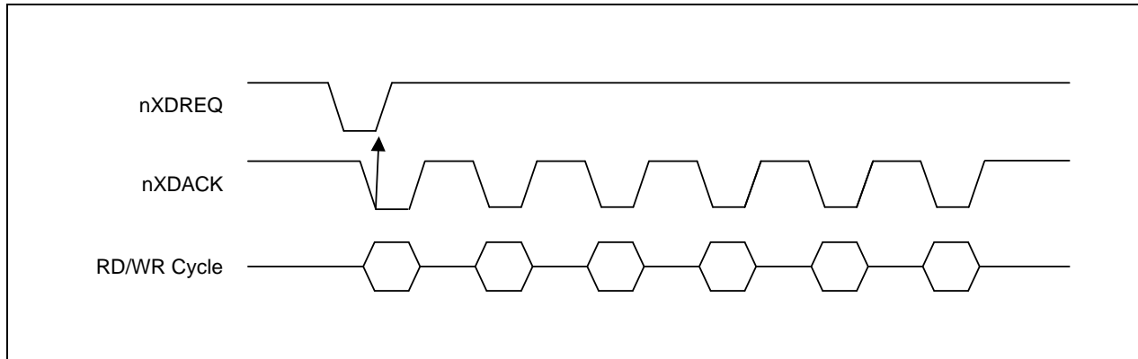
Figure 9-6. External DMA Requests (Block Mode)
