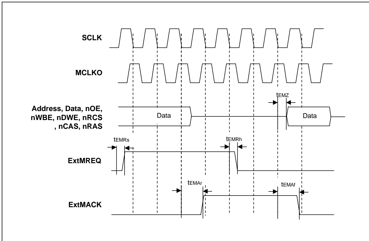
Figure 4-5. External Bus Request Timing
