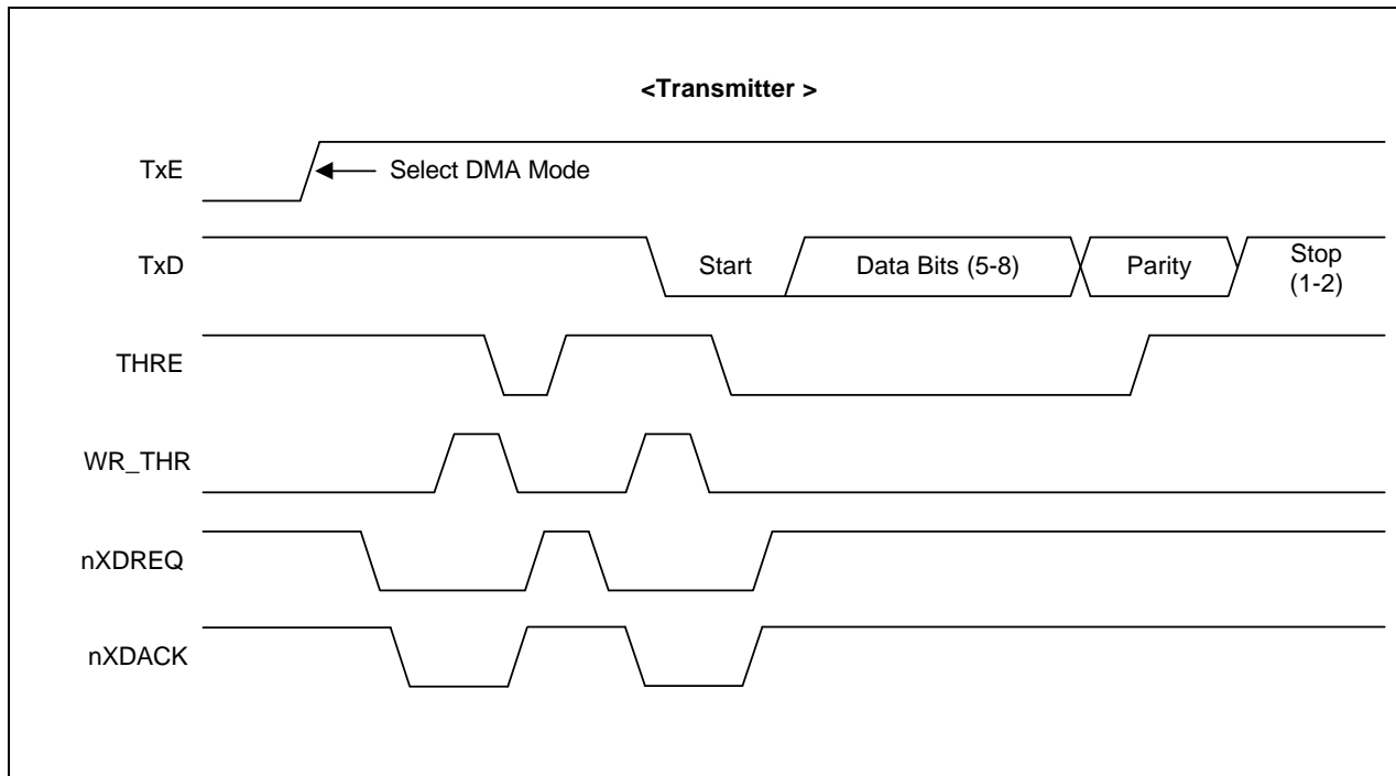
Figure 10-11. DMA-Based Serial I/O Timing Diagram (Tx Only)
