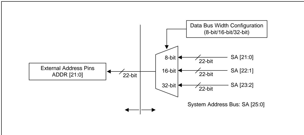
Figure 4-3. External Address Bus Diagram
