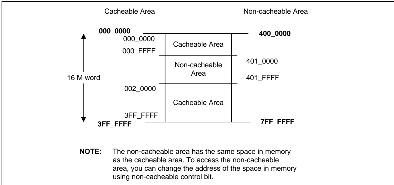
Figure 5-3. Non-Cacheable Area Control
