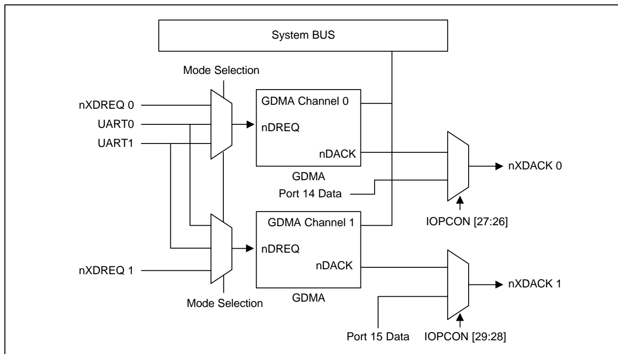
Figure 9-1. GDMA Controller Block Diagram
