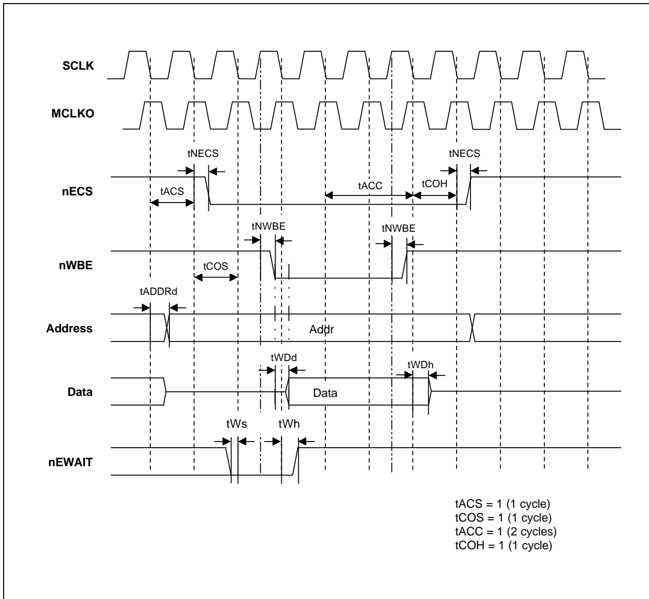
Figure 4-16. External I/O Write Timing with nEWAIT
