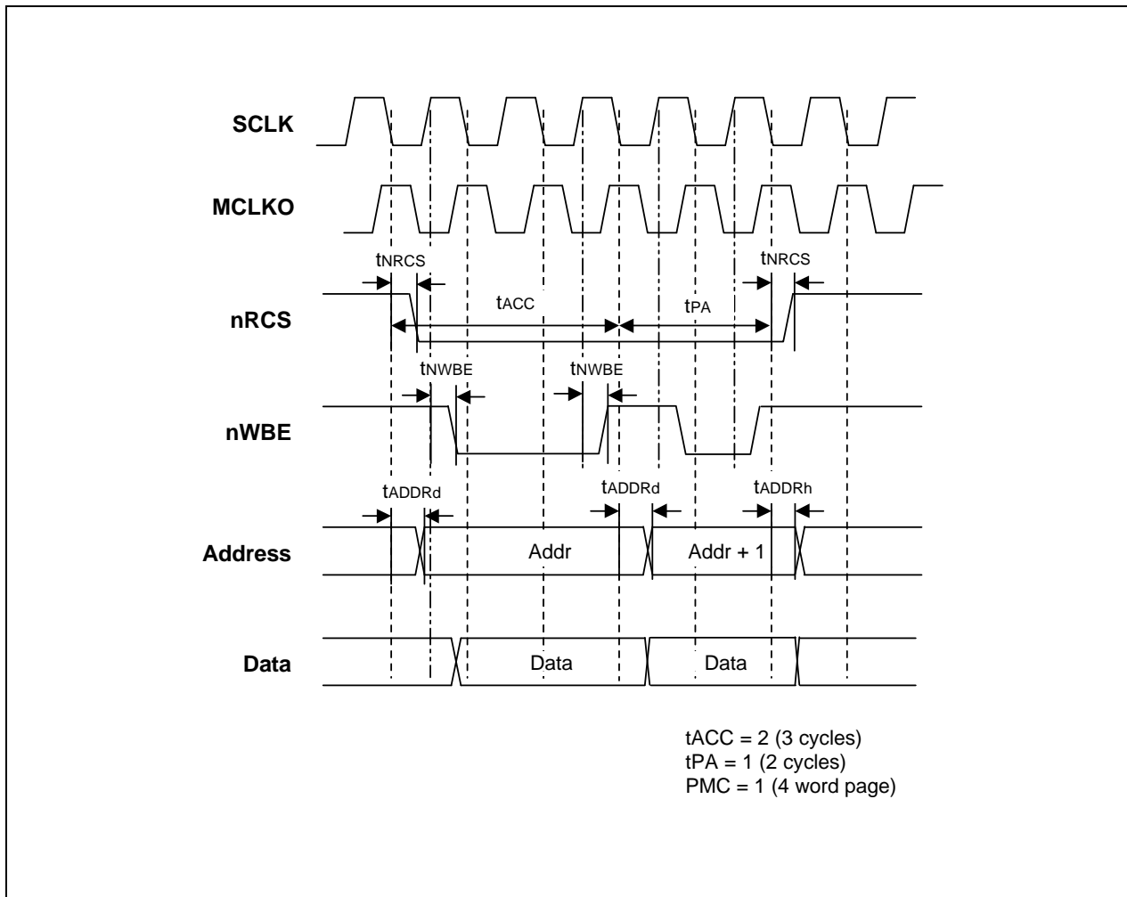
Figure 4-22. ROM/SRAM/Flash Page Write Access Timing
