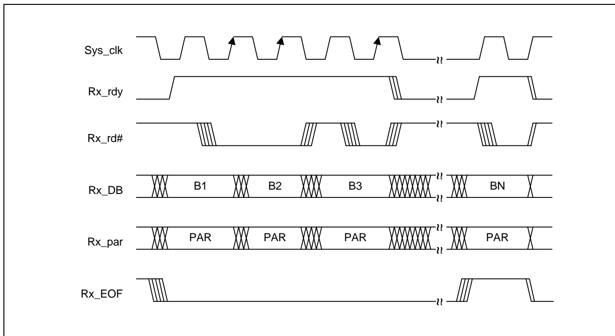
Figure 7-21. BDI Receive Data Timing
