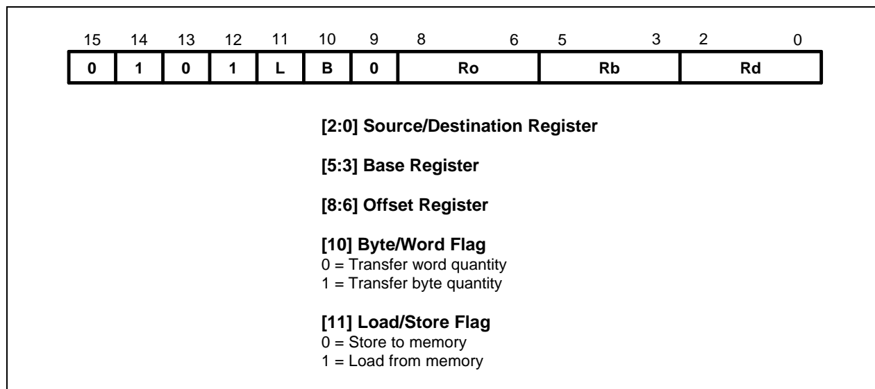
Figure 3-36. Format 7
