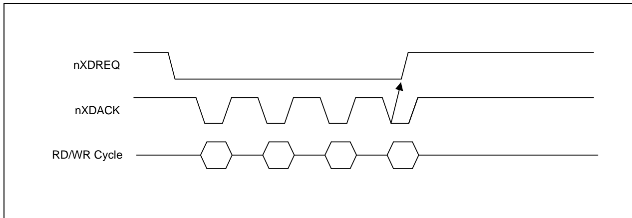
Figure 9-7. External DMA Requests (Demand Mode)
