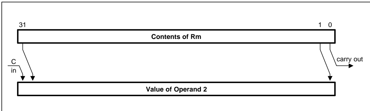
Figure 3-10. Rotate Right Extended
