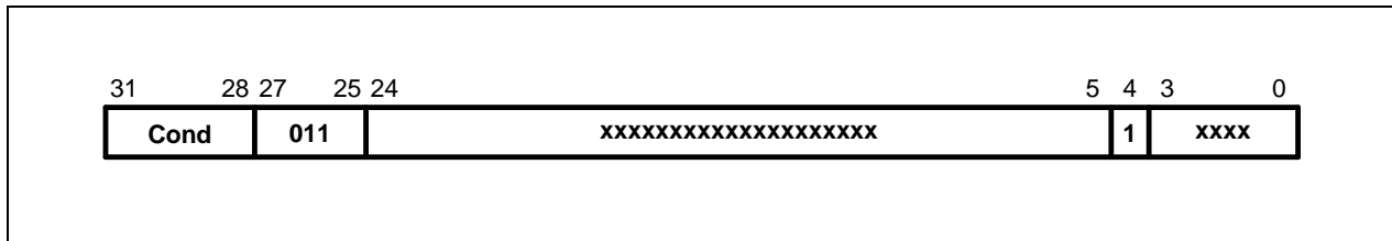
Figure 3-28. Undefined Instruction
