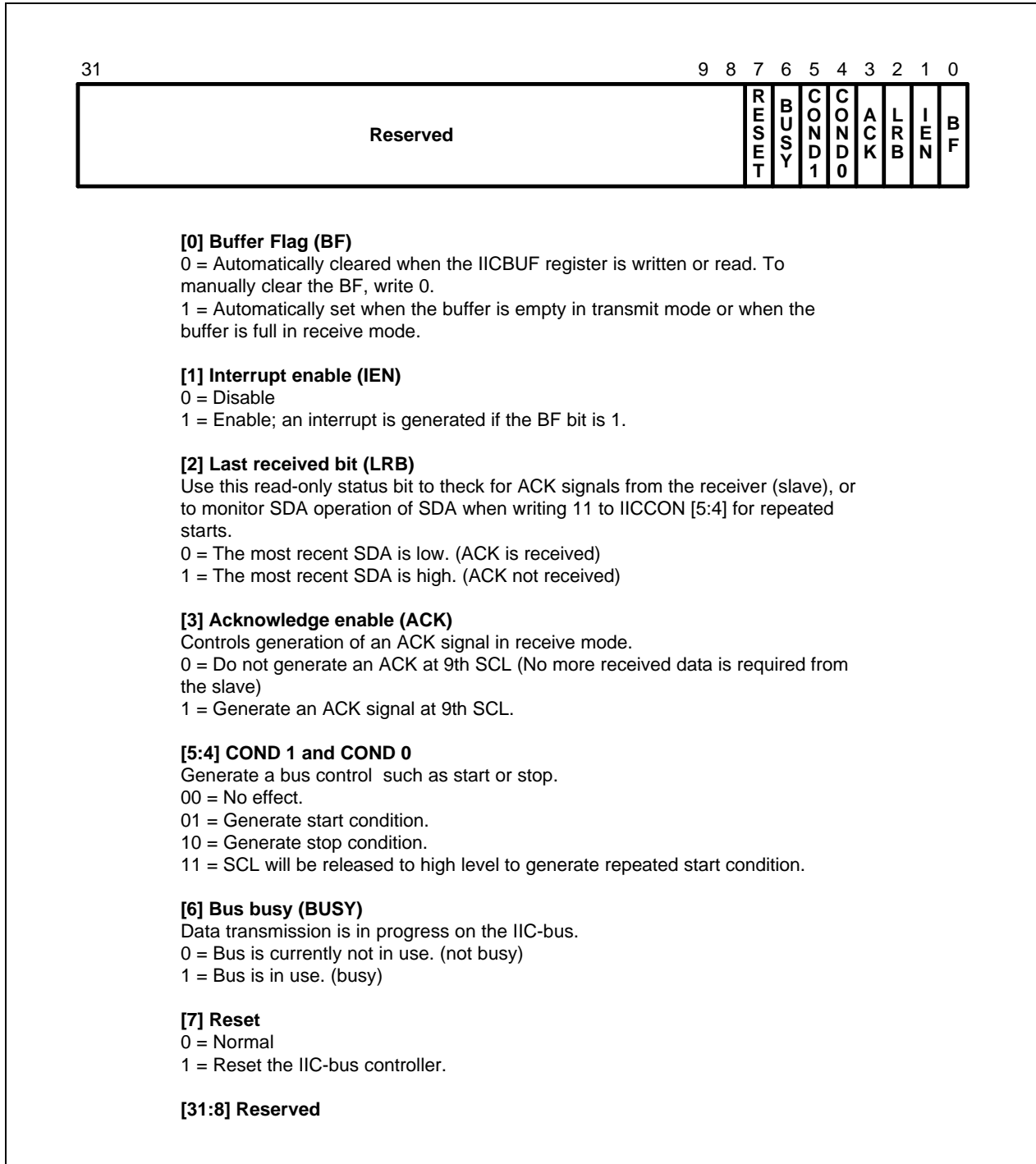
Figure 6-4. I 2 C Control Status Register
