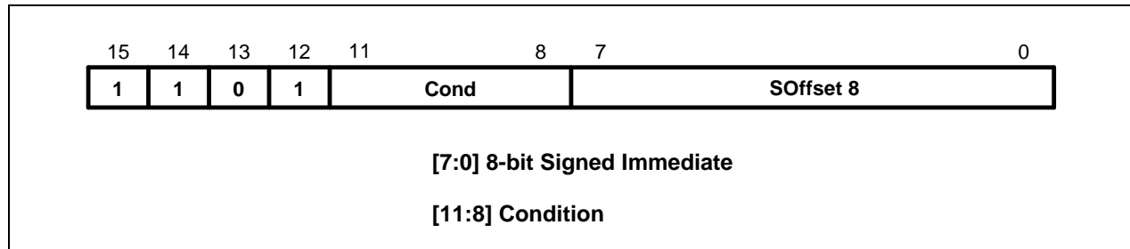
Figure 3-45. Format 16
