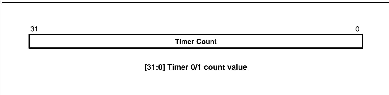
Figure 11-5. Timer Counter Registers (TCNT0, TCNT1)
