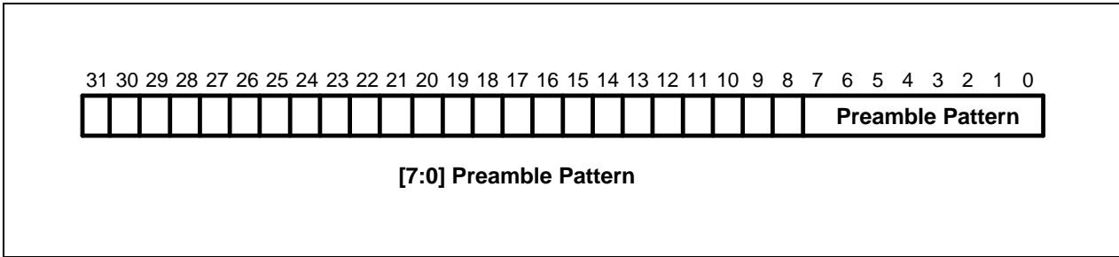
Figure 8-22. HDLC Preamble Constant Register
