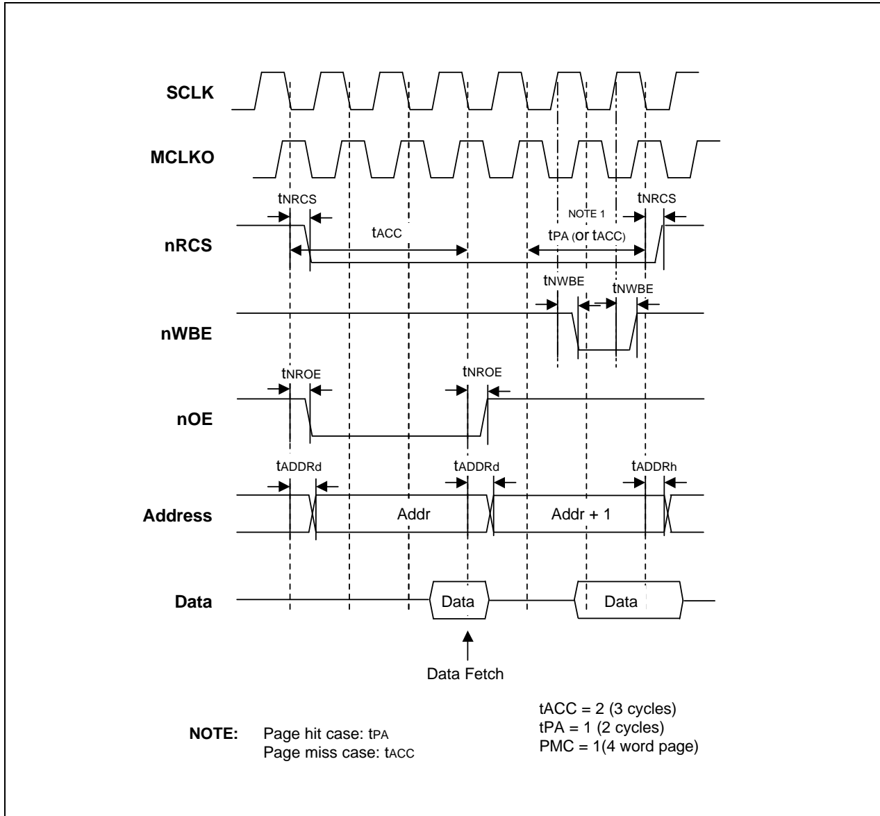
Figure 4-23. ROM/SRAM/Flash Read and Write Access Timing
