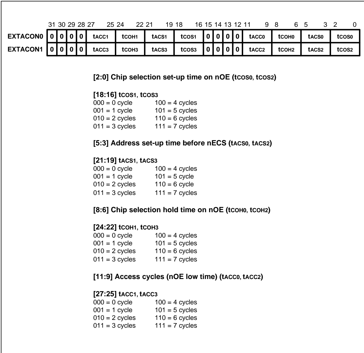
Figure 4-10. External I/O Access Control Registers (EXTACON0, EXTACON1)
