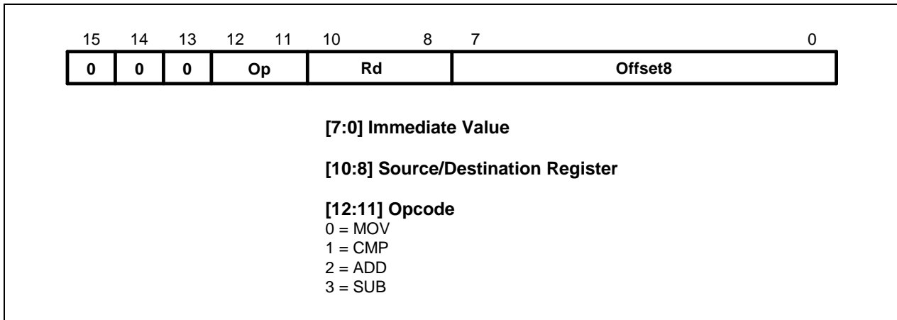
Figure 3-32. Format 3
