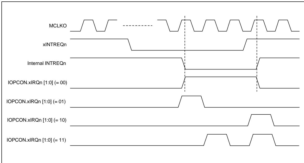
Figure 12-6. External Interrupt Request Timing (Active Low)
