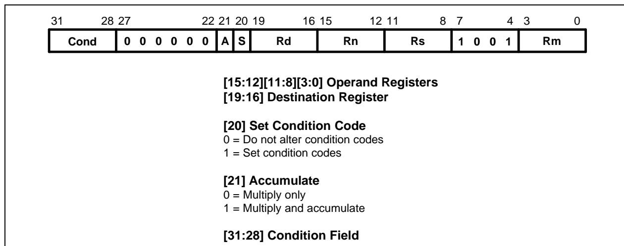
Figure 3-12. Multiply Instructions
