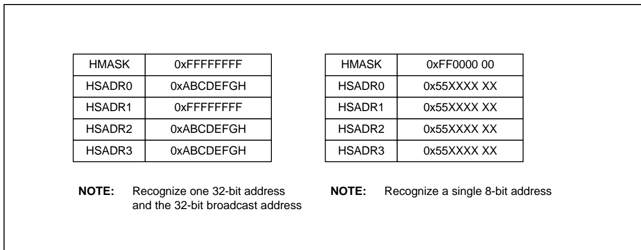
Figure 8-23. Address Recognition
