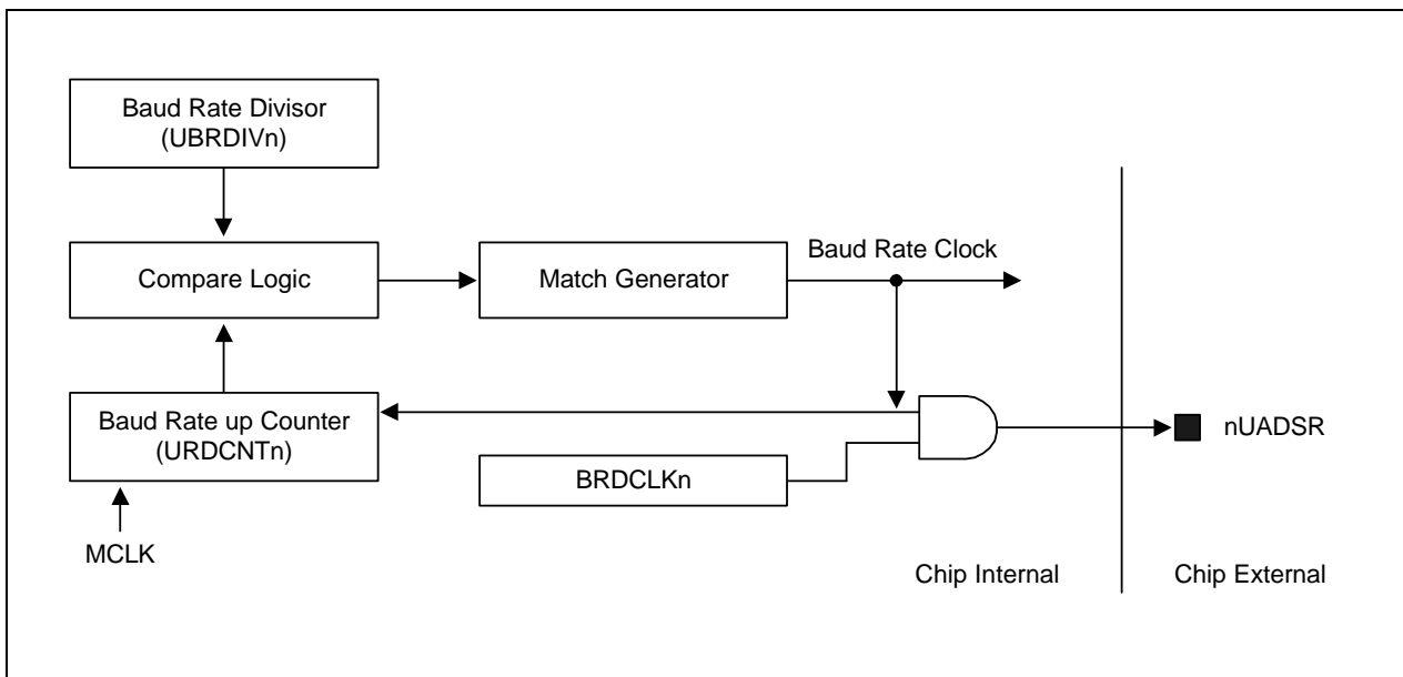
Figure 10-8. UART Baud Rate Clock Test Scheme
