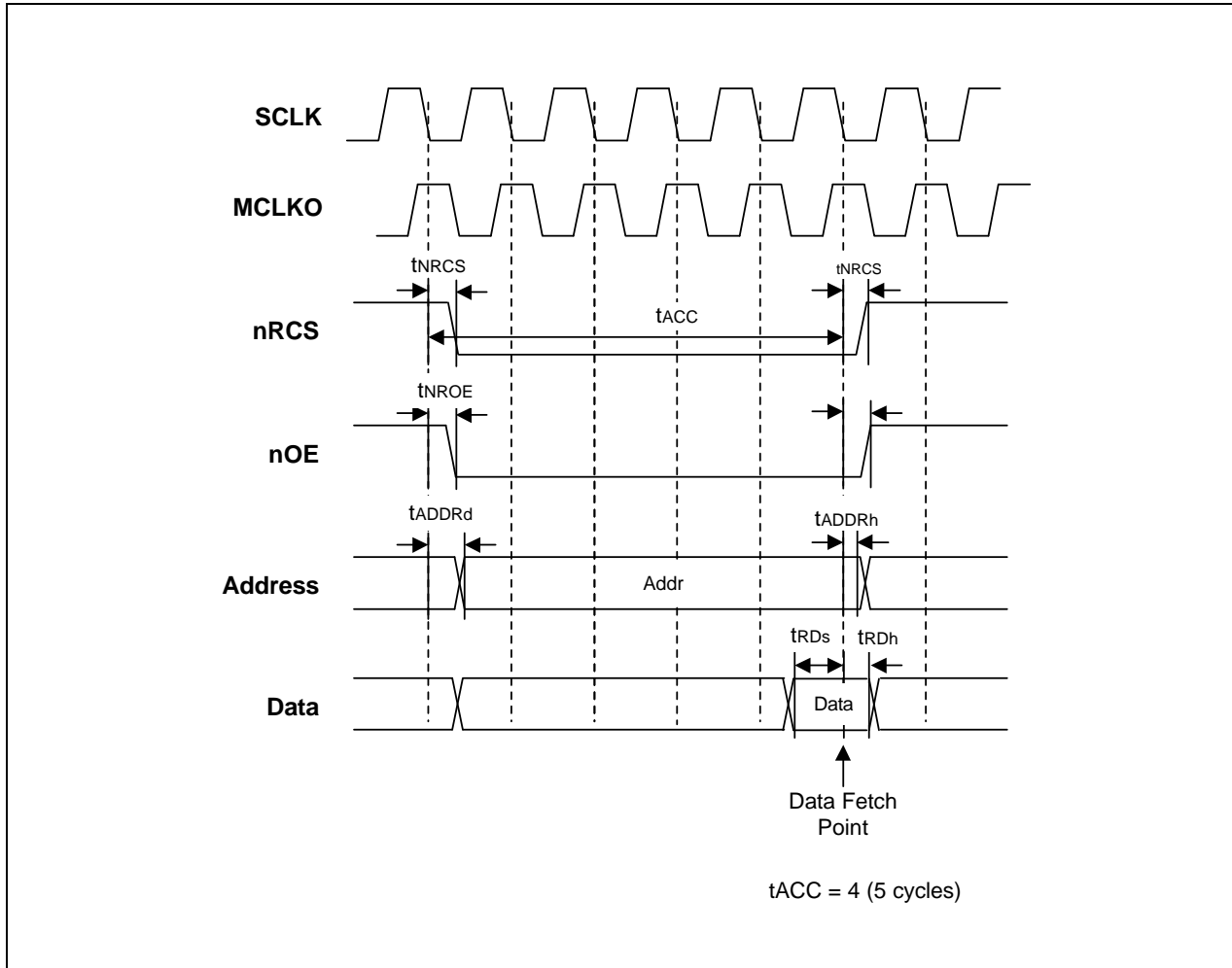
Figure 4-19. ROM/SRAM/Flash Read Access Timing
