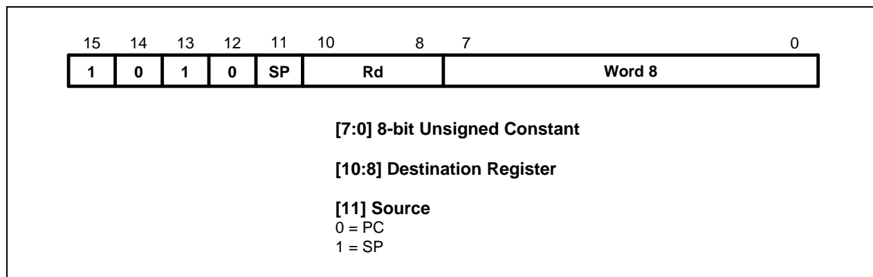
Figure 3-41. Format 12
