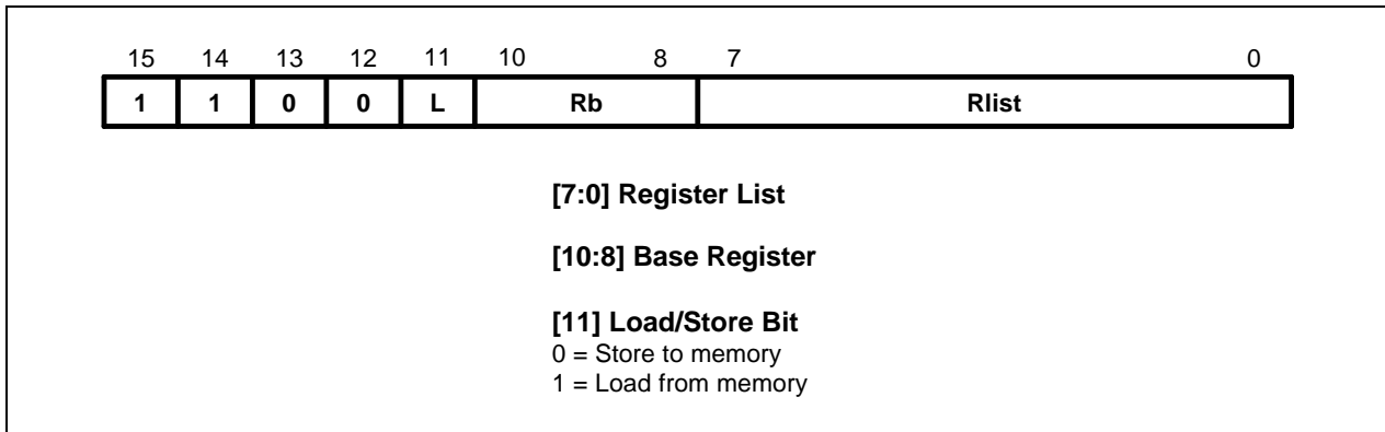
Figure 3-44. Format 15
