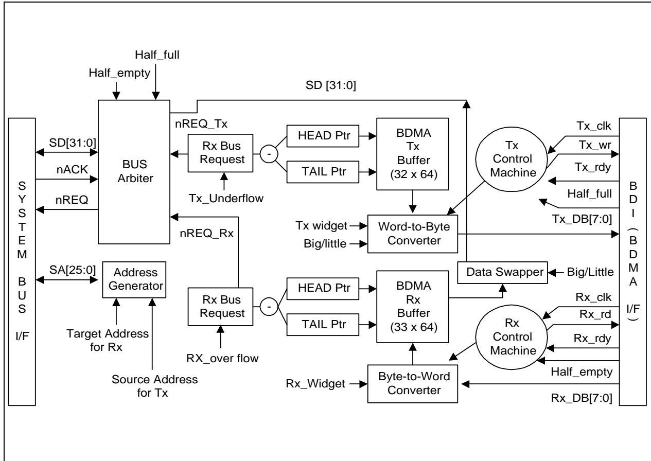
Figure 7-5. BDMA Control Blocks
