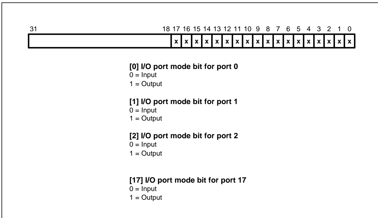
Figure 12-2. I/O Port Mode Register (IOPMOD)
