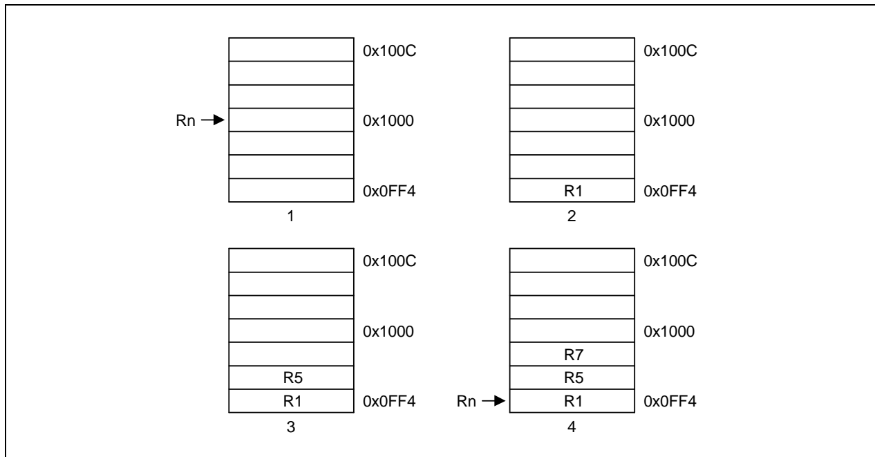
Figure 3-22. Pre-Decrement Addressing
