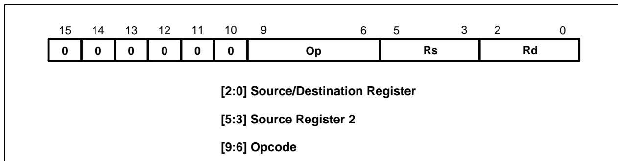
Figure 3-33. Format 4
