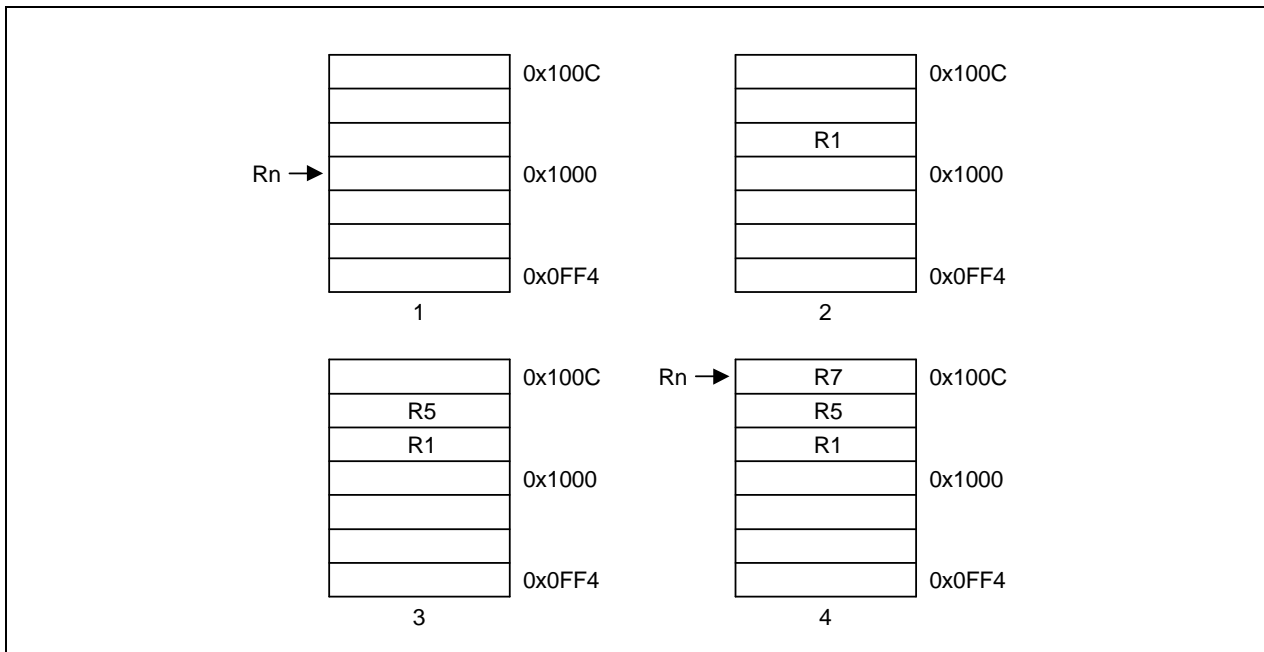
Figure 3-20. Pre-Increment Addressing
