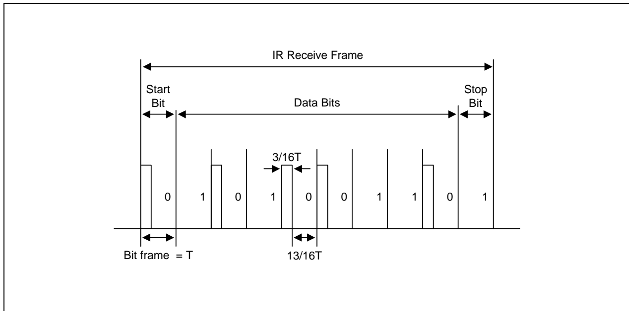
Figure 10-15. Infra-Red Receive Mode Frame Timing Diagram
