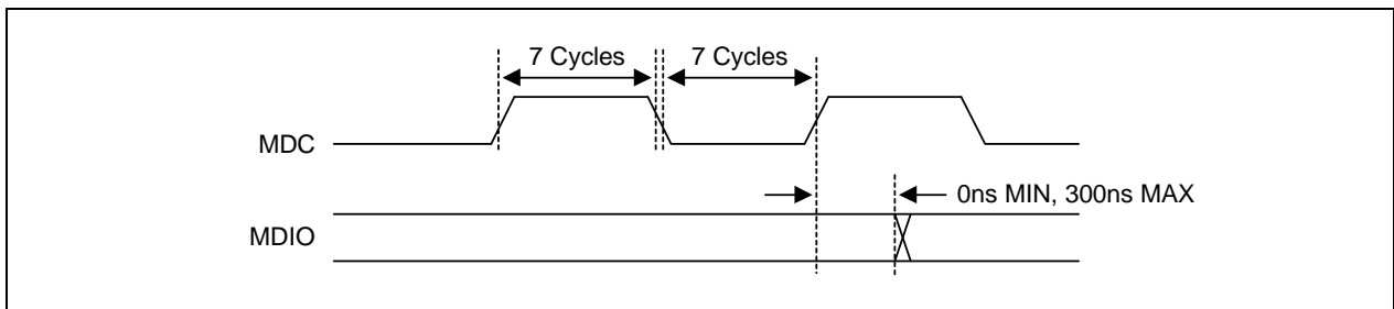
Figure 7-27. MDIO Sourced by PHY
