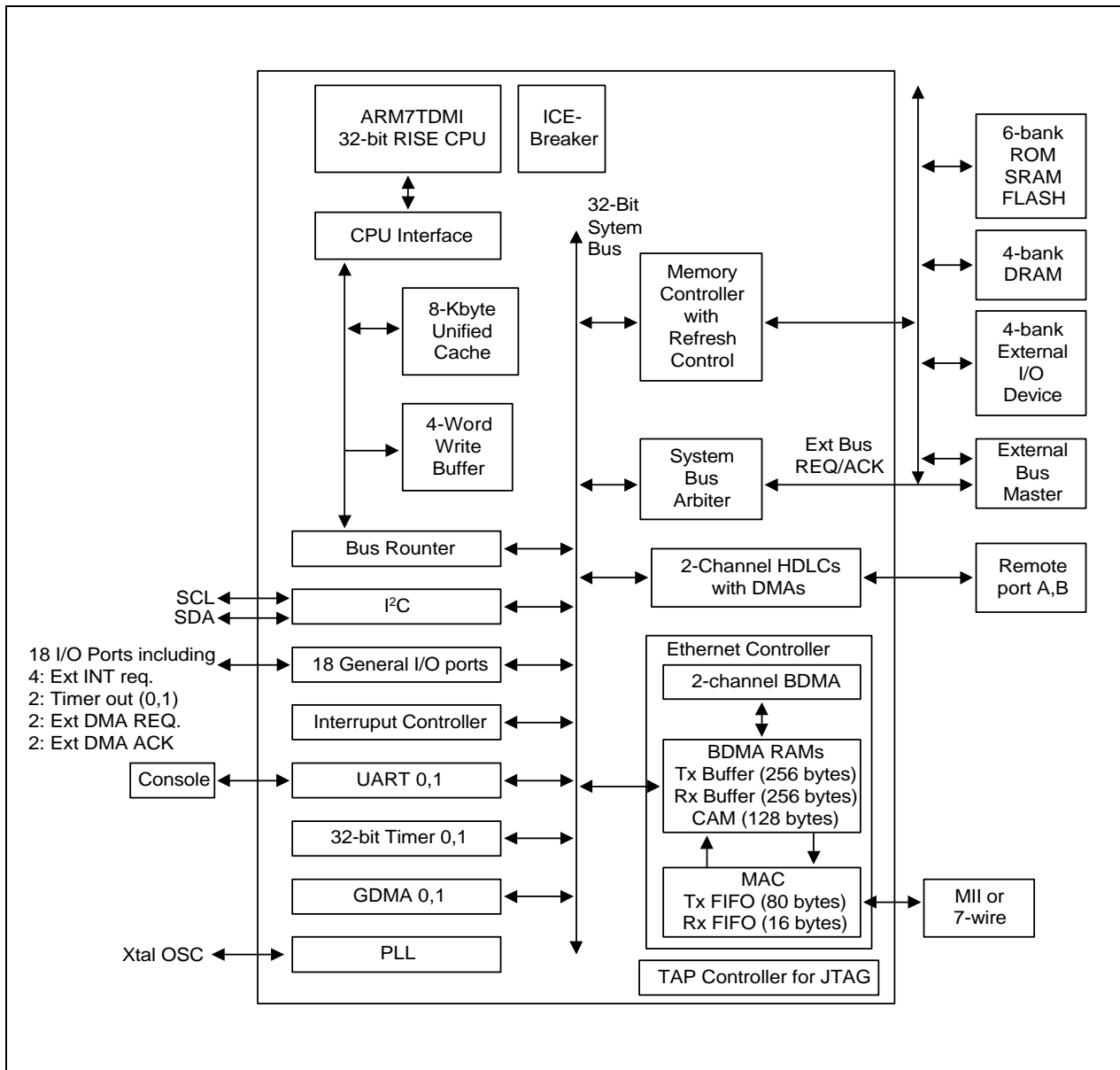
Figure 1-1. S3C4510B Block Diagram
