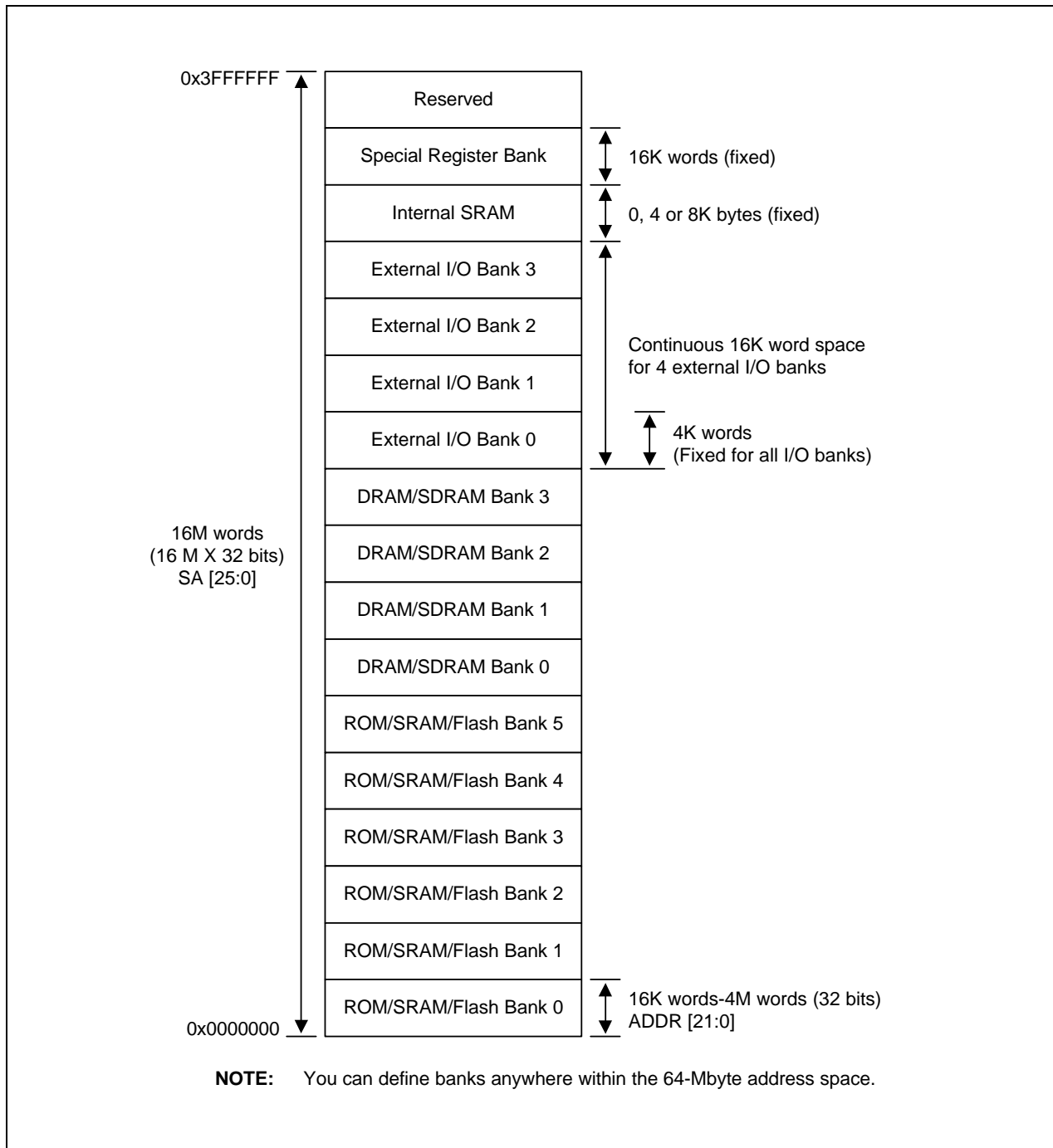
Figure 4-1. S3C4510B System Memory Map
