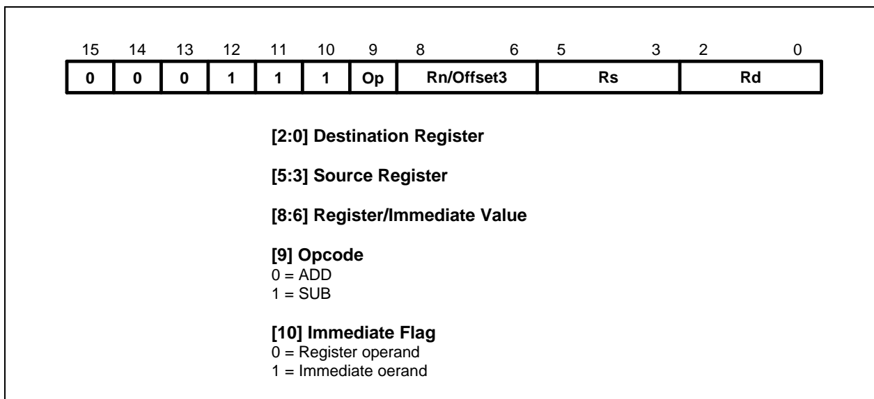
Figure 3-31. Format 2
