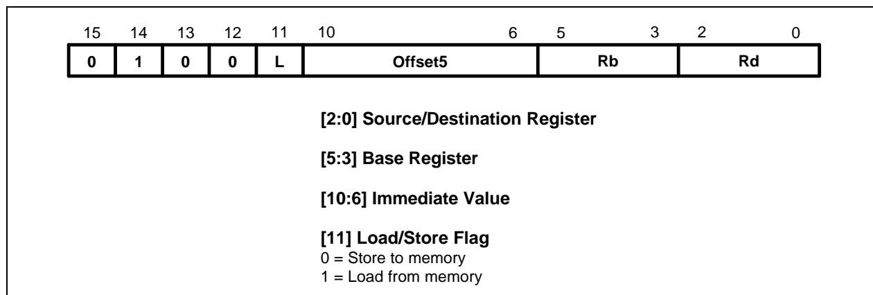
Figure 3-39. Format 10
