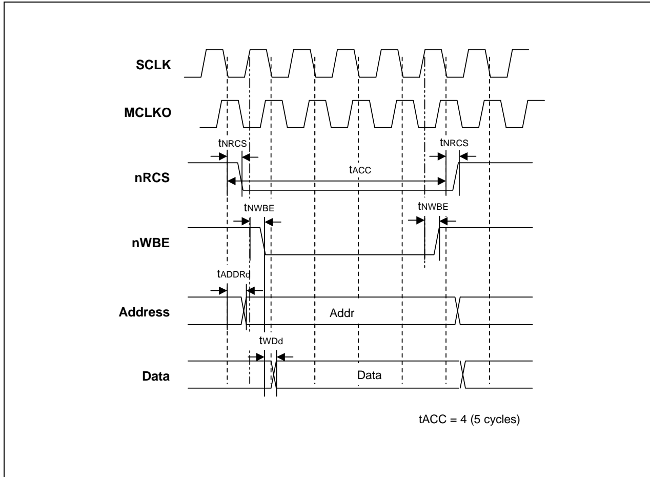
Figure 4-21. ROM/SRAM/Flash Write Access Timing
