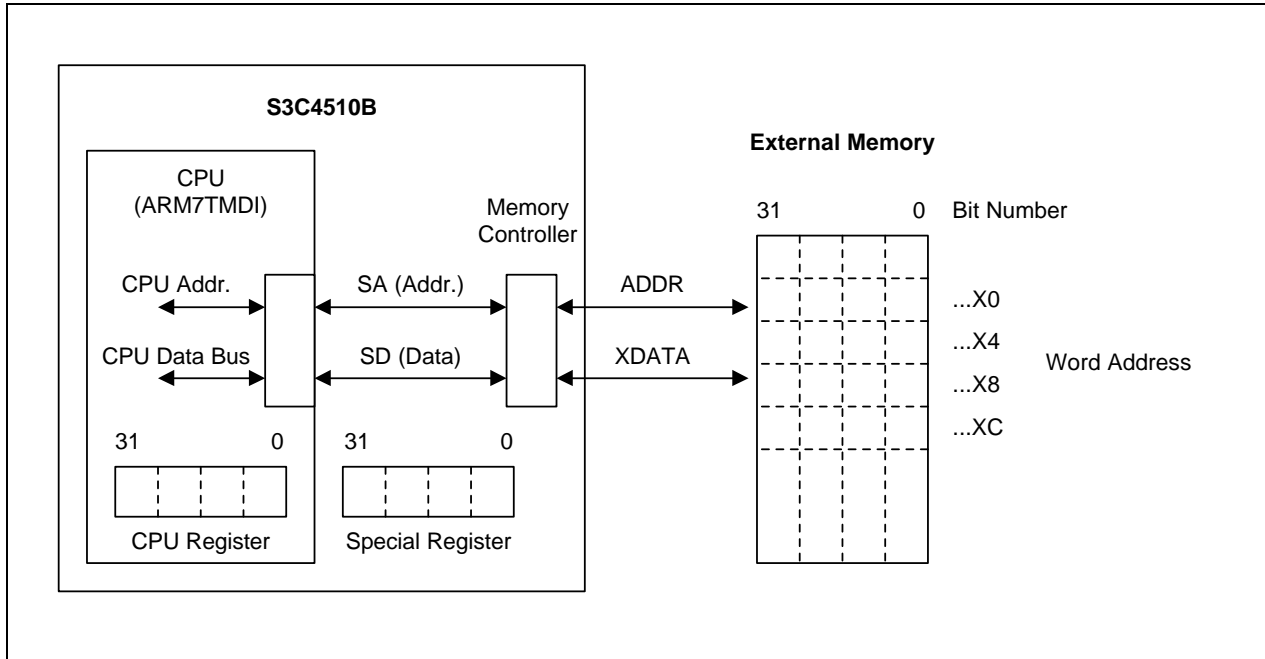
Figure 4-4. Data Bus Connection with External Memory
