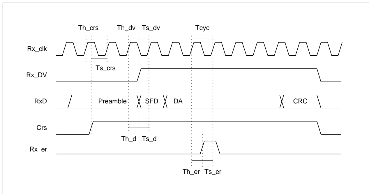
Figure 7-28. Rx Timing in 7 Wire Interface
