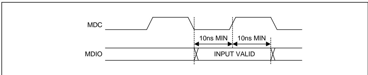
Figure 7-28. MDIO Sourced by STA
