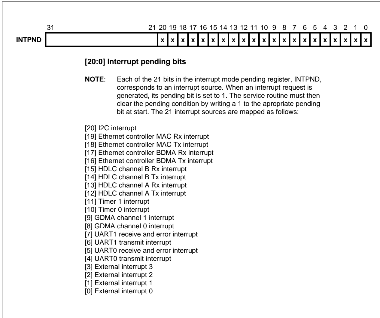
Figure 13-2. Interrupt Pending Register (INTPND)
