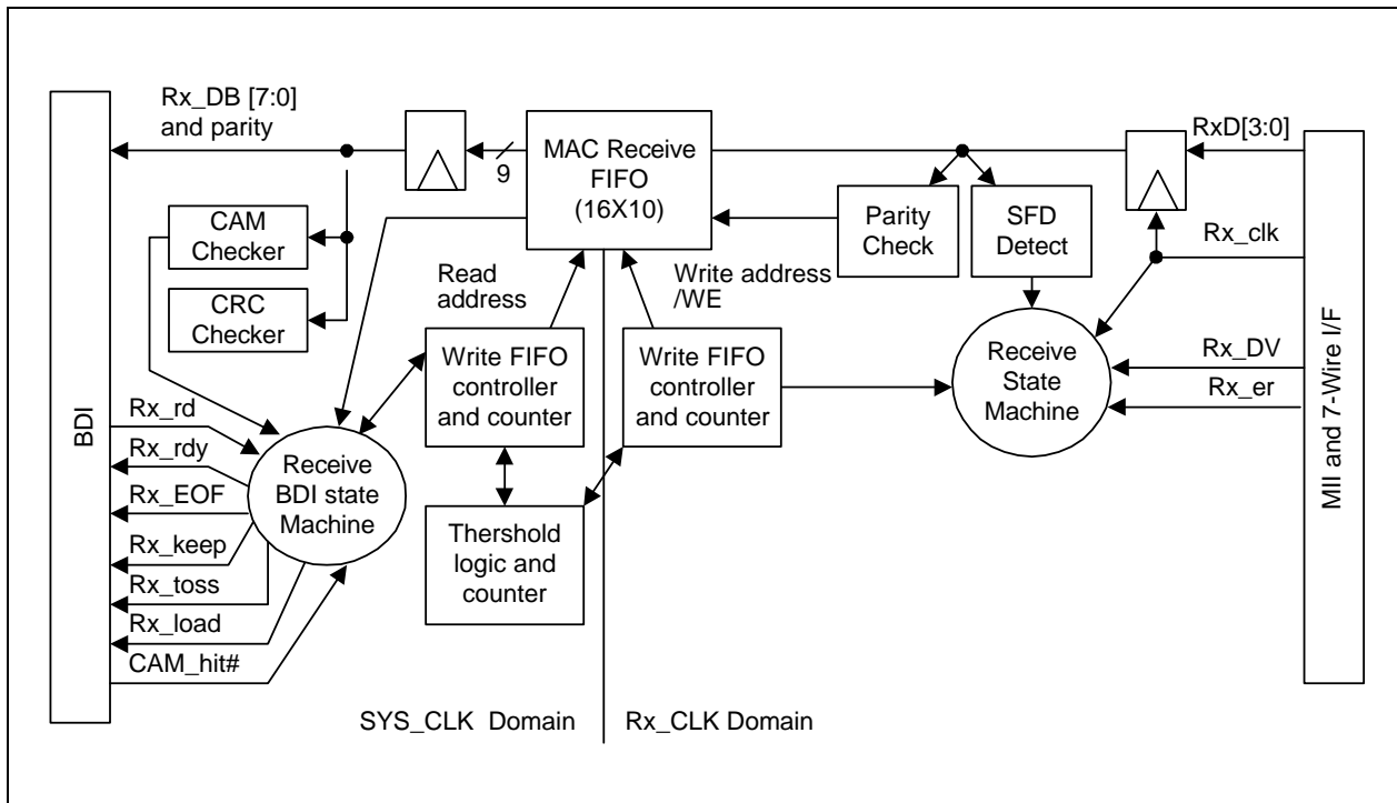
Figure 7-4. MAC Receive Function Blocks
