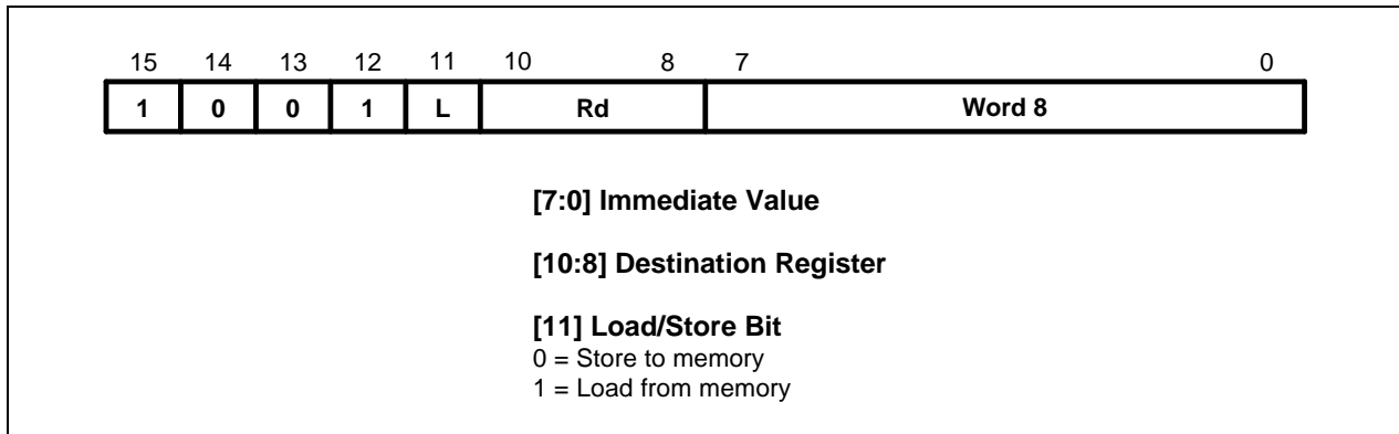
Figure 3-40. Format 11
