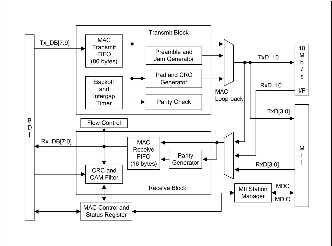
Figure 7-2. MAC Layer Flow Control Function Blocks
