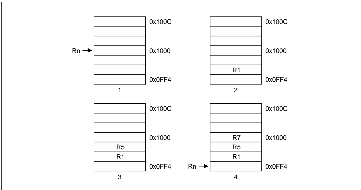
Figure 3-21. Post-Decrement Addressing
