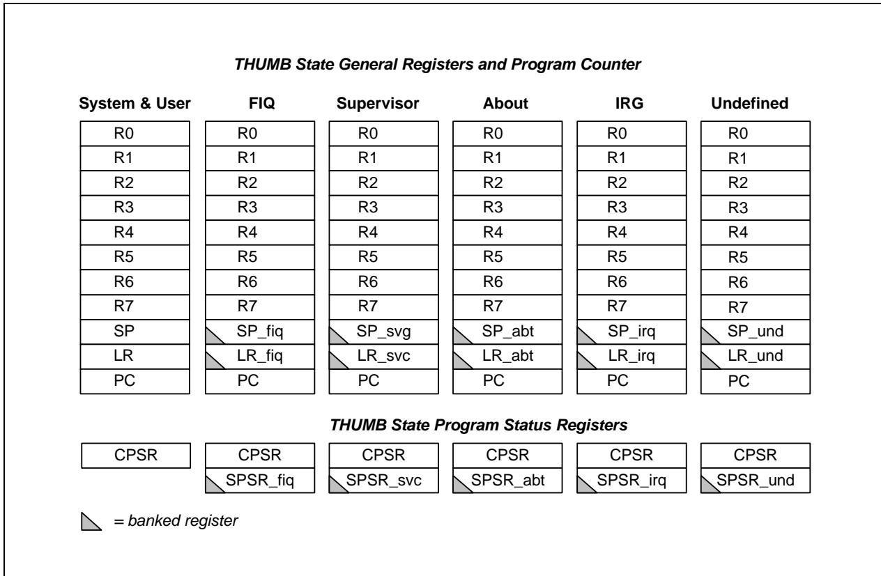
Figure 2-4. Register Organization in THUMB State
