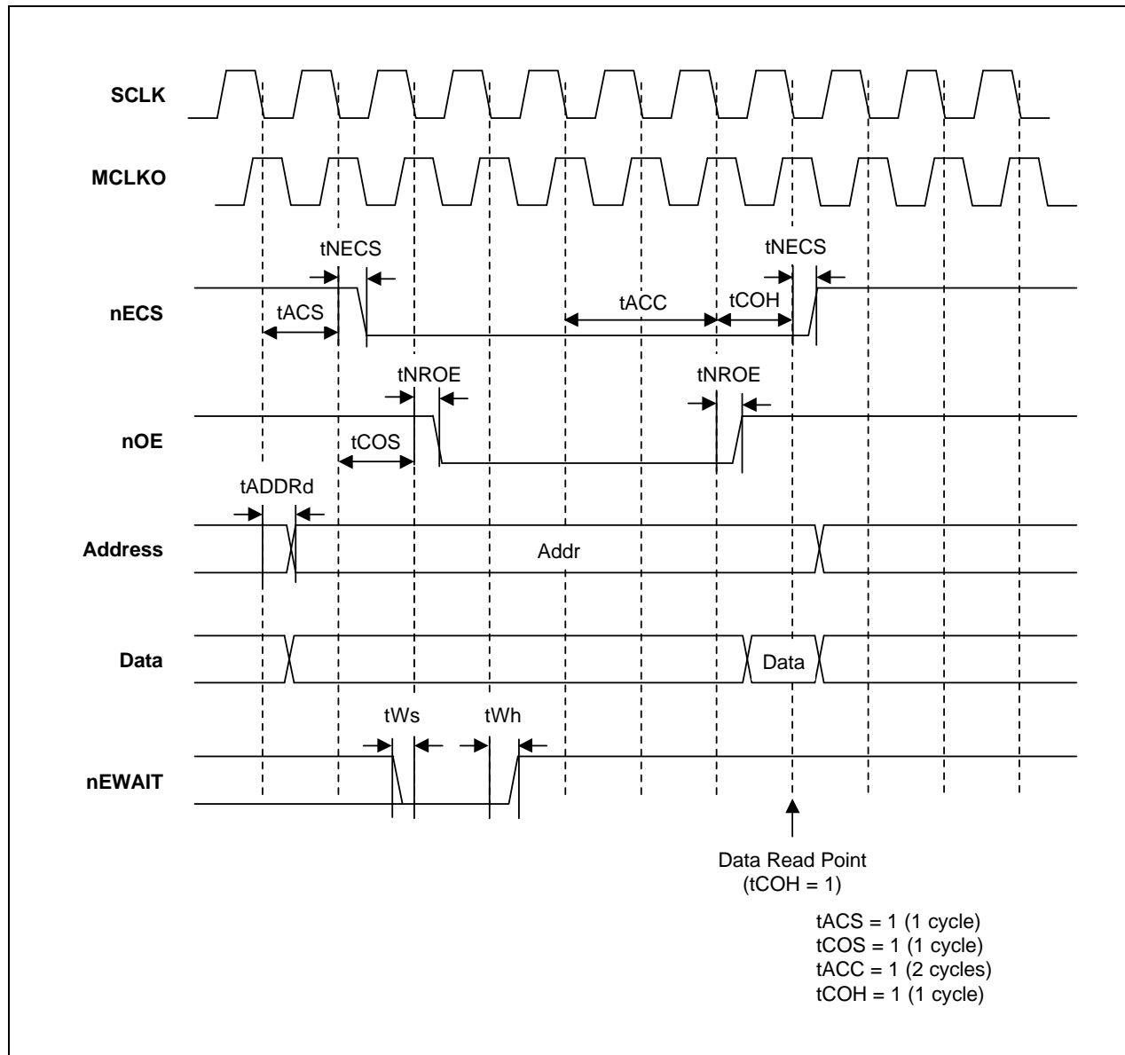
Figure 4-13. External I/O Read Timing with nEWAIT
