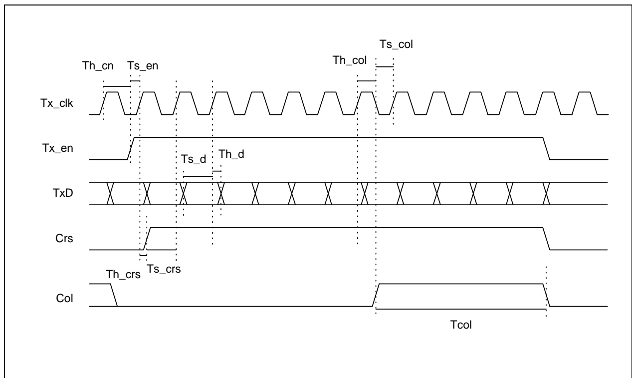
Figure 7-29. Tx Timing in 7 Wire Interface
