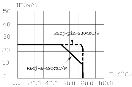
FIG.5 MAXIMUM FORWARD DC CURRENT VS AMBIENT TEMPERATURE . DERATING BASED ON T_{jmax}=95^{\circ}C
