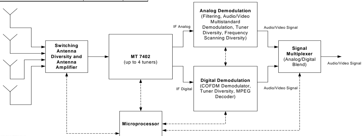
MT7402 Block Diagram
